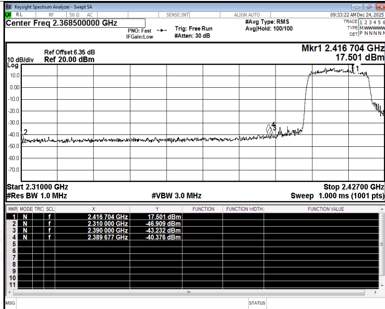
Restrict Band NVNT be20 2412MHz Ant2 Peak
