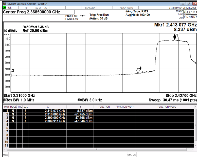
Restrict Band NVNT ax20 2412MHz Ant4 Average
