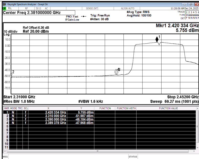
Restrict Band NVNT n40 2422MHz Ant4 Average
