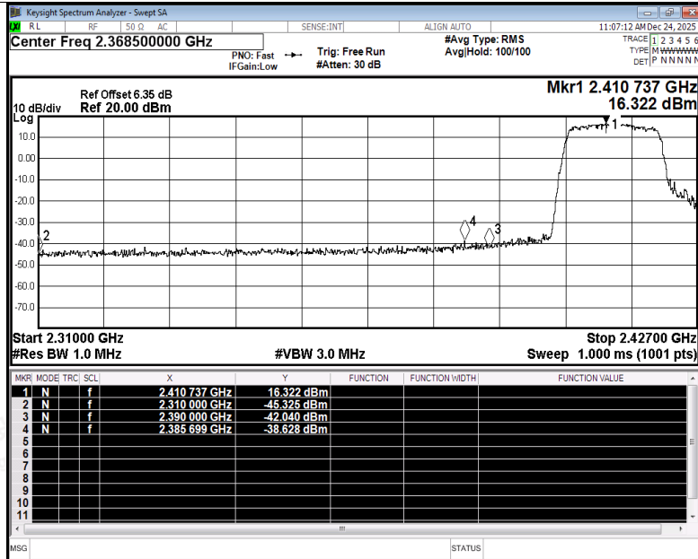
Restrict Band NVNT g 2412MHz Ant4 Peak
