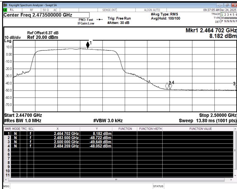
Restrict Band NVNT be20 2462MHz Ant2 Average
