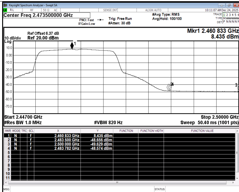
Restrict Band NVNT n20 2462MHz Ant3 Average
