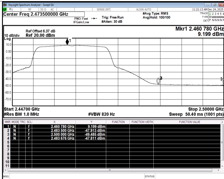
Restrict Band NVNT n20 2462MHz Ant4 Average
