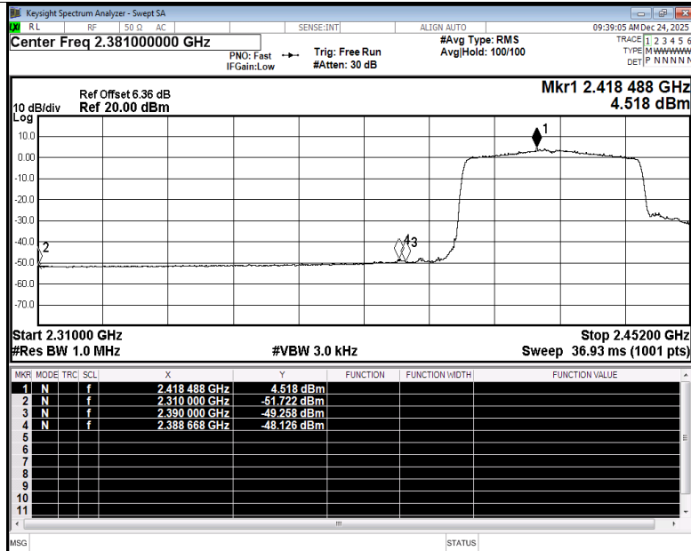
Restrict Band NVNT be40 2422MHz Ant2 Average
