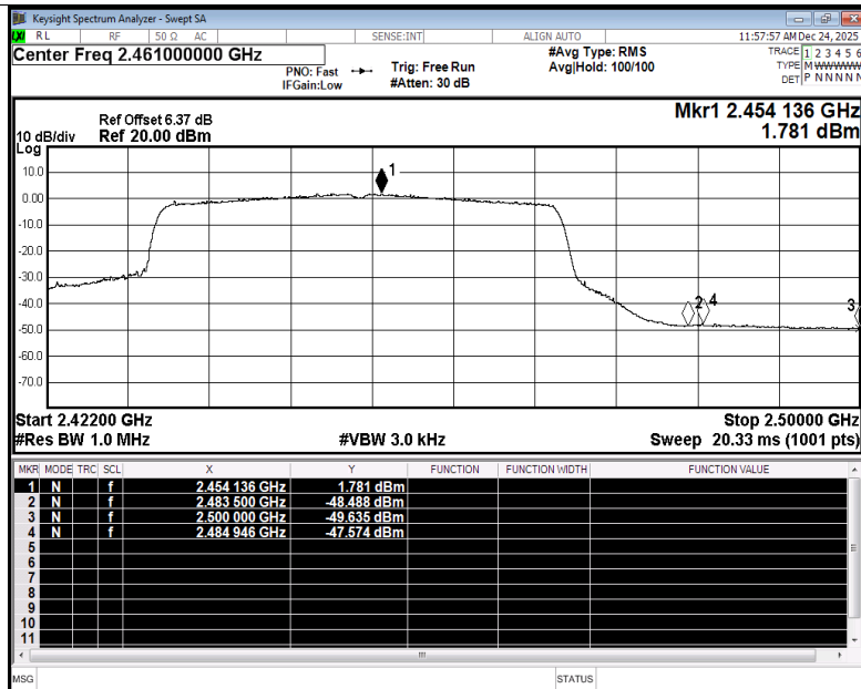
Restrict Band NVNT ax40 2452MHz Ant4 Average
