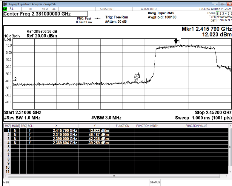
Restrict Band NVNT ax40 2422MHz Ant3 Peak
