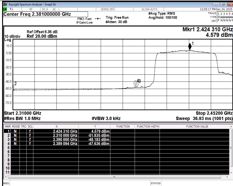
Restrict Band NVNT be40 2422MHz Ant4 Average
