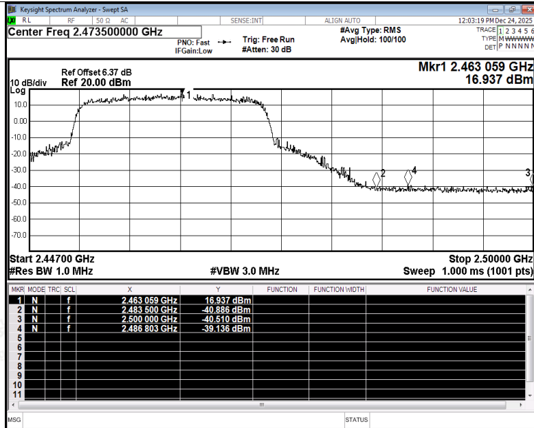
Restrict Band NVNT be20 2462MHz Ant4 Peak
