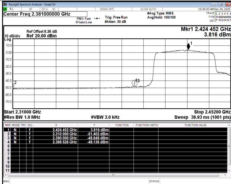
Restrict Band NVNT ax40 2422MHz Ant3 Average
