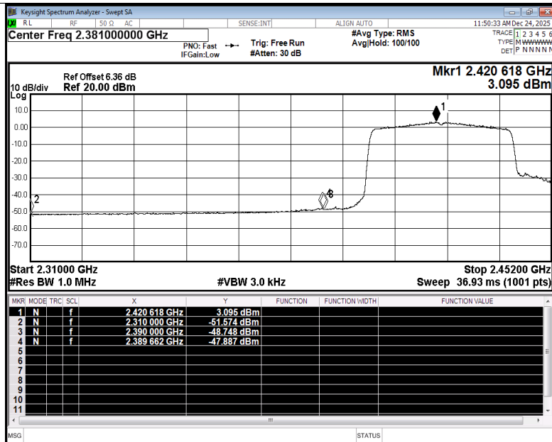
Restrict Band NVNT ax40 2422MHz Ant4 Average
