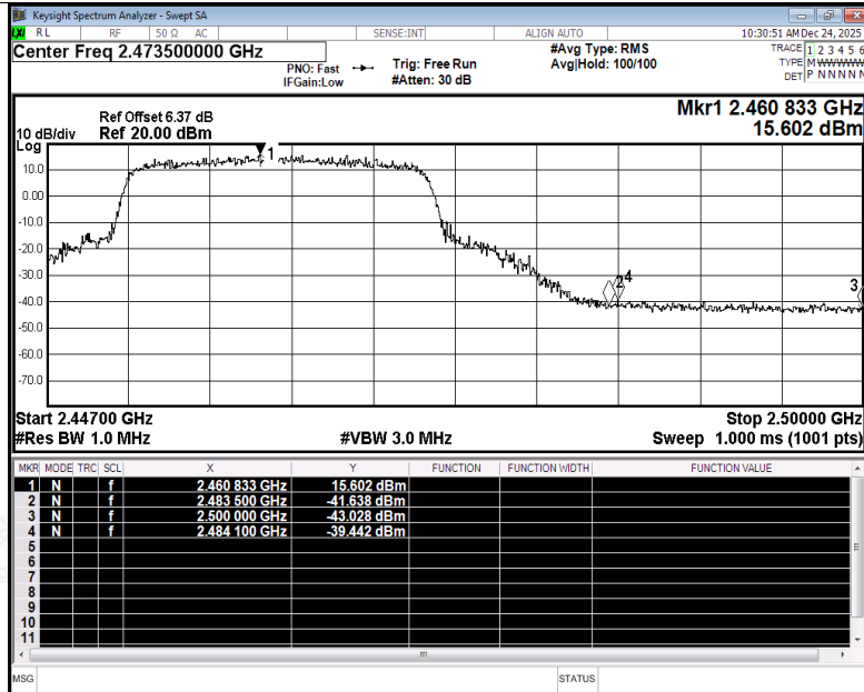
Restrict Band NVNT ax20 2462MHz Ant3 Peak
