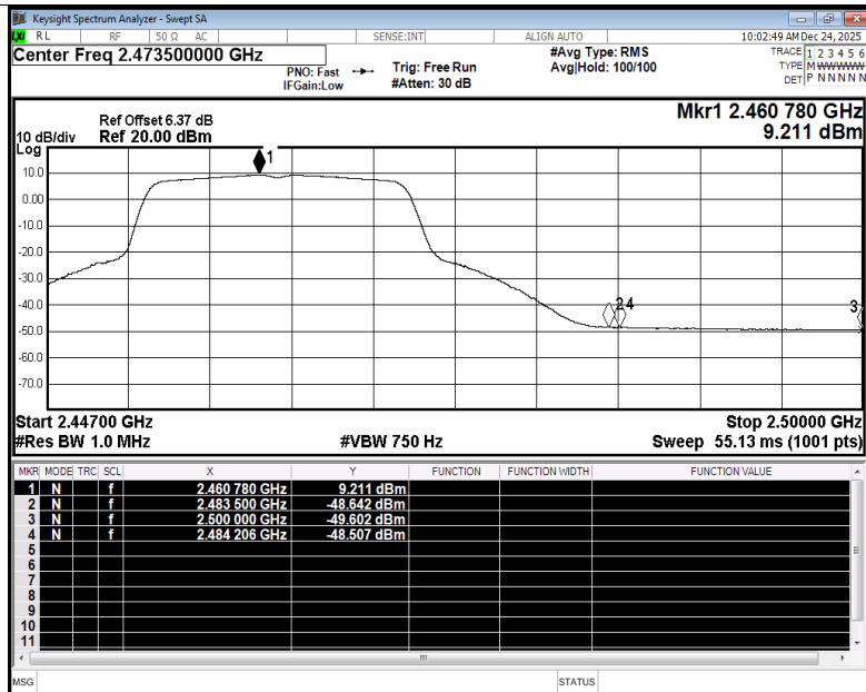
Restrict Band NVNT g 2462MHz Ant3 Average
