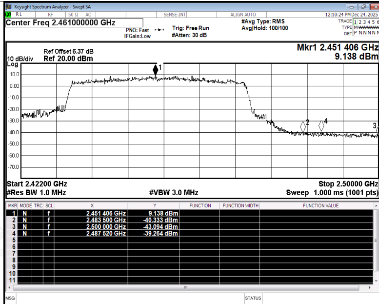
Restrict Band NVNT be40 2452MHz Ant4 Peak
