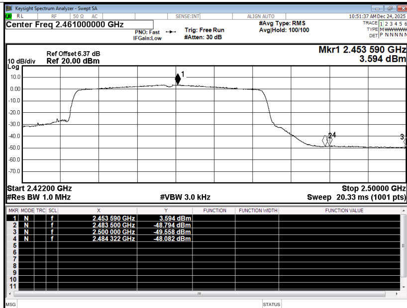
Restrict Band NVNT be40 2452MHz Ant3 Average
