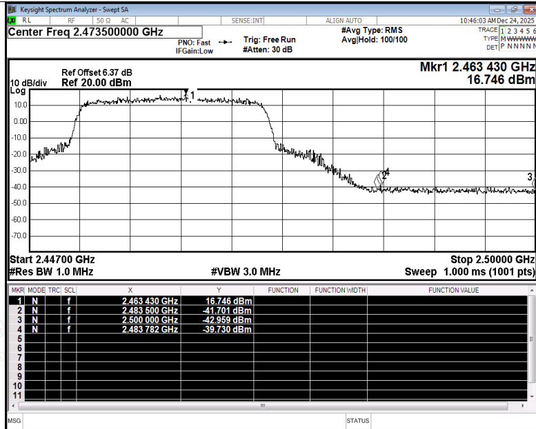
Restrict Band NVNT be20 2462MHz Ant3 Peak
