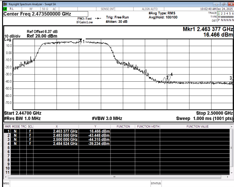
Restrict Band NVNT g 2462MHz Ant3 Peak
