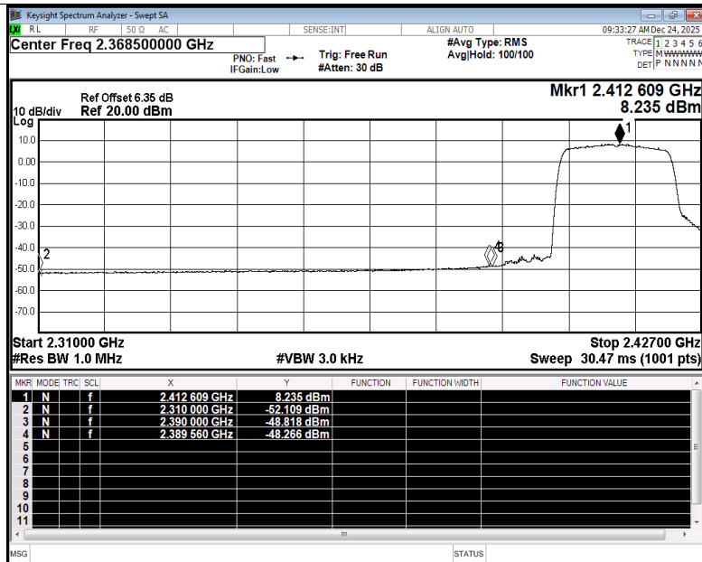
Restrict Band NVNT be20 2412MHz Ant2 Average
