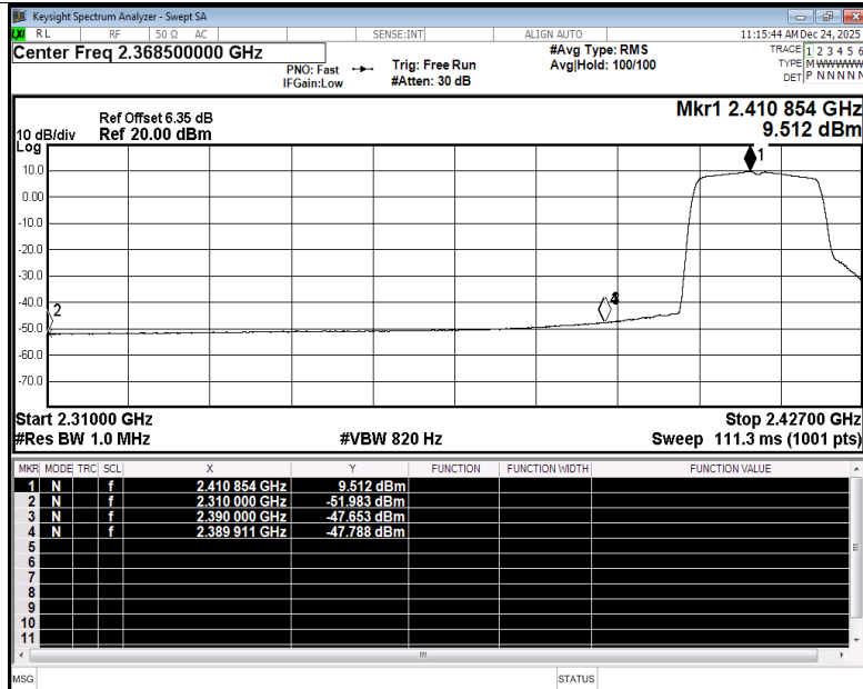
Restrict Band NVNT n20 2412MHz Ant4 Average
