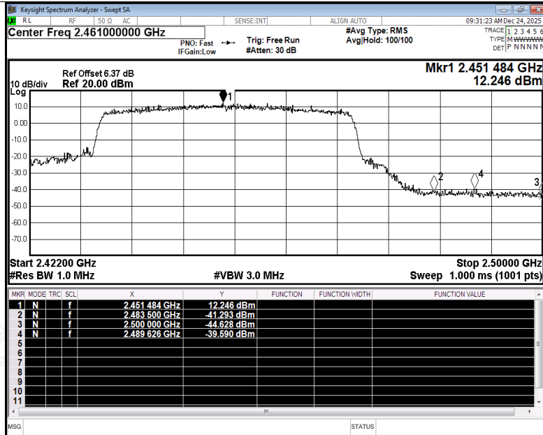
Restrict Band NVNT ax40 2452MHz Ant2 Peak
