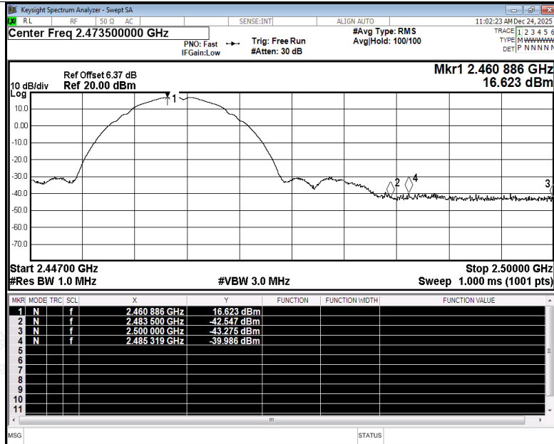
Restrict Band NVNT b 2462MHz Ant4 Peak
