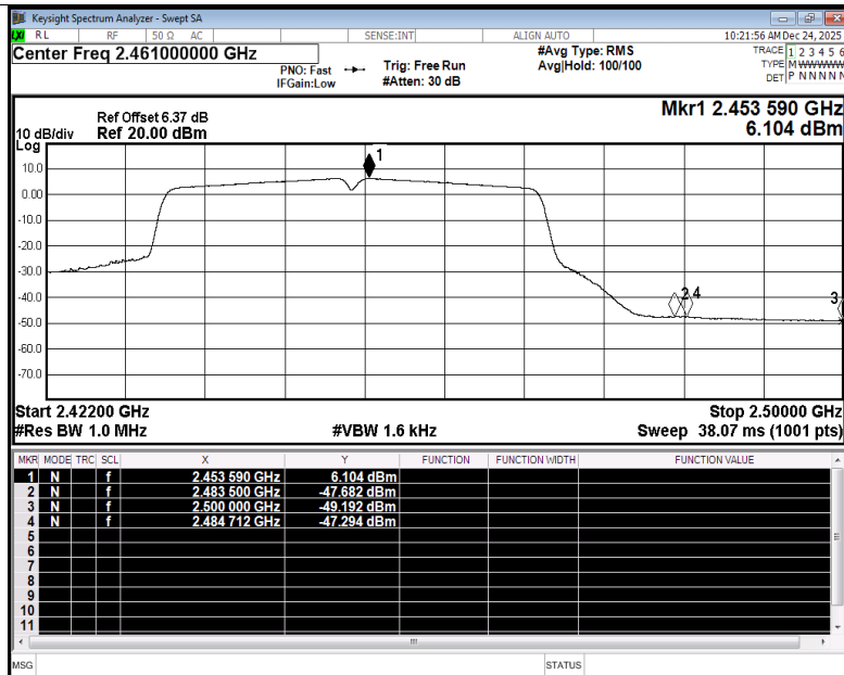
Restrict Band NVNT n40 2452MHz Ant3 Average
