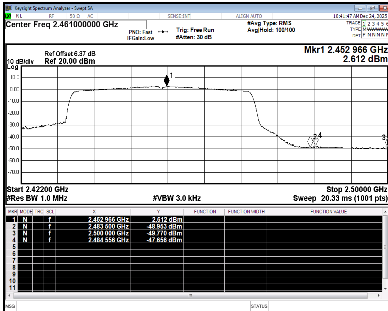
Restrict Band NVNT ax40 2452MHz Ant3 Average
