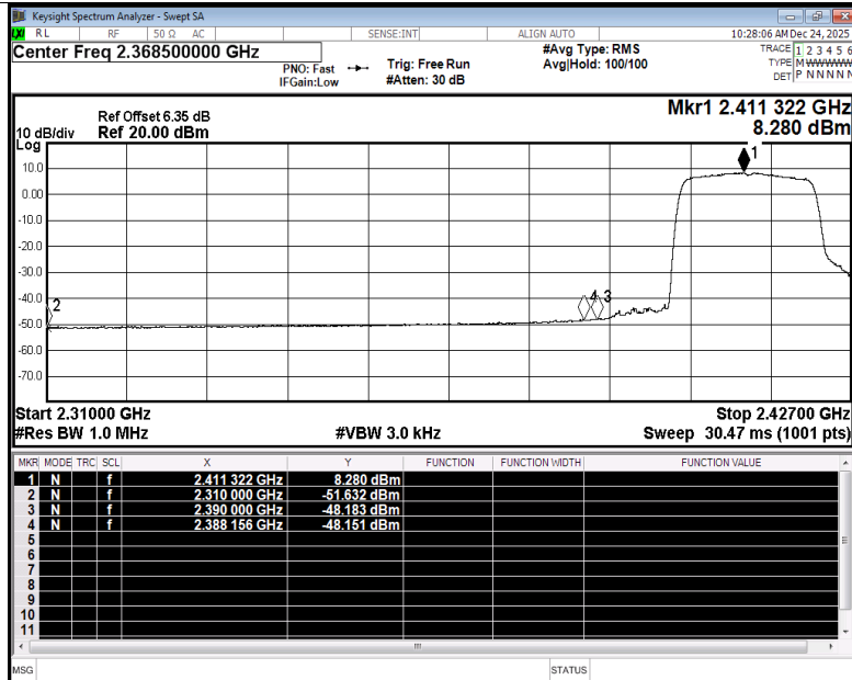
Restrict Band NVNT ax20 2412MHz Ant3 Average
