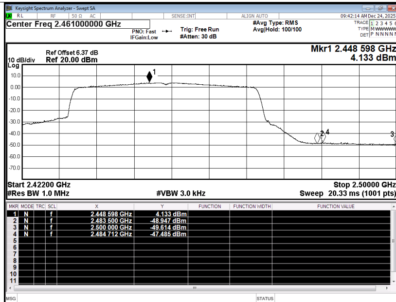
Restrict Band NVNT be40 2452MHz Ant2 Average
