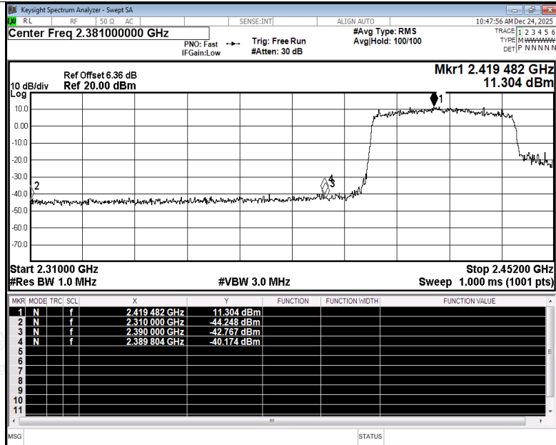
Restrict Band NVNT be40 2422MHz Ant3 Peak
