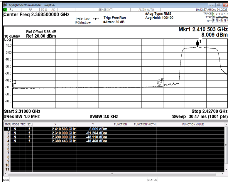
Restrict Band NVNT be20 2412MHz Ant3 Average
