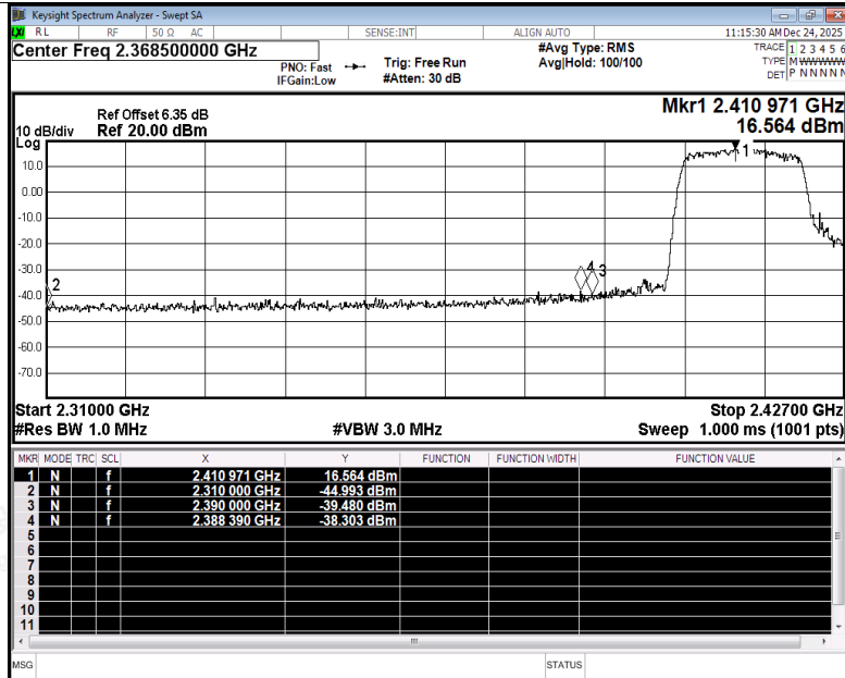
Restrict Band NVNT n20 2412MHz Ant4 Peak
