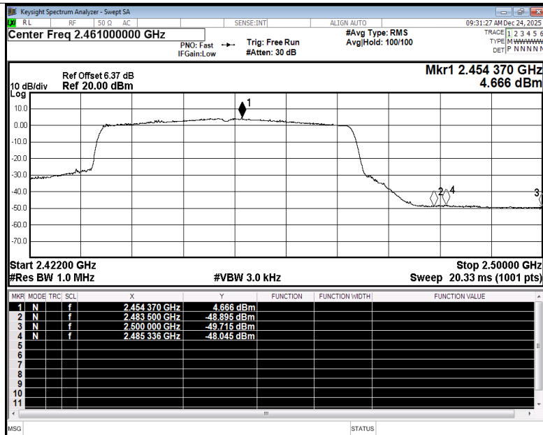
Restrict Band NVNT ax40 2452MHz Ant2 Average
