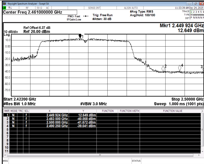
Restrict Band NVNT n40 2452MHz Ant4 Peak
