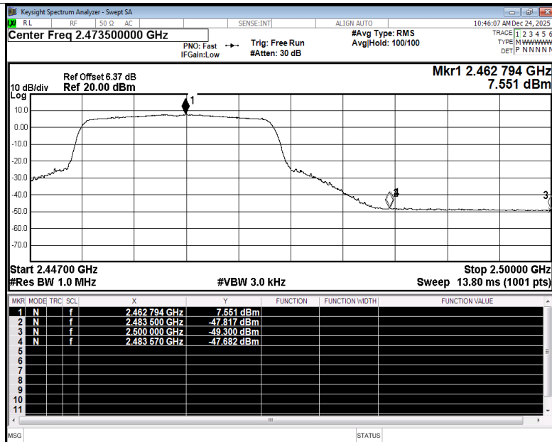
Restrict Band NVNT be20 2462MHz Ant3 Average
