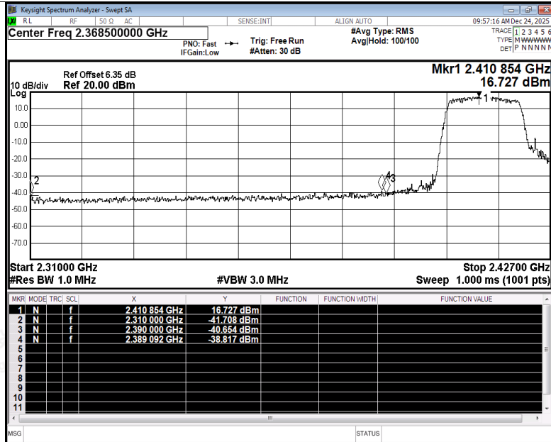
Restrict Band NVNT g 2412MHz Ant3 Peak
