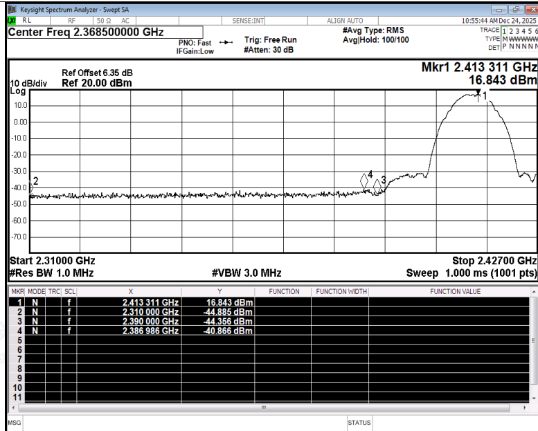
Restrict Band NVNT b 2412MHz Ant4 Peak
