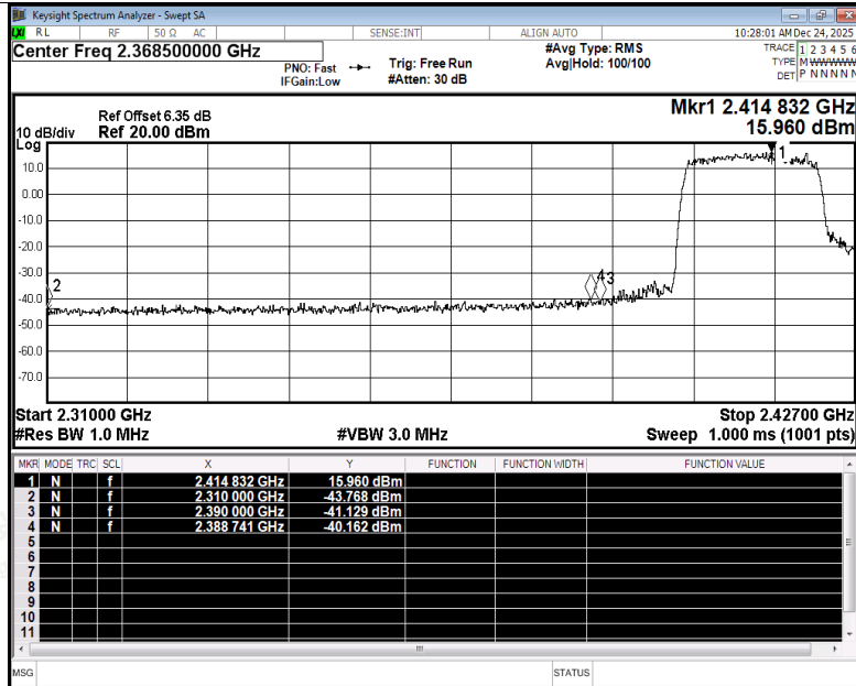
Restrict Band NVNT ax20 2412MHz Ant3 Peak
