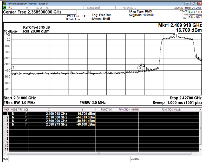
Restrict Band NVNT be20 2412MHz Ant4 Peak
