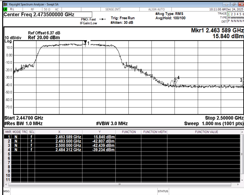
Restrict Band NVNT n20 2462MHz Ant3 Peak
