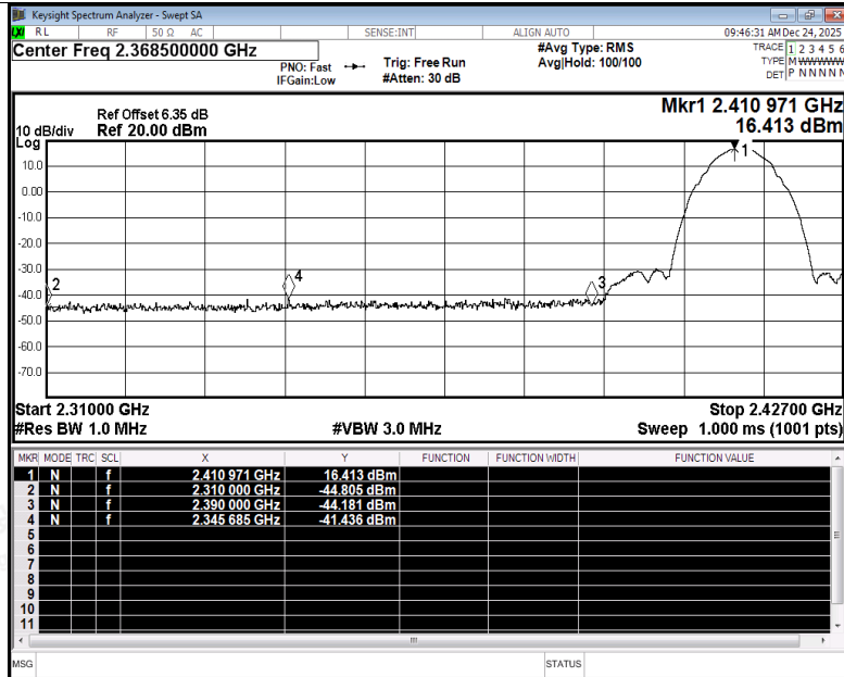
Restrict Band NVNT b 2412MHz Ant3 Peak
