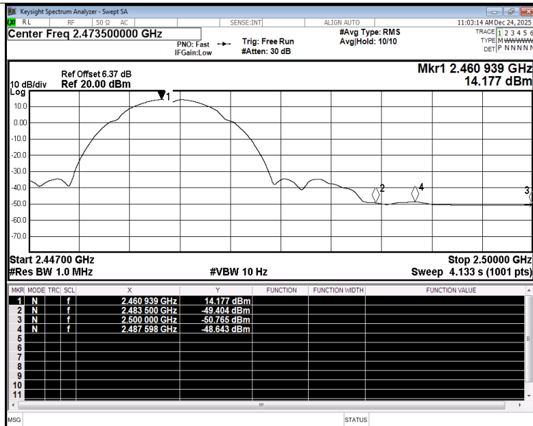
Restrict Band NVNT b 2462MHz Ant4 Average
