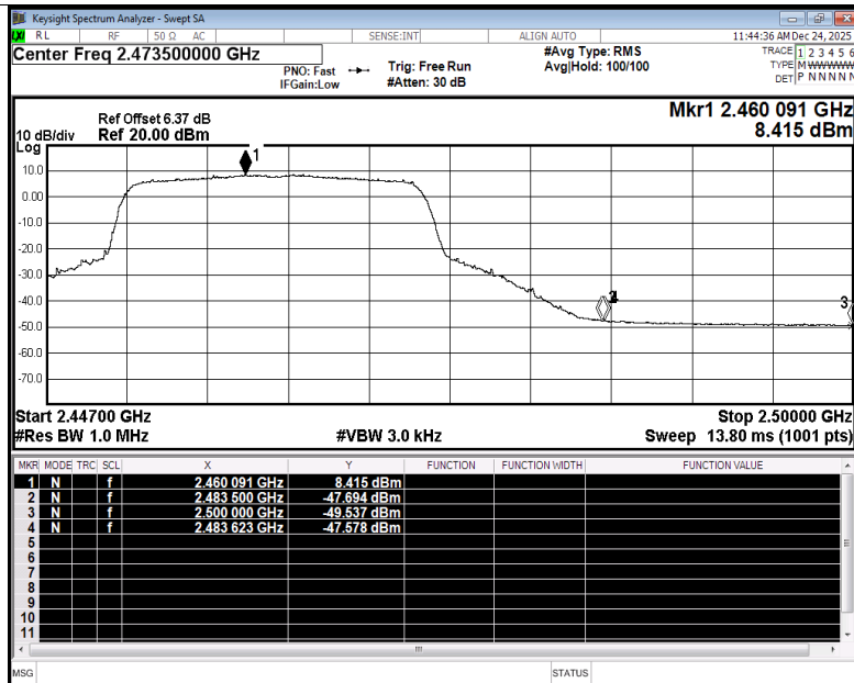
Restrict Band NVNT ax20 2462MHz Ant4 Average
