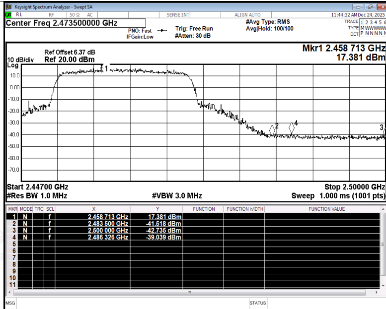
Restrict Band NVNT ax20 2462MHz Ant4 Peak
