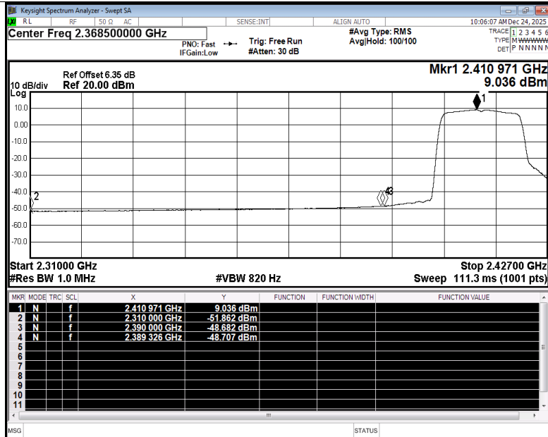
Restrict Band NVNT n20 2412MHz Ant3 Average
