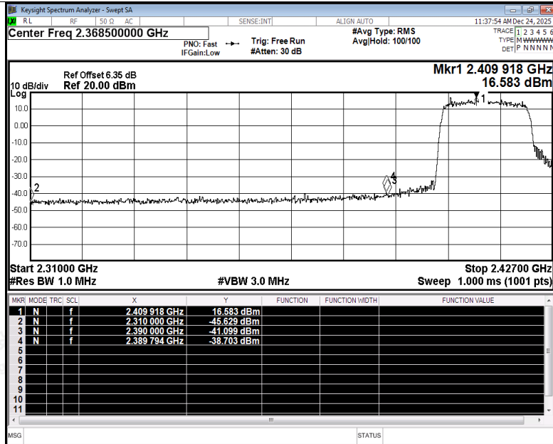
Restrict Band NVNT ax20 2412MHz Ant4 Peak
