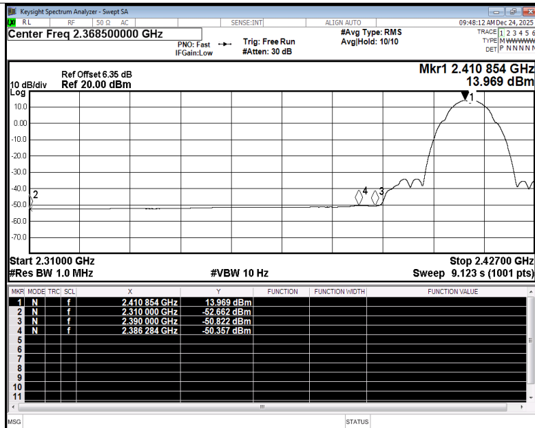
Restrict Band NVNT b 2412MHz Ant3 Average
