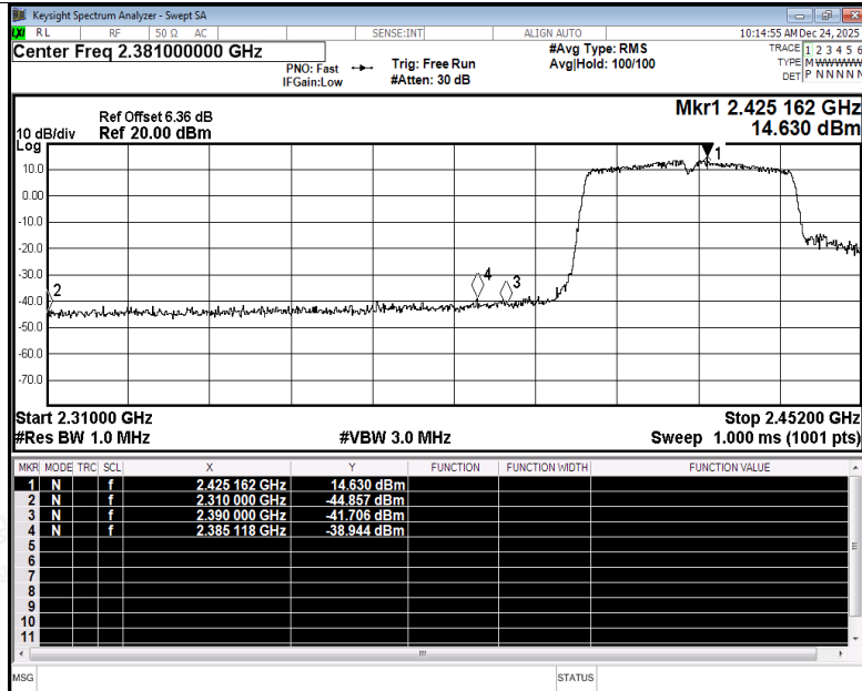
Restrict Band NVNT n40 2422MHz Ant3 Peak
