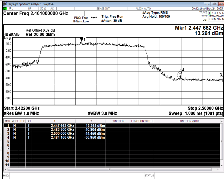
Restrict Band NVNT be40 2452MHz Ant2 Peak
