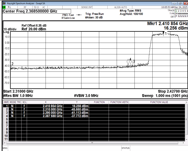
Restrict Band NVNT n20 2412MHz Ant3 Peak
