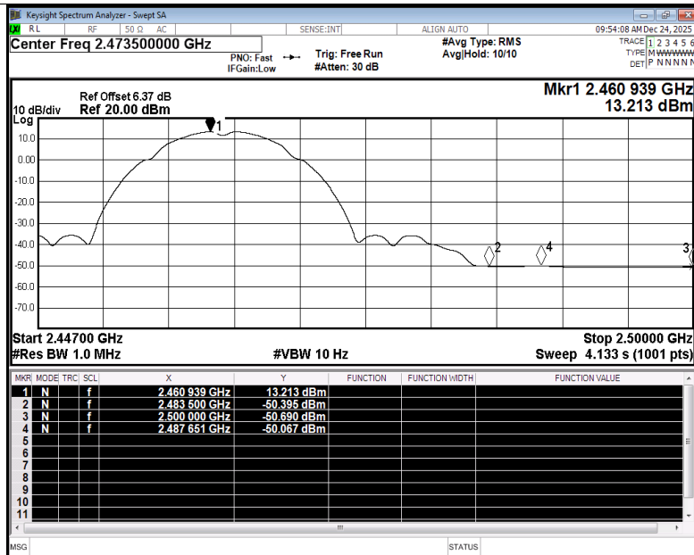
Restrict Band NVNT b 2462MHz Ant3 Average
