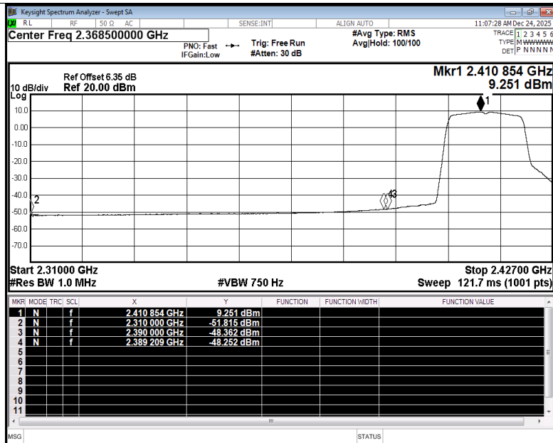
Restrict Band NVNT g 2412MHz Ant4 Average
