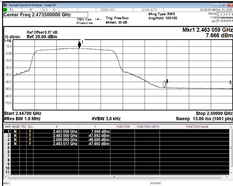
Restrict Band NVNT ax20 2462MHz Ant3 Average
