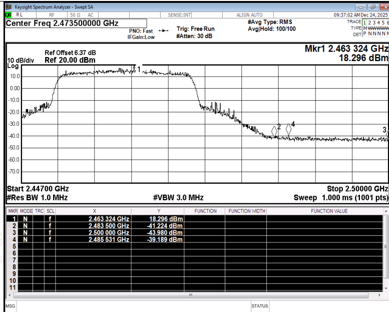
Restrict Band NVNT be20 2462MHz Ant2 Peak
