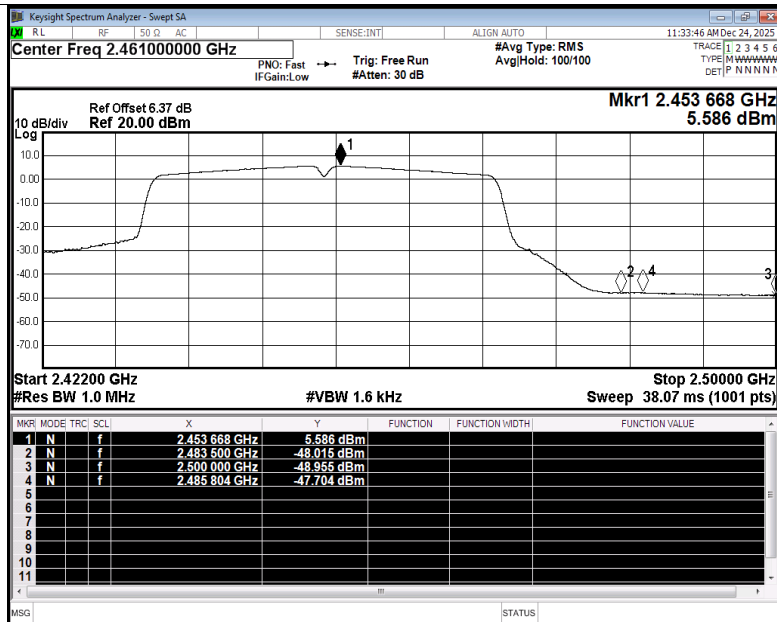
Restrict Band NVNT n40 2452MHz Ant4 Average
