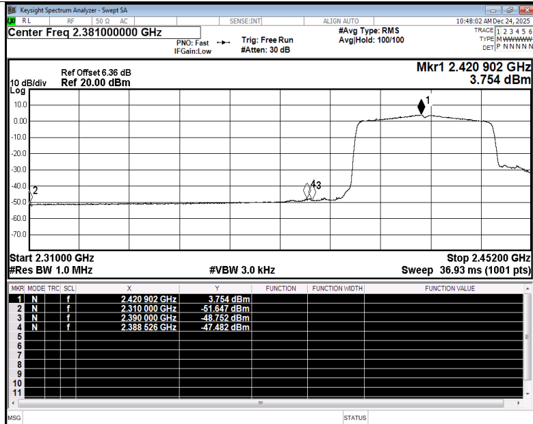
Restrict Band NVNT be40 2422MHz Ant3 Average
