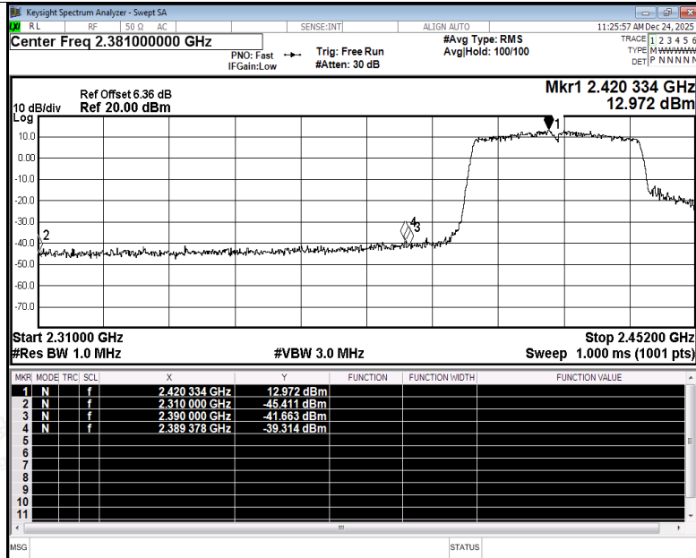
Restrict Band NVNT n40 2422MHz Ant4 Peak
