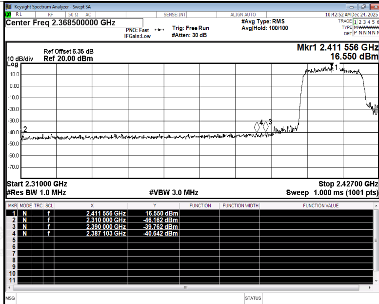
Restrict Band NVNT be20 2412MHz Ant3 Peak
