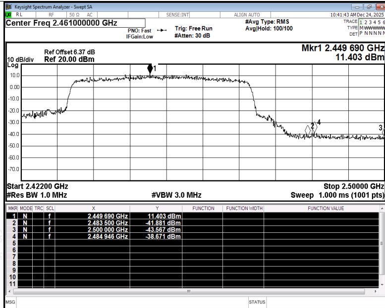
Restrict Band NVNT ax40 2452MHz Ant3 Peak
