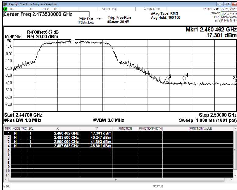
Restrict Band NVNT g 2462MHz Ant4 Peak
