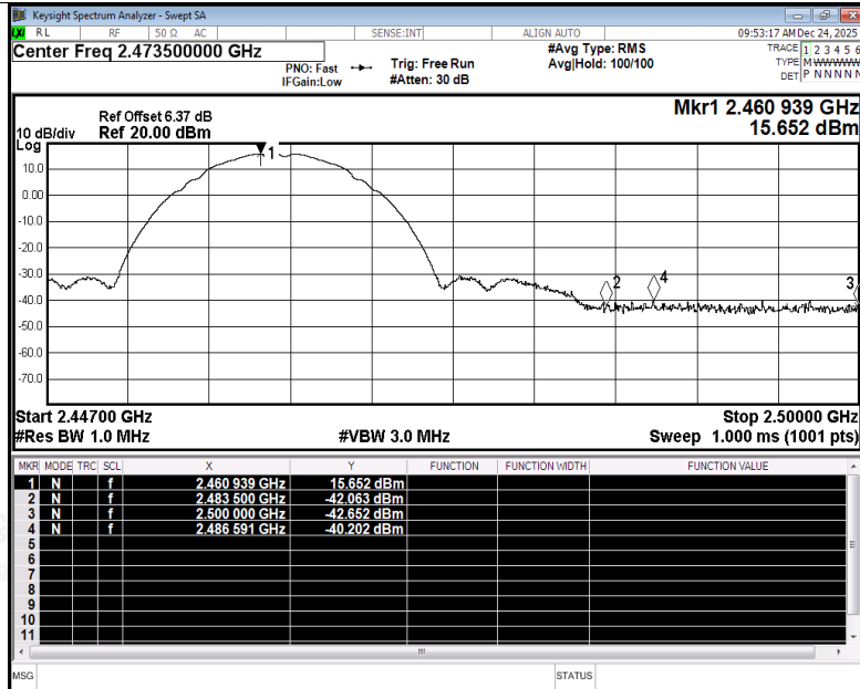
Restrict Band NVNT b 2462MHz Ant3 Peak
