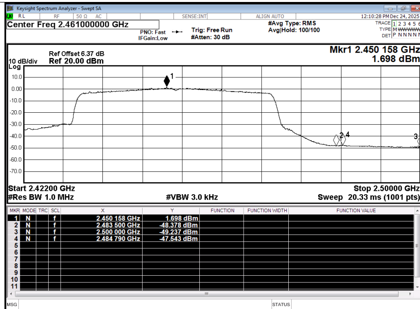
Restrict Band NVNT be40 2452MHz Ant4 Average
