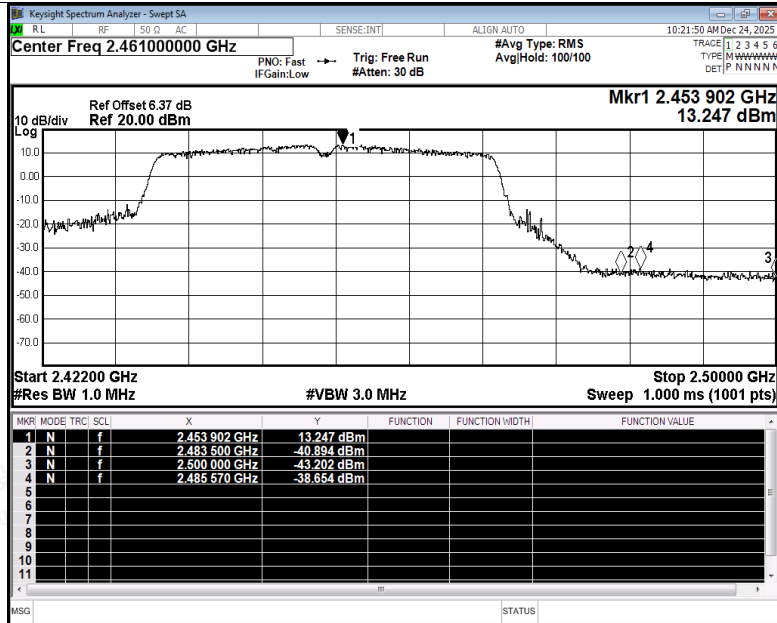
Restrict Band NVNT n40 2452MHz Ant3 Peak
