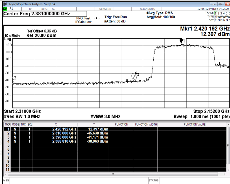
Restrict Band NVNT be40 2422MHz Ant4 Peak
