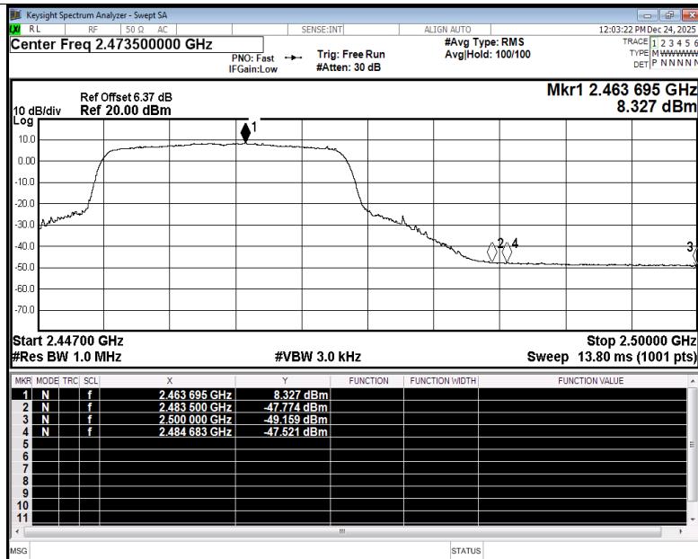
Restrict Band NVNT be20 2462MHz Ant4 Average
