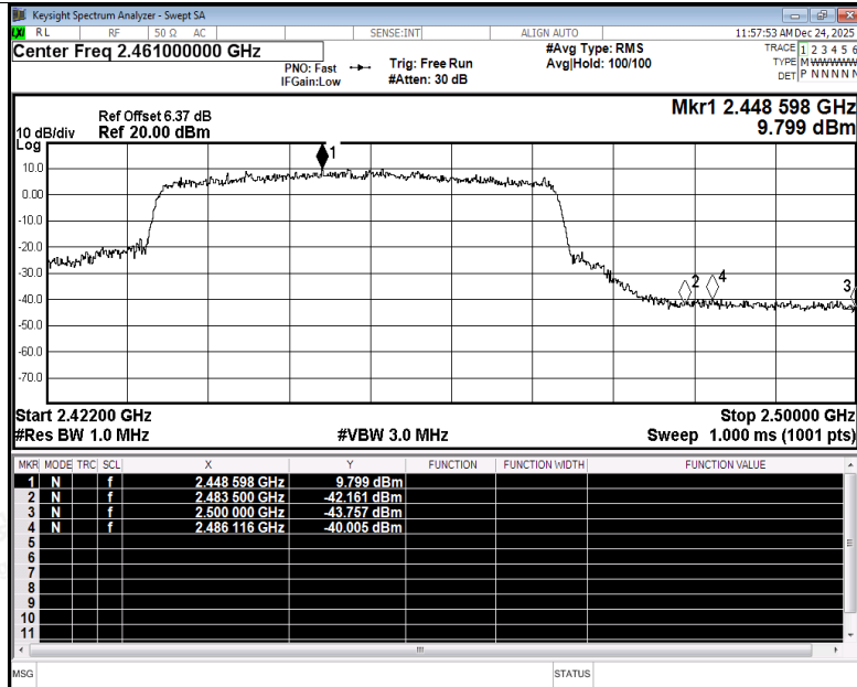
Restrict Band NVNT ax40 2452MHz Ant4 Peak
