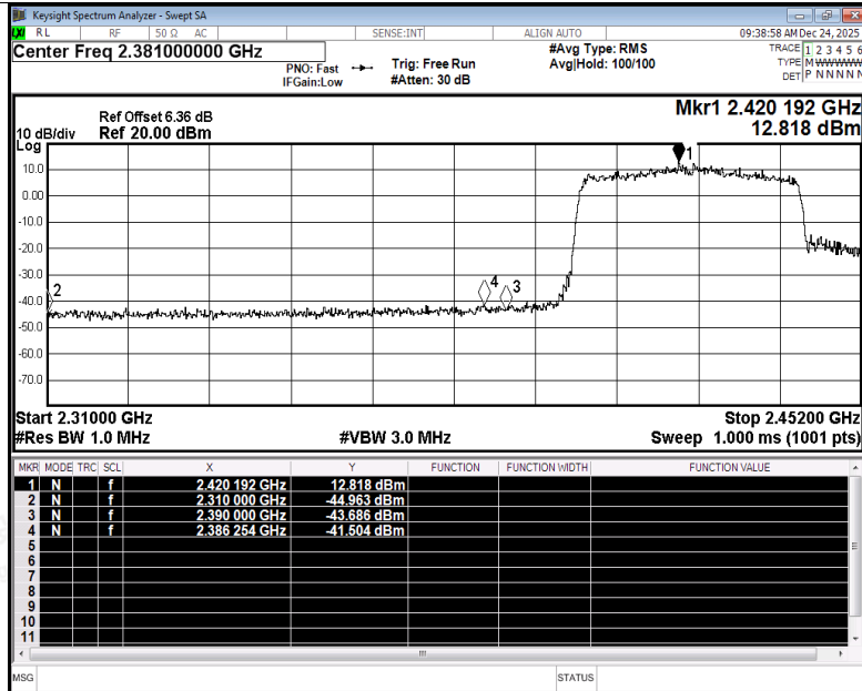
Restrict Band NVNT be40 2422MHz Ant2 Peak
