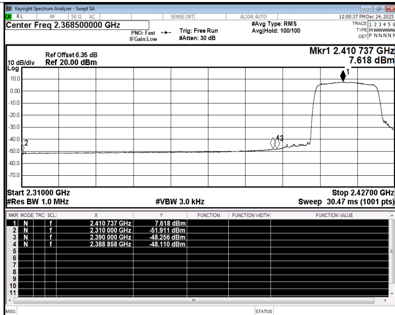
Restrict Band NVNT be20 2412MHz Ant4 Average
