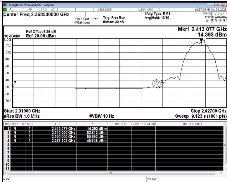
Restrict Band NVNT b 2412MHz Ant4 Average
