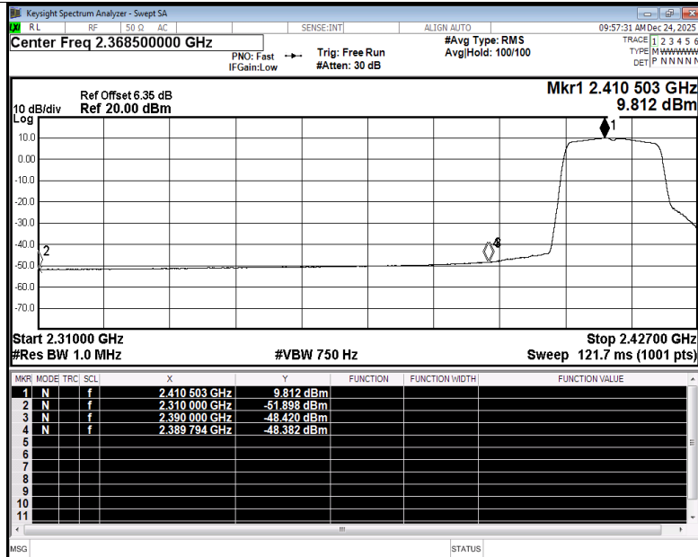
Restrict Band NVNT g 2412MHz Ant3 Average
