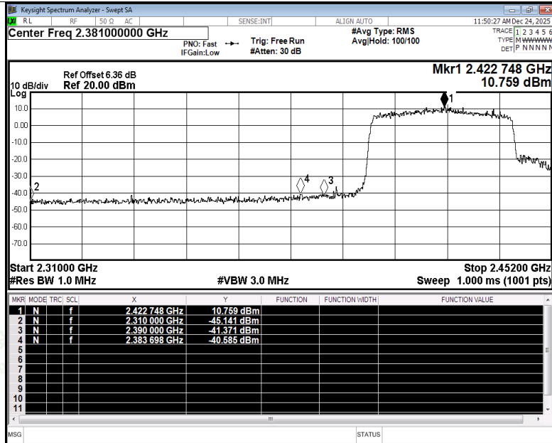
Restrict Band NVNT ax40 2422MHz Ant4 Peak
