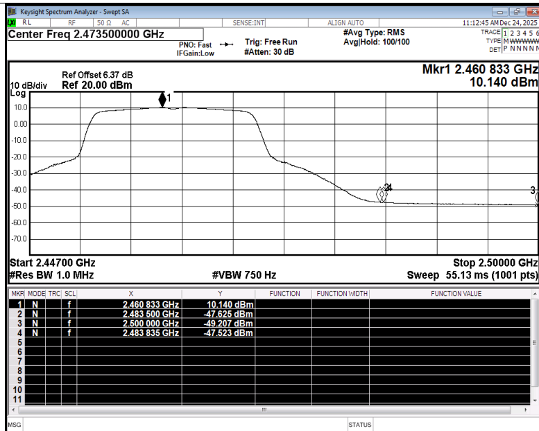
Restrict Band NVNT g 2462MHz Ant4 Average
