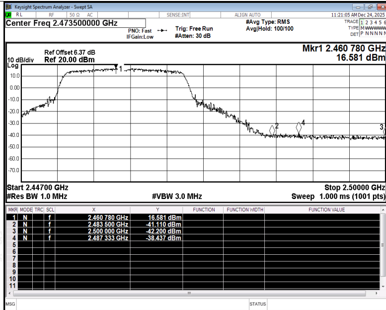
Restrict Band NVNT n20 2462MHz Ant4 Peak
