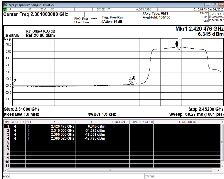
Restrict Band NVNT n40 2422MHz Ant3 Average
