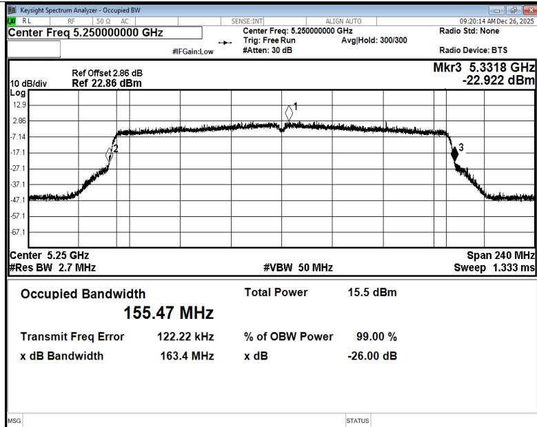
-26dB Bandwidth NVNT ax160 5250MHz Ant2
