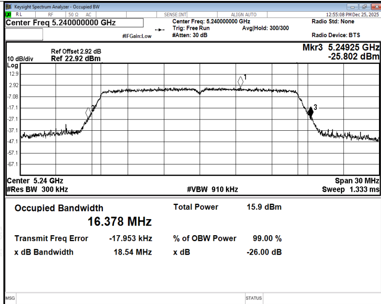
-26dB Bandwidth NVNT a 5240MHz Ant2
