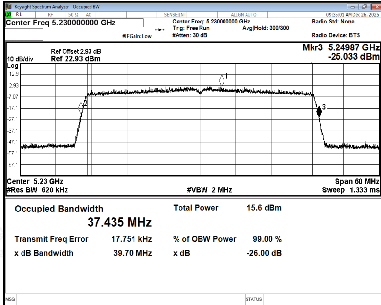
-26dB Bandwidth NVNT be40 5230MHz Ant2
