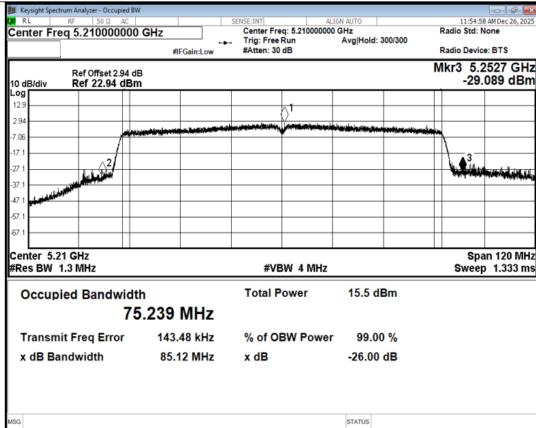
-26dB Bandwidth NVNT ac80 5210MHz Ant4
