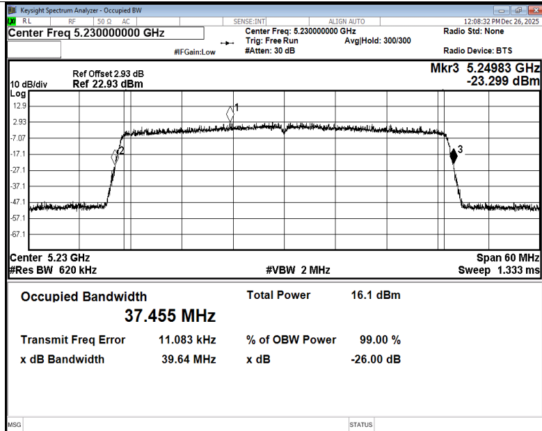
-26dB Bandwidth NVNT ax40 5230MHz Ant4
