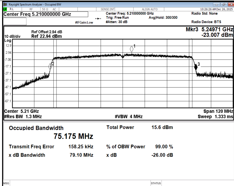
-26dB Bandwidth NVNT ac80 5210MHz Ant3
