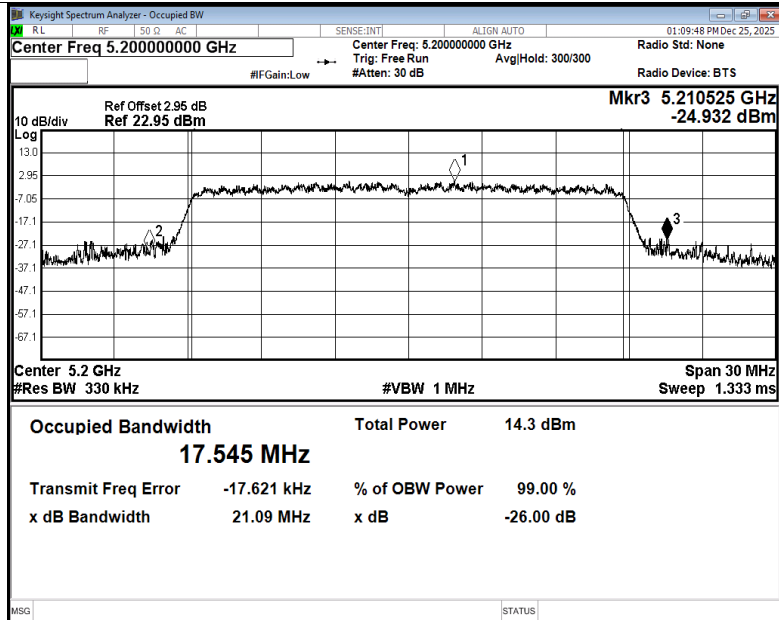
-26dB Bandwidth NVNT ac20 5200MHz Ant2
