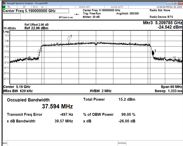
-26dB Bandwidth NVNT ax40 5190MHz Ant4
