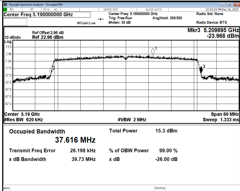
-26dB Bandwidth NVNT be40 5190MHz Ant4
