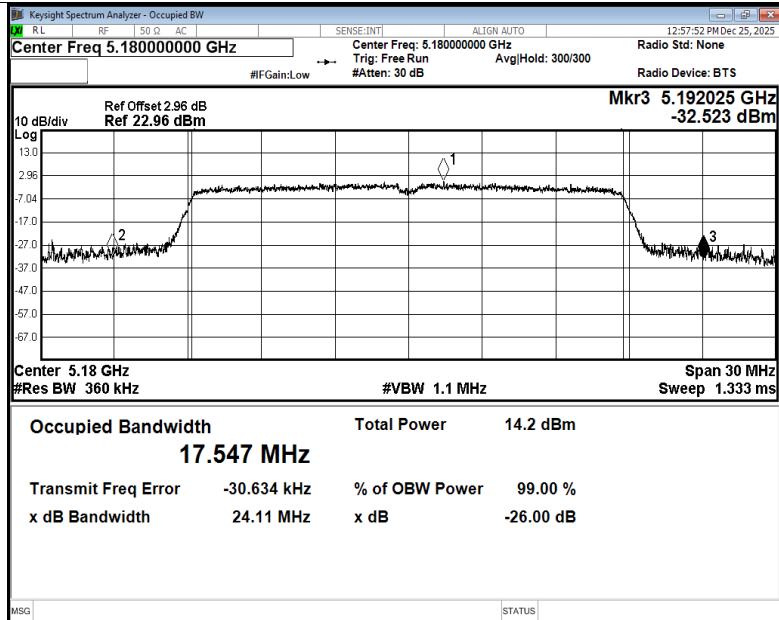
-26dB Bandwidth NVNT n20 5180MHz Ant2
