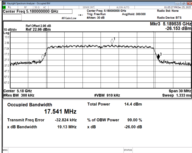
-26dB Bandwidth NVNT ac20 5180MHz Ant2
