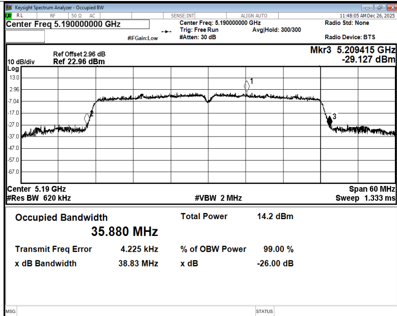
-26dB Bandwidth NVNT ac40 5190MHz Ant4
