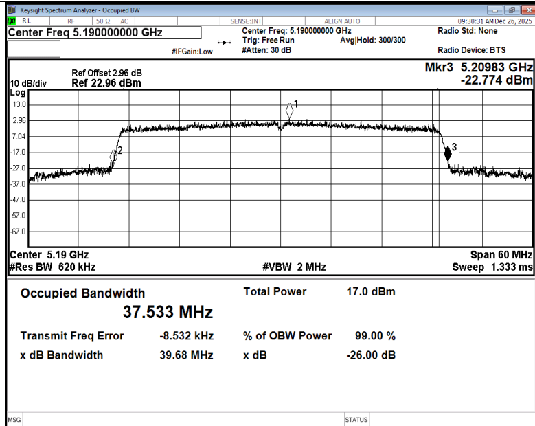
-26dB Bandwidth NVNT be40 5190MHz Ant2
