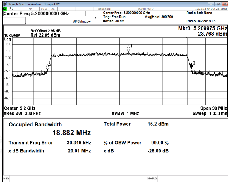
-26dB Bandwidth NVNT ax20 5200MHz Ant3
