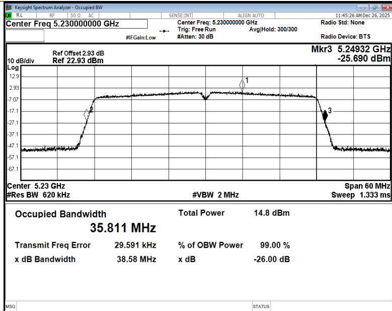
-26dB Bandwidth NVNT n40 5230MHz Ant4
