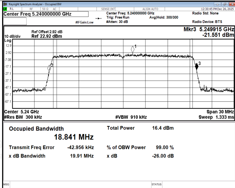
-26dB Bandwidth NVNT be20 5240MHz Ant4
