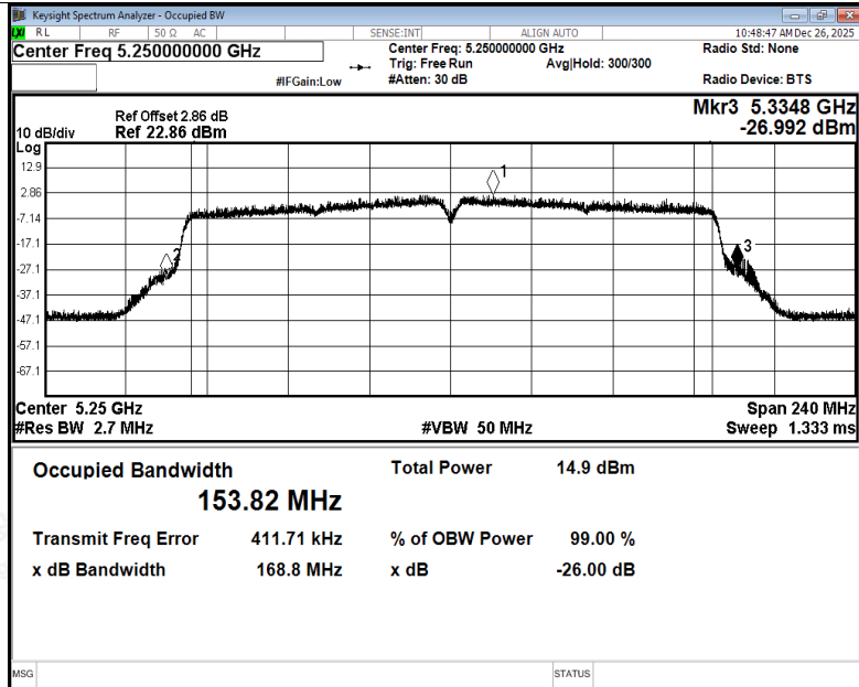
-26dB Bandwidth NVNT ac160 5250MHz Ant3
