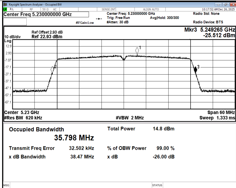
-26dB Bandwidth NVNT n40 5230MHz Ant3
