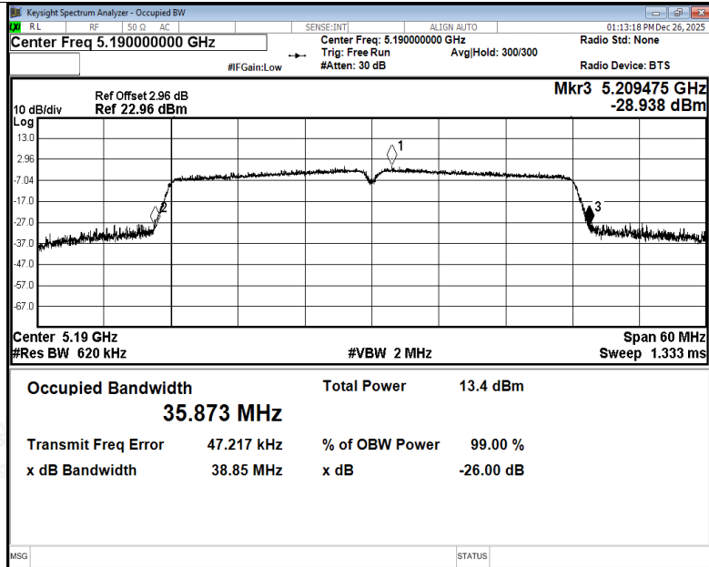
-26dB Bandwidth NVNT n40 5190MHz Ant5
