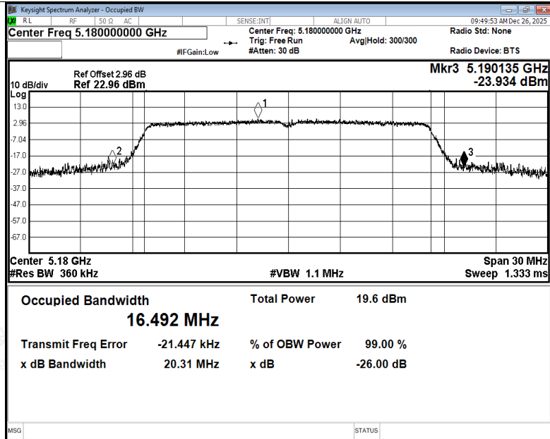
-26dB Bandwidth NVNT a 5180MHz Ant3
