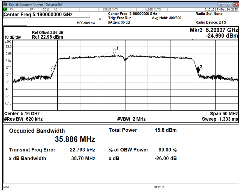
-26dB Bandwidth NVNT ac40 5190MHz Ant1
