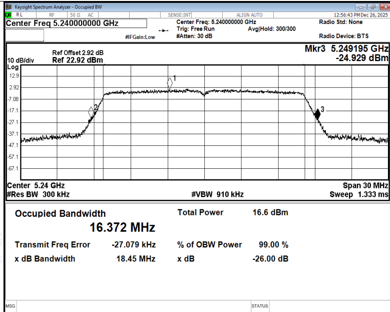
-26dB Bandwidth NVNT a 5240MHz Ant5
