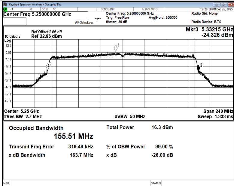
-26dB Bandwidth NVNT ax160 5250MHz Ant4
