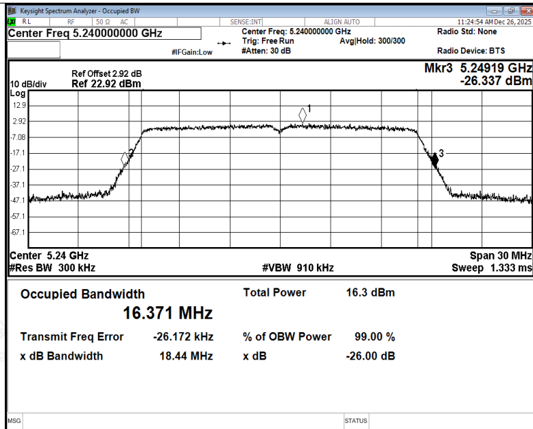
-26dB Bandwidth NVNT a 5240MHz Ant4
