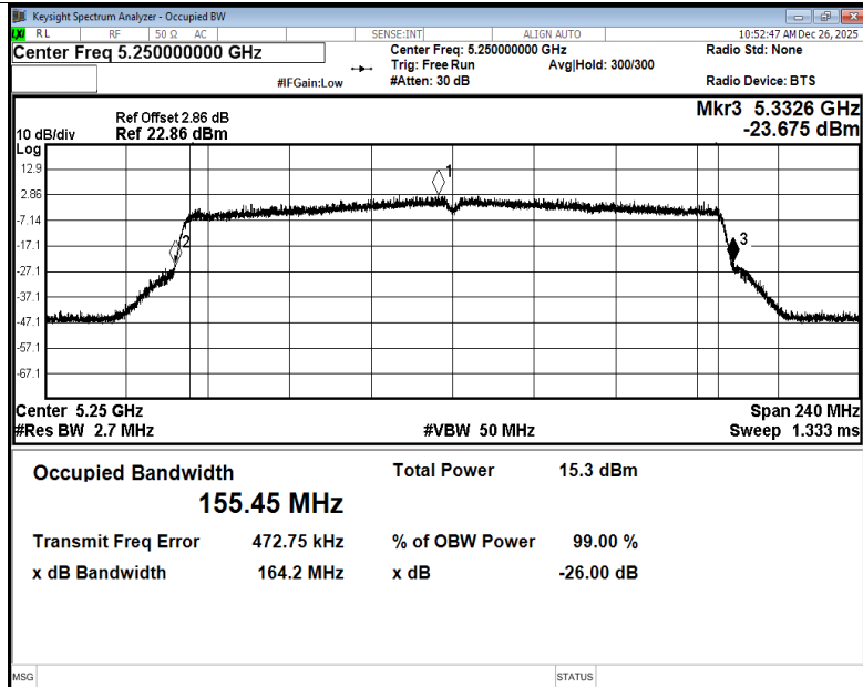
-26dB Bandwidth NVNT ax160 5250MHz Ant3
