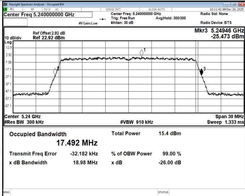
-26dB Bandwidth NVNT ac20 5240MHz Ant3
