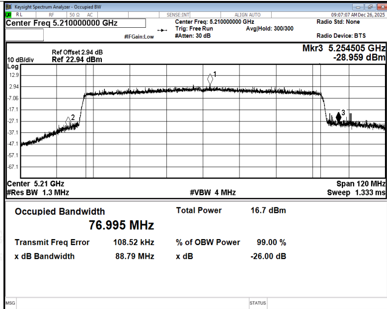
-26dB Bandwidth NVNT ax80 5210MHz Ant2
