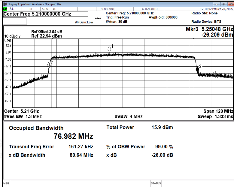
-26dB Bandwidth NVNT ax80 5210MHz Ant4
