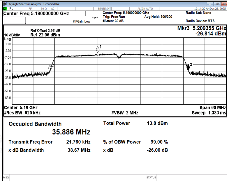
-26dB Bandwidth NVNT n40 5190MHz Ant3
