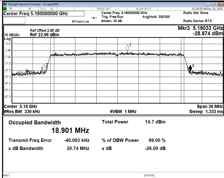
-26dB Bandwidth NVNT ax20 5180MHz Ant3
