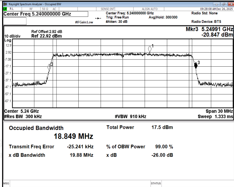
-26dB Bandwidth NVNT be20 5240MHz Ant2
