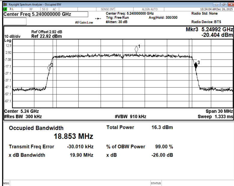
-26dB Bandwidth NVNT ax20 5240MHz Ant3
