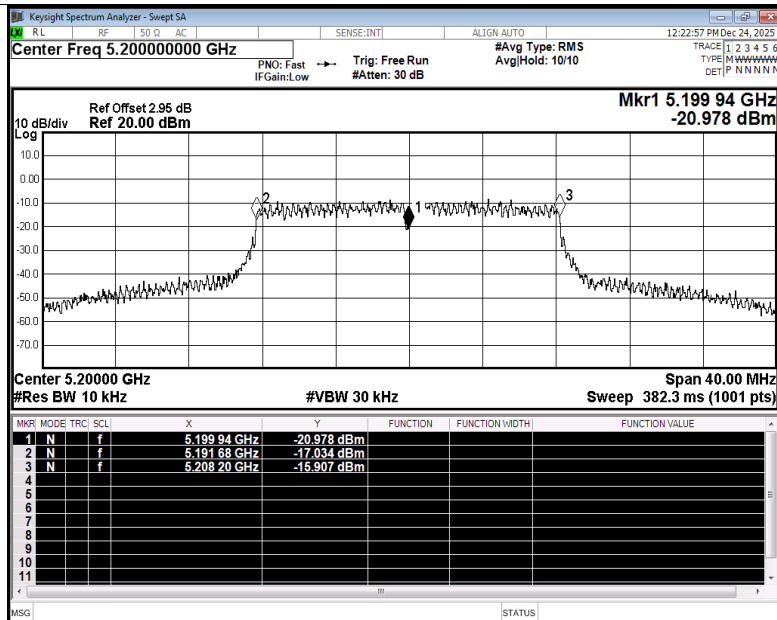
Freq. Stability NVNT a 5200MHz Ant1
