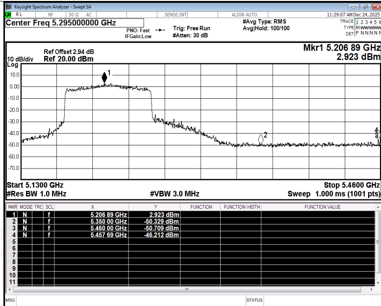
Restrict Band NVNT ax80 5210MHz Ant5 Peak
