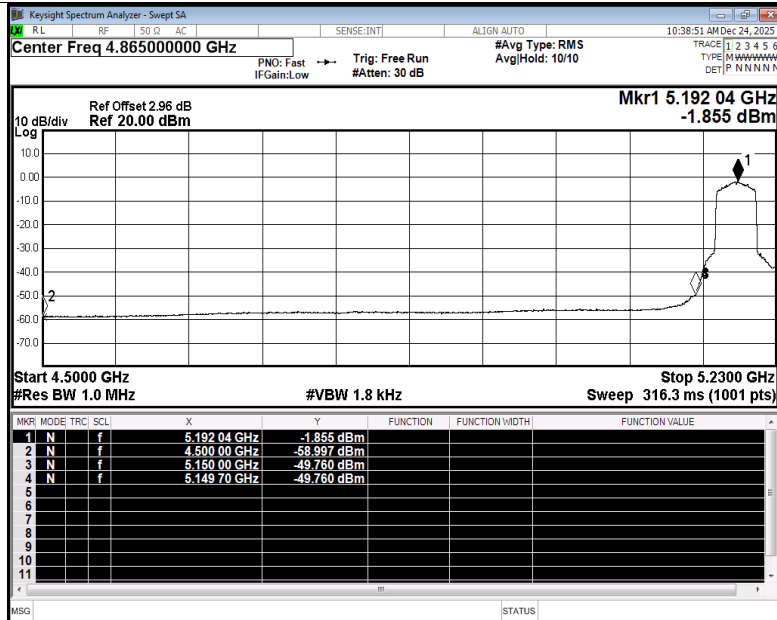
Restrict Band NVNT be40 5190MHz Ant4 Average
