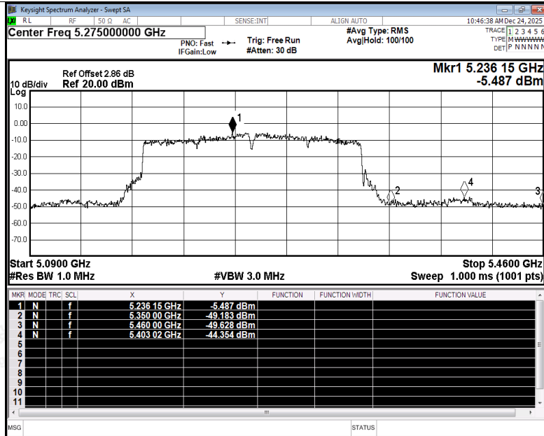
Restrict Band NVNT ac160 5250MHz Ant4 Peak
