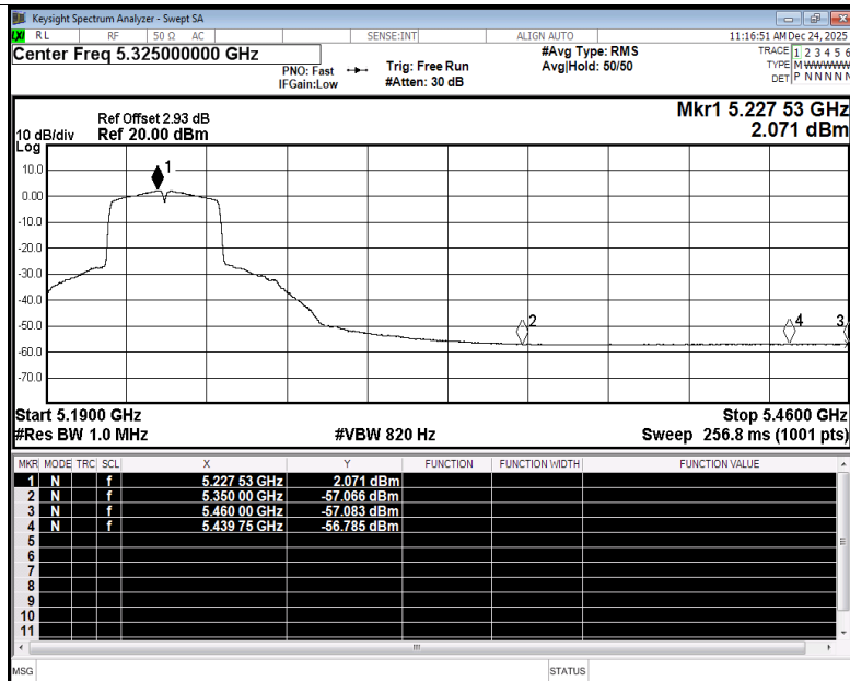
Restrict Band NVNT ac40 5230MHz Ant5 Average
