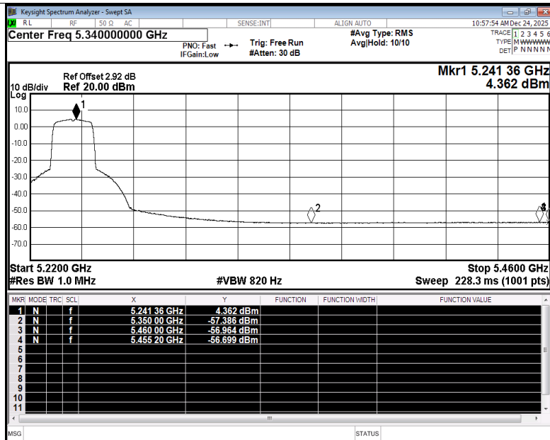
Restrict Band NVNT n20 5240MHz Ant5 Average
