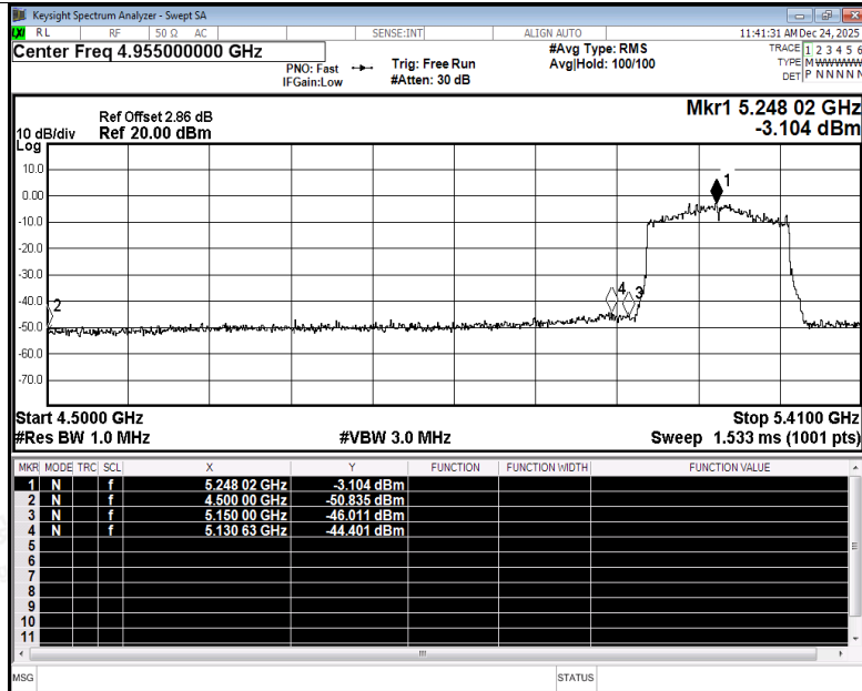
Restrict Band NVNT be160 5250MHz Ant5 Peak
