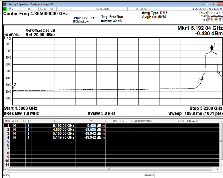
Restrict Band NVNT be40 5190MHz Ant5 Average
