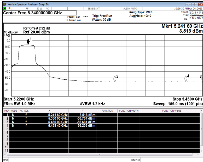
Restrict Band NVNT be20 5240MHz Ant4 Average
