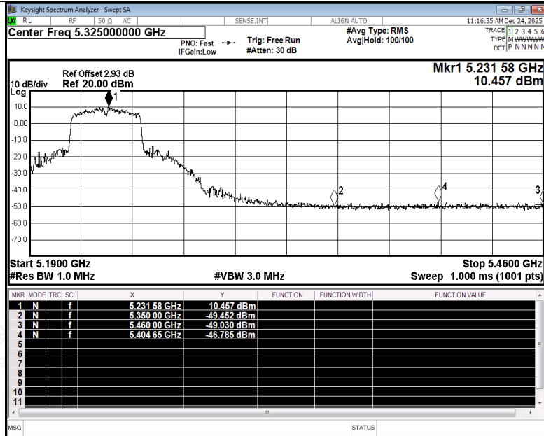
Restrict Band NVNT ac40 5230MHz Ant5 Peak
