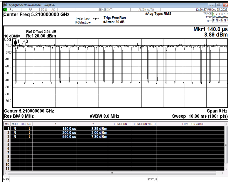
Duty Cycle NVNT be80 5210MHz Ant1
