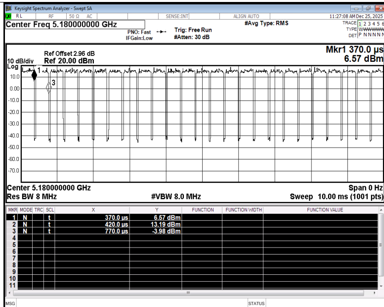
Duty Cycle NVNT ax20 5180MHz Ant1
