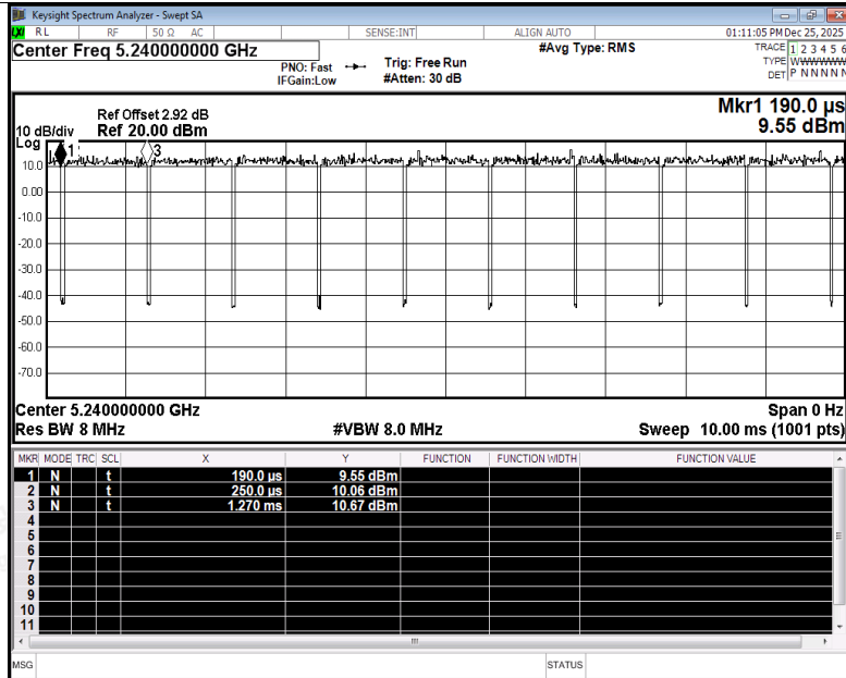
Duty Cycle NVNT ac20 5240MHz Ant2
