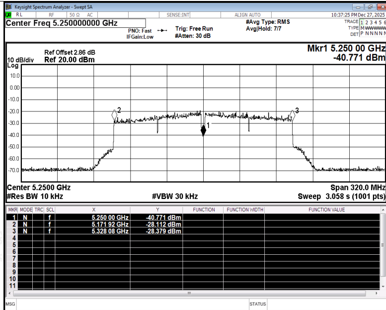
Freq. Stability NVNT ac160 5250MHz Ant5
