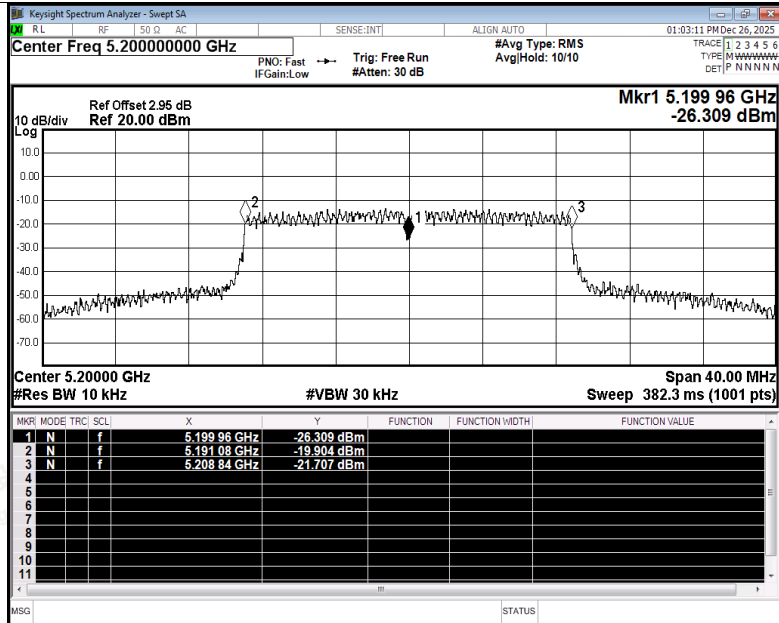
Freq. Stability NVNT n20 5200MHz Ant5
