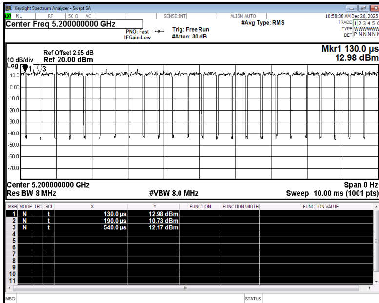
Duty Cycle NVNT be20 5200MHz Ant3
