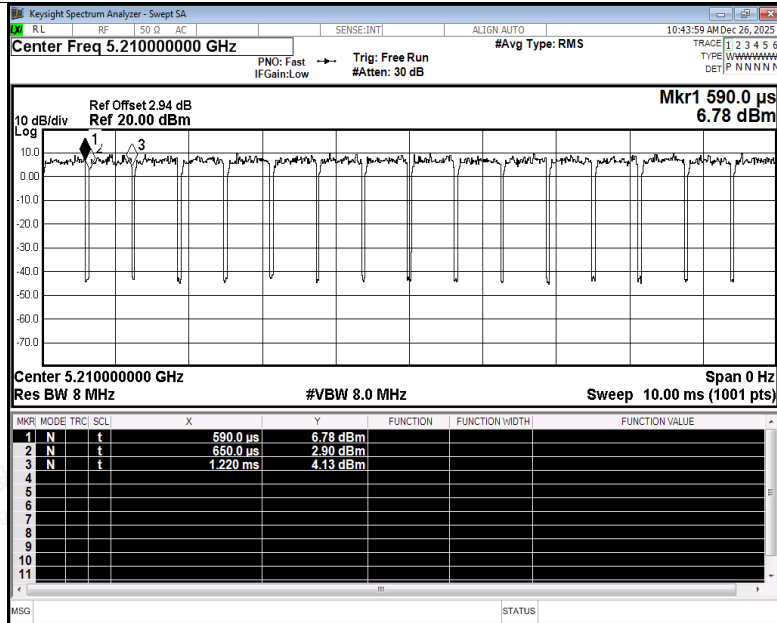
Duty Cycle NVNT ax80 5210MHz Ant3
