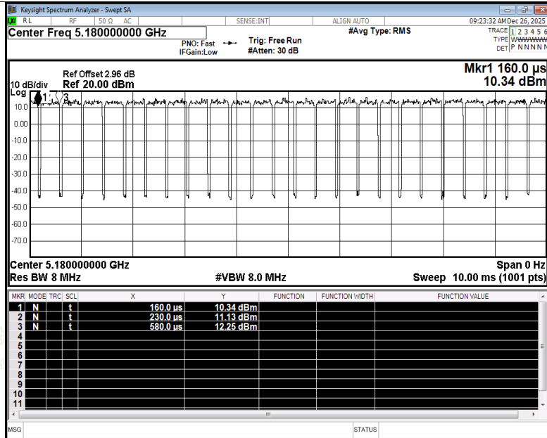
Duty Cycle NVNT be20 5180MHz Ant2
