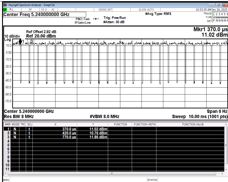
Duty Cycle NVNT ax20 5240MHz Ant3
