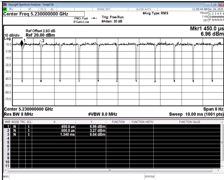
Duty Cycle NVNT be40 5230MHz Ant3
