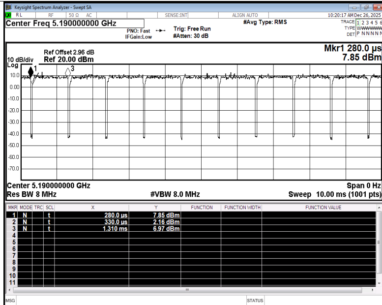
Duty Cycle NVNT ac40 5190MHz Ant3
