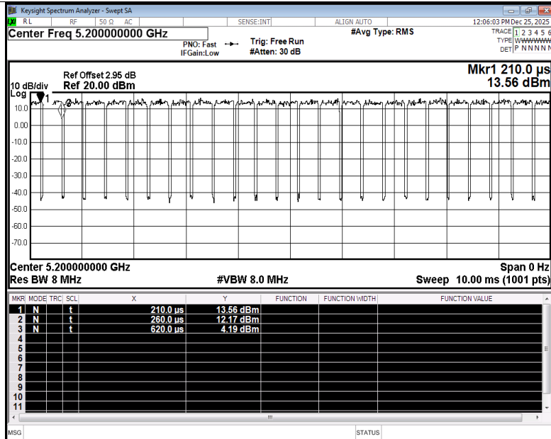
Duty Cycle NVNT be20 5200MHz Ant1
