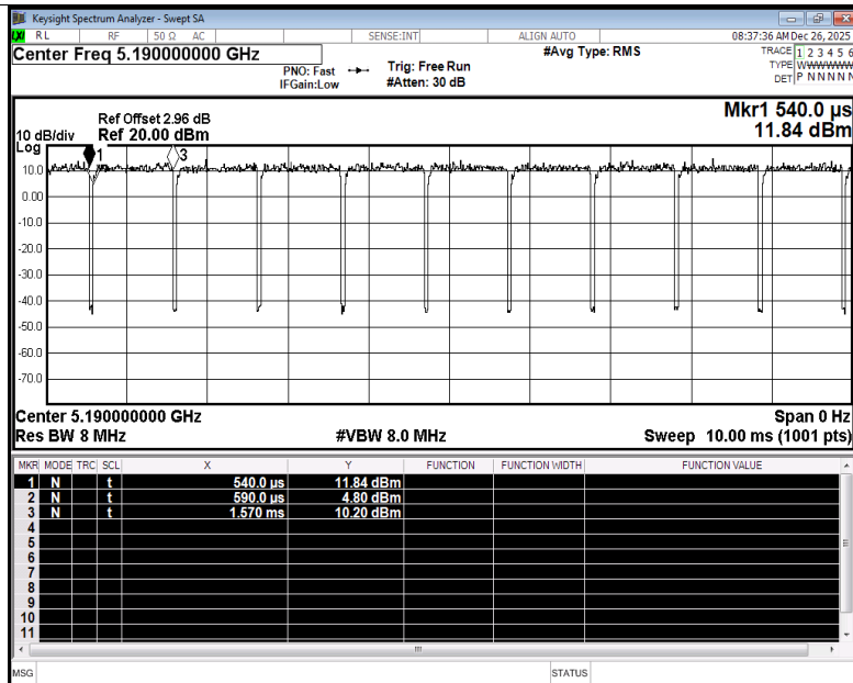
Duty Cycle NVNT ac40 5190MHz Ant2
