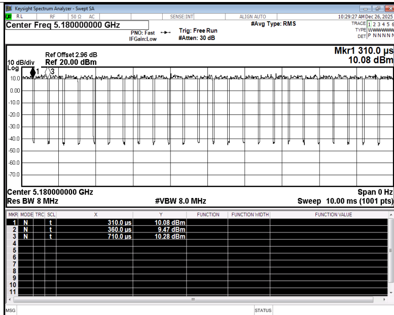
Duty Cycle NVNT ax20 5180MHz Ant3
