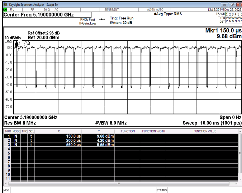
Duty Cycle NVNT be40 5190MHz Ant1
