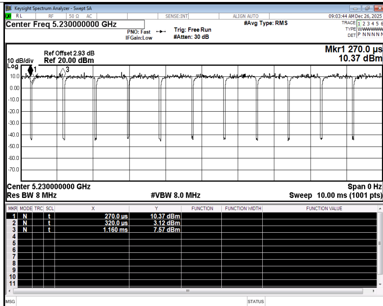
Duty Cycle NVNT ax40 5230MHz Ant2
