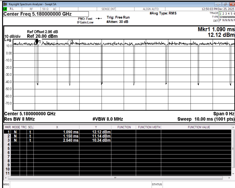
Duty Cycle NVNT a 5180MHz Ant2
