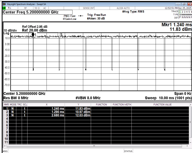
Duty Cycle NVNT a 5200MHz Ant2
