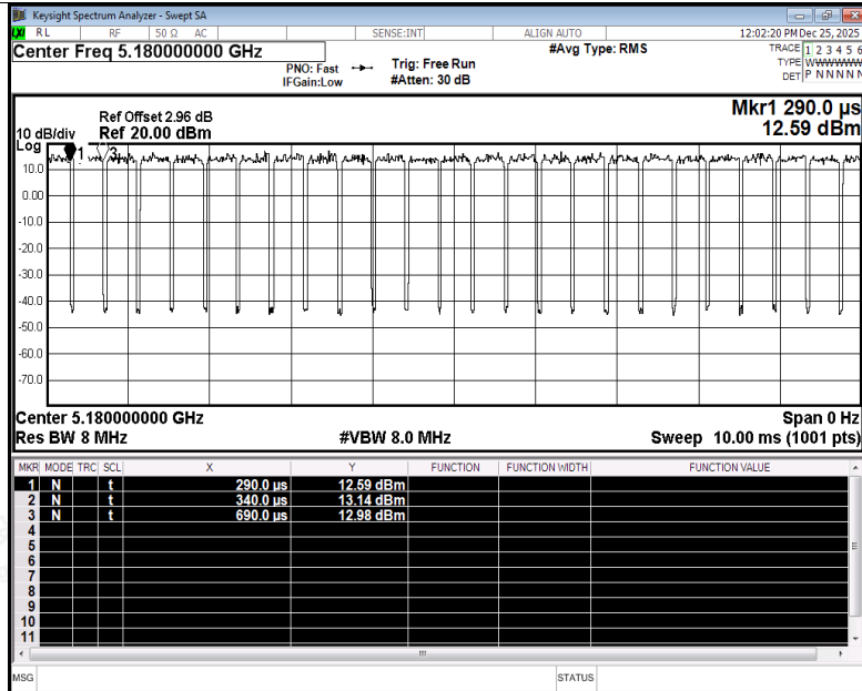
Duty Cycle NVNT be20 5180MHz Ant1
