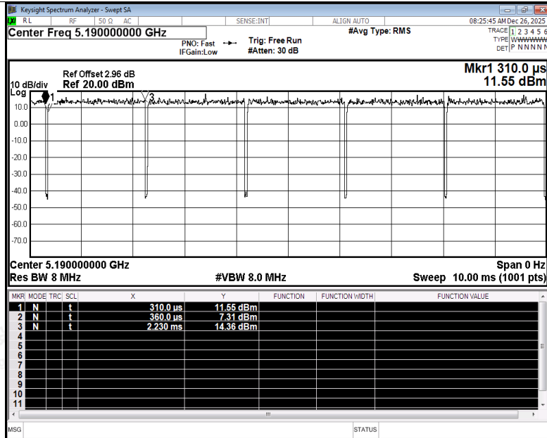
Duty Cycle NVNT n40 5190MHz Ant2
