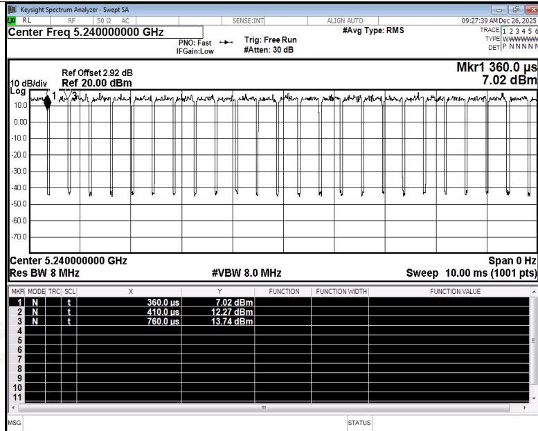
Duty Cycle NVNT be20 5240MHz Ant2
