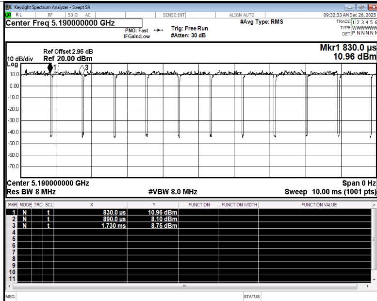
Duty Cycle NVNT be40 5190MHz Ant2
