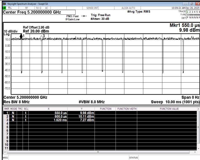
Duty Cycle NVNT ac20 5200MHz Ant3
