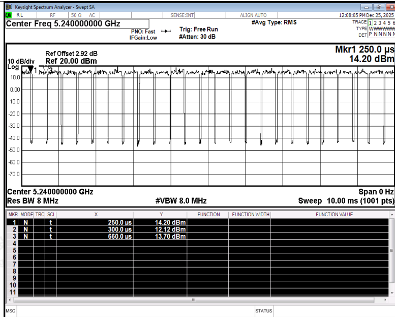
Duty Cycle NVNT be20 5240MHz Ant1
