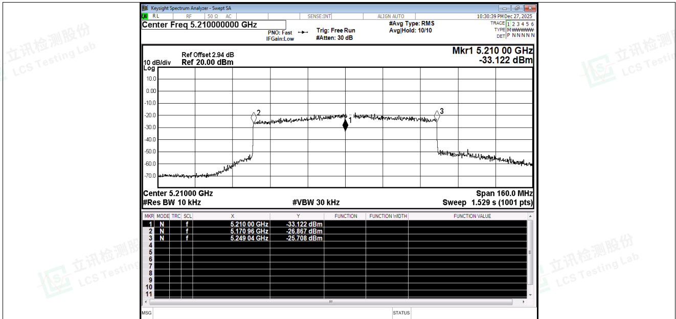
Freq. Stability NVNT ax80 5210MHz Ant5
