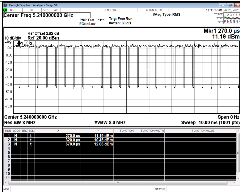
Duty Cycle NVNT ax20 5240MHz Ant1
