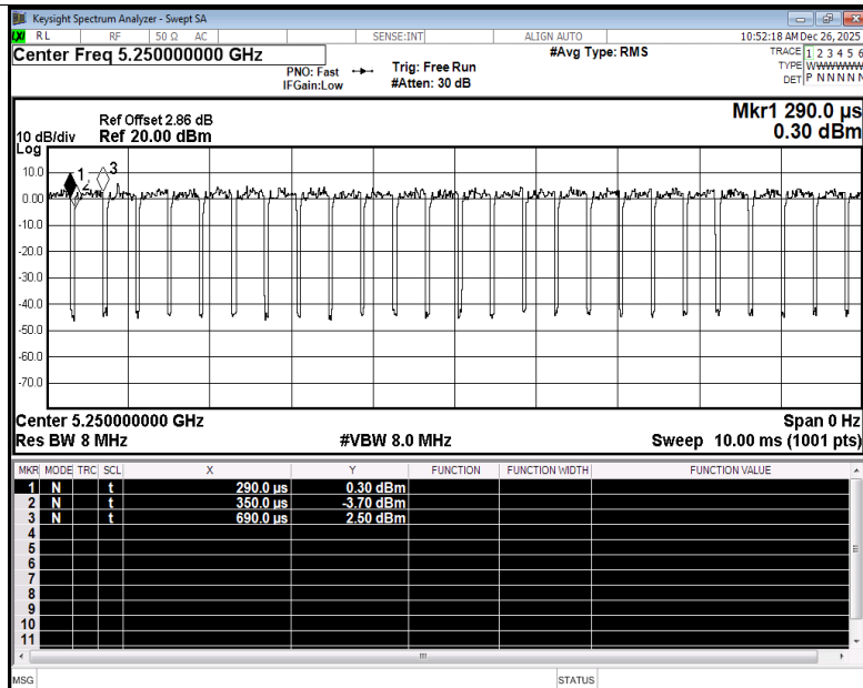
Duty Cycle NVNT ax160 5250MHz Ant3
