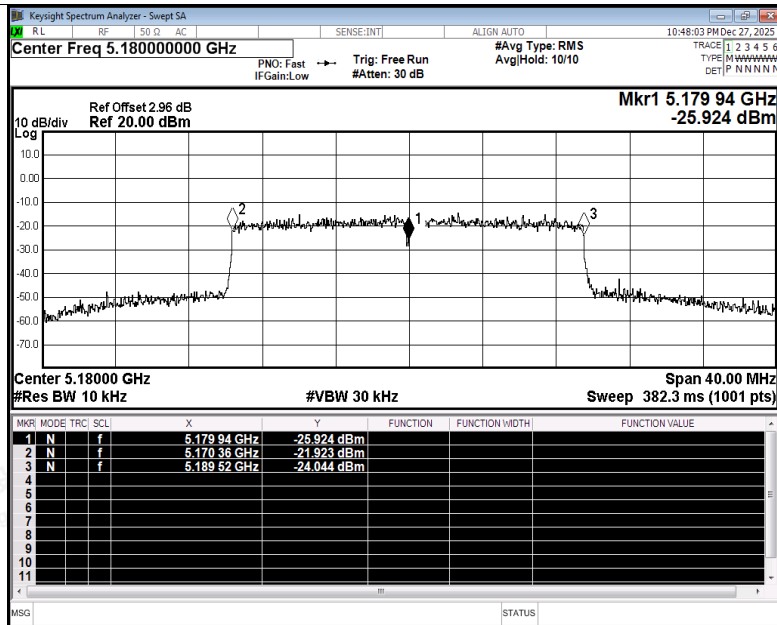
Freq. Stability NVNT be20 5180MHz Ant5
