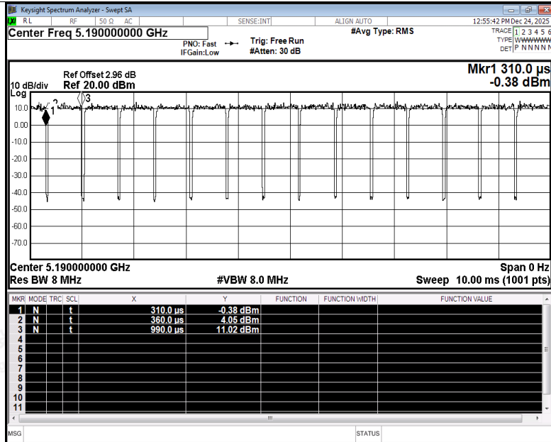
Duty Cycle NVNT n40 5190MHz Ant1
