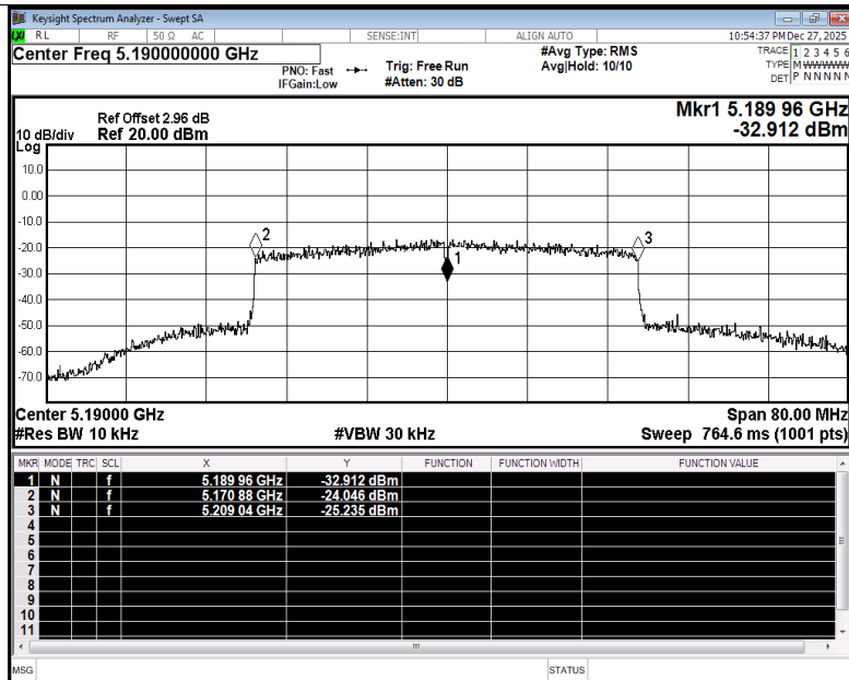
Freq. Stability NVNT be40 5190MHz Ant5
