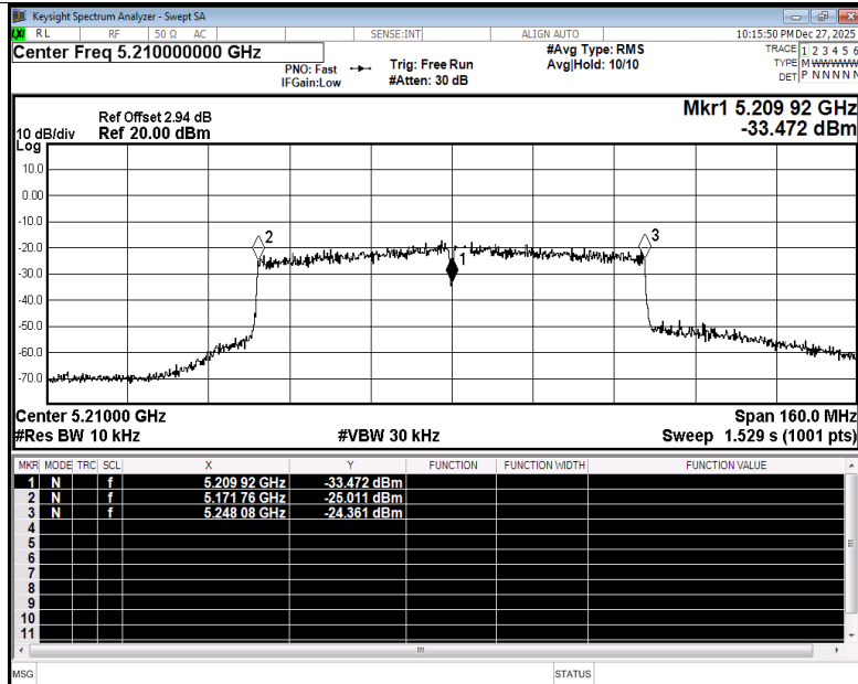
Freq. Stability NVNT ac80 5210MHz Ant5
