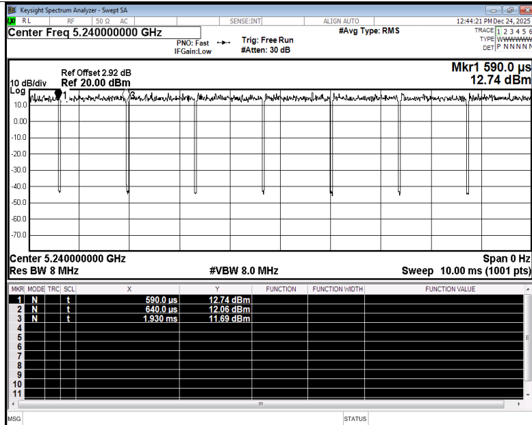
Duty Cycle NVNT n20 5240MHz Ant1
