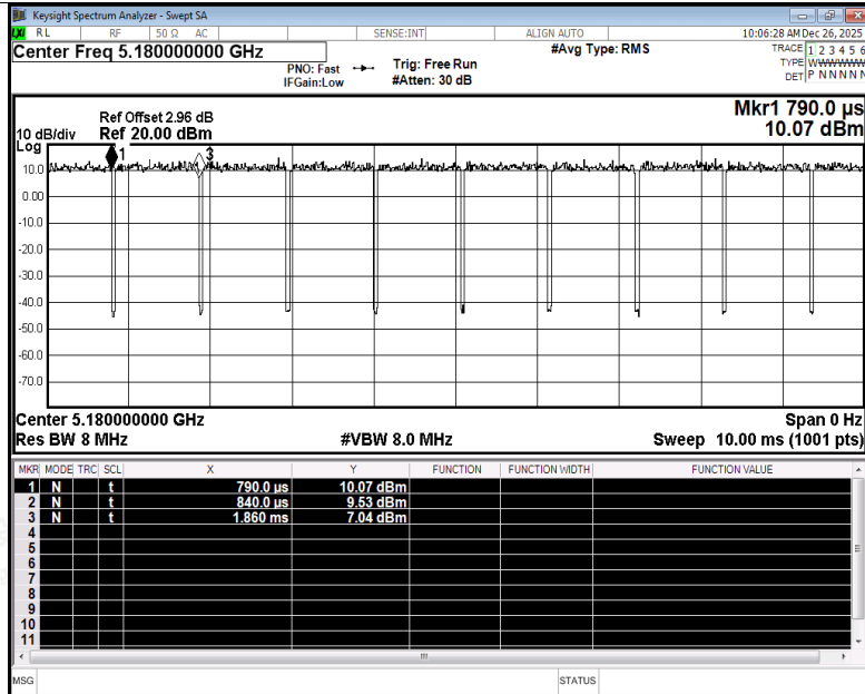
Duty Cycle NVNT ac20 5180MHz Ant3
