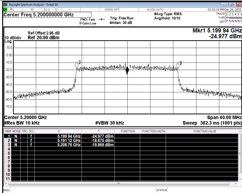
Freq. Stability NVNT ac20 5200MHz Ant5
