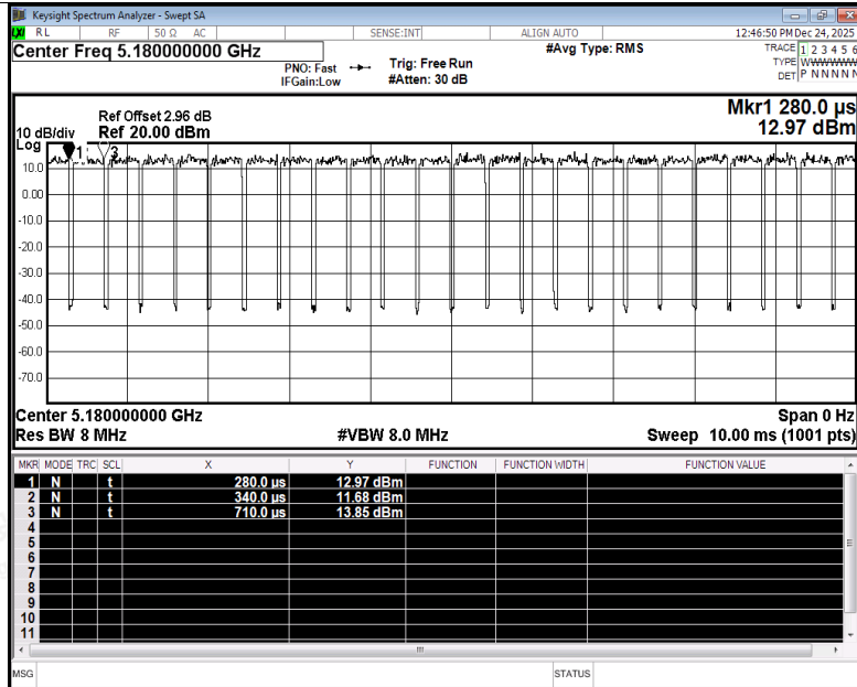
Duty Cycle NVNT ac20 5180MHz Ant1
