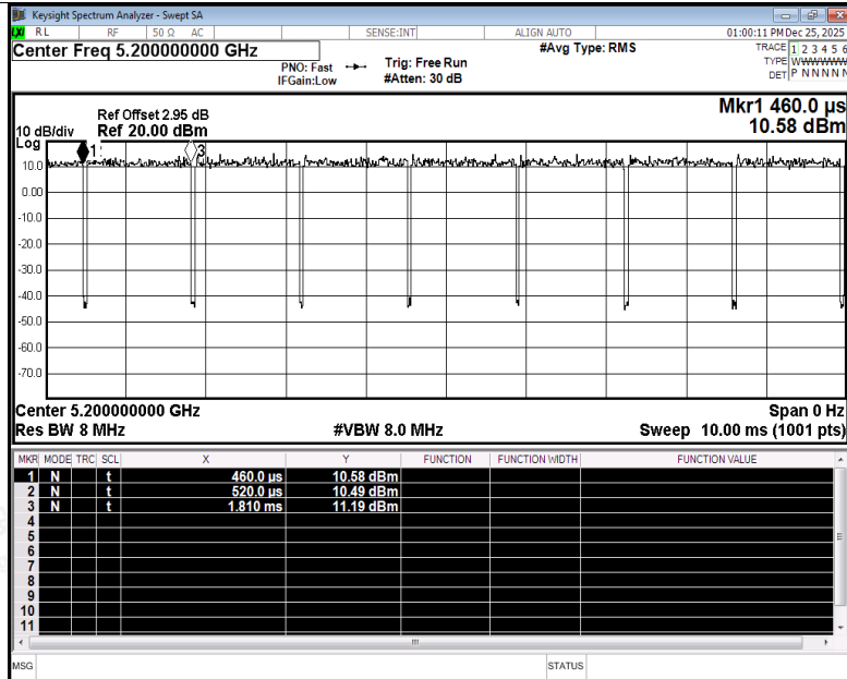
Duty Cycle NVNT n20 5200MHz Ant2
