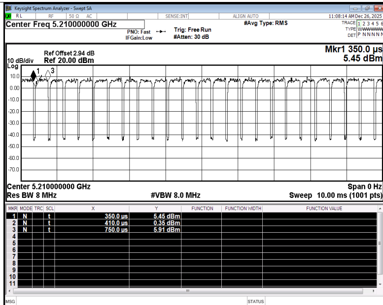
Duty Cycle NVNT be80 5210MHz Ant3
