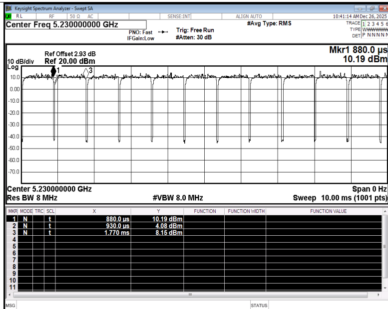
Duty Cycle NVNT ax40 5230MHz Ant3
