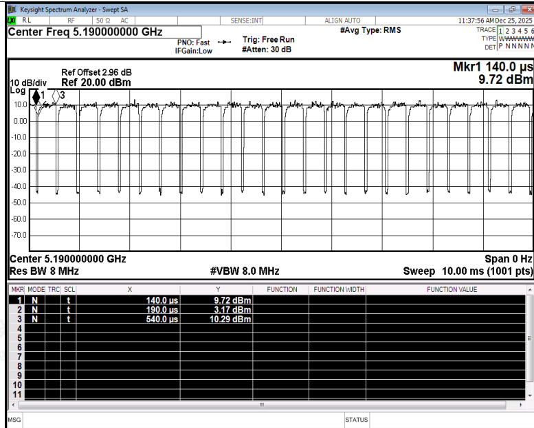
Duty Cycle NVNT ax40 5190MHz Ant1
