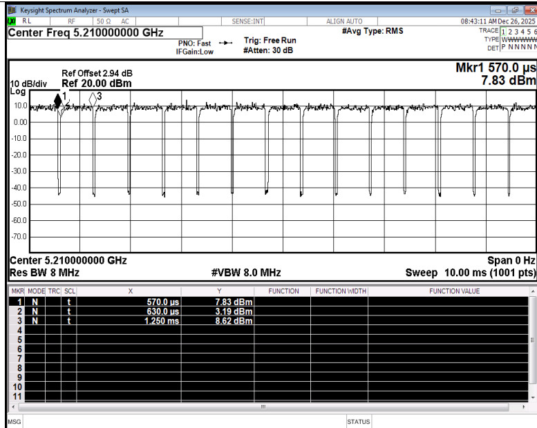
Duty Cycle NVNT ac80 5210MHz Ant2
