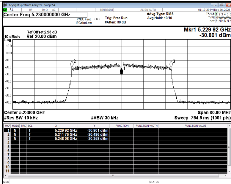
Freq. Stability NVNT n40 5230MHz Ant5
