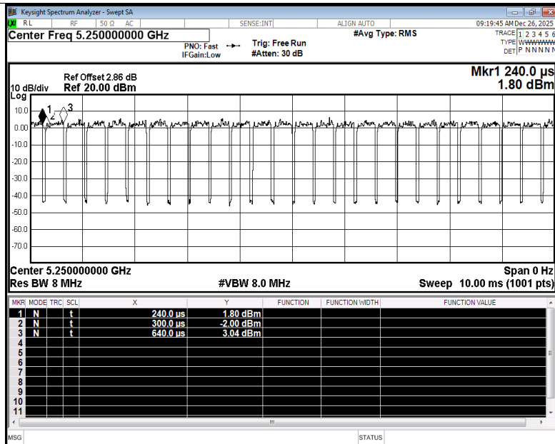
Duty Cycle NVNT ax160 5250MHz Ant2
