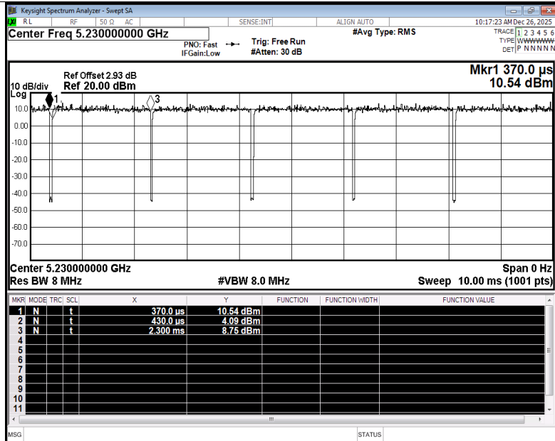
Duty Cycle NVNT n40 5230MHz Ant3
