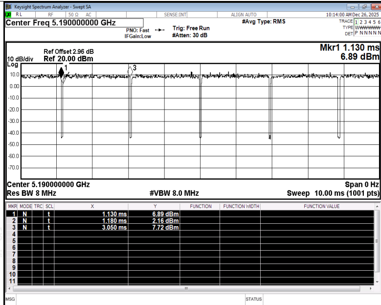
Duty Cycle NVNT n40 5190MHz Ant3
