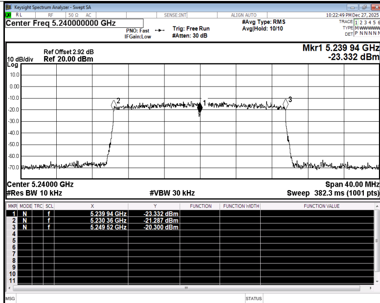
Freq. Stability NVNT ax20 5240MHz Ant5
