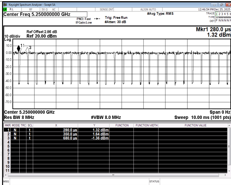
Duty Cycle NVNT ac160 5250MHz Ant1
