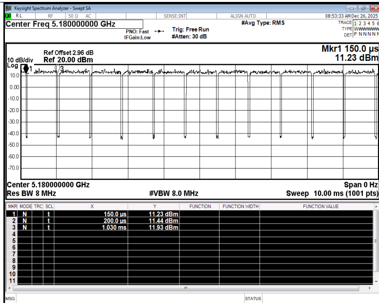
Duty Cycle NVNT ax20 5180MHz Ant2
