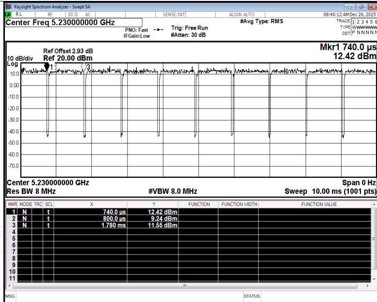
Duty Cycle NVNT ac40 5230MHz Ant2
