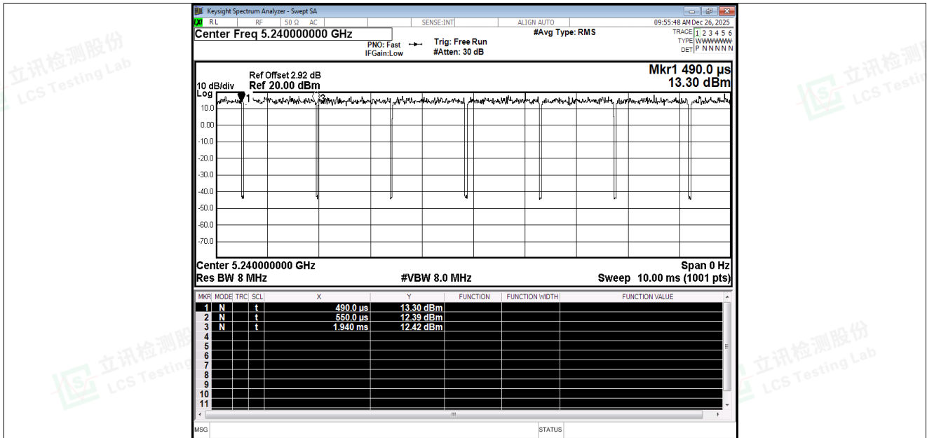
Duty Cycle NVNT a 5240MHz Ant3
