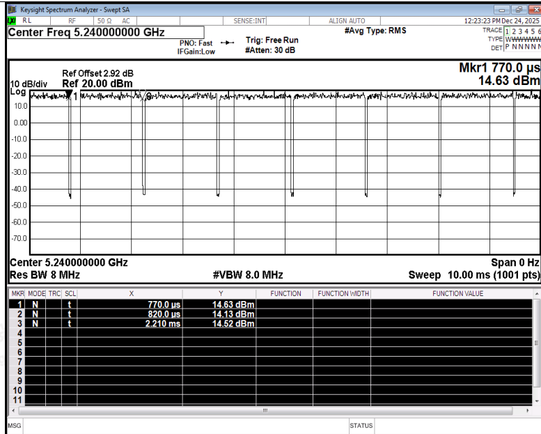
Duty Cycle NVNT a 5240MHz Ant1
