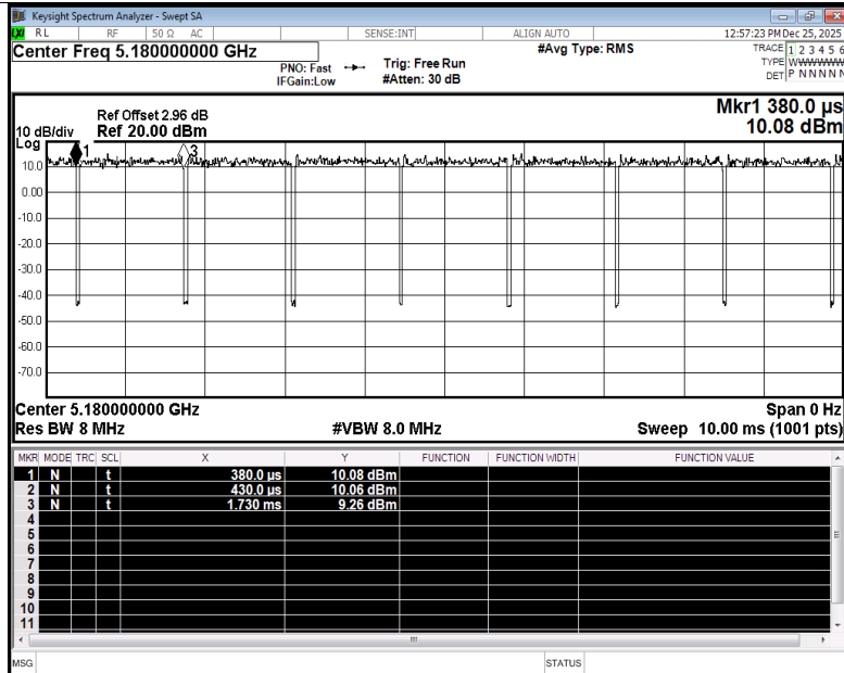
Duty Cycle NVNT n20 5180MHz Ant2
