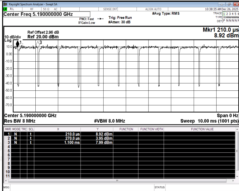
Duty Cycle NVNT ax40 5190MHz Ant3
