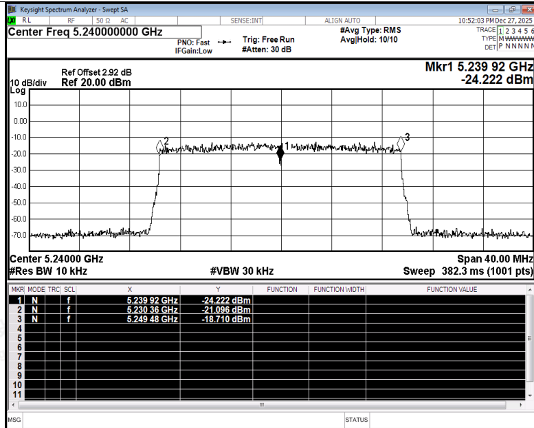
Freq. Stability NVNT be20 5240MHz Ant5
