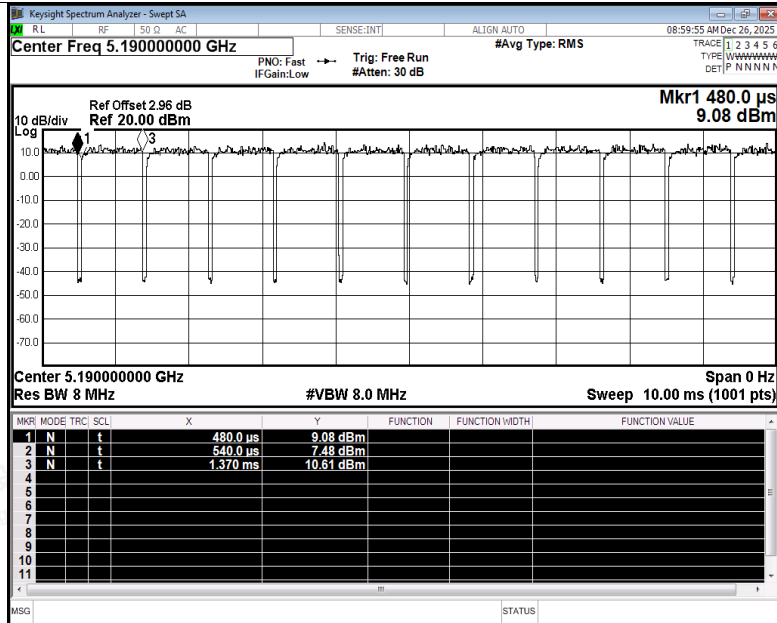
Duty Cycle NVNT ax40 5190MHz Ant2
