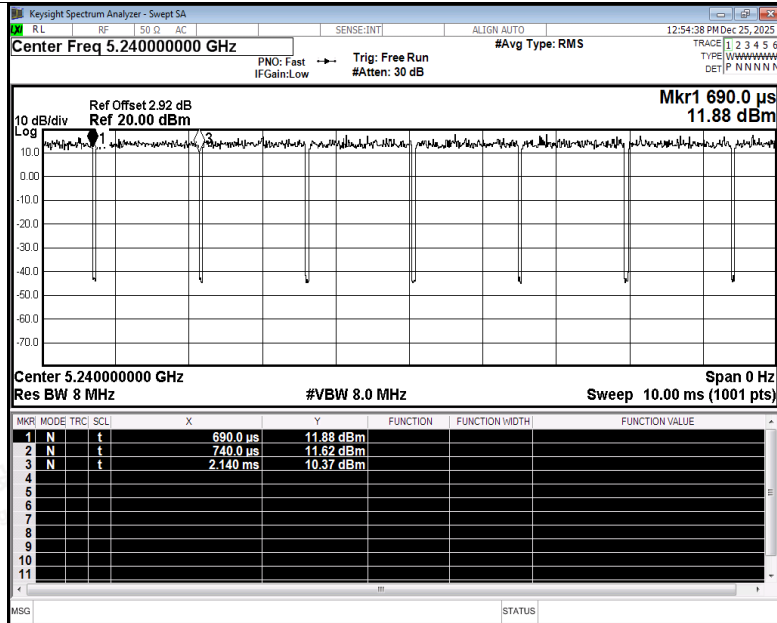
Duty Cycle NVNT a 5240MHz Ant2
