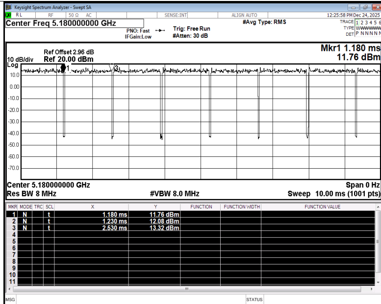
Duty Cycle NVNT n20 5180MHz Ant1
