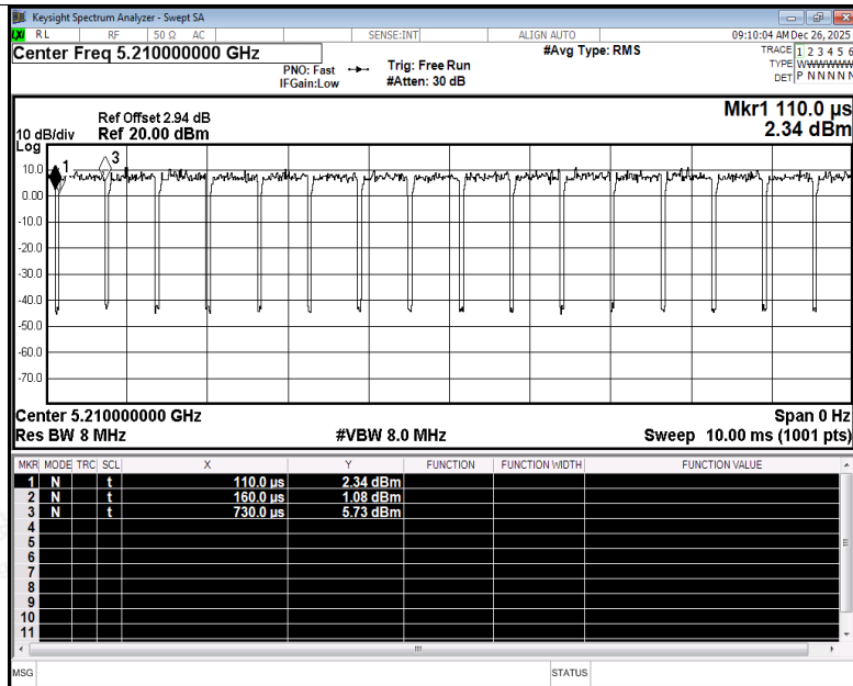
Duty Cycle NVNT ax80 5210MHz Ant2
