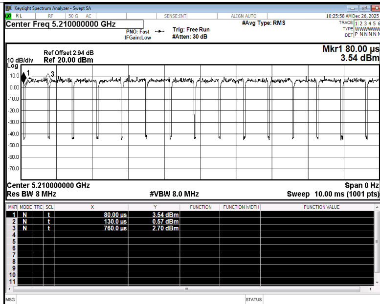
Duty Cycle NVNT ac80 5210MHz Ant3
