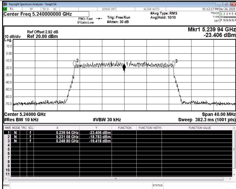
Freq. Stability NVNT ac20 5240MHz Ant5
