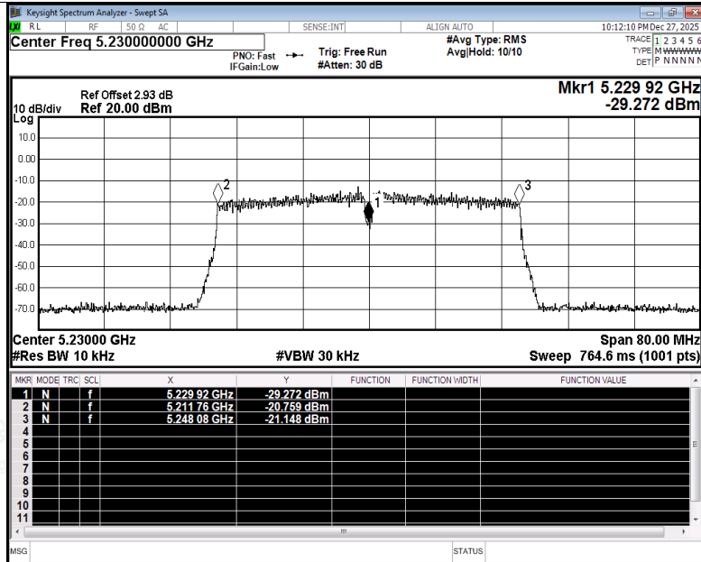
Freq. Stability NVNT ac40 5230MHz Ant5
