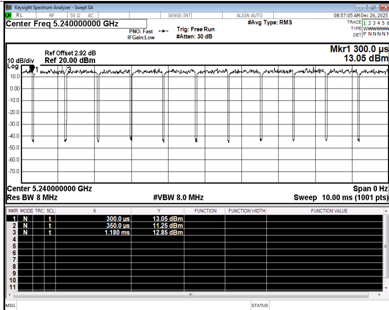
Duty Cycle NVNT ax20 5240MHz Ant2
