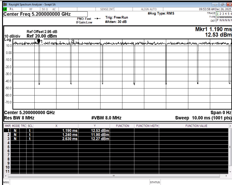
Duty Cycle NVNT a 5200MHz Ant3
