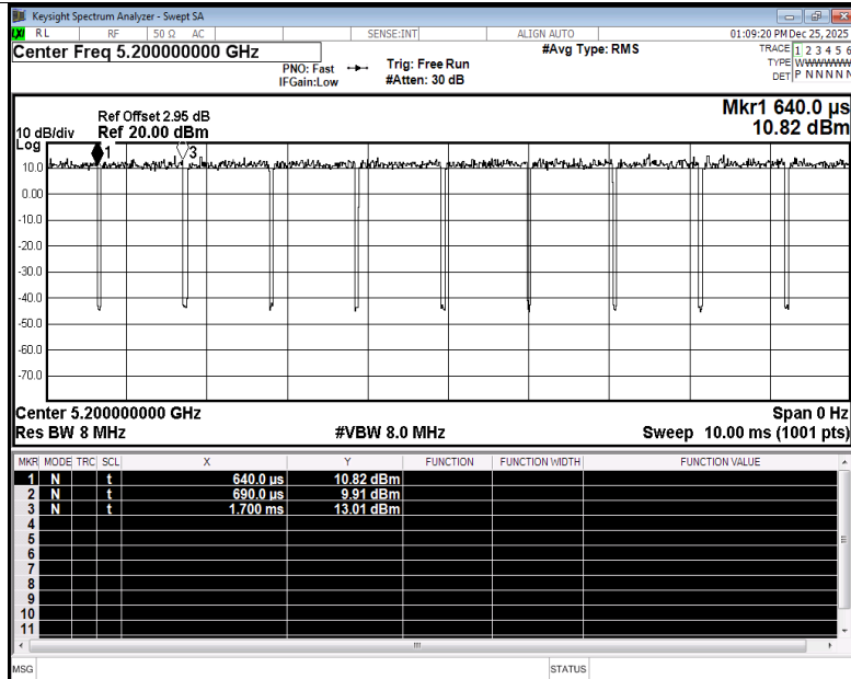
Duty Cycle NVNT ac20 5200MHz Ant2
