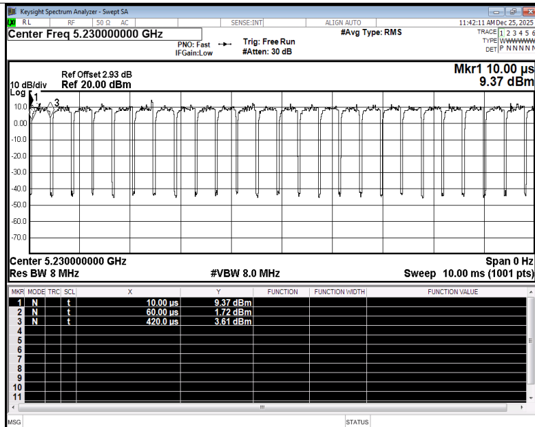
Duty Cycle NVNT ax40 5230MHz Ant1
