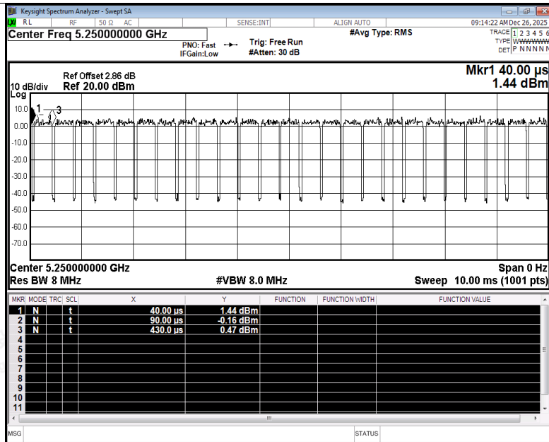
Duty Cycle NVNT ac160 5250MHz Ant2
