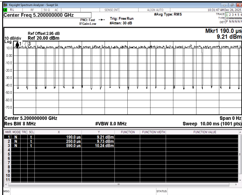
Duty Cycle NVNT ax20 5200MHz Ant3
