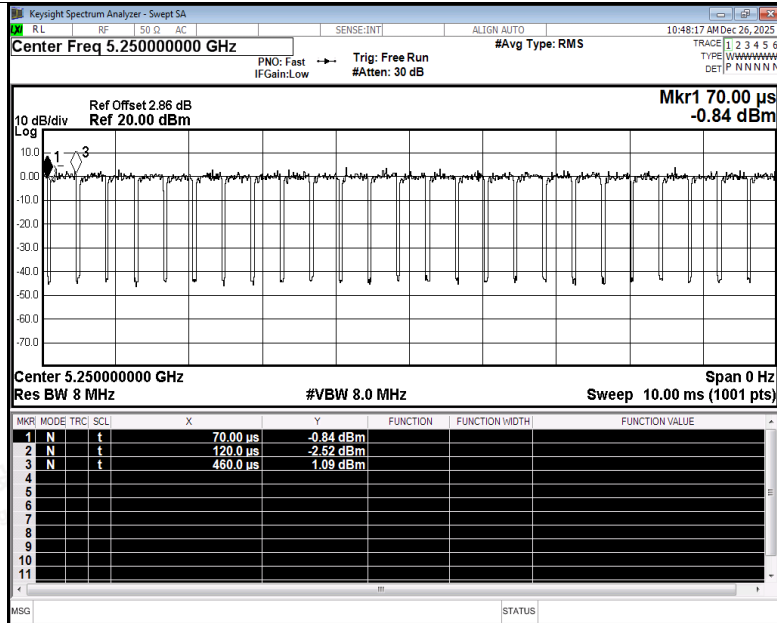
Duty Cycle NVNT ac160 5250MHz Ant3
