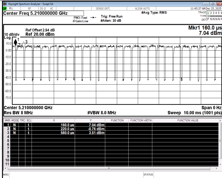
Duty Cycle NVNT ax80 5210MHz Ant1
