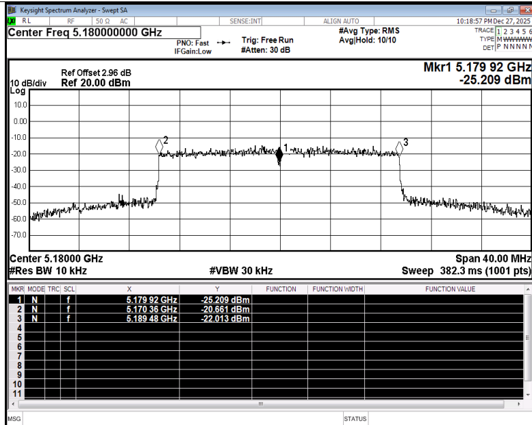
Freq. Stability NVNT ax20 5180MHz Ant5
