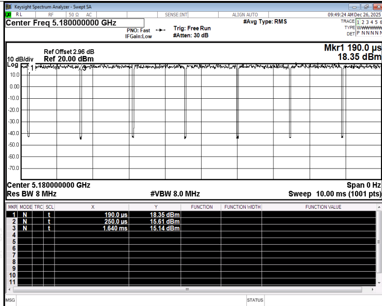
Duty Cycle NVNT a 5180MHz Ant3
