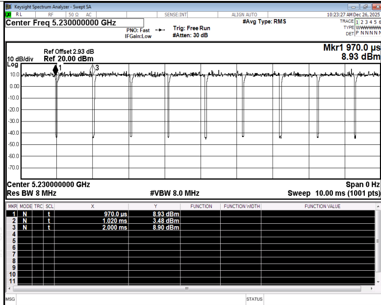
Duty Cycle NVNT ac40 5230MHz Ant3
