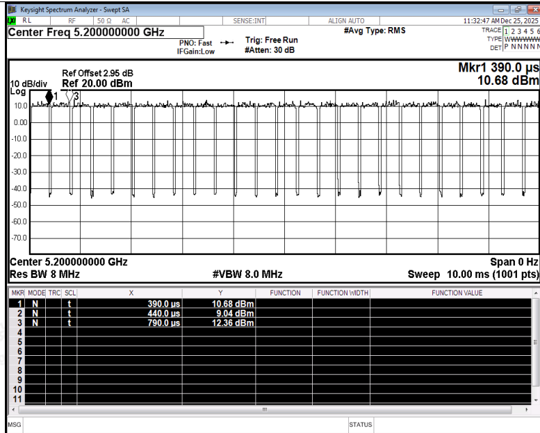
Duty Cycle NVNT ax20 5200MHz Ant1
