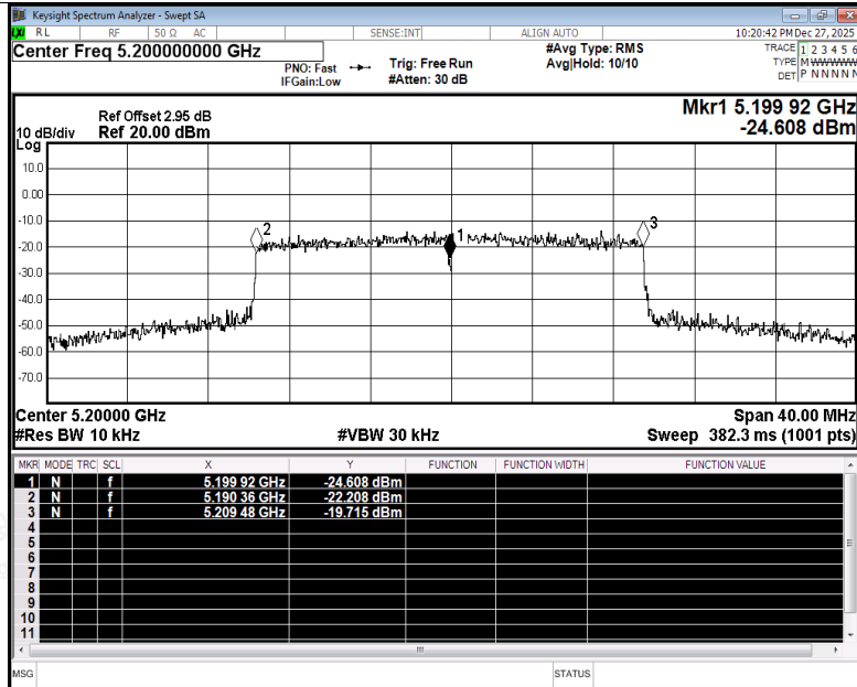
Freq. Stability NVNT ax20 5200MHz Ant5
