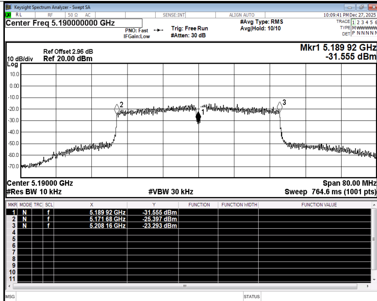
Freq. Stability NVNT ac40 5190MHz Ant5
