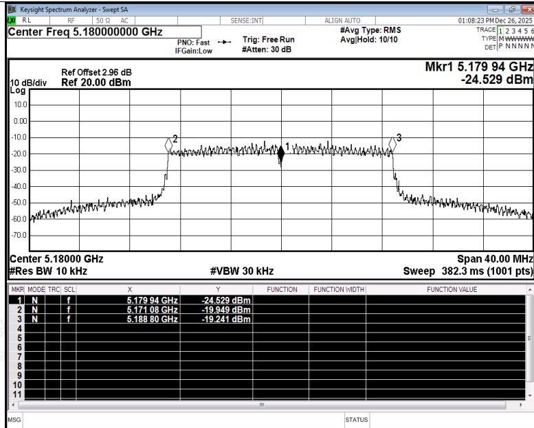
Freq. Stability NVNT ac20 5180MHz Ant5
