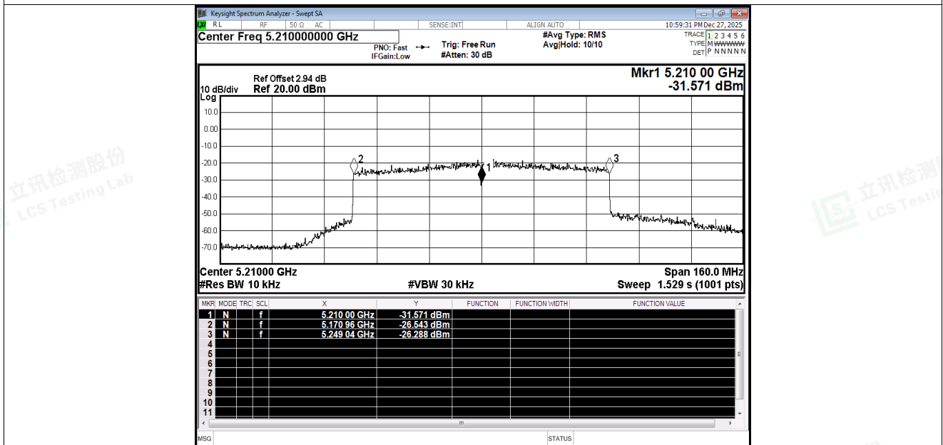
Freq. Stability NVNT be80 5210MHz Ant5
