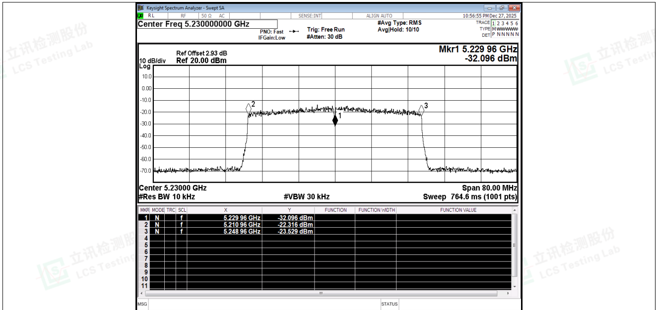
Freq. Stability NVNT be40 5230MHz Ant5
