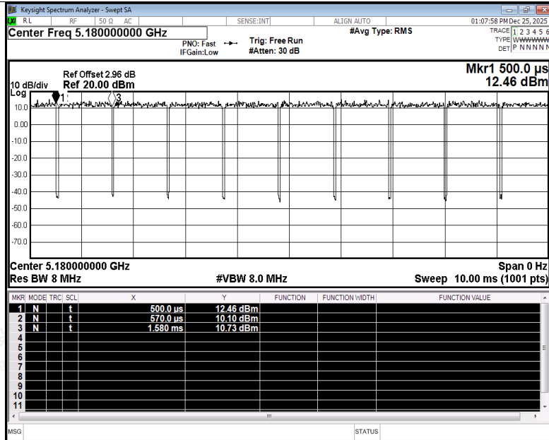
Duty Cycle NVNT ac20 5180MHz Ant2
