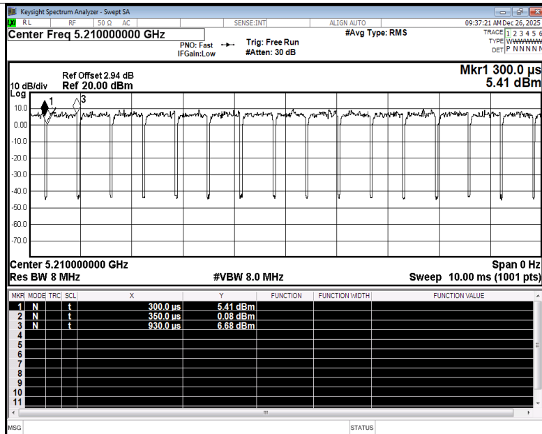
Duty Cycle NVNT be80 5210MHz Ant2
