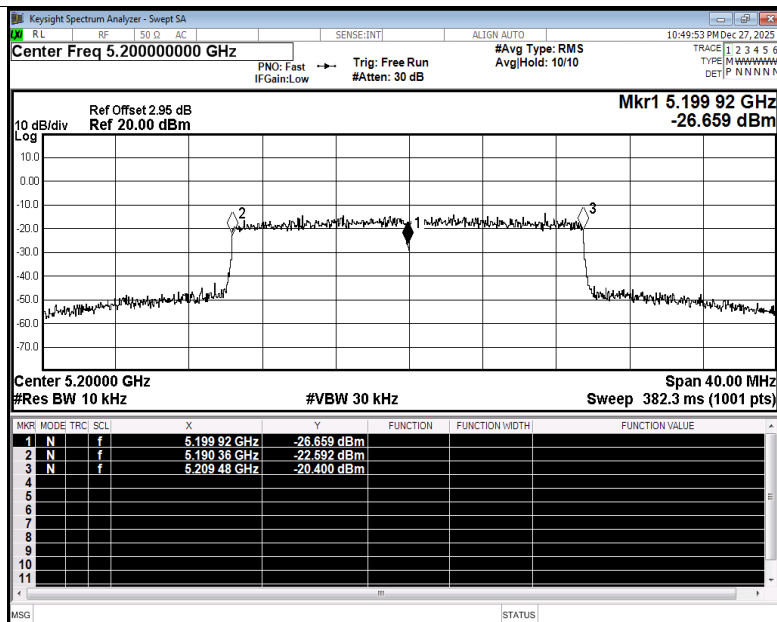
Freq. Stability NVNT be20 5200MHz Ant5
