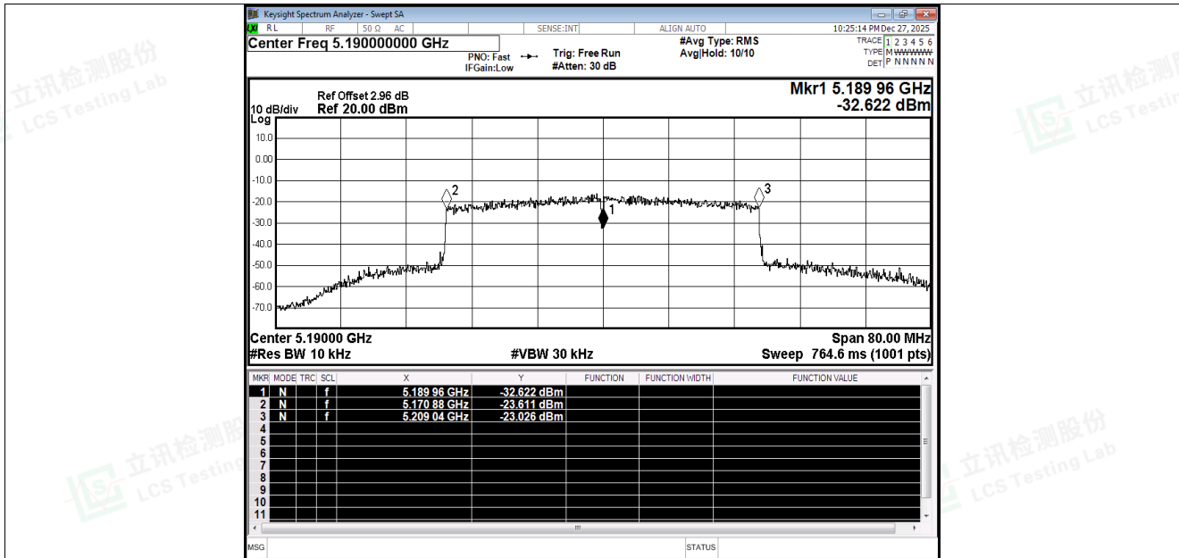
Freq. Stability NVNT ax40 5190MHz Ant5
