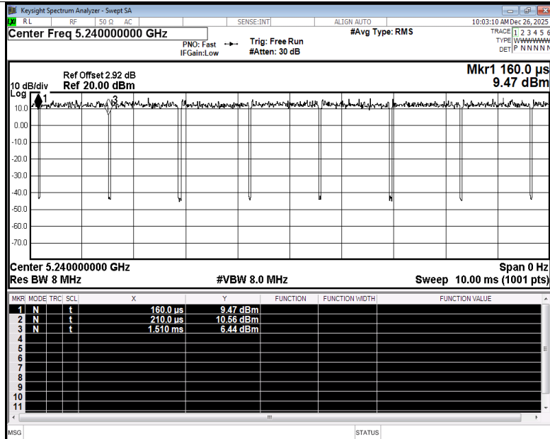
Duty Cycle NVNT n20 5240MHz Ant3
