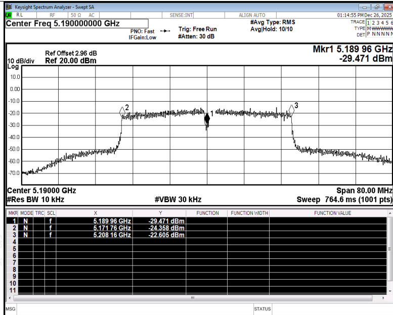
Freq. Stability NVNT n40 5190MHz Ant5
