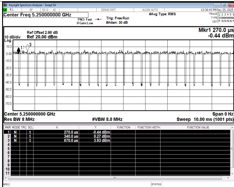
Duty Cycle NVNT ax160 5250MHz Ant1
