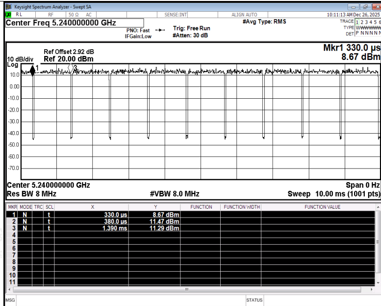
Duty Cycle NVNT ac20 5240MHz Ant3
