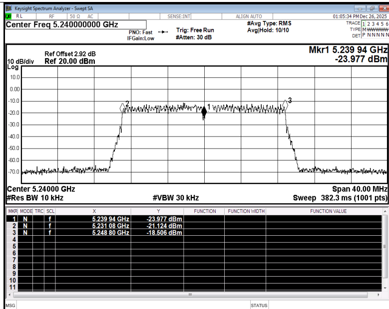
Freq. Stability NVNT n20 5240MHz Ant5
