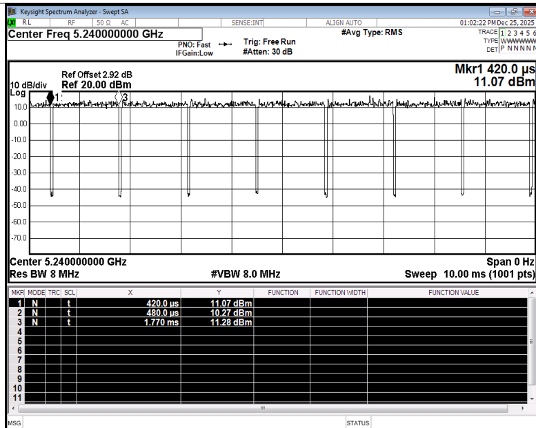
Duty Cycle NVNT n20 5240MHz Ant2
