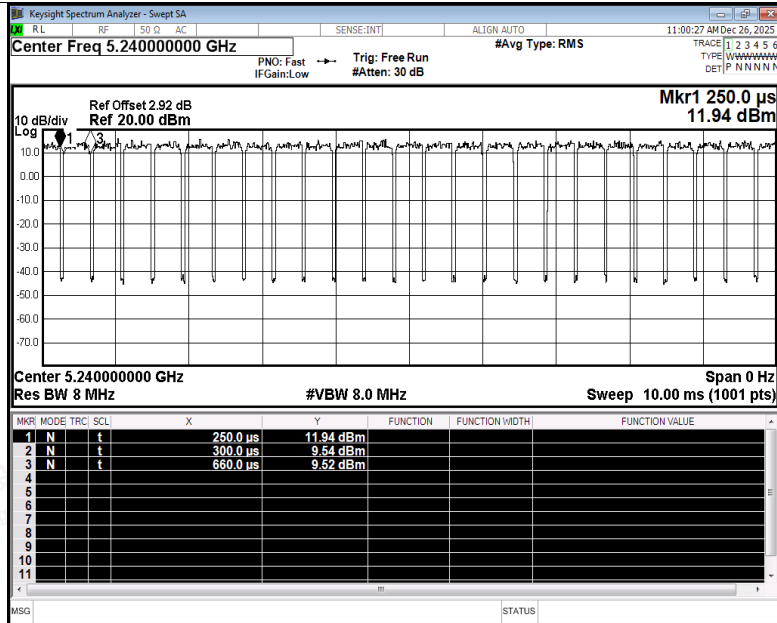
Duty Cycle NVNT be20 5240MHz Ant3
