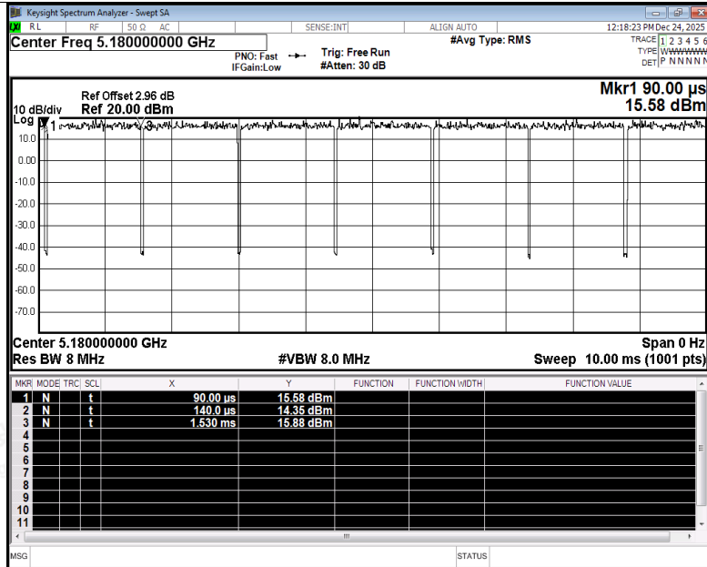
Duty Cycle NVNT a 5180MHz Ant1
