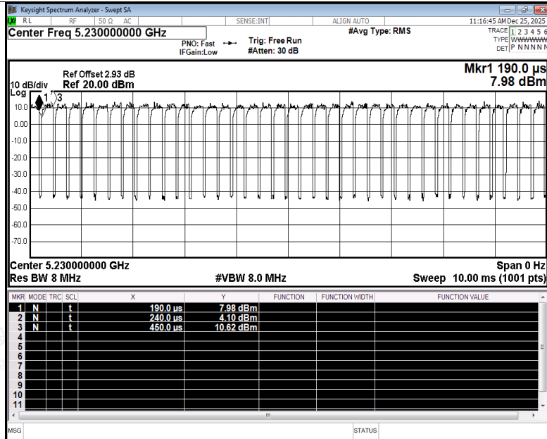
Duty Cycle NVNT ac40 5230MHz Ant1
