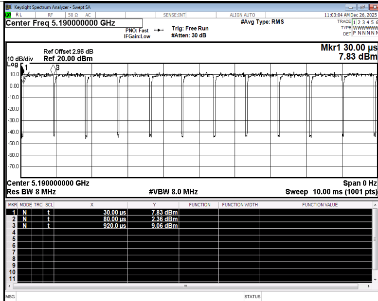
Duty Cycle NVNT be40 5190MHz Ant3
