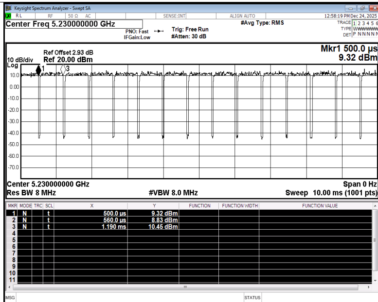
Duty Cycle NVNT n40 5230MHz Ant1
