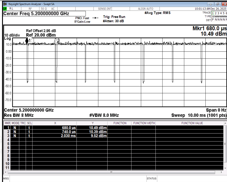
Duty Cycle NVNT n20 5200MHz Ant3
