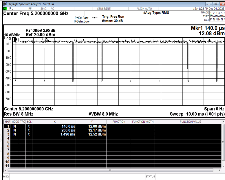
Duty Cycle NVNT n20 5200MHz Ant1
