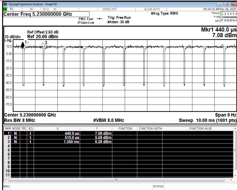
Duty Cycle NVNT be40 5230MHz Ant2
