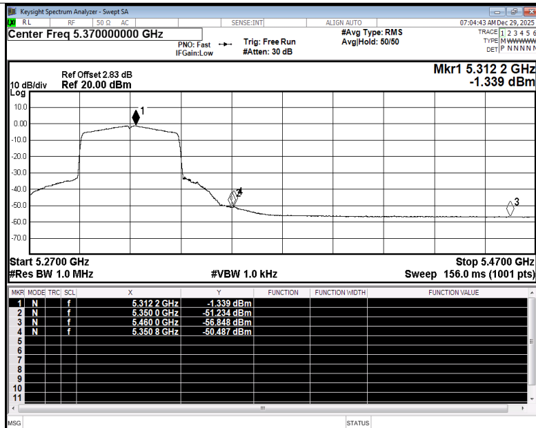
Restrict Band NVNT be40 5310MHz Ant3 Average
