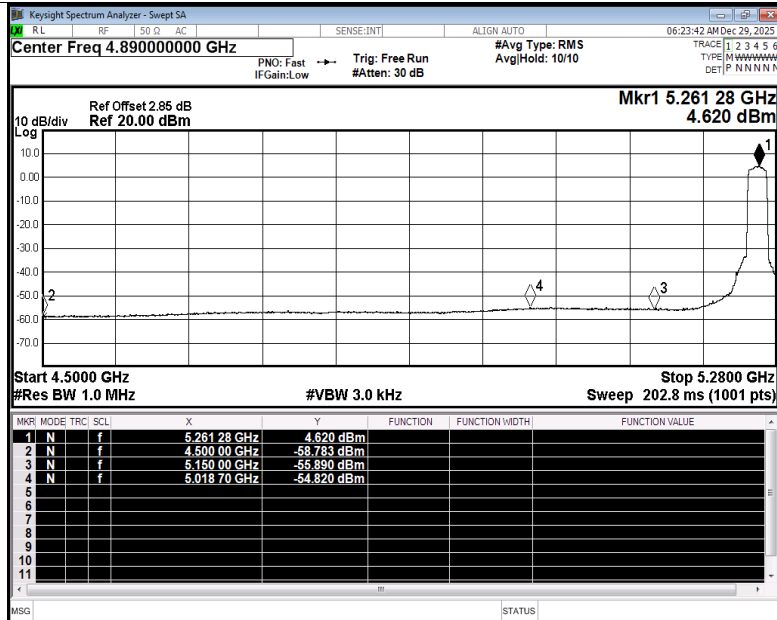
Restrict Band NVNT be20 5260MHz Ant2 Average
