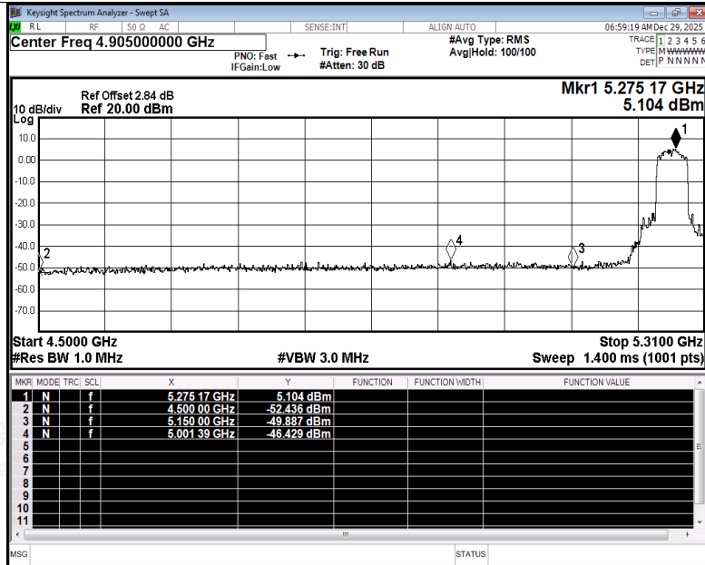
Restrict Band NVNT ac40 5270MHz Ant3 Peak
