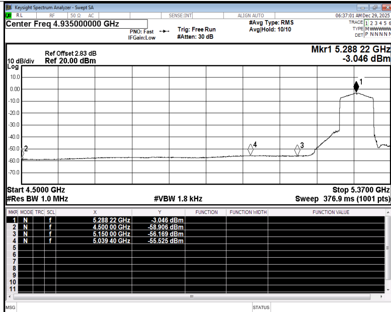
Restrict Band NVNT be80 5290MHz Ant2 Average
