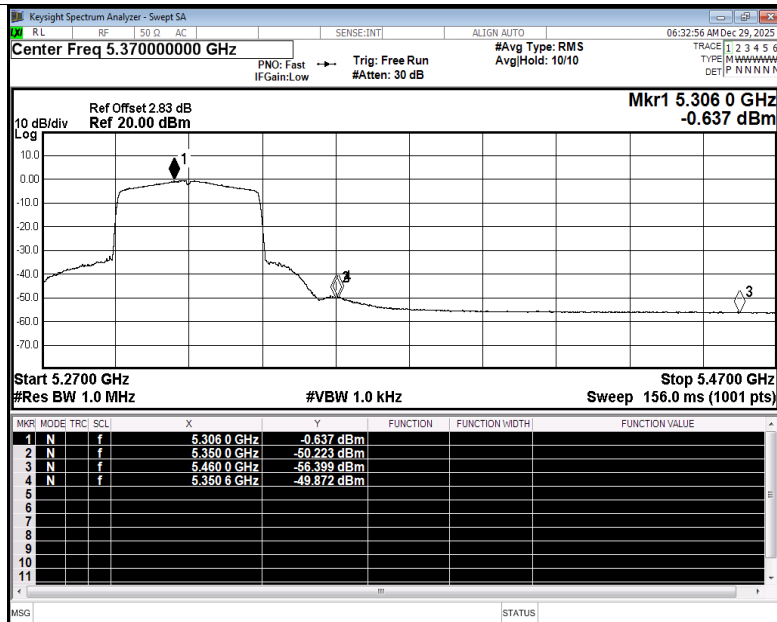
Restrict Band NVNT be40 5310MHz Ant2 Average
