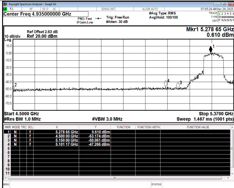
Restrict Band NVNT ac80 5290MHz Ant3 Peak
