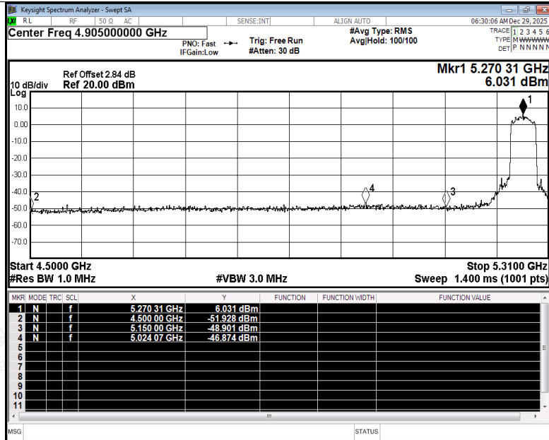
Restrict Band NVNT ax40 5270MHz Ant2 Peak
