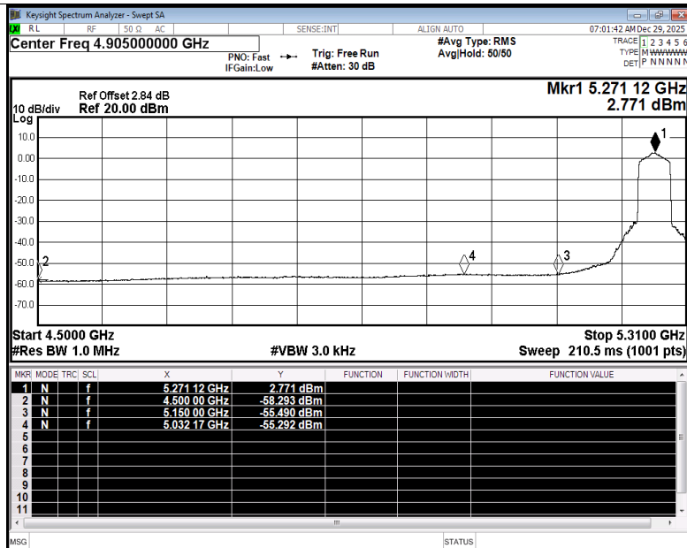
Restrict Band NVNT ax40 5270MHz Ant3 Average
