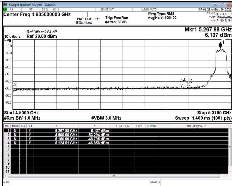
Restrict Band NVNT ax40 5270MHz Ant3 Peak
