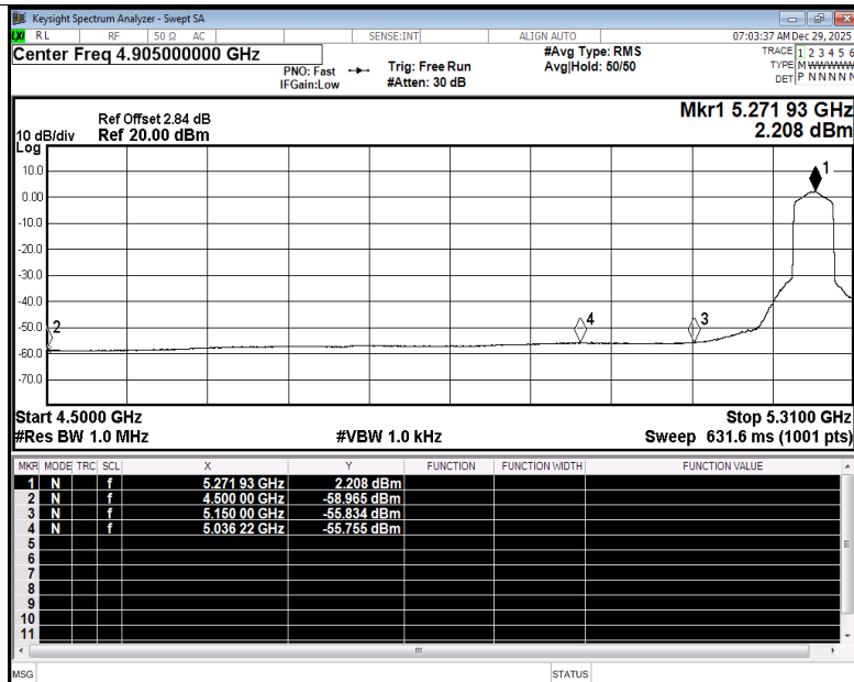
Restrict Band NVNT be40 5270MHz Ant3 Average
