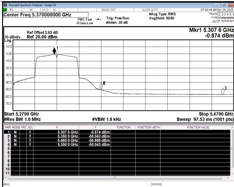
Restrict Band NVNT ac40 5310MHz Ant3 Average
