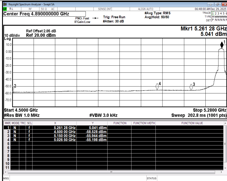
Restrict Band NVNT ax20 5260MHz Ant3 Average
