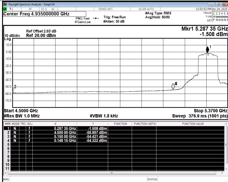
Restrict Band NVNT ac80 5290MHz Ant1 Average
