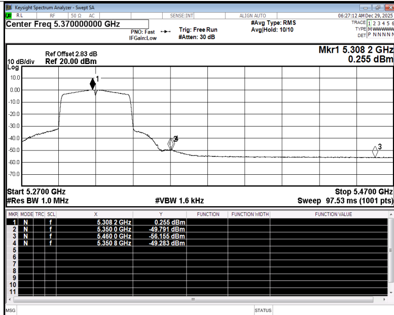
Restrict Band NVNT n40 5310MHz Ant2 Average
