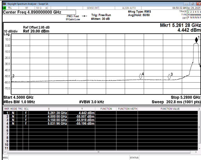
Restrict Band NVNT be20 5260MHz Ant3 Average
