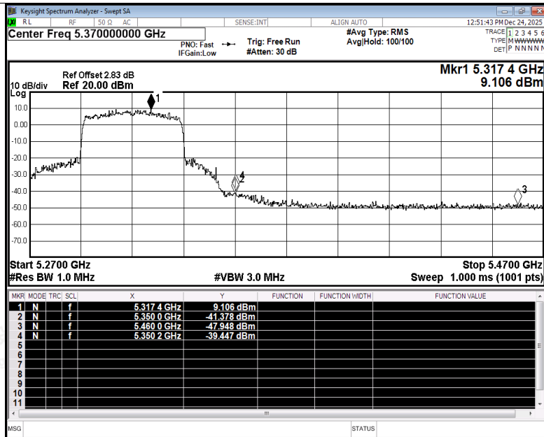
Restrict Band NVNT be40 5310MHz Ant1 Peak
