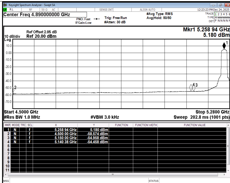
Restrict Band NVNT ax20 5260MHz Ant1 Average
