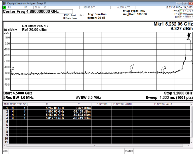
Restrict Band NVNT be20 5260MHz Ant1 Peak
