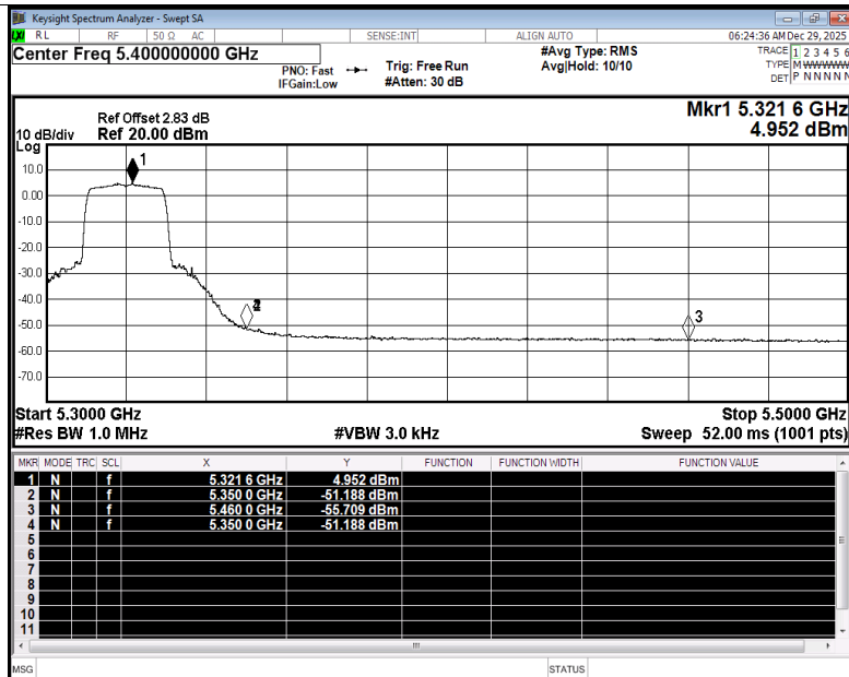
Restrict Band NVNT be20 5320MHz Ant2 Average
