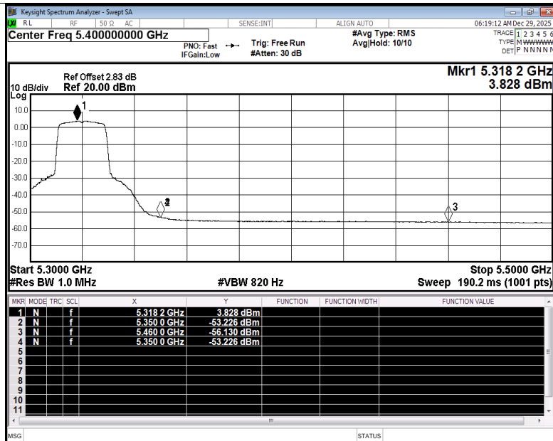
Restrict Band NVNT n20 5320MHz Ant2 Average
