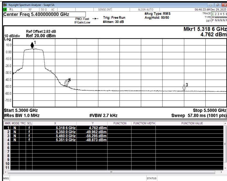
Restrict Band NVNT ac20 5320MHz Ant3 Average
