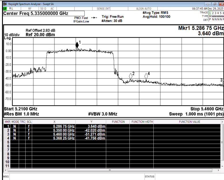
Restrict Band NVNT be80 5290MHz Ant2 Peak
