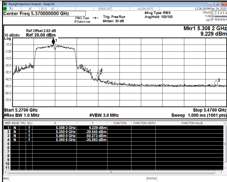
Restrict Band NVNT ac40 5310MHz Ant1 Peak
