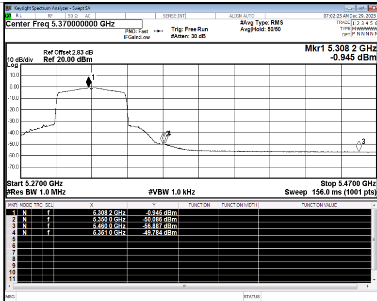
Restrict Band NVNT ax40 5310MHz Ant3 Average
