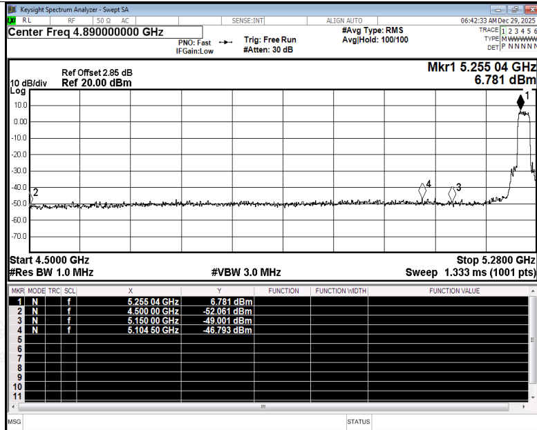
Restrict Band NVNT n20 5260MHz Ant3 Peak
