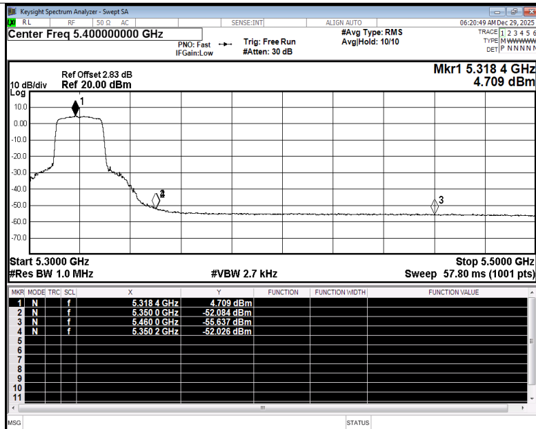
Restrict Band NVNT ac20 5320MHz Ant2 Average
