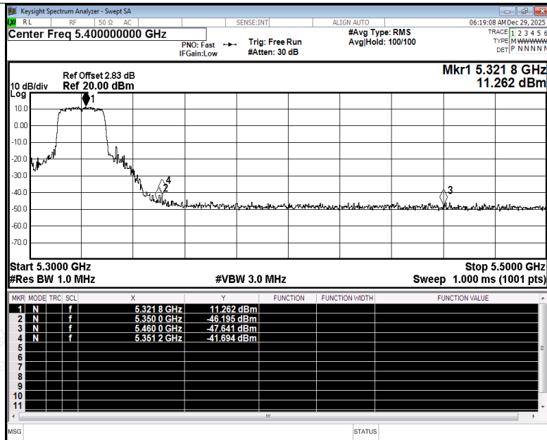
Restrict Band NVNT n20 5320MHz Ant2 Peak
