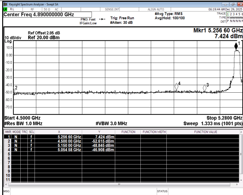
Restrict Band NVNT ac20 5260MHz Ant2 Peak
