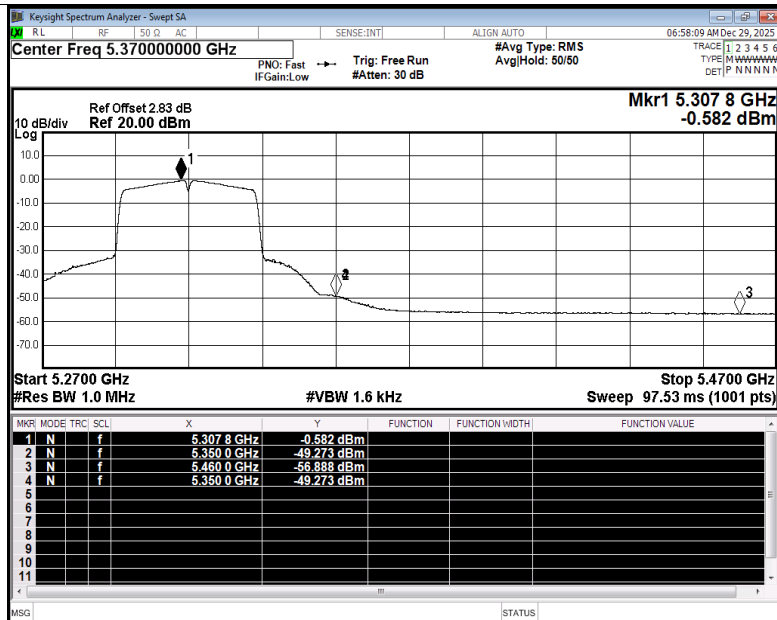
Restrict Band NVNT n40 5310MHz Ant3 Average
