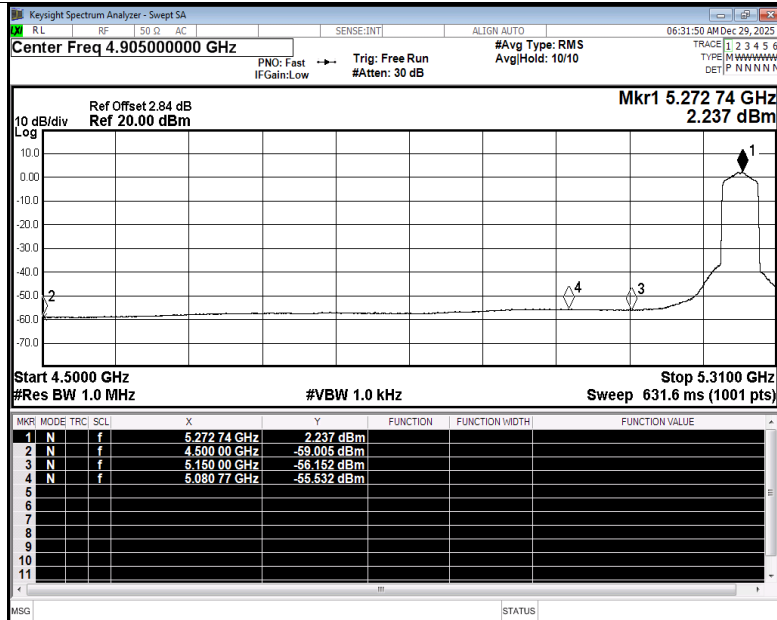
Restrict Band NVNT be40 5270MHz Ant2 Average
