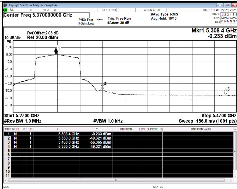
Restrict Band NVNT ax40 5310MHz Ant2 Average
