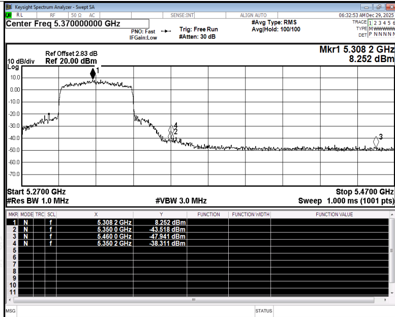
Restrict Band NVNT be40 5310MHz Ant2 Peak
