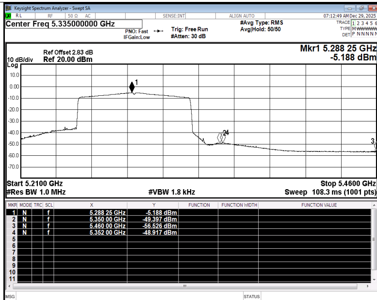
Restrict Band NVNT ax80 5290MHz Ant3 Average
