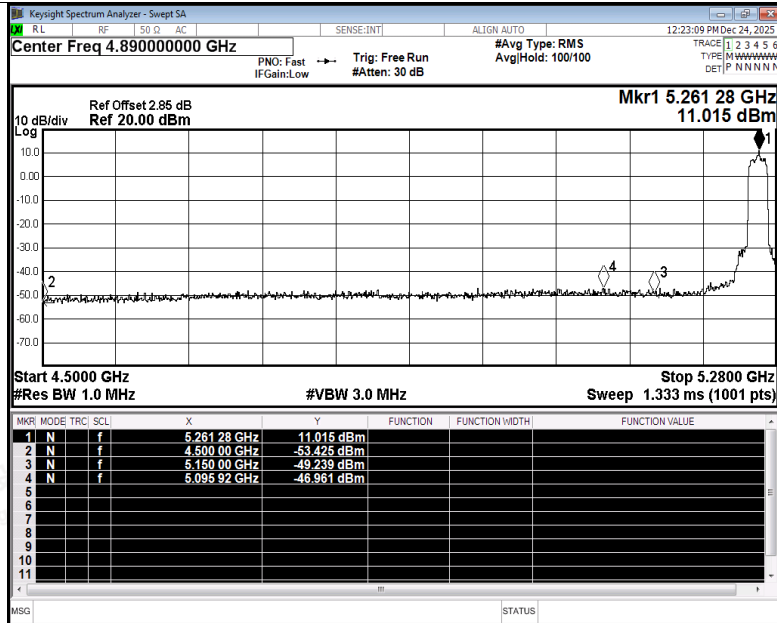
Restrict Band NVNT ax20 5260MHz Ant1 Peak
