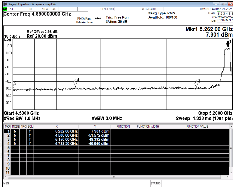
Restrict Band NVNT be20 5260MHz Ant3 Peak
