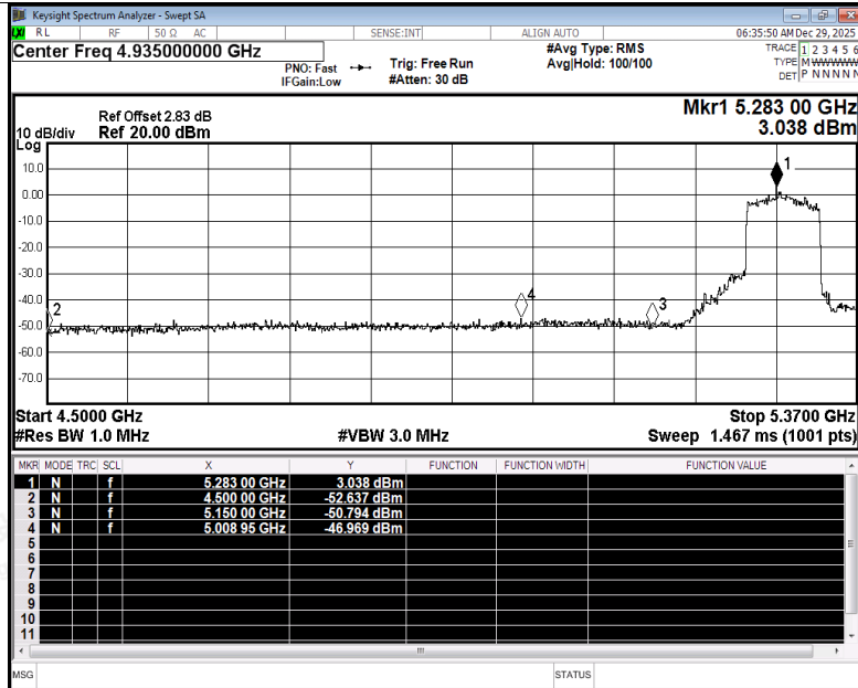
Restrict Band NVNT ax80 5290MHz Ant2 Peak
