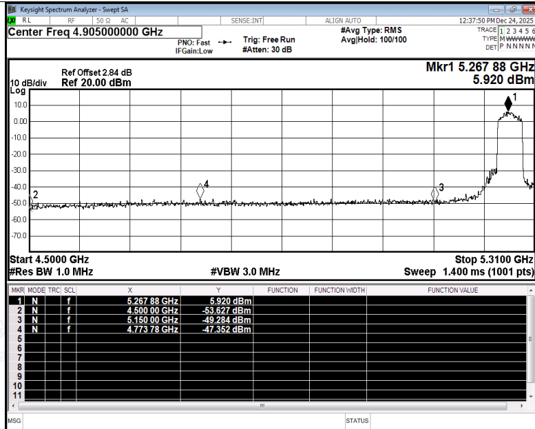
Restrict Band NVNT ax40 5270MHz Ant1 Peak
