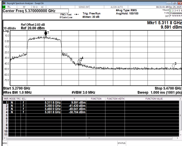
Restrict Band NVNT ax40 5310MHz Ant2 Peak
