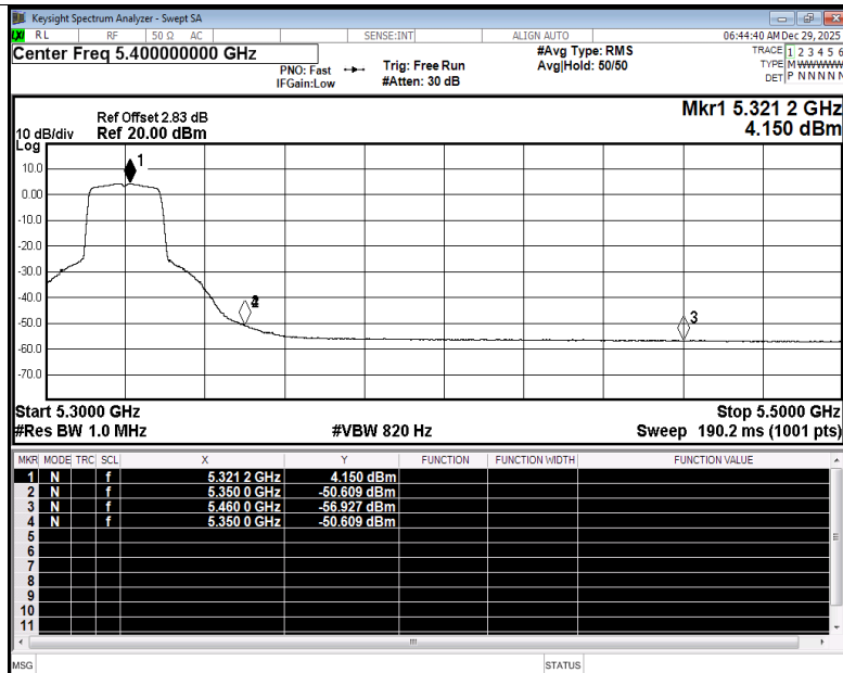
Restrict Band NVNT n20 5320MHz Ant3 Average
