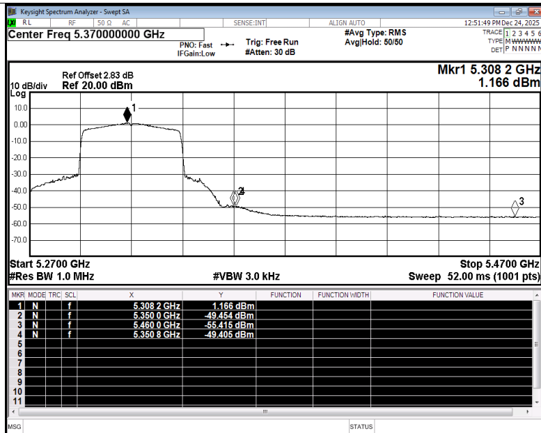
Restrict Band NVNT be40 5310MHz Ant1 Average
