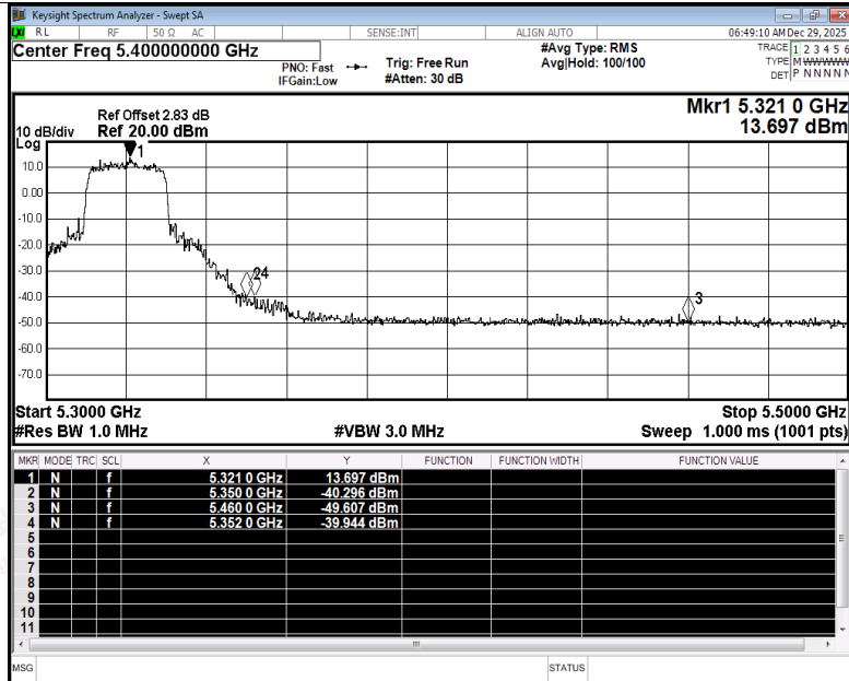
Restrict Band NVNT ax20 5320MHz Ant3 Peak
