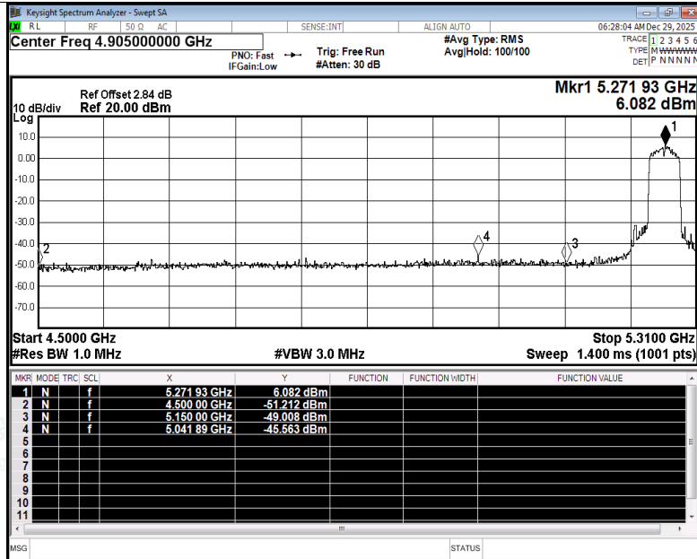
Restrict Band NVNT ac40 5270MHz Ant2 Peak
