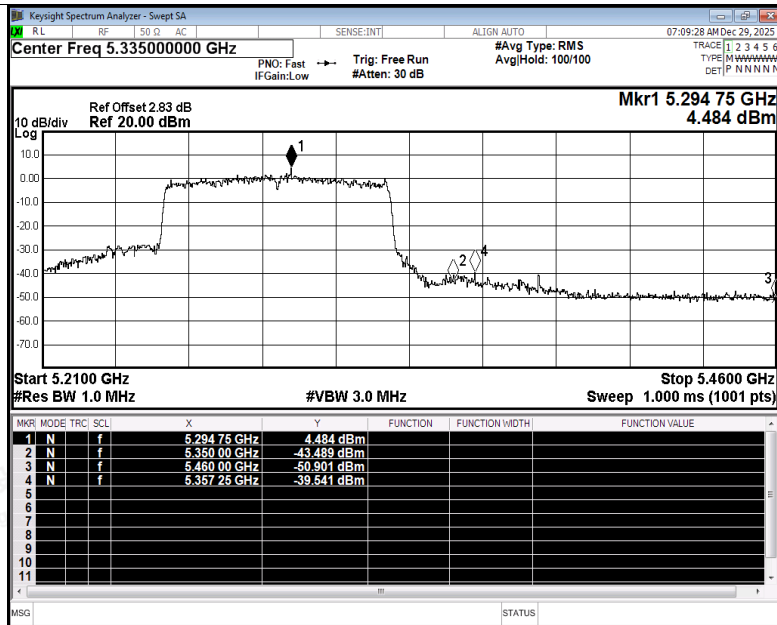
Restrict Band NVNT ac80 5290MHz Ant3 Peak
