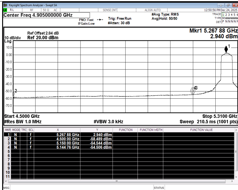
Restrict Band NVNT be40 5270MHz Ant1 Average
