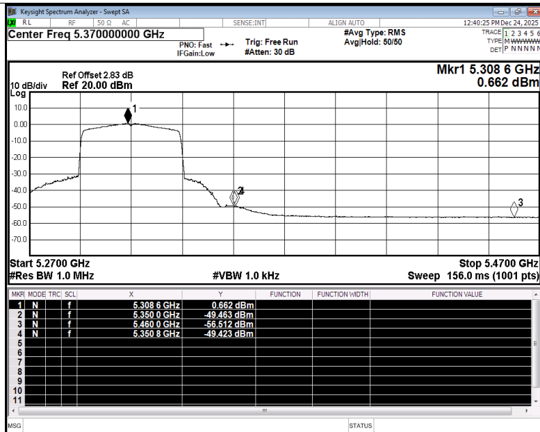
Restrict Band NVNT ax40 5310MHz Ant1 Average
