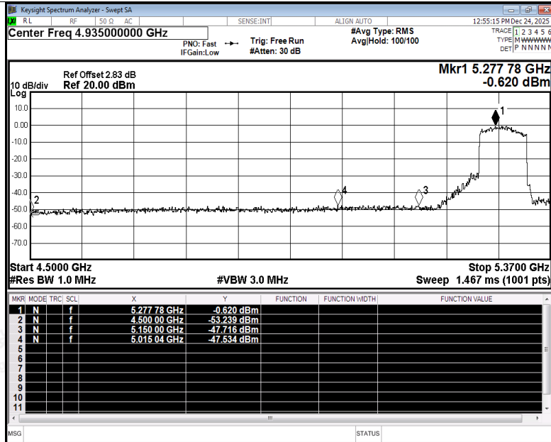
Restrict Band NVNT ax80 5290MHz Ant1 Peak
