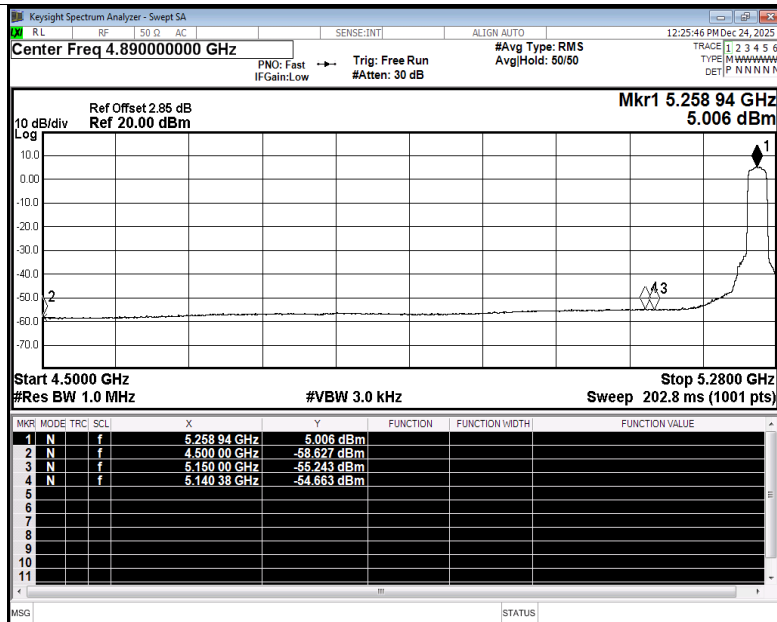
Restrict Band NVNT be20 5260MHz Ant1 Average
