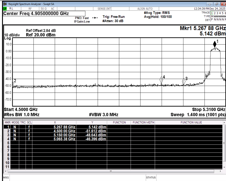
Restrict Band NVNT ac40 5270MHz Ant1 Peak
