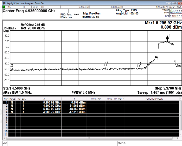
Restrict Band NVNT be80 5290MHz Ant1 Peak
