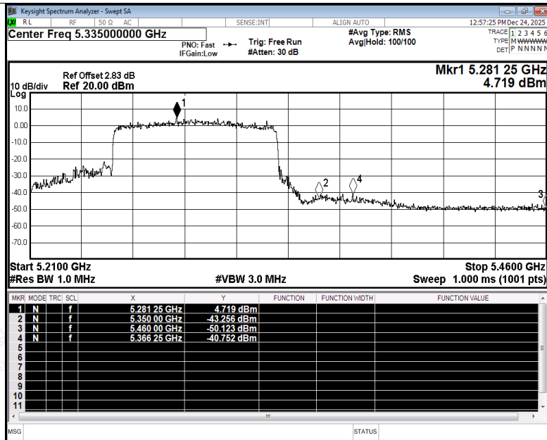
Restrict Band NVNT be80 5290MHz Ant1 Peak
