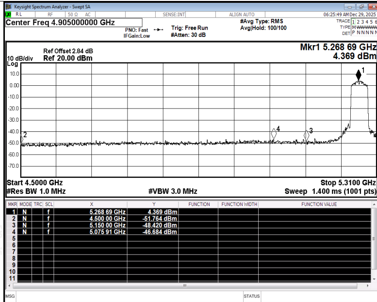
Restrict Band NVNT n40 5270MHz Ant2 Peak
