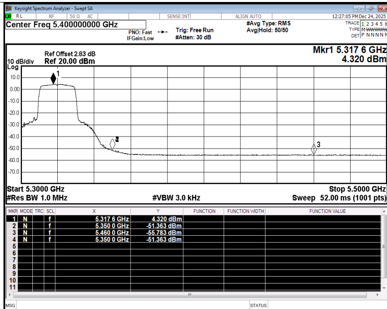
Restrict Band NVNT be20 5320MHz Ant1 Average
