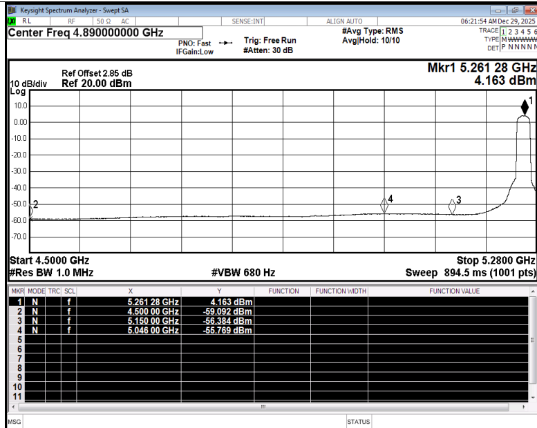
Restrict Band NVNT ax20 5260MHz Ant2 Average
