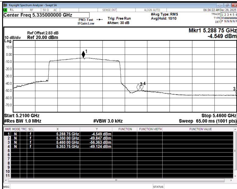
Restrict Band NVNT ax80 5290MHz Ant2 Average
