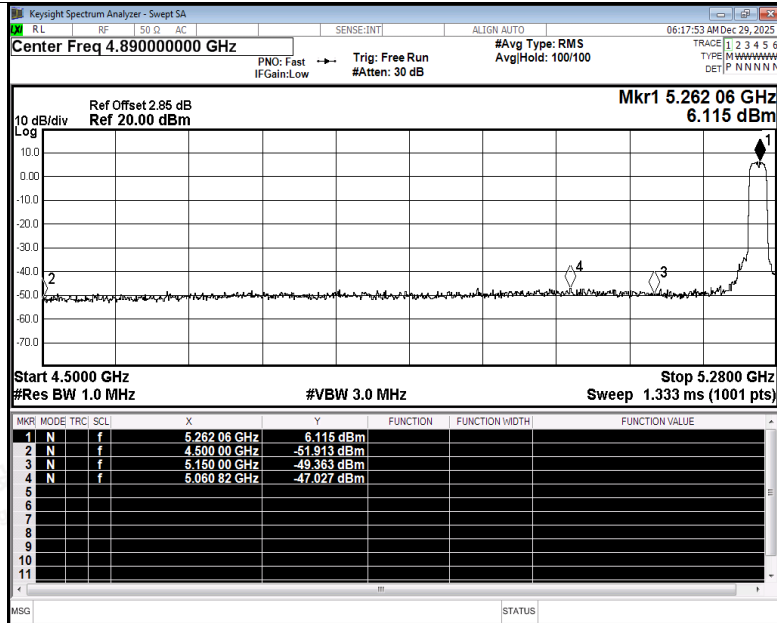
Restrict Band NVNT n20 5260MHz Ant2 Peak
