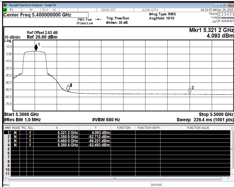
Restrict Band NVNT ax20 5320MHz Ant2 Average
