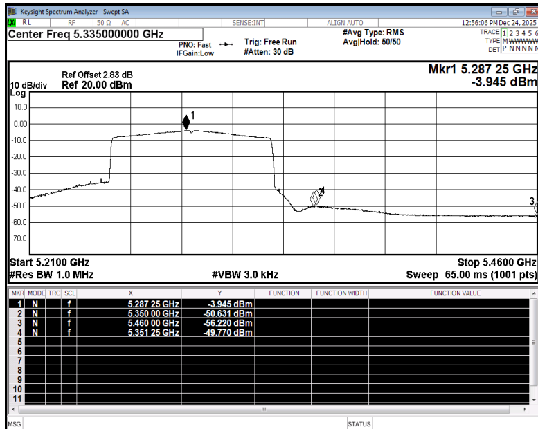
Restrict Band NVNT ax80 5290MHz Ant1 Average
