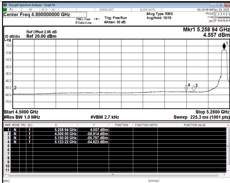
Restrict Band NVNT ac20 5260MHz Ant2 Average
