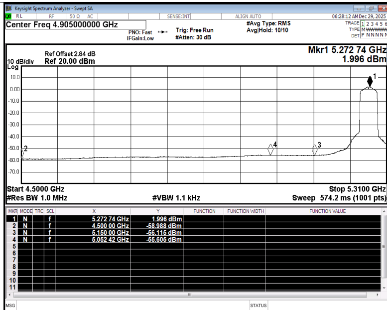
Restrict Band NVNT ac40 5270MHz Ant2 Average
