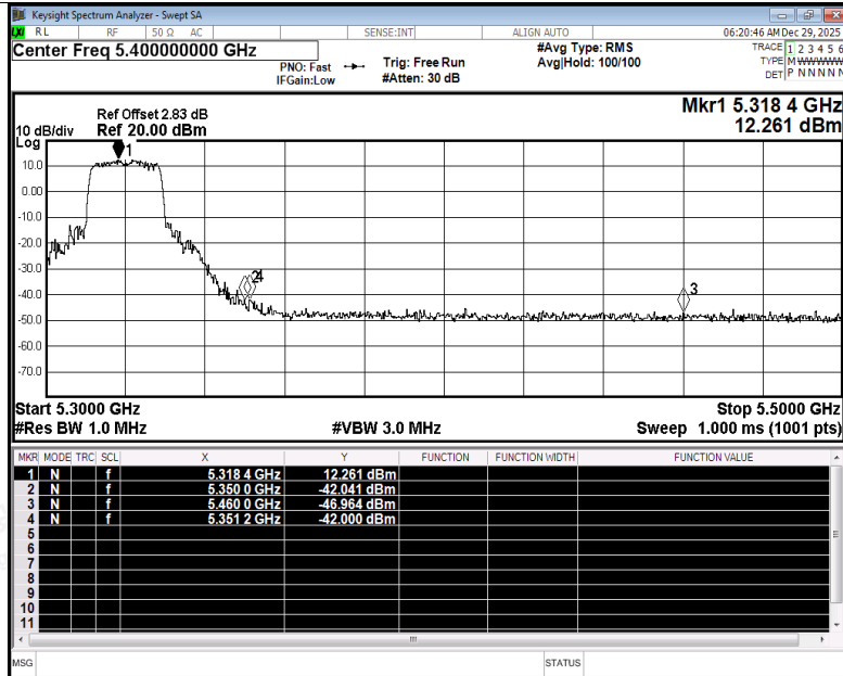
Restrict Band NVNT ac20 5320MHz Ant2 Peak
