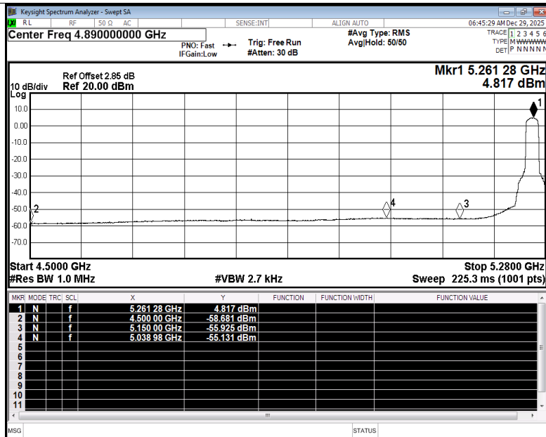
Restrict Band NVNT ac20 5260MHz Ant3 Average
