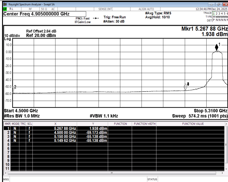
Restrict Band NVNT ac40 5270MHz Ant1 Average
