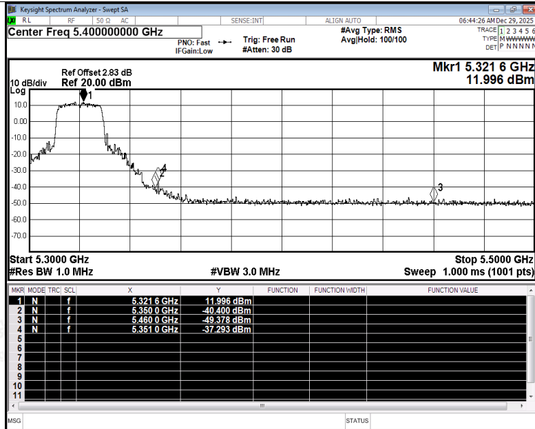
Restrict Band NVNT n20 5320MHz Ant3 Peak
