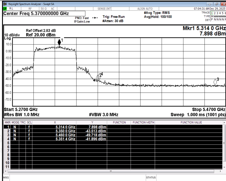
Restrict Band NVNT be40 5310MHz Ant3 Peak
