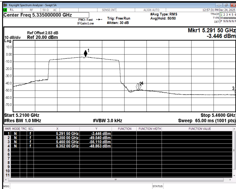
Restrict Band NVNT be80 5290MHz Ant1 Average
