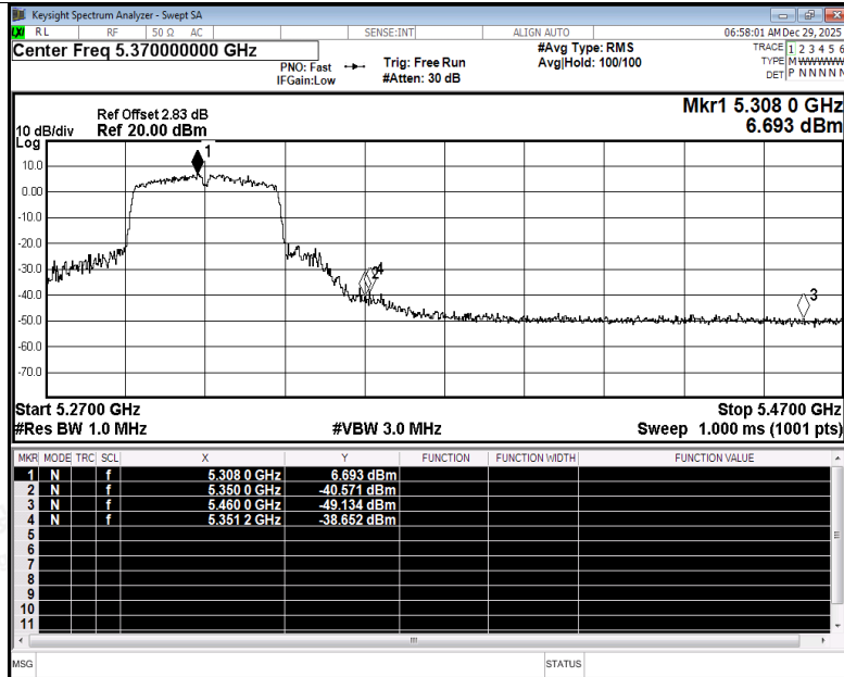
Restrict Band NVNT n40 5310MHz Ant3 Peak
