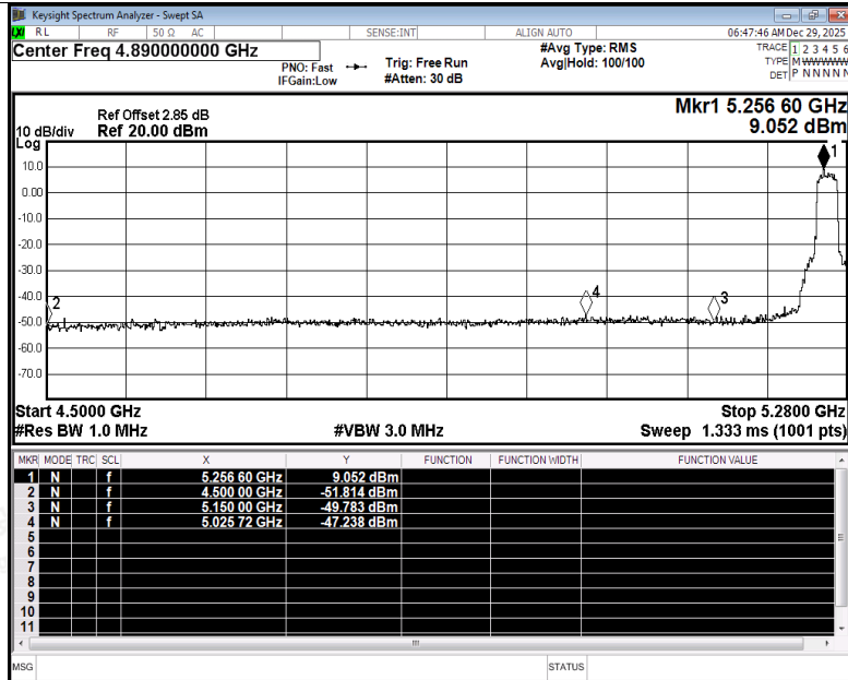
Restrict Band NVNT ax20 5260MHz Ant3 Peak
