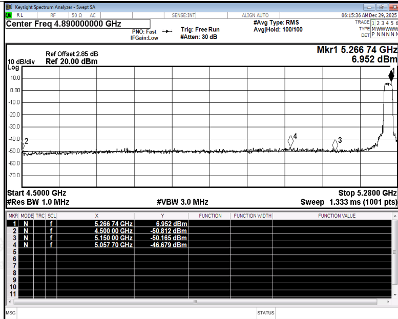
Restrict Band NVNT a 5260MHz Ant2 Peak
