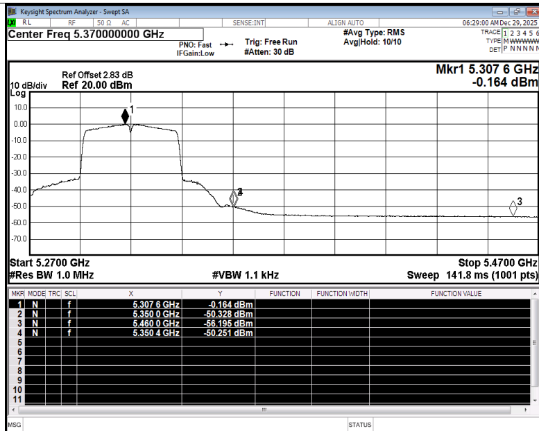
Restrict Band NVNT ac40 5310MHz Ant2 Average
