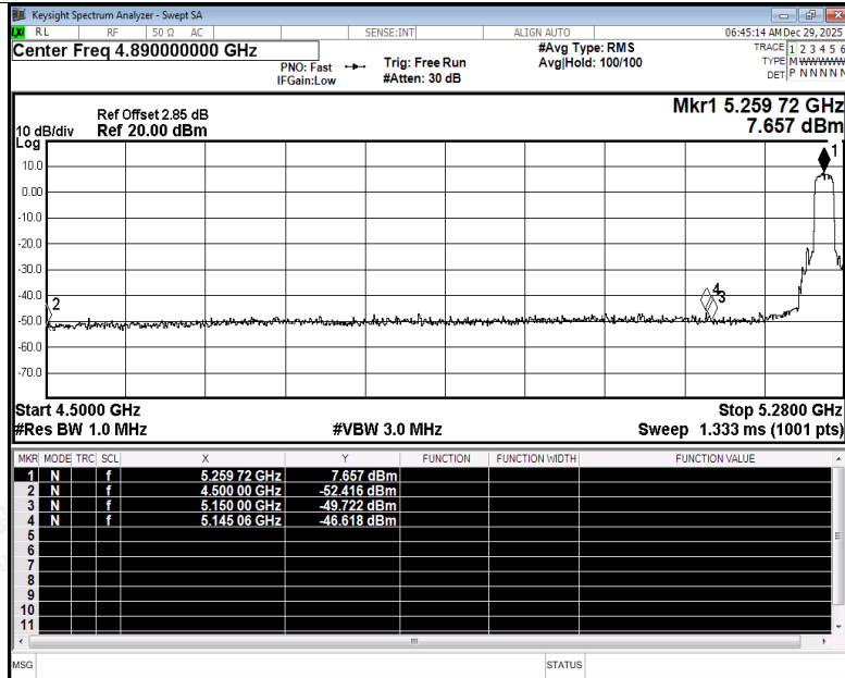
Restrict Band NVNT ac20 5260MHz Ant3 Peak
