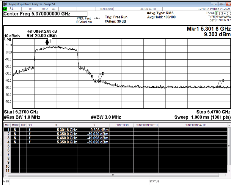
Restrict Band NVNT ax40 5310MHz Ant1 Peak
