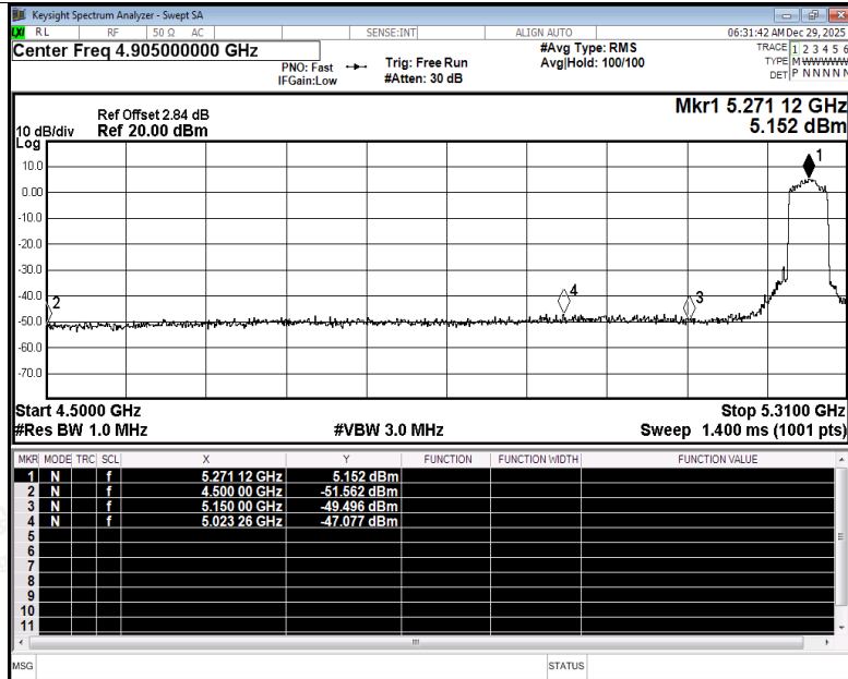
Restrict Band NVNT be40 5270MHz Ant2 Peak
