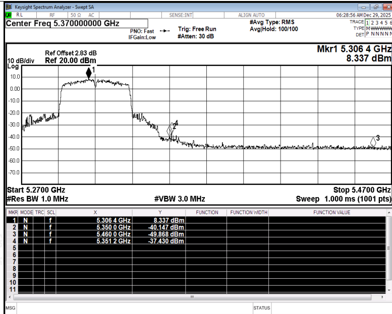
Restrict Band NVNT ac40 5310MHz Ant2 Peak
