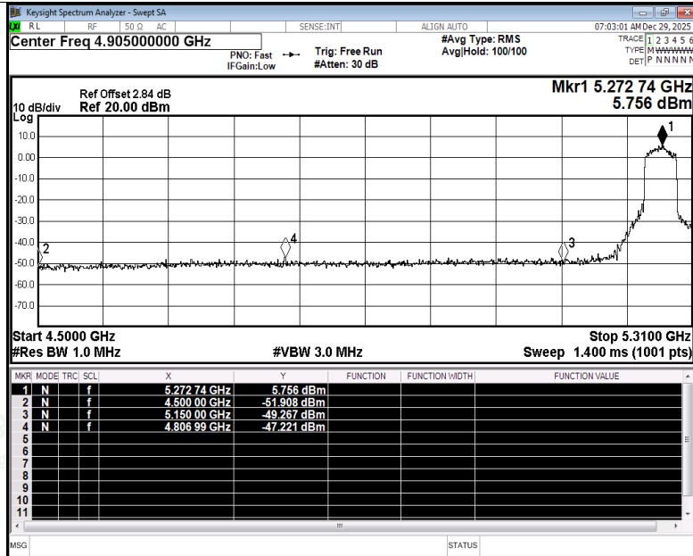
Restrict Band NVNT be40 5270MHz Ant3 Peak
