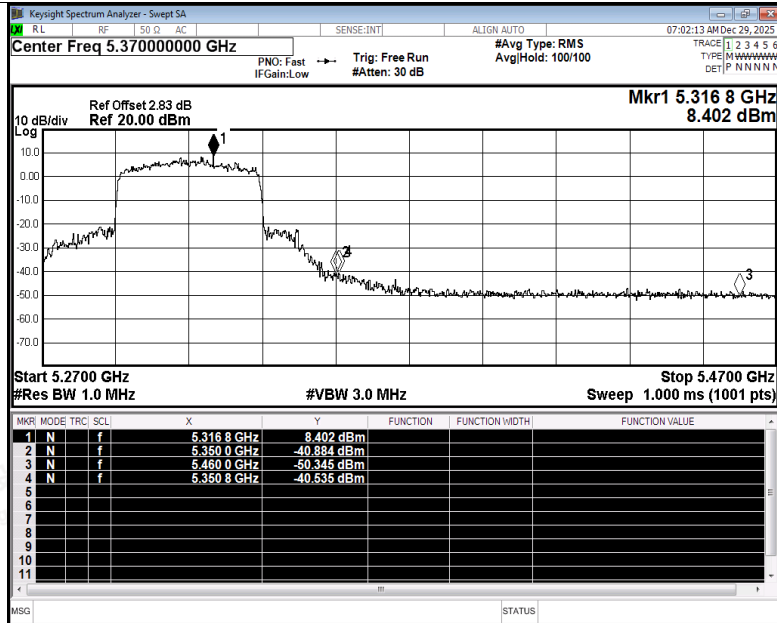
Restrict Band NVNT ax40 5310MHz Ant3 Peak
