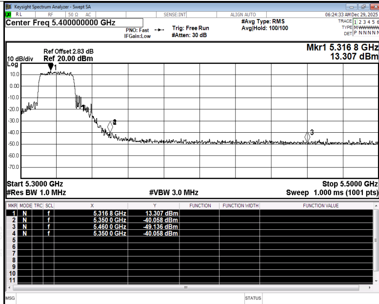
Restrict Band NVNT be20 5320MHz Ant2 Peak
