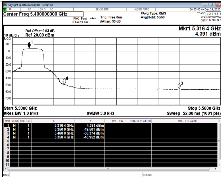
Restrict Band NVNT be20 5320MHz Ant3 Average
