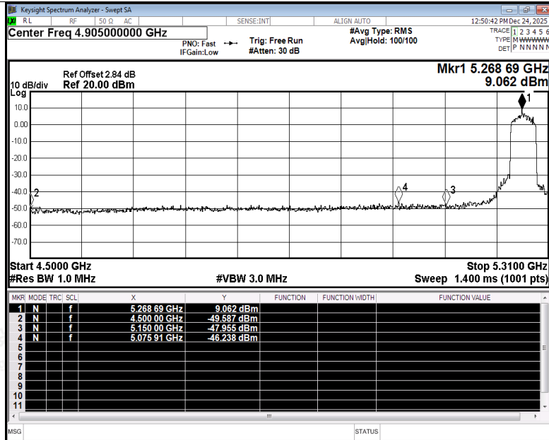
Restrict Band NVNT be40 5270MHz Ant1 Peak
