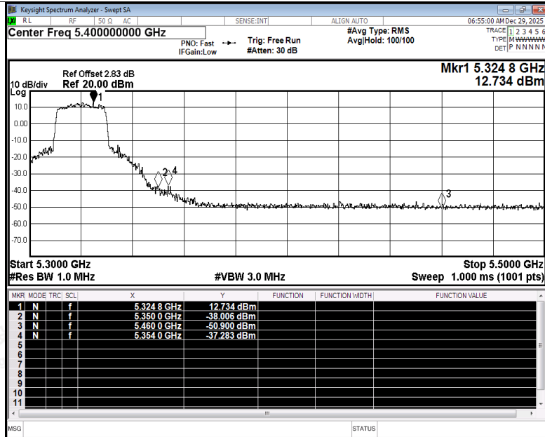
Restrict Band NVNT be20 5320MHz Ant3 Peak
