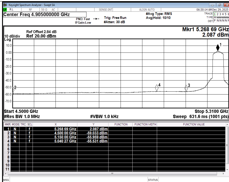
Restrict Band NVNT ax40 5270MHz Ant2 Average
