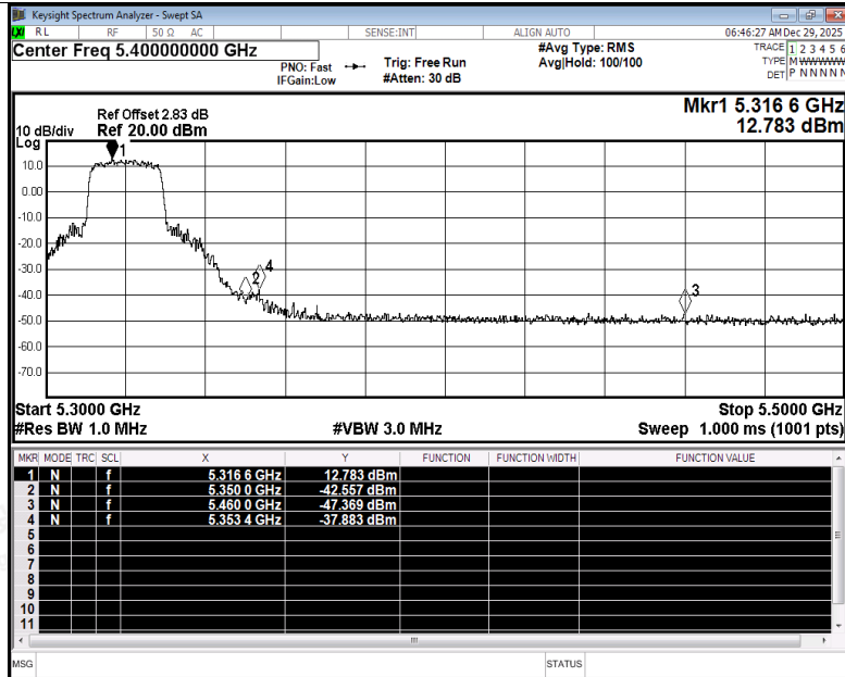
Restrict Band NVNT ac20 5320MHz Ant3 Peak
