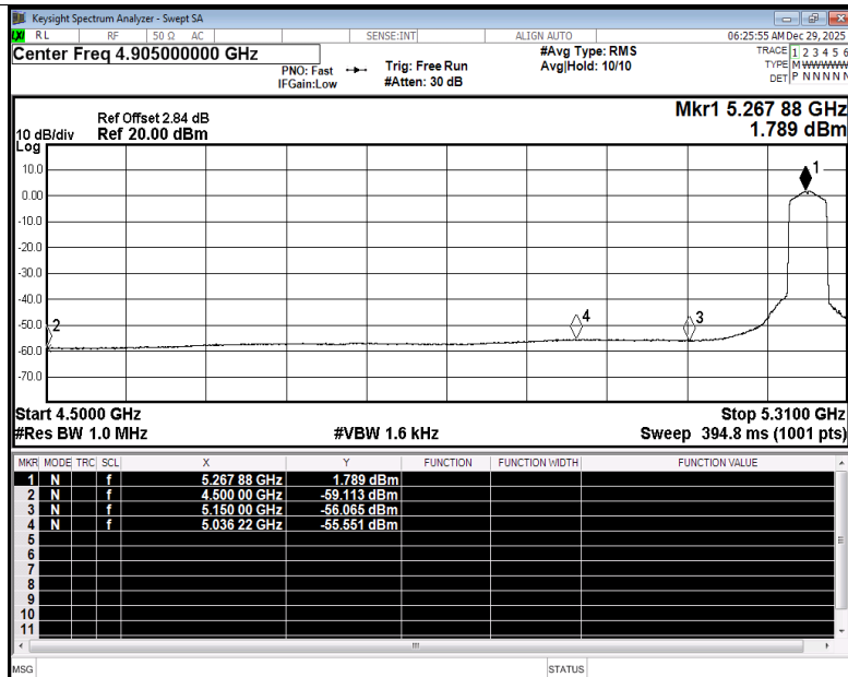
Restrict Band NVNT n40 5270MHz Ant2 Average
