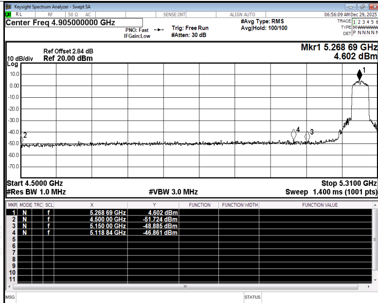
Restrict Band NVNT n40 5270MHz Ant3 Peak
