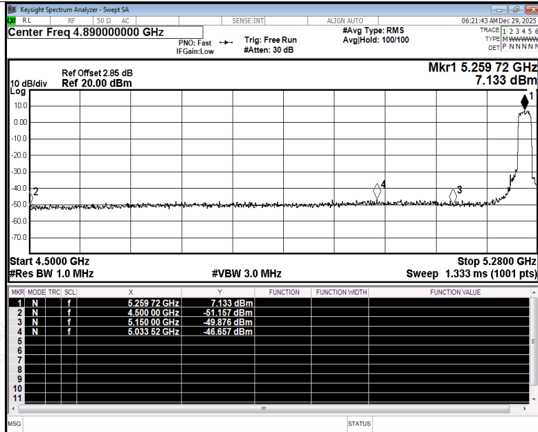
Restrict Band NVNT ax20 5260MHz Ant2 Peak
