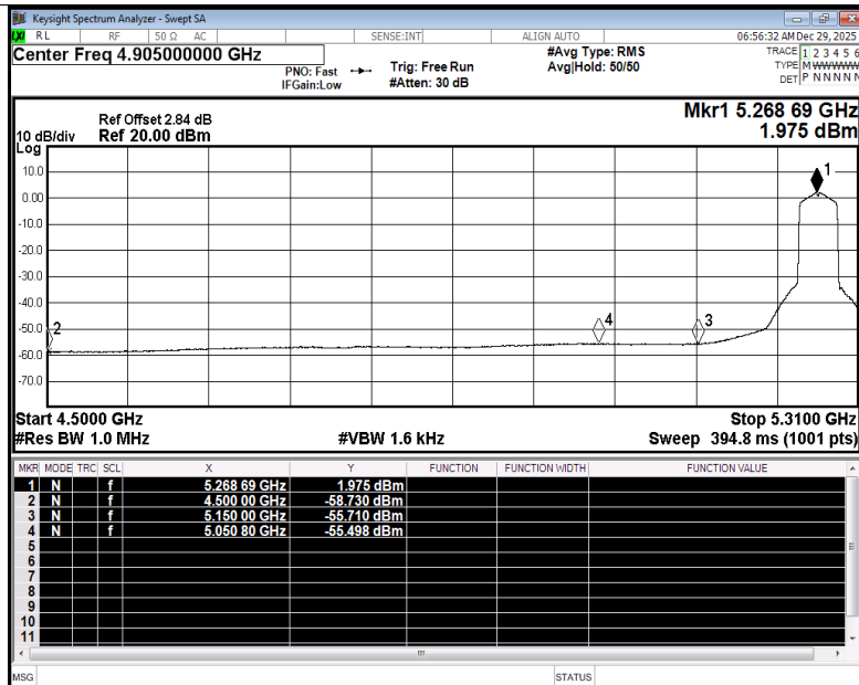
Restrict Band NVNT n40 5270MHz Ant3 Average
