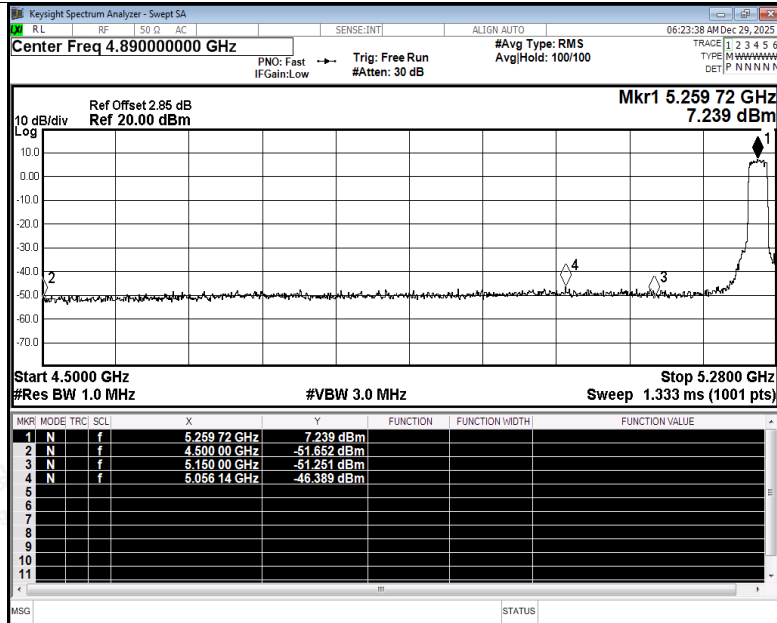
Restrict Band NVNT be20 5260MHz Ant2 Peak
