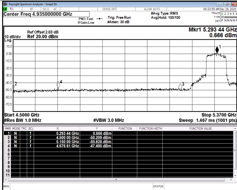
Restrict Band NVNT ac80 5290MHz Ant2 Peak
