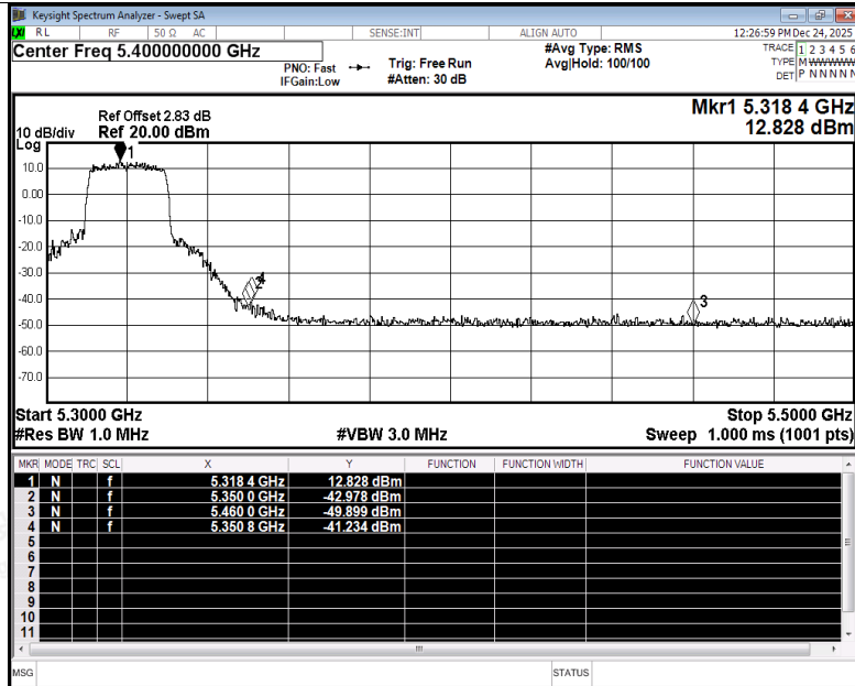
Restrict Band NVNT be20 5320MHz Ant1 Peak
