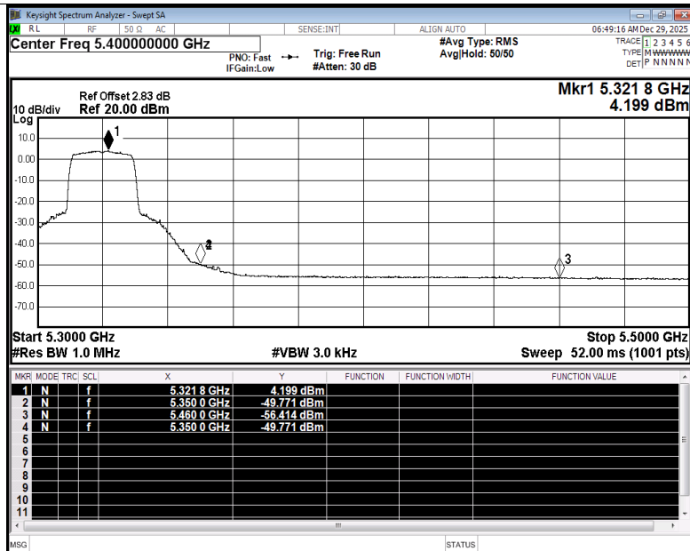
Restrict Band NVNT ax20 5320MHz Ant3 Average
