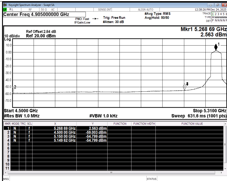
Restrict Band NVNT ax40 5270MHz Ant1 Average
