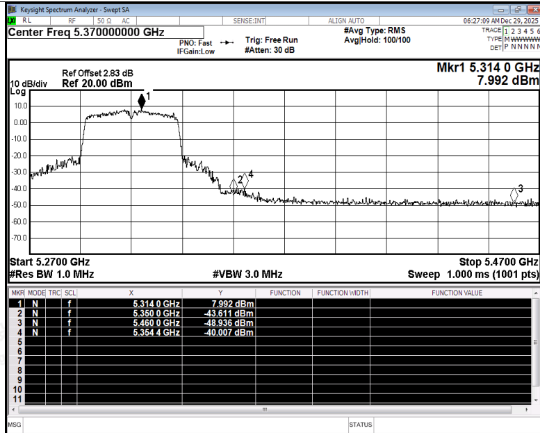
Restrict Band NVNT n40 5310MHz Ant2 Peak
