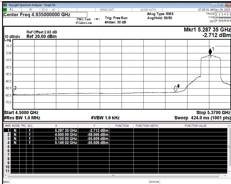
Restrict Band NVNT ac80 5290MHz Ant3 Average
