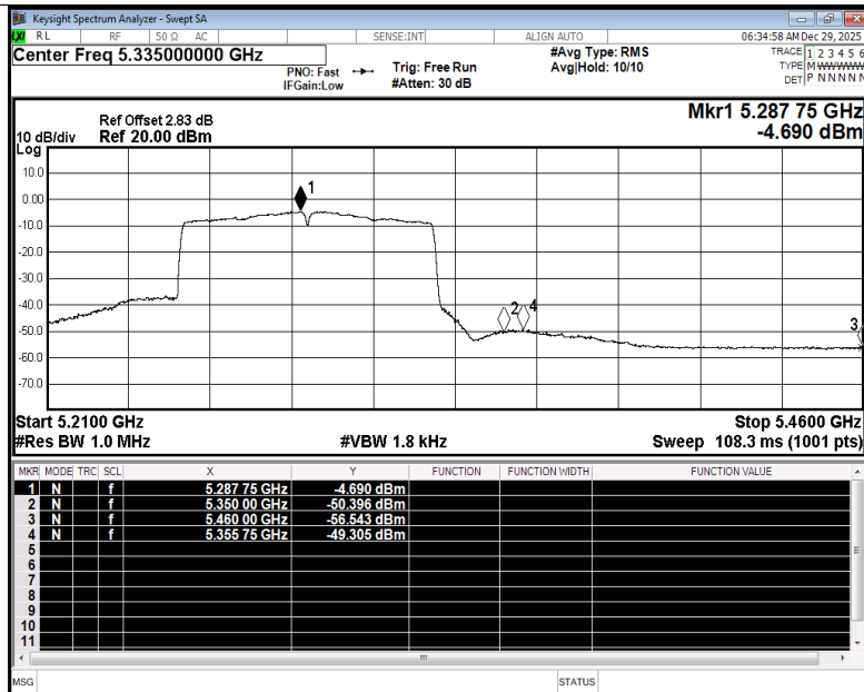
Restrict Band NVNT ac80 5290MHz Ant2 Average
