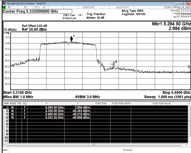
Restrict Band NVNT ac80 5290MHz Ant1 Peak
