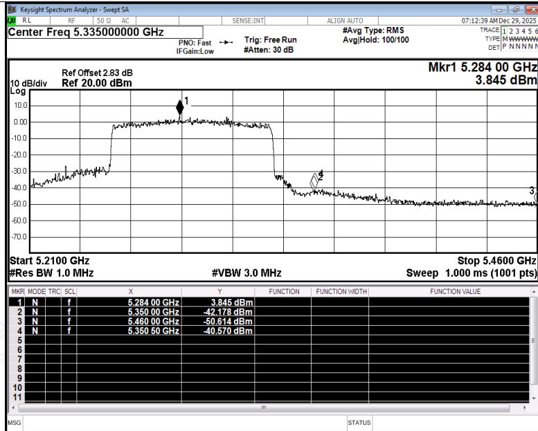
Restrict Band NVNT ax80 5290MHz Ant3 Peak
