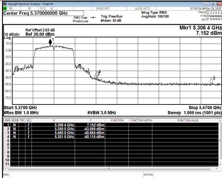
Restrict Band NVNT ac40 5310MHz Ant3 Peak
