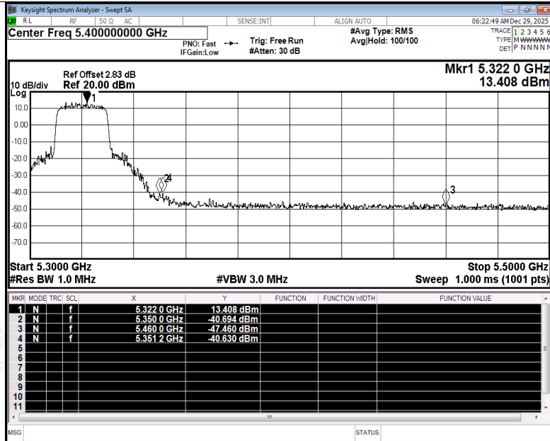
Restrict Band NVNT ax20 5320MHz Ant2 Peak
