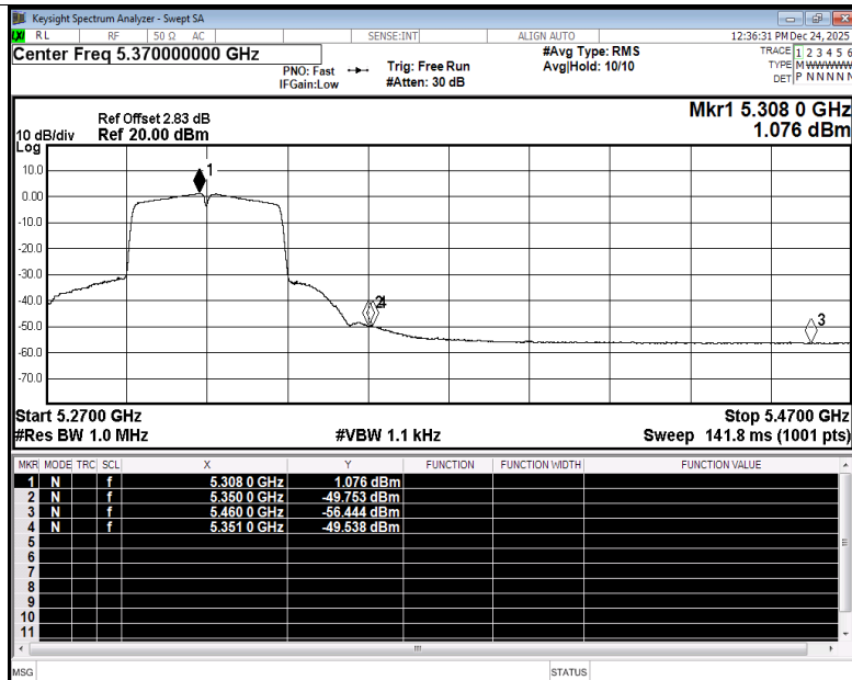
Restrict Band NVNT ac40 5310MHz Ant1 Average
