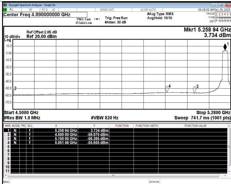
Restrict Band NVNT n20 5260MHz Ant2 Average
