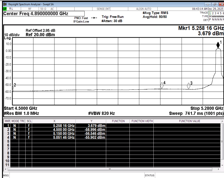
Restrict Band NVNT n20 5260MHz Ant3 Average
