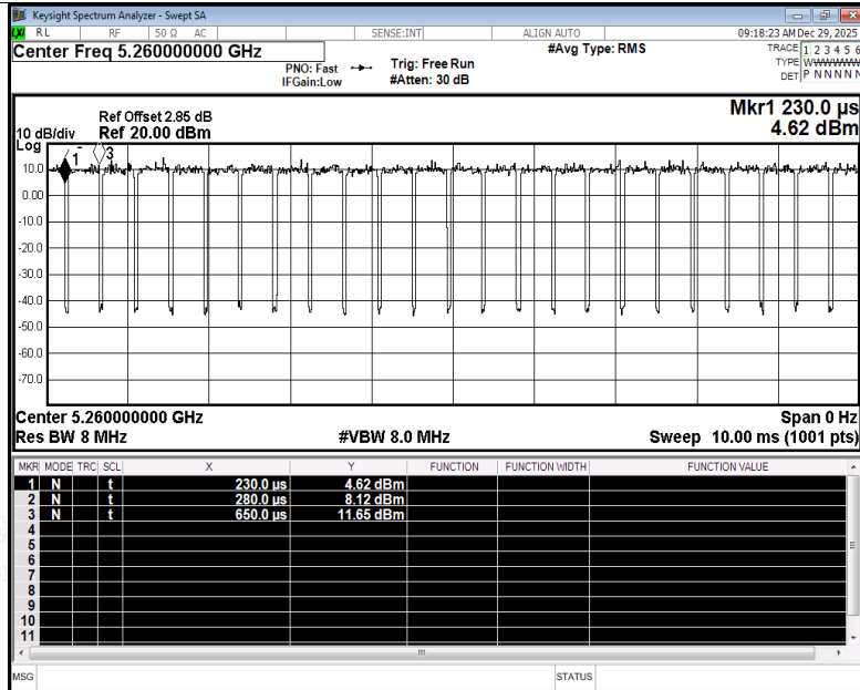
Duty Cycle NVNT ac20 5260MHz Ant2
