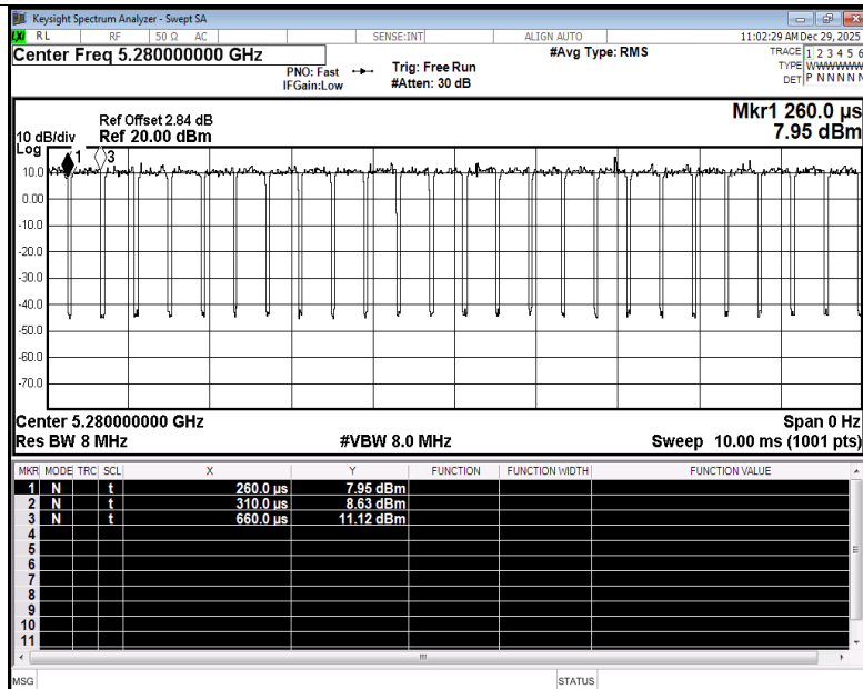
Duty Cycle NVNT ax20 5280MHz Ant3
