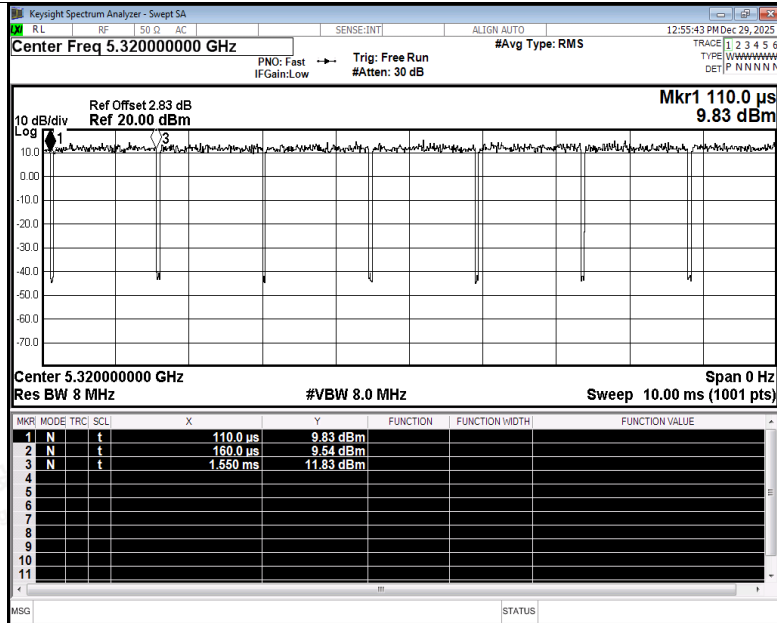
Duty Cycle NVNT a 5320MHz Ant5
