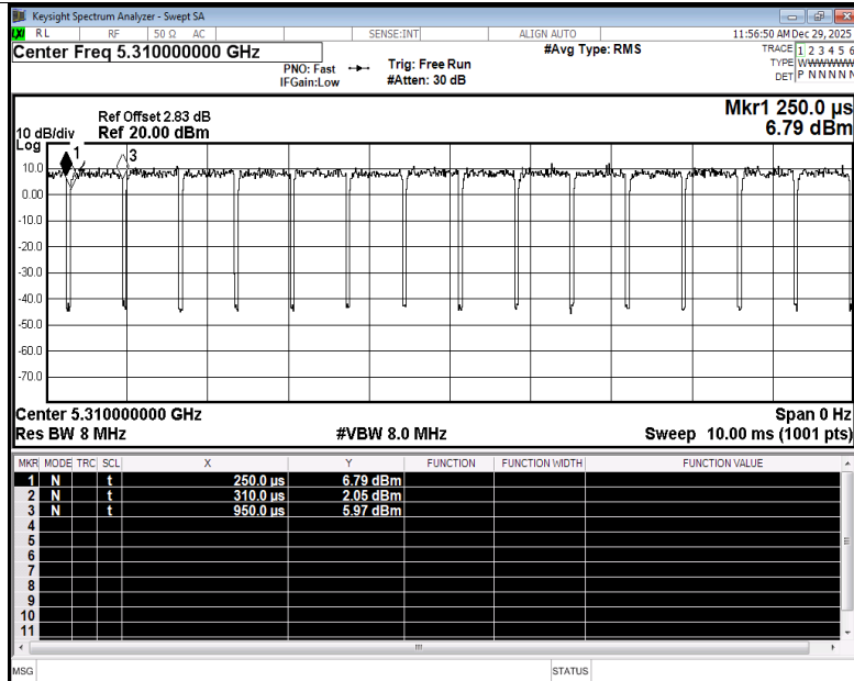
Duty Cycle NVNT n40 5310MHz Ant4
