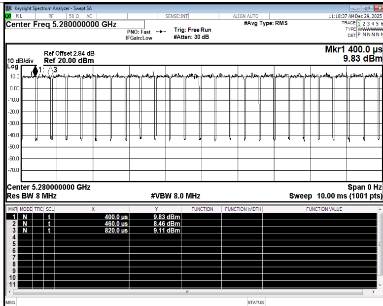
Duty Cycle NVNT be20 5280MHz Ant3
