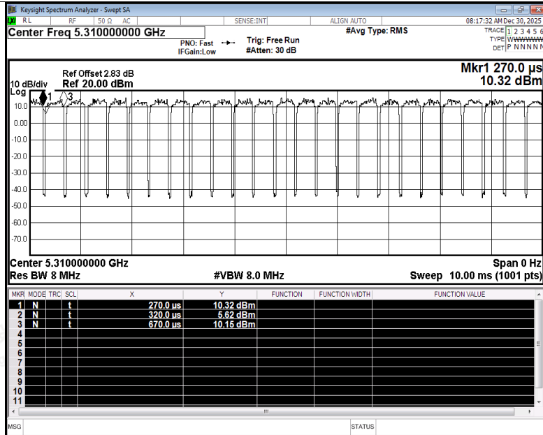
Duty Cycle NVNT ax40 5310MHz Ant5
