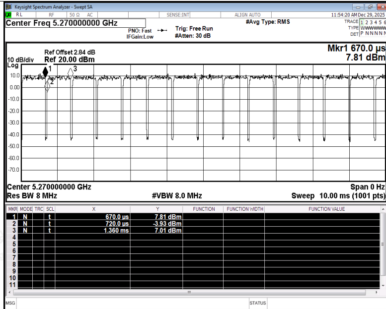
Duty Cycle NVNT n40 5270MHz Ant4
