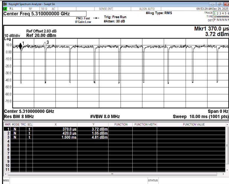
Duty Cycle NVNT ax40 5310MHz Ant2
