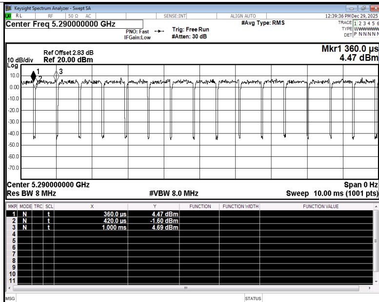
Duty Cycle NVNT be80 5290MHz Ant4
