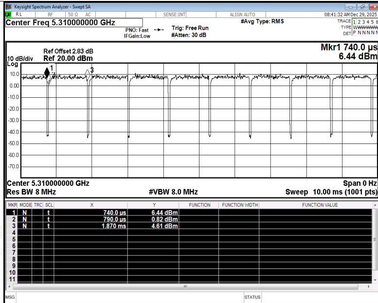
Duty Cycle NVNT ax40 5310MHz Ant1
