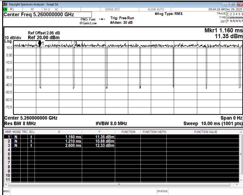
Duty Cycle NVNT a 5260MHz Ant2
