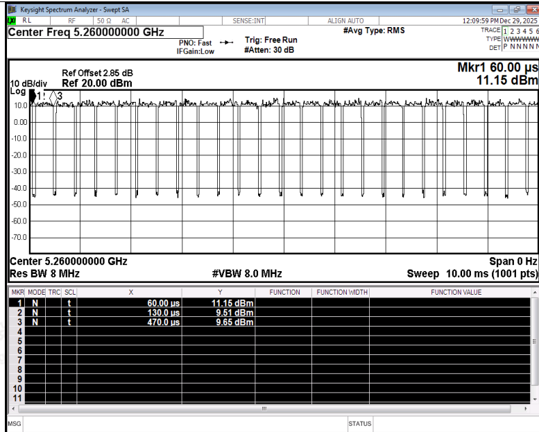
Duty Cycle NVNT ax20 5260MHz Ant4
