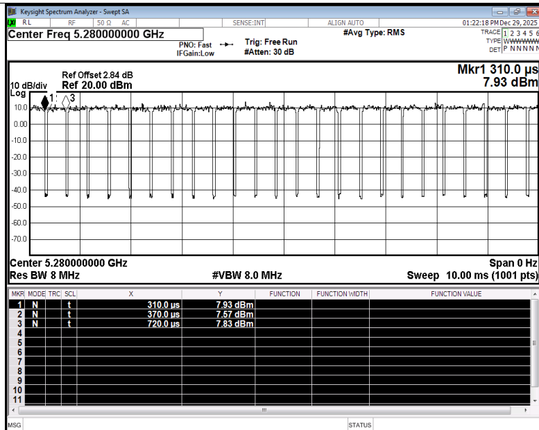
Duty Cycle NVNT be20 5280MHz Ant5
