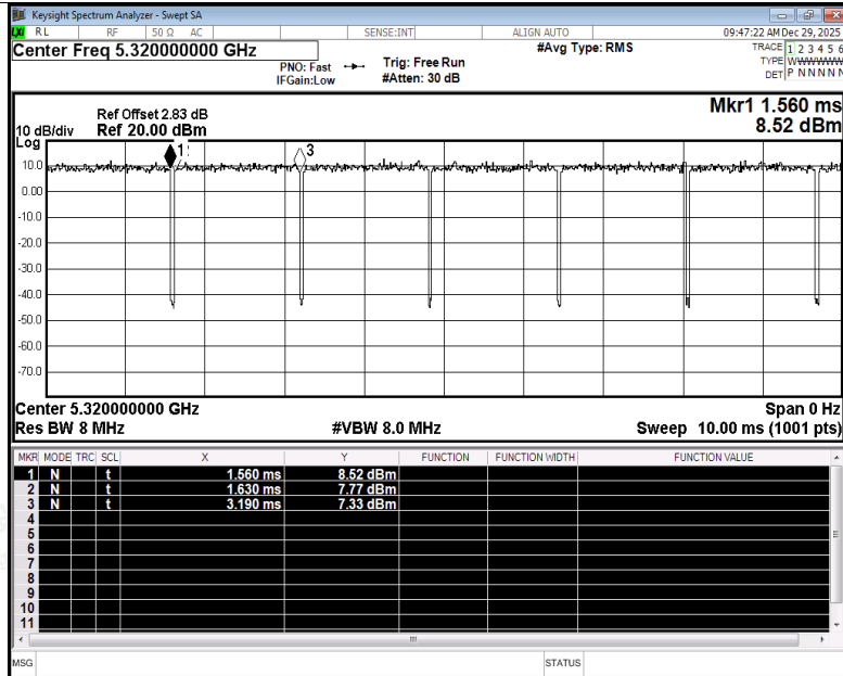
Duty Cycle NVNT ax20 5320MHz Ant2
