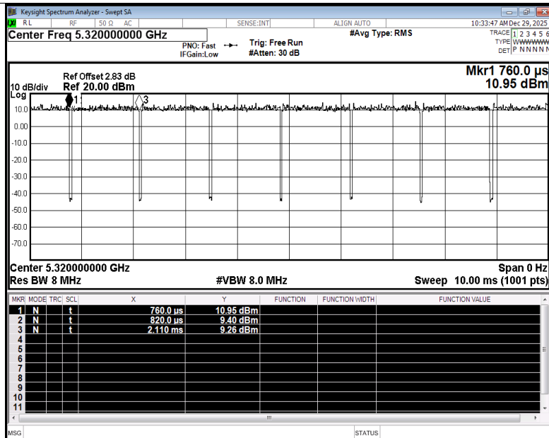
Duty Cycle NVNT n20 5320MHz Ant3
