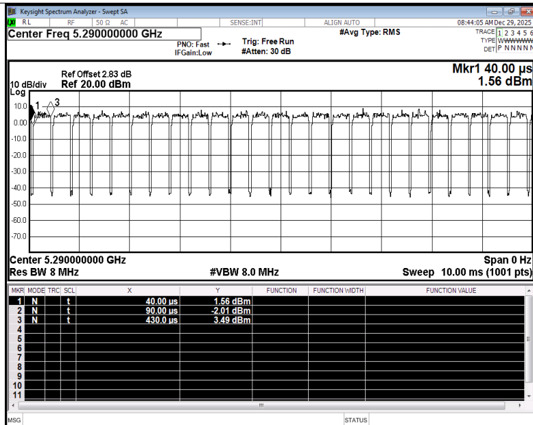
Duty Cycle NVNT ax80 5290MHz Ant1
