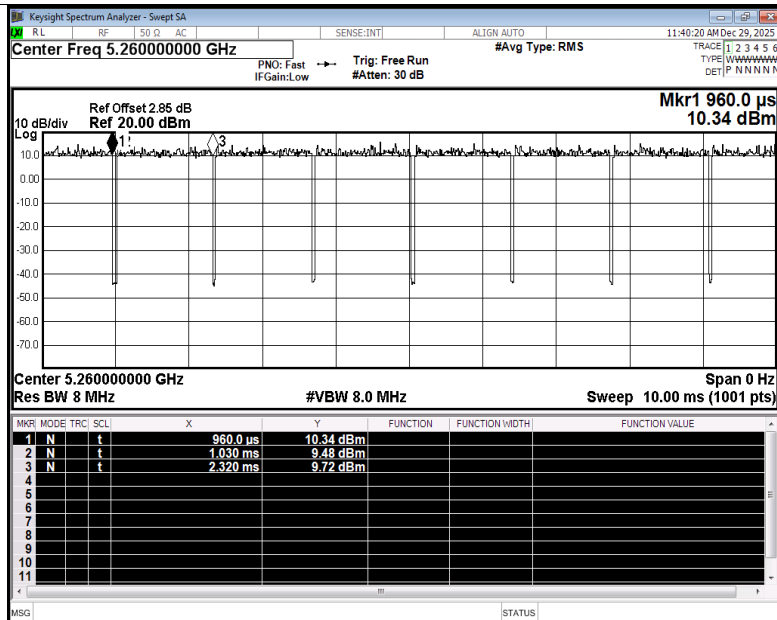
Duty Cycle NVNT n20 5260MHz Ant4
