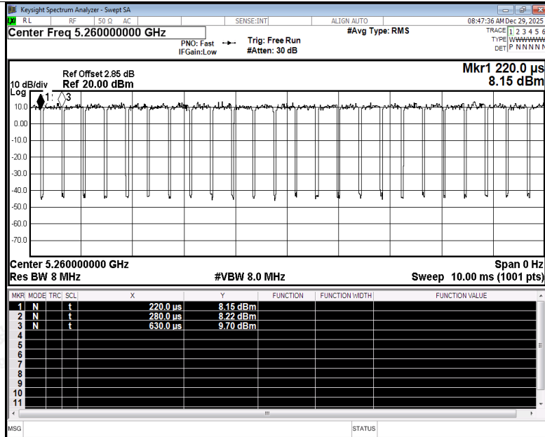
Duty Cycle NVNT be20 5260MHz Ant1
