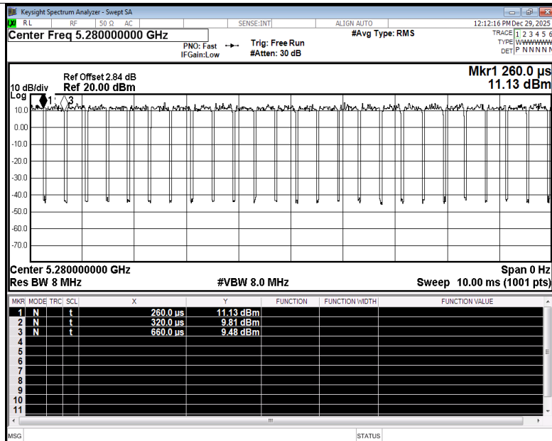
Duty Cycle NVNT ax20 5280MHz Ant4
