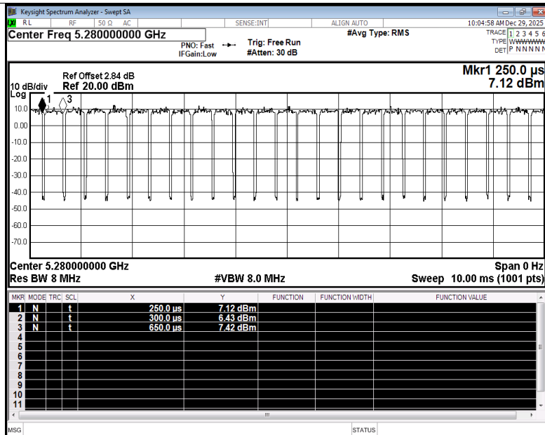
Duty Cycle NVNT be20 5280MHz Ant2
