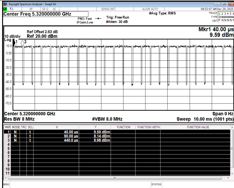
Duty Cycle NVNT be20 5320MHz Ant1
