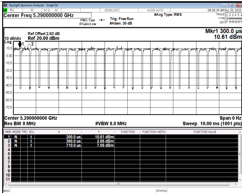
Duty Cycle NVNT be80 5290MHz Ant5
