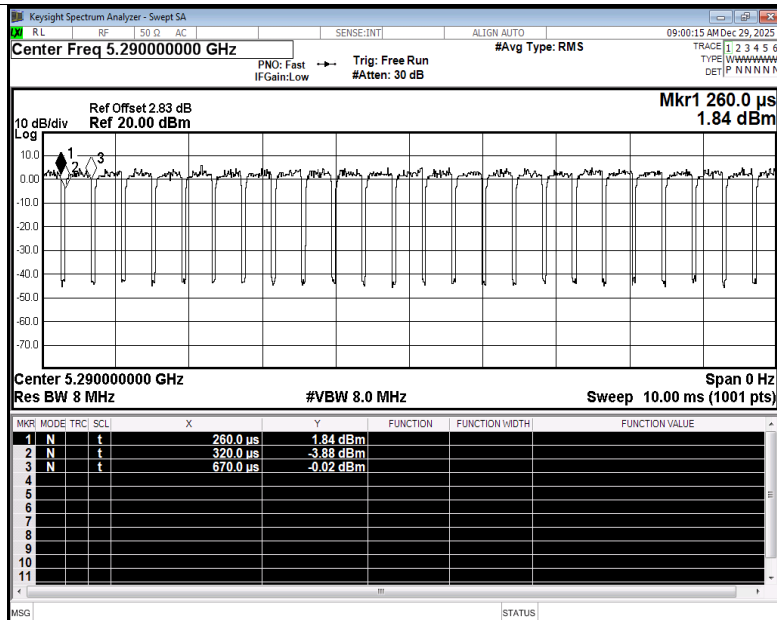
Duty Cycle NVNT be80 5290MHz Ant1
