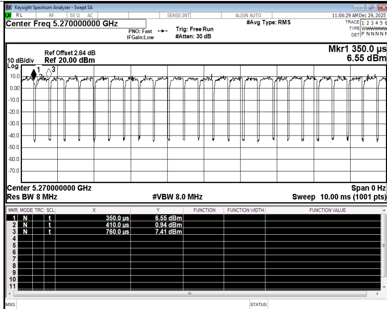
Duty Cycle NVNT ax40 5270MHz Ant3
