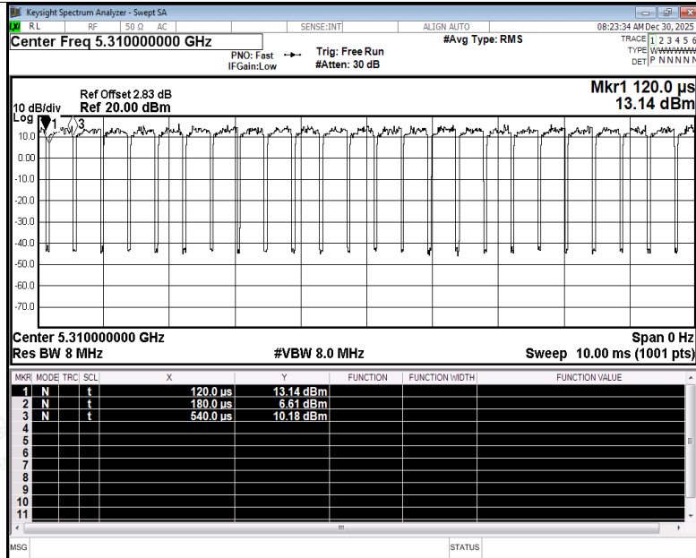
Duty Cycle NVNT be40 5310MHz Ant5
