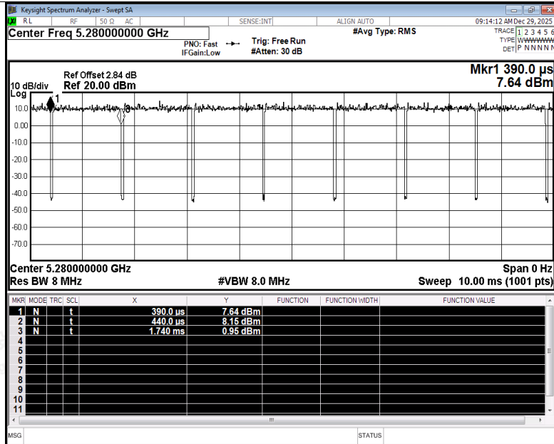
Duty Cycle NVNT n20 5280MHz Ant2
