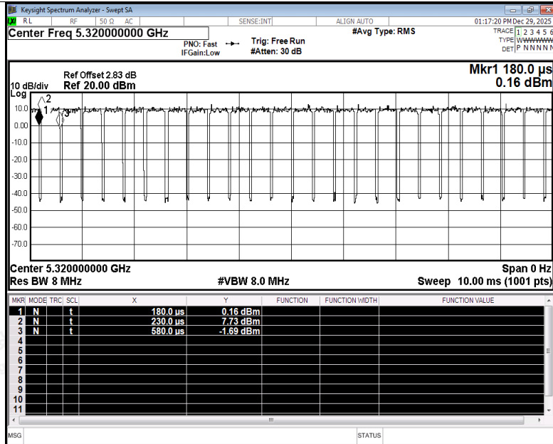
Duty Cycle NVNT ax20 5320MHz Ant5
