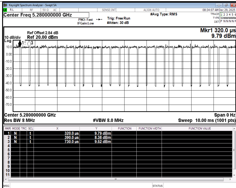
Duty Cycle NVNT ax20 5280MHz Ant1
