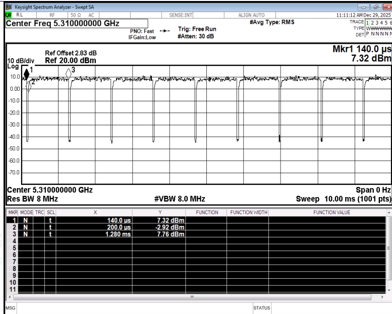
Duty Cycle NVNT ax40 5310MHz Ant3
