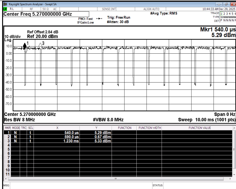
Duty Cycle NVNT n40 5270MHz Ant3
