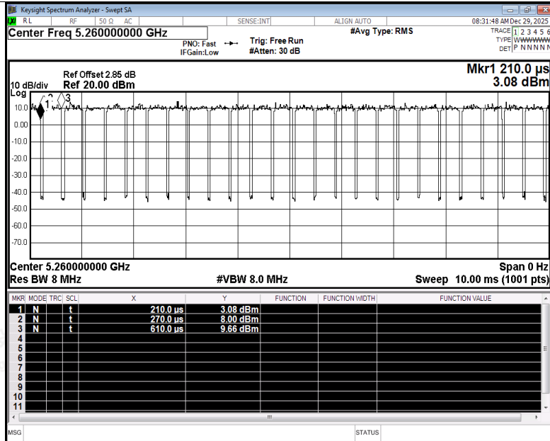
Duty Cycle NVNT ax20 5260MHz Ant1
