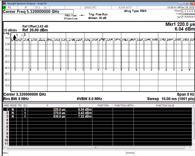
Duty Cycle NVNT be20 5320MHz Ant2
