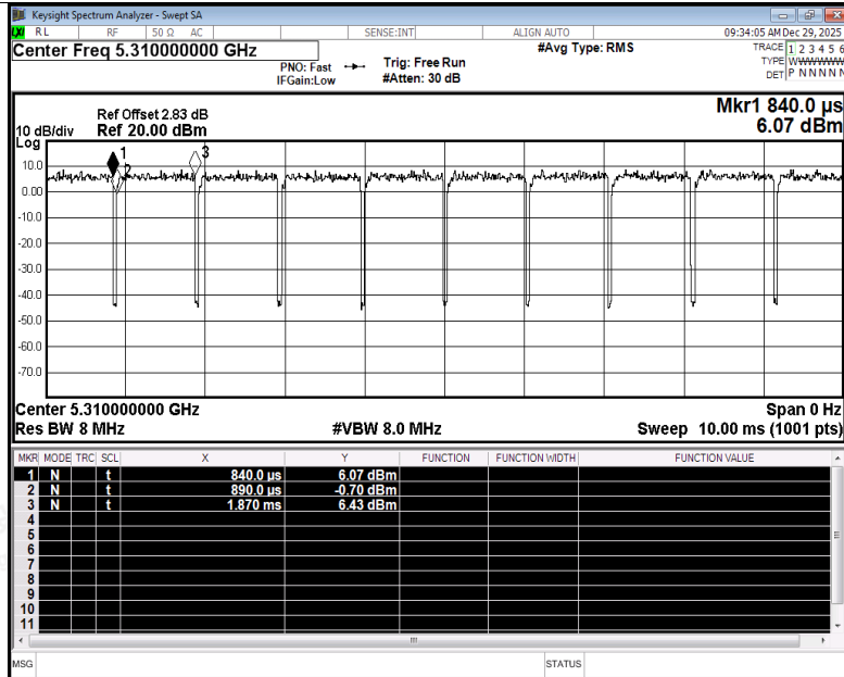
Duty Cycle NVNT ac40 5310MHz Ant2
