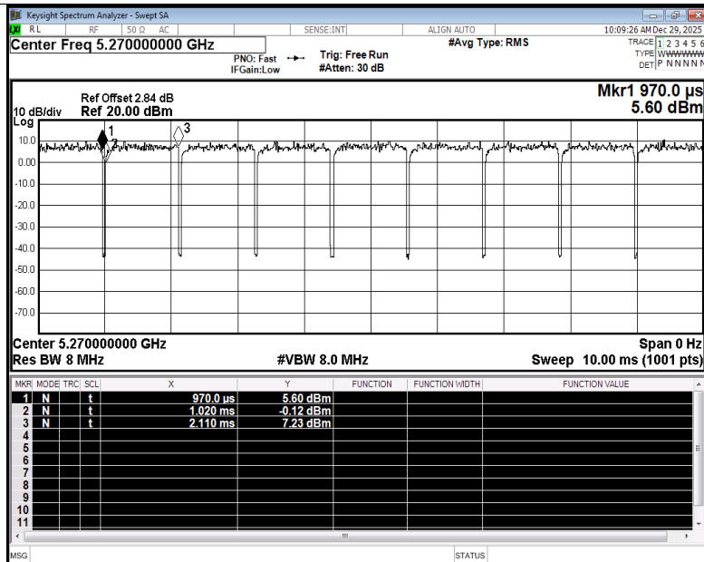
Duty Cycle NVNT be40 5270MHz Ant2
