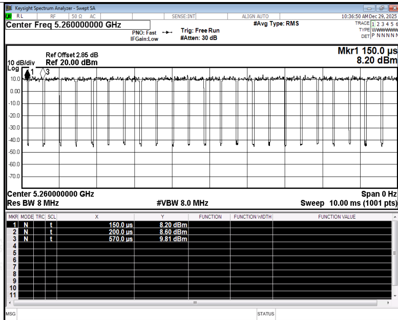
Duty Cycle NVNT ac20 5260MHz Ant3
