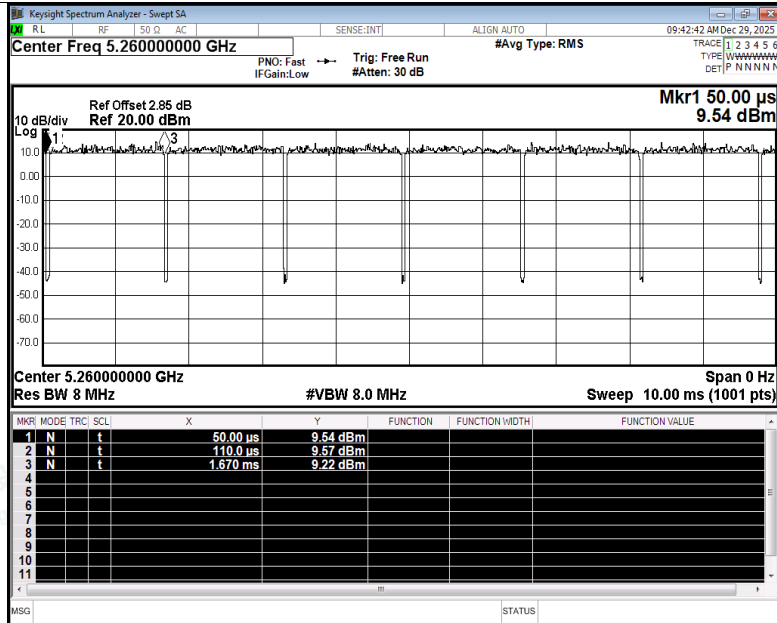
Duty Cycle NVNT ax20 5260MHz Ant2
