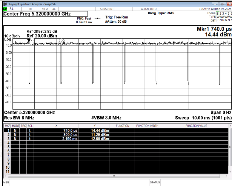
Duty Cycle NVNT a 5320MHz Ant3
