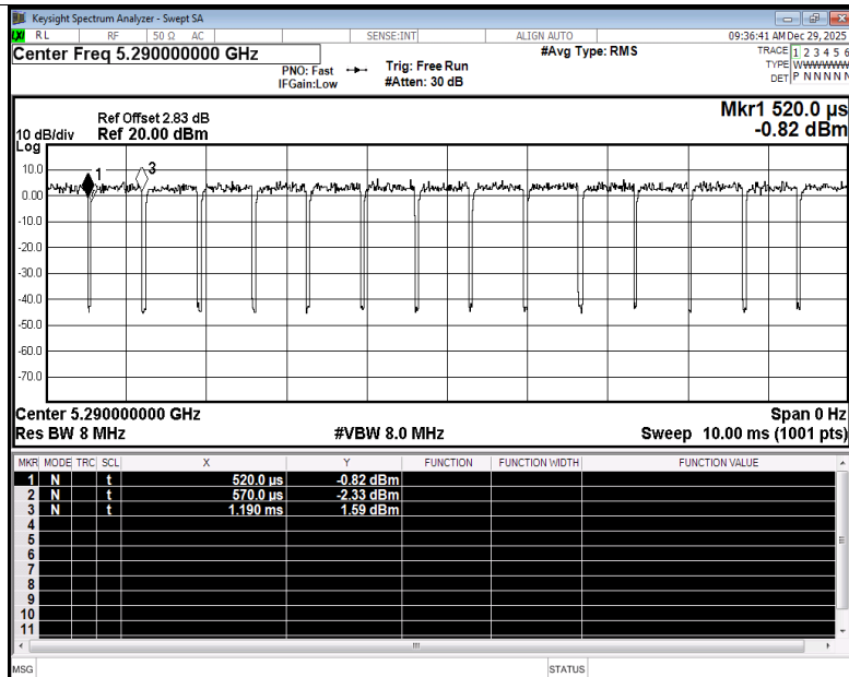
Duty Cycle NVNT ac80 5290MHz Ant2
