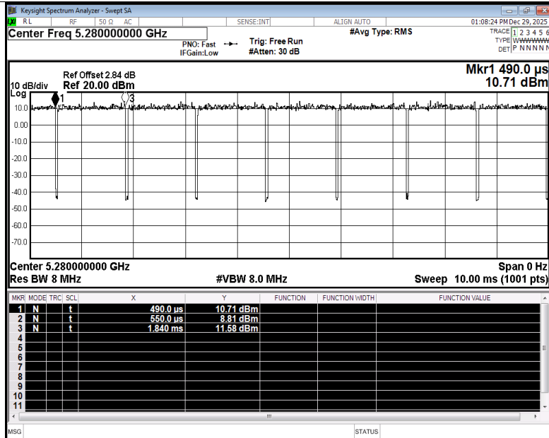
Duty Cycle NVNT ac20 5280MHz Ant5
