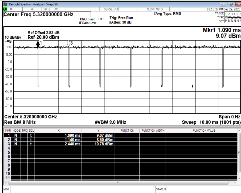
Duty Cycle NVNT ac20 5320MHz Ant5
