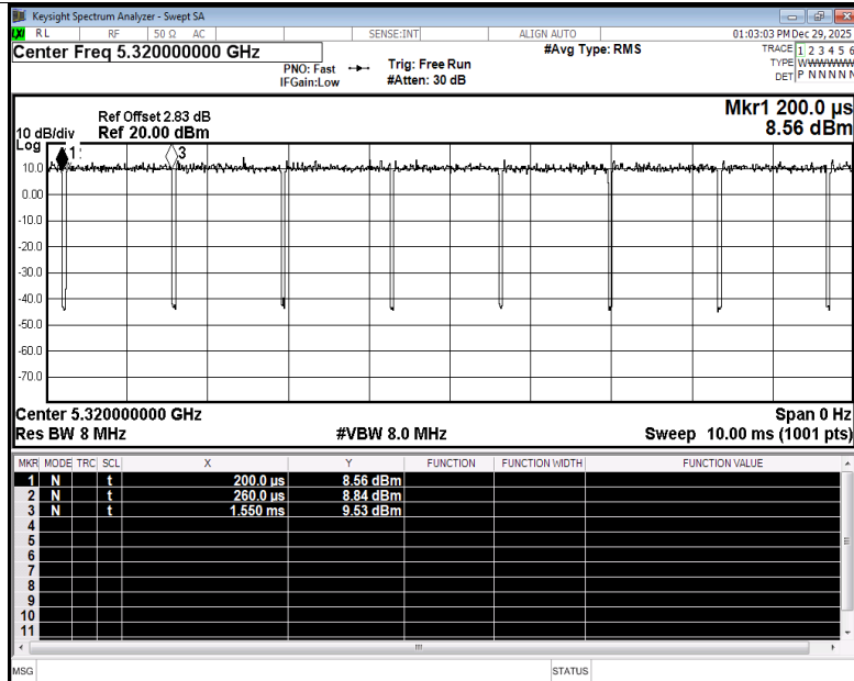
Duty Cycle NVNT n20 5320MHz Ant5
