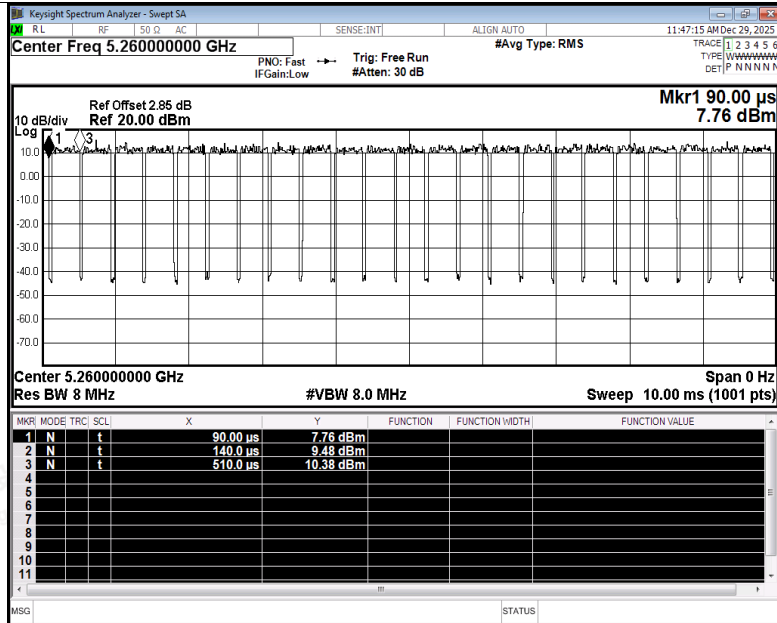
Duty Cycle NVNT ac20 5260MHz Ant4
