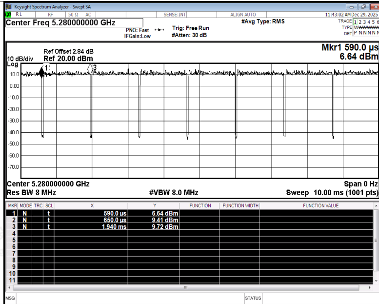
Duty Cycle NVNT n20 5280MHz Ant4
