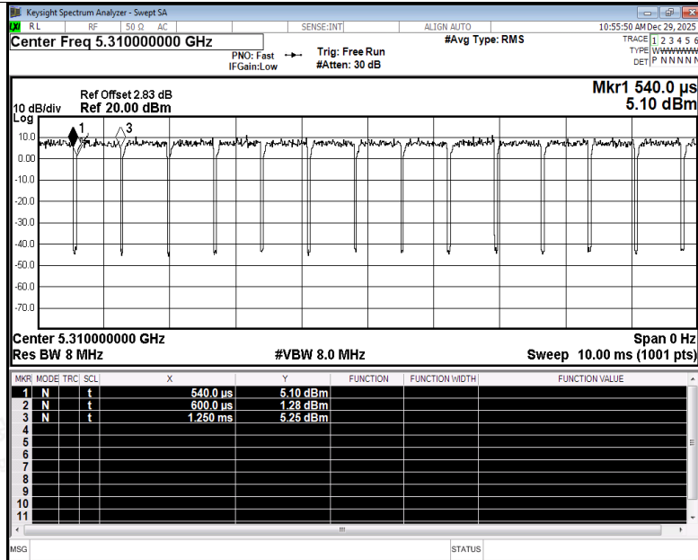
Duty Cycle NVNT ac40 5310MHz Ant3
