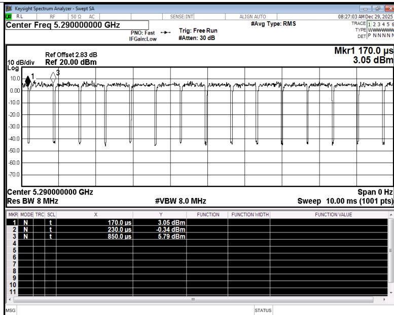
Duty Cycle NVNT ac80 5290MHz Ant1
