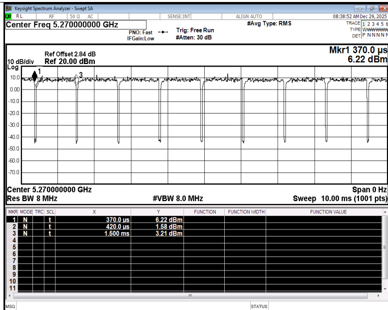
Duty Cycle NVNT ax40 5270MHz Ant1
