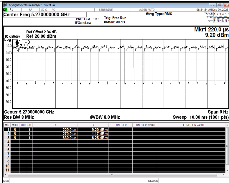
Duty Cycle NVNT be40 5270MHz Ant1
