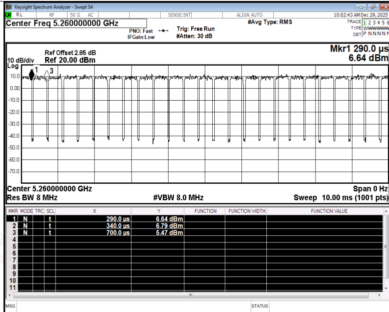
Duty Cycle NVNT be20 5260MHz Ant2
