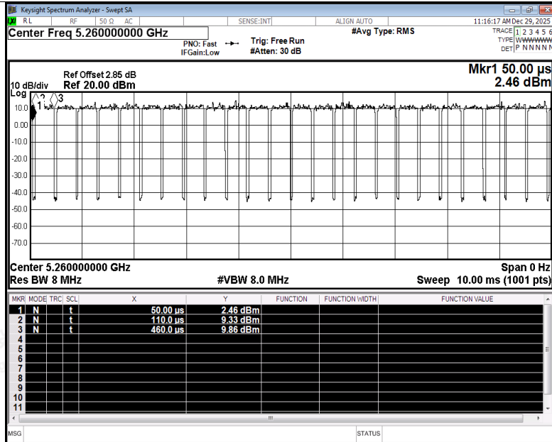
Duty Cycle NVNT be20 5260MHz Ant3
