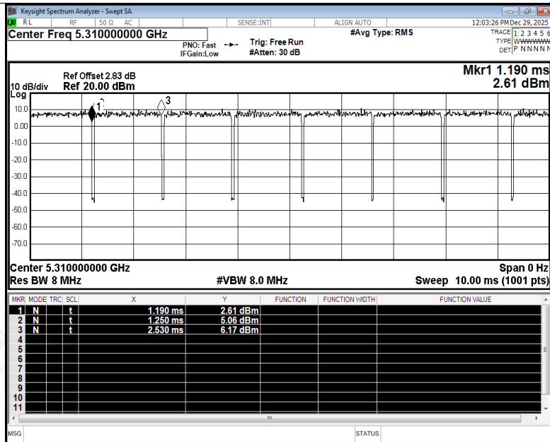
Duty Cycle NVNT ac40 5310MHz Ant4
