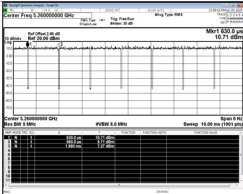
Duty Cycle NVNT n20 5260MHz Ant5
