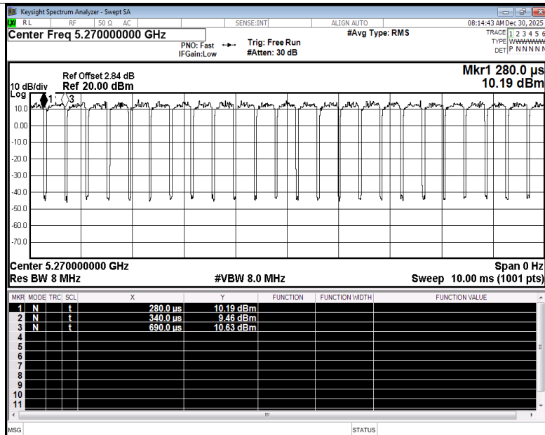
Duty Cycle NVNT ax40 5270MHz Ant5
