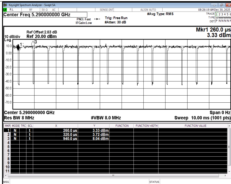
Duty Cycle NVNT ac80 5290MHz Ant5
