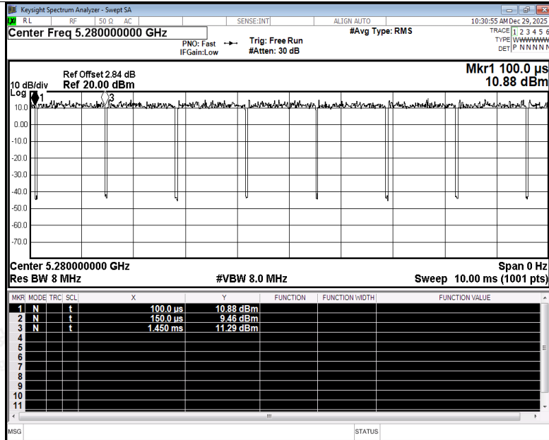
Duty Cycle NVNT n20 5280MHz Ant3
