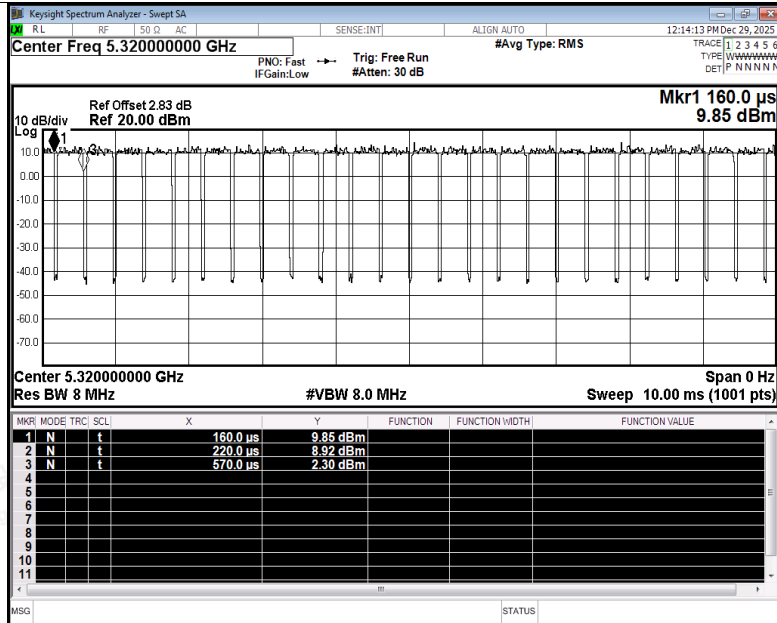
Duty Cycle NVNT ax20 5320MHz Ant4
