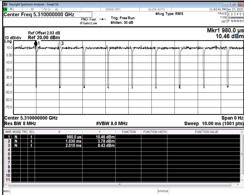
Duty Cycle NVNT ac40 5310MHz Ant1
