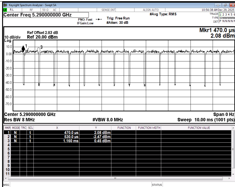
Duty Cycle NVNT ac80 5290MHz Ant3
