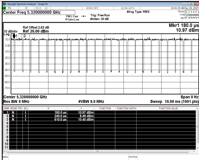
Duty Cycle NVNT ac20 5320MHz Ant3
