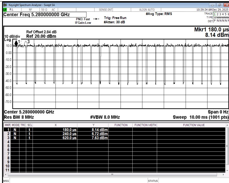
Duty Cycle NVNT ac20 5280MHz Ant3
