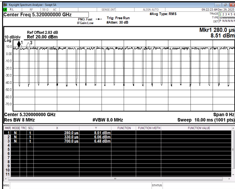
Duty Cycle NVNT ac20 5320MHz Ant2
