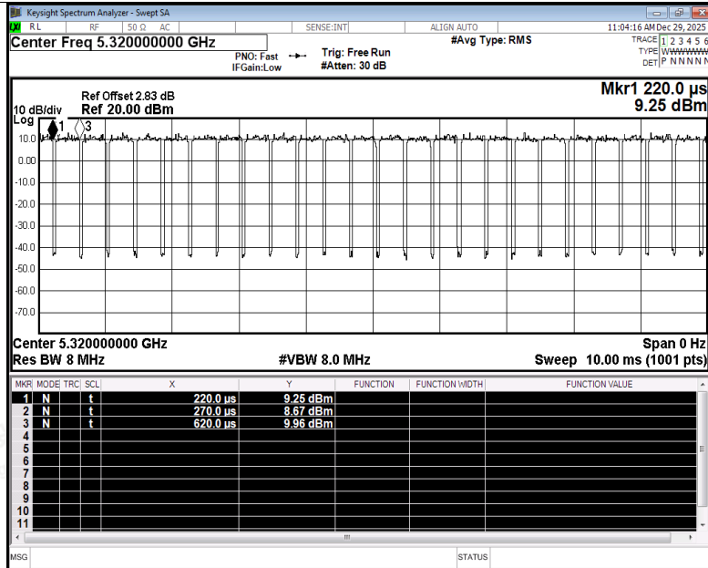
Duty Cycle NVNT ax20 5320MHz Ant3
