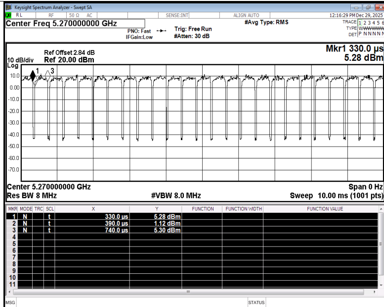
Duty Cycle NVNT ax40 5270MHz Ant4
