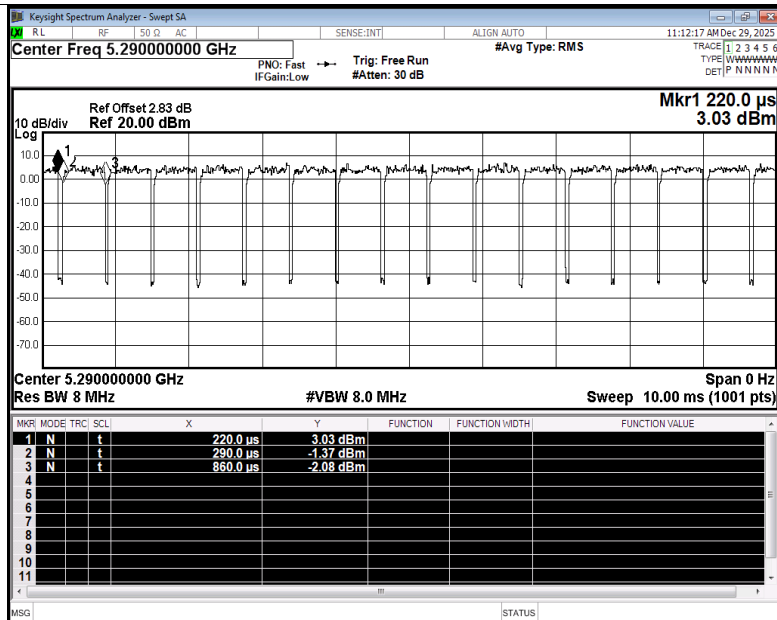
Duty Cycle NVNT ax80 5290MHz Ant3
