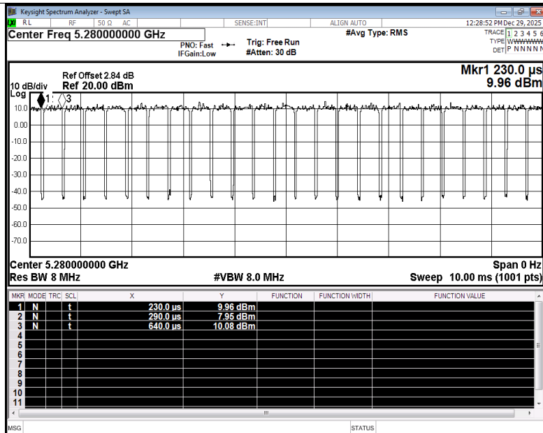
Duty Cycle NVNT be20 5280MHz Ant4
