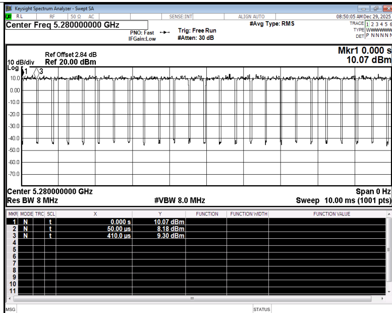
Duty Cycle NVNT be20 5280MHz Ant1
