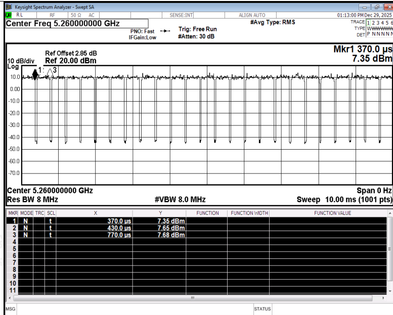
Duty Cycle NVNT ax20 5260MHz Ant5
