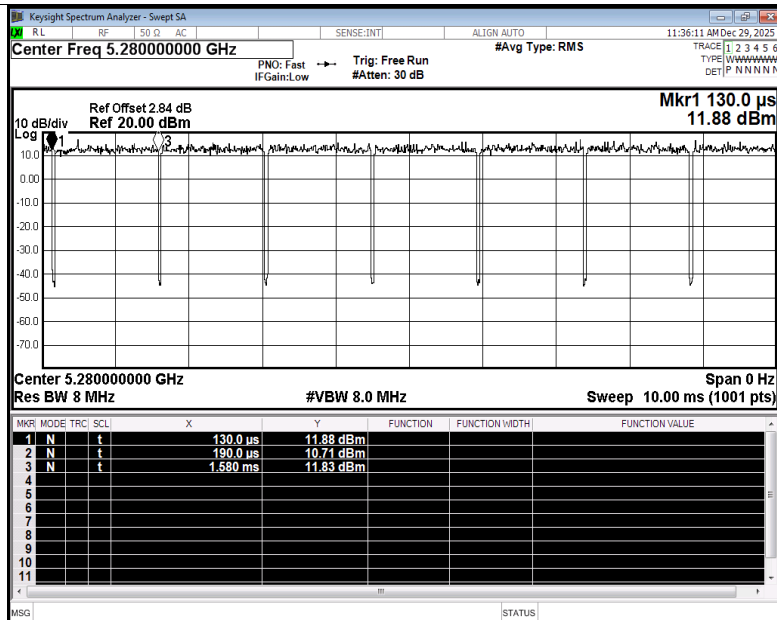
Duty Cycle NVNT a 5280MHz Ant4
