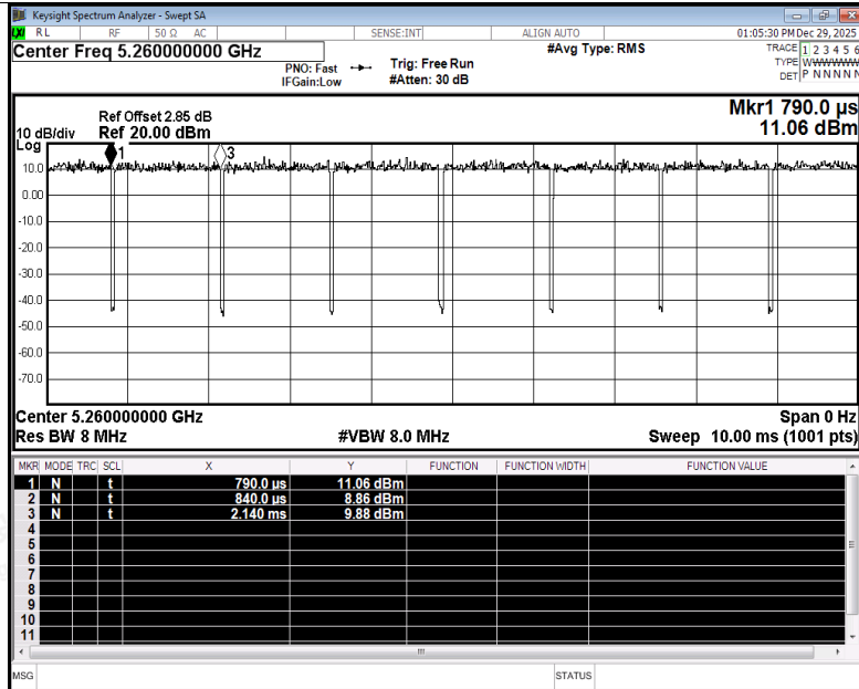
Duty Cycle NVNT ac20 5260MHz Ant5
