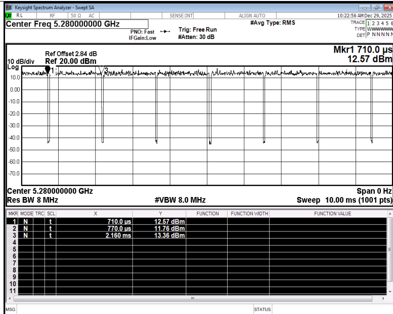
Duty Cycle NVNT a 5280MHz Ant3
