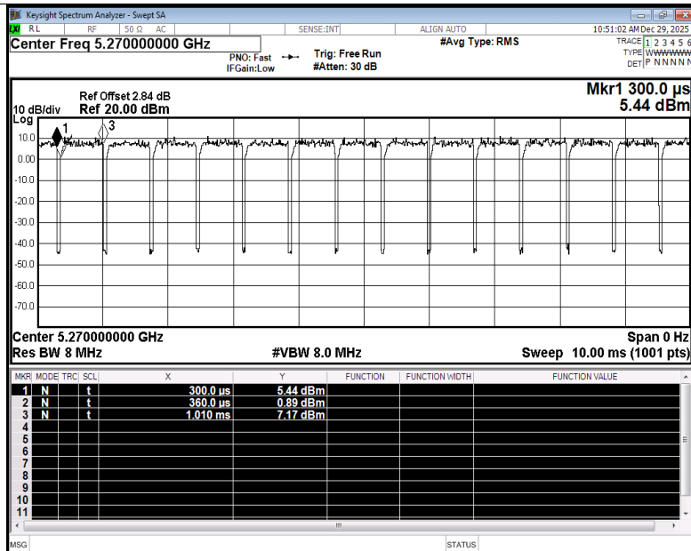
Duty Cycle NVNT ac40 5270MHz Ant3
