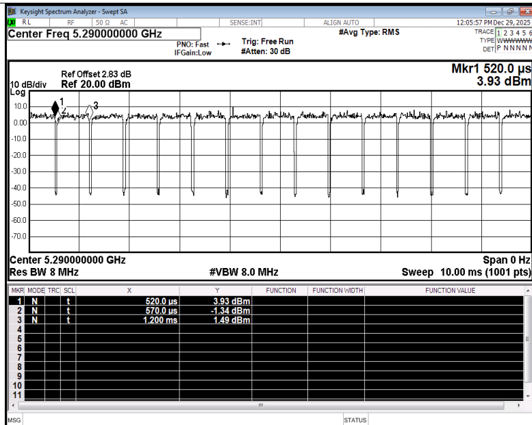
Duty Cycle NVNT ac80 5290MHz Ant4
