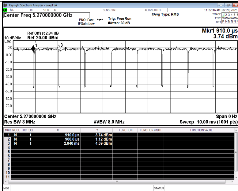
Duty Cycle NVNT be40 5270MHz Ant3
