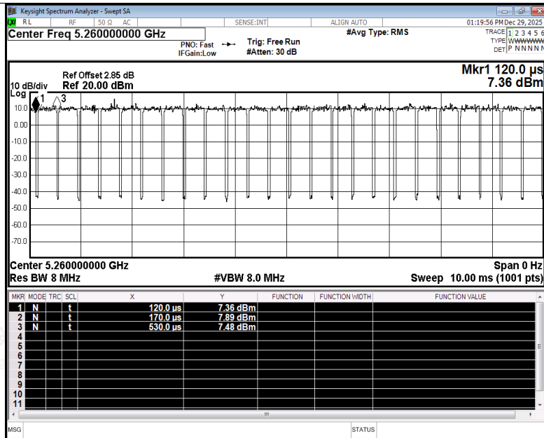
Duty Cycle NVNT be20 5260MHz Ant5
