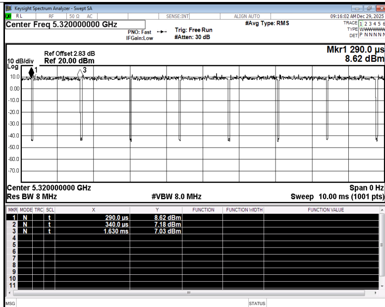
Duty Cycle NVNT n20 5320MHz Ant2
