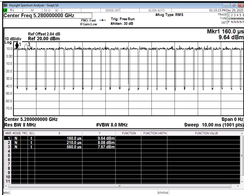
Duty Cycle NVNT ax20 5280MHz Ant5
