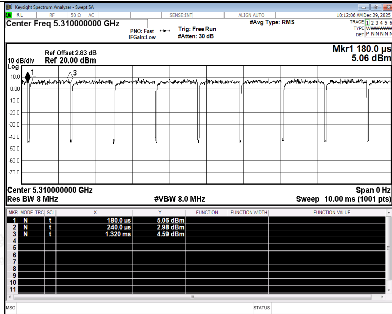
Duty Cycle NVNT be40 5310MHz Ant2
