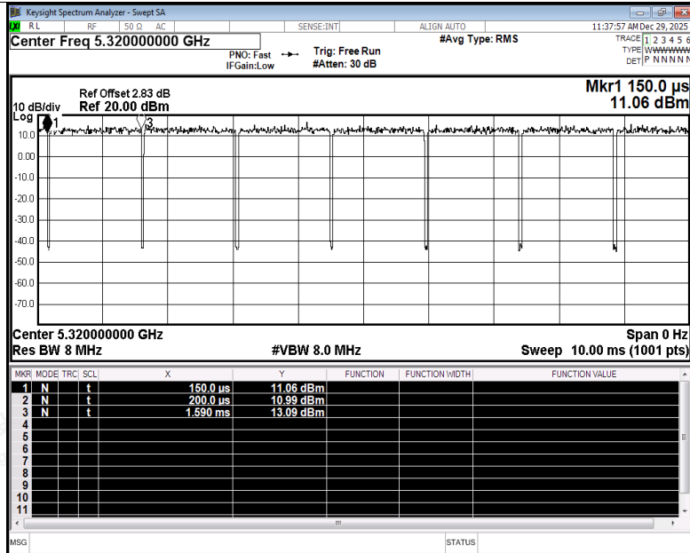
Duty Cycle NVNT a 5320MHz Ant4
