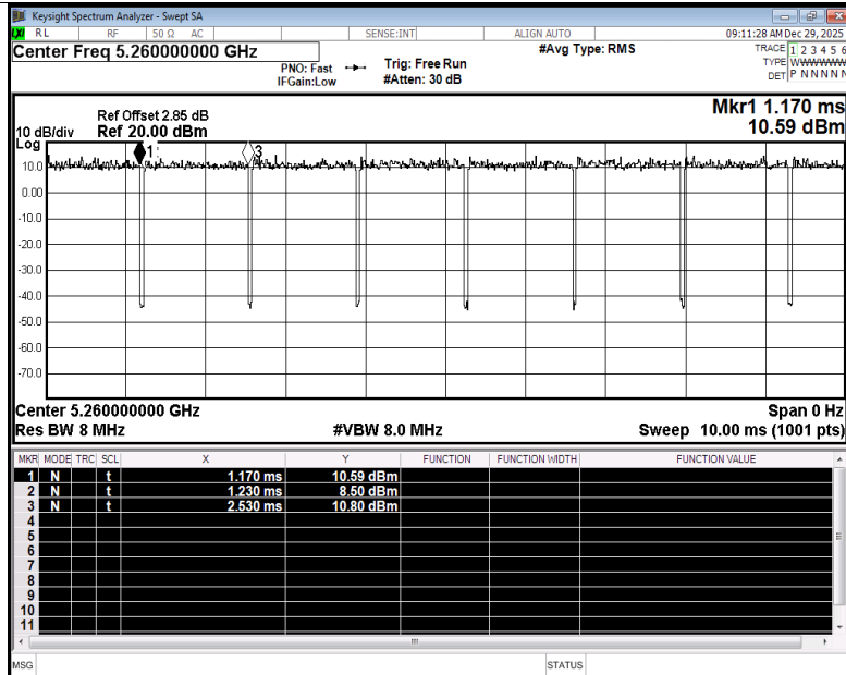
Duty Cycle NVNT n20 5260MHz Ant2
