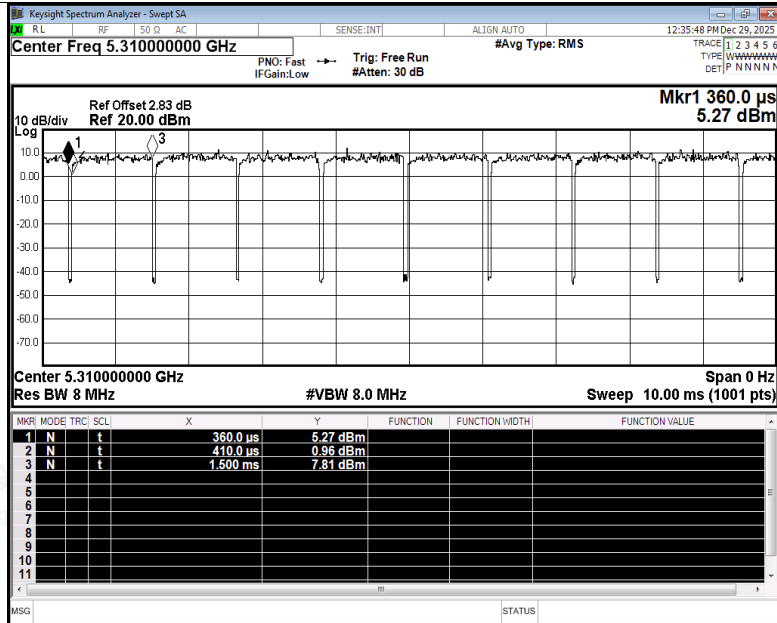
Duty Cycle NVNT be40 5310MHz Ant4
