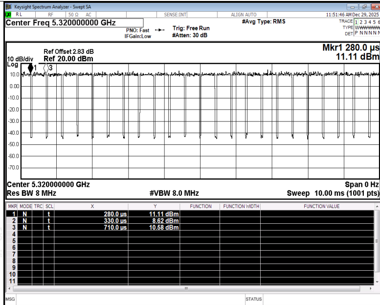
Duty Cycle NVNT ac20 5320MHz Ant4
