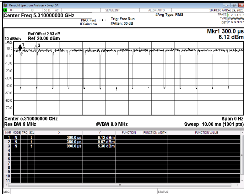
Duty Cycle NVNT n40 5310MHz Ant3
