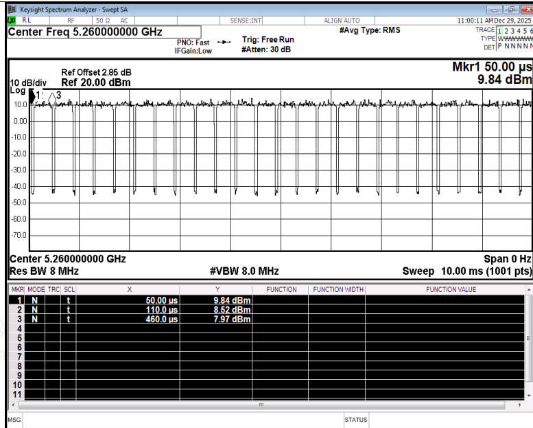
Duty Cycle NVNT ax20 5260MHz Ant3
