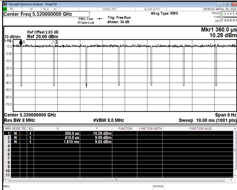
Duty Cycle NVNT a 5320MHz Ant2
