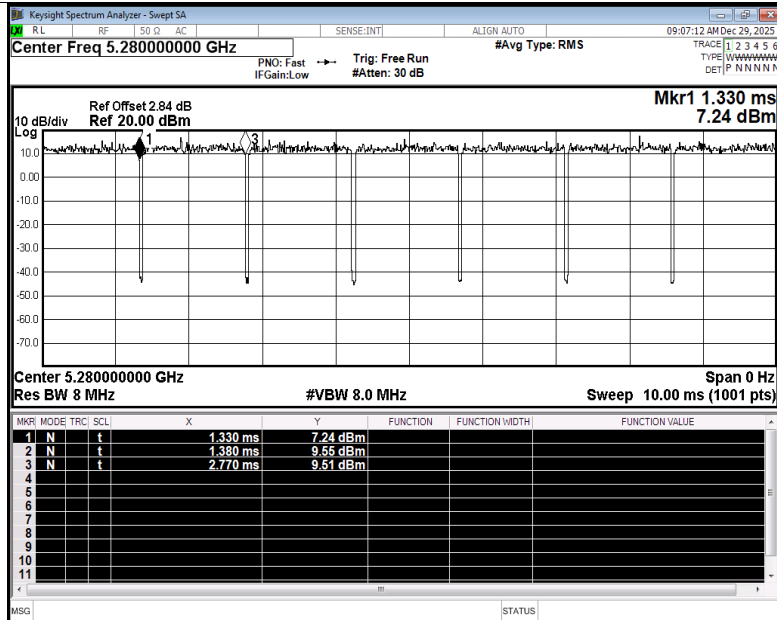
Duty Cycle NVNT a 5280MHz Ant2
