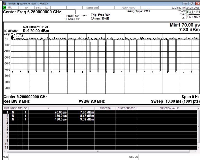
Duty Cycle NVNT be20 5260MHz Ant4
