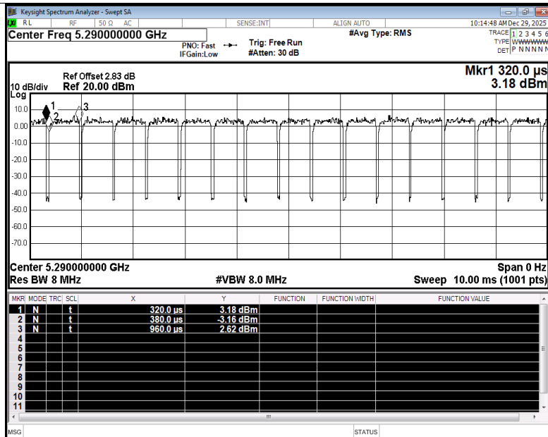
Duty Cycle NVNT be80 5290MHz Ant2
