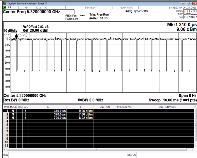
Duty Cycle NVNT ax20 5320MHz Ant1
