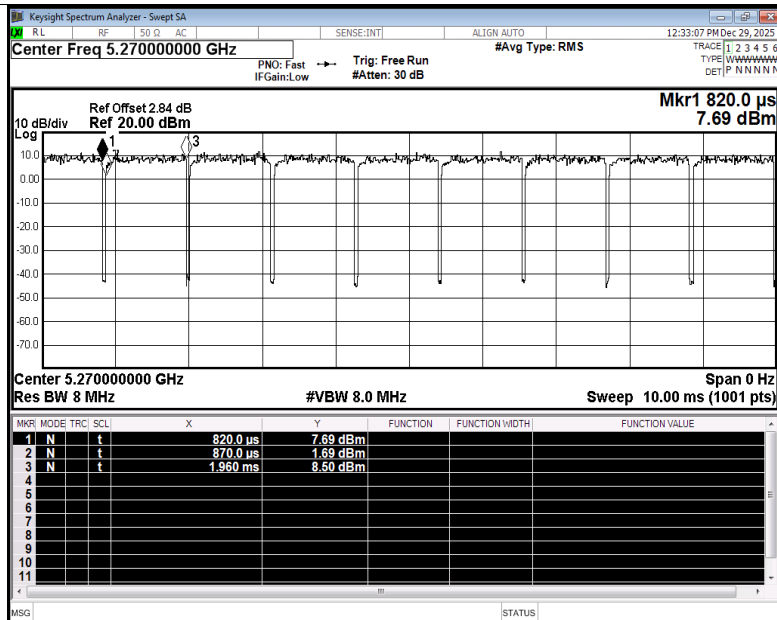
Duty Cycle NVNT be40 5270MHz Ant4
