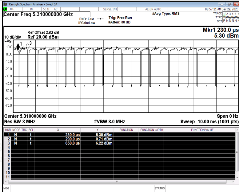
Duty Cycle NVNT be40 5310MHz Ant1
