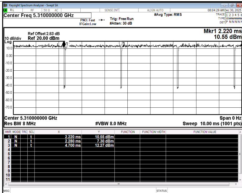
Duty Cycle NVNT n40 5310MHz Ant5
