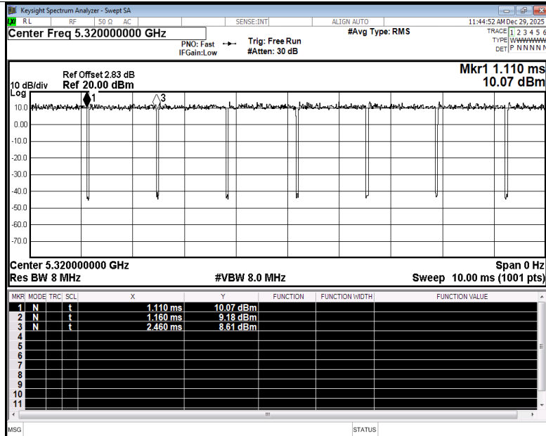
Duty Cycle NVNT n20 5320MHz Ant4
