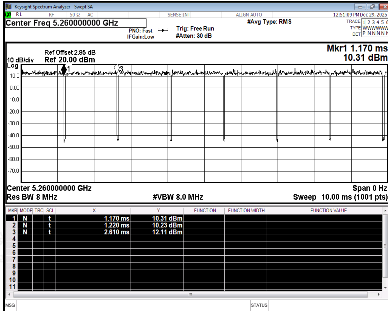
Duty Cycle NVNT a 5260MHz Ant5
