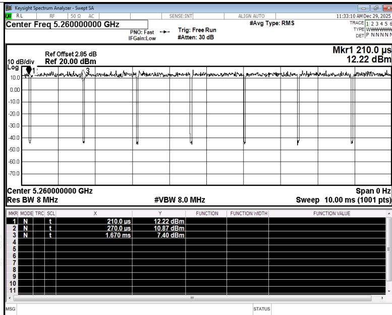
Duty Cycle NVNT a 5260MHz Ant4
