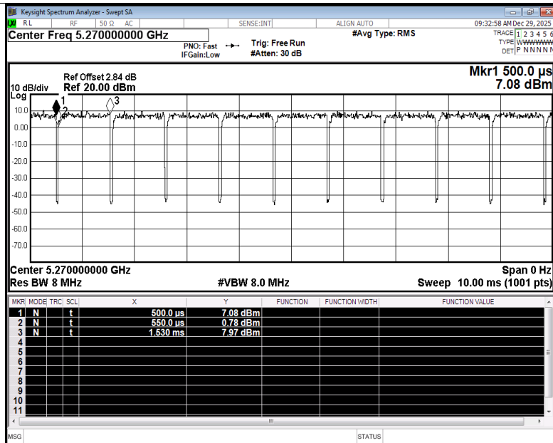
Duty Cycle NVNT ac40 5270MHz Ant2
