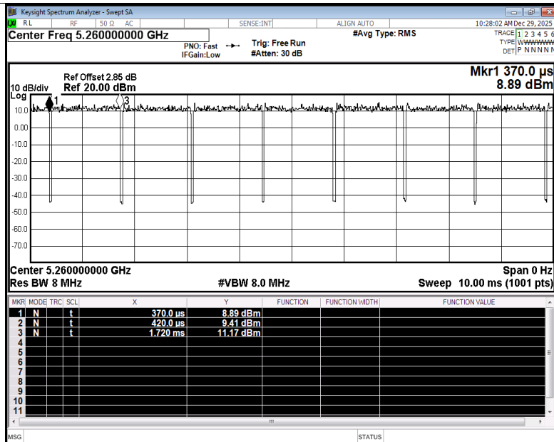
Duty Cycle NVNT n20 5260MHz Ant3
