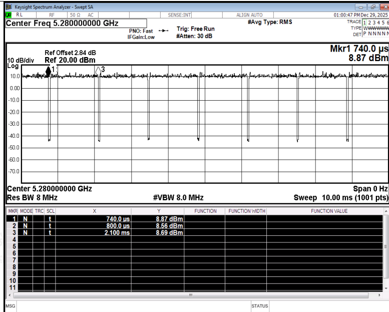
Duty Cycle NVNT n20 5280MHz Ant5
