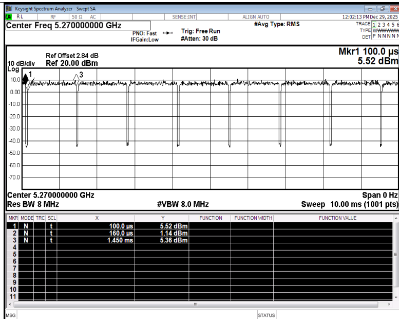
Duty Cycle NVNT ac40 5270MHz Ant4
