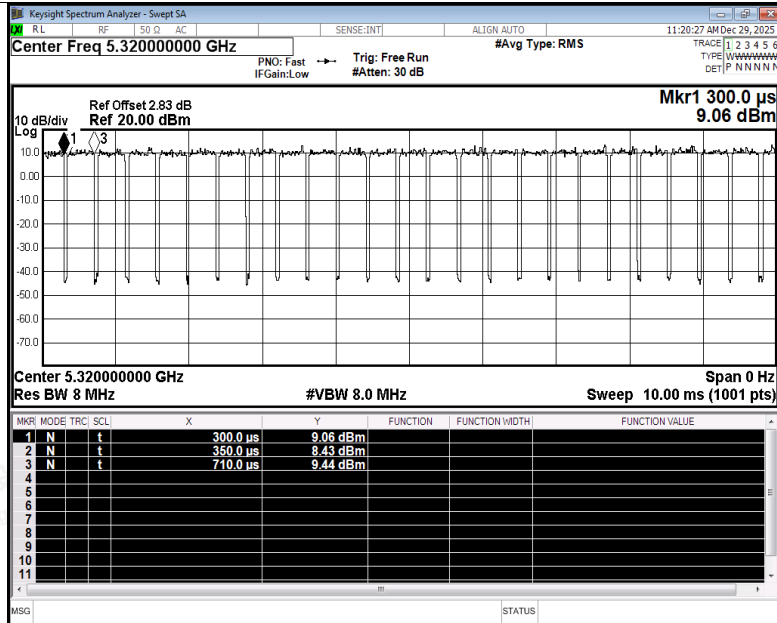
Duty Cycle NVNT be20 5320MHz Ant3
