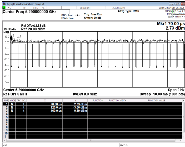
Duty Cycle NVNT ax80 5290MHz Ant2
