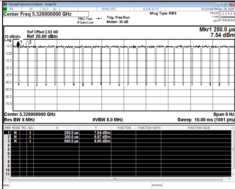
Duty Cycle NVNT be20 5320MHz Ant5
