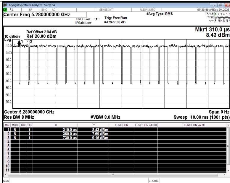
Duty Cycle NVNT ac20 5280MHz Ant2
