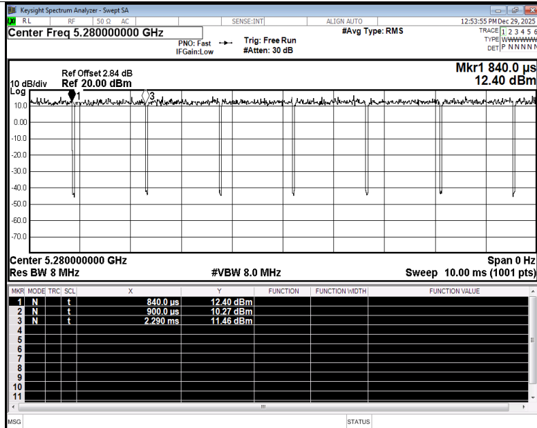
Duty Cycle NVNT a 5280MHz Ant5
