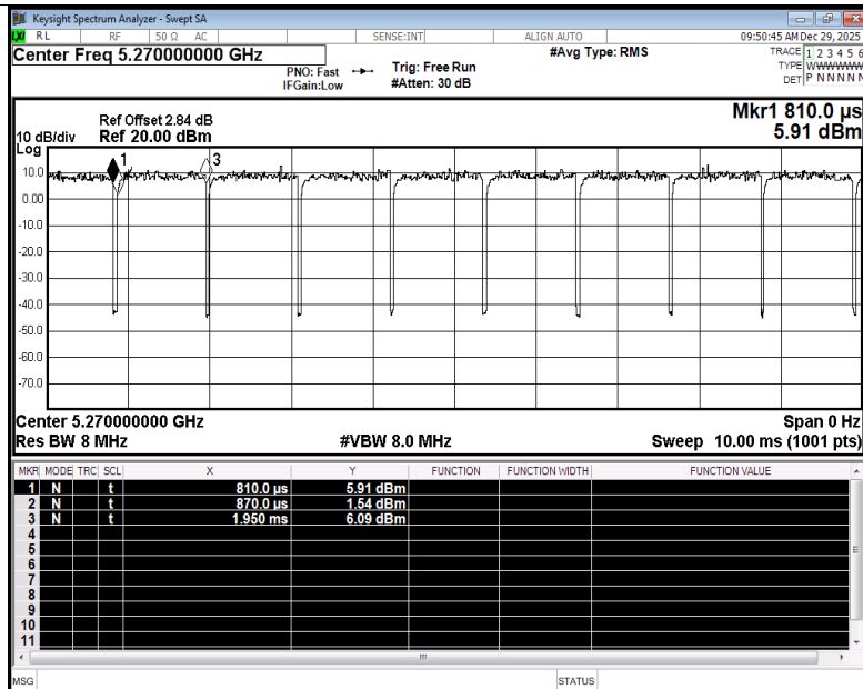
Duty Cycle NVNT ax40 5270MHz Ant2
