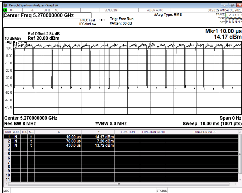
Duty Cycle NVNT be40 5270MHz Ant5
