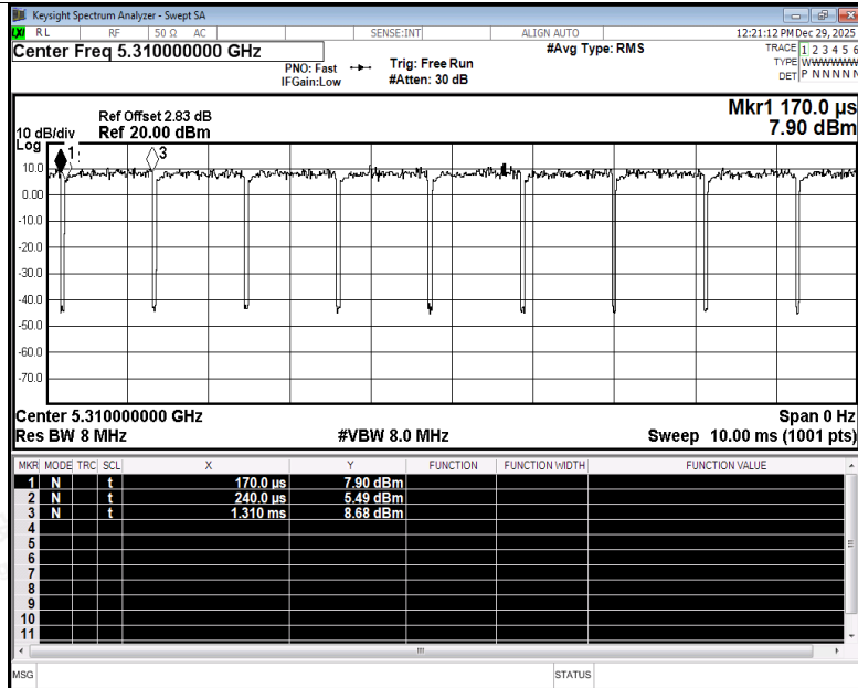
Duty Cycle NVNT ax40 5310MHz Ant4
