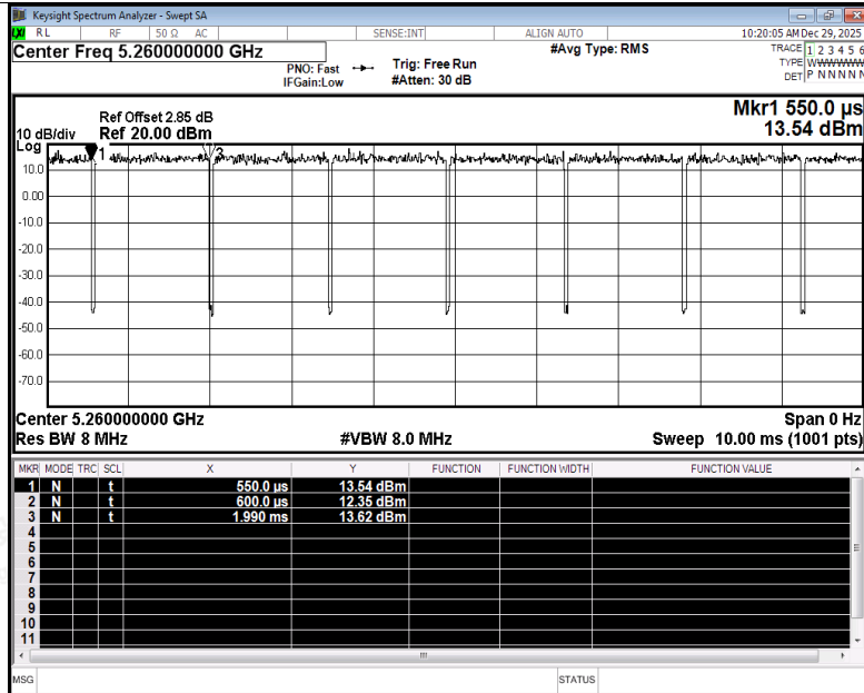
Duty Cycle NVNT a 5260MHz Ant3
