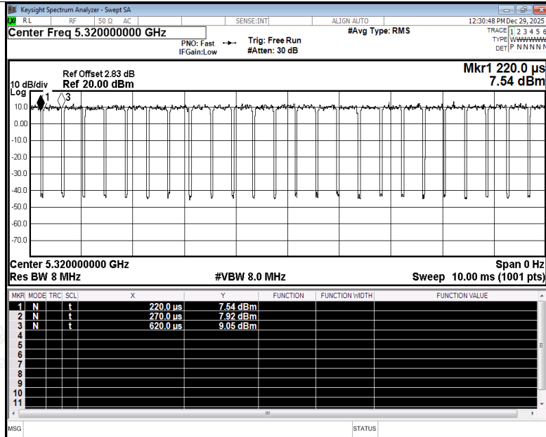
Duty Cycle NVNT be20 5320MHz Ant4
