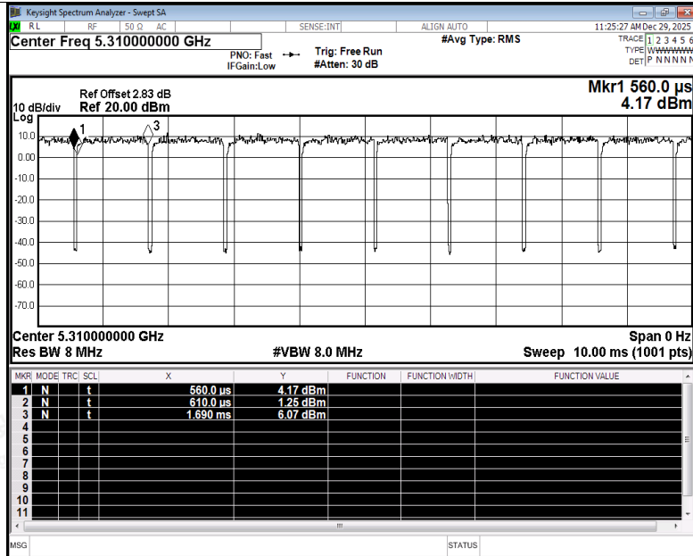
Duty Cycle NVNT be40 5310MHz Ant3
