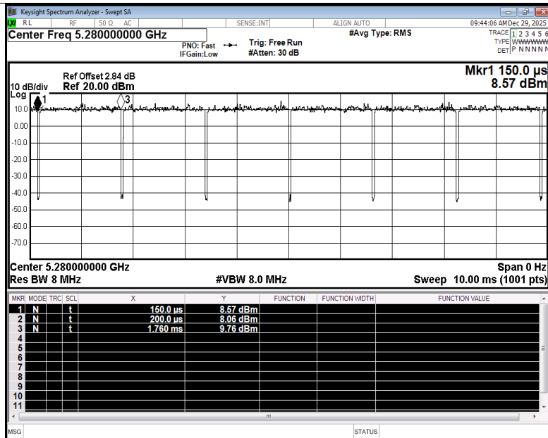
Duty Cycle NVNT ax20 5280MHz Ant2
