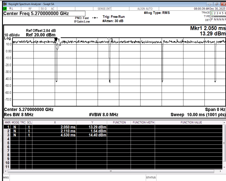
Duty Cycle NVNT n40 5270MHz Ant5
