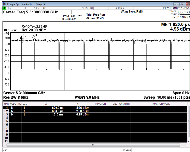
Duty Cycle NVNT n40 5310MHz Ant2
