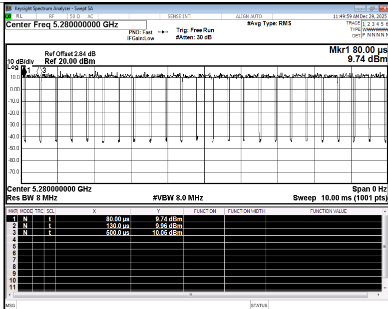
Duty Cycle NVNT ac20 5280MHz Ant4
