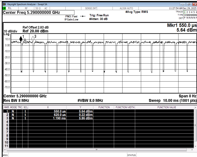
Duty Cycle NVNT be80 5290MHz Ant3
