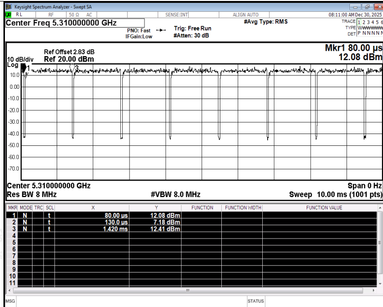
Duty Cycle NVNT ac40 5310MHz Ant5
