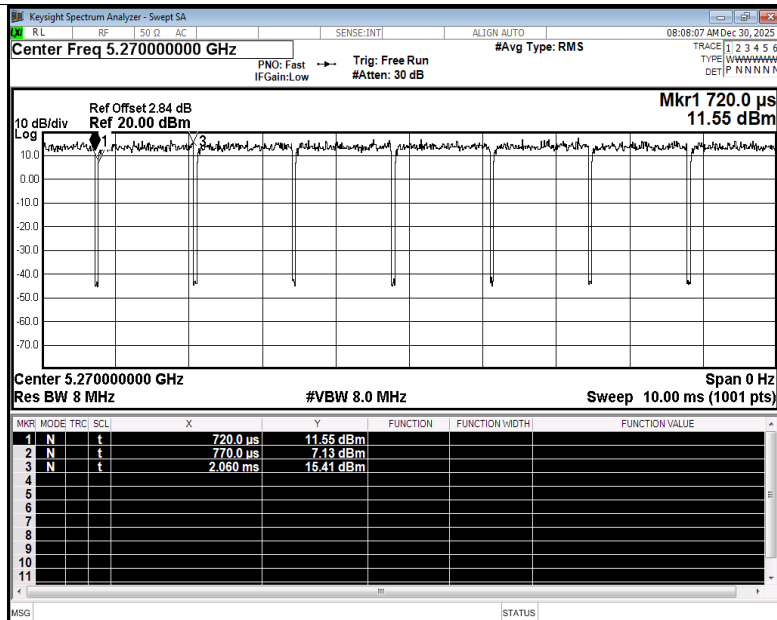
Duty Cycle NVNT ac40 5270MHz Ant5
