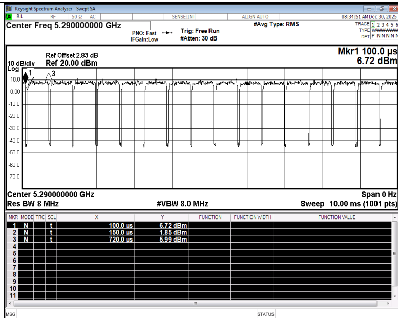
Duty Cycle NVNT ax80 5290MHz Ant5
