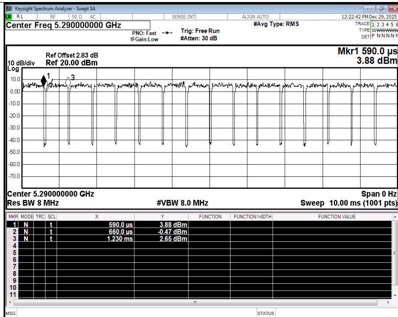
Duty Cycle NVNT ax80 5290MHz Ant4
