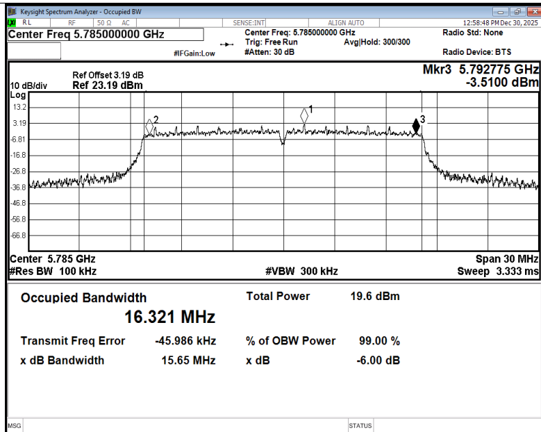
-6dB Bandwidth NVNT a 5785MHz Ant5
