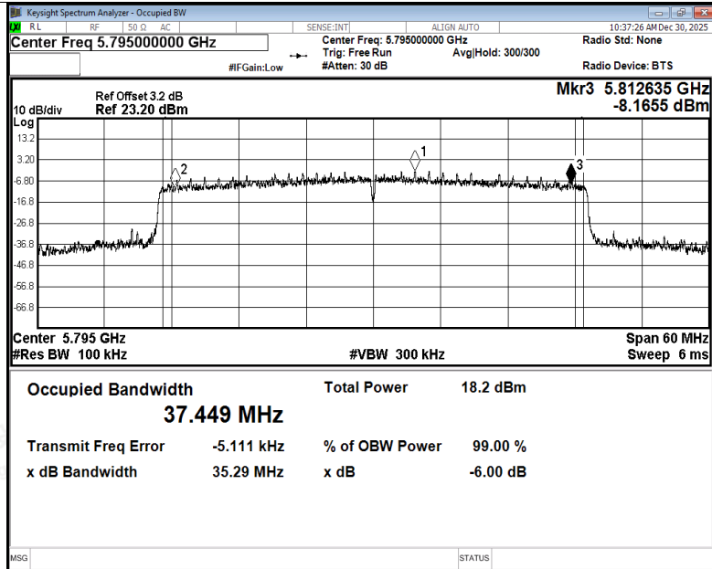
-6dB Bandwidth NVNT ax40 5795MHz Ant2
