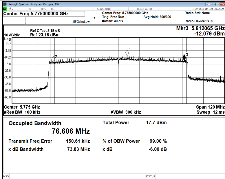
-6dB Bandwidth NVNT be80 5775MHz Ant2
