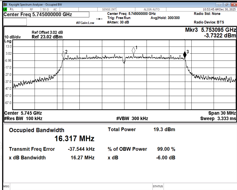
-6dB Bandwidth NVNT a 5745MHz Ant3
