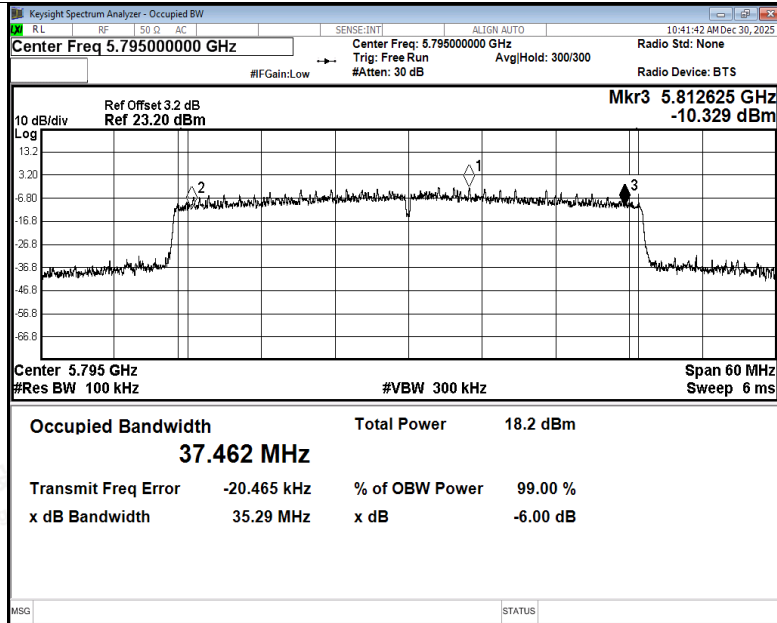
-6dB Bandwidth NVNT be40 5795MHz Ant2
