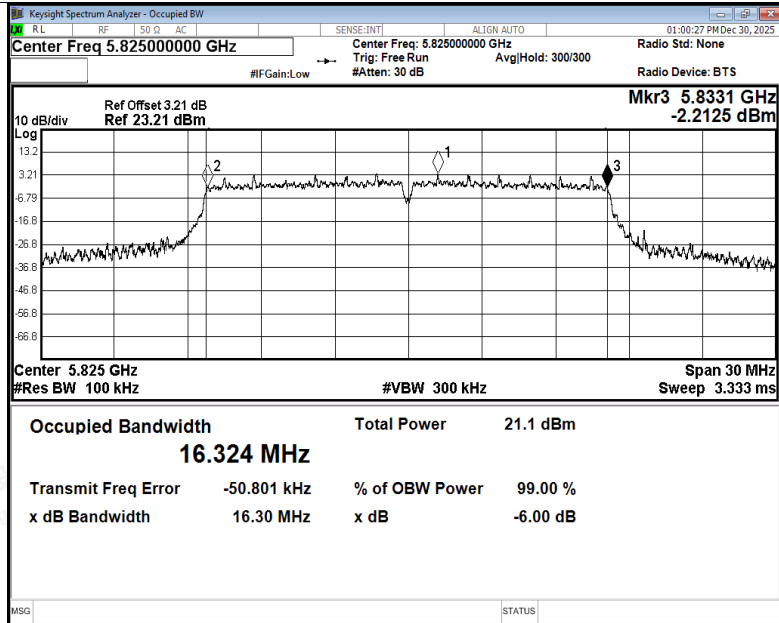
-6dB Bandwidth NVNT a 5825MHz Ant5
