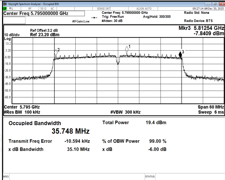
-6dB Bandwidth NVNT ac40 5795MHz Ant1
