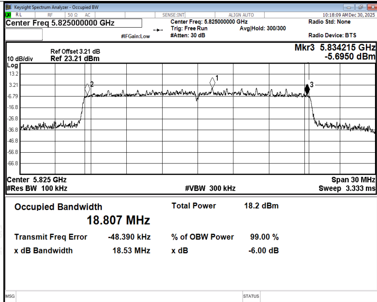
-6dB Bandwidth NVNT ax20 5825MHz Ant2
