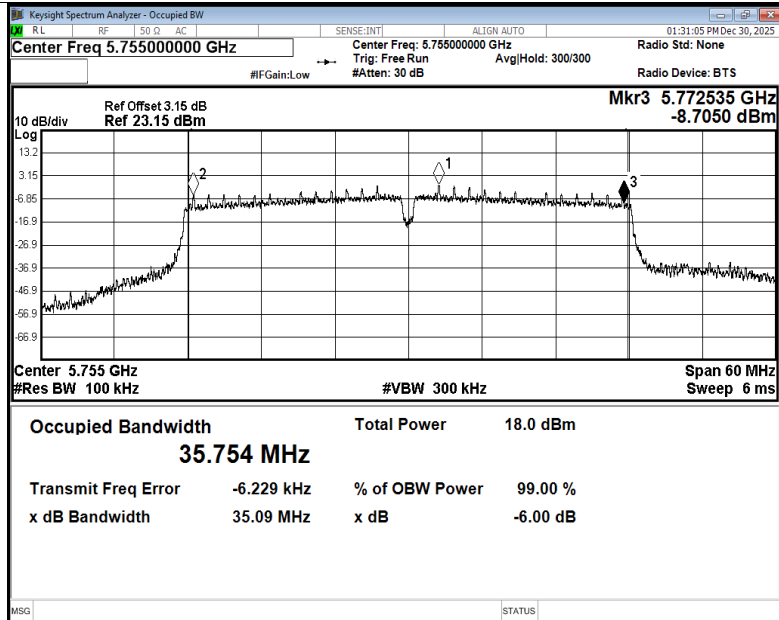
-6dB Bandwidth NVNT ac40 5755MHz Ant5
