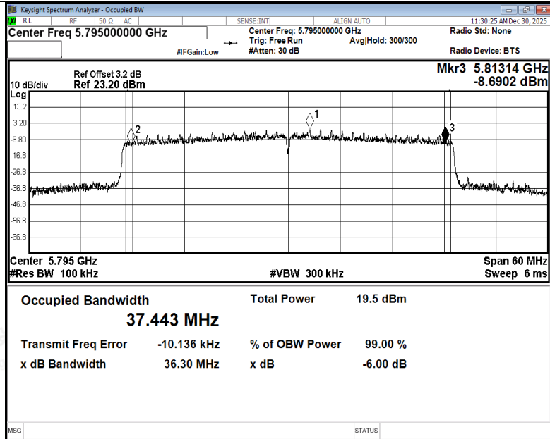
-6dB Bandwidth NVNT ax40 5795MHz Ant3
