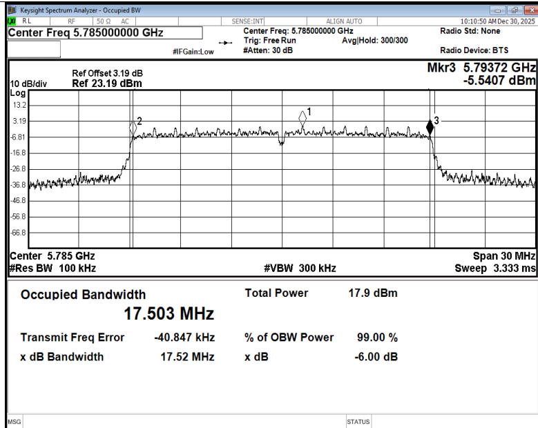
-6dB Bandwidth NVNT ac20 5785MHz Ant2
