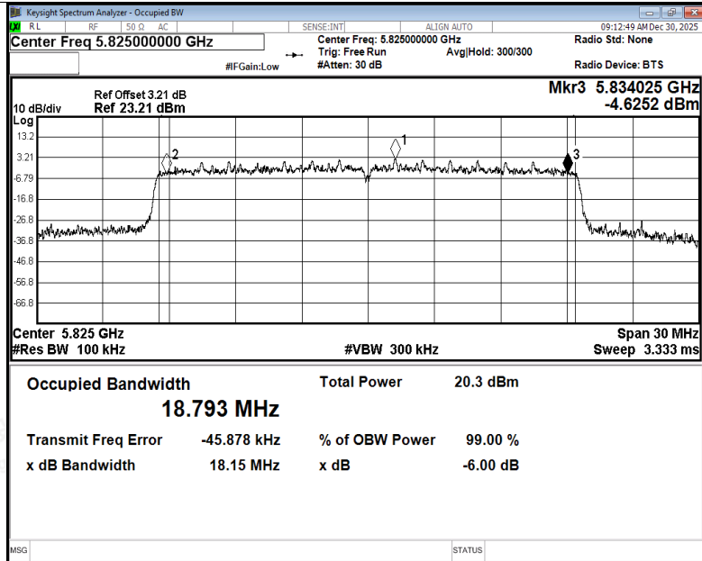
-6dB Bandwidth NVNT ax20 5825MHz Ant1
