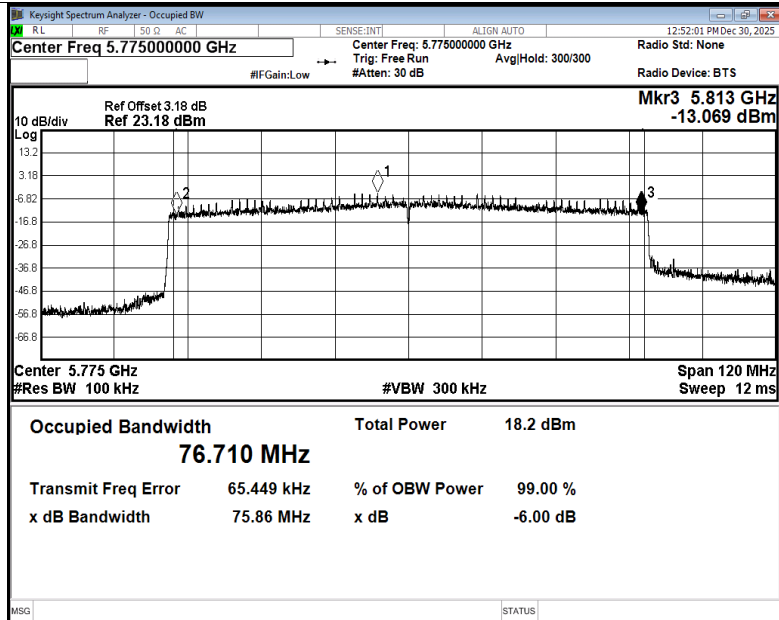
-6dB Bandwidth NVNT be80 5775MHz Ant4
