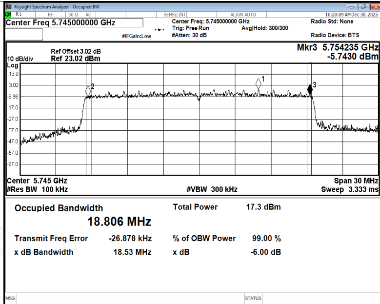
-6dB Bandwidth NVNT be20 5745MHz Ant2
