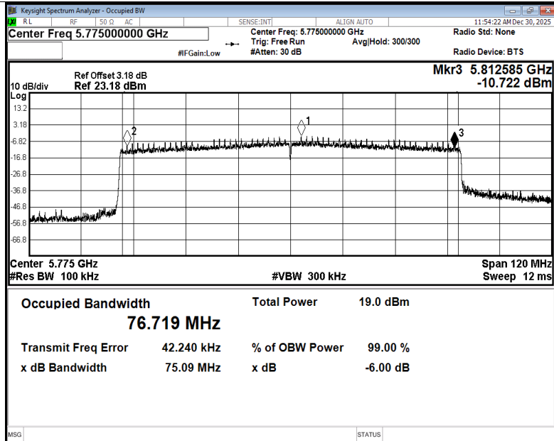
-6dB Bandwidth NVNT be80 5775MHz Ant3
