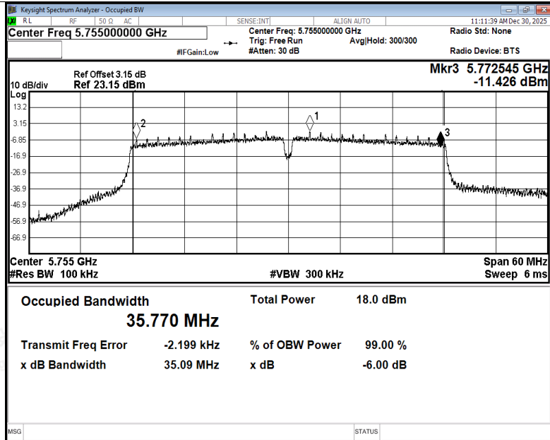
-6dB Bandwidth NVNT n40 5755MHz Ant3
