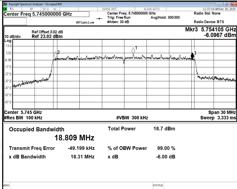
-6dB Bandwidth NVNT ax20 5745MHz Ant3
