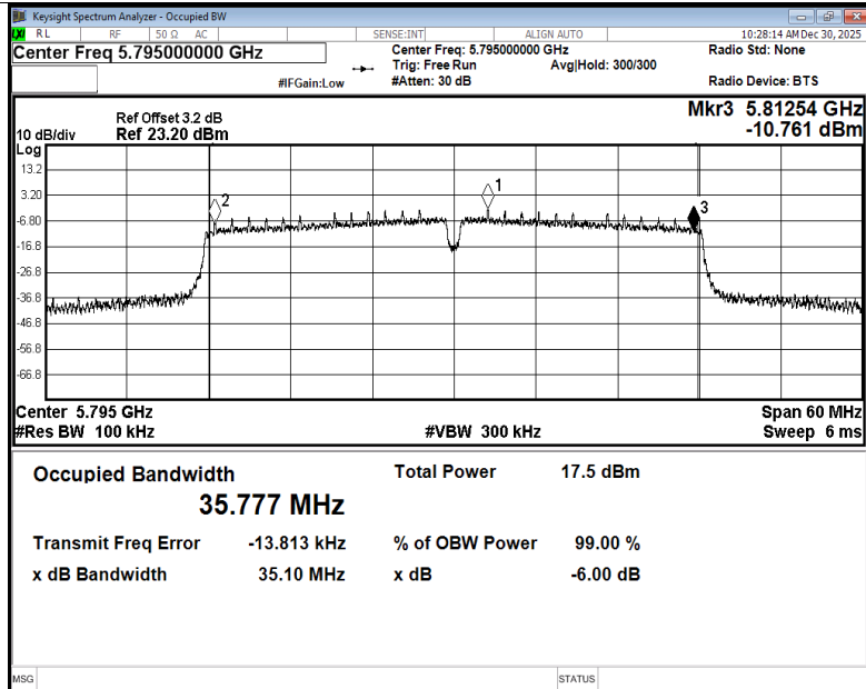
-6dB Bandwidth NVNT n40 5795MHz Ant2
