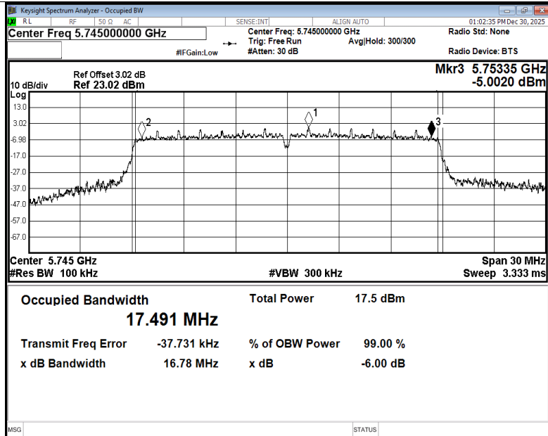
-6dB Bandwidth NVNT n20 5745MHz Ant5
