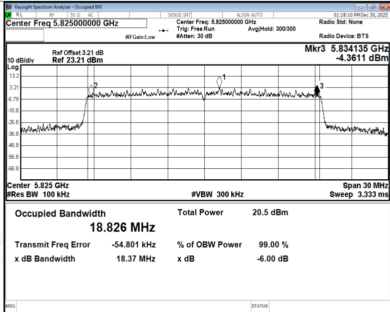
-6dB Bandwidth NVNT ax20 5825MHz Ant5
