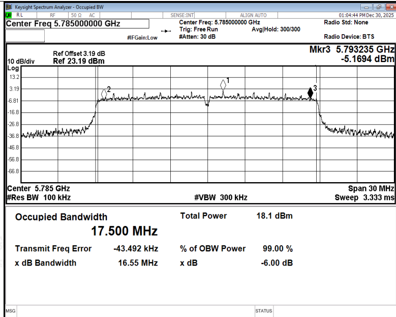
-6dB Bandwidth NVNT n20 5785MHz Ant5
