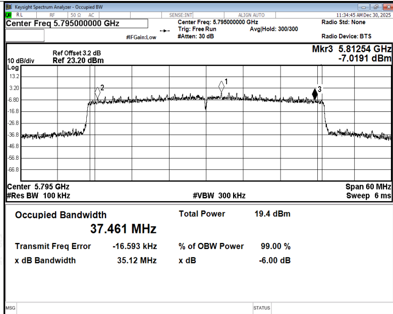
-6dB Bandwidth NVNT be40 5795MHz Ant3
