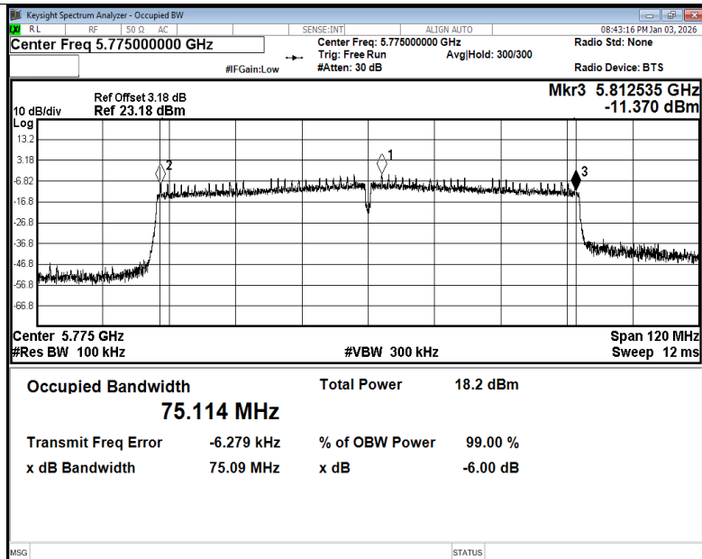
-6dB Bandwidth NVNT ac80 5775MHz Ant5
