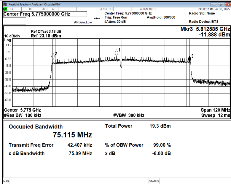
-6dB Bandwidth NVNT ac80 5775MHz Ant1
