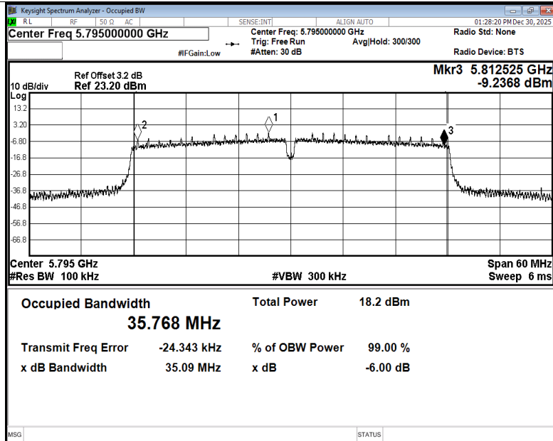
-6dB Bandwidth NVNT n40 5795MHz Ant5
