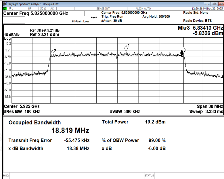
-6dB Bandwidth NVNT ax20 5825MHz Ant4
