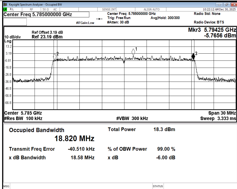
-6dB Bandwidth NVNT be20 5785MHz Ant2
