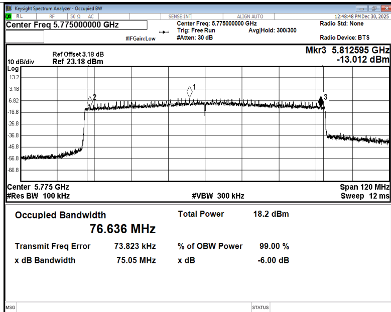
-6dB Bandwidth NVNT ax80 5775MHz Ant4
