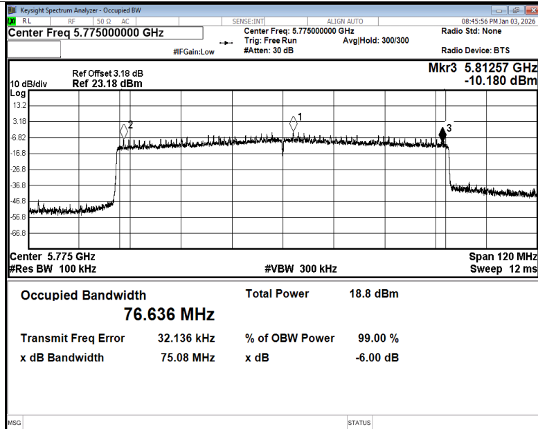
-6dB Bandwidth NVNT ax80 5775MHz Ant5
