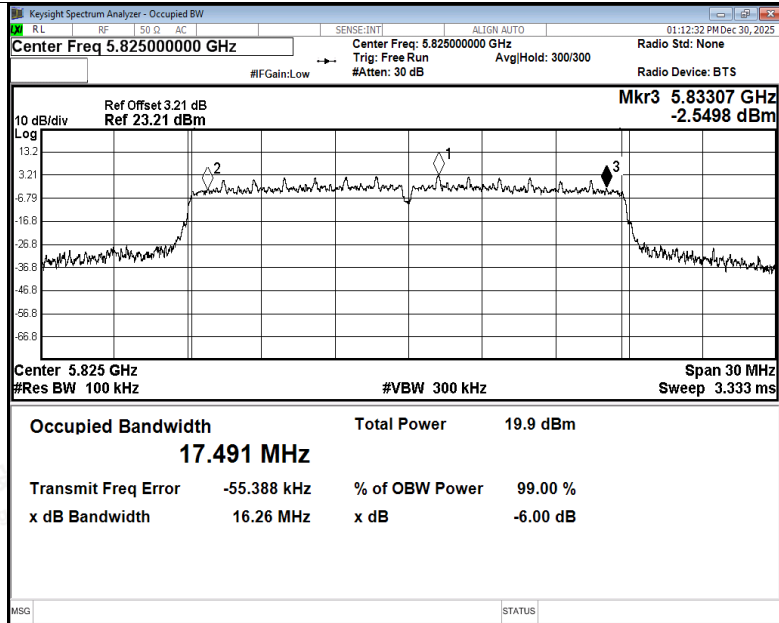
-6dB Bandwidth NVNT ac20 5825MHz Ant5
