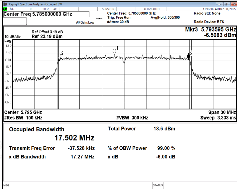
-6dB Bandwidth NVNT n20 5785MHz Ant3
