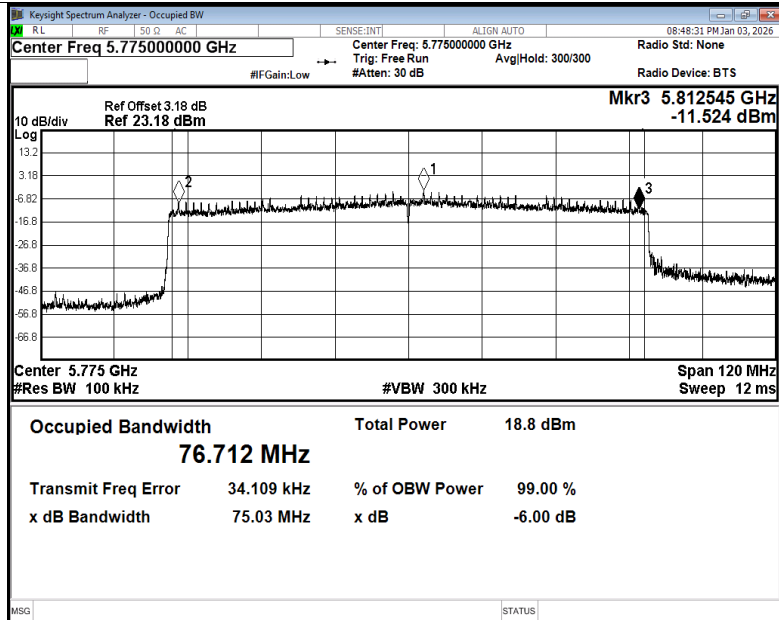
-6dB Bandwidth NVNT be80 5775MHz Ant5
