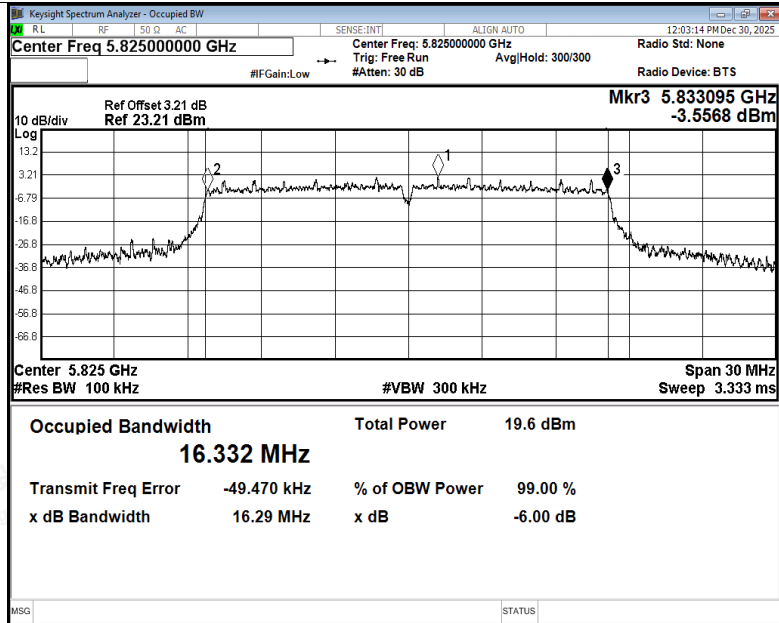
-6dB Bandwidth NVNT a 5825MHz Ant4
