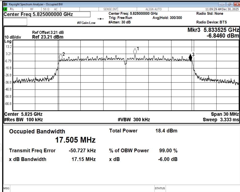
-6dB Bandwidth NVNT ac20 5825MHz Ant3
