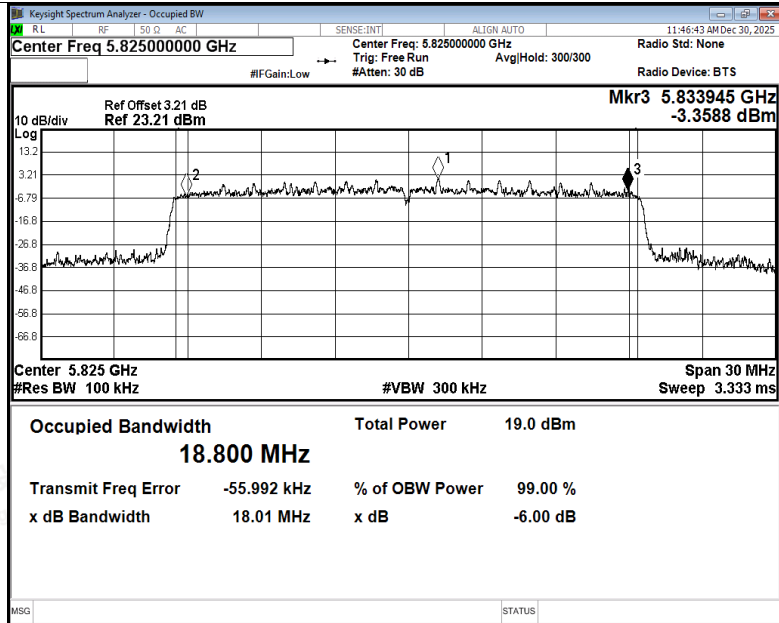
-6dB Bandwidth NVNT be20 5825MHz Ant3
