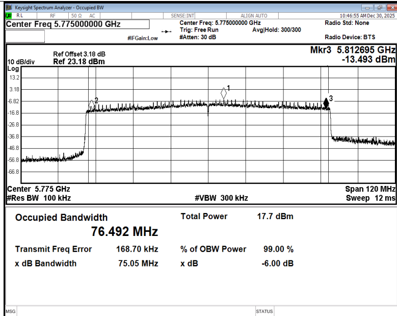
-6dB Bandwidth NVNT ax80 5775MHz Ant2
