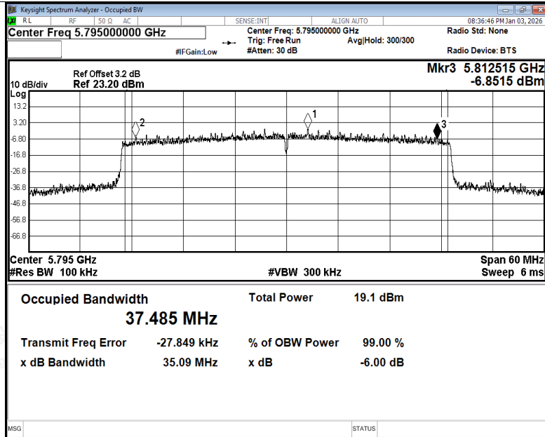
-6dB Bandwidth NVNT ax40 5795MHz Ant5
