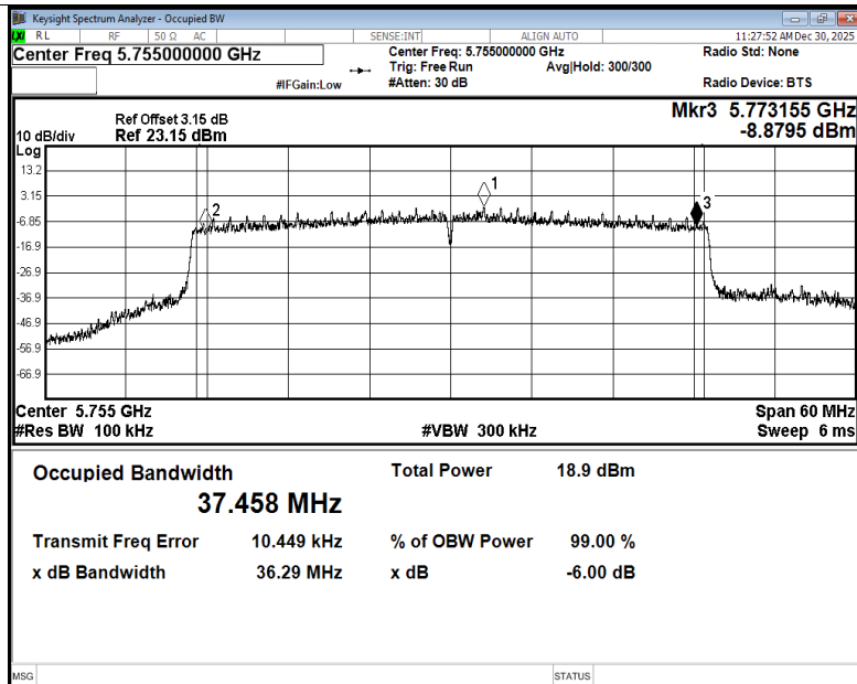
-6dB Bandwidth NVNT ax40 5755MHz Ant3
