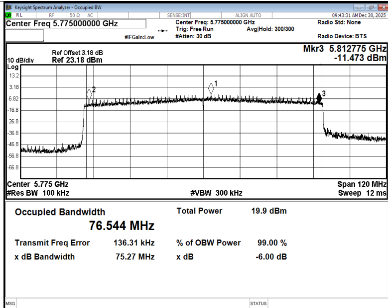
-6dB Bandwidth NVNT be80 5775MHz Ant1
