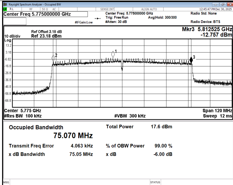
-6dB Bandwidth NVNT ac80 5775MHz Ant4
