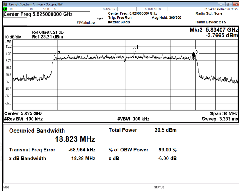
-6dB Bandwidth NVNT be20 5825MHz Ant5
