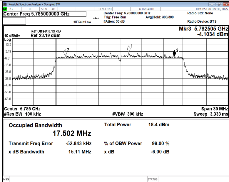
-6dB Bandwidth NVNT ac20 5785MHz Ant5
