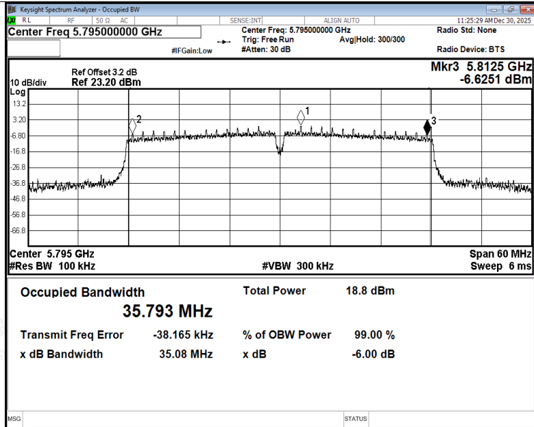
-6dB Bandwidth NVNT ac40 5795MHz Ant3
