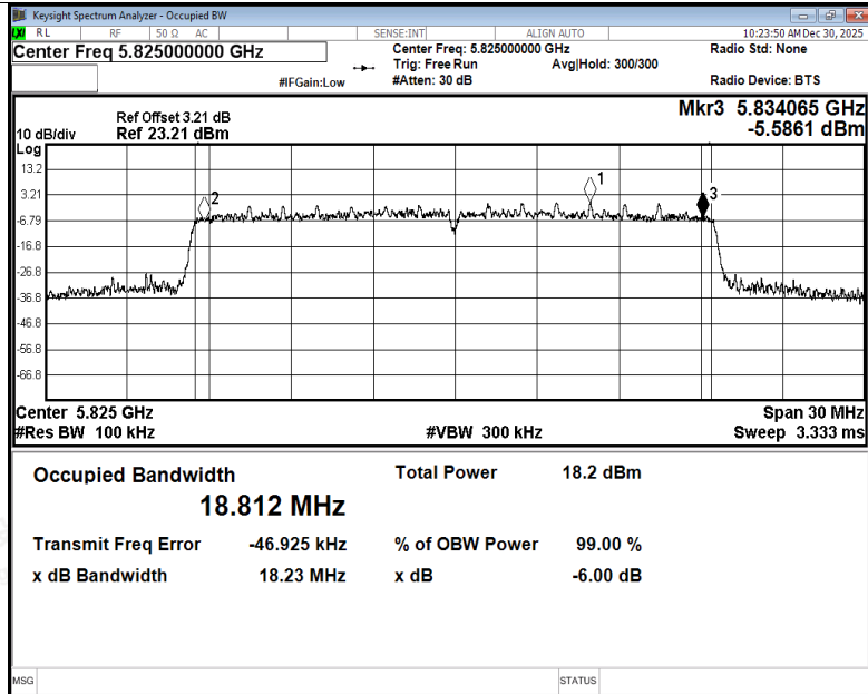
-6dB Bandwidth NVNT be20 5825MHz Ant2
