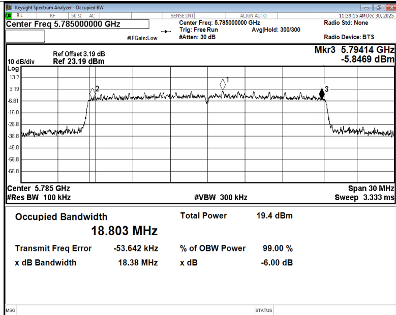
-6dB Bandwidth NVNT ax20 5785MHz Ant3
