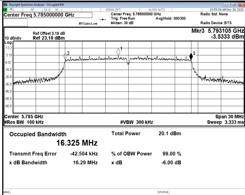
-6dB Bandwidth NVNT a 5785MHz Ant3
