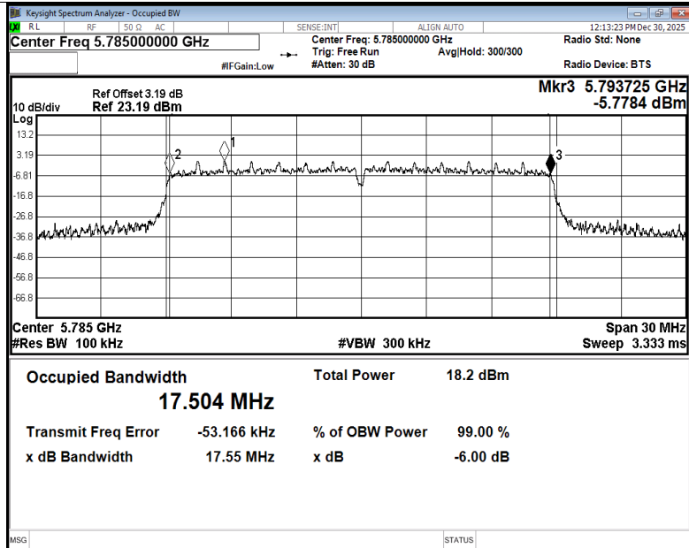
-6dB Bandwidth NVNT ac20 5785MHz Ant4
