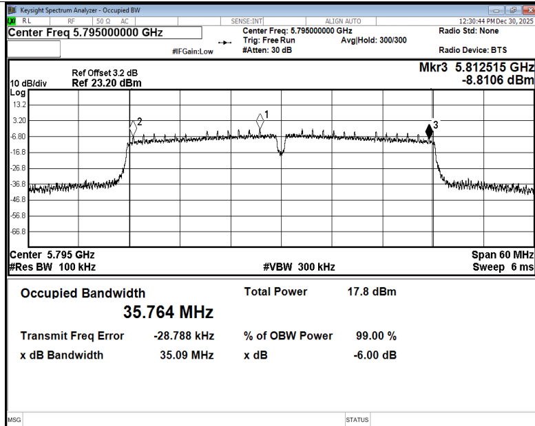
-6dB Bandwidth NVNT n40 5795MHz Ant4
