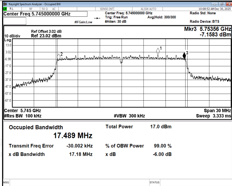
-6dB Bandwidth NVNT ac20 5745MHz Ant2
