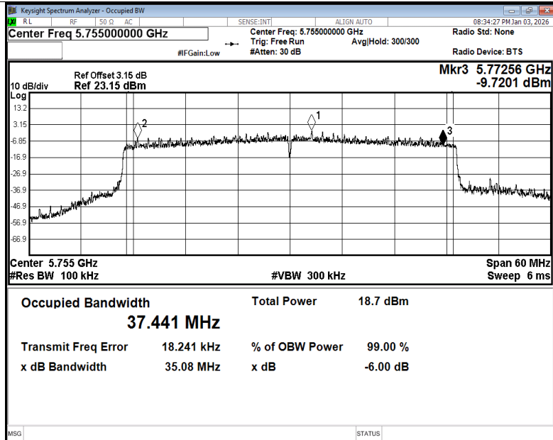
-6dB Bandwidth NVNT ax40 5755MHz Ant5
