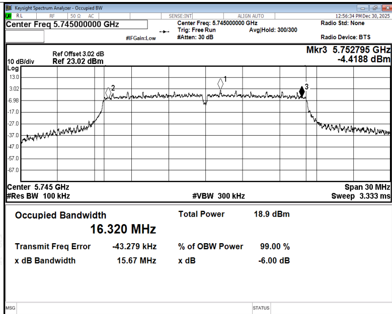
-6dB Bandwidth NVNT a 5745MHz Ant5
