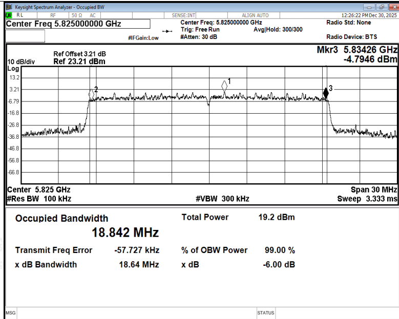
-6dB Bandwidth NVNT be20 5825MHz Ant4
