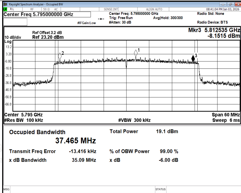
-6dB Bandwidth NVNT be40 5795MHz Ant5
