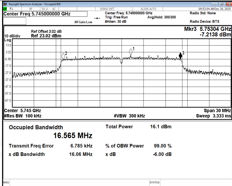
-6dB Bandwidth NVNT a 5745MHz Ant2
