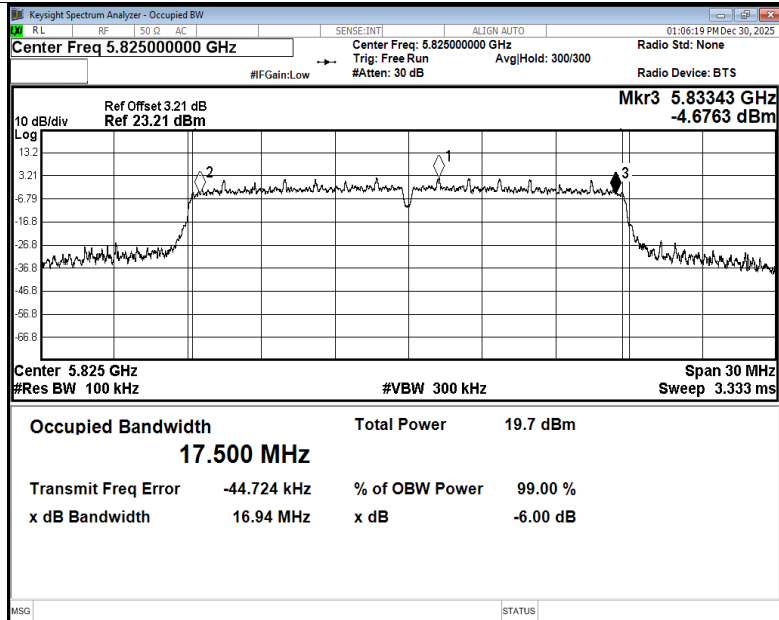
-6dB Bandwidth NVNT n20 5825MHz Ant5
