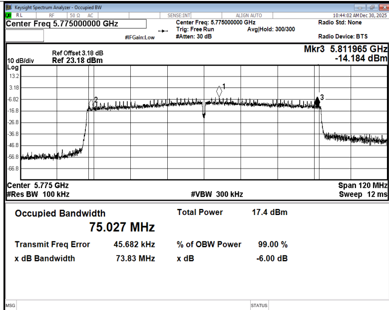
-6dB Bandwidth NVNT ac80 5775MHz Ant2
