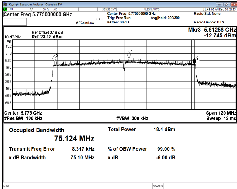
-6dB Bandwidth NVNT ac80 5775MHz Ant3
