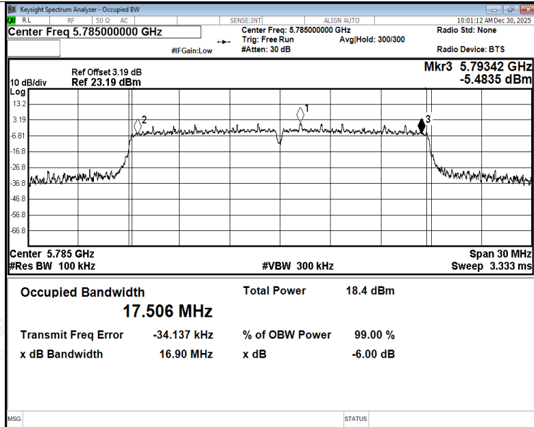
-6dB Bandwidth NVNT n20 5785MHz Ant2
