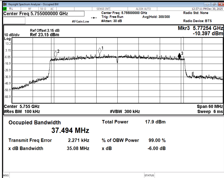
-6dB Bandwidth NVNT ax40 5755MHz Ant4
