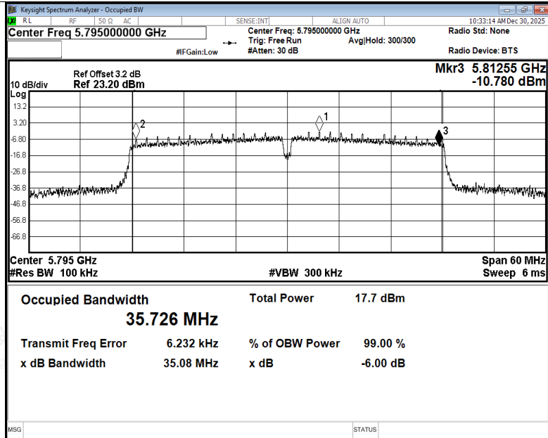
-6dB Bandwidth NVNT ac40 5795MHz Ant2
