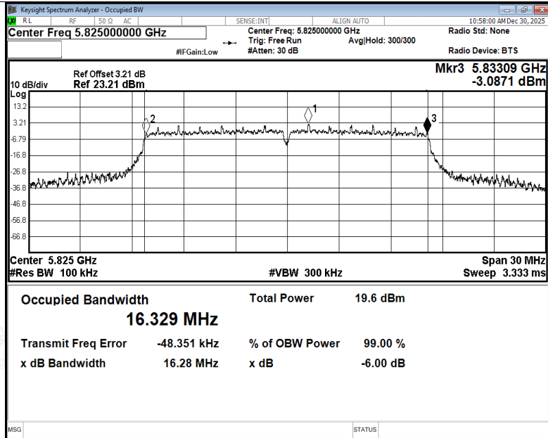
-6dB Bandwidth NVNT a 5825MHz Ant3
