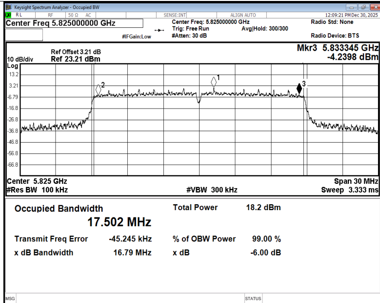
-6dB Bandwidth NVNT n20 5825MHz Ant4
