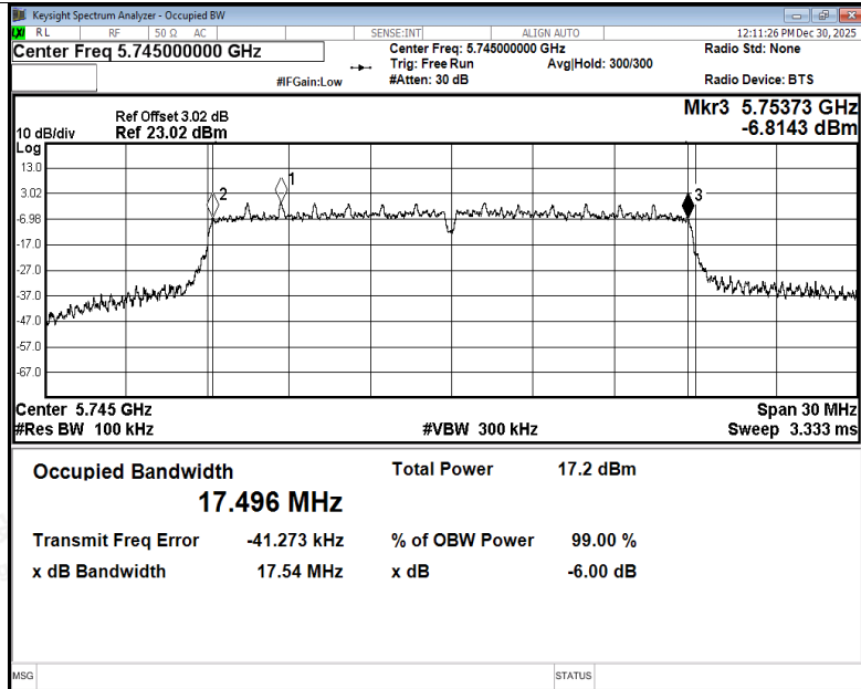
-6dB Bandwidth NVNT ac20 5745MHz Ant4
