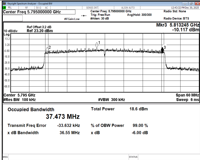
-6dB Bandwidth NVNT be40 5795MHz Ant4
