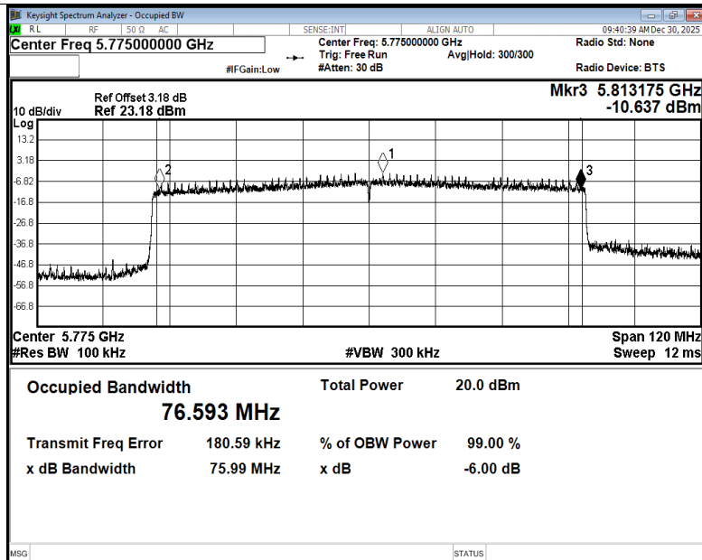
-6dB Bandwidth NVNT ax80 5775MHz Ant1
