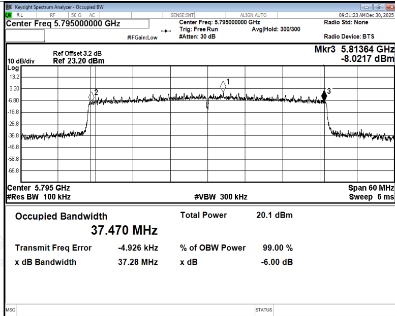
-6dB Bandwidth NVNT ax40 5795MHz Ant1
