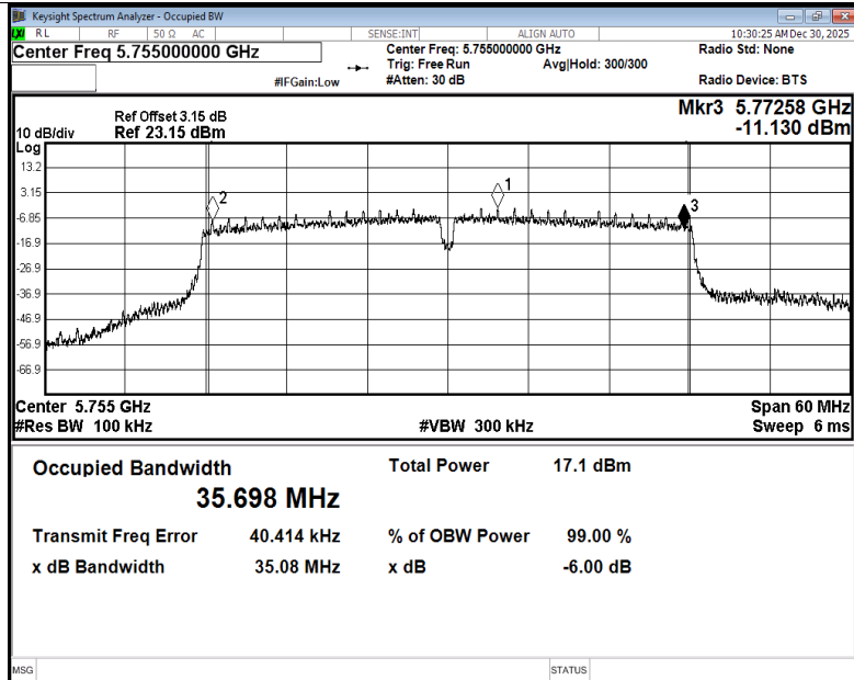
-6dB Bandwidth NVNT ac40 5755MHz Ant2
