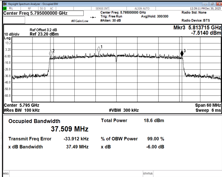
-6dB Bandwidth NVNT ax40 5795MHz Ant4
