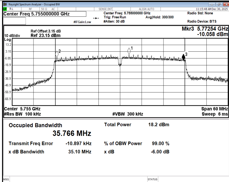
-6dB Bandwidth NVNT ac40 5755MHz Ant3
