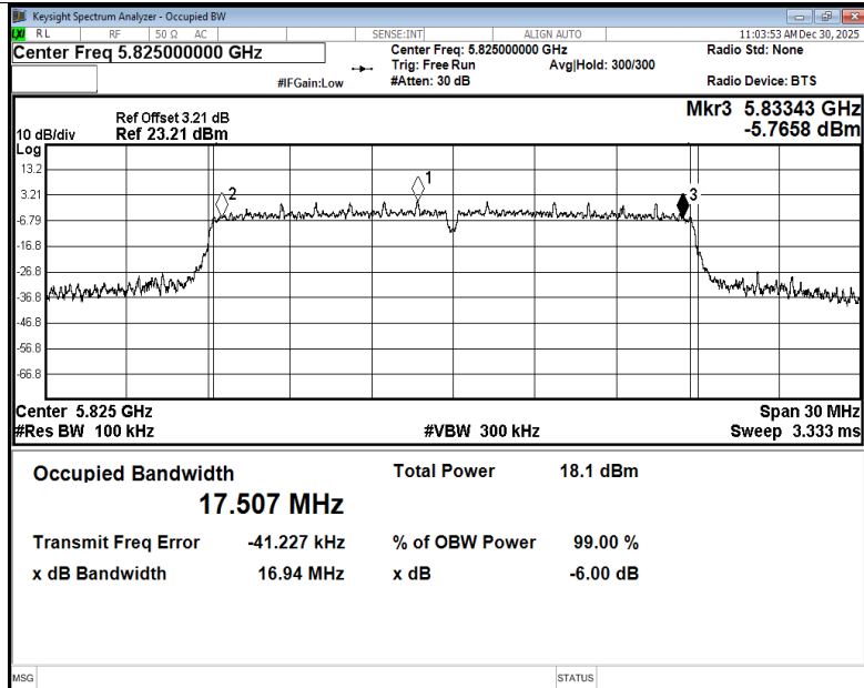
-6dB Bandwidth NVNT n20 5825MHz Ant3
