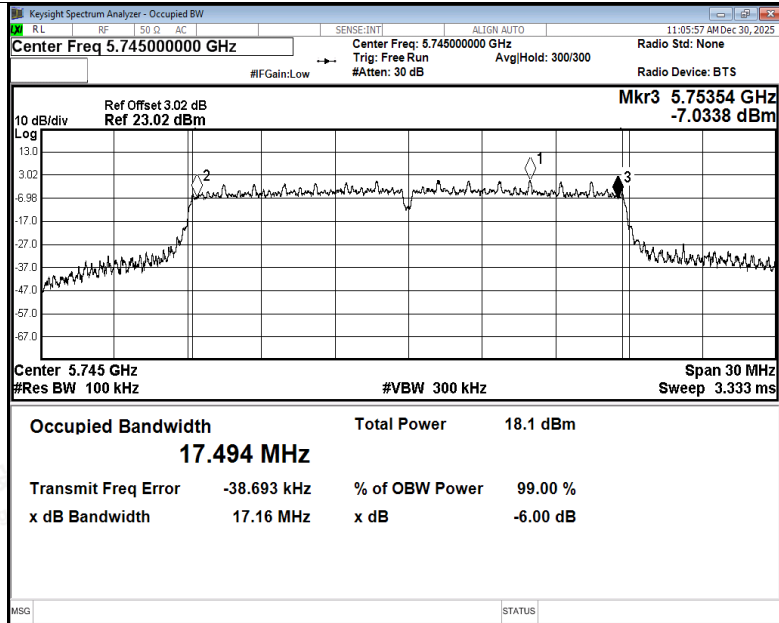
-6dB Bandwidth NVNT ac20 5745MHz Ant3
