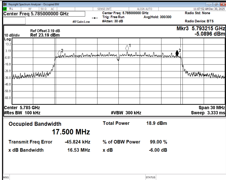
-6dB Bandwidth NVNT ac20 5785MHz Ant3
