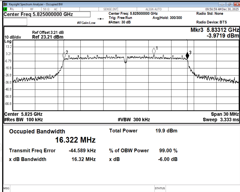
-6dB Bandwidth NVNT a 5825MHz Ant2
