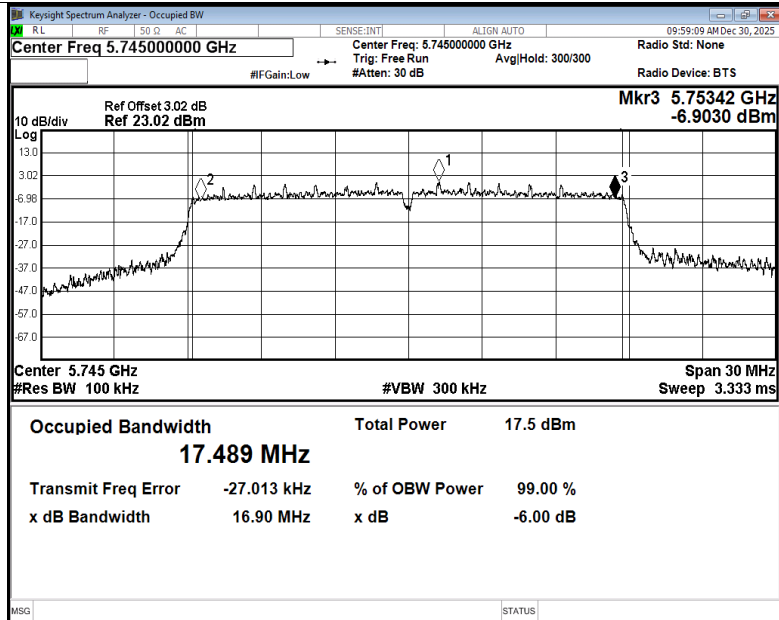
-6dB Bandwidth NVNT n20 5745MHz Ant2
