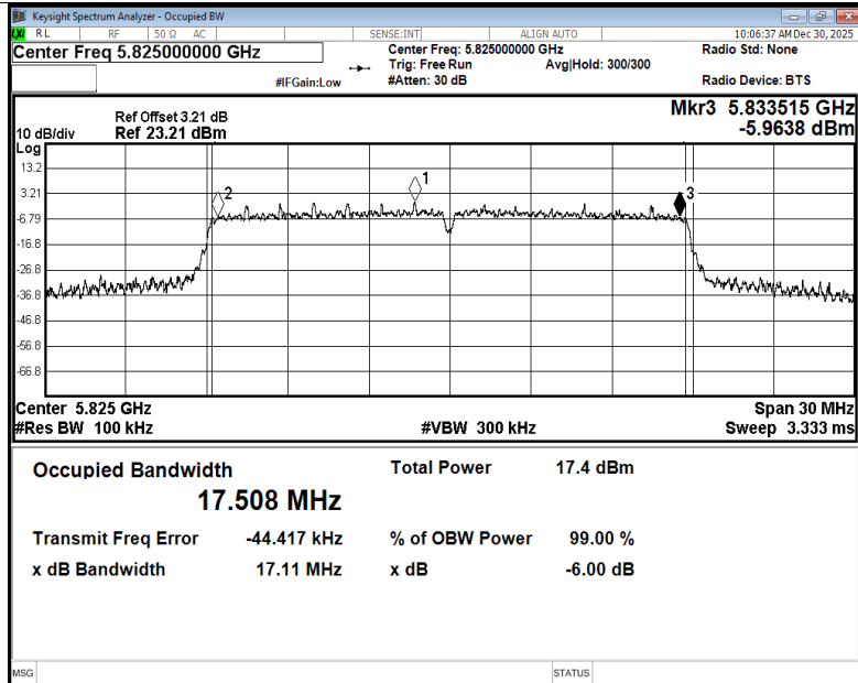
-6dB Bandwidth NVNT n20 5825MHz Ant2
