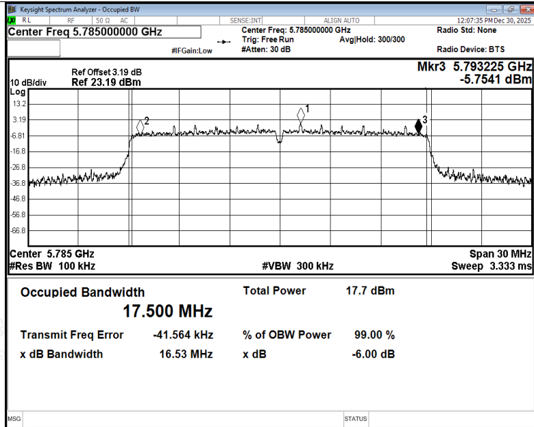
-6dB Bandwidth NVNT n20 5785MHz Ant4
