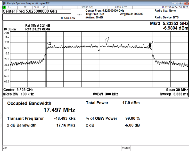
-6dB Bandwidth NVNT ac20 5825MHz Ant2
