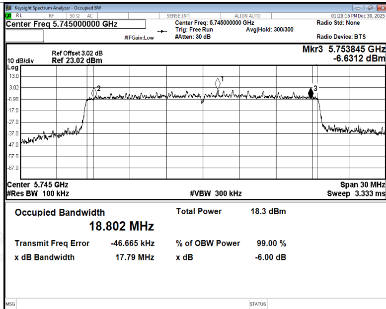
-6dB Bandwidth NVNT be20 5745MHz Ant5
