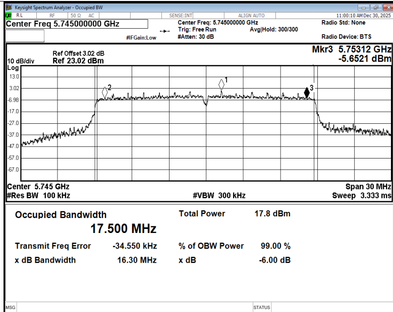
-6dB Bandwidth NVNT n20 5745MHz Ant3
