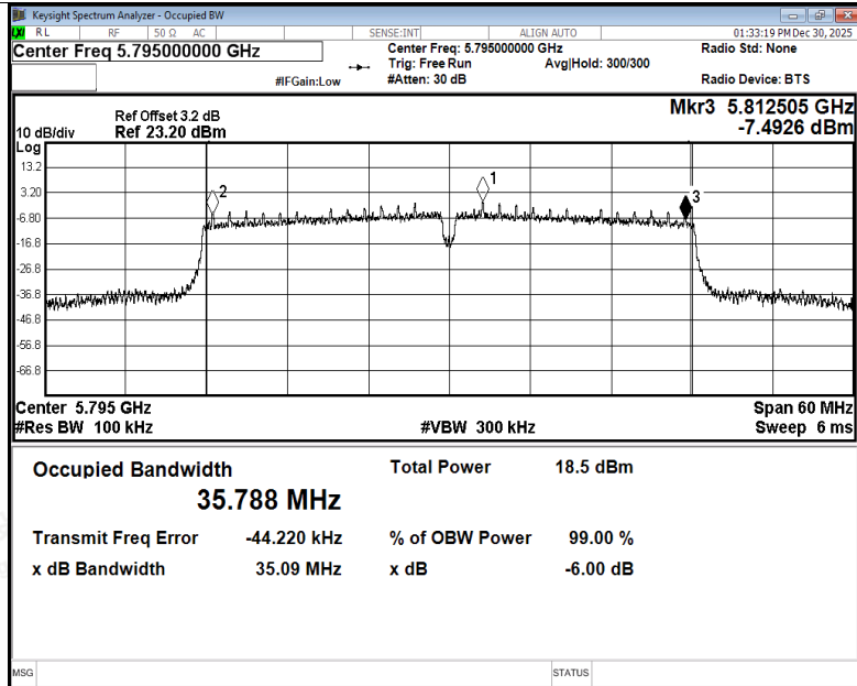
-6dB Bandwidth NVNT ac40 5795MHz Ant5
