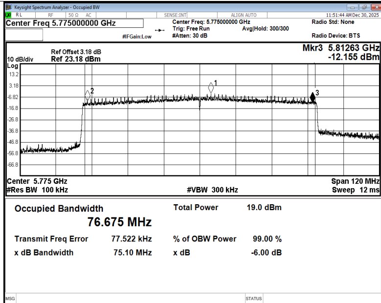
-6dB Bandwidth NVNT ax80 5775MHz Ant3
