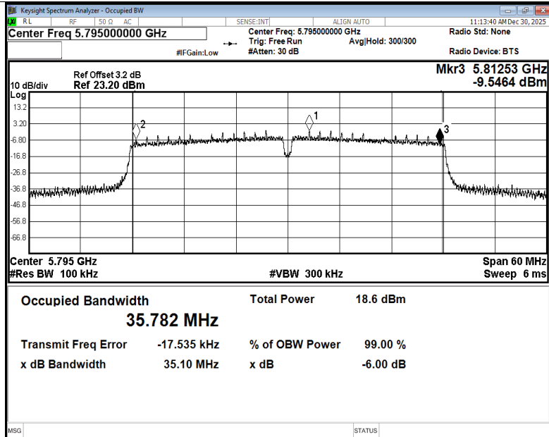
-6dB Bandwidth NVNT n40 5795MHz Ant3
