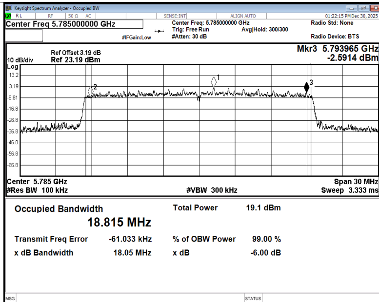
-6dB Bandwidth NVNT be20 5785MHz Ant5
