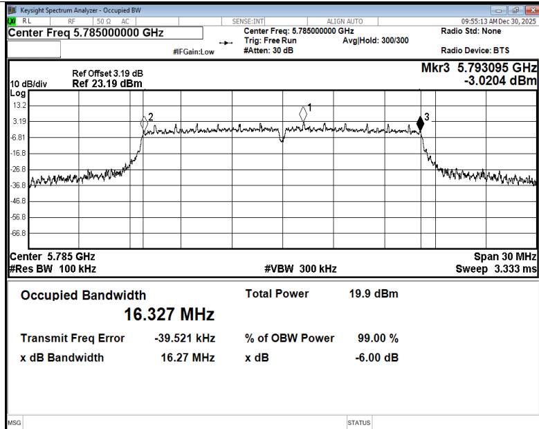
-6dB Bandwidth NVNT a 5785MHz Ant2
