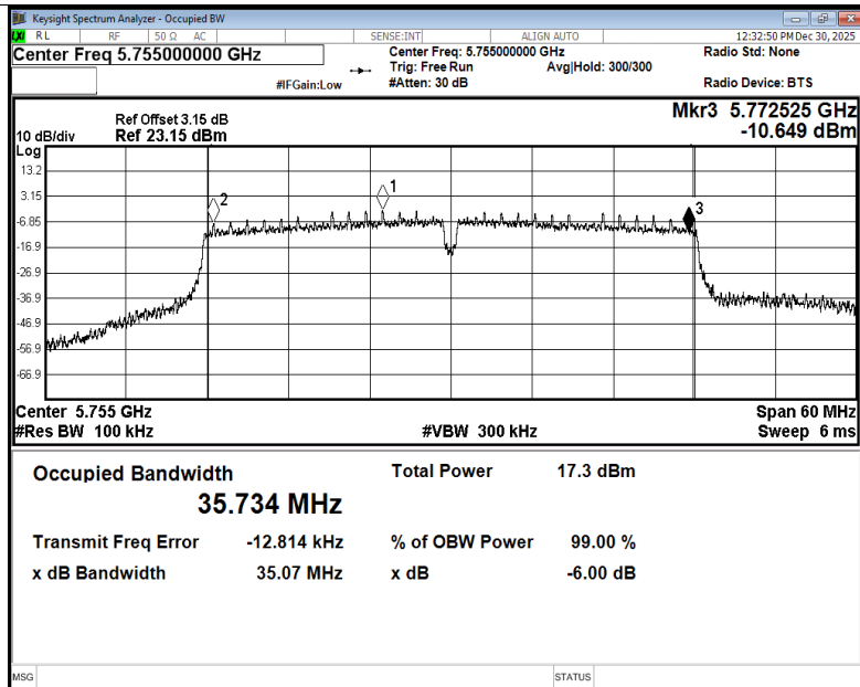
-6dB Bandwidth NVNT ac40 5755MHz Ant4
