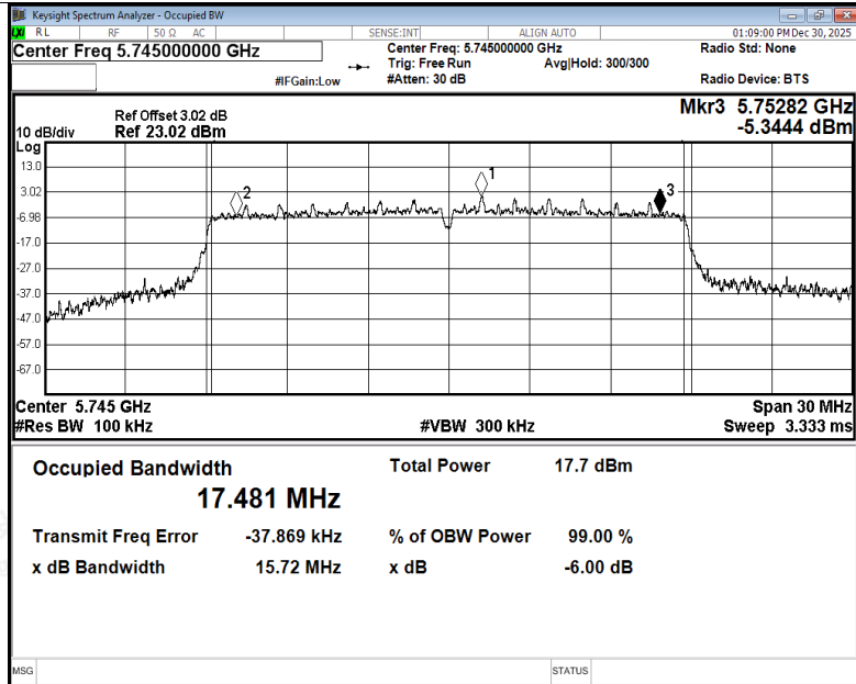
-6dB Bandwidth NVNT ac20 5745MHz Ant5
