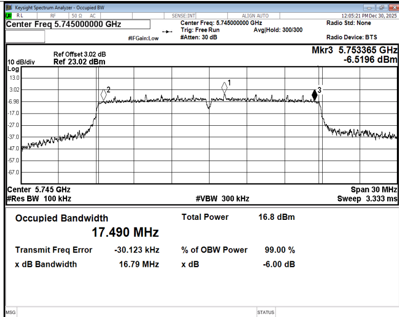
-6dB Bandwidth NVNT n20 5745MHz Ant4
