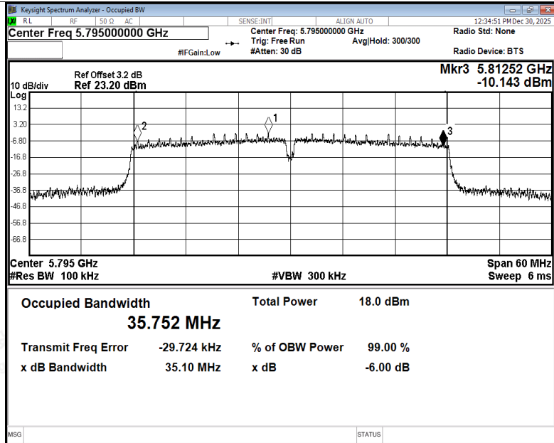
-6dB Bandwidth NVNT ac40 5795MHz Ant4
