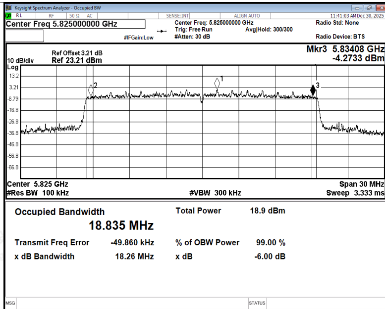
-6dB Bandwidth NVNT ax20 5825MHz Ant3
