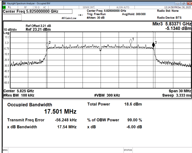
-6dB Bandwidth NVNT ac20 5825MHz Ant4
