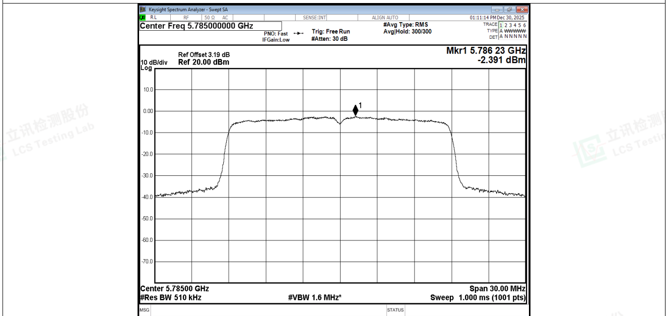
PSD NVNT ac20 5785MHz Ant5
