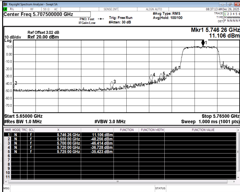
Restrict Band NVNT n20 5745MHz Ant1 Peak
