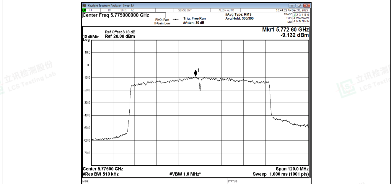
PSD NVNT ac80 5775MHz Ant2
