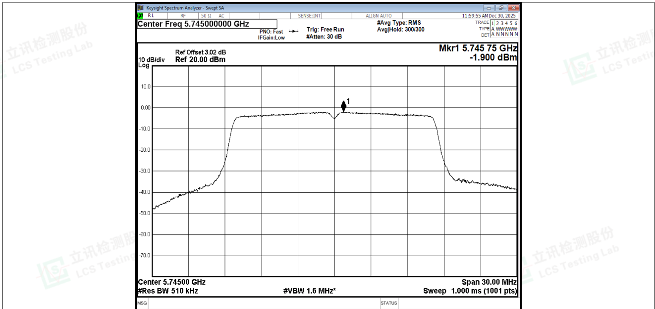
PSD NVNT a 5745MHz Ant4
