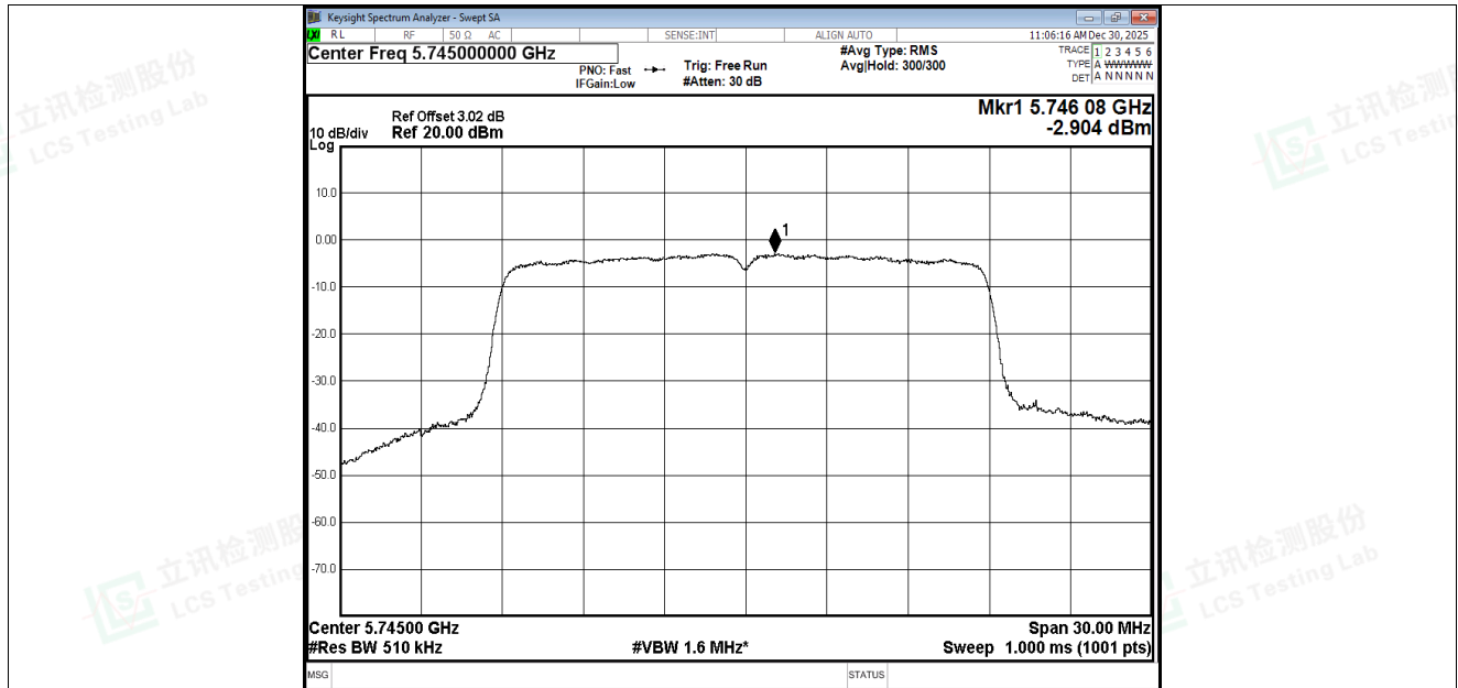
PSD NVNT ac20 5745MHz Ant3
