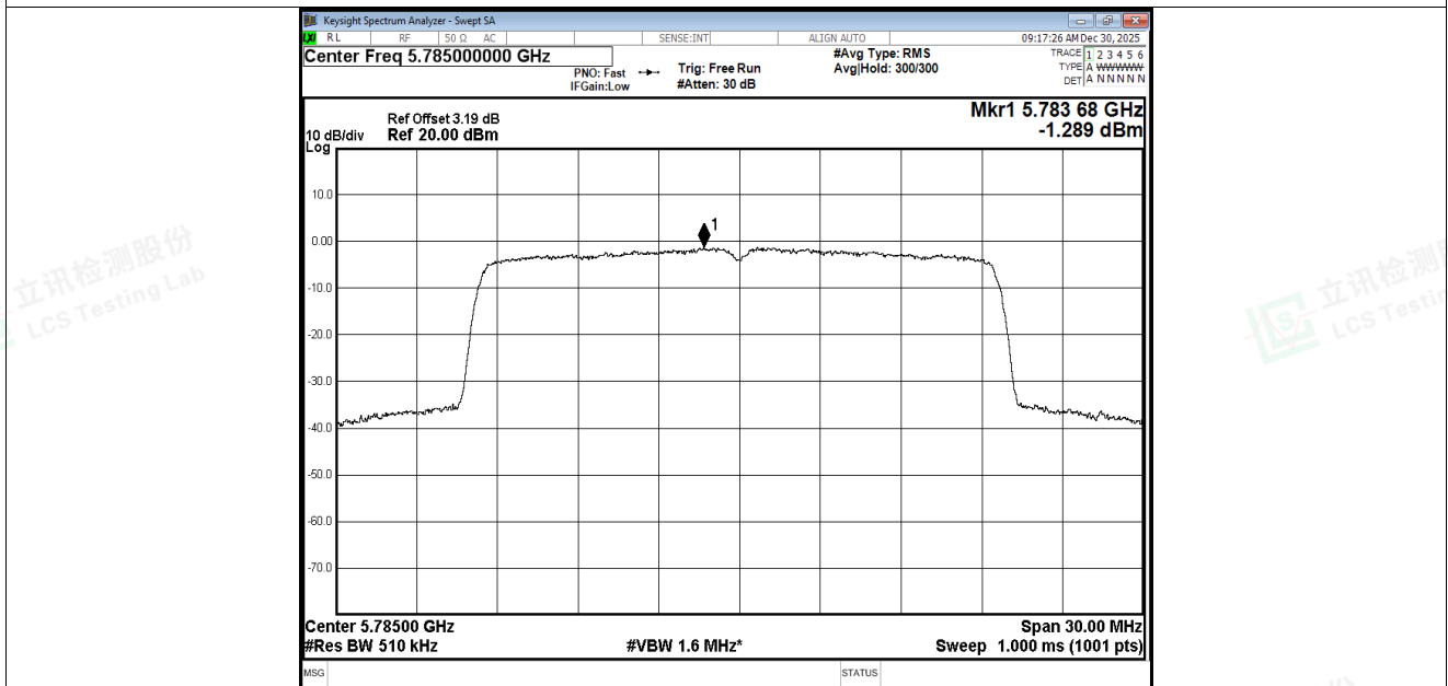
PSD NVNT be20 5785MHz Ant1
