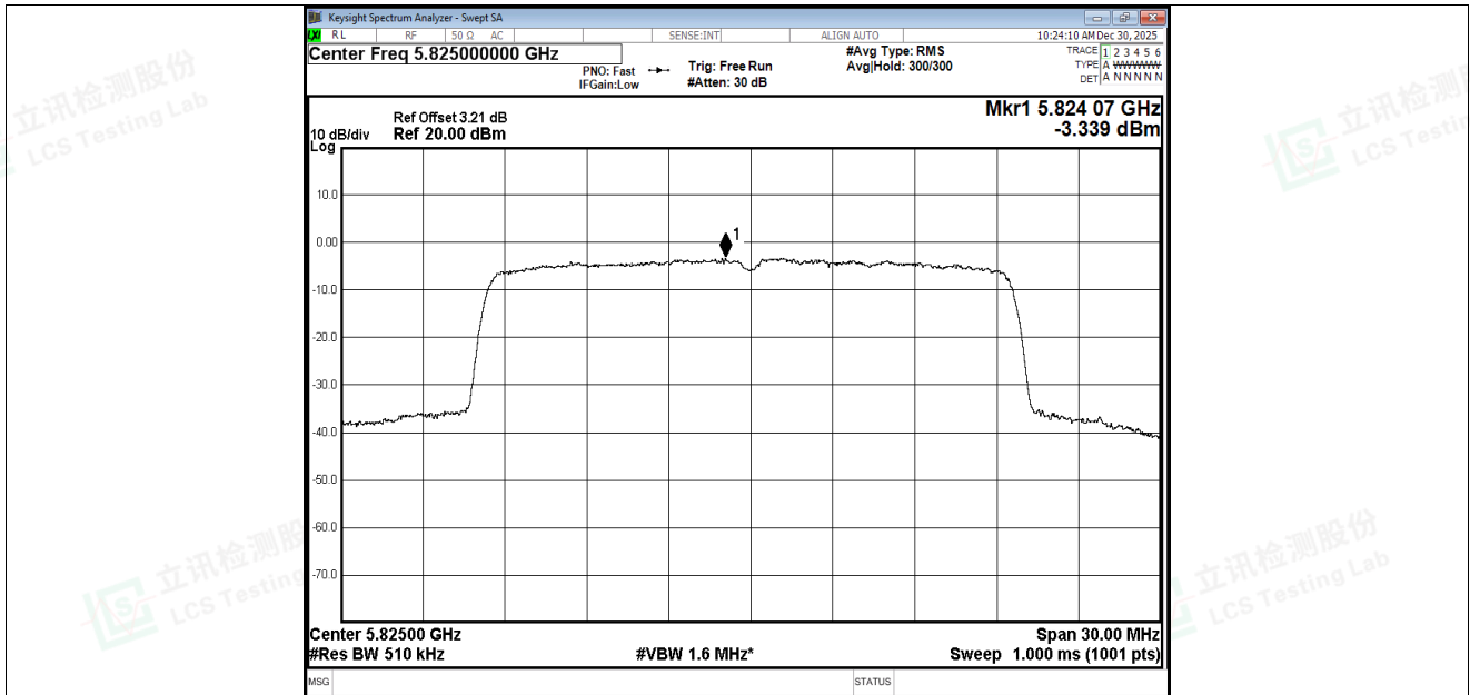
PSD NVNT be20 5825MHz Ant2
