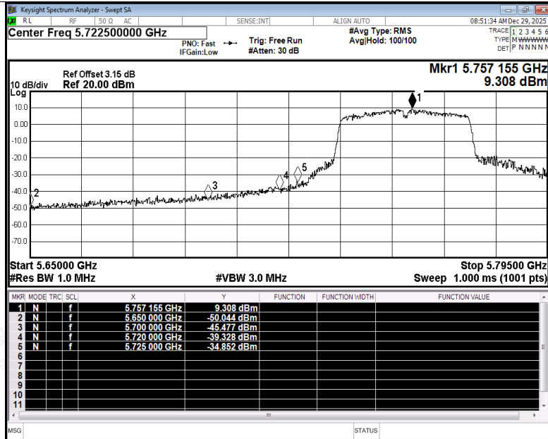
Restrict Band NVNT n40 5755MHz Ant1 Peak
