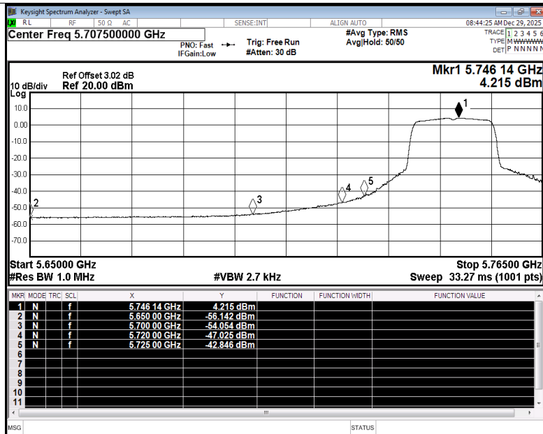
Restrict Band NVNT ac20 5745MHz Ant1 Average
