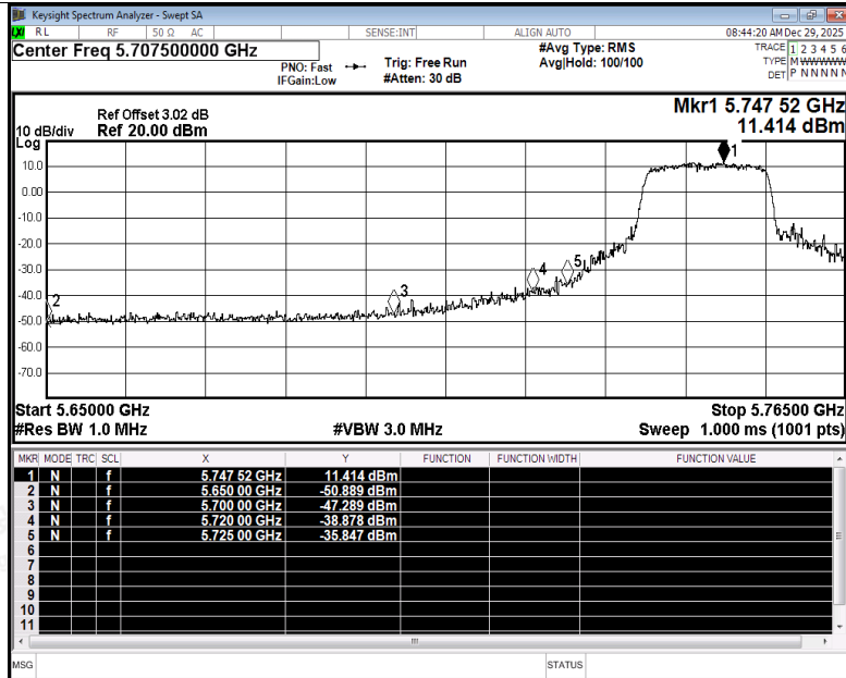
Restrict Band NVNT ac20 5745MHz Ant1 Peak
