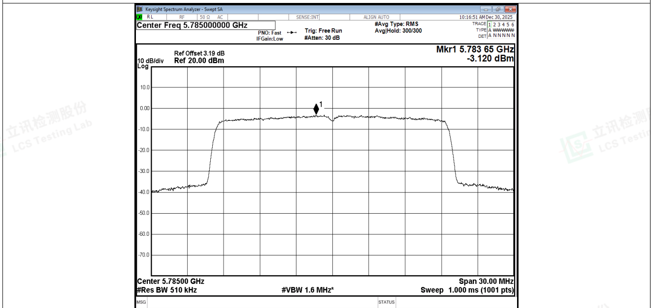
PSD NVNT ax20 5785MHz Ant2
