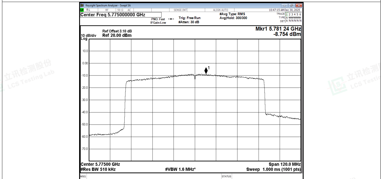
PSD NVNT ax80 5775MHz Ant2
