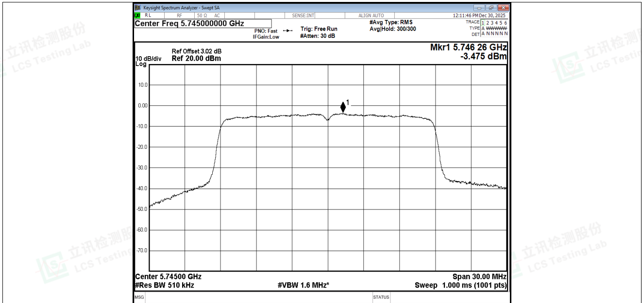
PSD NVNT ac20 5745MHz Ant4
