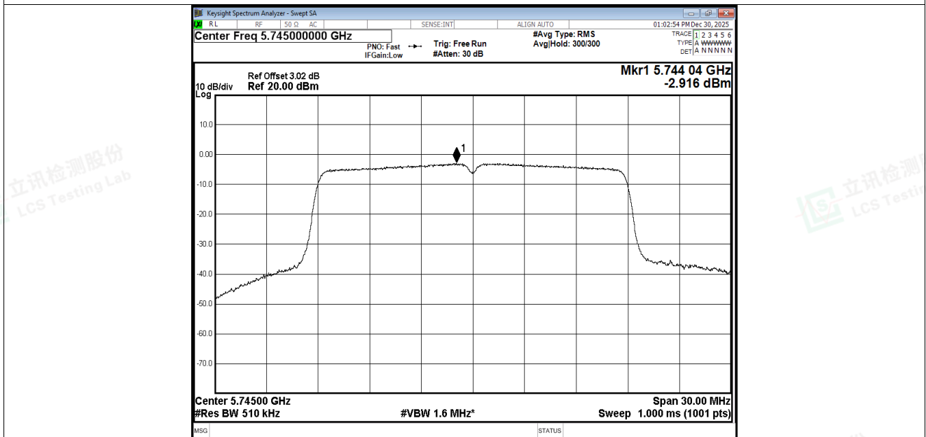
PSD NVNT n20 5745MHz Ant5
