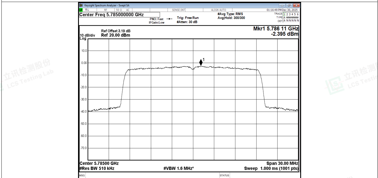
PSD NVNT ax20 5785MHz Ant5
