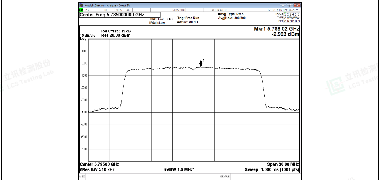
PSD NVNT ax20 5785MHz Ant4
