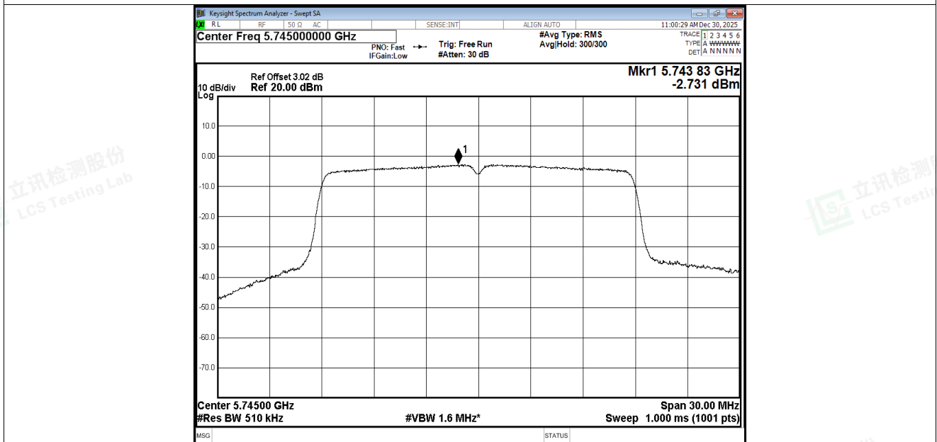
PSD NVNT n20 5745MHz Ant3
