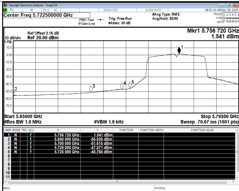
Restrict Band NVNT n40 5755MHz Ant1 Average
