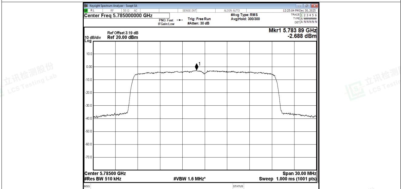
PSD NVNT be20 5785MHz Ant4
