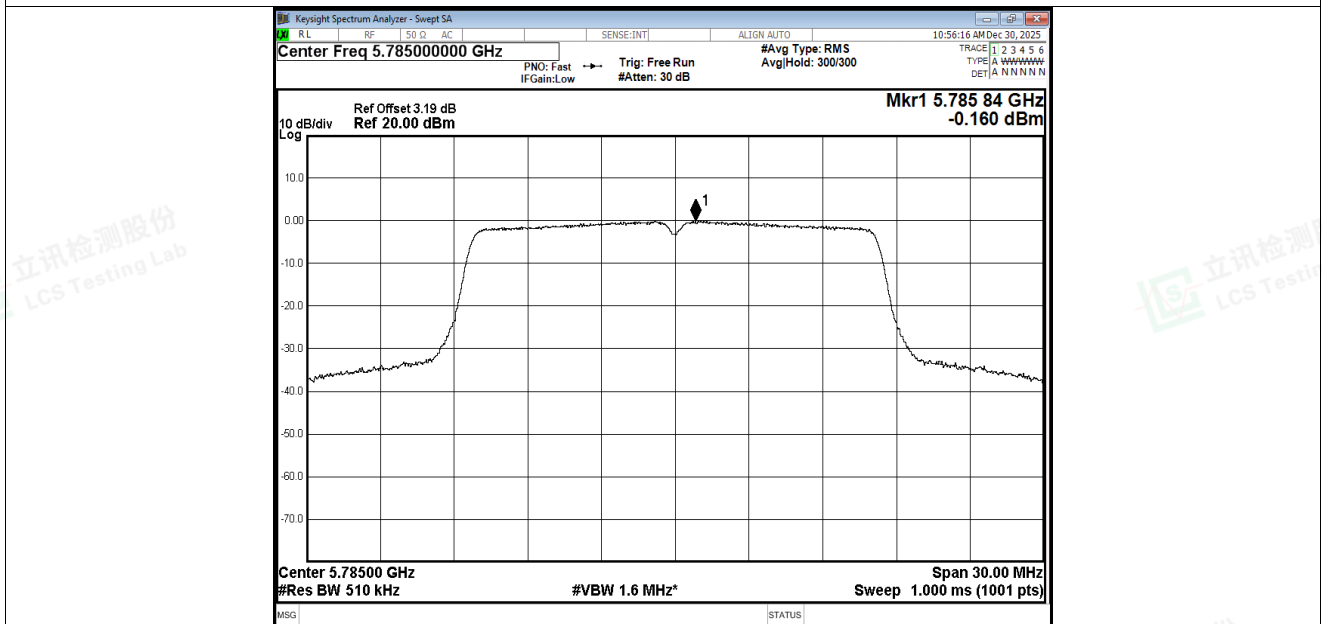
PSD NVNT a 5785MHz Ant3
