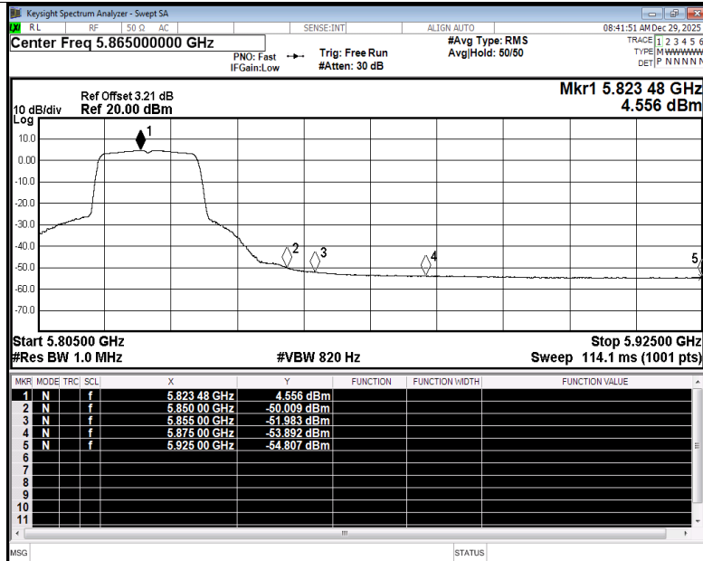
Restrict Band NVNT n20 5825MHz Ant1 Average
