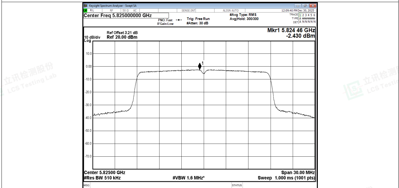
PSD NVNT n20 5825MHz Ant4
