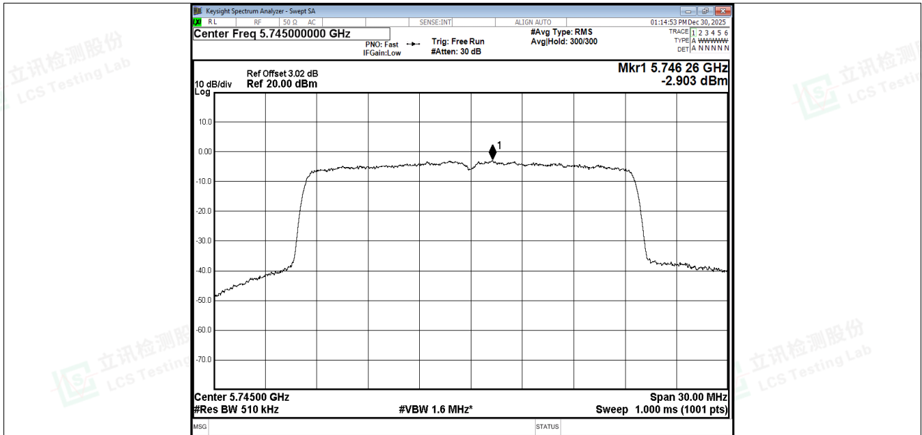
PSD NVNT ax20 5745MHz Ant5
