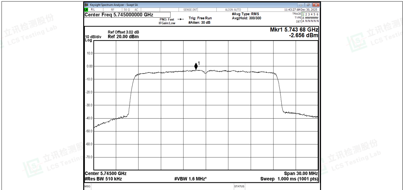
PSD NVNT be20 5745MHz Ant3
