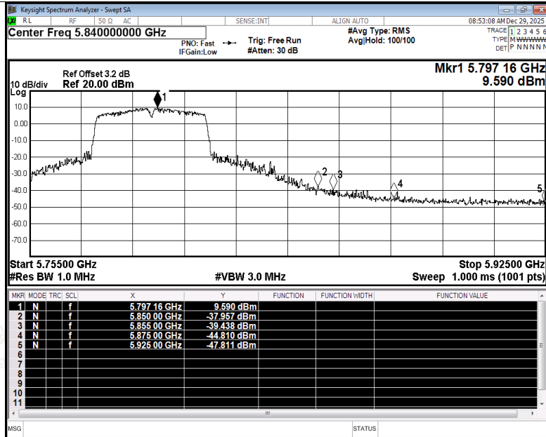
Restrict Band NVNT n40 5795MHz Ant1 Peak
