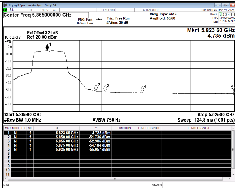
Restrict Band NVNT a 5825MHz Ant1 Average
