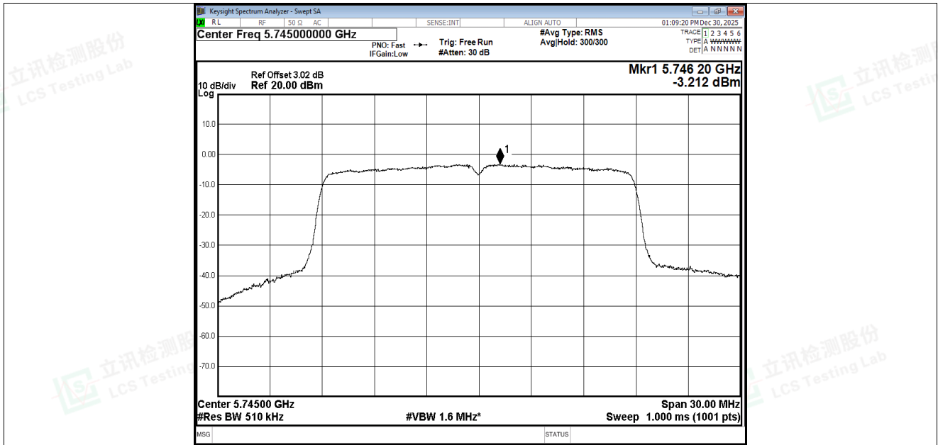
PSD NVNT ac20 5745MHz Ant5
