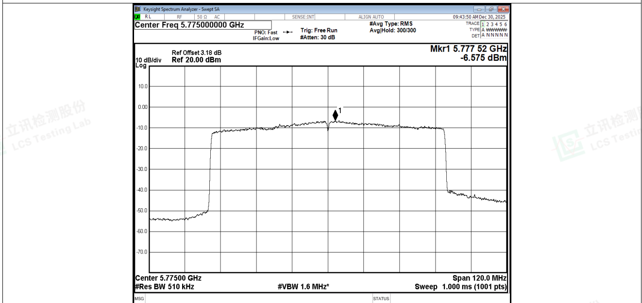
PSD NVNT be80 5775MHz Ant1
