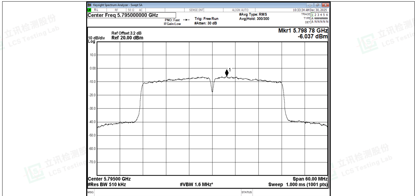
PSD NVNT ac40 5795MHz Ant2
