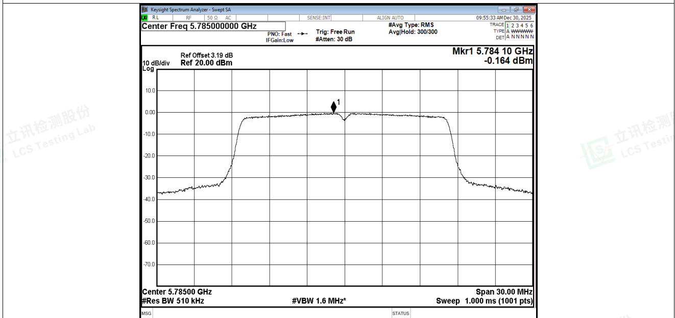
PSD NVNT a 5785MHz Ant2
