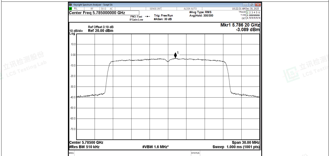
PSD NVNT be20 5785MHz Ant2
