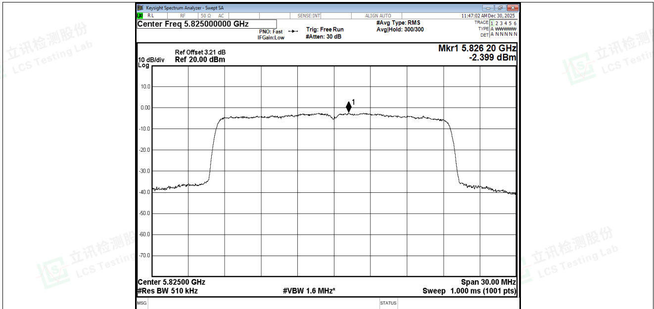
PSD NVNT be20 5825MHz Ant3
