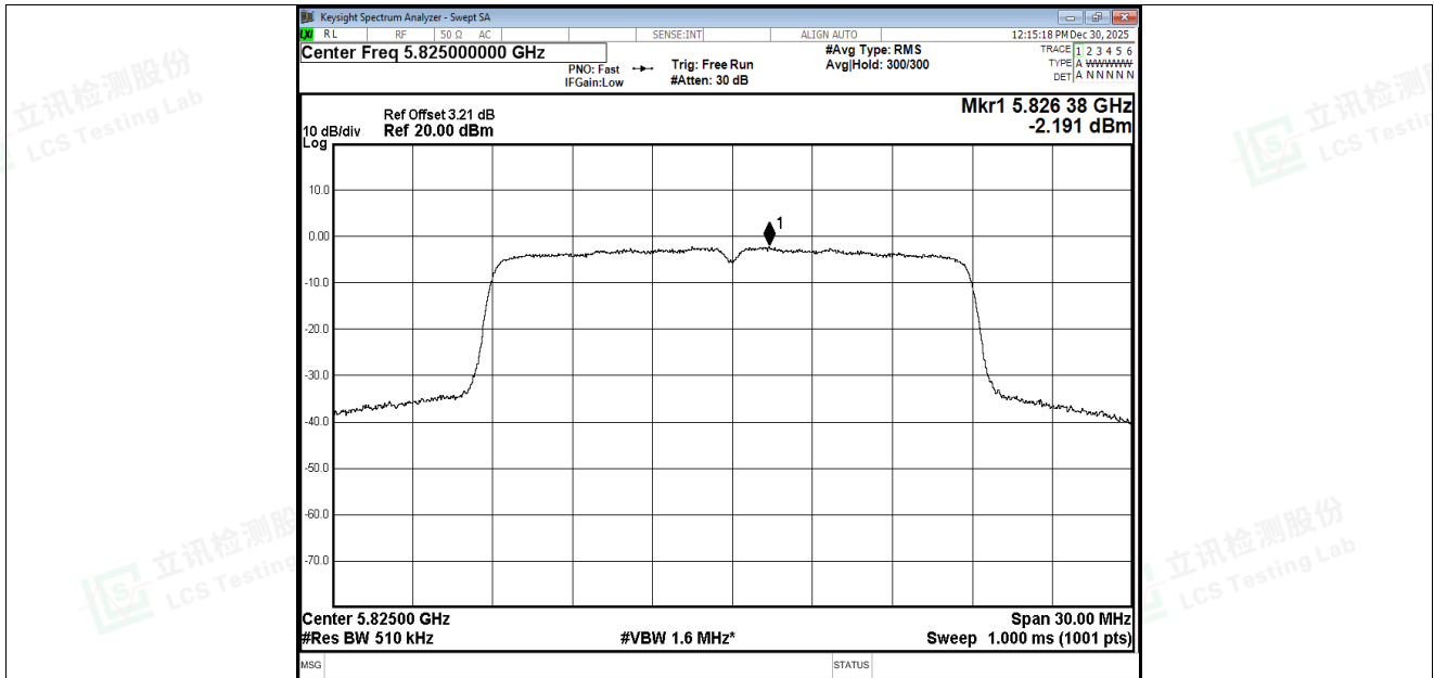
PSD NVNT ac20 5825MHz Ant4
