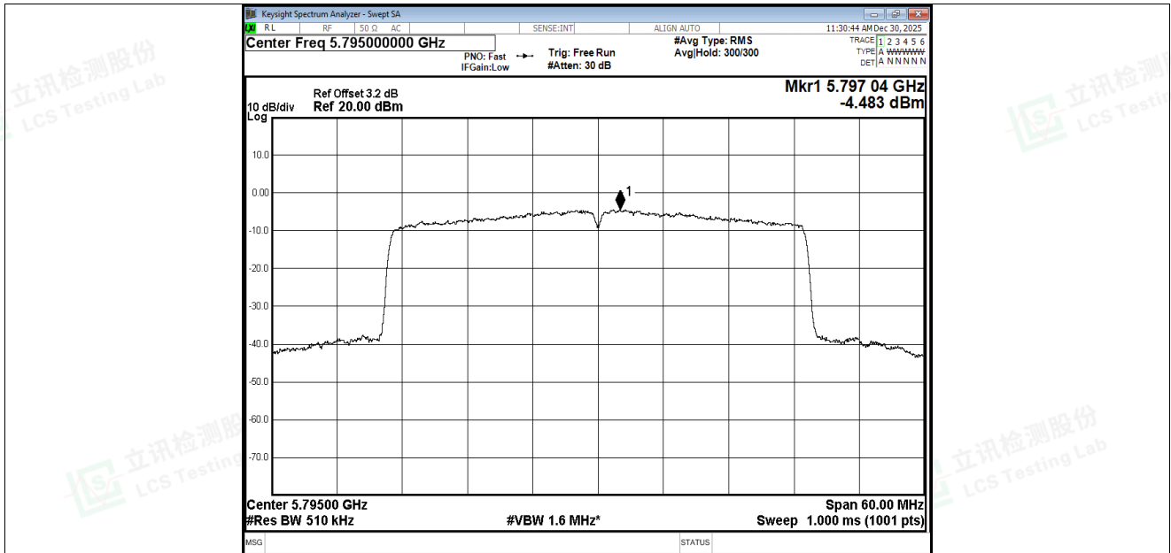
PSD NVNT ax40 5795MHz Ant3
