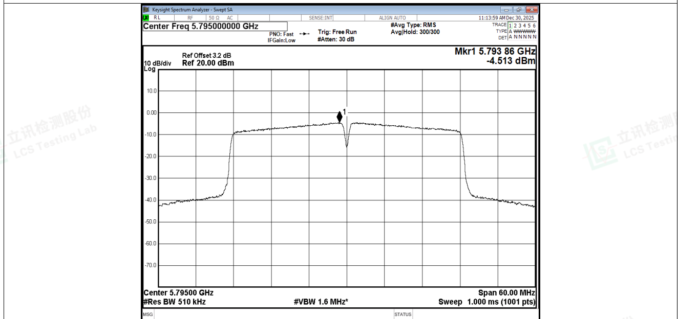
PSD NVNT n40 5795MHz Ant3
