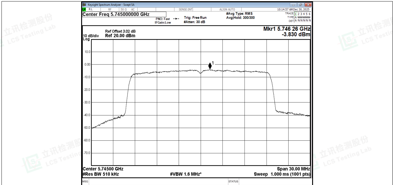
PSD NVNT ax20 5745MHz Ant2
