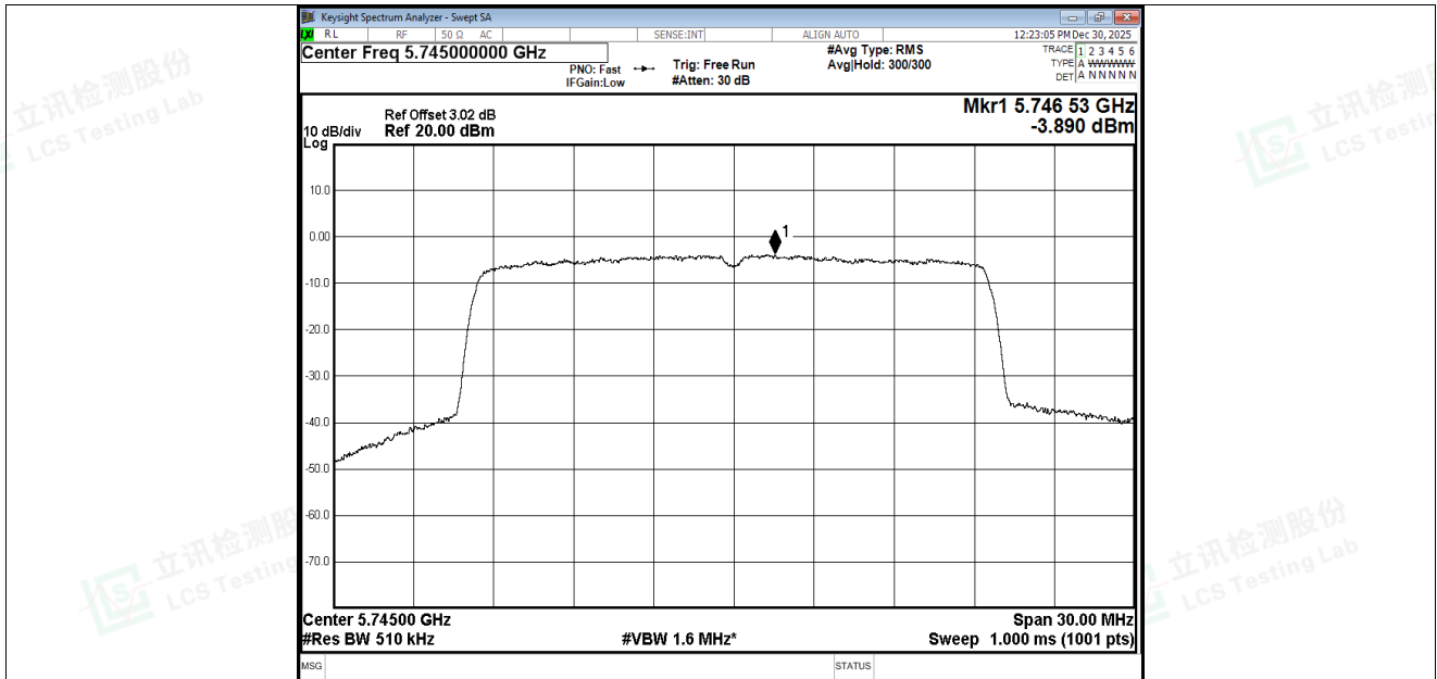
PSD NVNT be20 5745MHz Ant4
