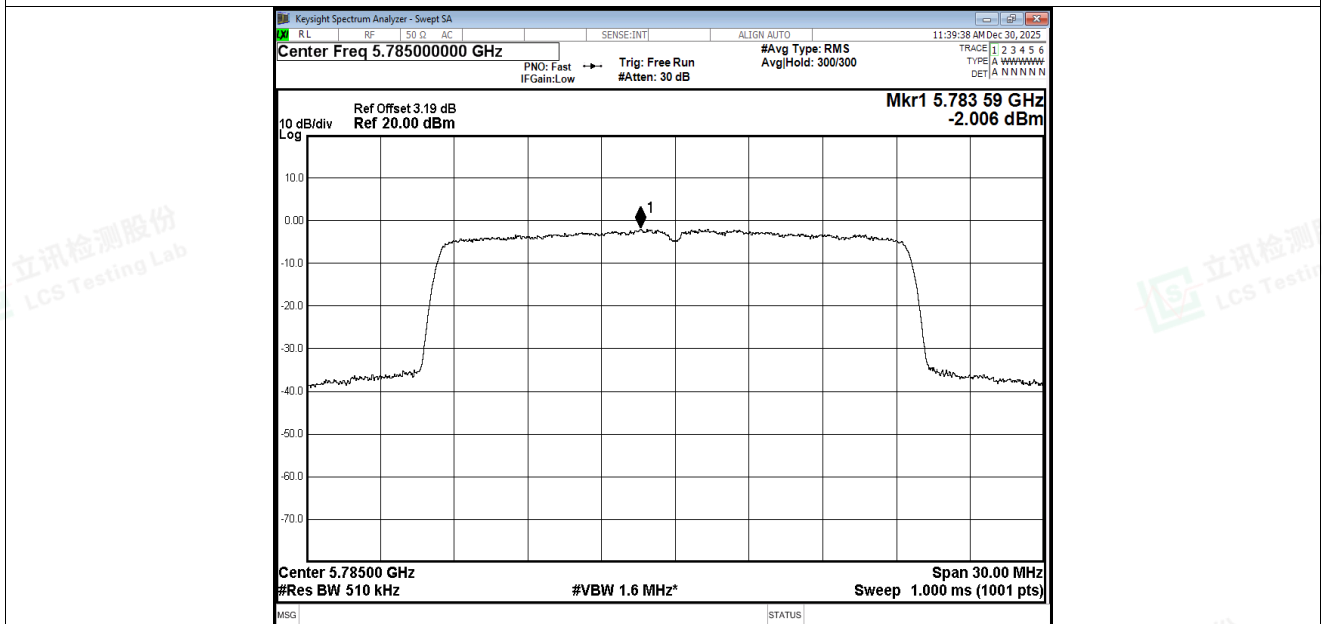
PSD NVNT ax20 5785MHz Ant3
