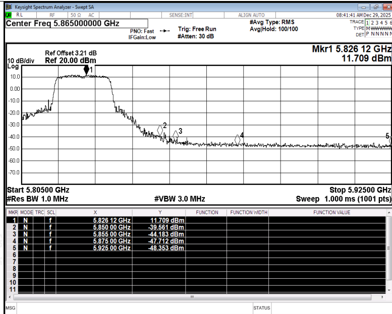
Restrict Band NVNT n20 5825MHz Ant1 Peak
