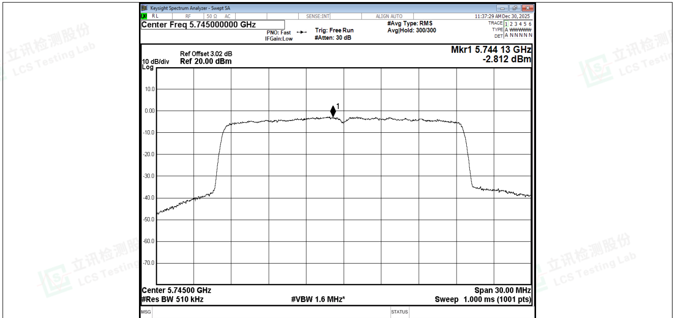
PSD NVNT ax20 5745MHz Ant3
