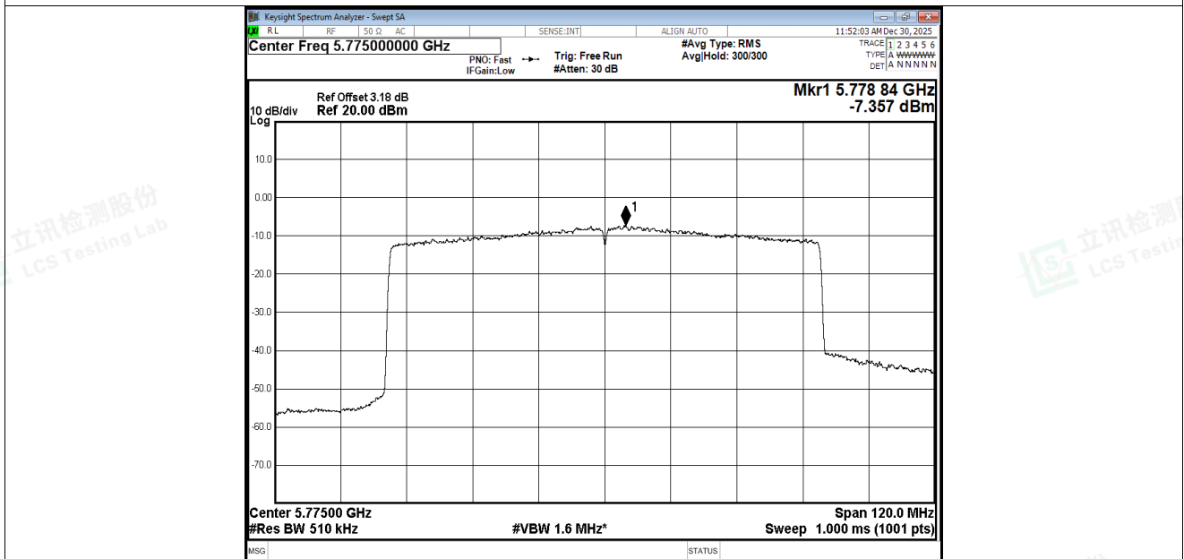
PSD NVNT ax80 5775MHz Ant3
