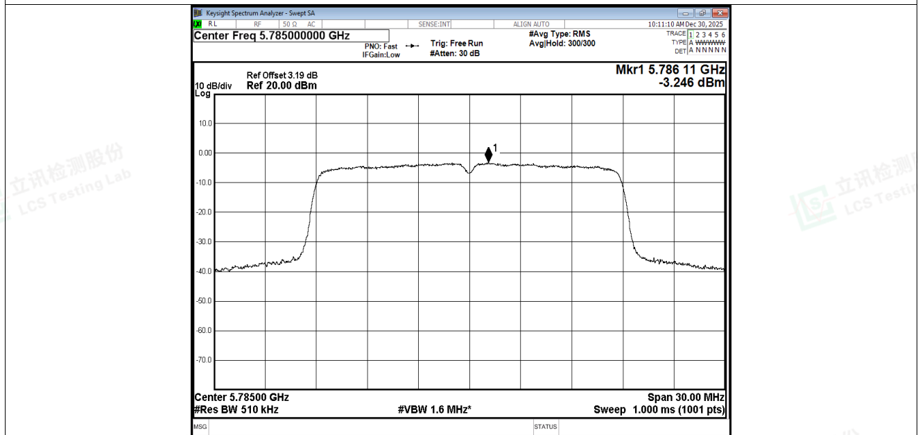
PSD NVNT ac20 5785MHz Ant2
