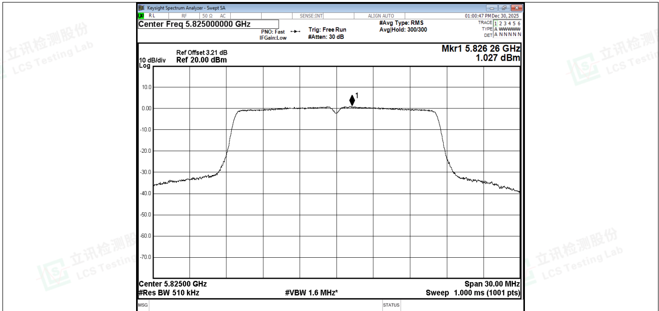
PSD NVNT a 5825MHz Ant5
