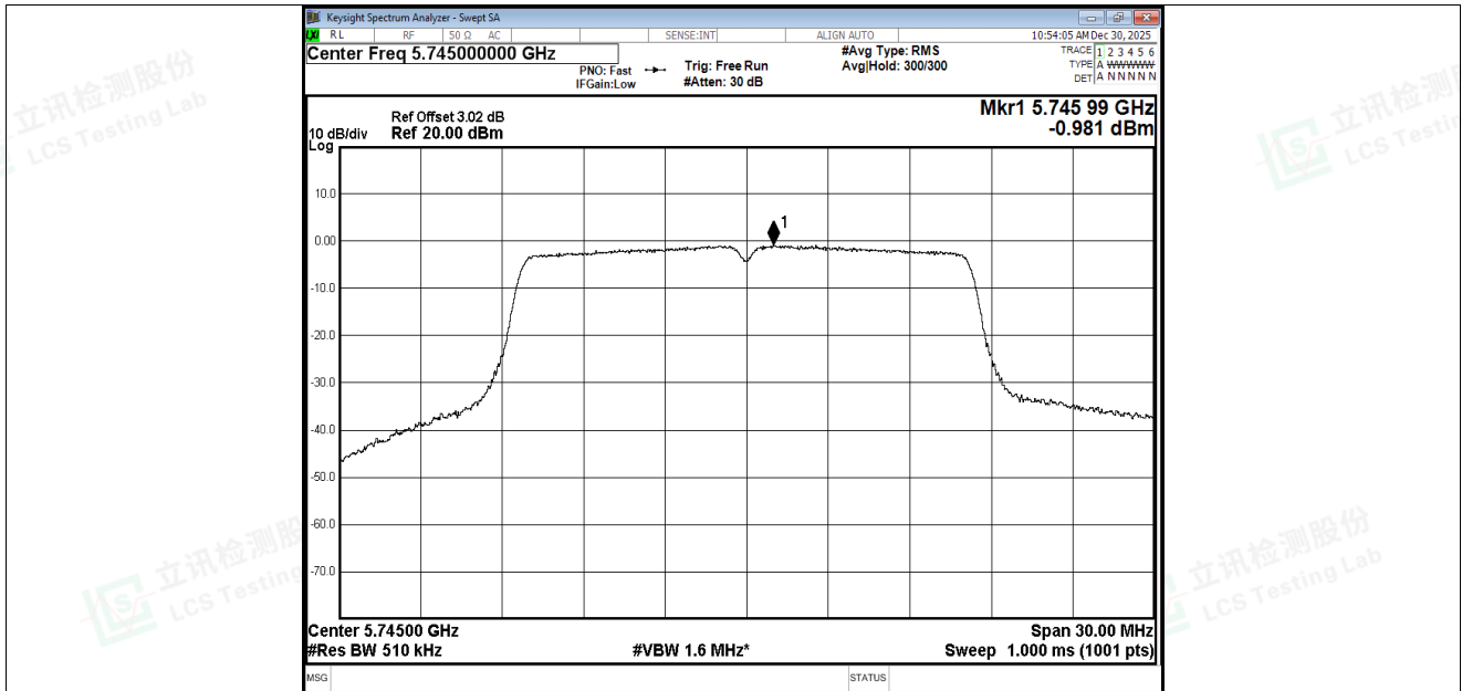
PSD NVNT a 5745MHz Ant3
