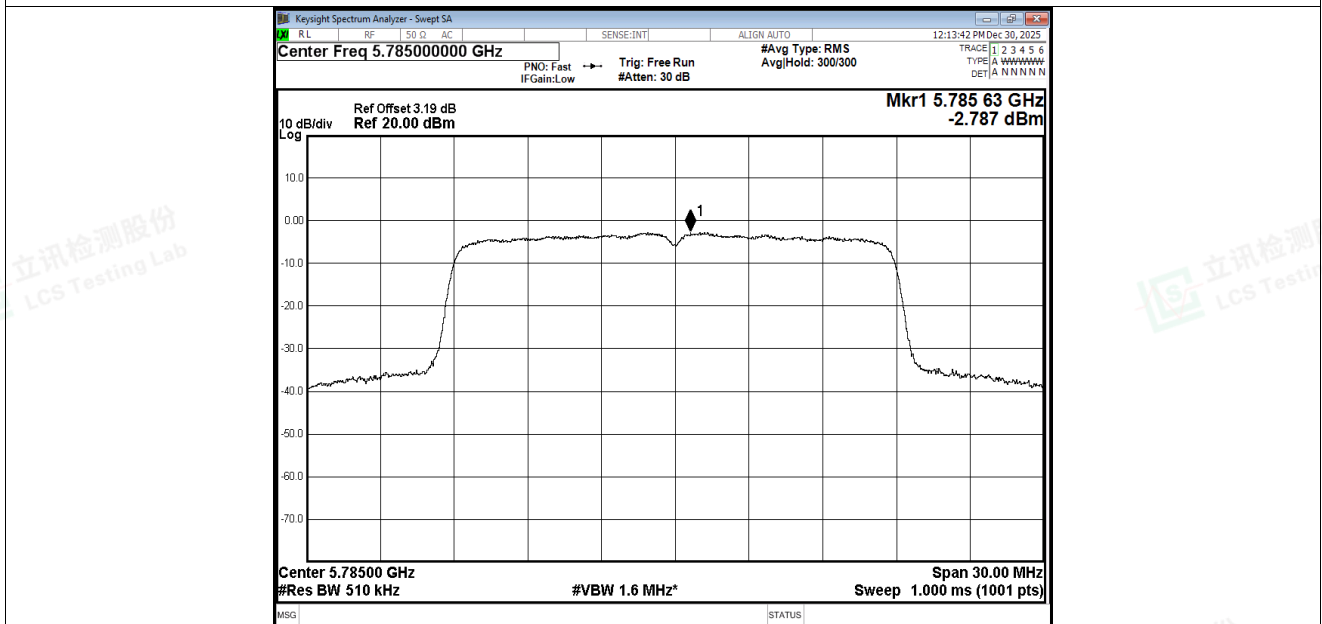
PSD NVNT ac20 5785MHz Ant4
