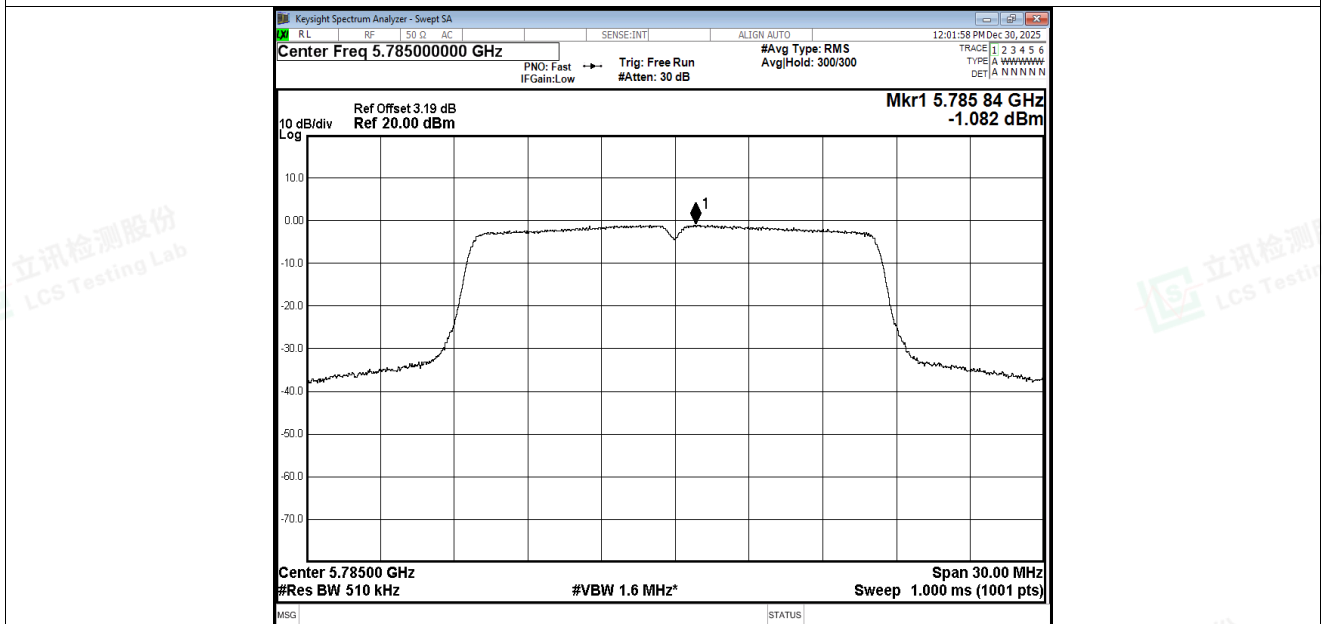
PSD NVNT a 5785MHz Ant4
