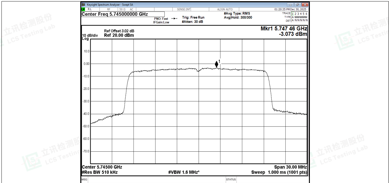
PSD NVNT be20 5745MHz Ant5
