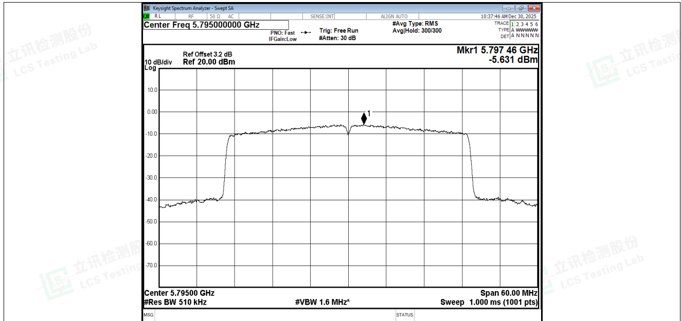
PSD NVNT ax40 5795MHz Ant2
