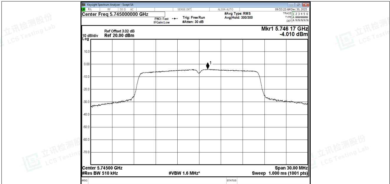
PSD NVNT a 5745MHz Ant2
