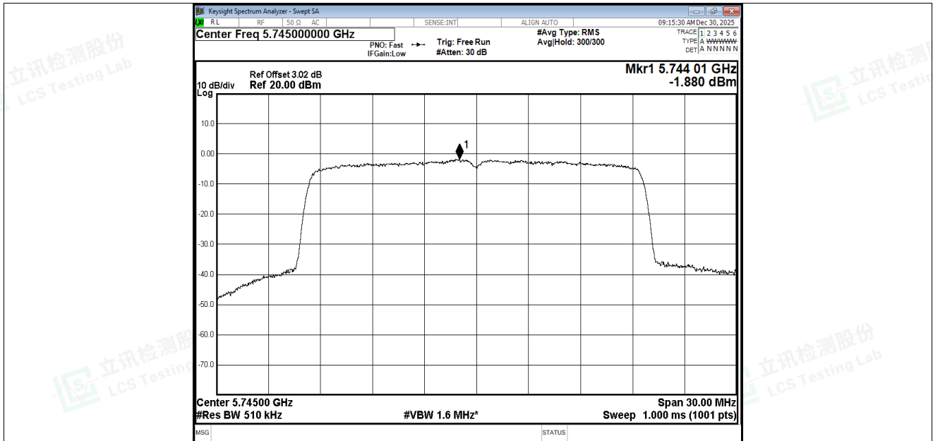
PSD NVNT be20 5745MHz Ant1
