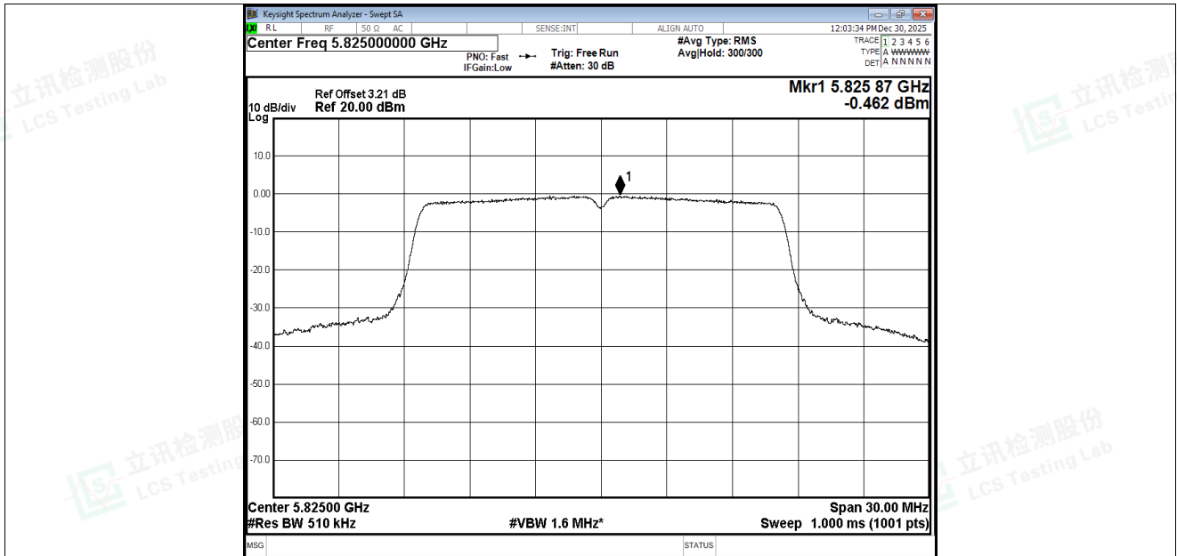
PSD NVNT a 5825MHz Ant4
