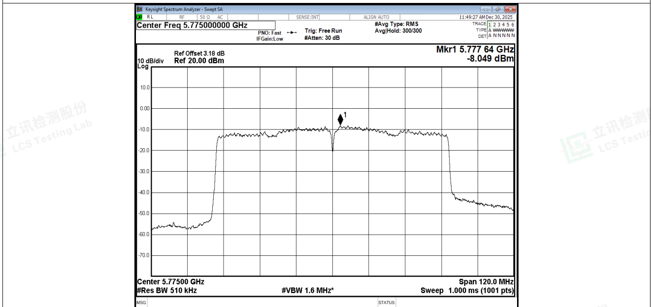
PSD NVNT ac80 5775MHz Ant3
