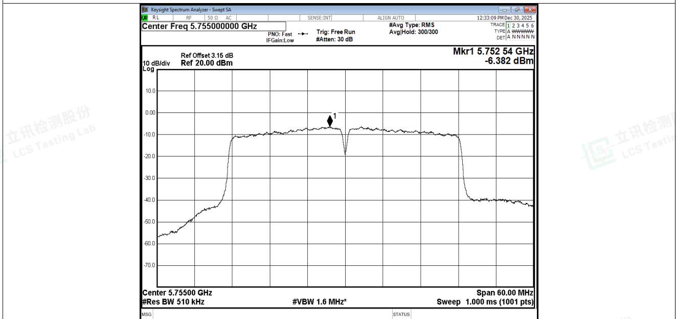
PSD NVNT ac40 5755MHz Ant4
