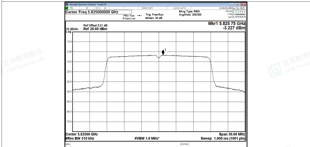
PSD NVNT n20 5825MHz Ant2
