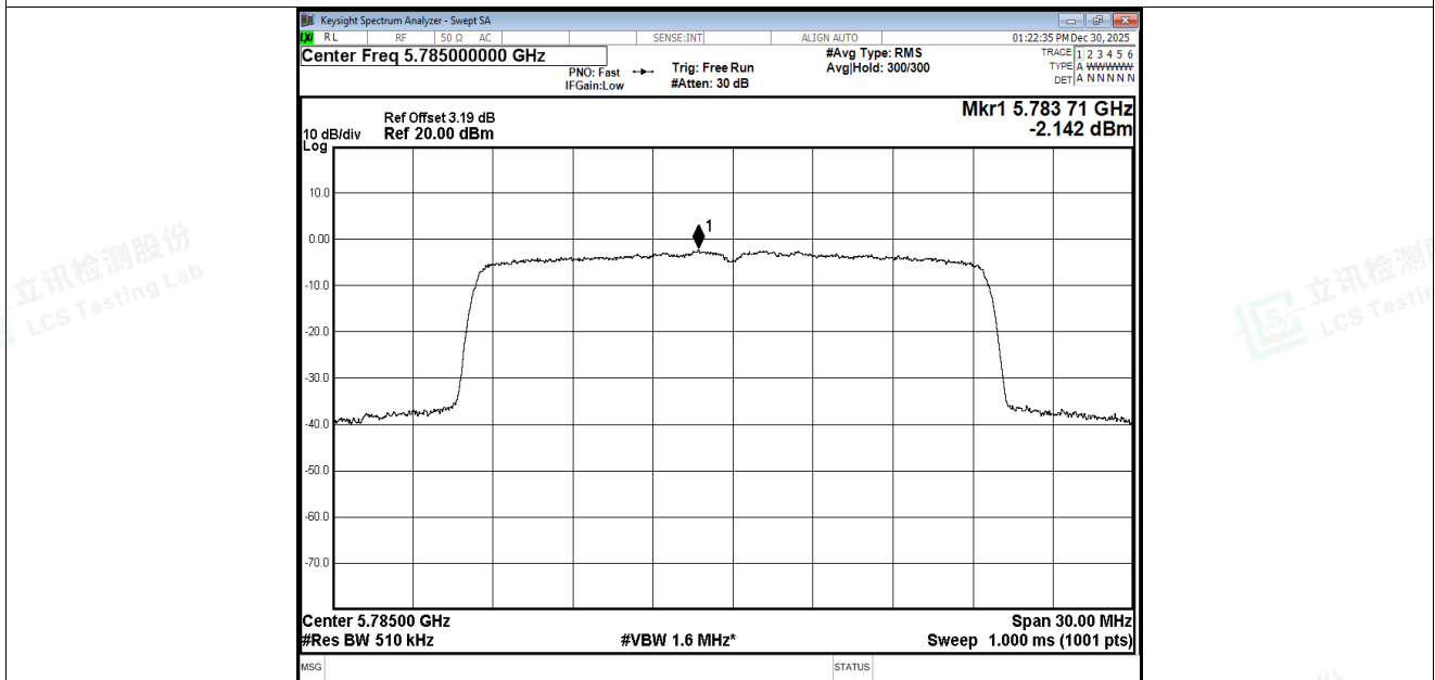
PSD NVNT be20 5785MHz Ant5
