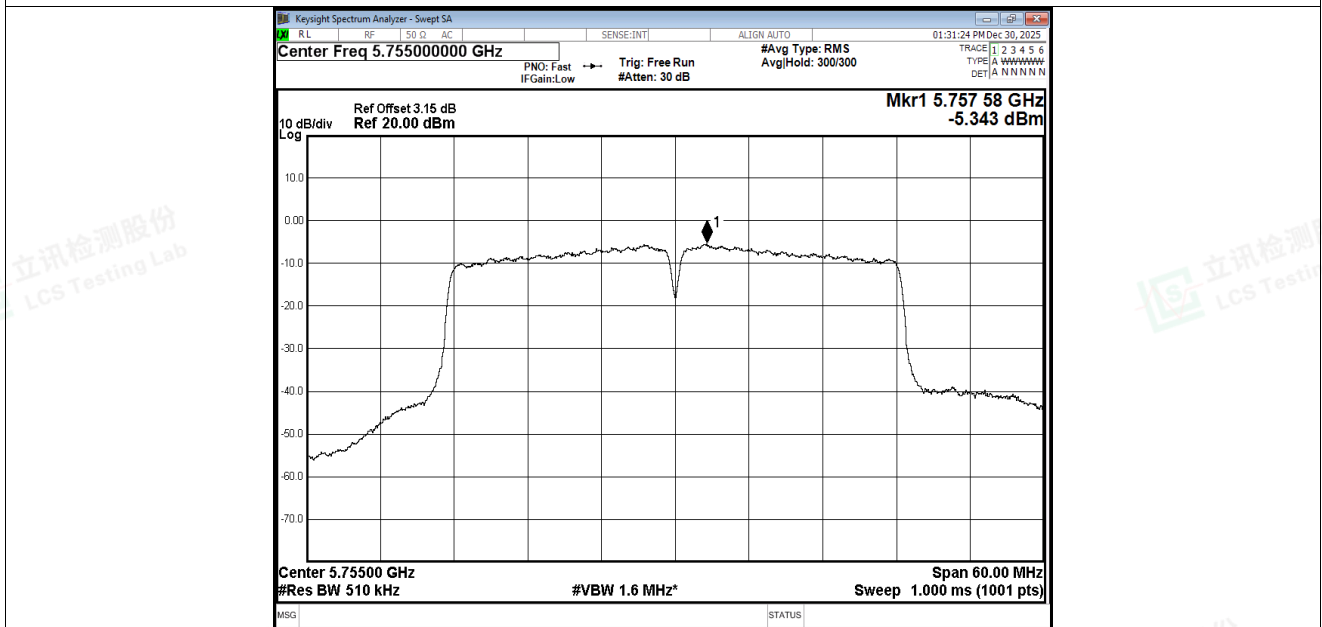
PSD NVNT ac40 5755MHz Ant5
