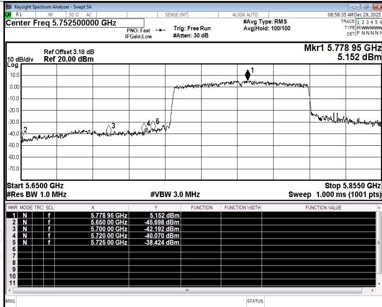
Restrict Band NVNT ac80 5775MHz Ant1 Peak
