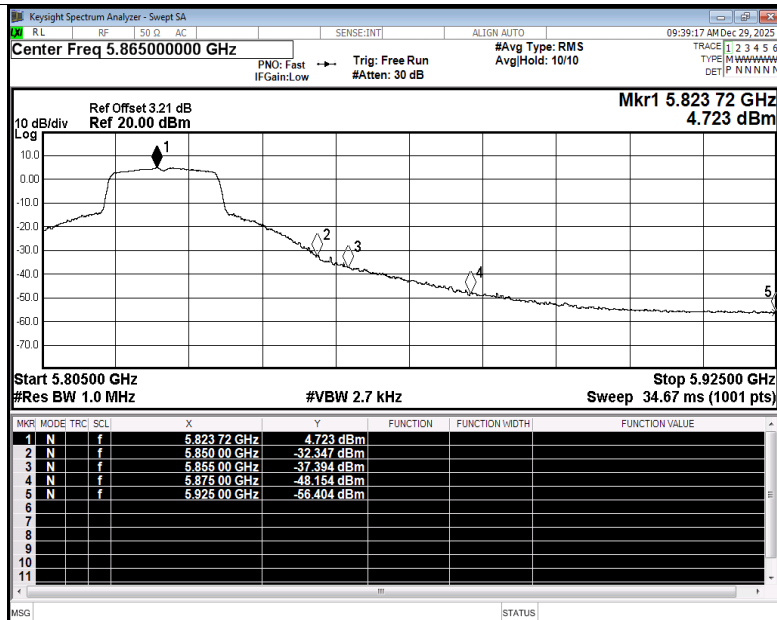
Restrict Band NVNT ac20 5825MHz Ant3 Average
