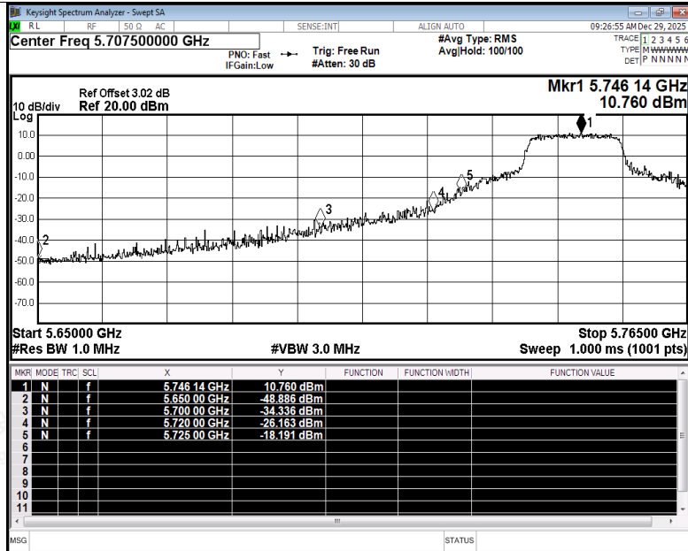
Restrict Band NVNT a 5745MHz Ant3 Peak
