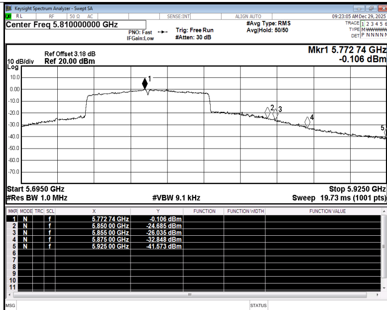
Restrict Band NVNT ac80 5775MHz Ant2 Average
