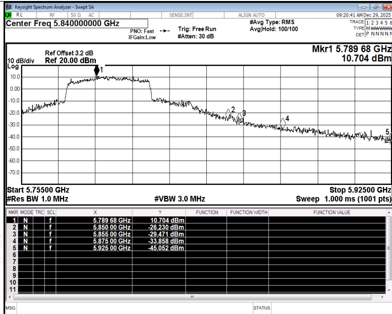
Restrict Band NVNT ax40 5795MHz Ant2 Peak
