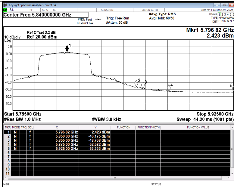
Restrict Band NVNT be40 5795MHz Ant1 Average
