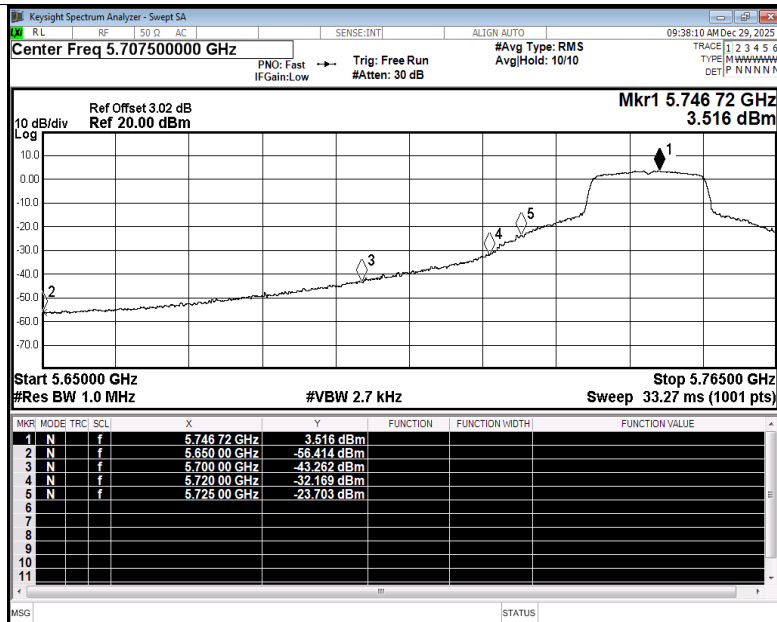
Restrict Band NVNT ac20 5745MHz Ant3 Average
