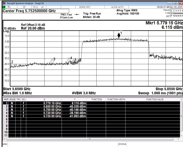
Restrict Band NVNT be80 5775MHz Ant1 Peak
