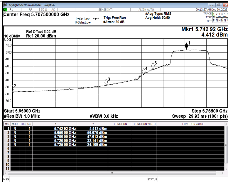
Restrict Band NVNT be20 5745MHz Ant2 Average
