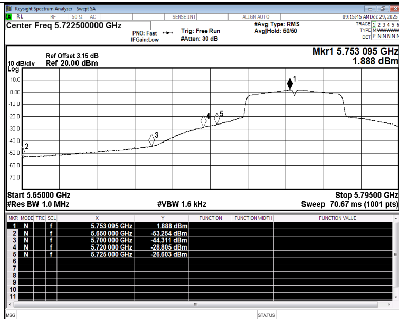
Restrict Band NVNT n40 5755MHz Ant2 Average
