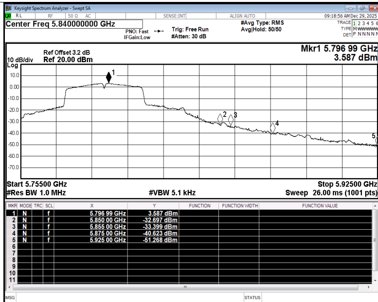
Restrict Band NVNT ac40 5795MHz Ant2 Average
