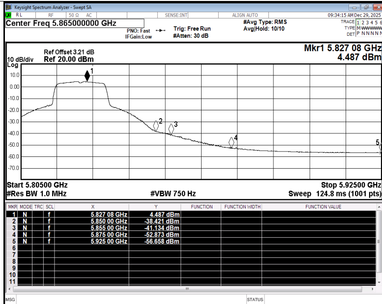
Restrict Band NVNT a 5825MHz Ant3 Average
