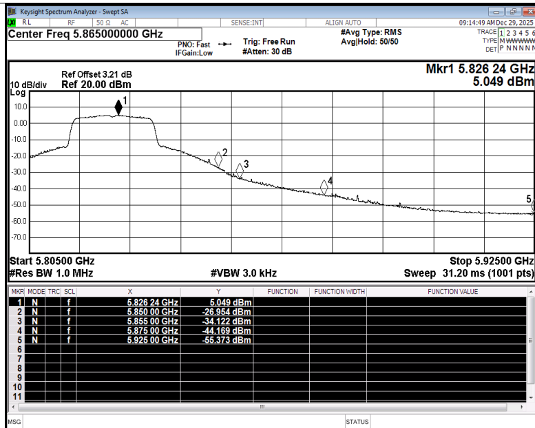
Restrict Band NVNT be20 5825MHz Ant2 Average
