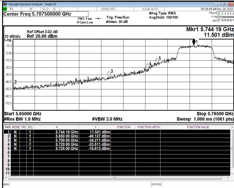
Restrict Band NVNT ac20 5745MHz Ant3 Peak
