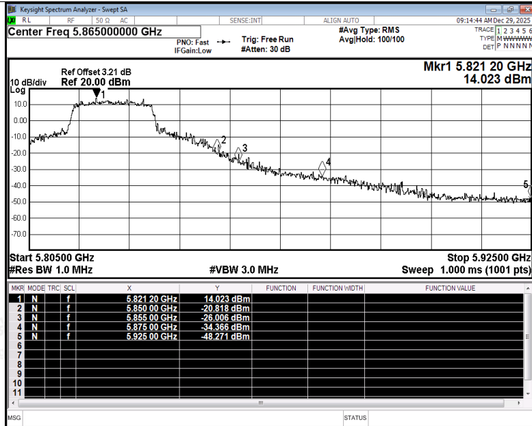
Restrict Band NVNT be20 5825MHz Ant2 Peak
