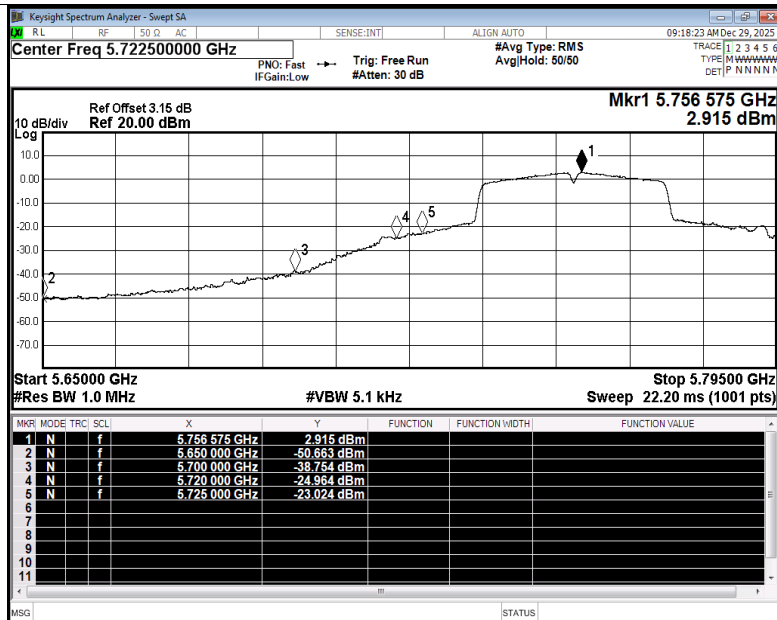
Restrict Band NVNT ac40 5755MHz Ant2 Average
