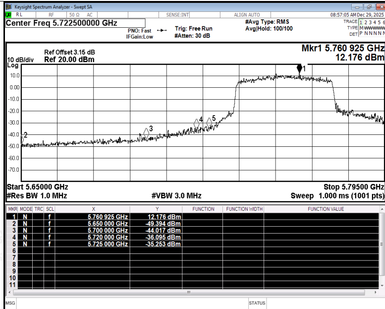
Restrict Band NVNT be40 5755MHz Ant1 Peak
