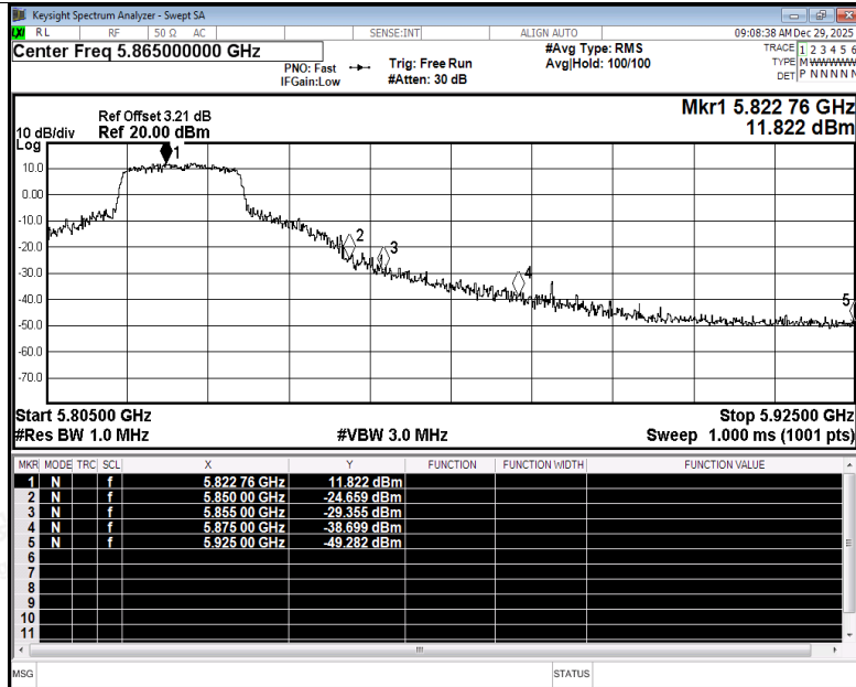
Restrict Band NVNT a 5825MHz Ant2 Peak
