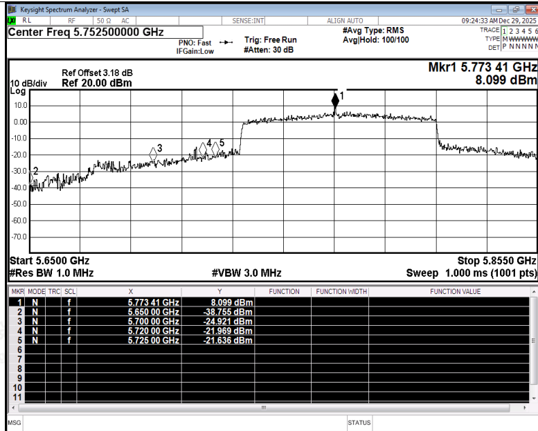
Restrict Band NVNT be80 5775MHz Ant2 Peak
