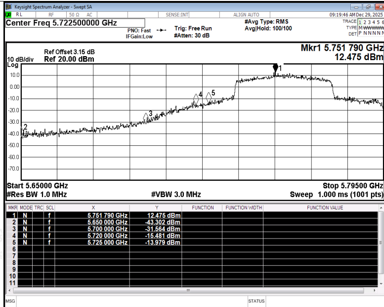
Restrict Band NVNT ax40 5755MHz Ant2 Peak
