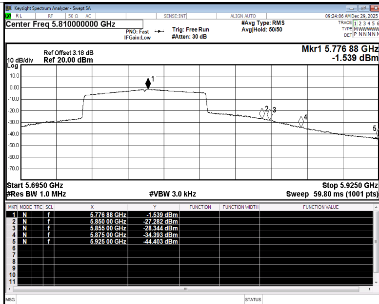
Restrict Band NVNT ax80 5775MHz Ant2 Average
