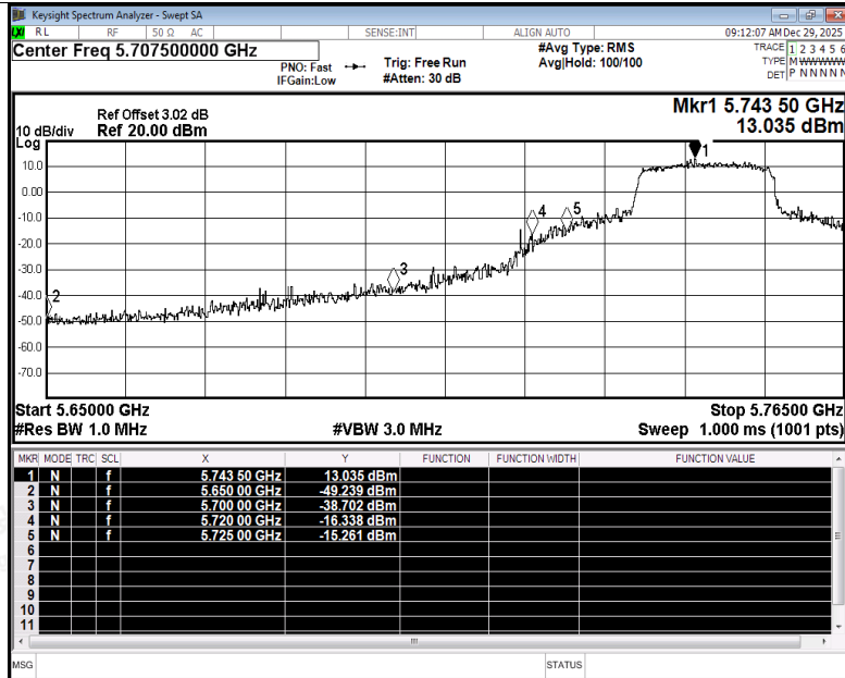
Restrict Band NVNT ax20 5745MHz Ant2 Peak
