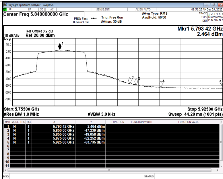
Restrict Band NVNT ax40 5795MHz Ant1 Average
