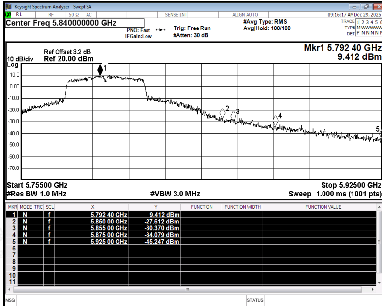
Restrict Band NVNT n40 5795MHz Ant2 Peak
