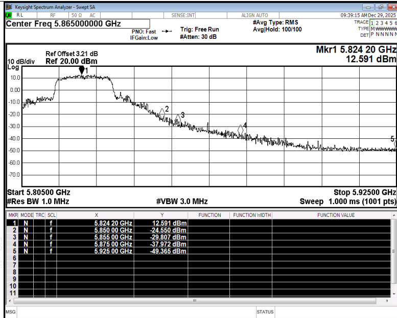
Restrict Band NVNT ac20 5825MHz Ant3 Peak
