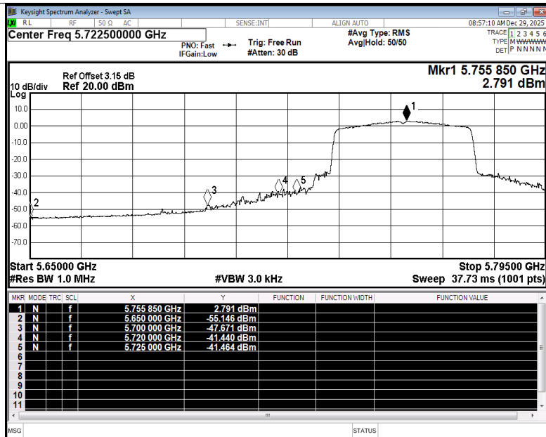
Restrict Band NVNT be40 5755MHz Ant1 Average
