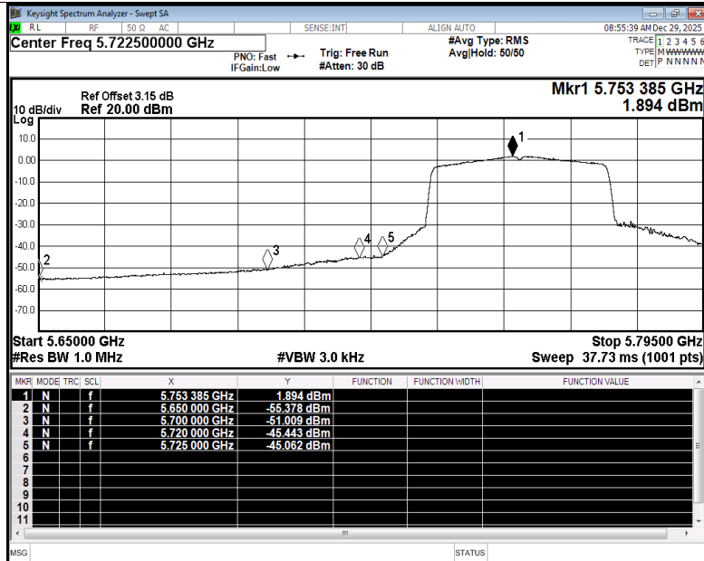
Restrict Band NVNT ax40 5755MHz Ant1 Average
