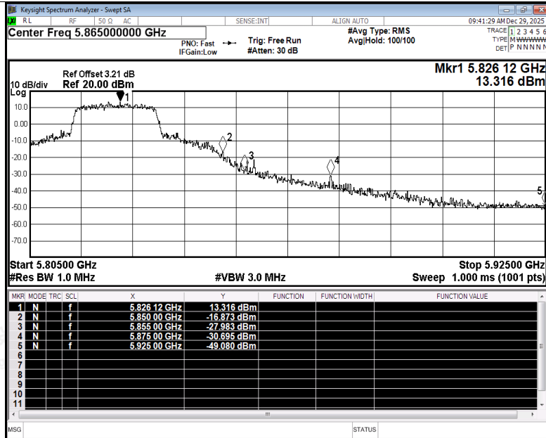
Restrict Band NVNT ax20 5825MHz Ant3 Peak
