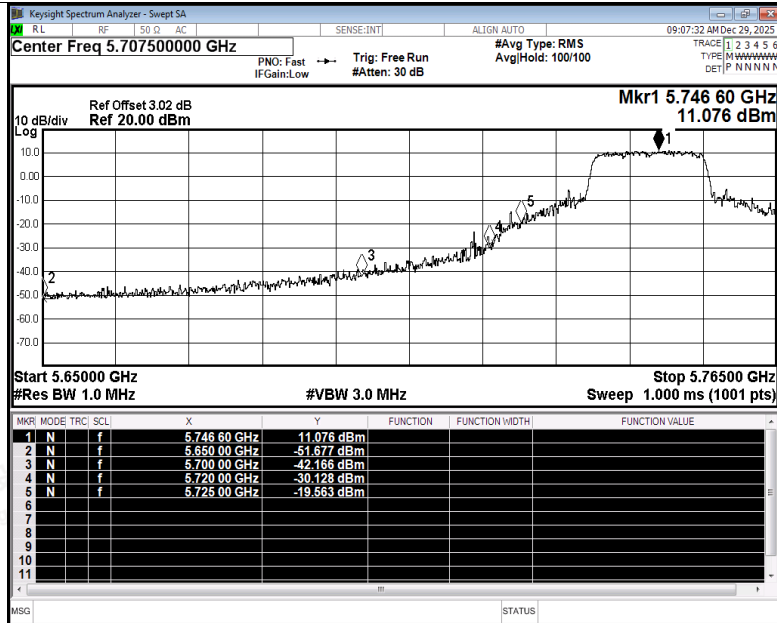
Restrict Band NVNT n20 5745MHz Ant2 Peak
