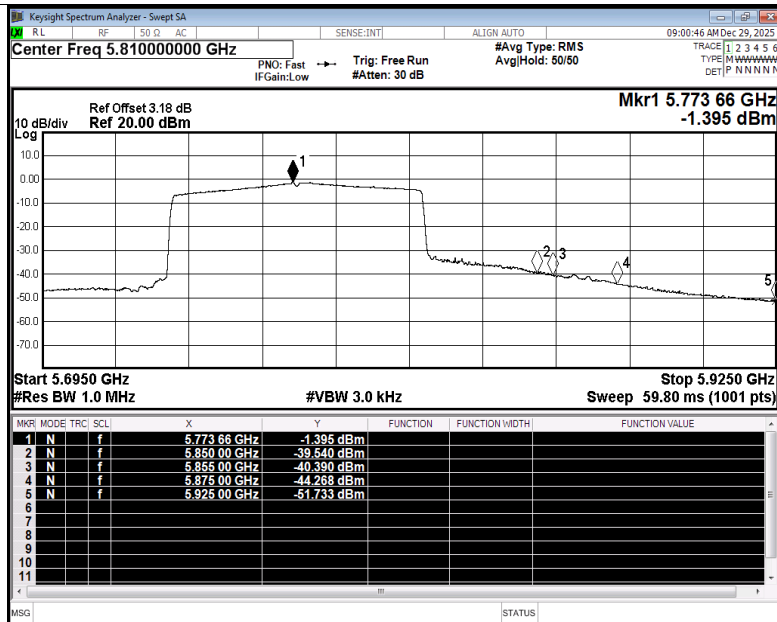
Restrict Band NVNT be80 5775MHz Ant1 Average
