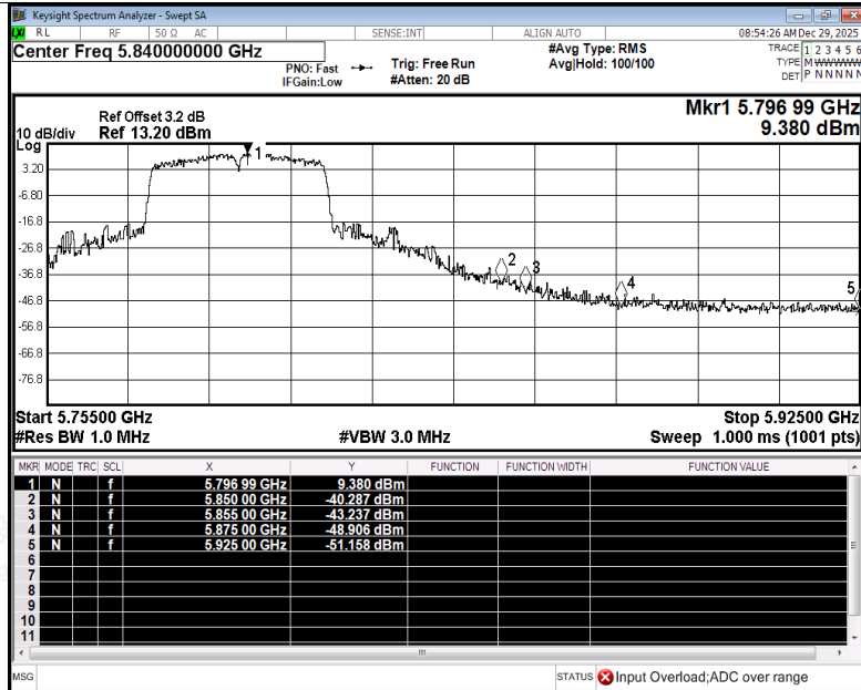
Restrict Band NVNT ac40 5795MHz Ant1 Peak
