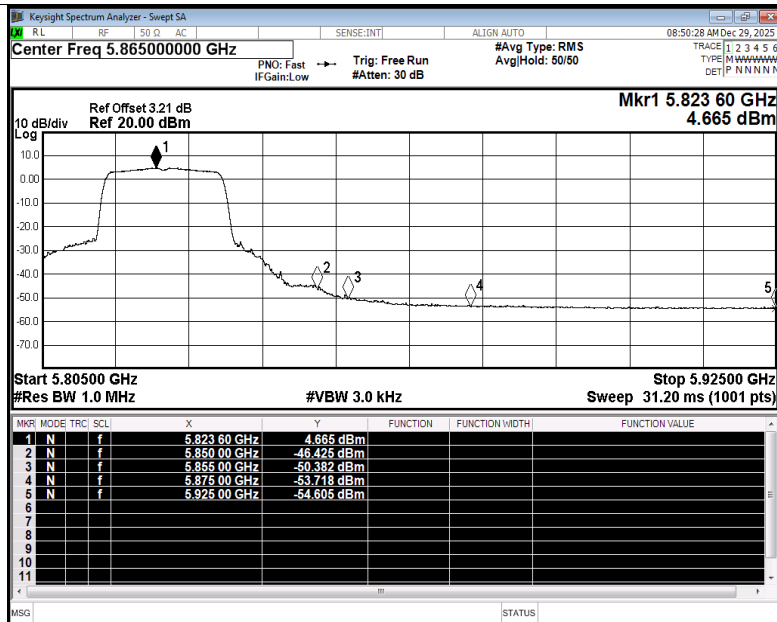
Restrict Band NVNT be20 5825MHz Ant1 Average
