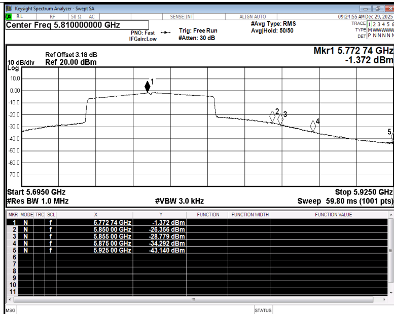
Restrict Band NVNT be80 5775MHz Ant2 Average
