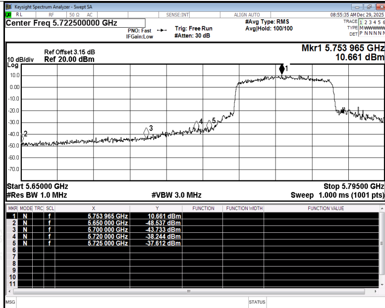
Restrict Band NVNT ax40 5755MHz Ant1 Peak
