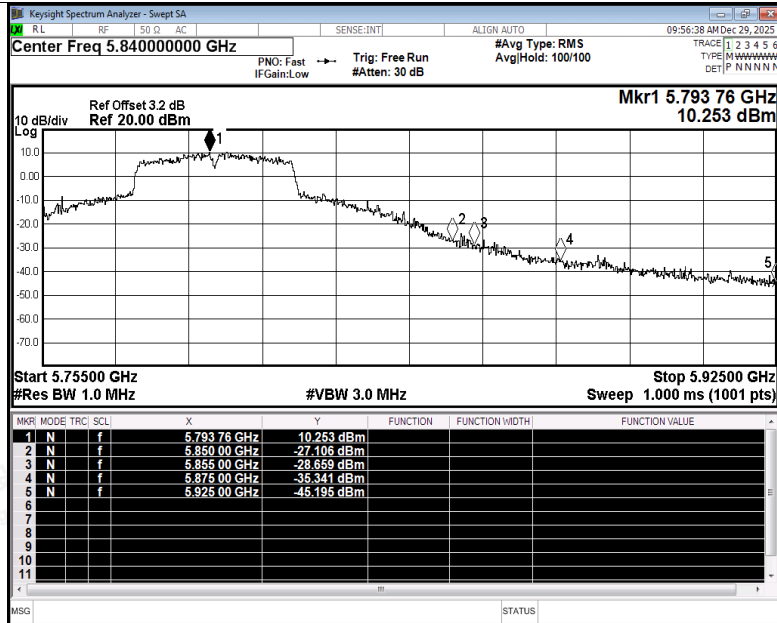
Restrict Band NVNT n40 5795MHz Ant3 Peak
