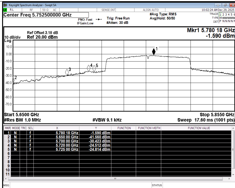
Restrict Band NVNT ac80 5775MHz Ant3 Average
