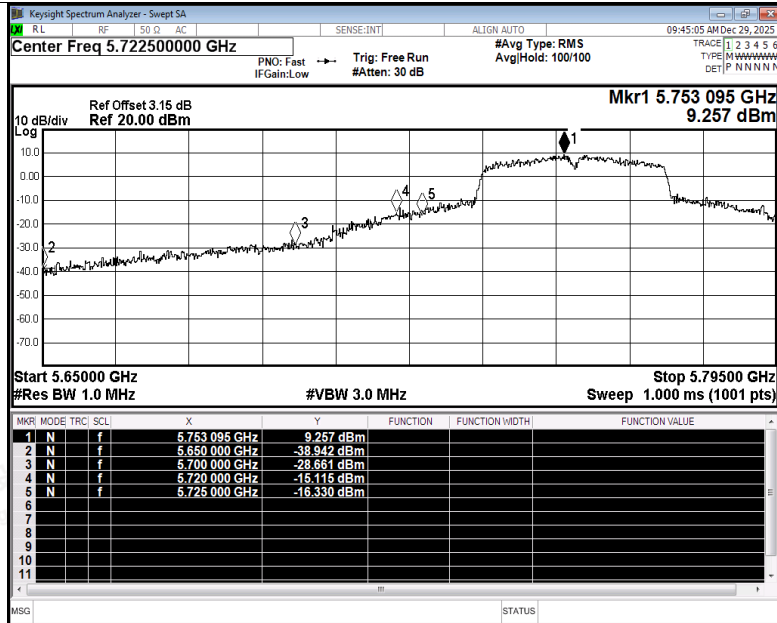
Restrict Band NVNT n40 5755MHz Ant3 Peak
