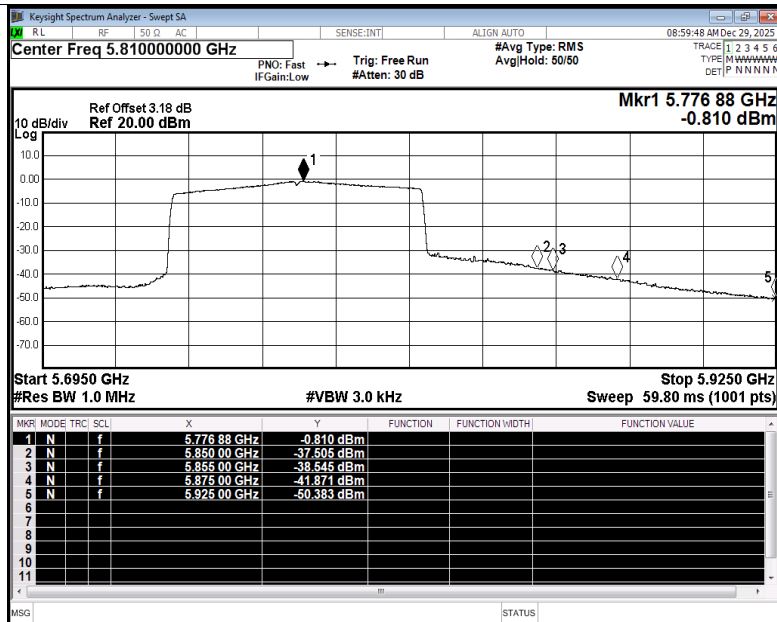
Restrict Band NVNT ax80 5775MHz Ant1 Average
