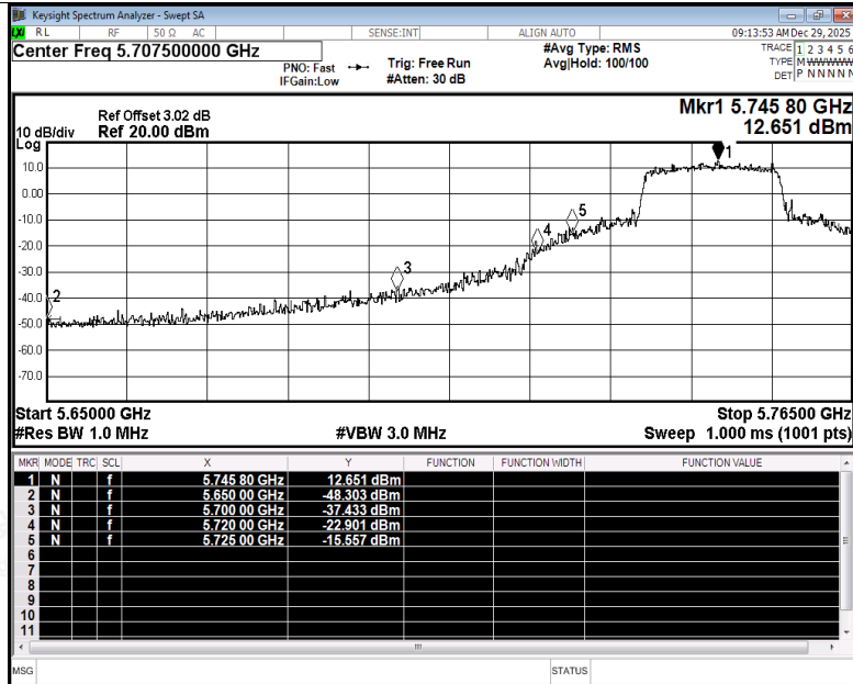
Restrict Band NVNT be20 5745MHz Ant2 Peak
