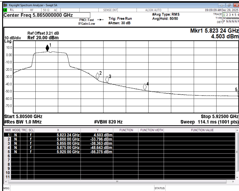
Restrict Band NVNT n20 5825MHz Ant2 Average
