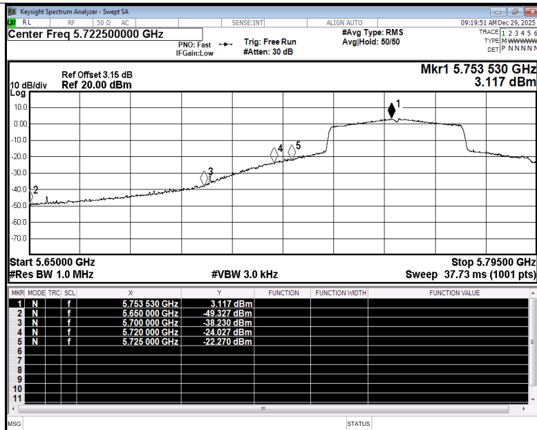
Restrict Band NVNT ax40 5755MHz Ant2 Average
