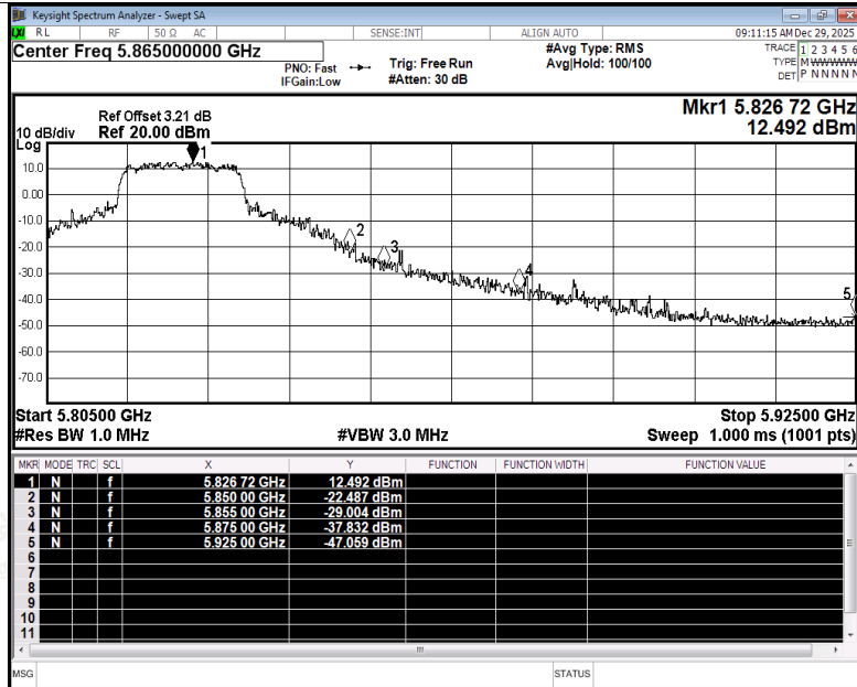
Restrict Band NVNT ac20 5825MHz Ant2 Peak
