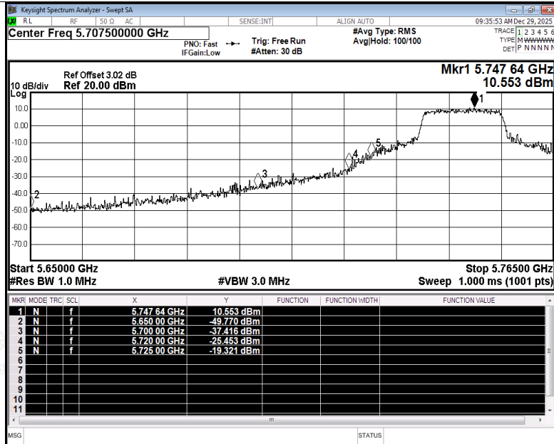
Restrict Band NVNT n20 5745MHz Ant3 Peak
