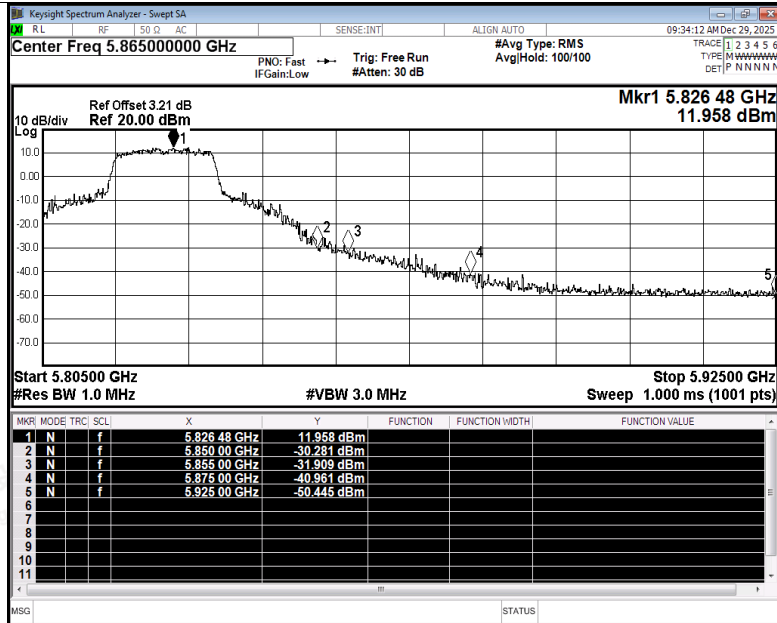
Restrict Band NVNT a 5825MHz Ant3 Peak
