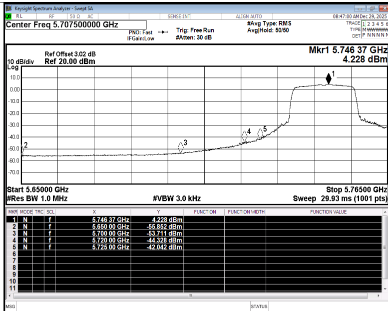
Restrict Band NVNT ax20 5745MHz Ant1 Average
