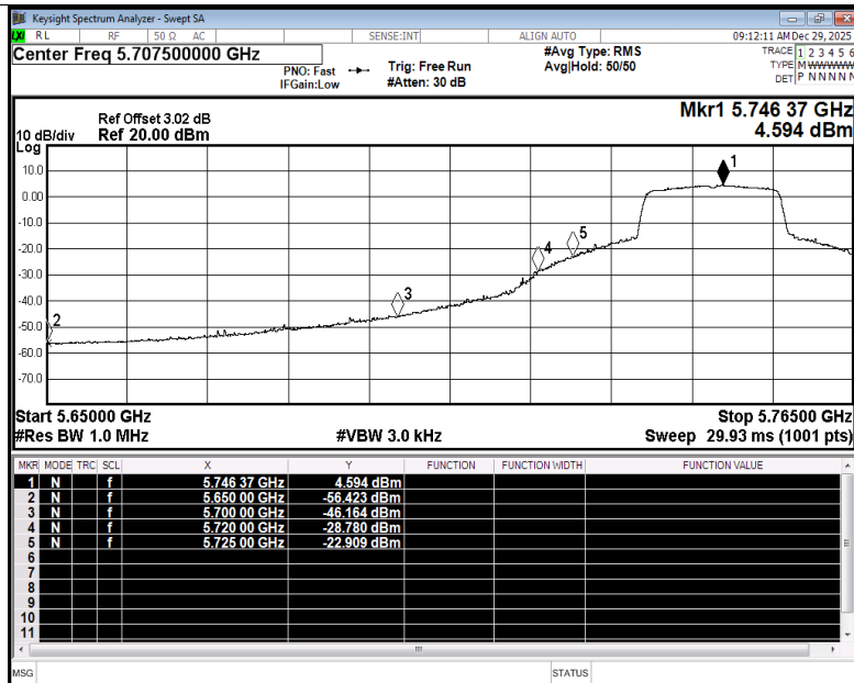
Restrict Band NVNT ax20 5745MHz Ant2 Average
