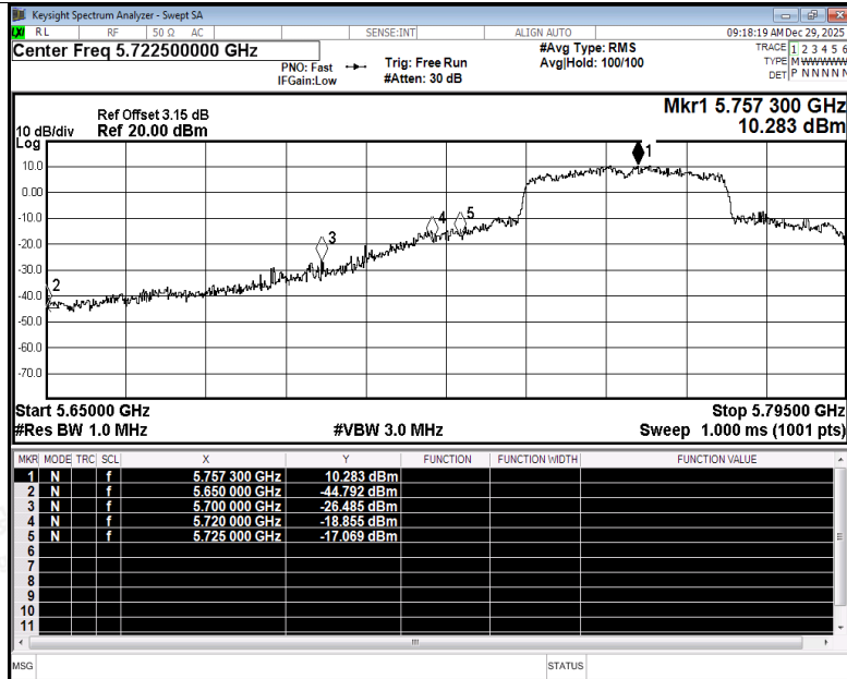
Restrict Band NVNT ac40 5755MHz Ant2 Peak
