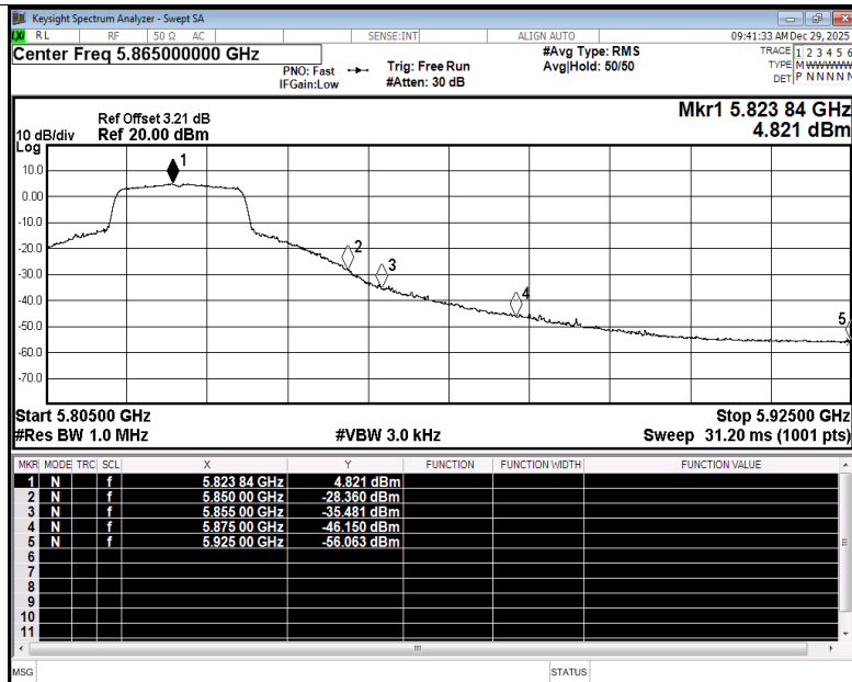
Restrict Band NVNT ax20 5825MHz Ant3 Average
