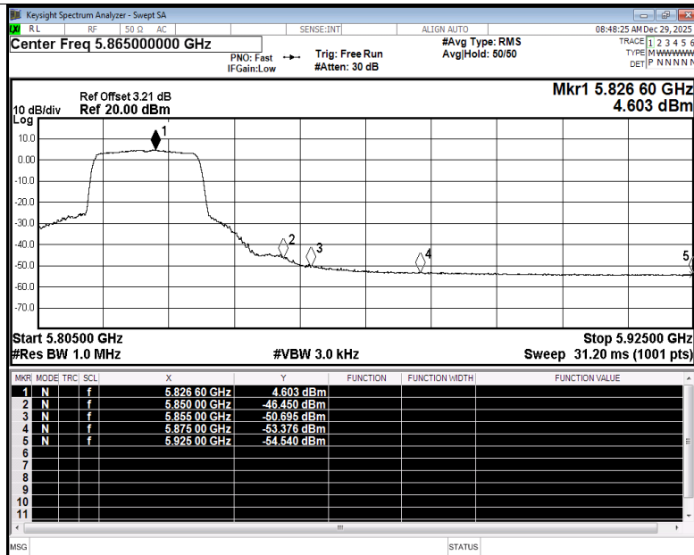
Restrict Band NVNT ax20 5825MHz Ant1 Average
