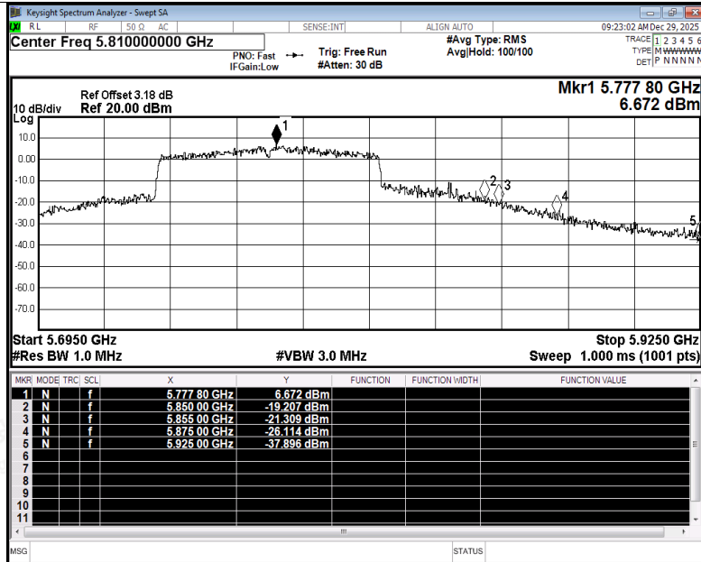
Restrict Band NVNT ac80 5775MHz Ant2 Peak
