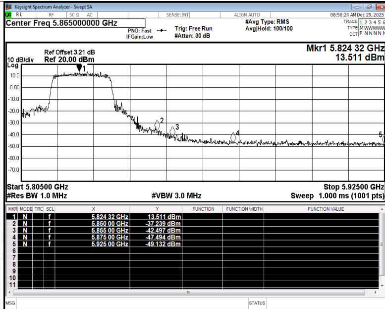
Restrict Band NVNT be20 5825MHz Ant1 Peak
