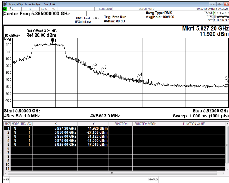
Restrict Band NVNT n20 5825MHz Ant3 Peak
