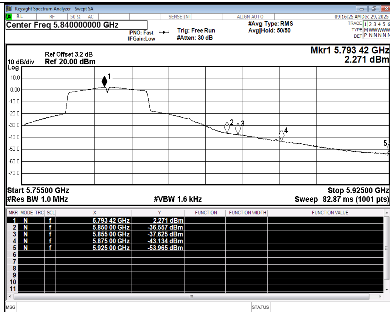
Restrict Band NVNT n40 5795MHz Ant2 Average
