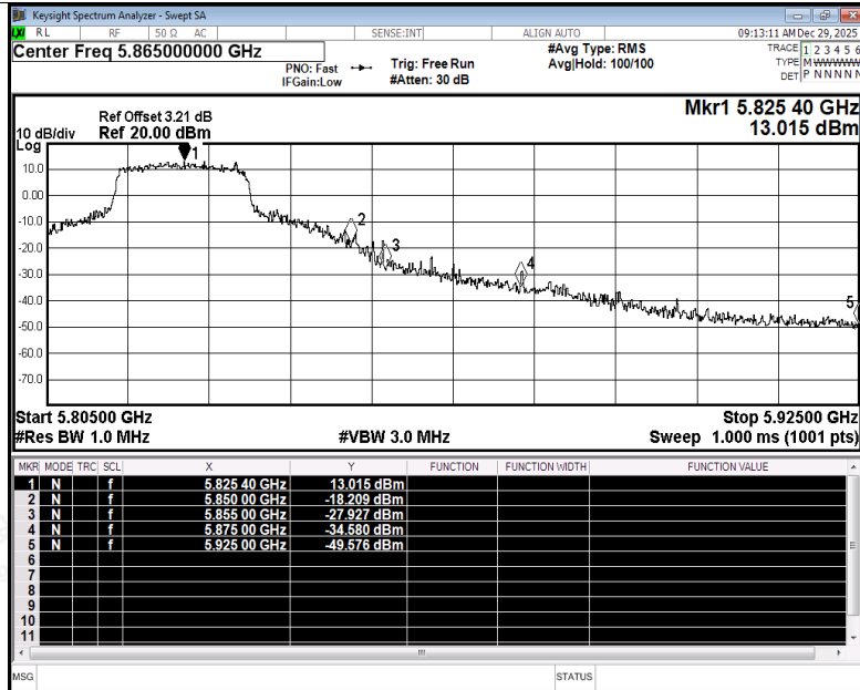
Restrict Band NVNT ax20 5825MHz Ant2 Peak
