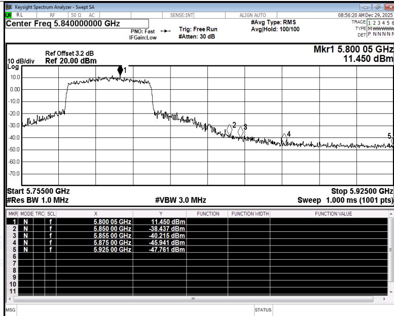
Restrict Band NVNT ax40 5795MHz Ant1 Peak
