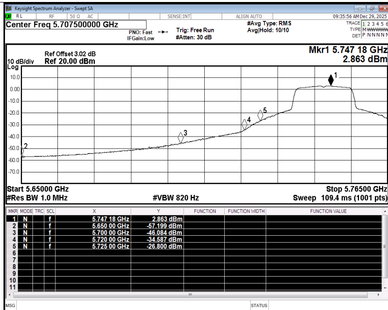
Restrict Band NVNT n20 5745MHz Ant3 Average
