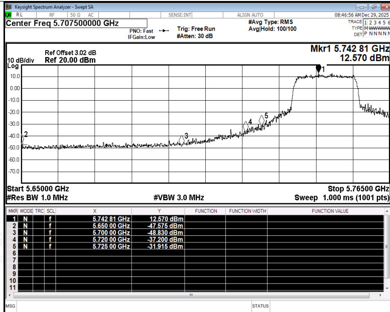
Restrict Band NVNT ax20 5745MHz Ant1 Peak
