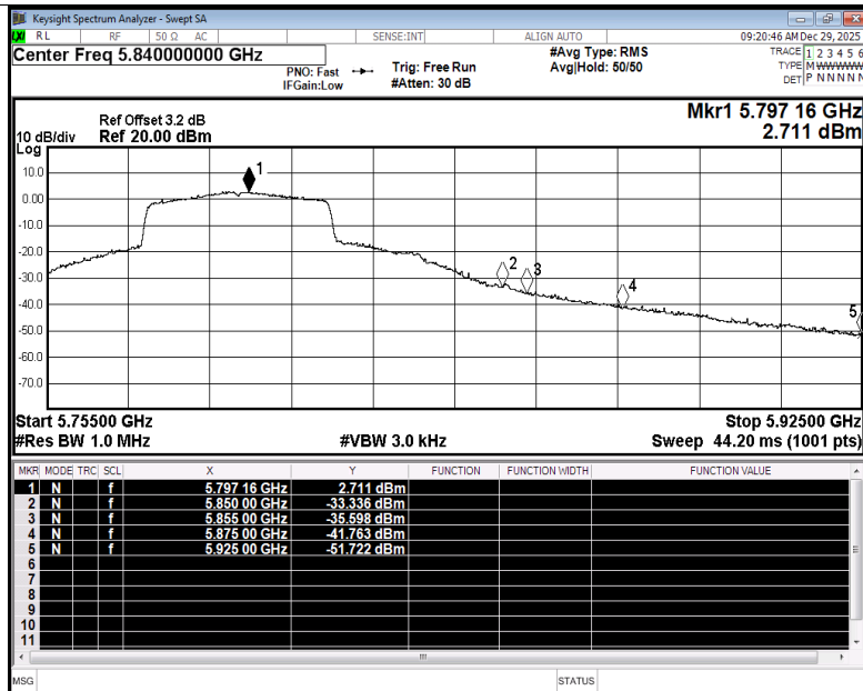
Restrict Band NVNT ax40 5795MHz Ant2 Average
