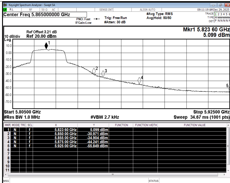
Restrict Band NVNT ac20 5825MHz Ant2 Average
