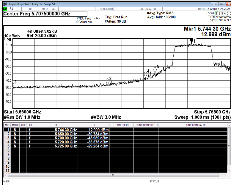
Restrict Band NVNT be20 5745MHz Ant1 Peak
