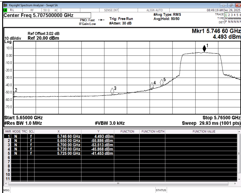
Restrict Band NVNT be20 5745MHz Ant1 Average
