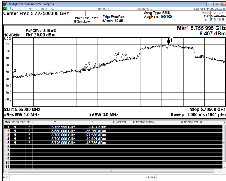
Restrict Band NVNT ac40 5755MHz Ant3 Peak
