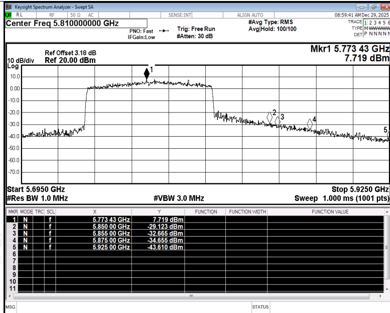
Restrict Band NVNT ax80 5775MHz Ant1 Peak
