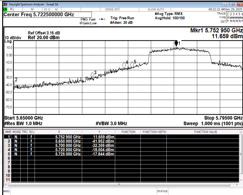
Restrict Band NVNT be40 5755MHz Ant2 Peak
