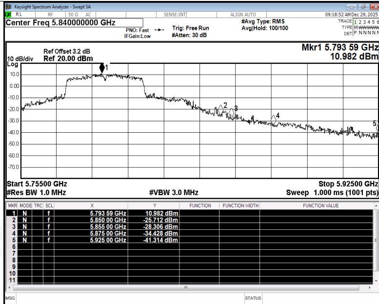
Restrict Band NVNT ac40 5795MHz Ant2 Peak
