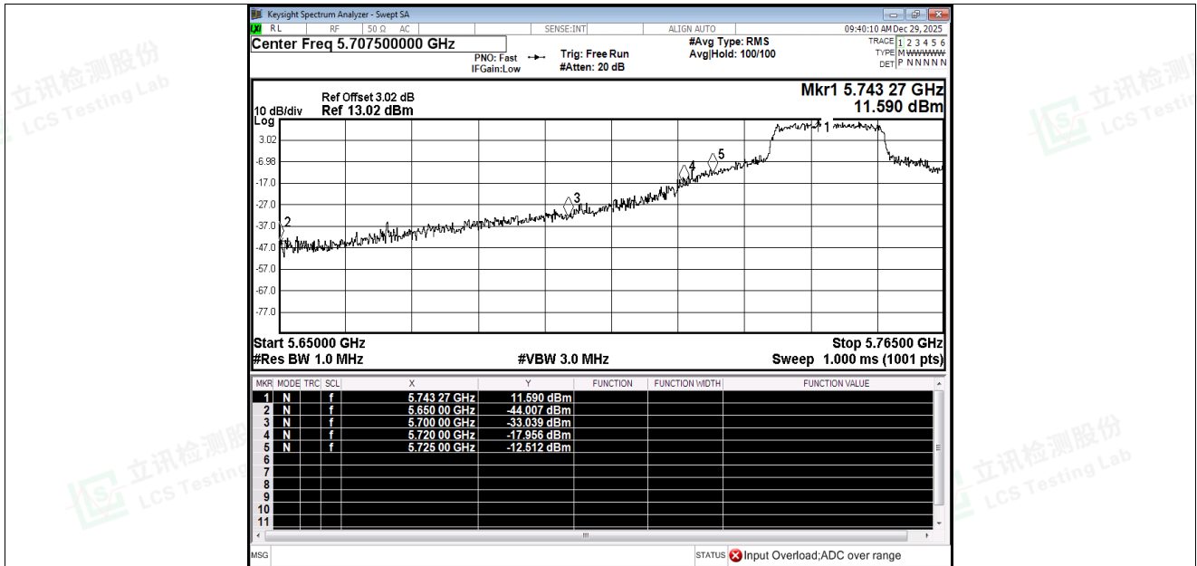
Restrict Band NVNT ax20 5745MHz Ant3 Peak
