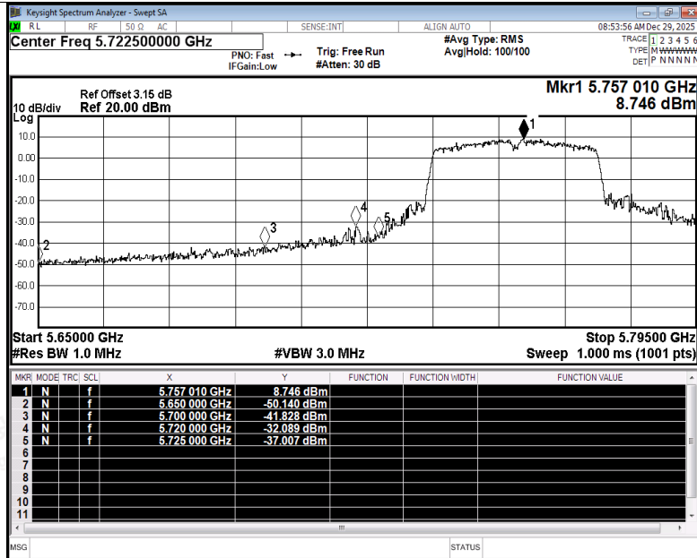
Restrict Band NVNT ac40 5755MHz Ant1 Peak
