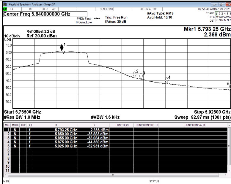
Restrict Band NVNT n40 5795MHz Ant3 Average
