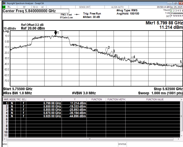
Restrict Band NVNT ac40 5795MHz Ant3 Peak
