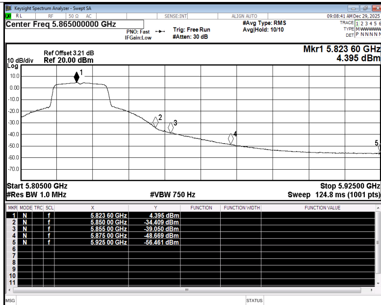
Restrict Band NVNT a 5825MHz Ant2 Average
