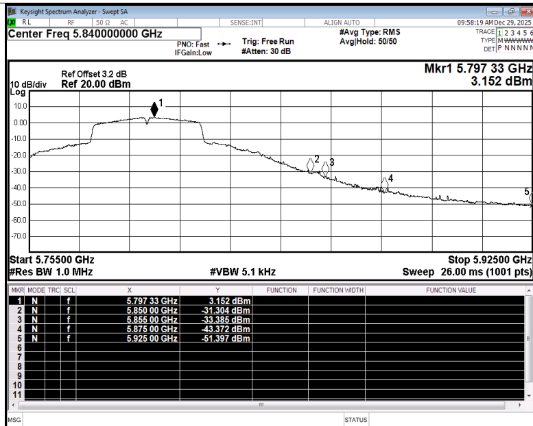
Restrict Band NVNT ac40 5795MHz Ant3 Average
