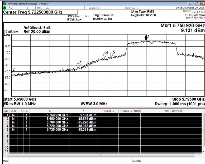
Restrict Band NVNT n40 5755MHz Ant2 Peak
