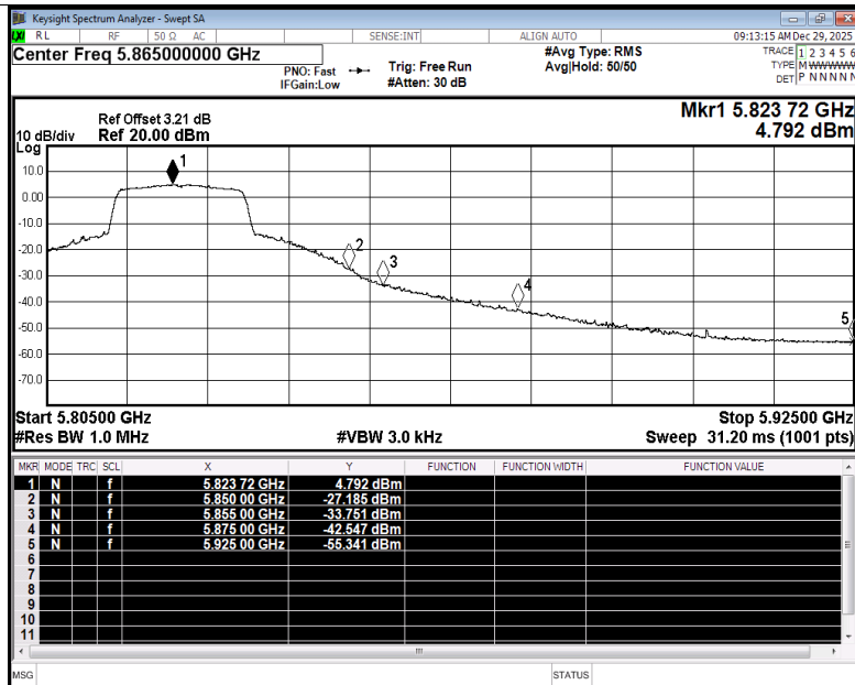
Restrict Band NVNT ax20 5825MHz Ant2 Average
