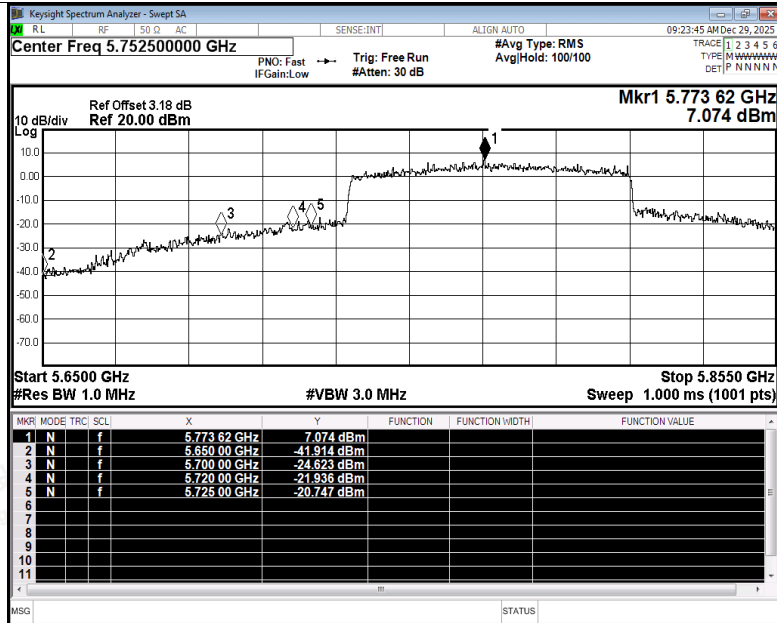
Restrict Band NVNT ax80 5775MHz Ant2 Peak
