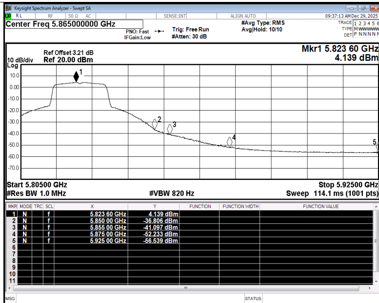
Restrict Band NVNT n20 5825MHz Ant3 Average
