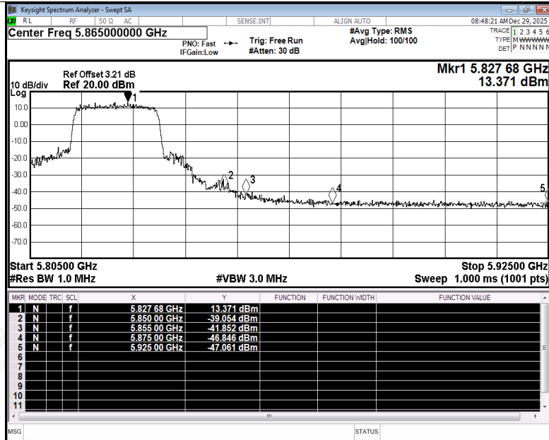
Restrict Band NVNT ax20 5825MHz Ant1 Peak
