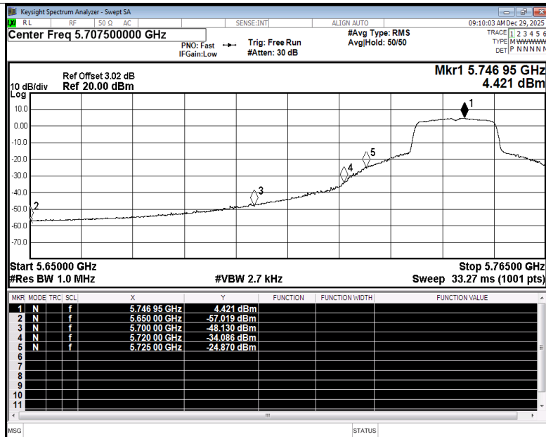
Restrict Band NVNT ac20 5745MHz Ant2 Average
