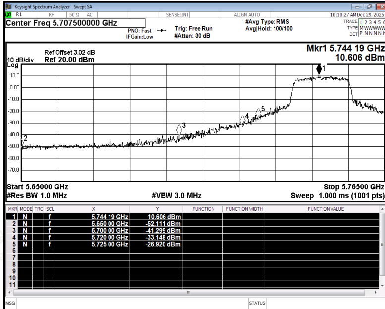
Restrict Band NVNT ac20 5745MHz Ant4 Peak
