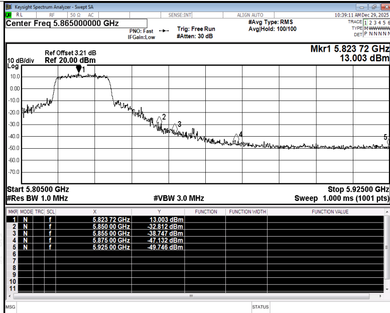
Restrict Band NVNT ac20 5825MHz Ant5 Peak
