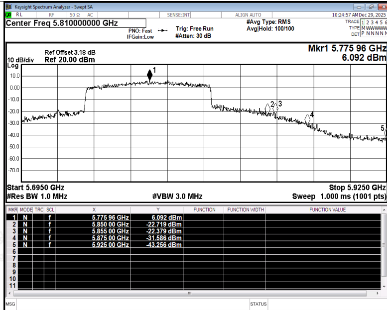
Restrict Band NVNT ax80 5775MHz Ant4 Peak
