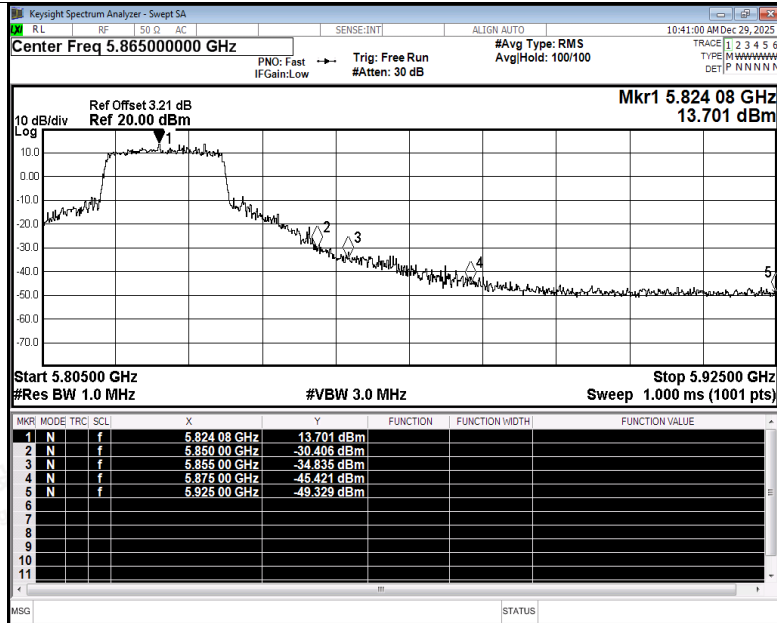
Restrict Band NVNT ax20 5825MHz Ant5 Peak
