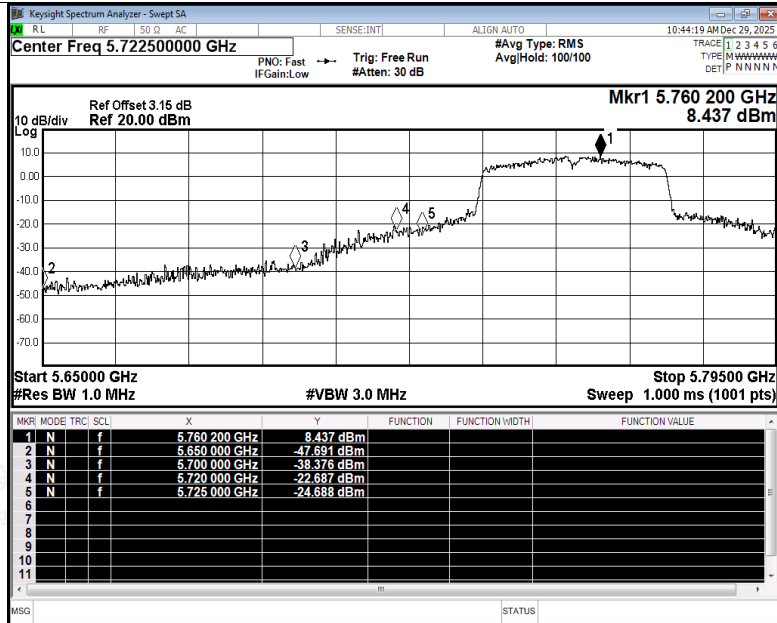
Restrict Band NVNT n40 5755MHz Ant5 Peak
