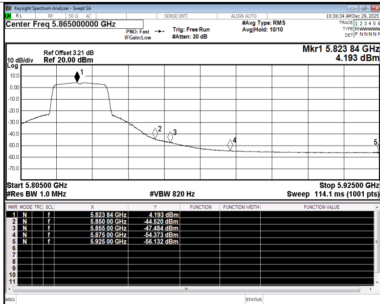
Restrict Band NVNT n20 5825MHz Ant5 Average
