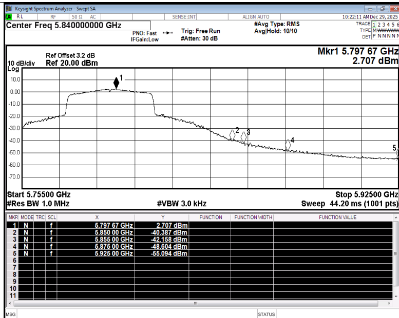
Restrict Band NVNT ax40 5795MHz Ant4 Average
