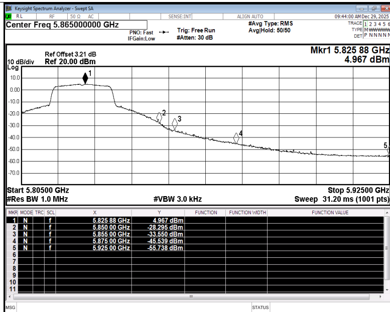
Restrict Band NVNT be20 5825MHz Ant3 Average
