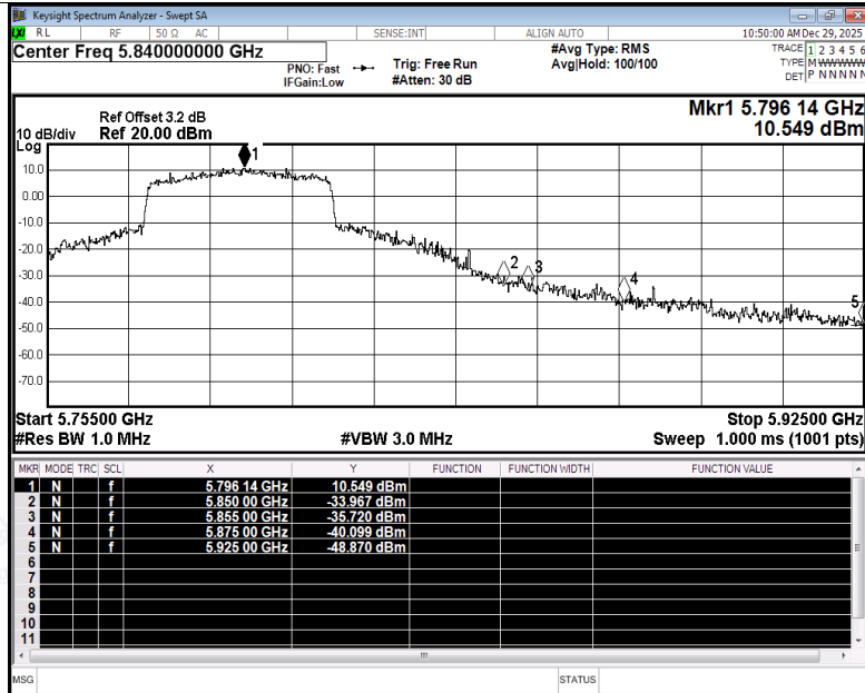
Restrict Band NVNT ax40 5795MHz Ant5 Peak
