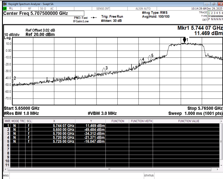
Restrict Band NVNT be20 5745MHz Ant4 Peak
