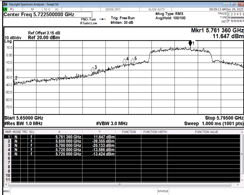
Restrict Band NVNT ax40 5755MHz Ant3 Peak
