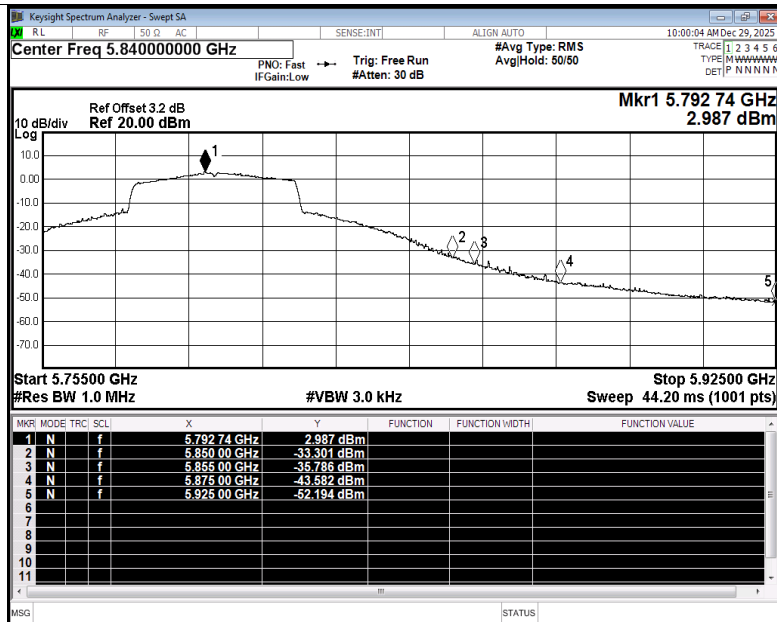
Restrict Band NVNT ax40 5795MHz Ant3 Average
