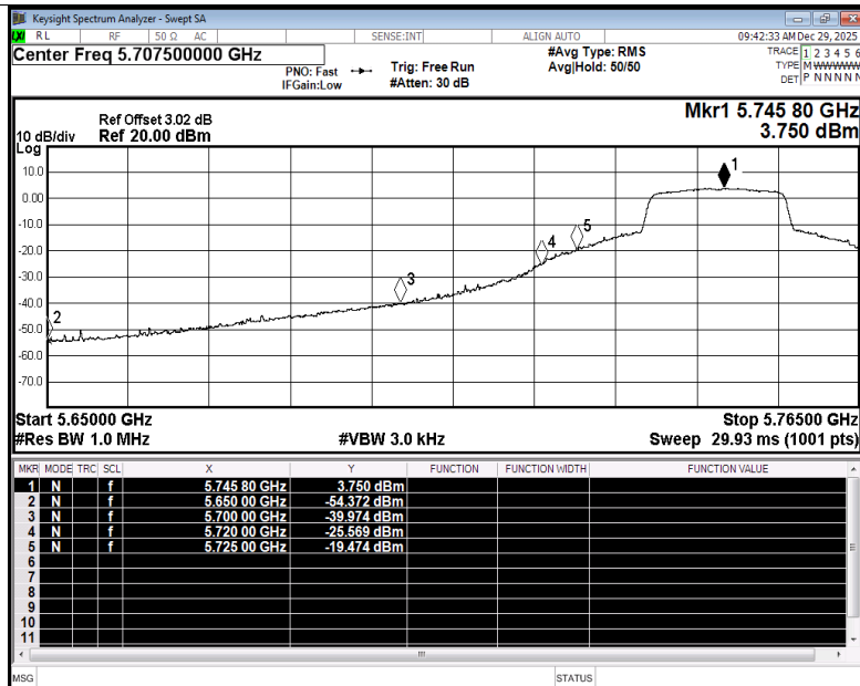
Restrict Band NVNT be20 5745MHz Ant3 Average
