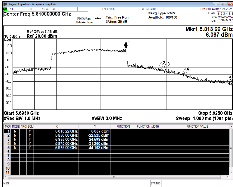
Restrict Band NVNT ax80 5775MHz Ant5 Peak
