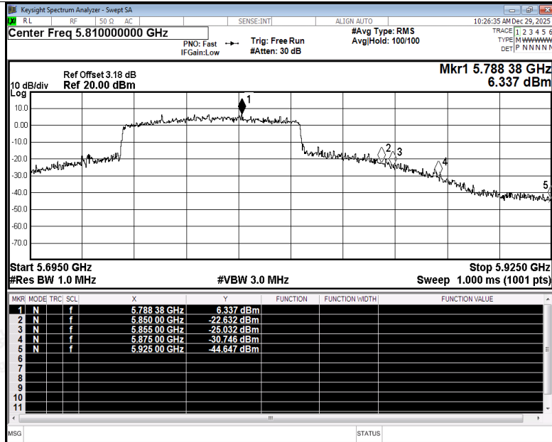
Restrict Band NVNT be80 5775MHz Ant4 Peak
