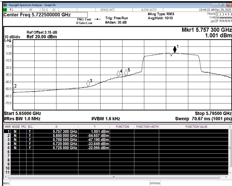
Restrict Band NVNT n40 5755MHz Ant5 Average
