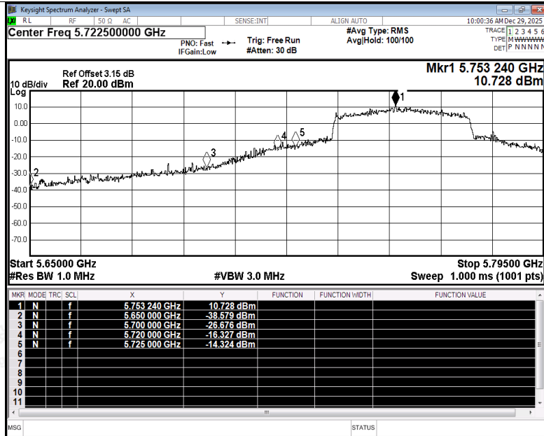
Restrict Band NVNT be40 5755MHz Ant3 Peak
