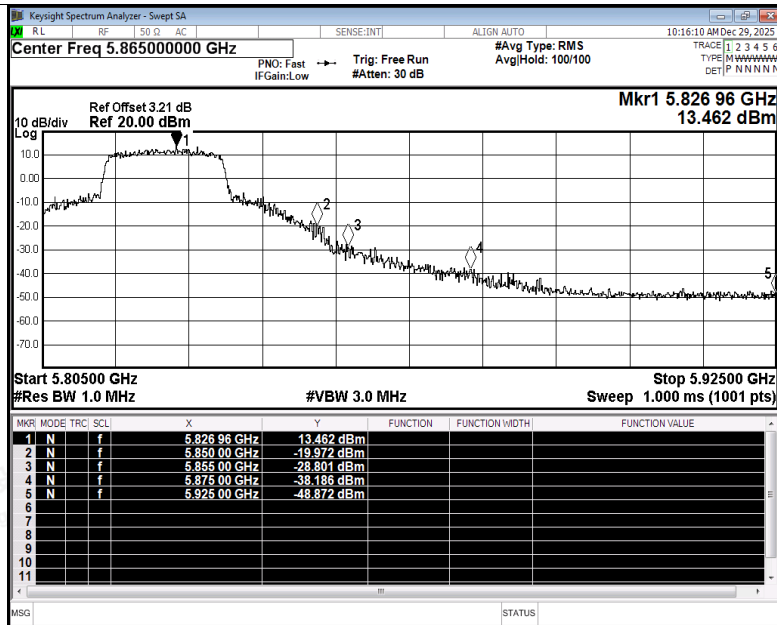
Restrict Band NVNT be20 5825MHz Ant4 Peak
