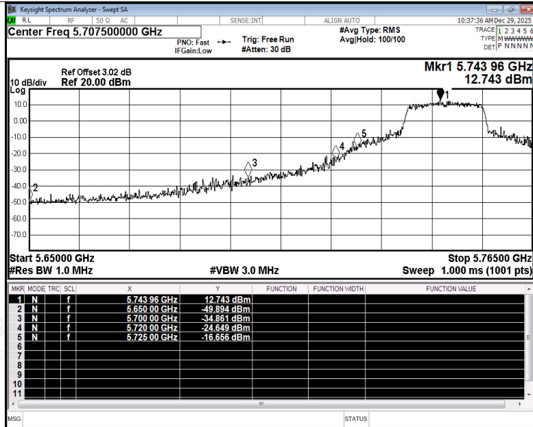
Restrict Band NVNT ac20 5745MHz Ant5 Peak
