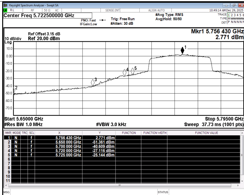
Restrict Band NVNT ax40 5755MHz Ant5 Average
