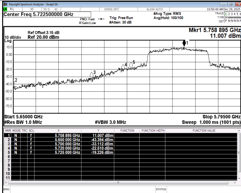
Restrict Band NVNT be40 5755MHz Ant5 Peak
