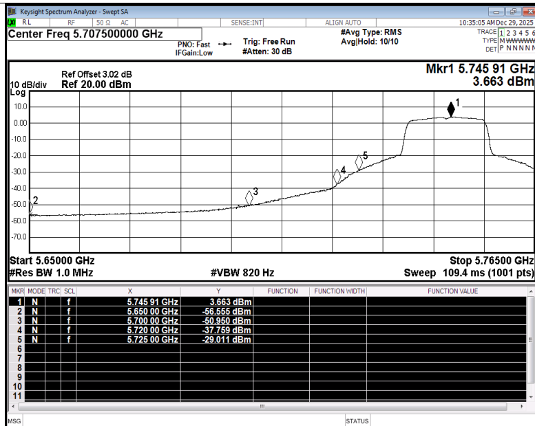
Restrict Band NVNT n20 5745MHz Ant5 Average
