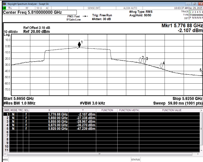
Restrict Band NVNT ax80 5775MHz Ant3 Average
