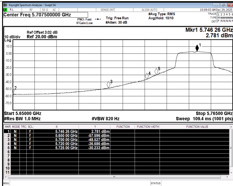
Restrict Band NVNT n20 5745MHz Ant4 Average
