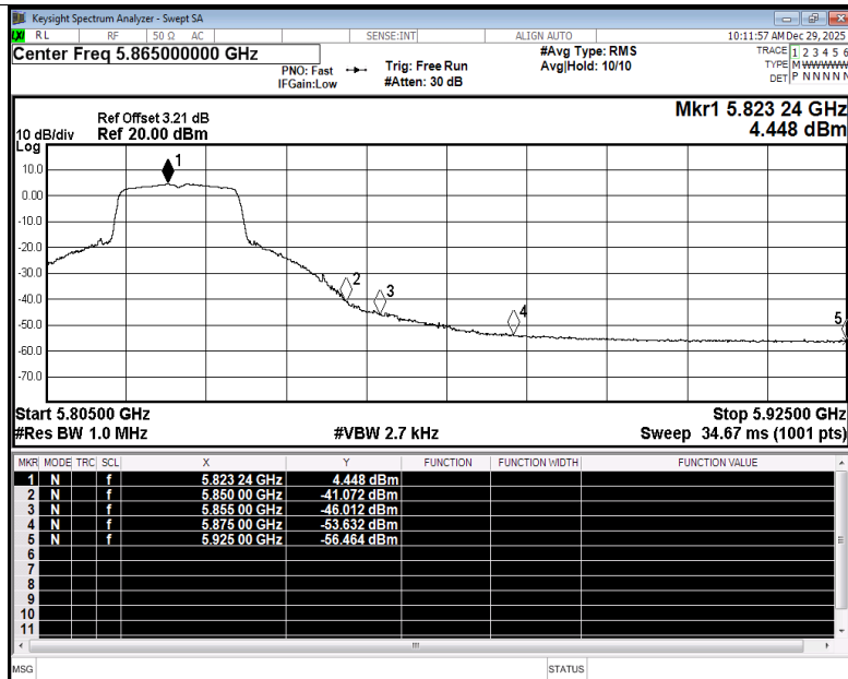
Restrict Band NVNT ac20 5825MHz Ant4 Average
