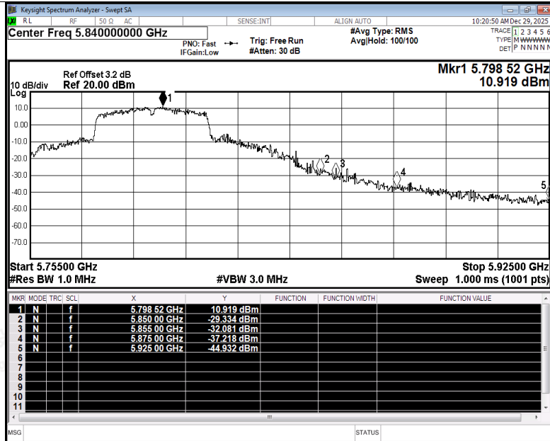
Restrict Band NVNT ac40 5795MHz Ant4 Peak
