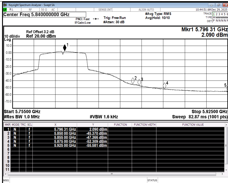
Restrict Band NVNT n40 5795MHz Ant5 Average
