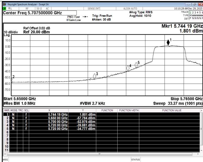
Restrict Band NVNT ac20 5745MHz Ant4 Average
