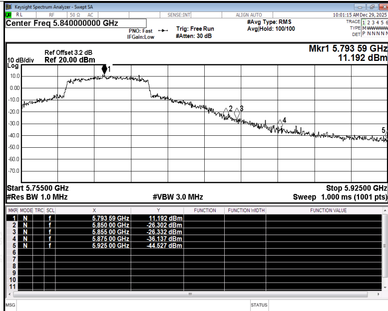
Restrict Band NVNT be40 5795MHz Ant3 Peak
