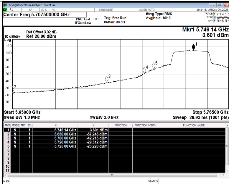
Restrict Band NVNT be20 5745MHz Ant4 Average
