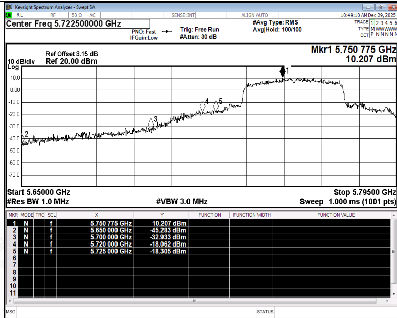
Restrict Band NVNT ax40 5755MHz Ant5 Peak
