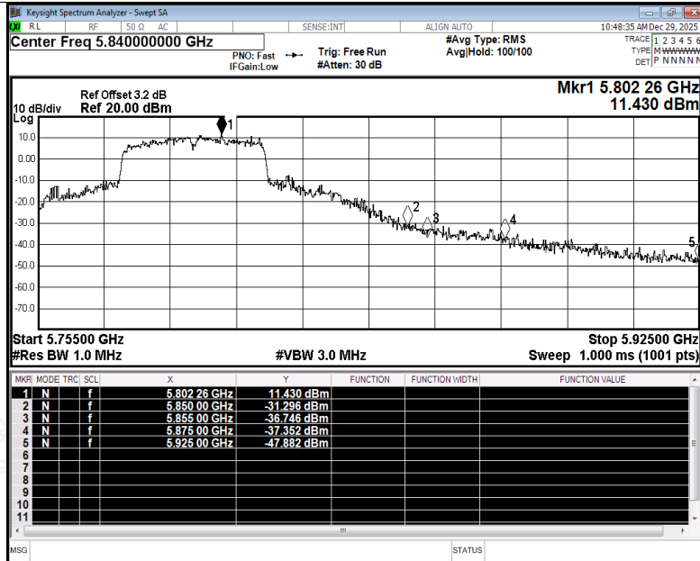
Restrict Band NVNT ac40 5795MHz Ant5 Peak
