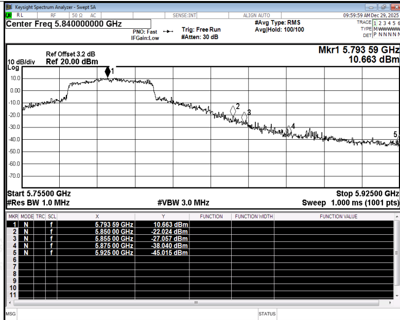
Restrict Band NVNT ax40 5795MHz Ant3 Peak
