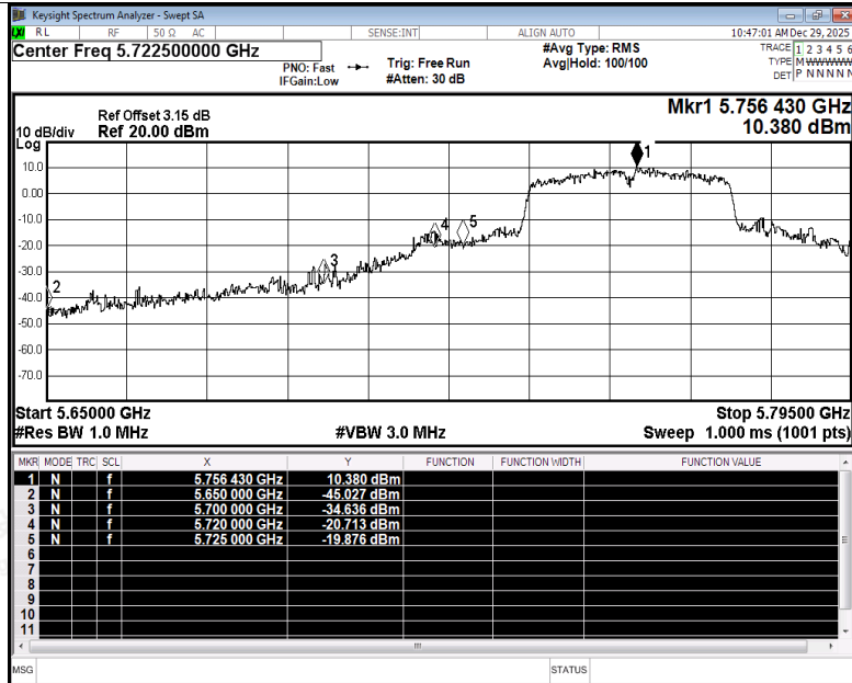
Restrict Band NVNT ac40 5755MHz Ant5 Peak
