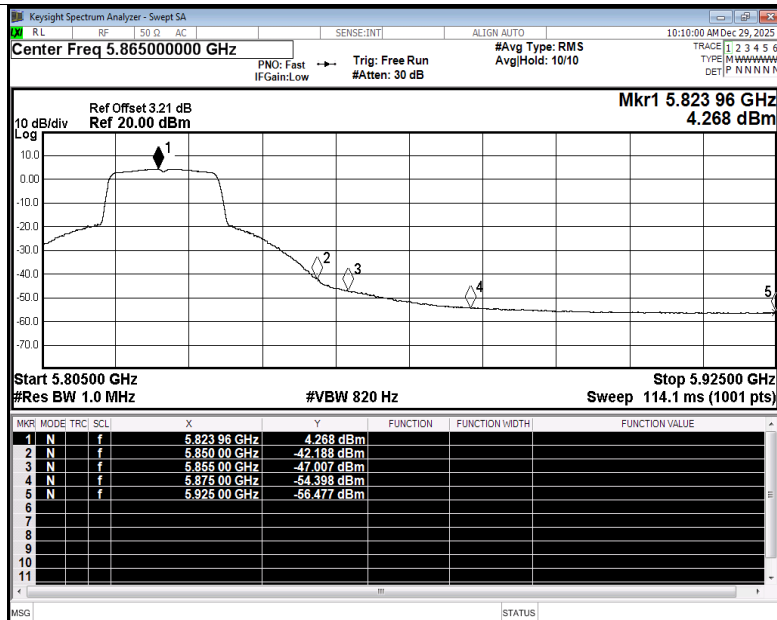
Restrict Band NVNT n20 5825MHz Ant4 Average
