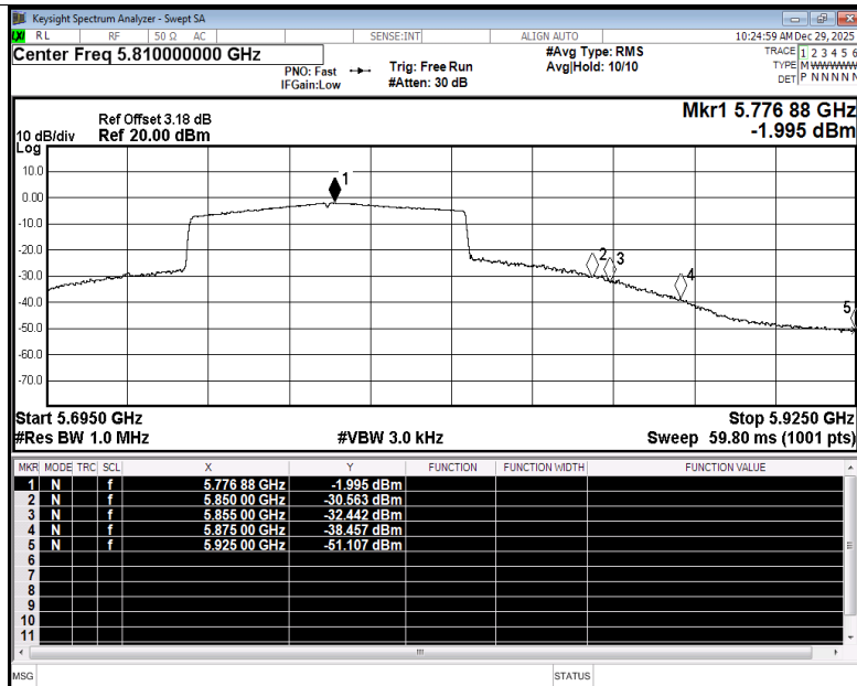
Restrict Band NVNT ax80 5775MHz Ant4 Average
