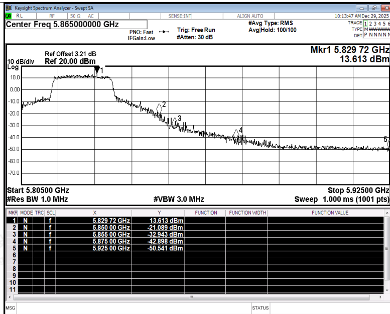
Restrict Band NVNT ax20 5825MHz Ant4 Peak
