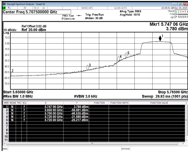
Restrict Band NVNT ax20 5745MHz Ant5 Average
