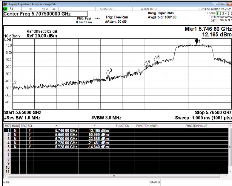
Restrict Band NVNT be20 5745MHz Ant5 Peak
