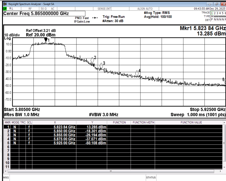
Restrict Band NVNT be20 5825MHz Ant3 Peak
