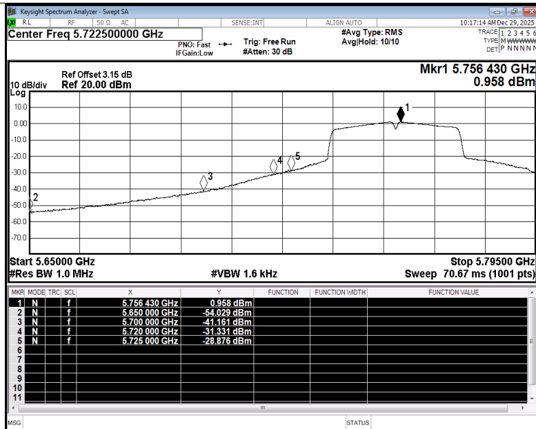
Restrict Band NVNT n40 5755MHz Ant4 Average
