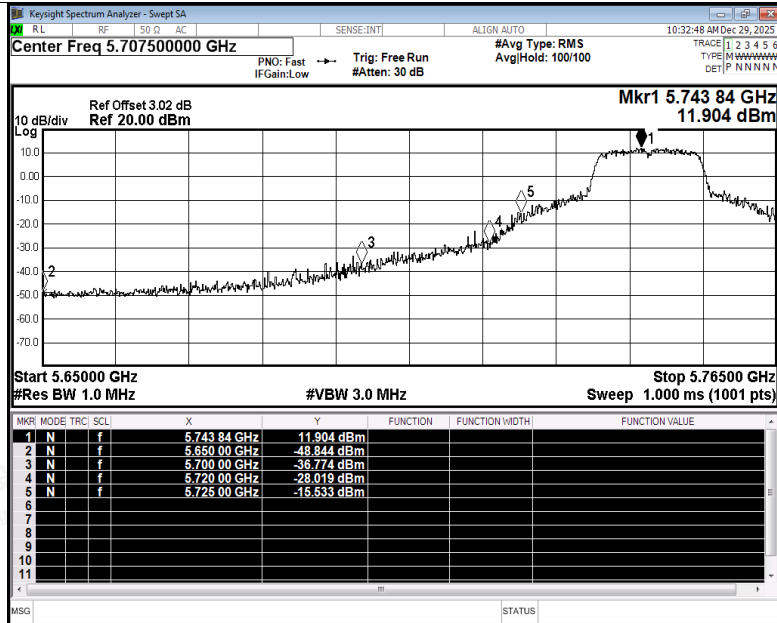
Restrict Band NVNT a 5745MHz Ant5 Peak
