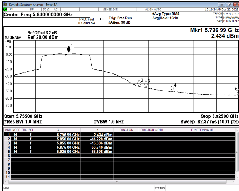
Restrict Band NVNT n40 5795MHz Ant4 Average
