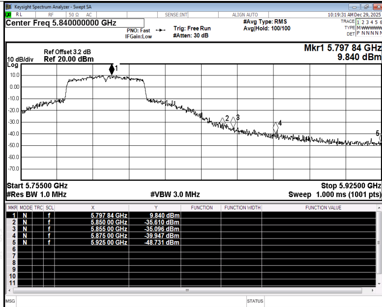
Restrict Band NVNT n40 5795MHz Ant4 Peak
