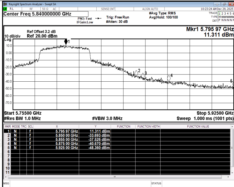
Restrict Band NVNT be40 5795MHz Ant4 Peak
