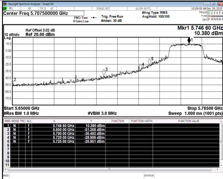
Restrict Band NVNT n20 5745MHz Ant4 Peak
