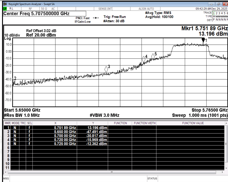
Restrict Band NVNT be20 5745MHz Ant3 Peak
