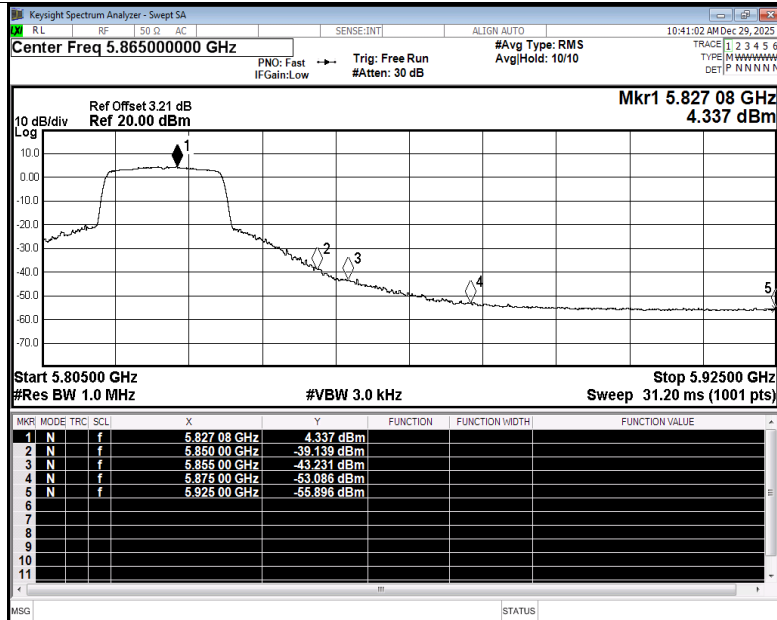
Restrict Band NVNT ax20 5825MHz Ant5 Average
