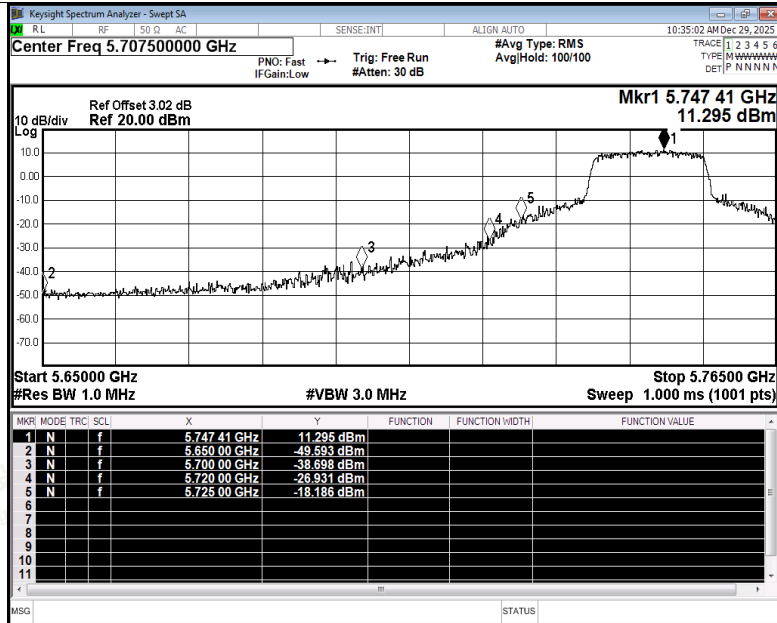
Restrict Band NVNT n20 5745MHz Ant5 Peak
