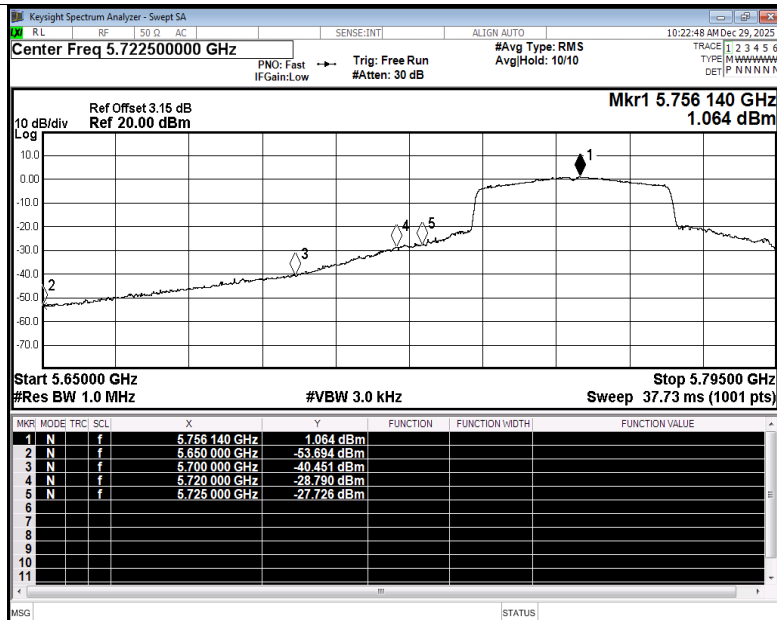
Restrict Band NVNT be40 5755MHz Ant4 Average
