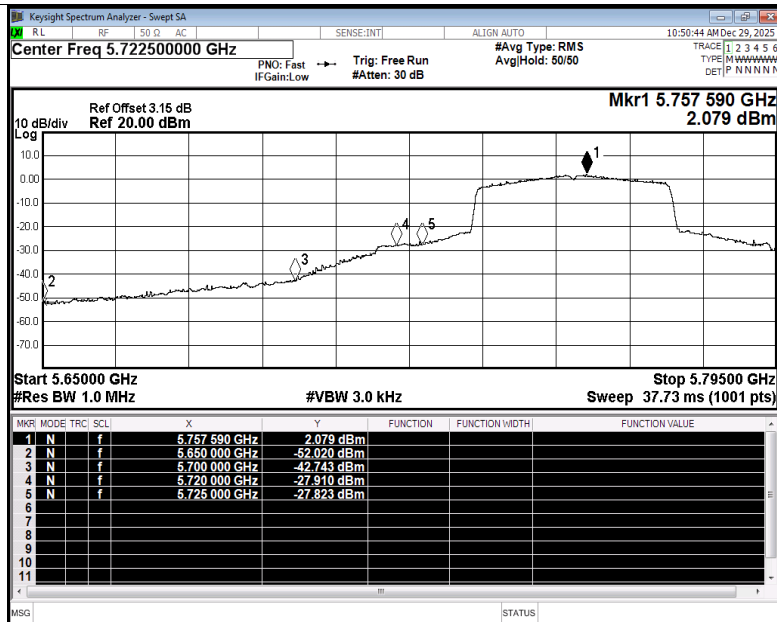
Restrict Band NVNT be40 5755MHz Ant5 Average
