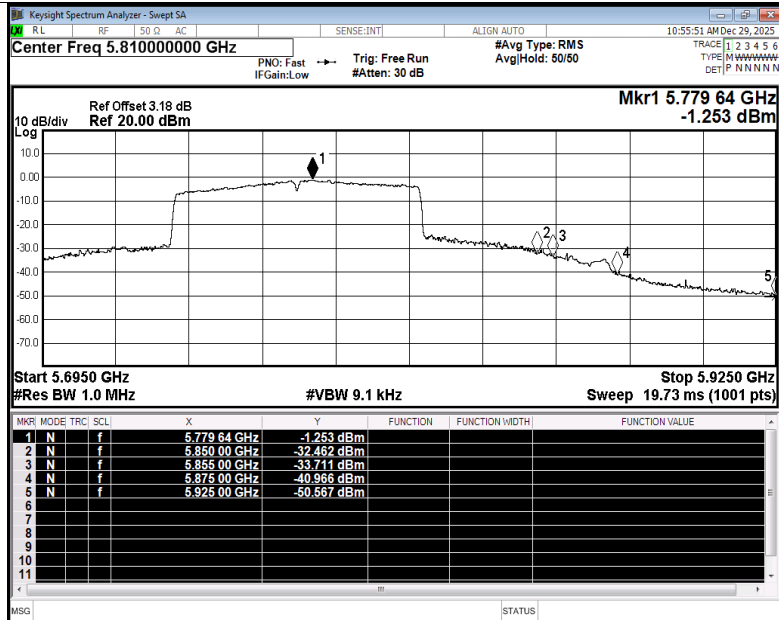
Restrict Band NVNT ac80 5775MHz Ant5 Average
