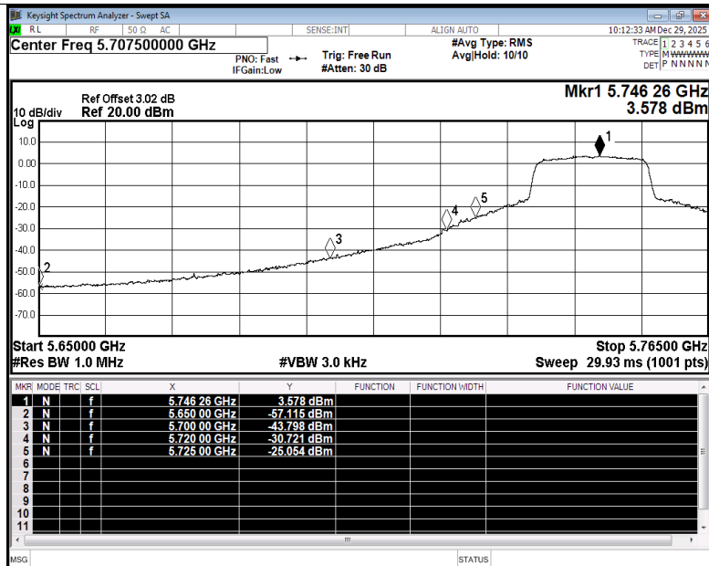
Restrict Band NVNT ax20 5745MHz Ant4 Average
