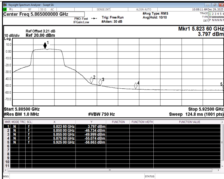
Restrict Band NVNT a 5825MHz Ant4 Average
