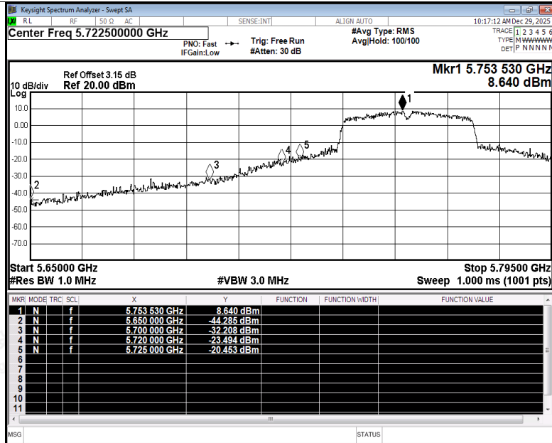
Restrict Band NVNT n40 5755MHz Ant4 Peak
