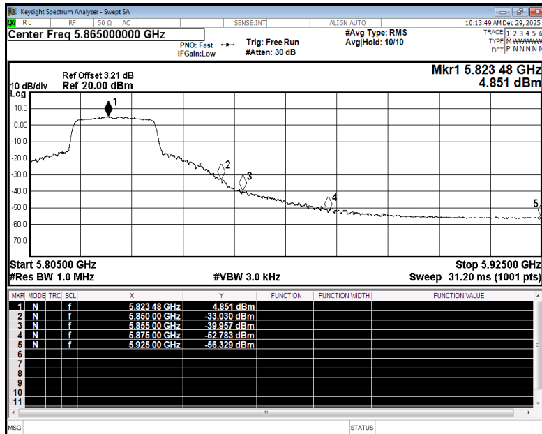
Restrict Band NVNT ax20 5825MHz Ant4 Average
