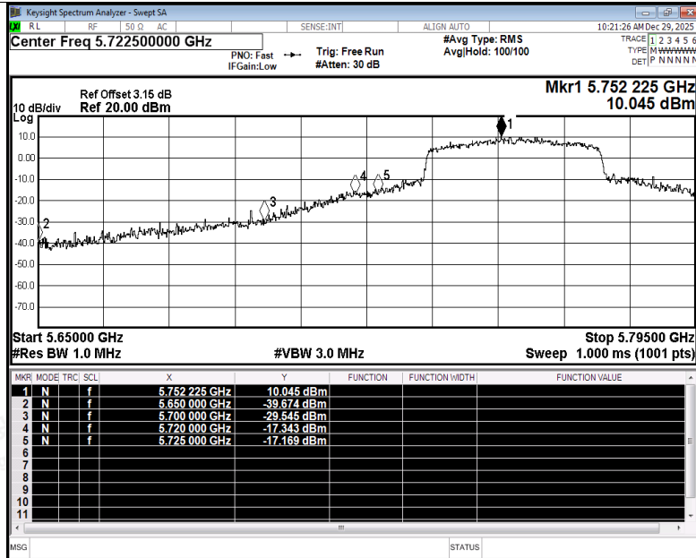
Restrict Band NVNT ax40 5755MHz Ant4 Peak
