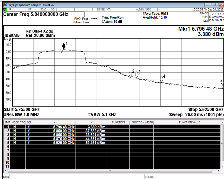
Restrict Band NVNT ac40 5795MHz Ant4 Average
