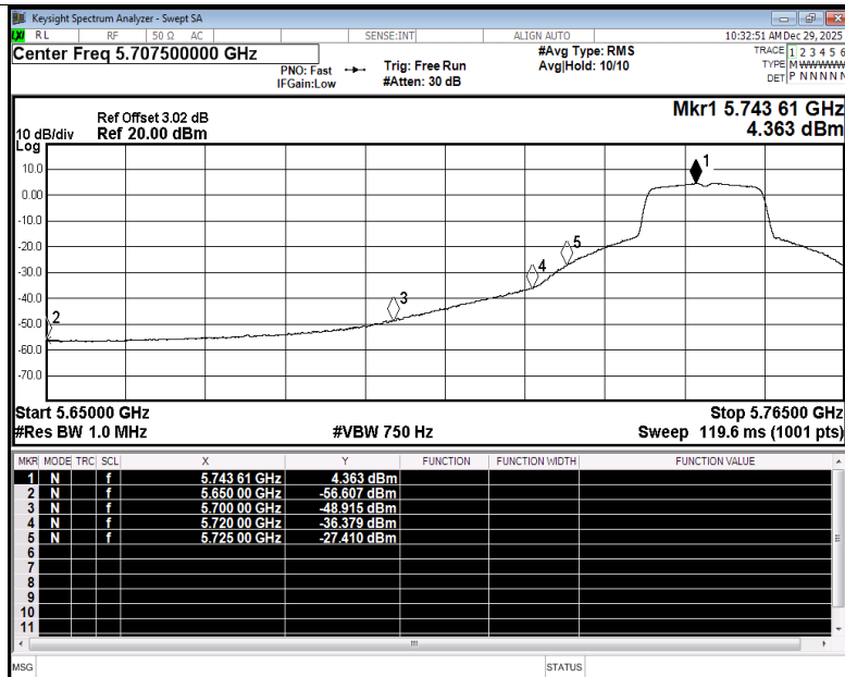
Restrict Band NVNT a 5745MHz Ant5 Average
