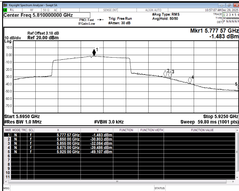
Restrict Band NVNT ax80 5775MHz Ant5 Average
