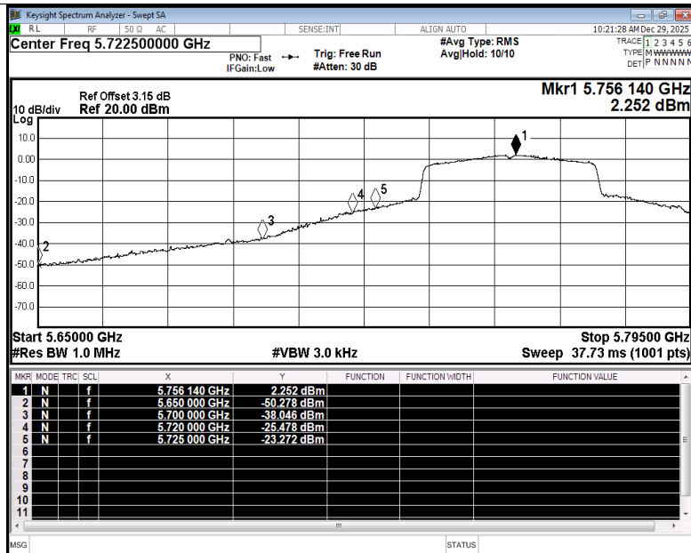
Restrict Band NVNT ax40 5755MHz Ant4 Average
