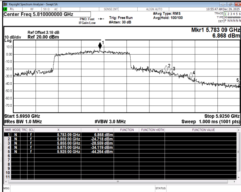
Restrict Band NVNT ac80 5775MHz Ant5 Peak
