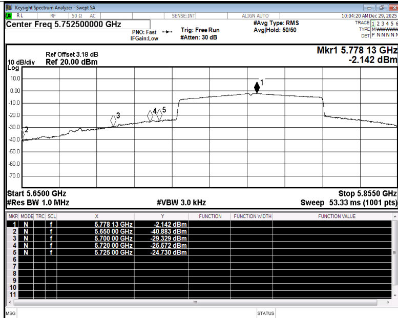
Restrict Band NVNT be80 5775MHz Ant3 Average
