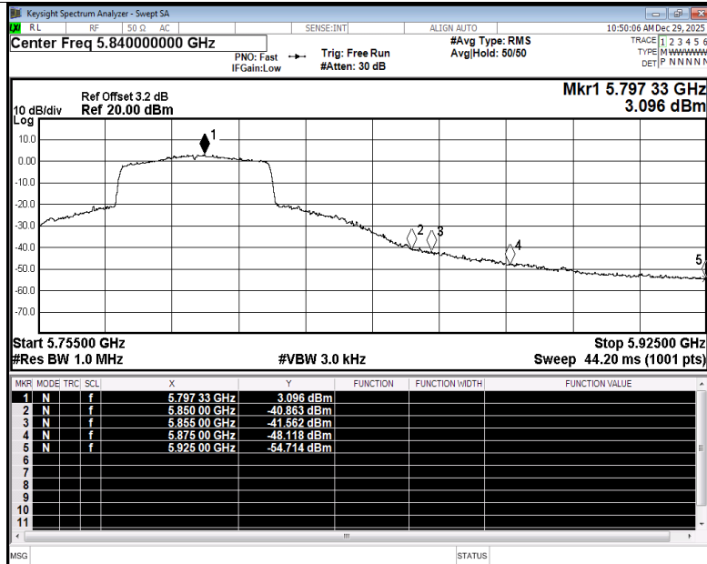
Restrict Band NVNT ax40 5795MHz Ant5 Average
