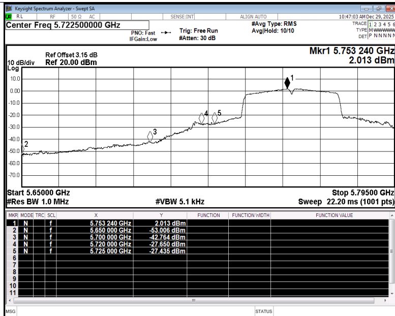
Restrict Band NVNT ac40 5755MHz Ant5 Average
