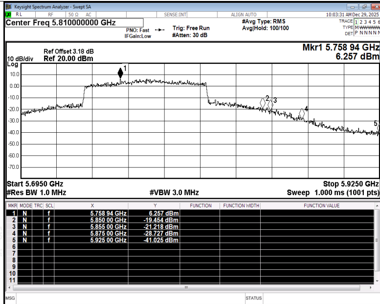
Restrict Band NVNT ax80 5775MHz Ant3 Peak
