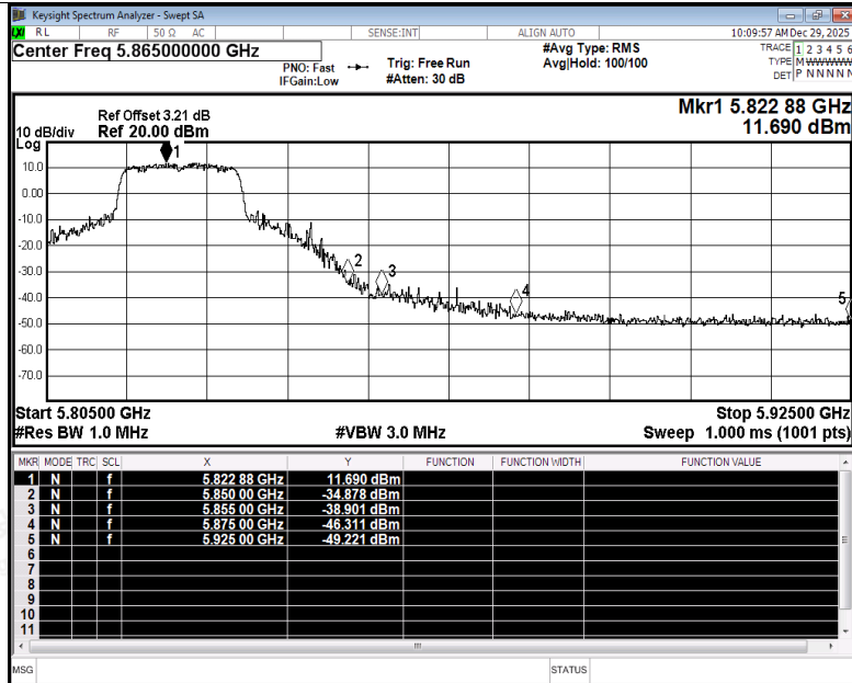
Restrict Band NVNT n20 5825MHz Ant4 Peak
