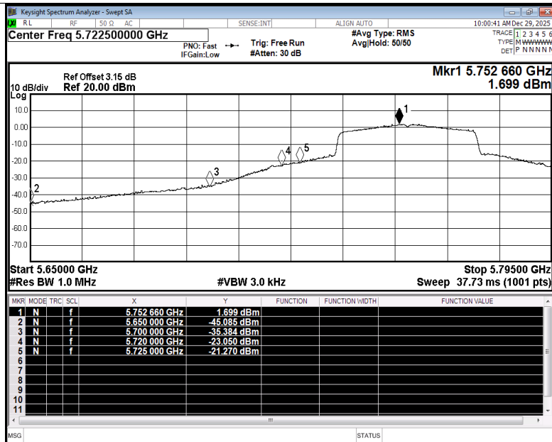
Restrict Band NVNT be40 5755MHz Ant3 Average
