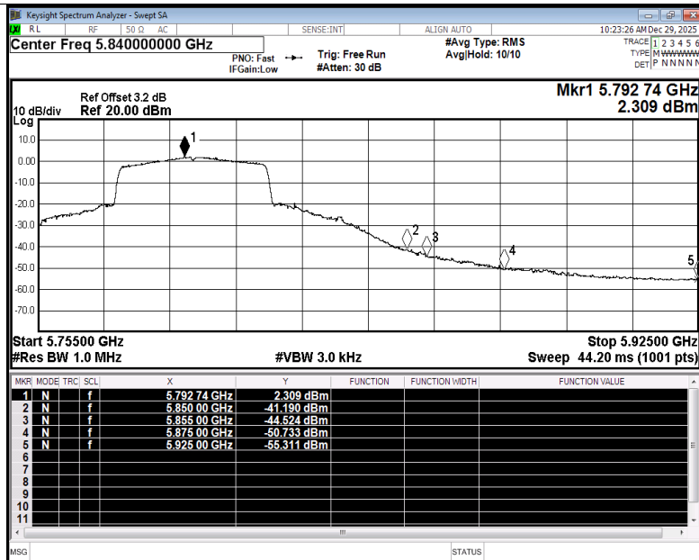
Restrict Band NVNT be40 5795MHz Ant4 Average
