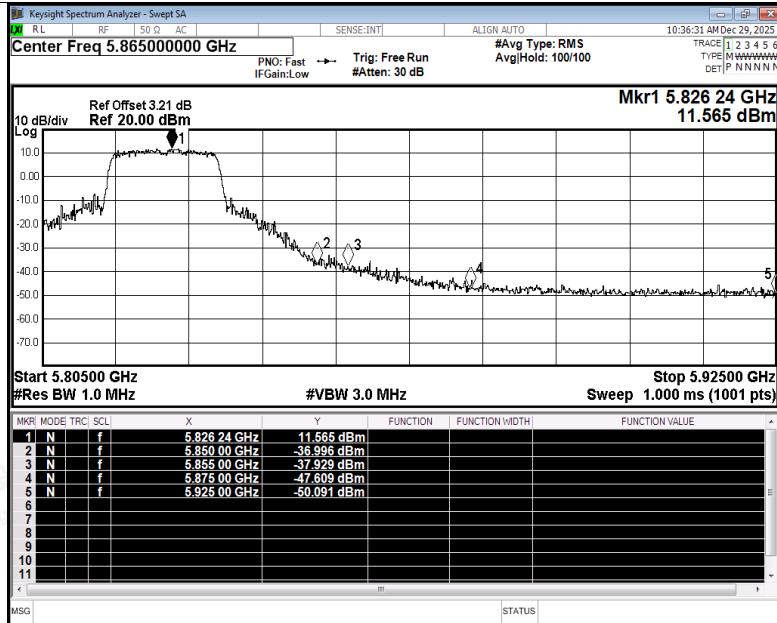
Restrict Band NVNT n20 5825MHz Ant5 Peak
