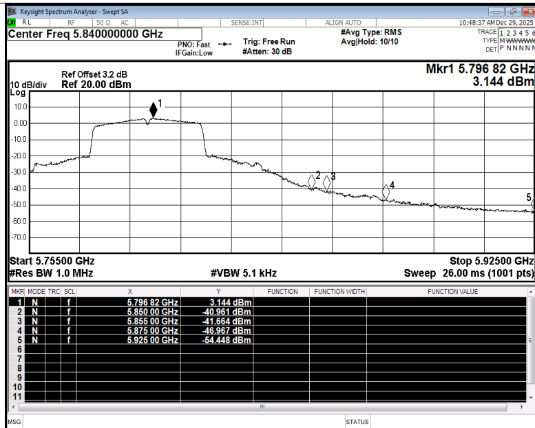
Restrict Band NVNT ac40 5795MHz Ant5 Average
