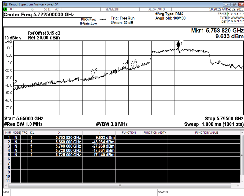
Restrict Band NVNT ac40 5755MHz Ant4 Peak
