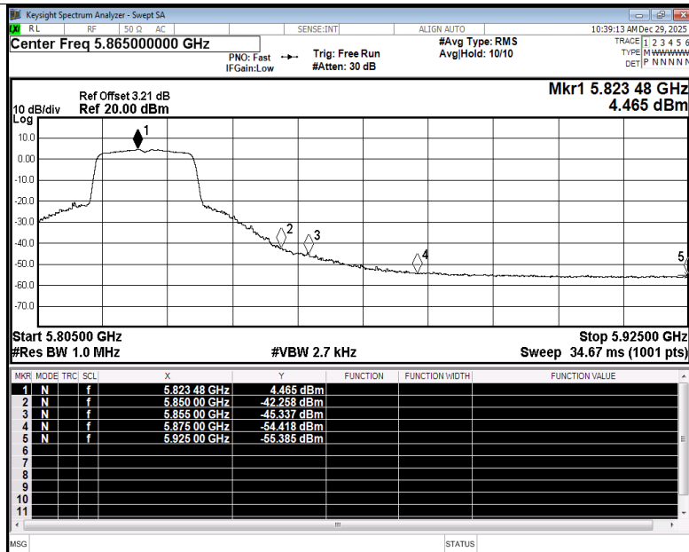
Restrict Band NVNT ac20 5825MHz Ant5 Average
