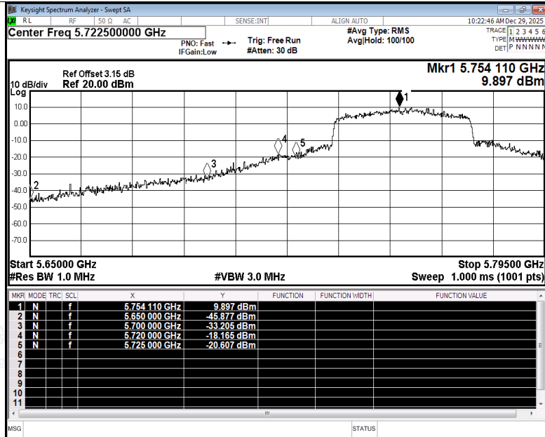
Restrict Band NVNT be40 5755MHz Ant4 Peak
