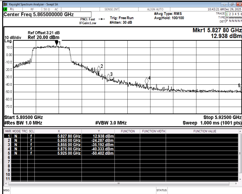
Restrict Band NVNT be20 5825MHz Ant5 Peak
