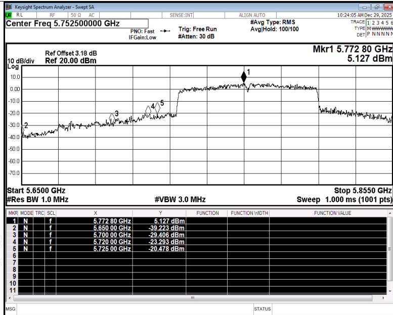
Restrict Band NVNT ac80 5775MHz Ant4 Peak
