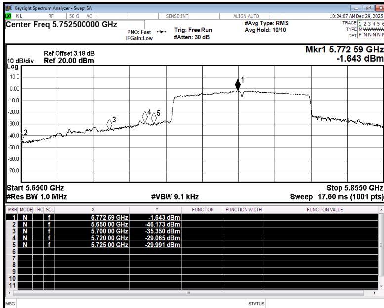
Restrict Band NVNT ac80 5775MHz Ant4 Average
