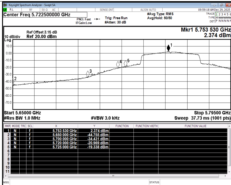
Restrict Band NVNT ax40 5755MHz Ant3 Average
