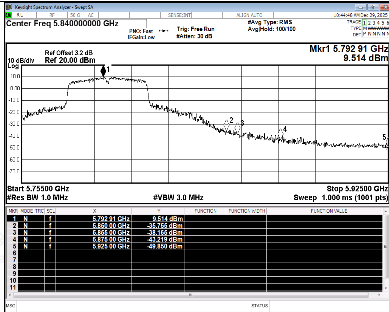
Restrict Band NVNT n40 5795MHz Ant5 Peak
