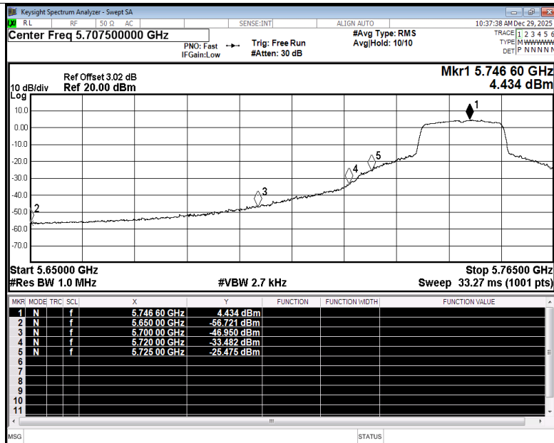
Restrict Band NVNT ac20 5745MHz Ant5 Average
