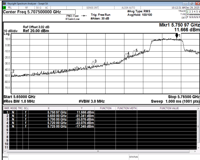
Restrict Band NVNT ax20 5745MHz Ant4 Peak
