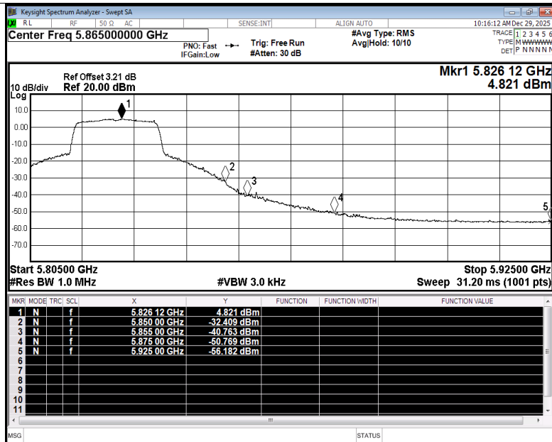
Restrict Band NVNT be20 5825MHz Ant4 Average
