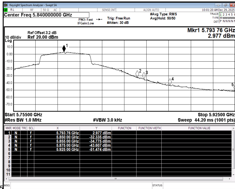
Restrict Band NVNT be40 5795MHz Ant3 Average
