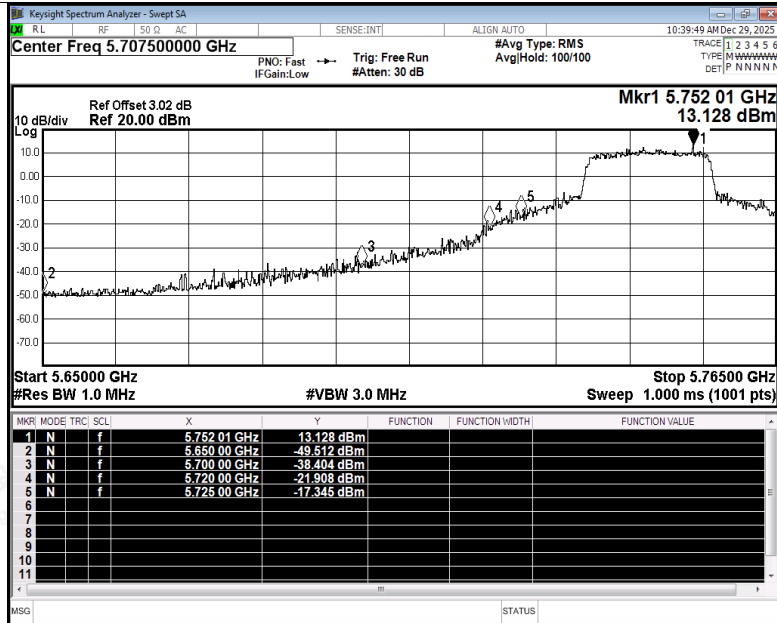
Restrict Band NVNT ax20 5745MHz Ant5 Peak
