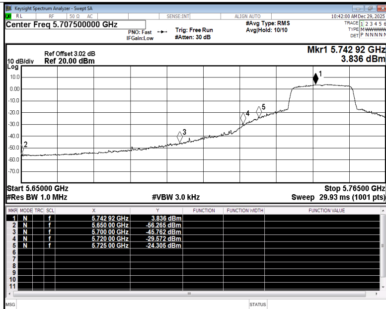
Restrict Band NVNT be20 5745MHz Ant5 Average
