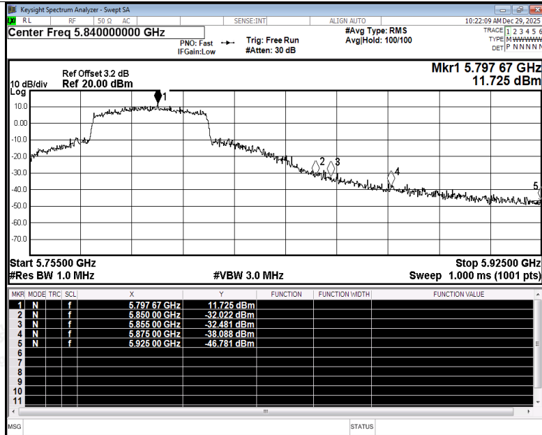
Restrict Band NVNT ax40 5795MHz Ant4 Peak
