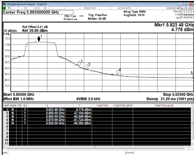
Restrict Band NVNT be20 5825MHz Ant5 Average
