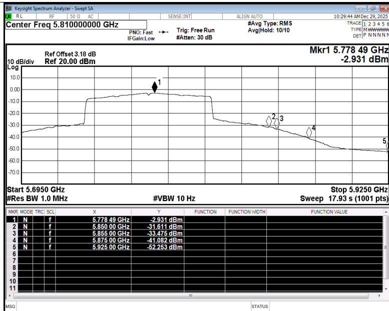
Restrict Band NVNT be80 5775MHz Ant4 Average
