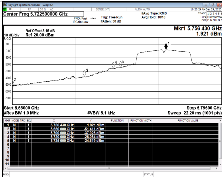
Restrict Band NVNT ac40 5755MHz Ant4 Average
