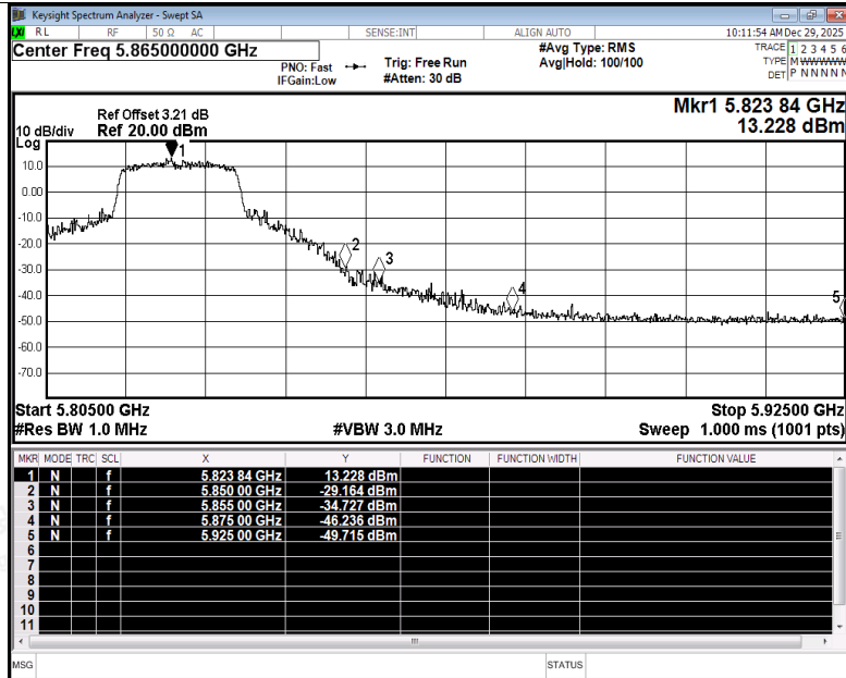
Restrict Band NVNT ac20 5825MHz Ant4 Peak
