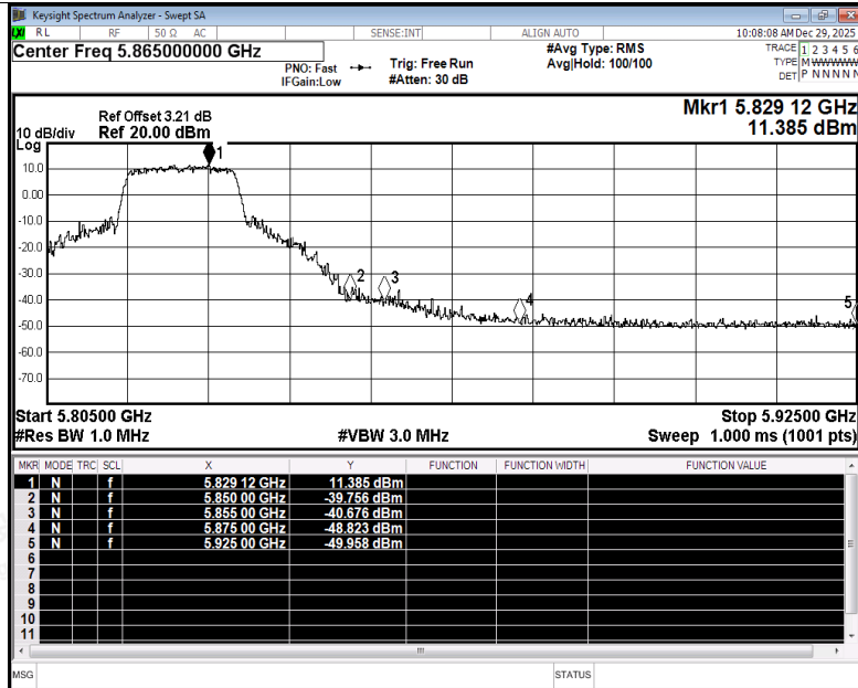
Restrict Band NVNT a 5825MHz Ant4 Peak
