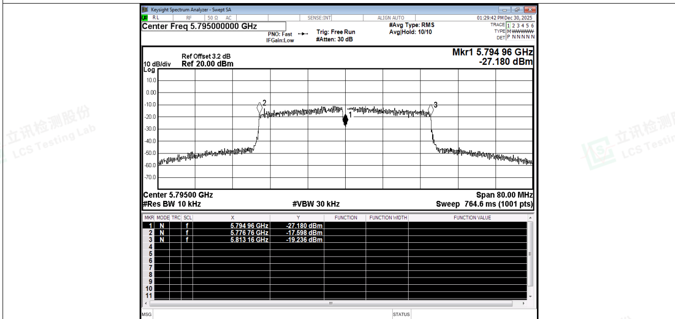
Freq. Stability NVNT n40 5795MHz Ant5
