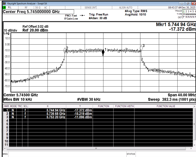
Freq. Stability NVNT a 5745MHz Ant1
