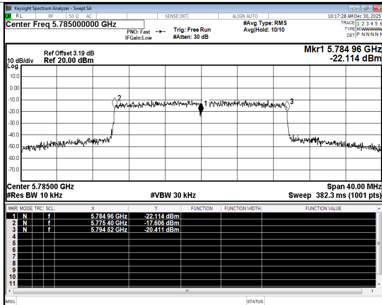
Freq. Stability NVNT ax20 5785MHz Ant2
