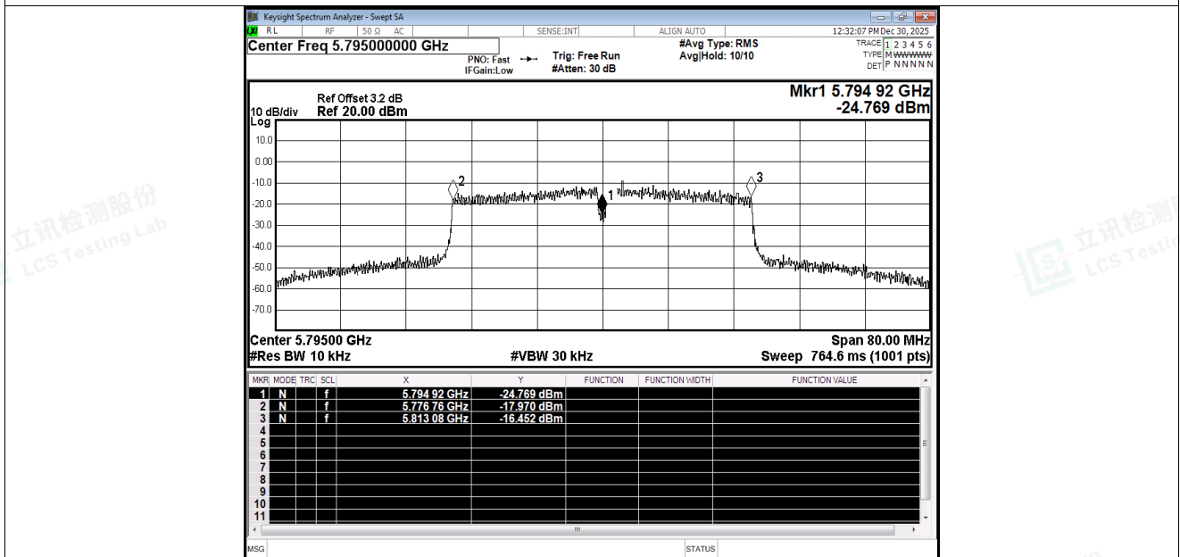
Freq. Stability NVNT n40 5795MHz Ant4
