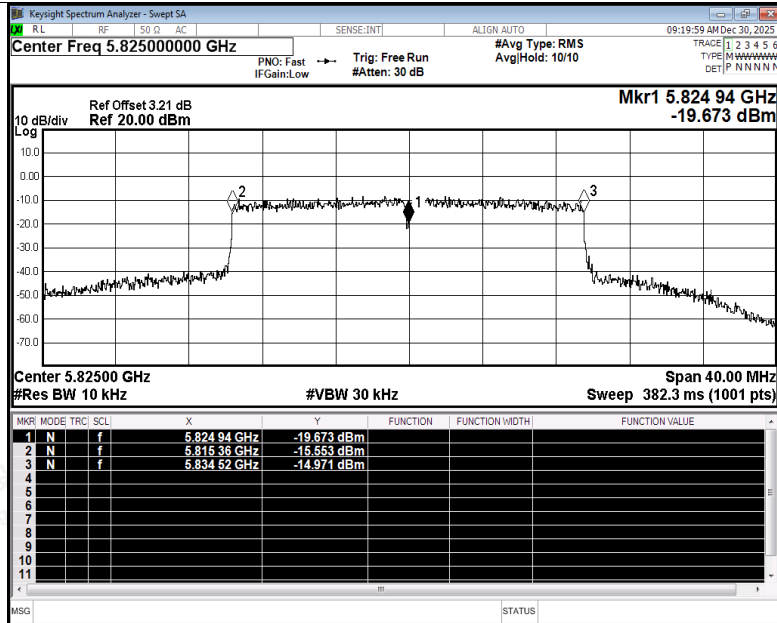
Freq. Stability NVNT be20 5825MHz Ant1
