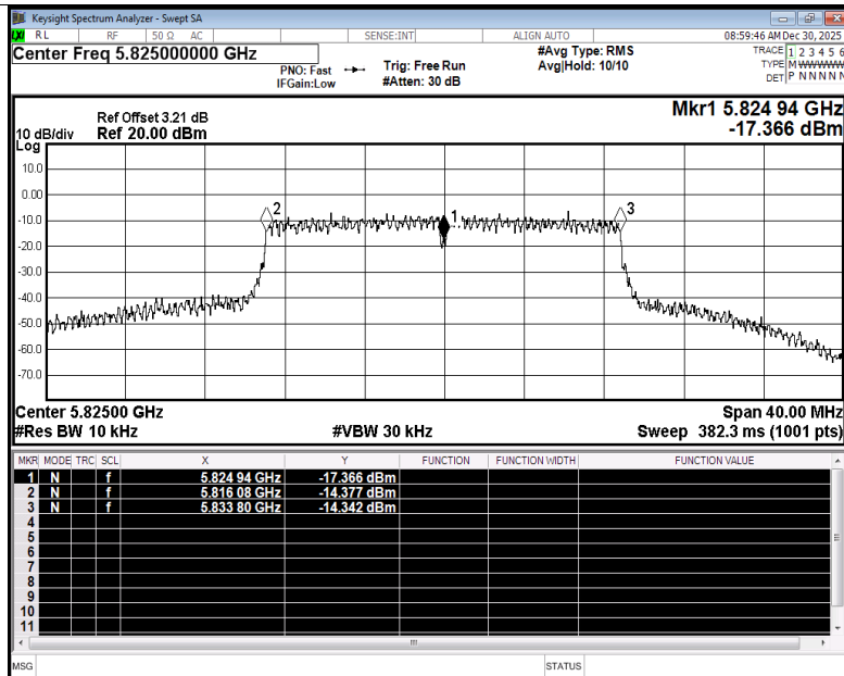
Freq. Stability NVNT n20 5825MHz Ant1
