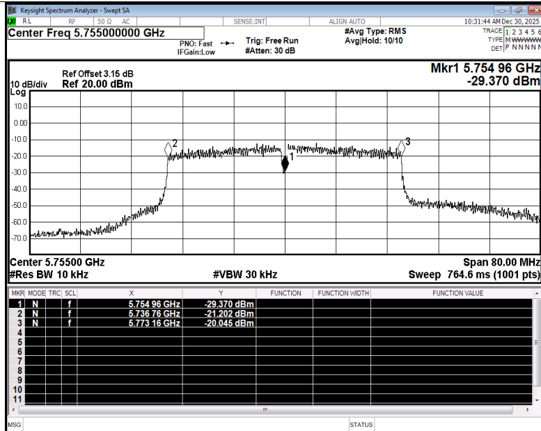
Freq. Stability NVNT ac40 5755MHz Ant2
