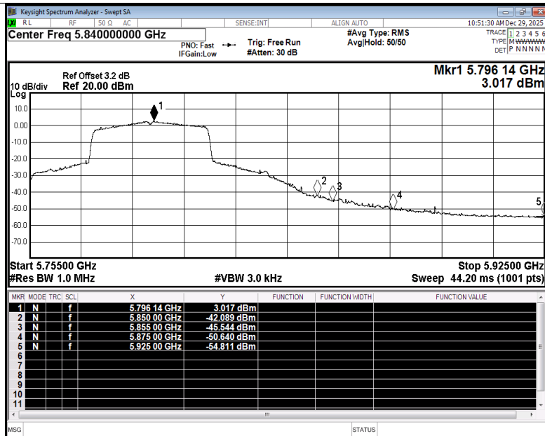
Restrict Band NVNT be40 5795MHz Ant5 Average
