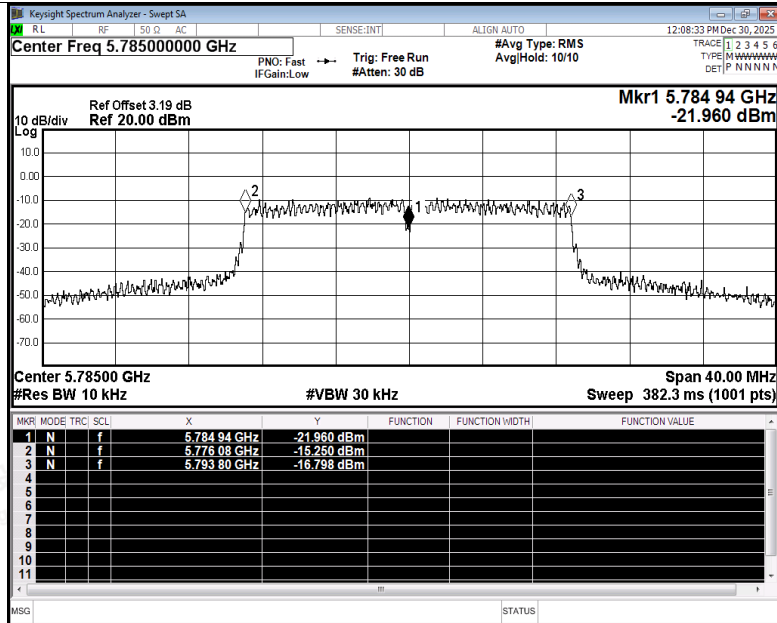
Freq. Stability NVNT n20 5785MHz Ant4
