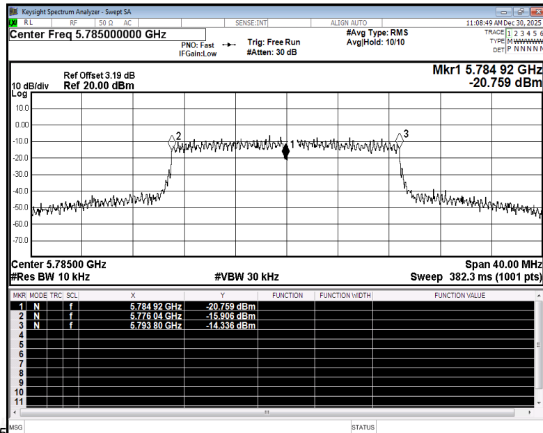
Freq. Stability NVNT ac20 5785MHz Ant3
