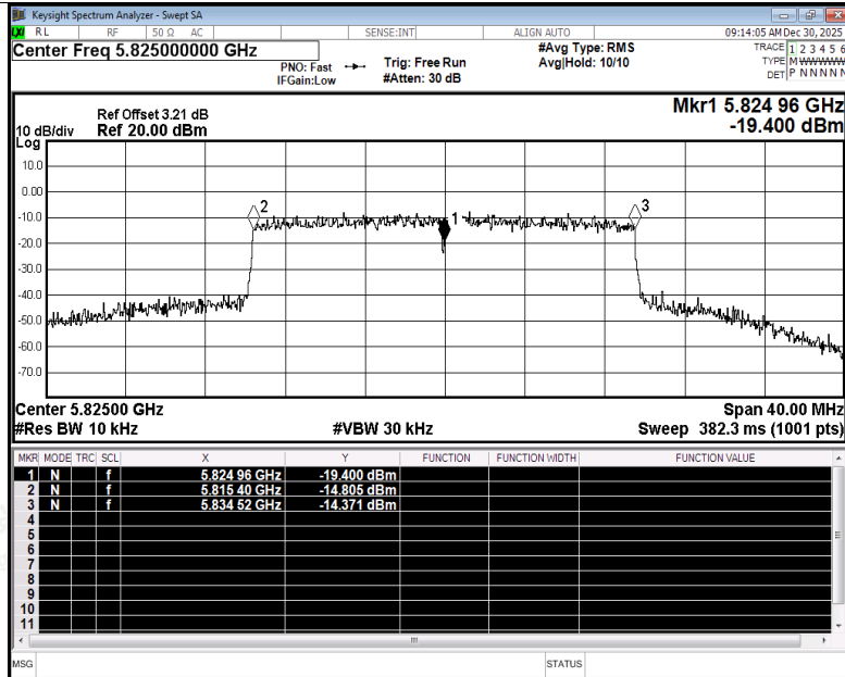
Freq. Stability NVNT ax20 5825MHz Ant1
