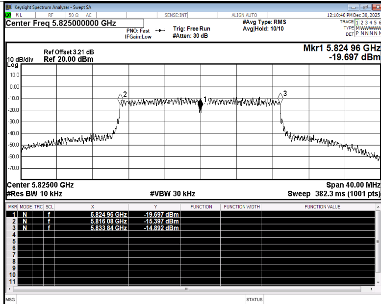
Freq. Stability NVNT n20 5825MHz Ant4
