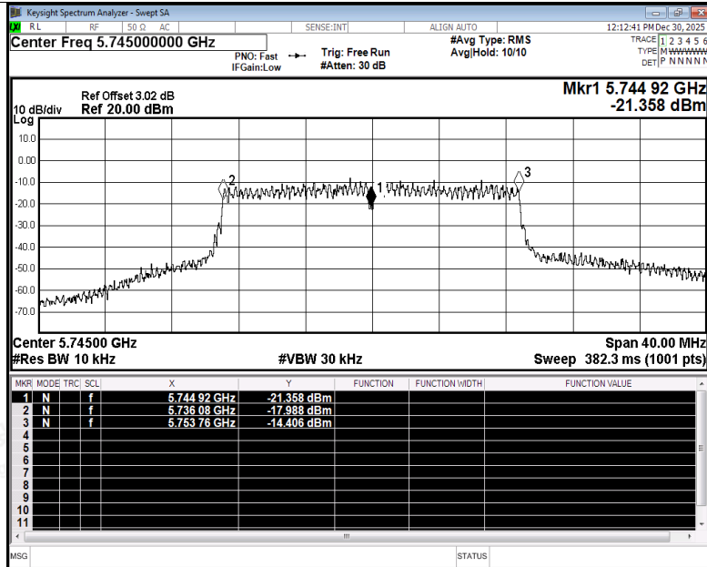
Freq. Stability NVNT ac20 5745MHz Ant4
