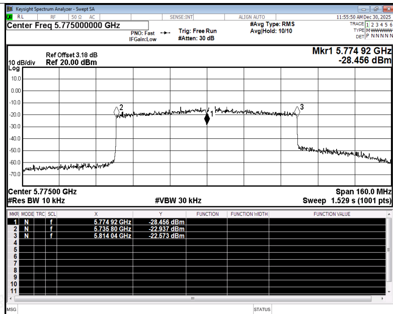
Freq. Stability NVNT be80 5775MHz Ant3
