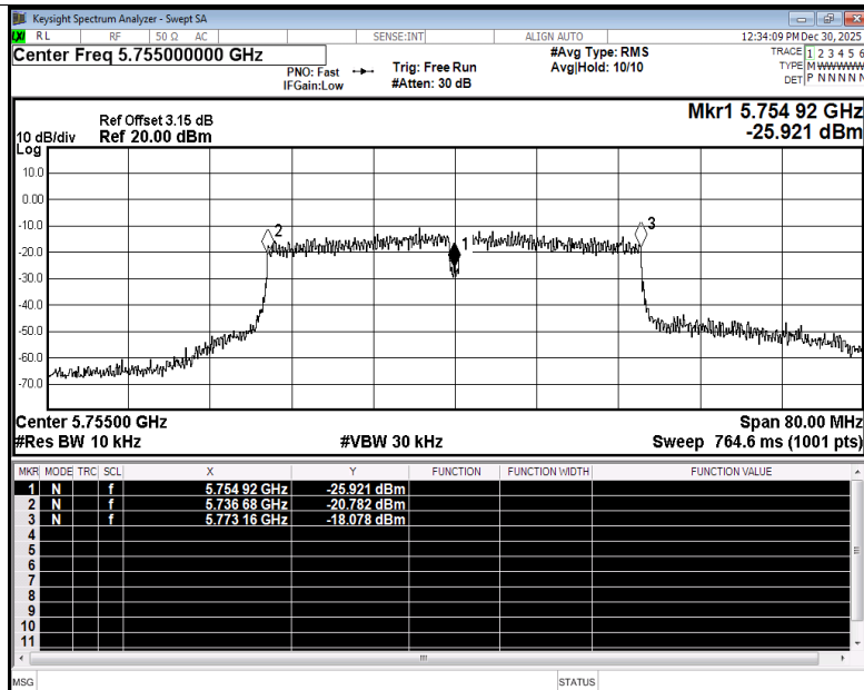
Freq. Stability NVNT ac40 5755MHz Ant4
