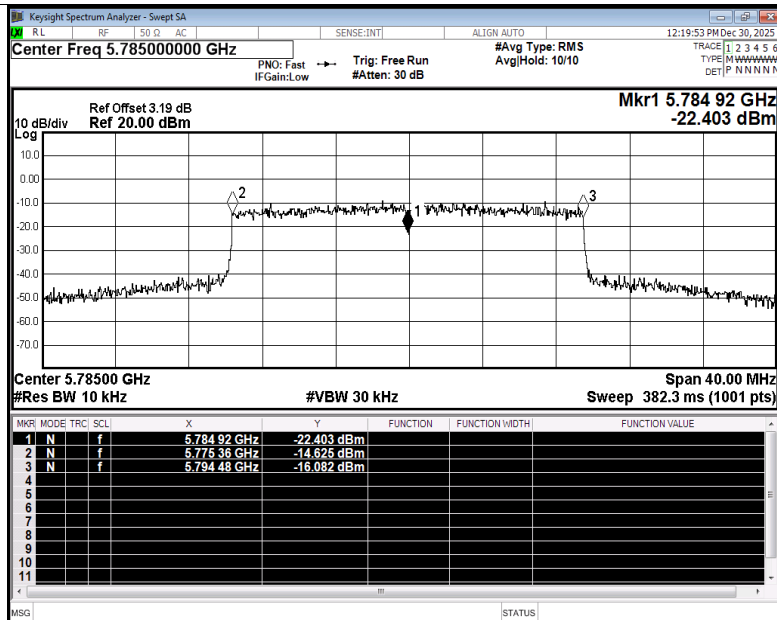
Freq. Stability NVNT ax20 5785MHz Ant4
