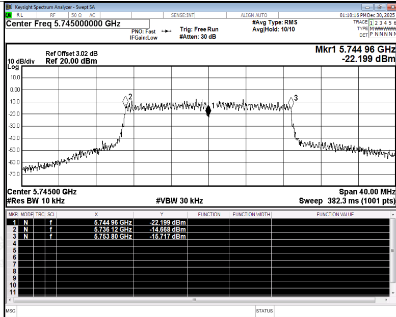
Freq. Stability NVNT ac20 5745MHz Ant5
