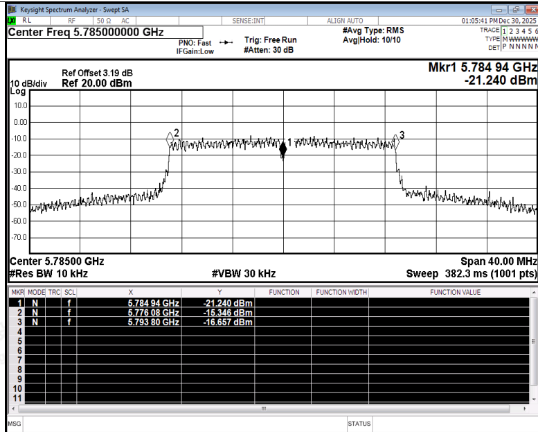
Freq. Stability NVNT n20 5785MHz Ant5
