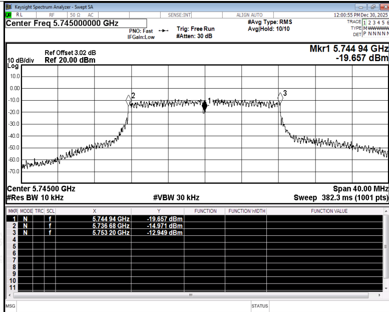
Freq. Stability NVNT a 5745MHz Ant4
