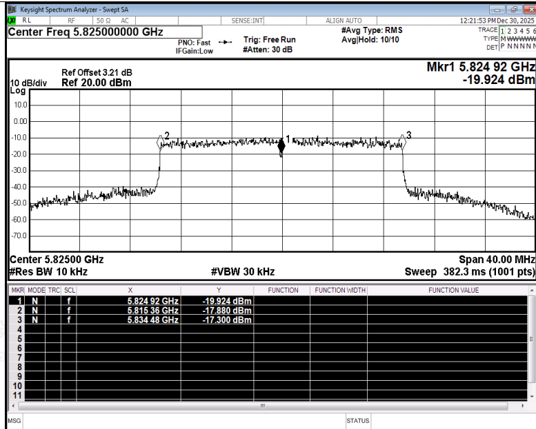
Freq. Stability NVNT ax20 5825MHz Ant4
