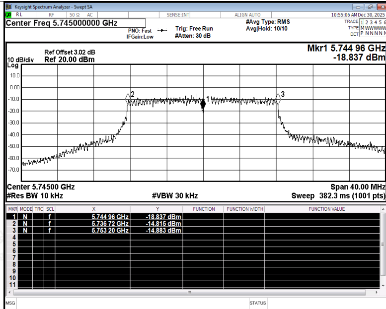
Freq. Stability NVNT a 5745MHz Ant3
