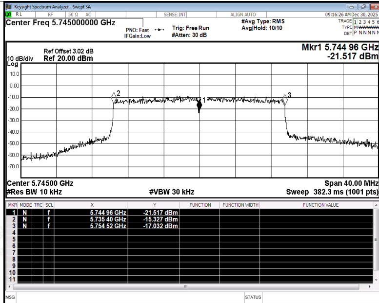
Freq. Stability NVNT be20 5745MHz Ant1
