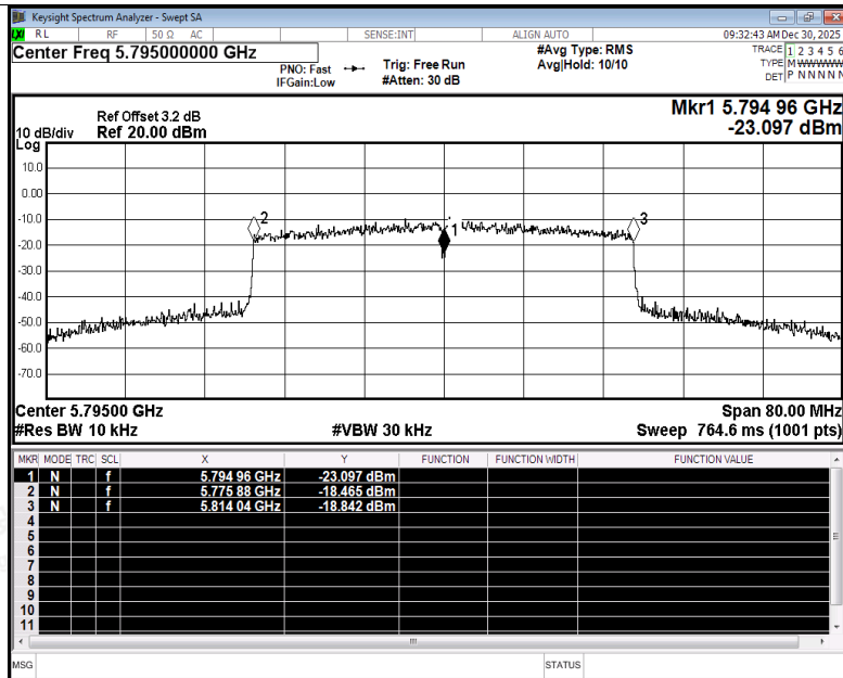
Freq. Stability NVNT ax40 5795MHz Ant1
