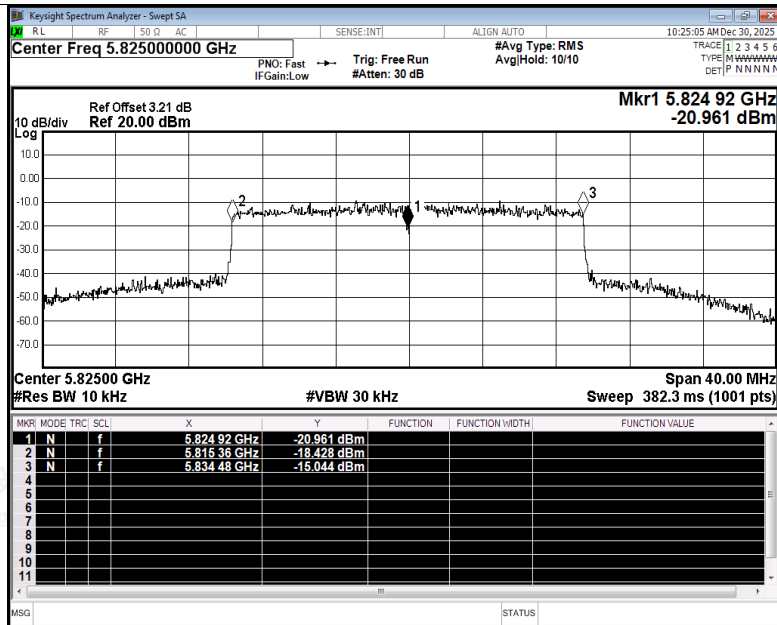
Freq. Stability NVNT be20 5825MHz Ant2
