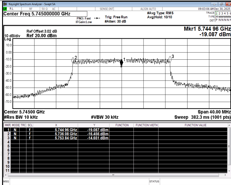
Freq. Stability NVNT ac20 5745MHz Ant1
