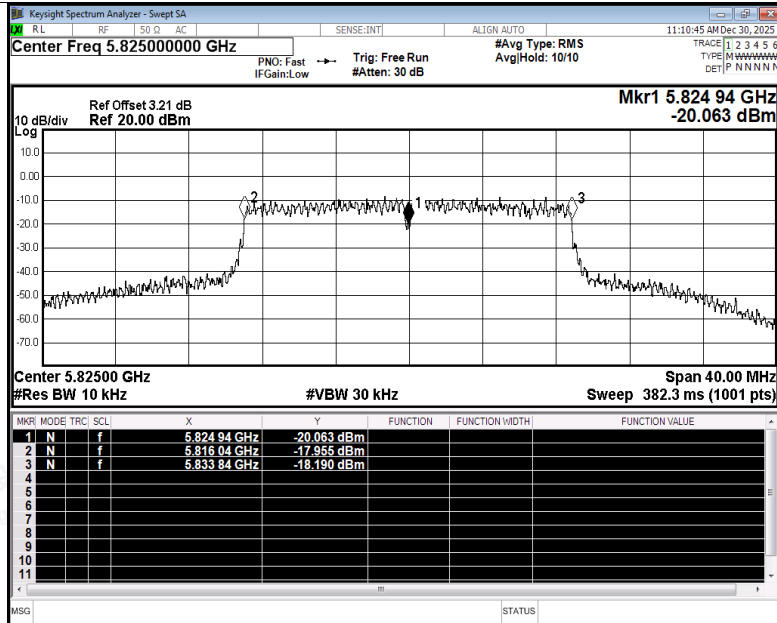
Freq. Stability NVNT ac20 5825MHz Ant3
