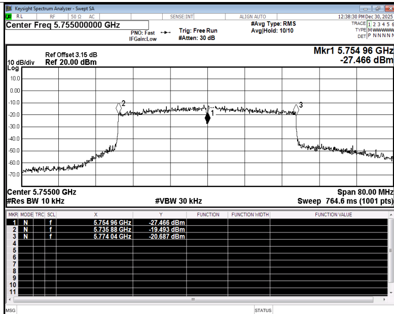
Freq. Stability NVNT ax40 5755MHz Ant4
