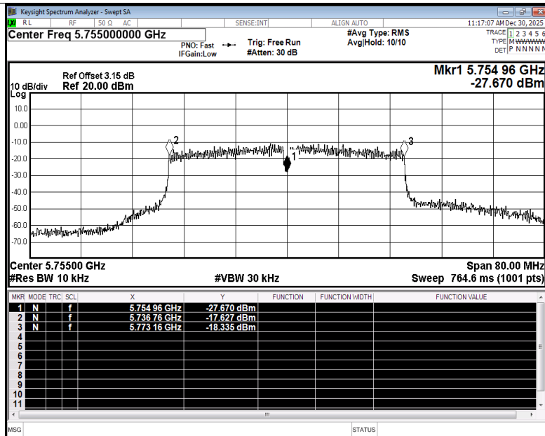
Freq. Stability NVNT ac40 5755MHz Ant3
