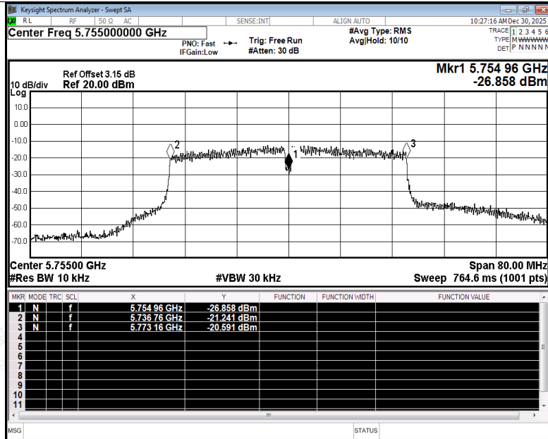
Freq. Stability NVNT n40 5755MHz Ant2
