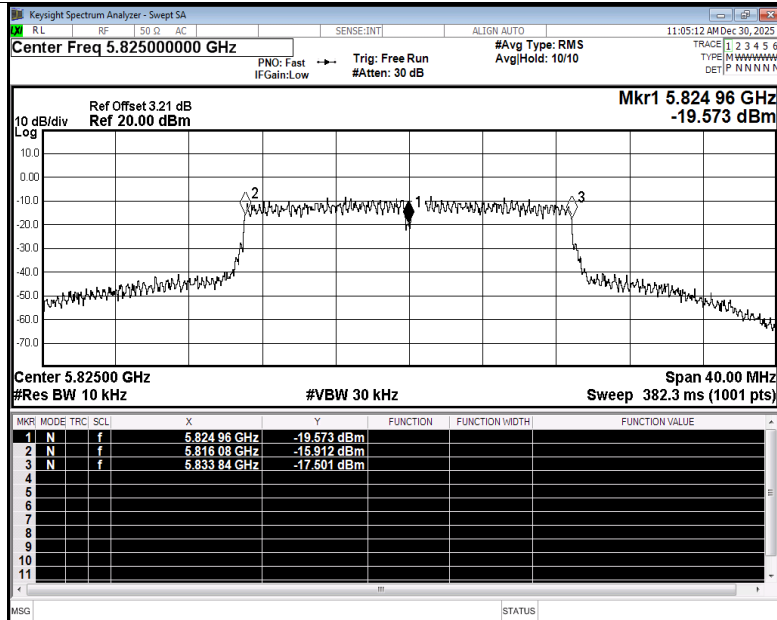
Freq. Stability NVNT n20 5825MHz Ant3
