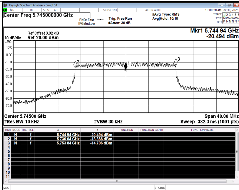
Freq. Stability NVNT n20 5745MHz Ant2
