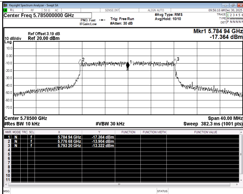
Freq. Stability NVNT a 5785MHz Ant2
