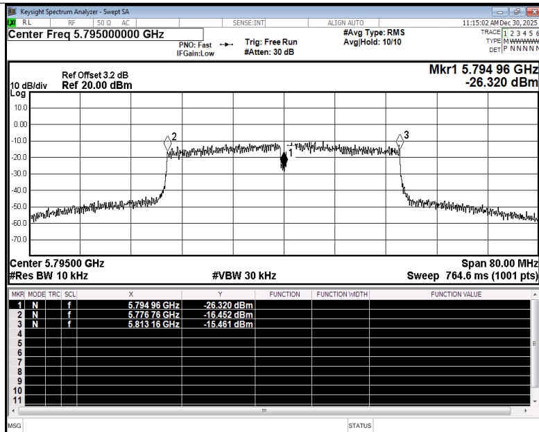
Freq. Stability NVNT n40 5795MHz Ant3
