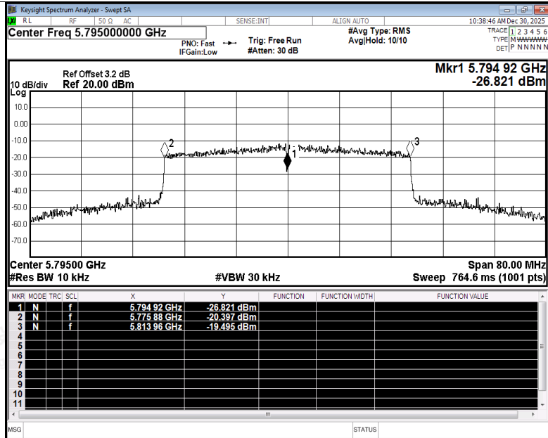
Freq. Stability NVNT ax40 5795MHz Ant2
