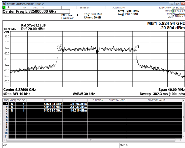
Freq. Stability NVNT ac20 5825MHz Ant4
