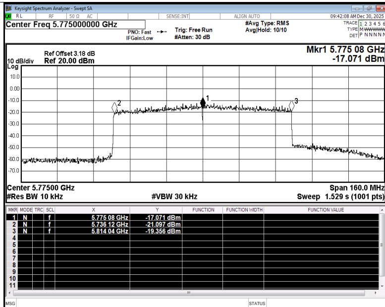
Freq. Stability NVNT ax80 5775MHz Ant1
