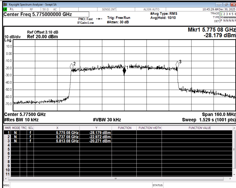
Freq. Stability NVNT ac80 5775MHz Ant2
