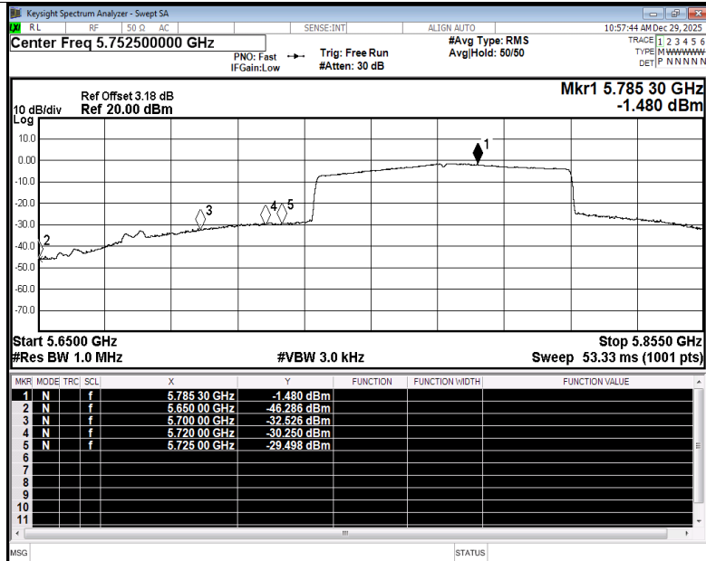
Restrict Band NVNT be80 5775MHz Ant5 Average
