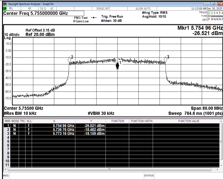
Freq. Stability NVNT n40 5755MHz Ant3
