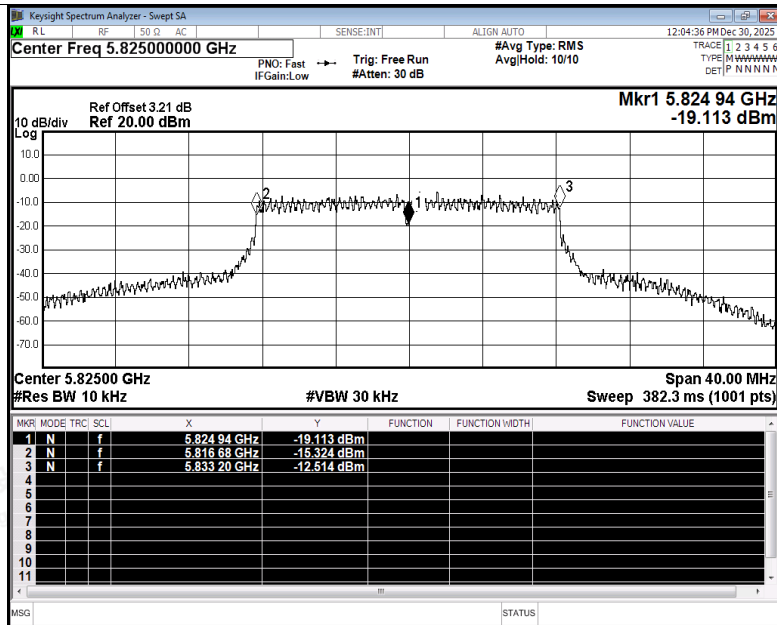
Freq. Stability NVNT a 5825MHz Ant4
