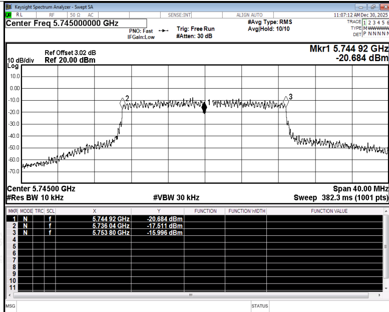
Freq. Stability NVNT ac20 5745MHz Ant3
