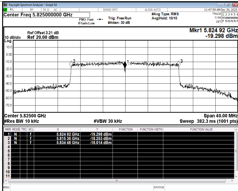
Freq. Stability NVNT be20 5825MHz Ant3
