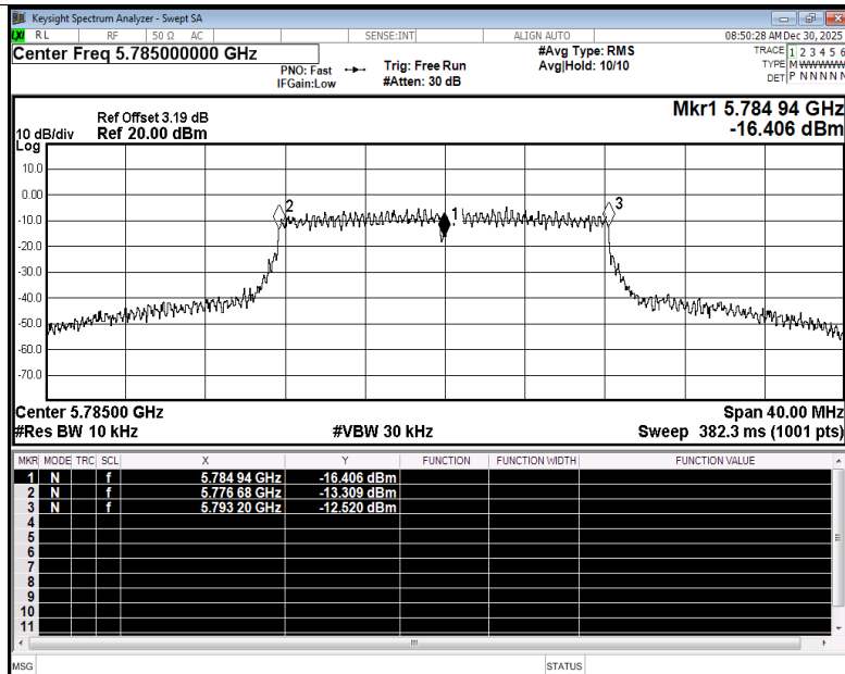
Freq. Stability NVNT a 5785MHz Ant1
