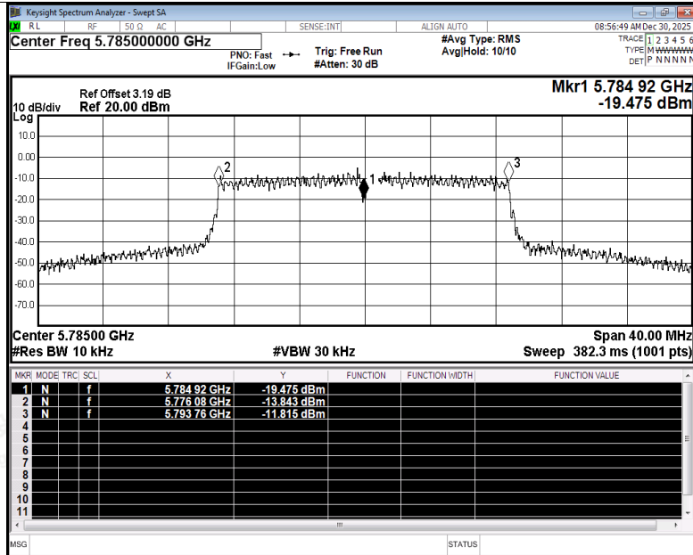
Freq. Stability NVNT n20 5785MHz Ant1
