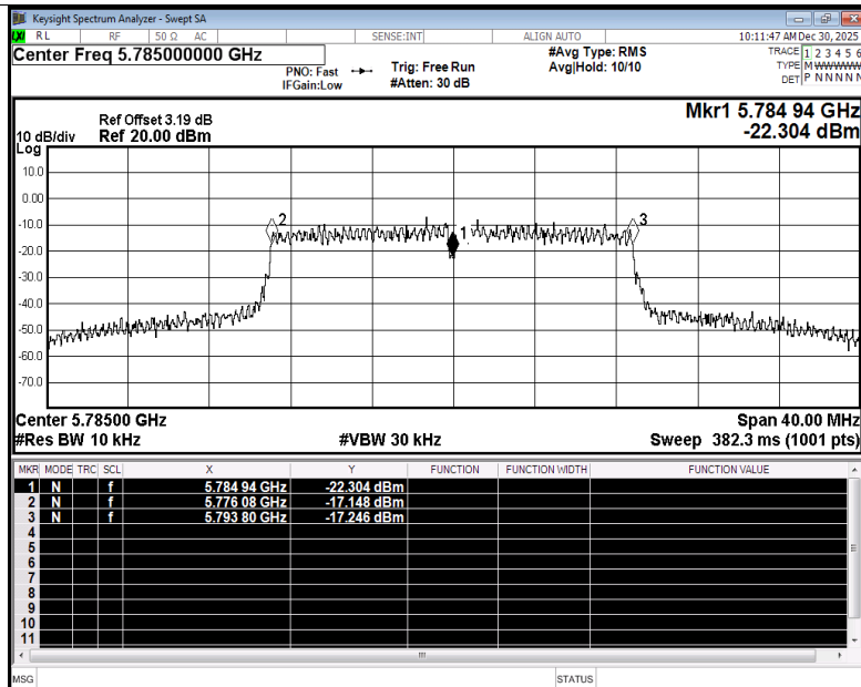
Freq. Stability NVNT ac20 5785MHz Ant2
