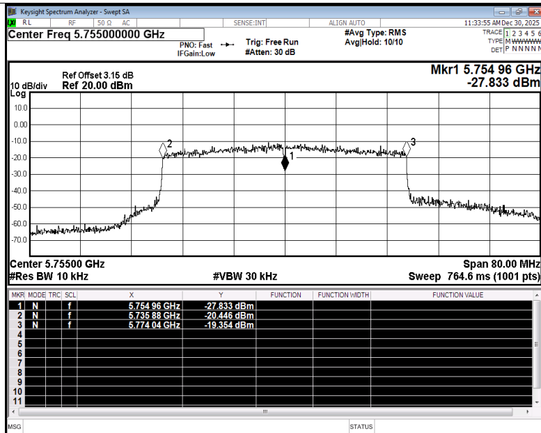
Freq. Stability NVNT be40 5755MHz Ant3
