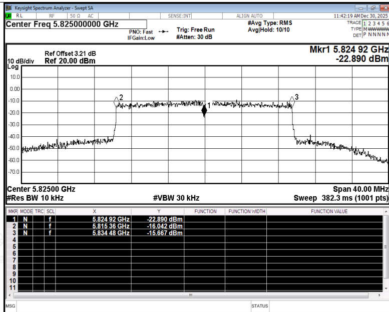
Freq. Stability NVNT ax20 5825MHz Ant3
