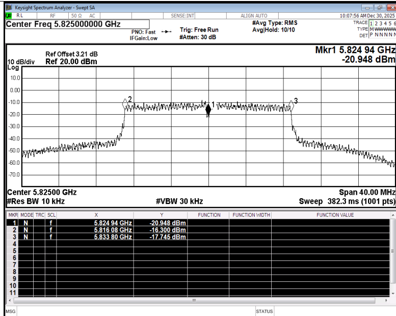
Freq. Stability NVNT n20 5825MHz Ant2
