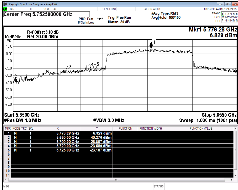
Restrict Band NVNT be80 5775MHz Ant5 Peak
