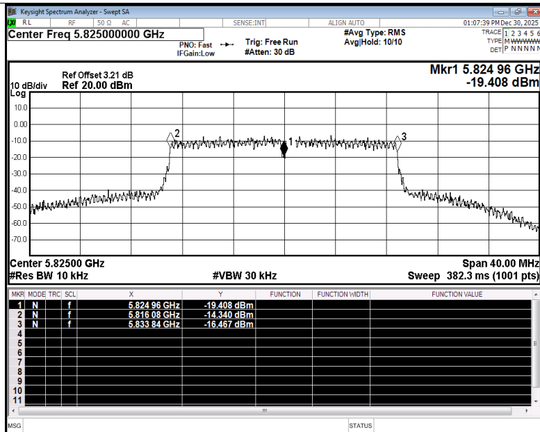
Freq. Stability NVNT n20 5825MHz Ant5
