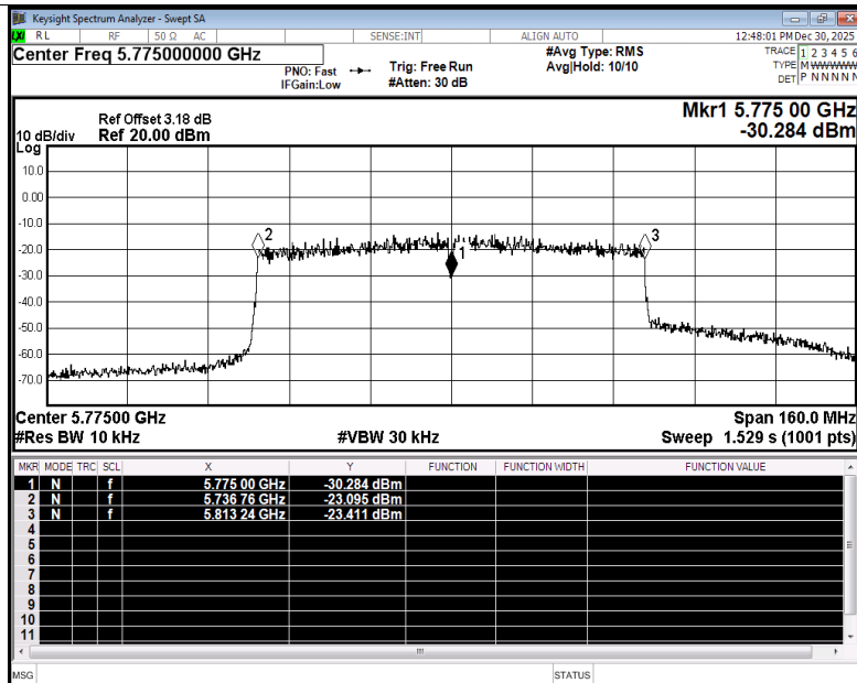
Freq. Stability NVNT ac80 5775MHz Ant4
