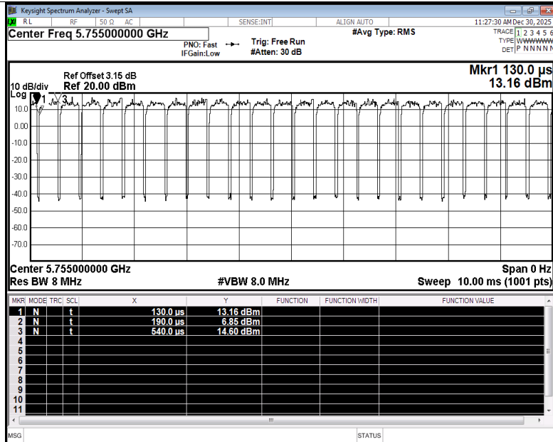
Duty Cycle NVNT ax40 5755MHz Ant3
