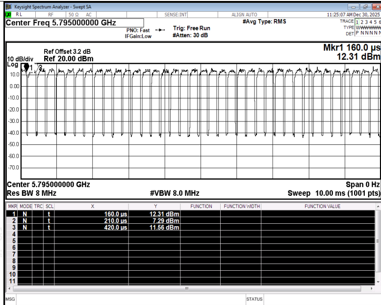
Duty Cycle NVNT ac40 5795MHz Ant3
