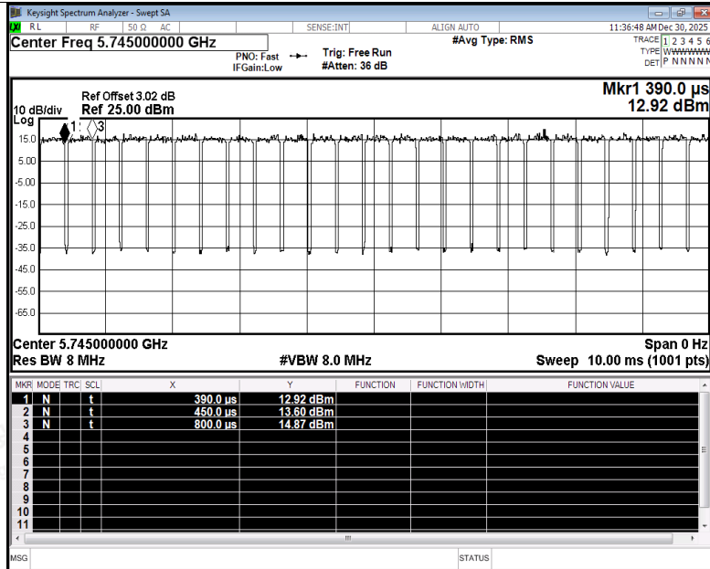
Duty Cycle NVNT ax20 5745MHz Ant3
