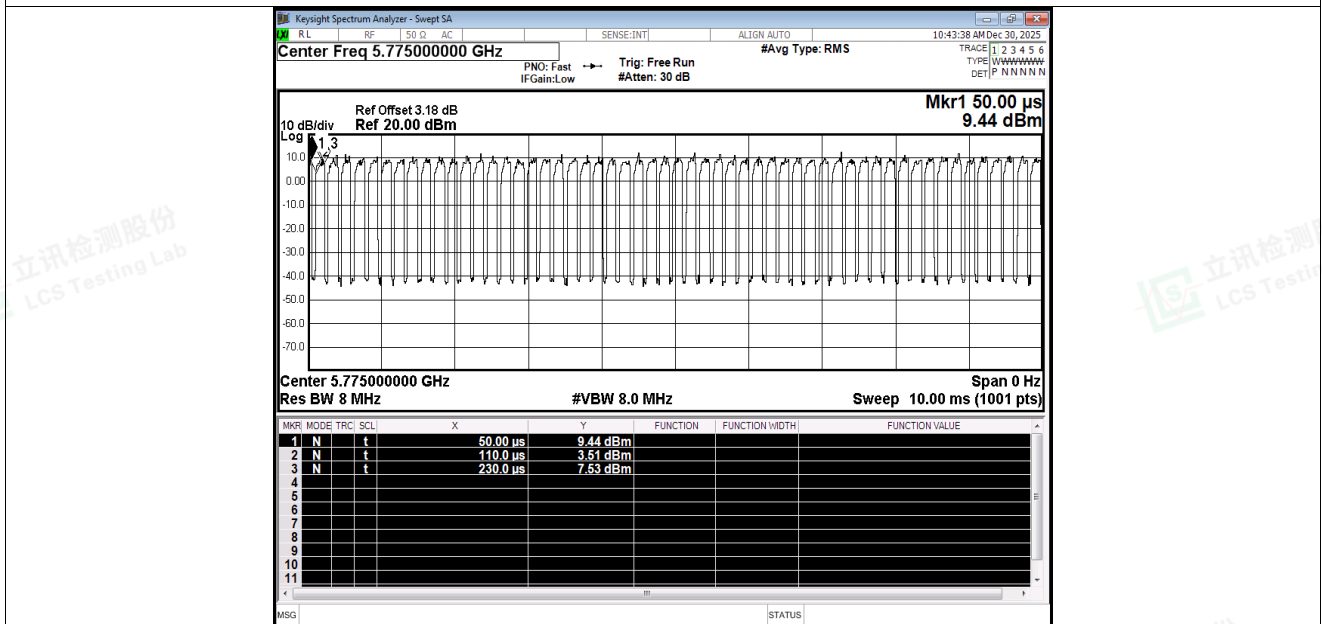
Duty Cycle NVNT ac80 5775MHz Ant2
