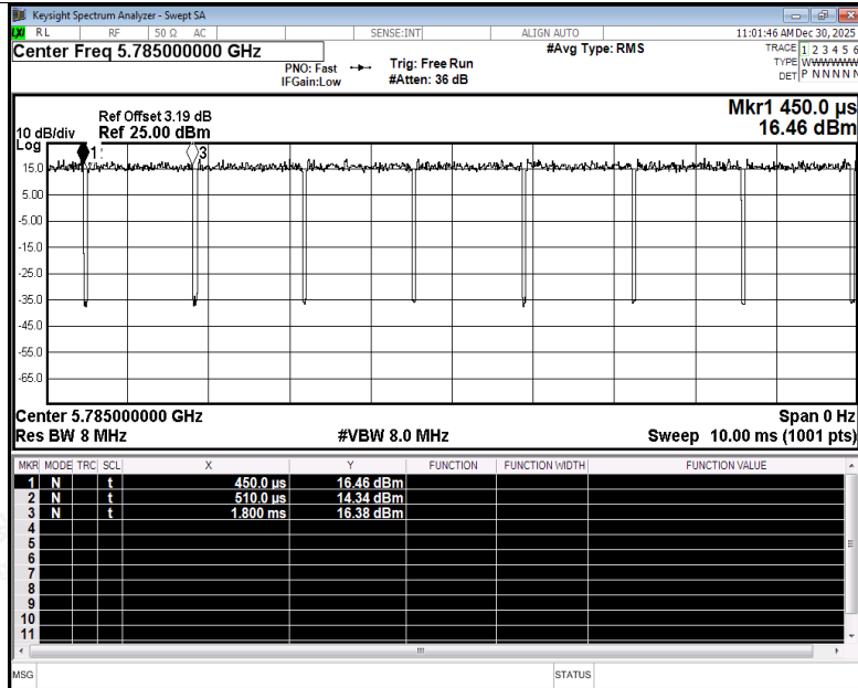
Duty Cycle NVNT n20 5785MHz Ant3
