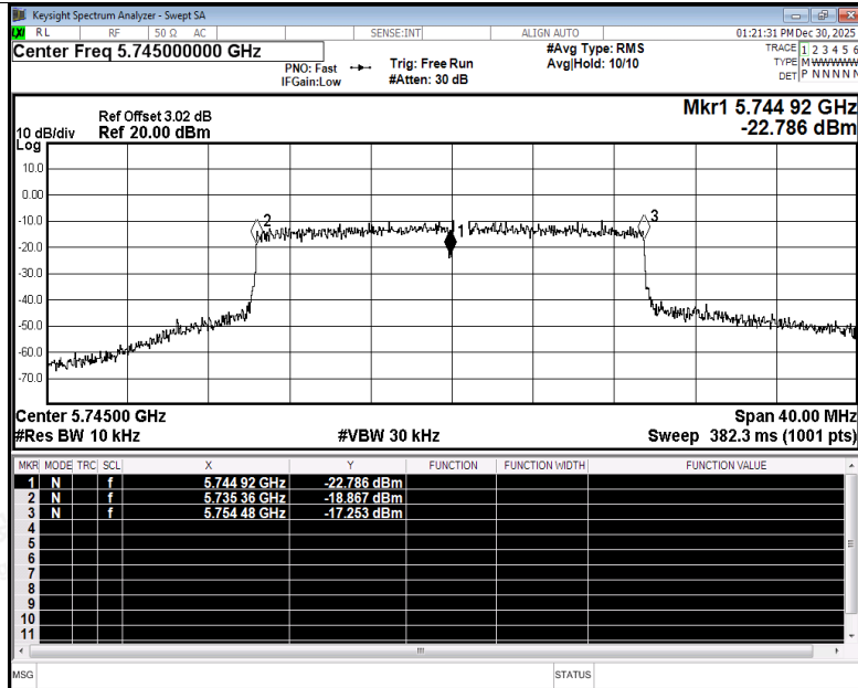
Freq. Stability NVNT be20 5745MHz Ant5
