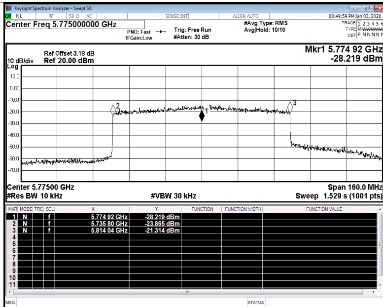
Freq. Stability NVNT be80 5775MHz Ant5
