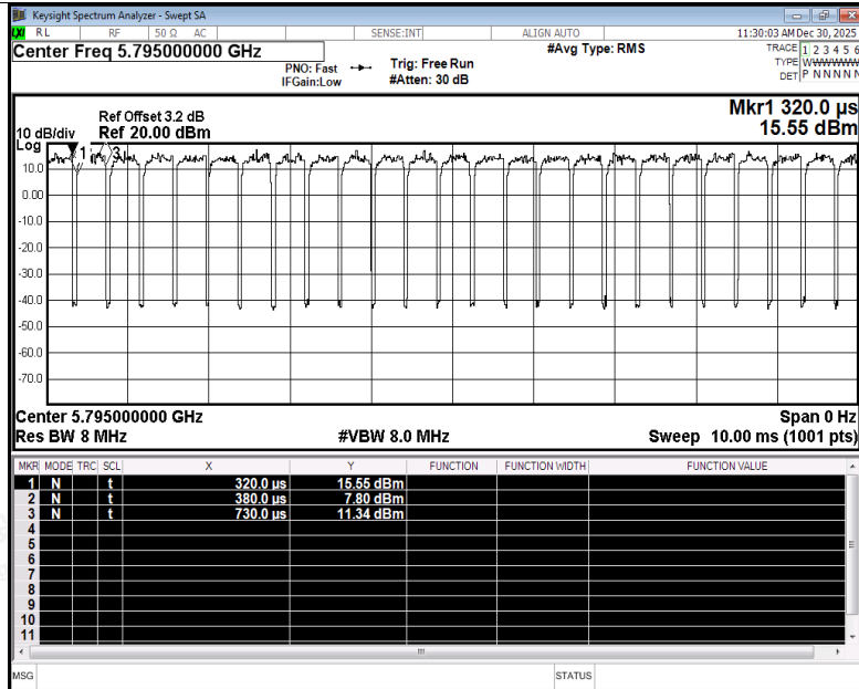
Duty Cycle NVNT ax40 5795MHz Ant3
