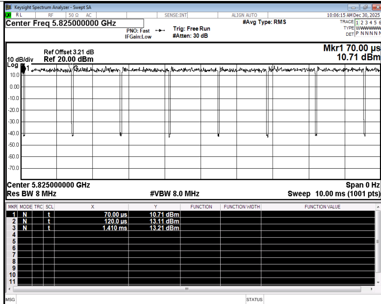
Duty Cycle NVNT n20 5825MHz Ant2
