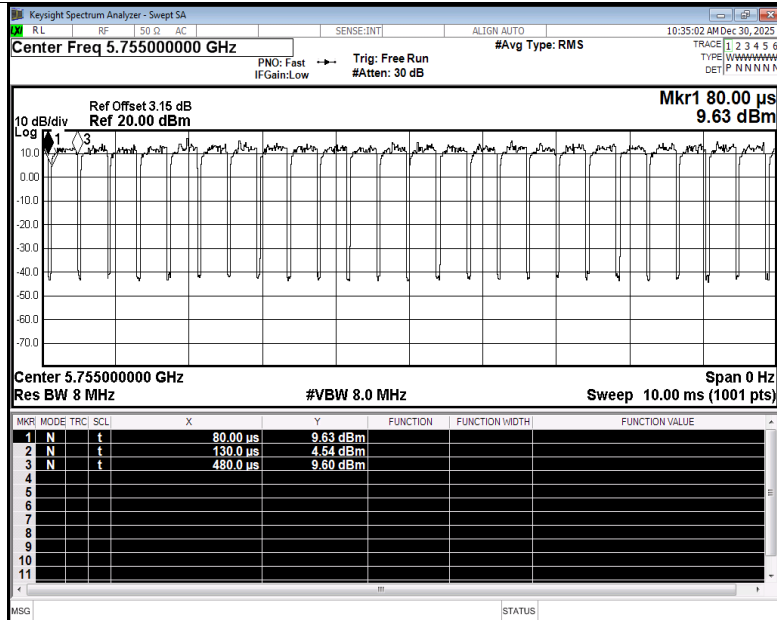
Duty Cycle NVNT ax40 5755MHz Ant2
