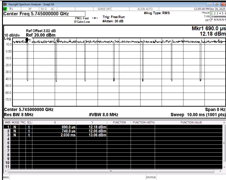
Duty Cycle NVNT n20 5745MHz Ant4
