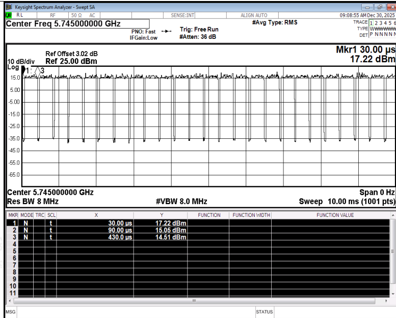
Duty Cycle NVNT ax20 5745MHz Ant1
