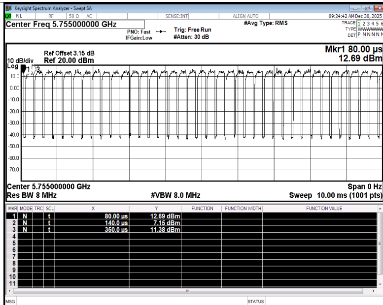
Duty Cycle NVNT ac40 5755MHz Ant1
