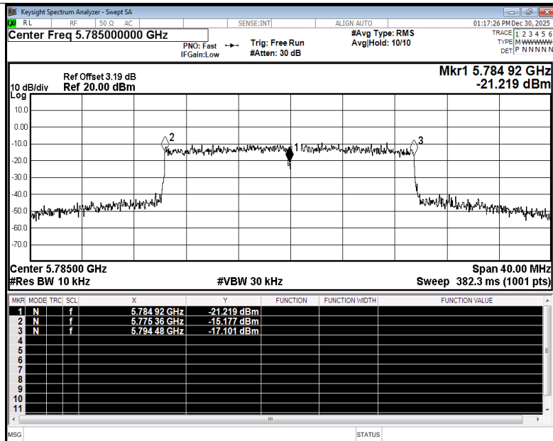
Freq. Stability NVNT ax20 5785MHz Ant5
