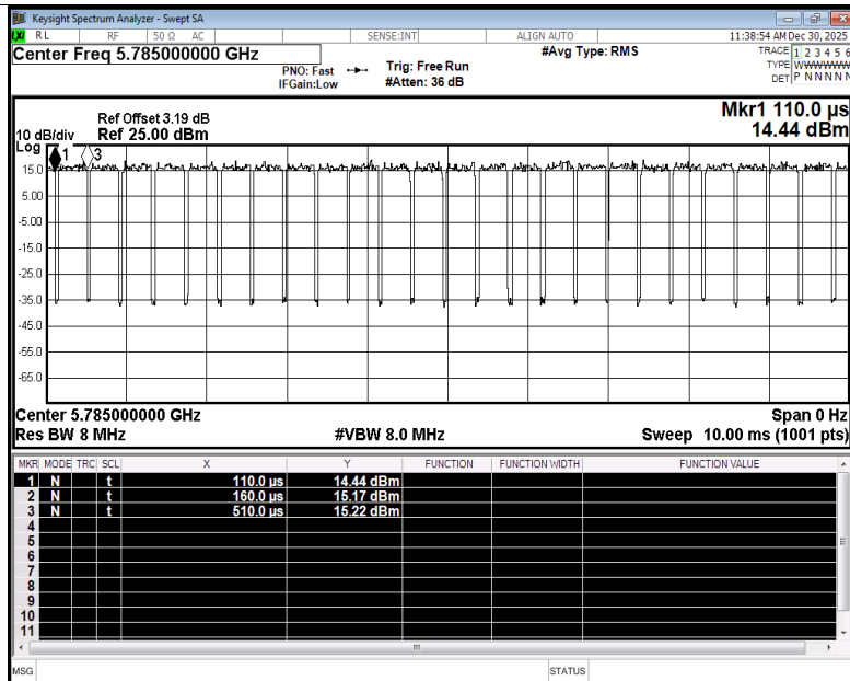
Duty Cycle NVNT ax20 5785MHz Ant3
