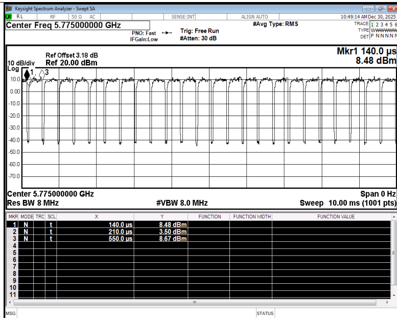
Duty Cycle NVNT be80 5775MHz Ant2
