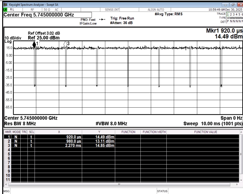
Duty Cycle NVNT n20 5745MHz Ant3
