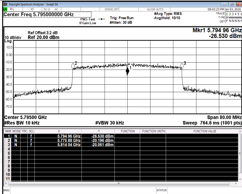
Freq. Stability NVNT be40 5795MHz Ant5
