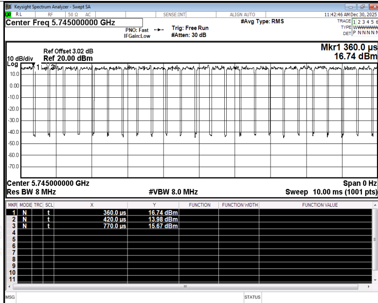
Duty Cycle NVNT be20 5745MHz Ant3
