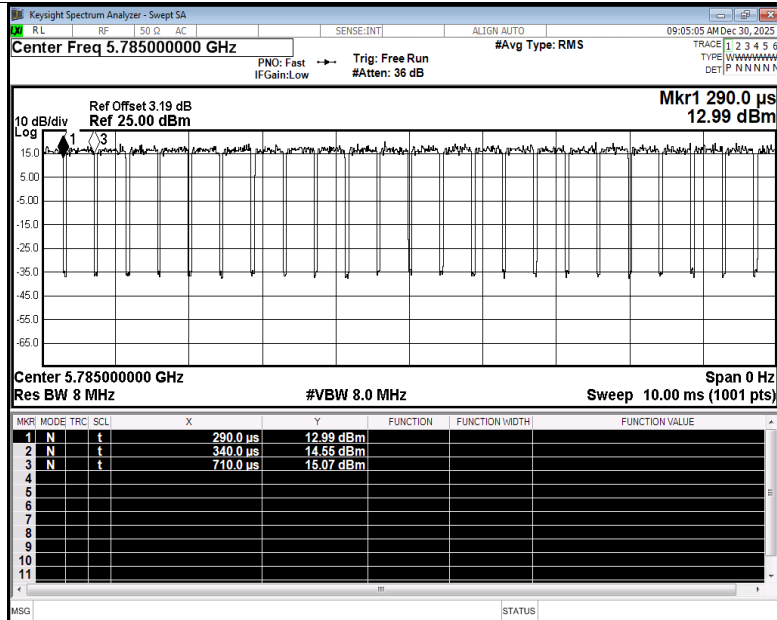
Duty Cycle NVNT ac20 5785MHz Ant1
