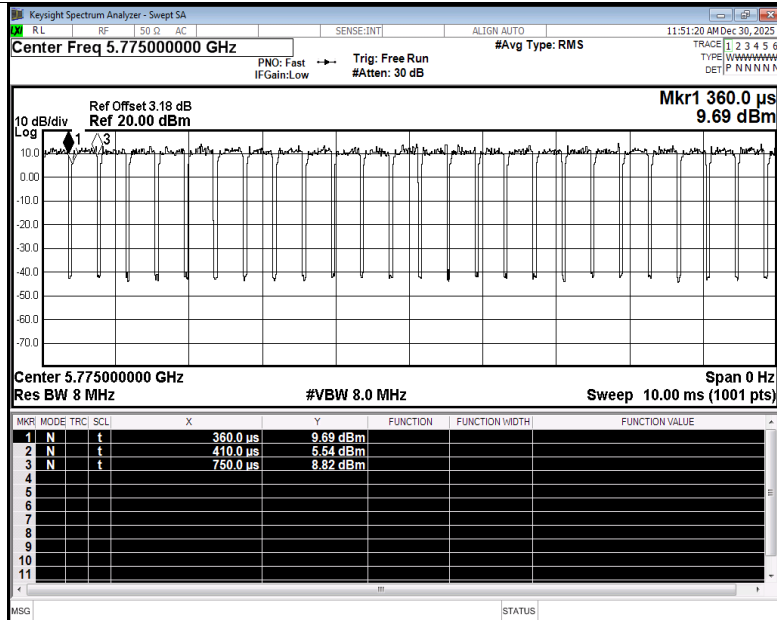
Duty Cycle NVNT ax80 5775MHz Ant3
