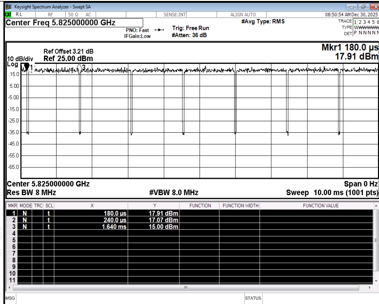
Duty Cycle NVNT a 5825MHz Ant1
