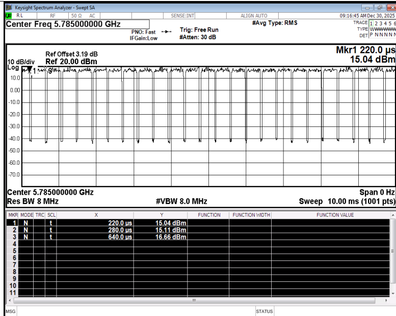
Duty Cycle NVNT be20 5785MHz Ant1
