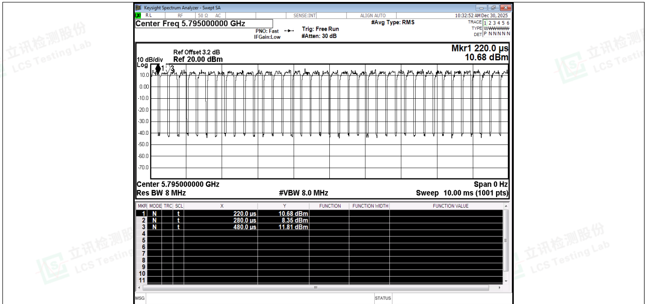
Duty Cycle NVNT ac40 5795MHz Ant2
