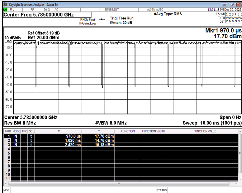
Duty Cycle NVNT a 5785MHz Ant4
