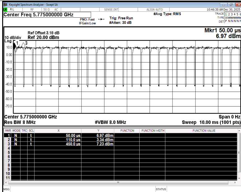
Duty Cycle NVNT ax80 5775MHz Ant2
