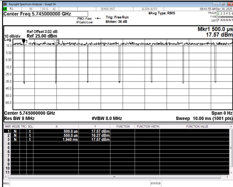
Duty Cycle NVNT a 5745MHz Ant1
