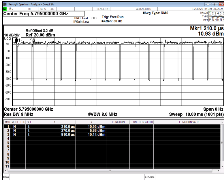
Duty Cycle NVNT n40 5795MHz Ant4
