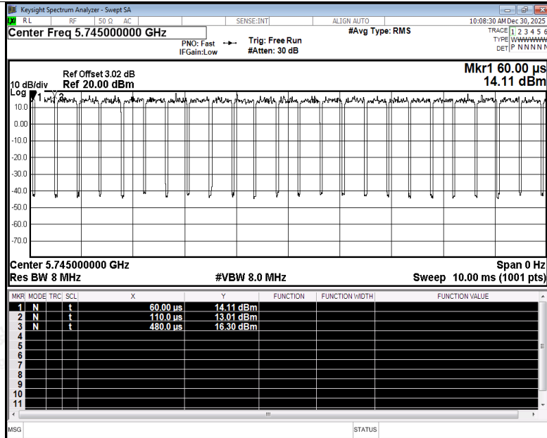
Duty Cycle NVNT ac20 5745MHz Ant2
