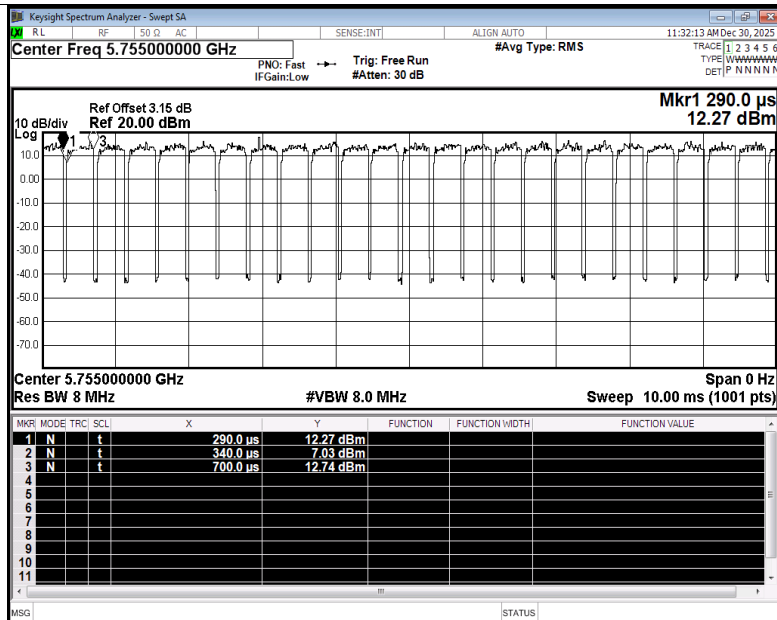
Duty Cycle NVNT be40 5755MHz Ant3
