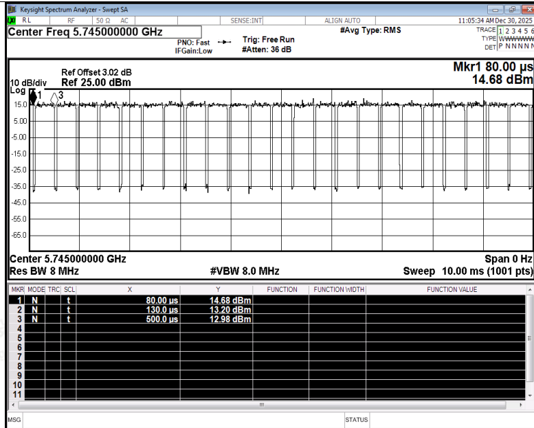
Duty Cycle NVNT ac20 5745MHz Ant3
