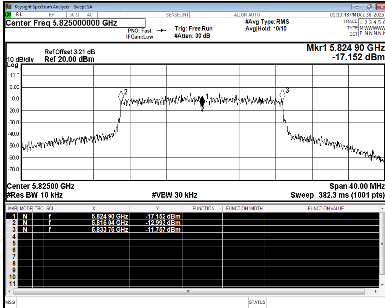
Freq. Stability NVNT ac20 5825MHz Ant5
