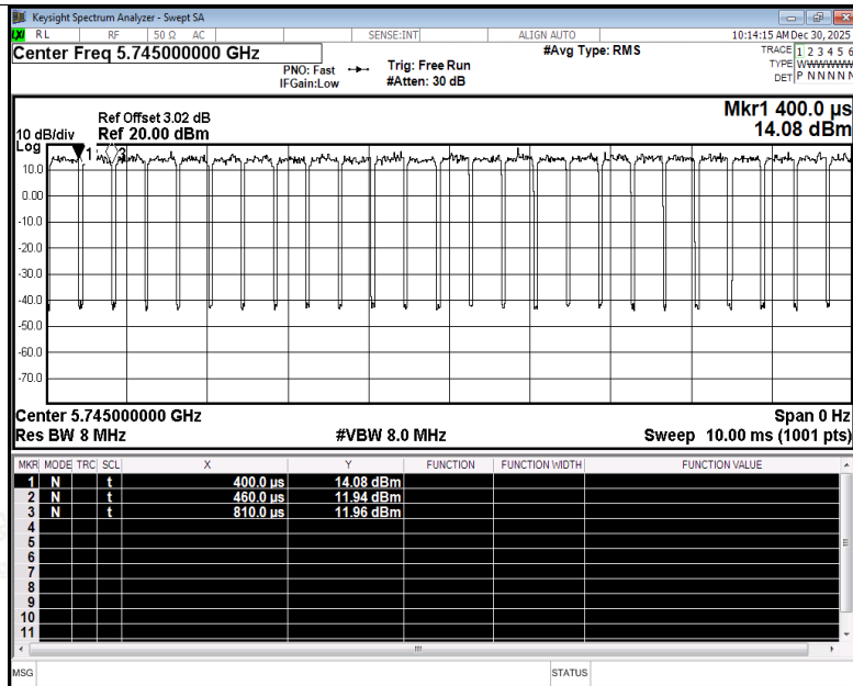
Duty Cycle NVNT ax20 5745MHz Ant2
