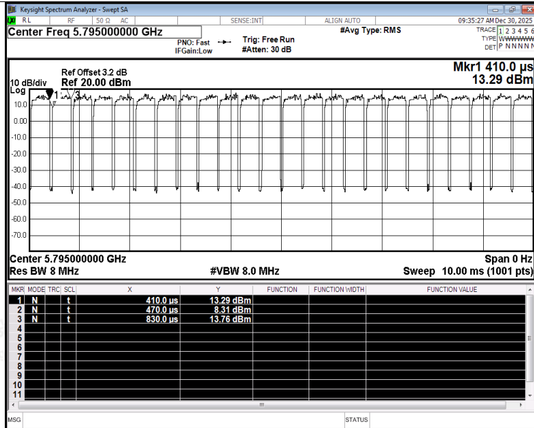
Duty Cycle NVNT be40 5795MHz Ant1
