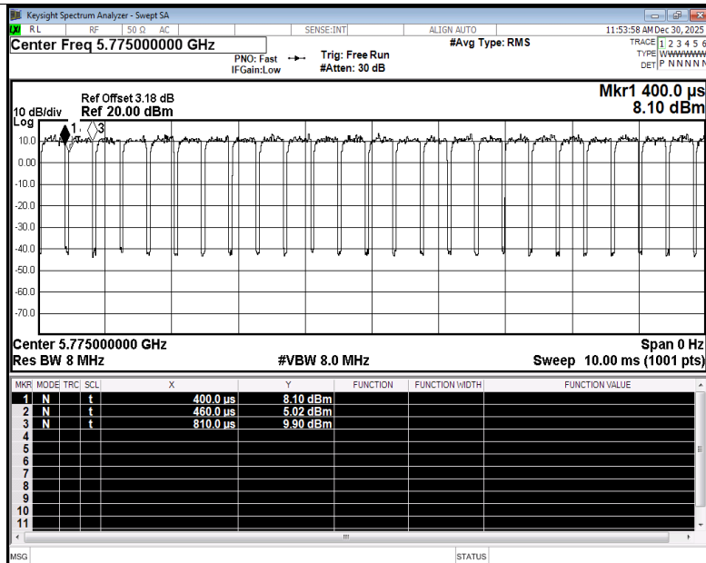
Duty Cycle NVNT be80 5775MHz Ant3
