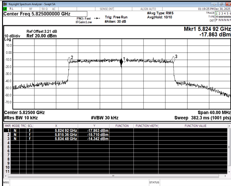
Freq. Stability NVNT ax20 5825MHz Ant5
