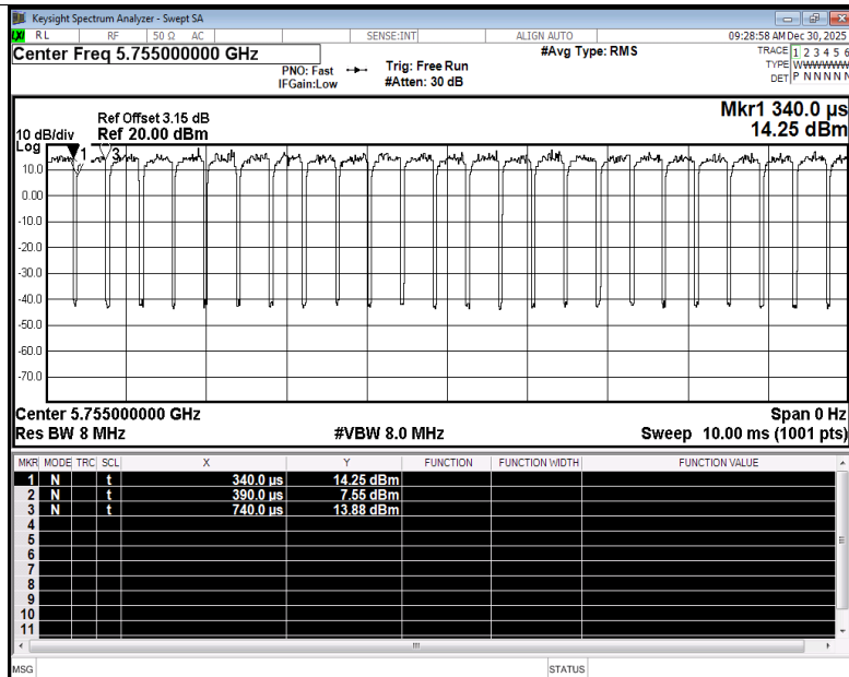
Duty Cycle NVNT ax40 5755MHz Ant1
