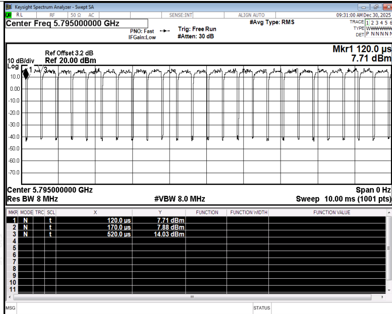
Duty Cycle NVNT ax40 5795MHz Ant1
