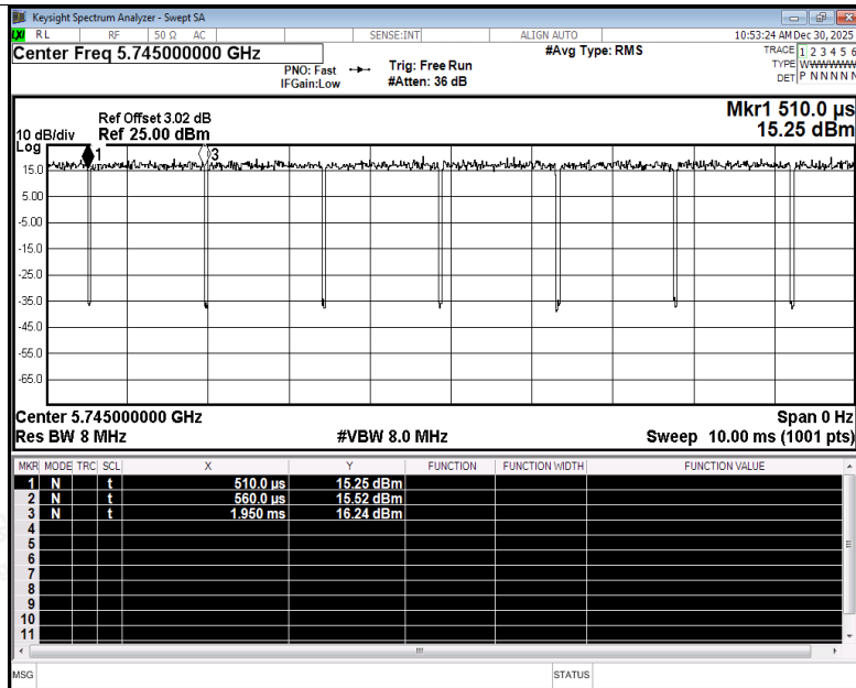
Duty Cycle NVNT a 5745MHz Ant3
