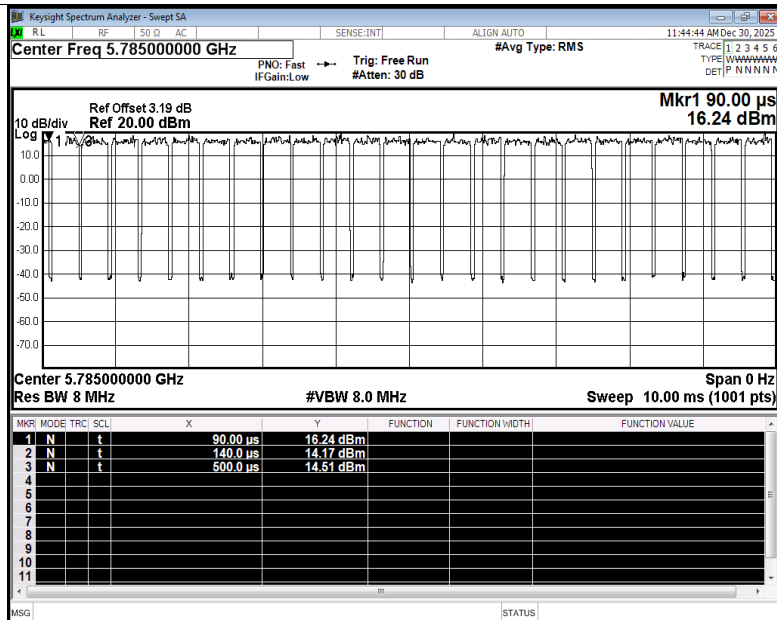
Duty Cycle NVNT be20 5785MHz Ant3
