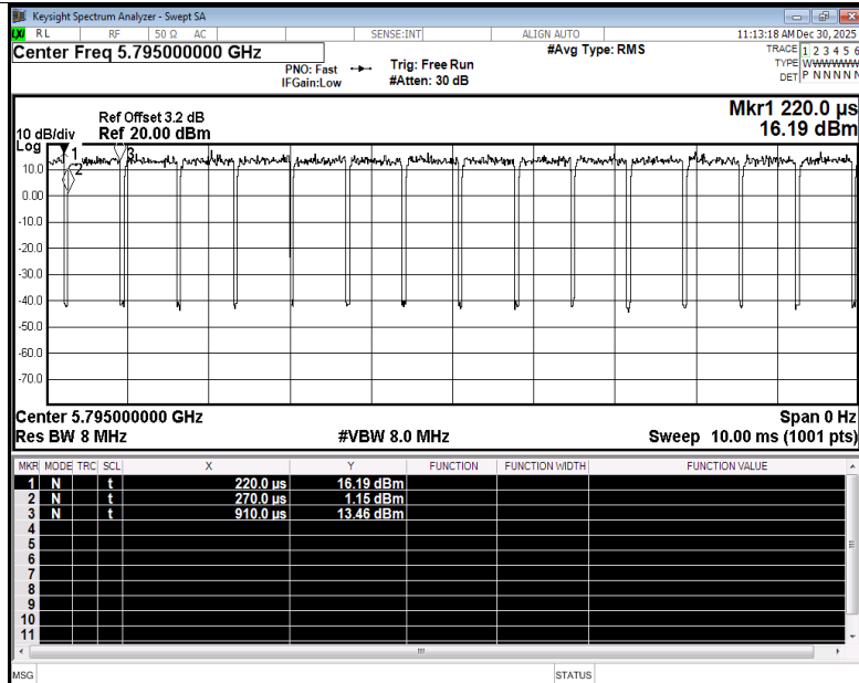
Duty Cycle NVNT n40 5795MHz Ant3
