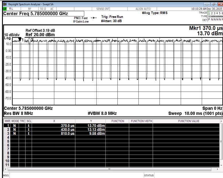
Duty Cycle NVNT ac20 5785MHz Ant2
