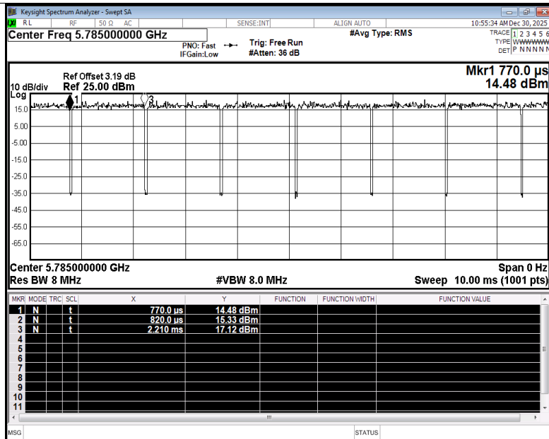
Duty Cycle NVNT a 5785MHz Ant3
