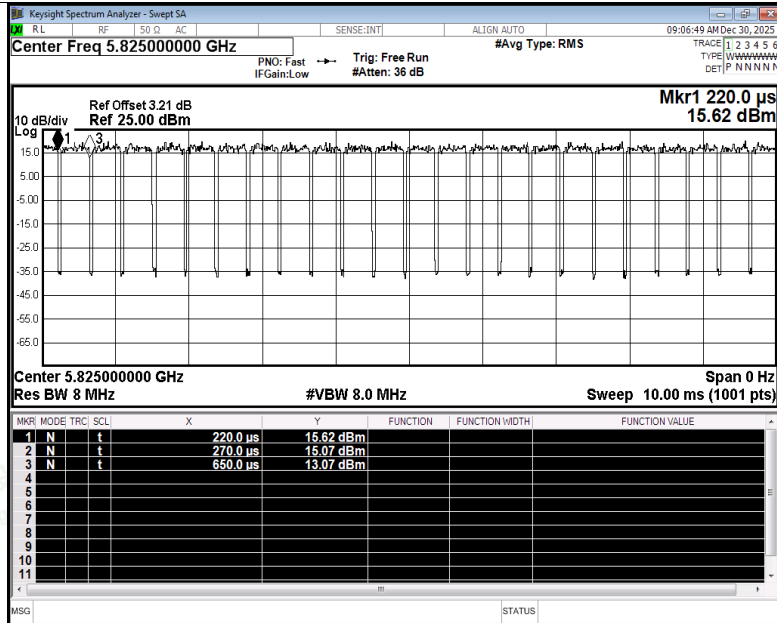
Duty Cycle NVNT ac20 5825MHz Ant1
