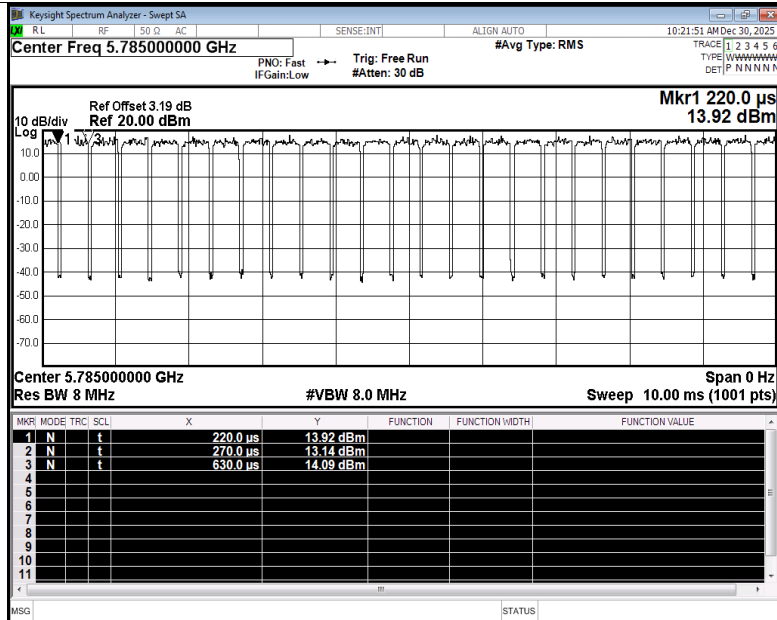
Duty Cycle NVNT be20 5785MHz Ant2
