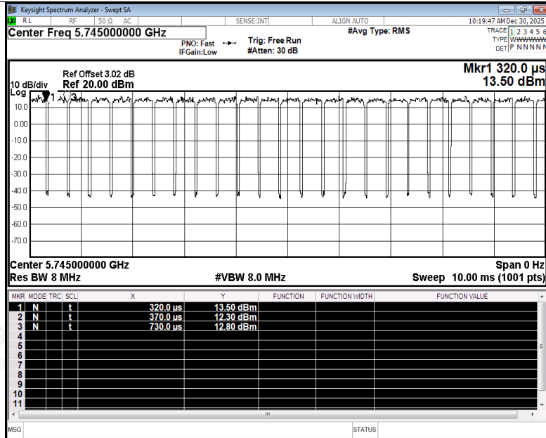
Duty Cycle NVNT be20 5745MHz Ant2
