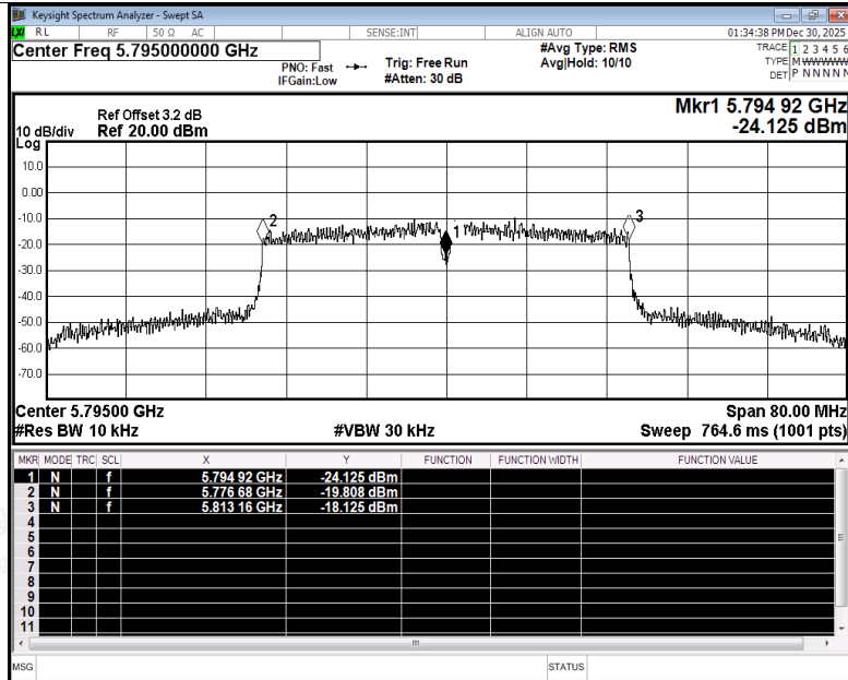
Freq. Stability NVNT ac40 5795MHz Ant5
