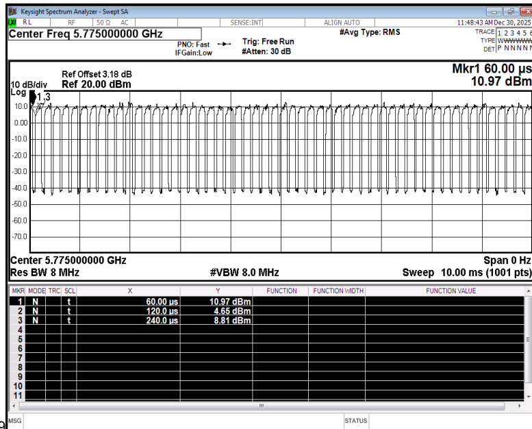
Duty Cycle NVNT ac80 5775MHz Ant3
