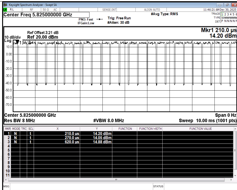
Duty Cycle NVNT be20 5825MHz Ant3
