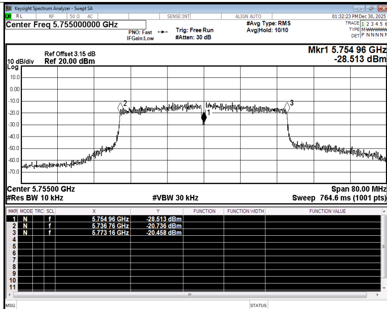
Freq. Stability NVNT ac40 5755MHz Ant5
