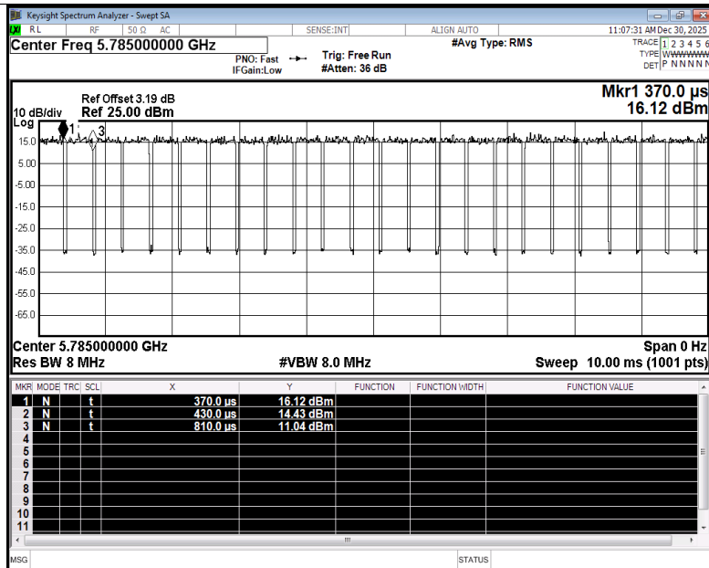
Duty Cycle NVNT ac20 5785MHz Ant3
