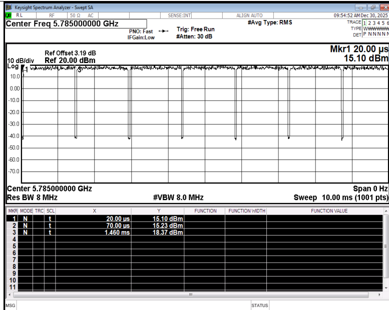
Duty Cycle NVNT a 5785MHz Ant2
