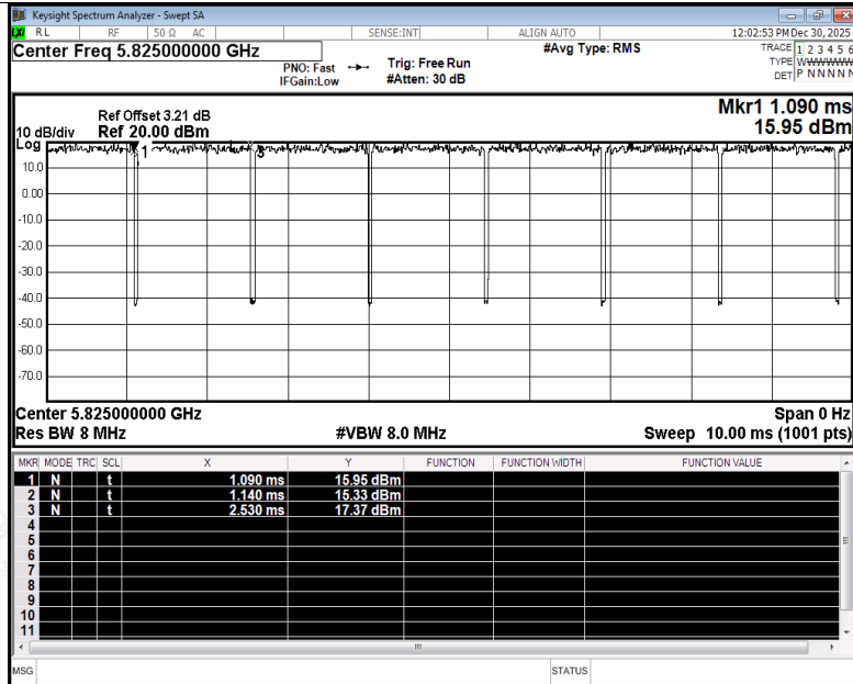
Duty Cycle NVNT a 5825MHz Ant4
