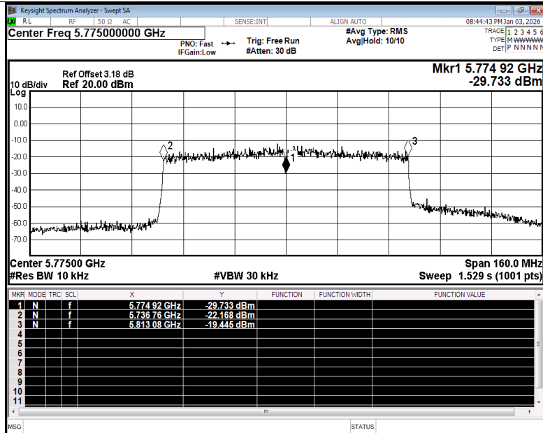
Freq. Stability NVNT ac80 5775MHz Ant5
