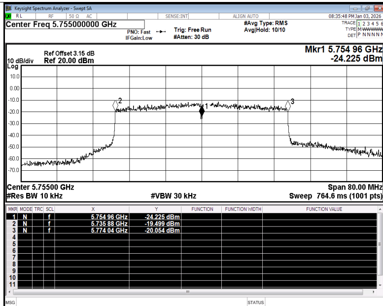
Freq. Stability NVNT ax40 5755MHz Ant5
