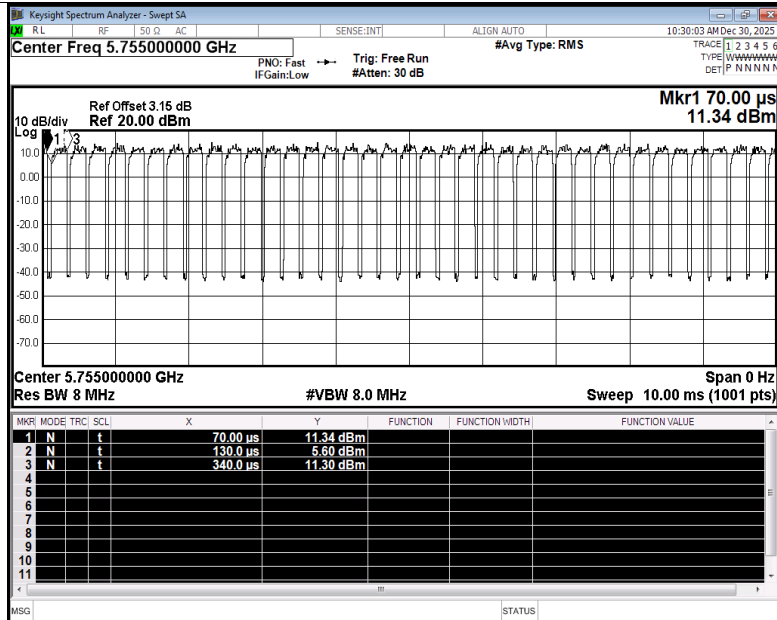
Duty Cycle NVNT ac40 5755MHz Ant2
