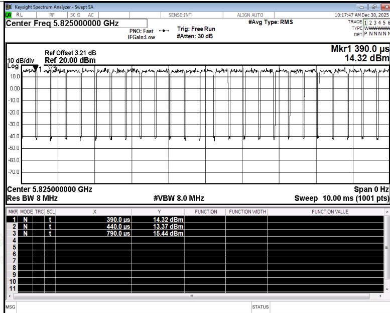
Duty Cycle NVNT ax20 5825MHz Ant2
