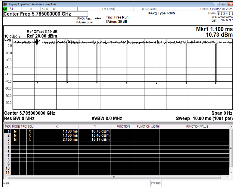
Duty Cycle NVNT n20 5785MHz Ant4
