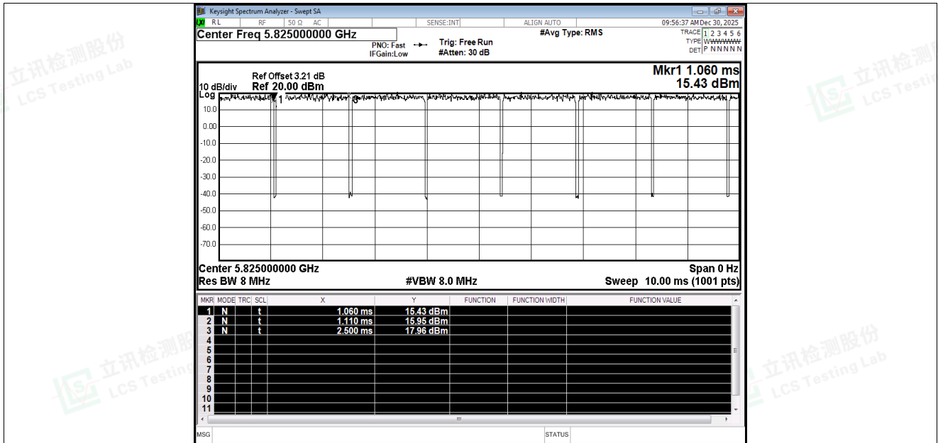
Duty Cycle NVNT a 5825MHz Ant2
