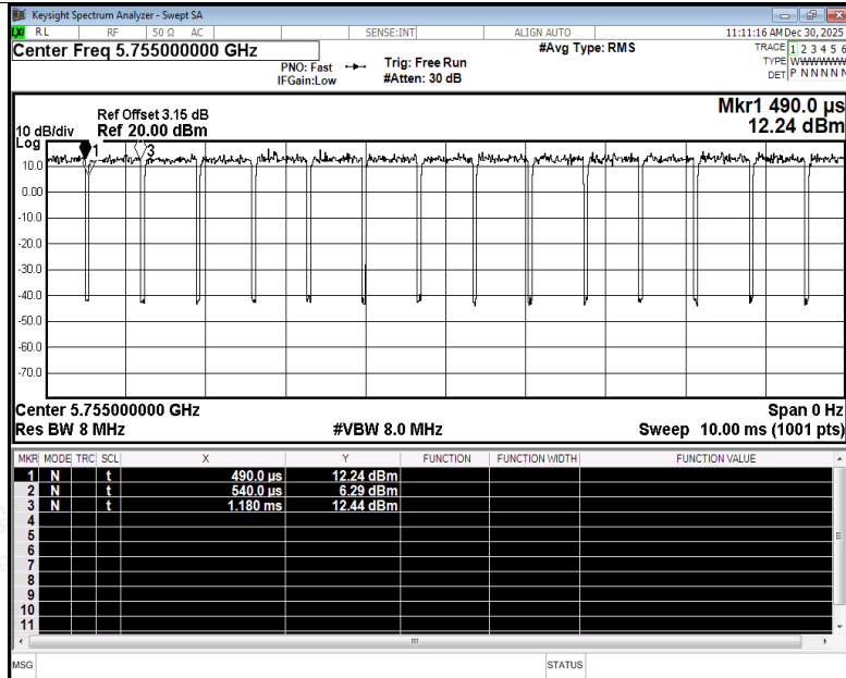
Duty Cycle NVNT n40 5755MHz Ant3
