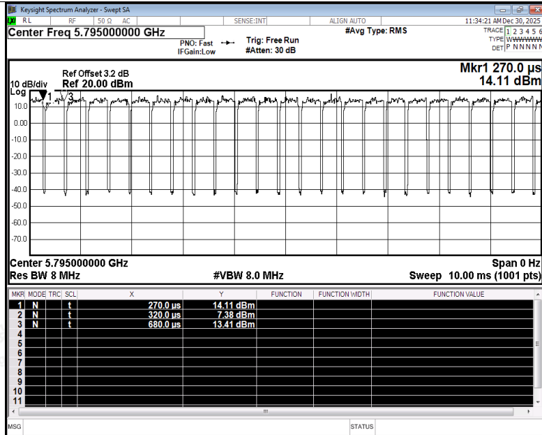
Duty Cycle NVNT be40 5795MHz Ant3
