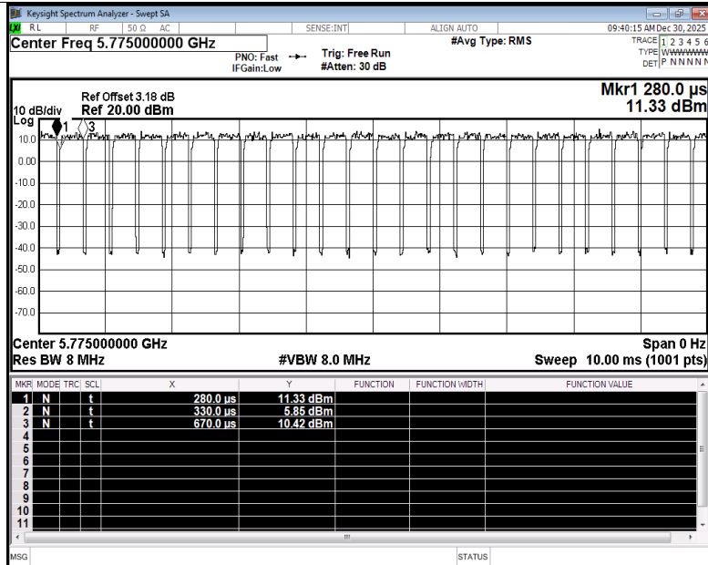
Duty Cycle NVNT ax80 5775MHz Ant1
