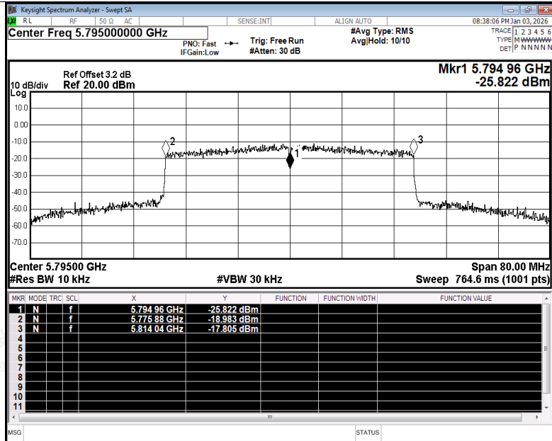
Freq. Stability NVNT ax40 5795MHz Ant5
