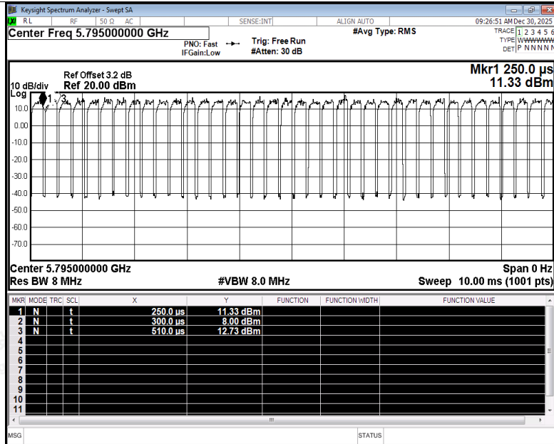
Duty Cycle NVNT ac40 5795MHz Ant1
