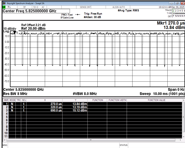
Duty Cycle NVNT ac20 5825MHz Ant2
