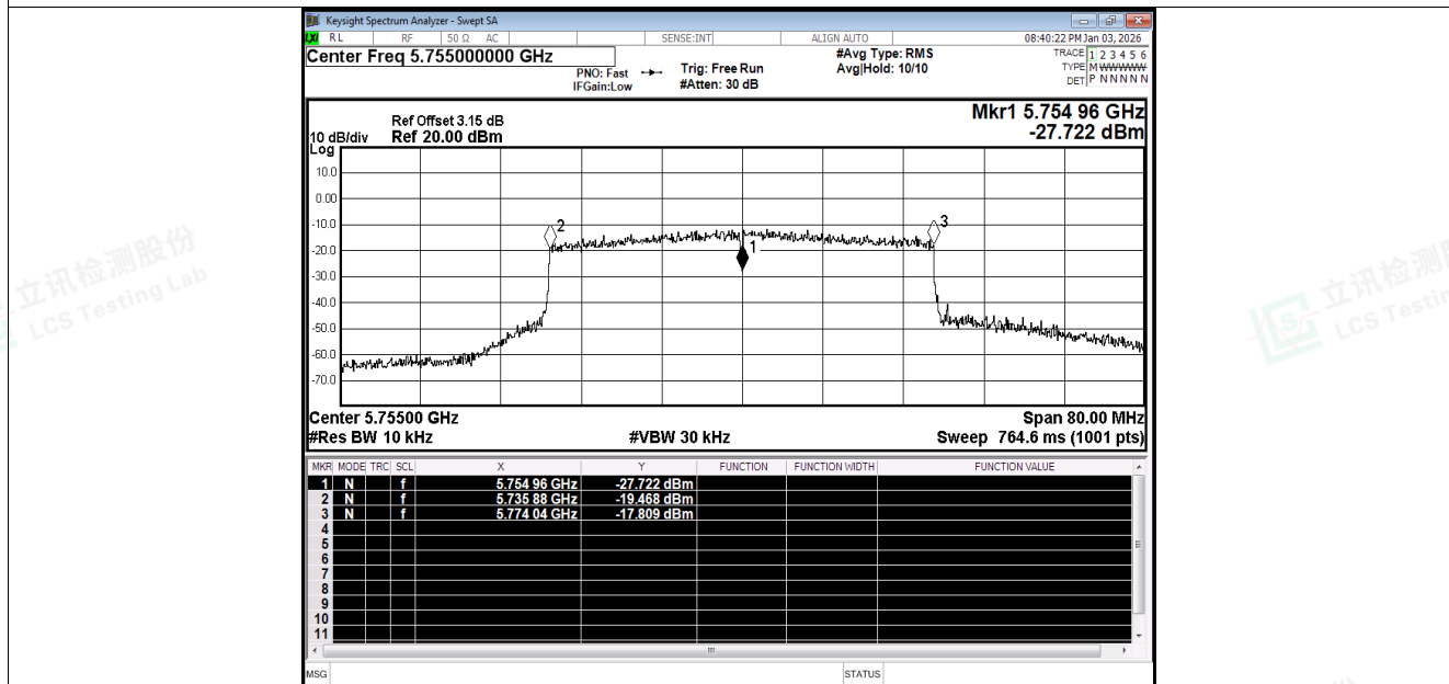
Freq. Stability NVNT be40 5755MHz Ant5
