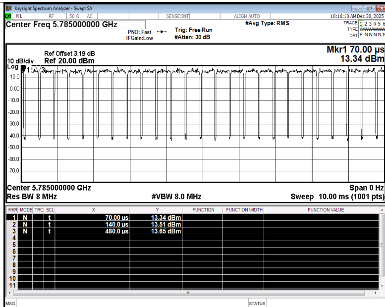
Duty Cycle NVNT ax20 5785MHz Ant2
