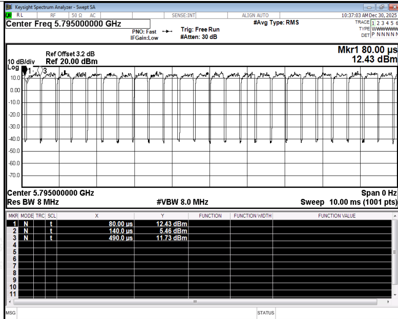
Duty Cycle NVNT ax40 5795MHz Ant2
