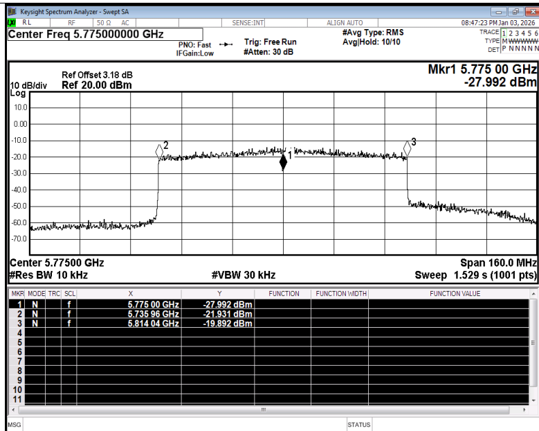
Freq. Stability NVNT ax80 5775MHz Ant5
