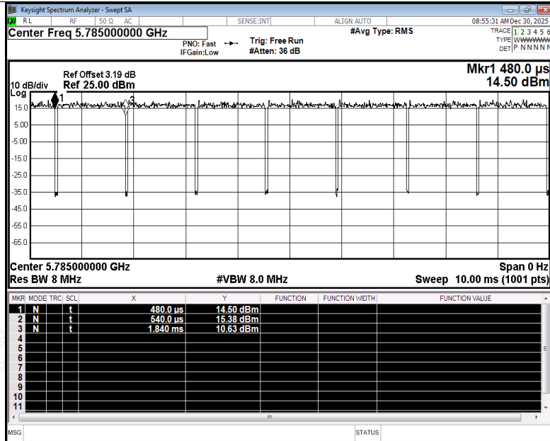
Duty Cycle NVNT n20 5785MHz Ant1
