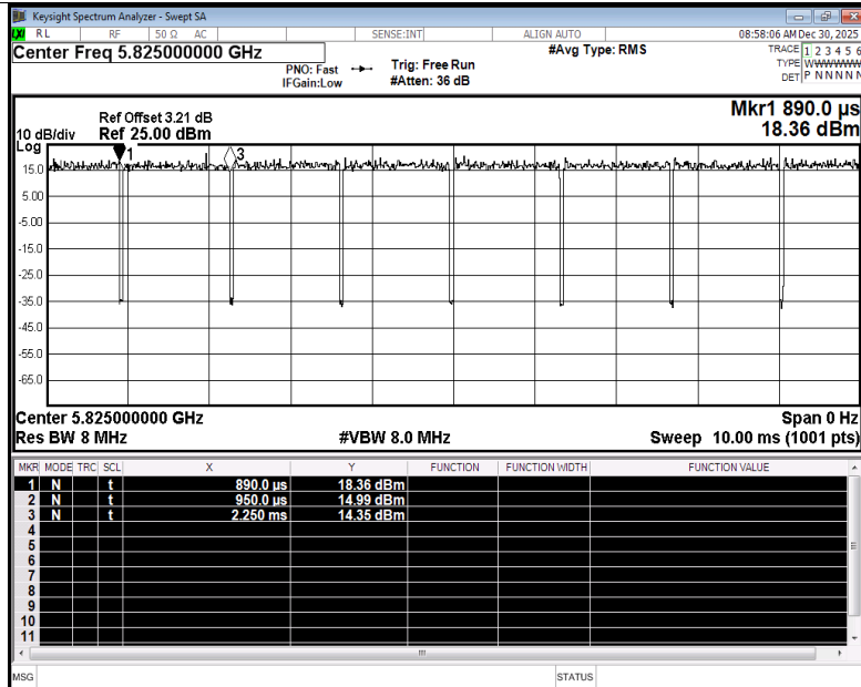
Duty Cycle NVNT n20 5825MHz Ant1
