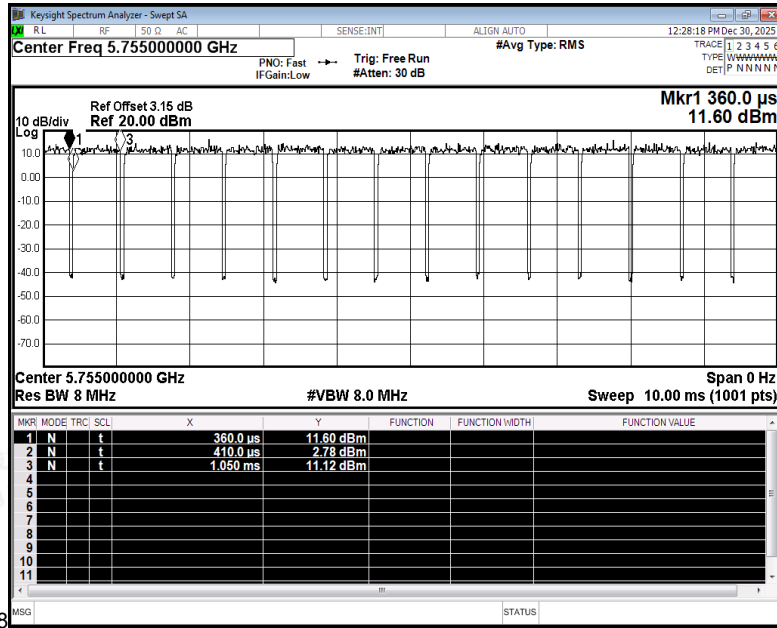
Duty Cycle NVNT n40 5755MHz Ant4
