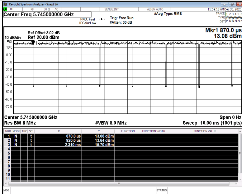
Duty Cycle NVNT a 5745MHz Ant4
