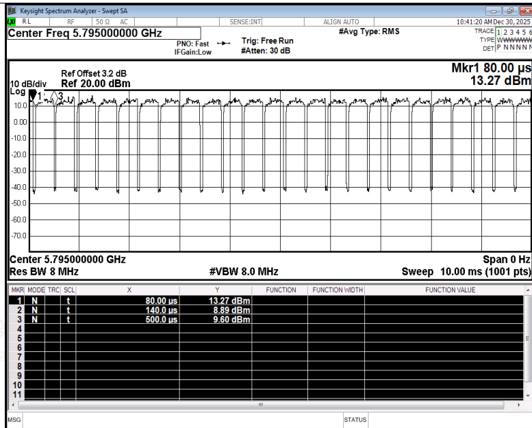
Duty Cycle NVNT be40 5795MHz Ant2
