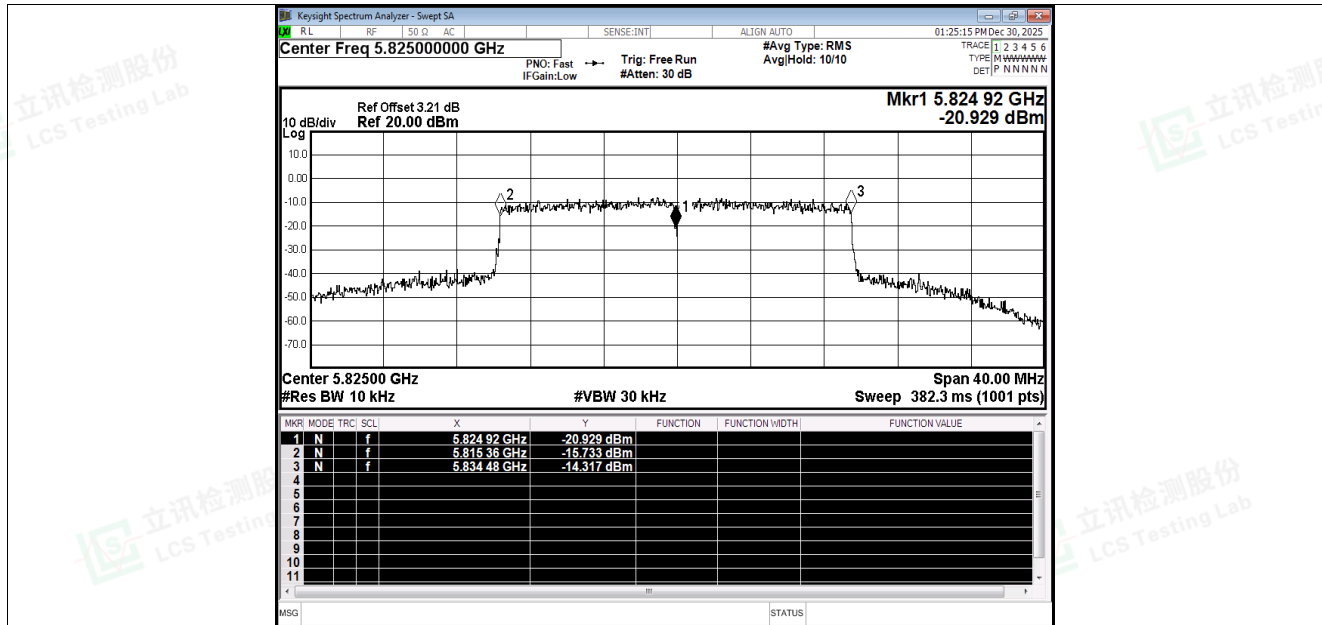
Freq. Stability NVNT be20 5825MHz Ant5
