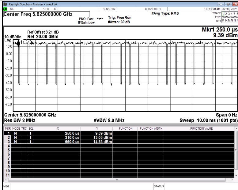
Duty Cycle NVNT be20 5825MHz Ant2
