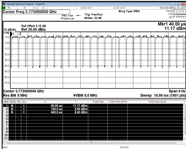
Duty Cycle NVNT be80 5775MHz Ant1
