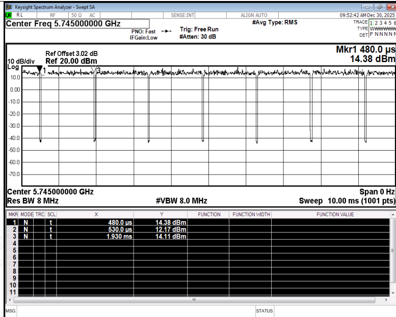
Duty Cycle NVNT a 5745MHz Ant2
