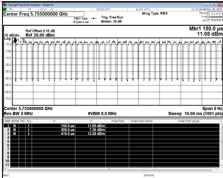
Duty Cycle NVNT ac40 5755MHz Ant3
