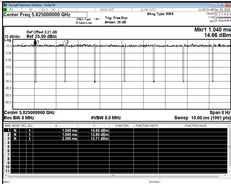
Duty Cycle NVNT n20 5825MHz Ant3
