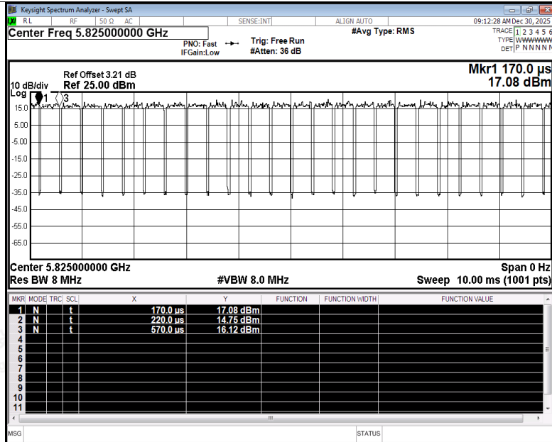
Duty Cycle NVNT ax20 5825MHz Ant1
