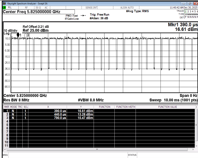
Duty Cycle NVNT ax20 5825MHz Ant3
