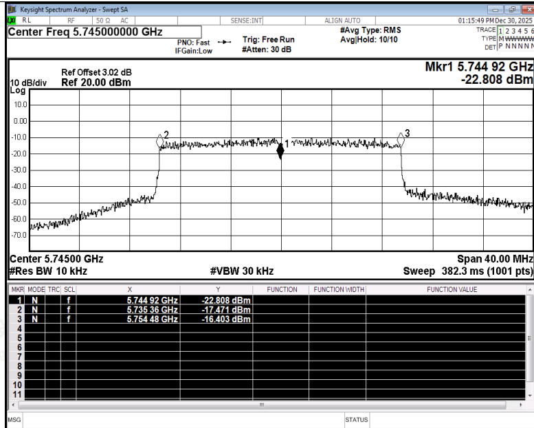
Freq. Stability NVNT ax20 5745MHz Ant5
