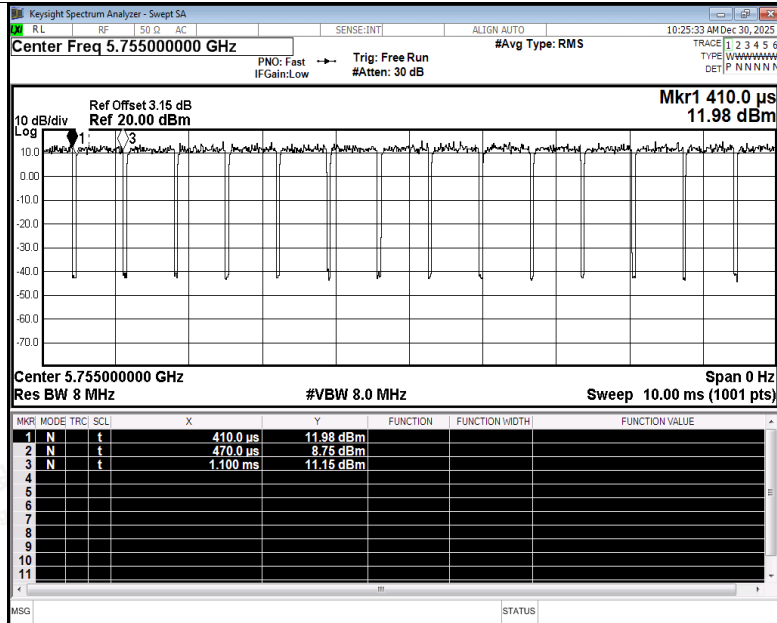
Duty Cycle NVNT n40 5755MHz Ant2
