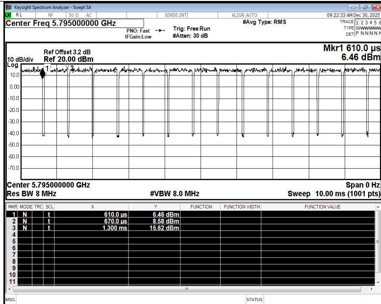
Duty Cycle NVNT n40 5795MHz Ant1
