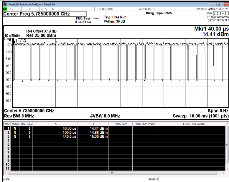
Duty Cycle NVNT ax20 5785MHz Ant1
