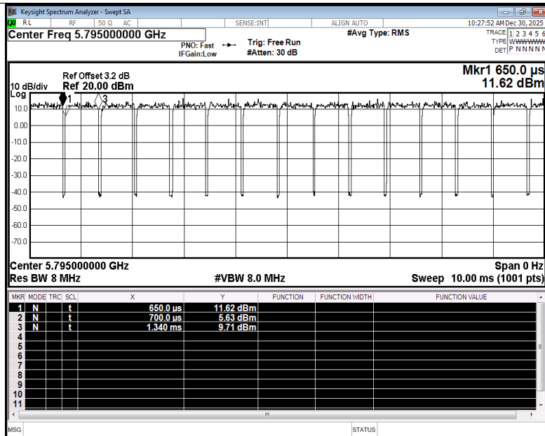
Duty Cycle NVNT n40 5795MHz Ant2
