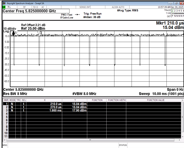
Duty Cycle NVNT a 5825MHz Ant3
