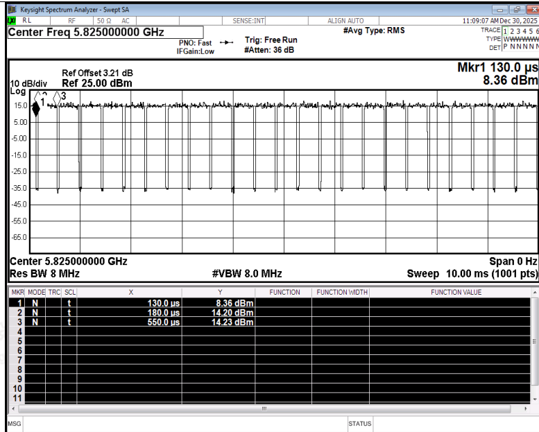
Duty Cycle NVNT ac20 5825MHz Ant3
