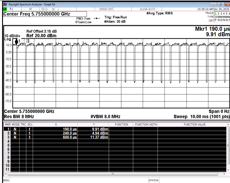
Duty Cycle NVNT be40 5755MHz Ant2
