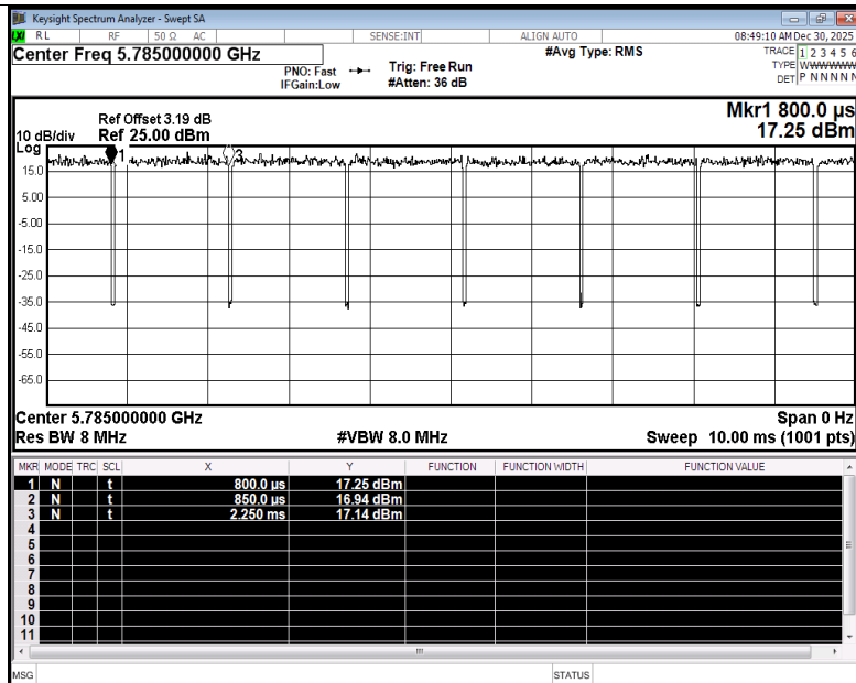
Duty Cycle NVNT a 5785MHz Ant1
