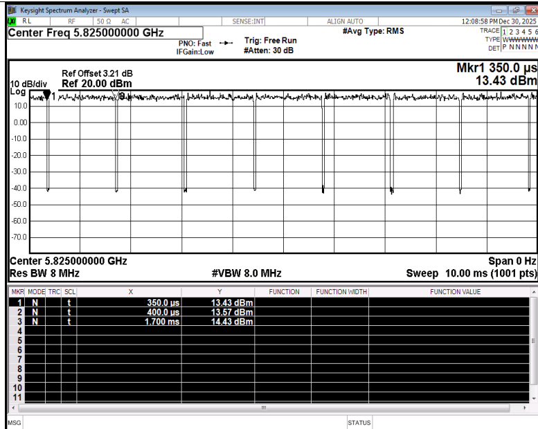
Duty Cycle NVNT n20 5825MHz Ant4
