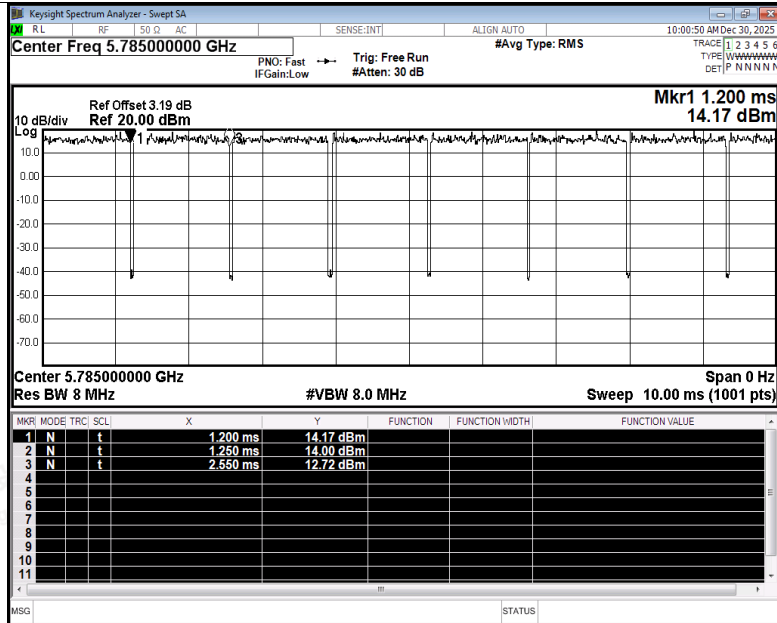
Duty Cycle NVNT n20 5785MHz Ant2
