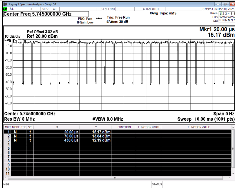
Duty Cycle NVNT be20 5745MHz Ant5
