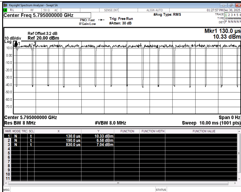
Duty Cycle NVNT n40 5795MHz Ant5
