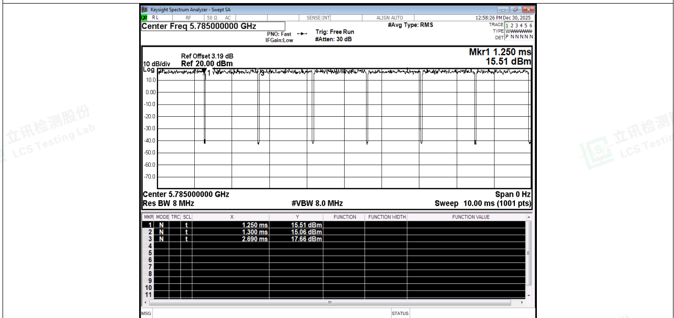
Duty Cycle NVNT a 5785MHz Ant5
