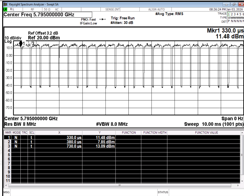
Duty Cycle NVNT ax40 5795MHz Ant5
