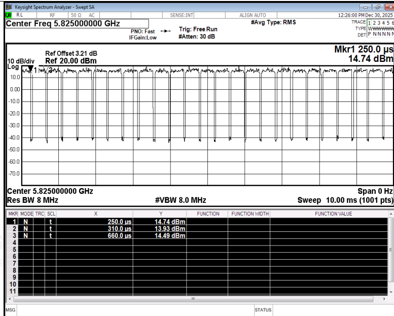
Duty Cycle NVNT be20 5825MHz Ant4
