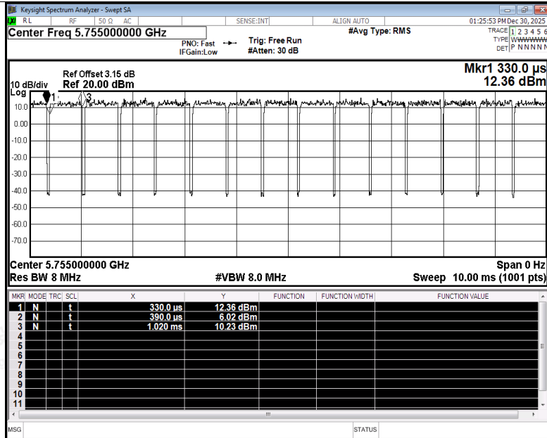
Duty Cycle NVNT n40 5755MHz Ant5
