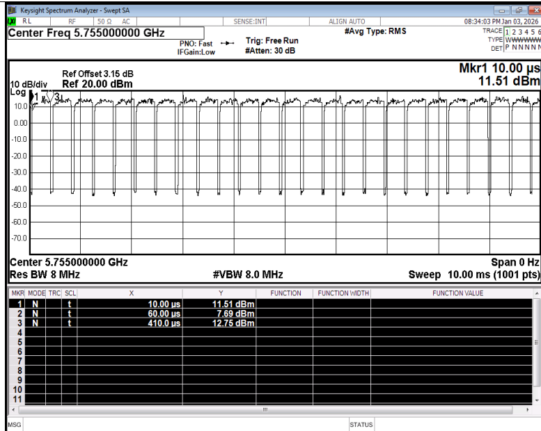
Duty Cycle NVNT ax40 5755MHz Ant5
