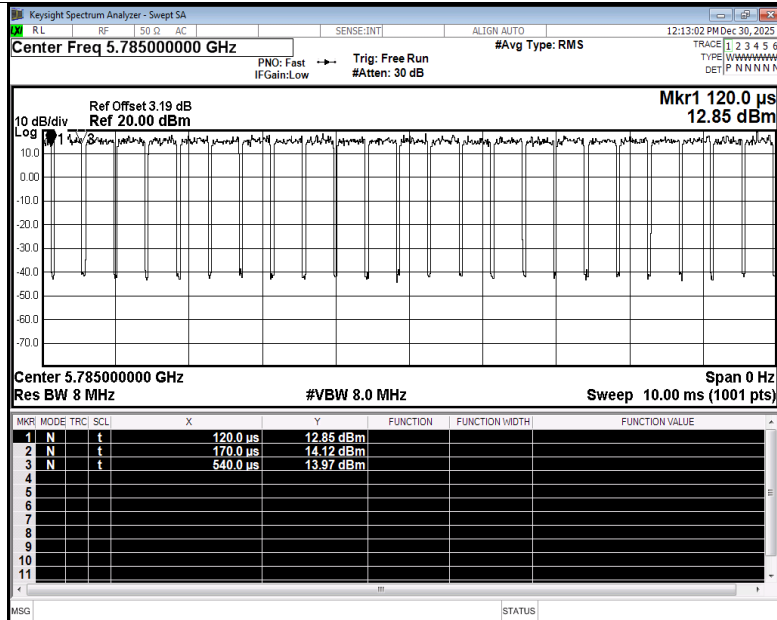
Duty Cycle NVNT ac20 5785MHz Ant4
