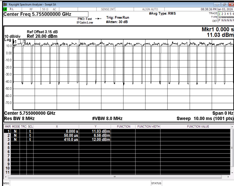
Duty Cycle NVNT be40 5755MHz Ant5
