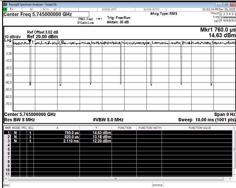
Duty Cycle NVNT n20 5745MHz Ant5
