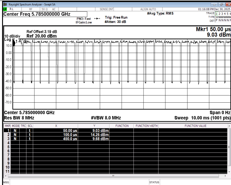
Duty Cycle NVNT ax20 5785MHz Ant5
