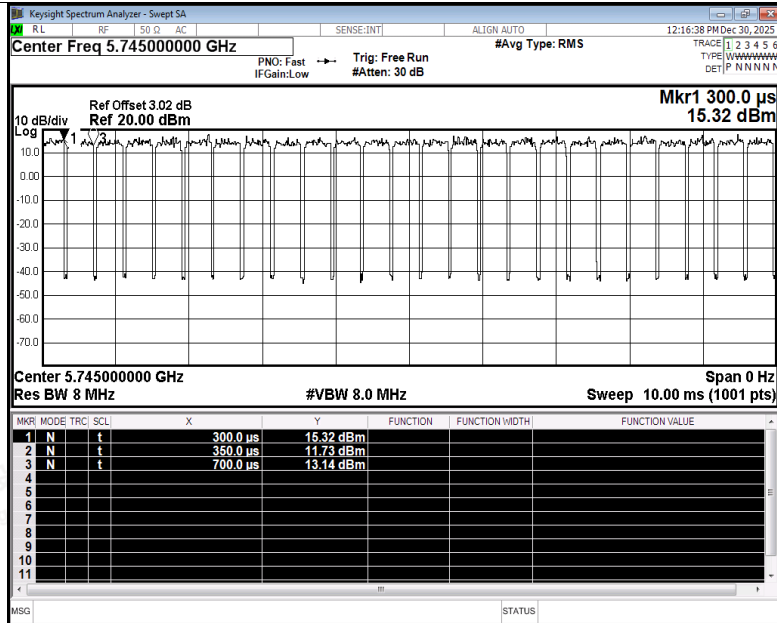
Duty Cycle NVNT ax20 5745MHz Ant4
