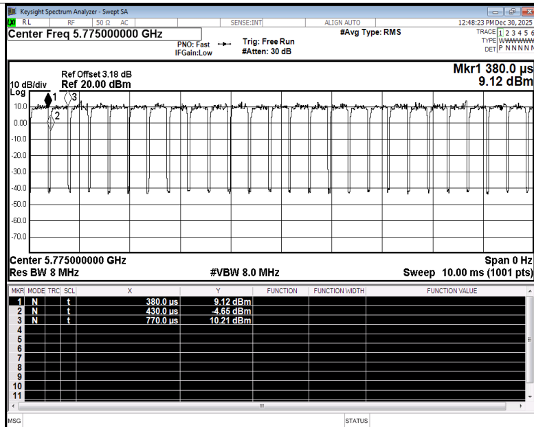
Duty Cycle NVNT ax80 5775MHz Ant4
