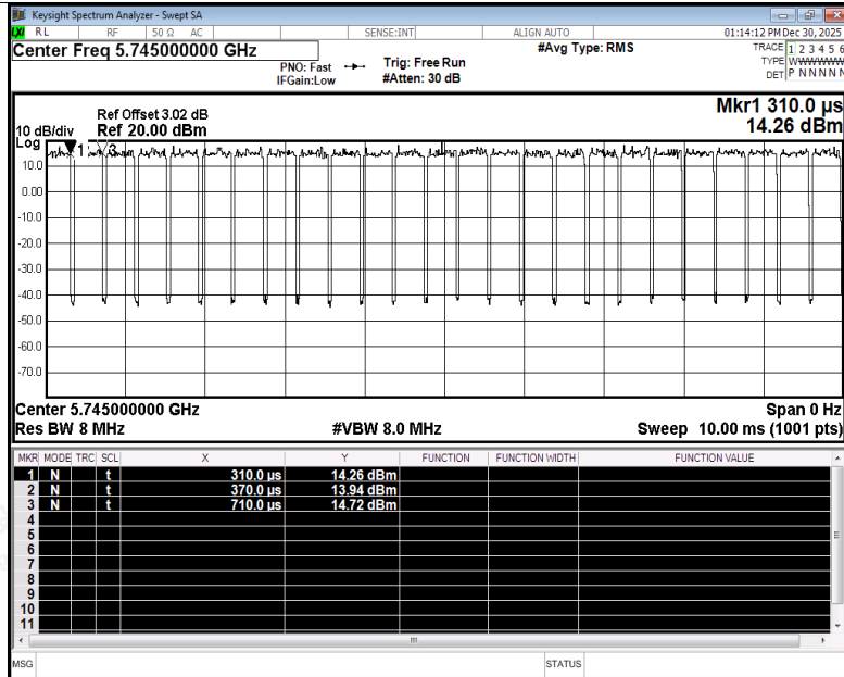
Duty Cycle NVNT ax20 5745MHz Ant5
