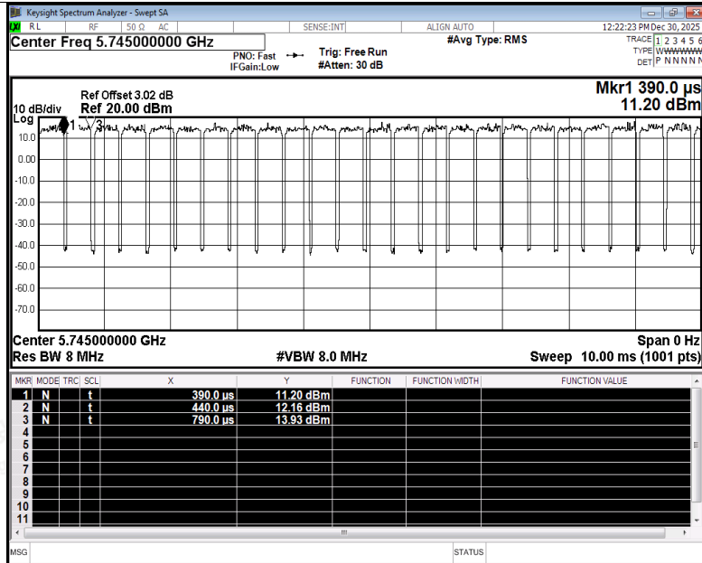
Duty Cycle NVNT be20 5745MHz Ant4
