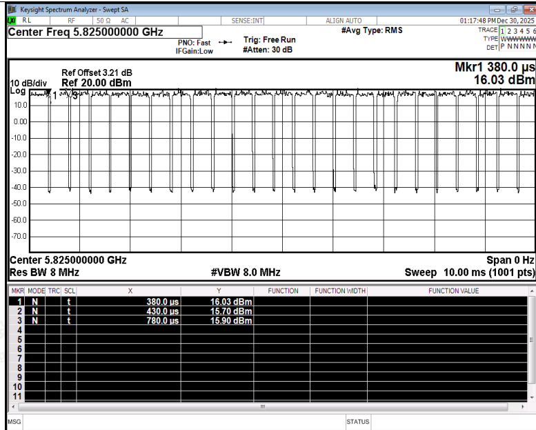
Duty Cycle NVNT ax20 5825MHz Ant5
