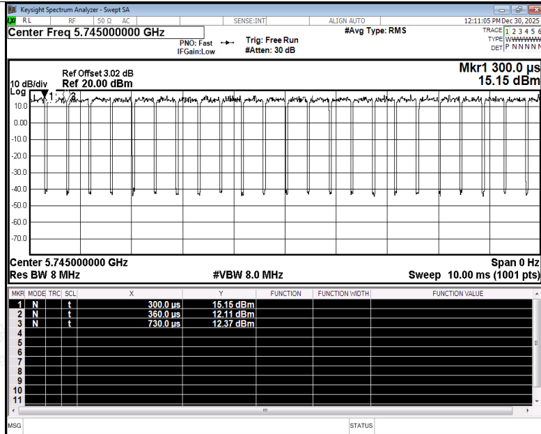
Duty Cycle NVNT ac20 5745MHz Ant4
