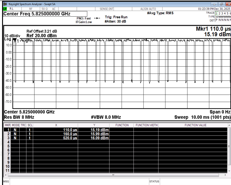
Duty Cycle NVNT be20 5825MHz Ant5
