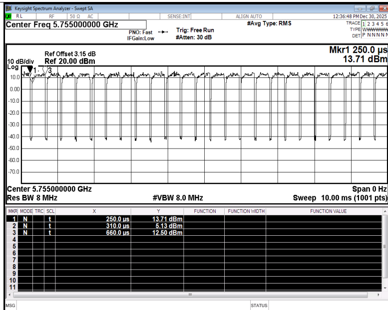
Duty Cycle NVNT ax40 5755MHz Ant4
