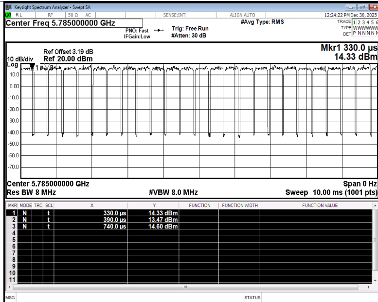
Duty Cycle NVNT be20 5785MHz Ant4
