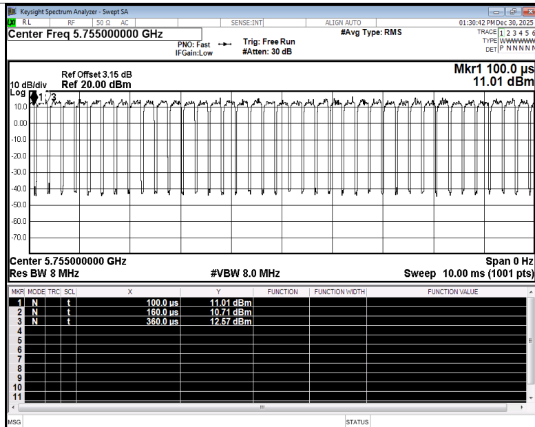
Duty Cycle NVNT ac40 5755MHz Ant5
