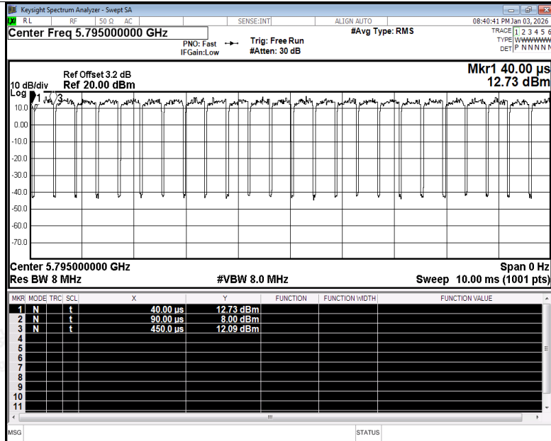
Duty Cycle NVNT be40 5795MHz Ant5
