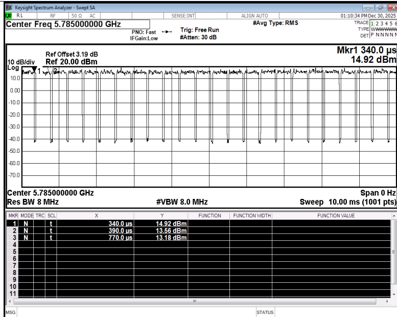
Duty Cycle NVNT ac20 5785MHz Ant5
