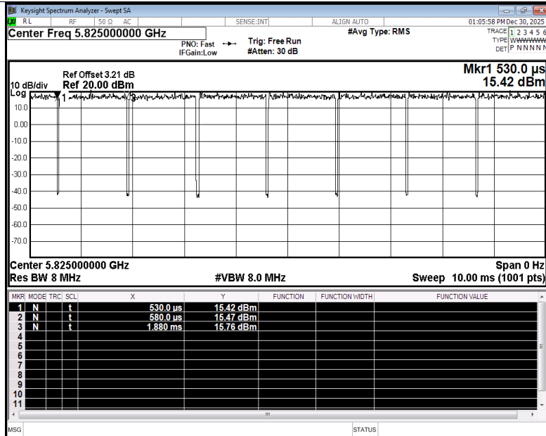
Duty Cycle NVNT n20 5825MHz Ant5
