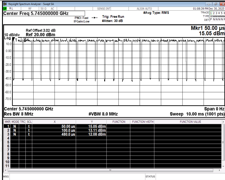
Duty Cycle NVNT ac20 5745MHz Ant5
