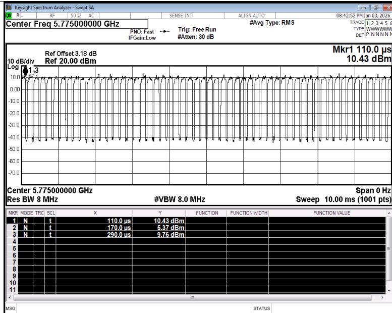
Duty Cycle NVNT ac80 5775MHz Ant5
