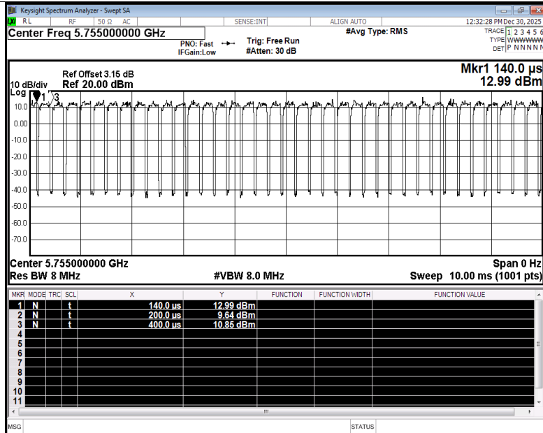
Duty Cycle NVNT ac40 5755MHz Ant4
