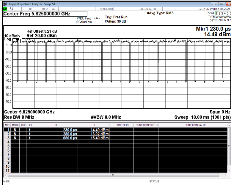
Duty Cycle NVNT ac20 5825MHz Ant4
