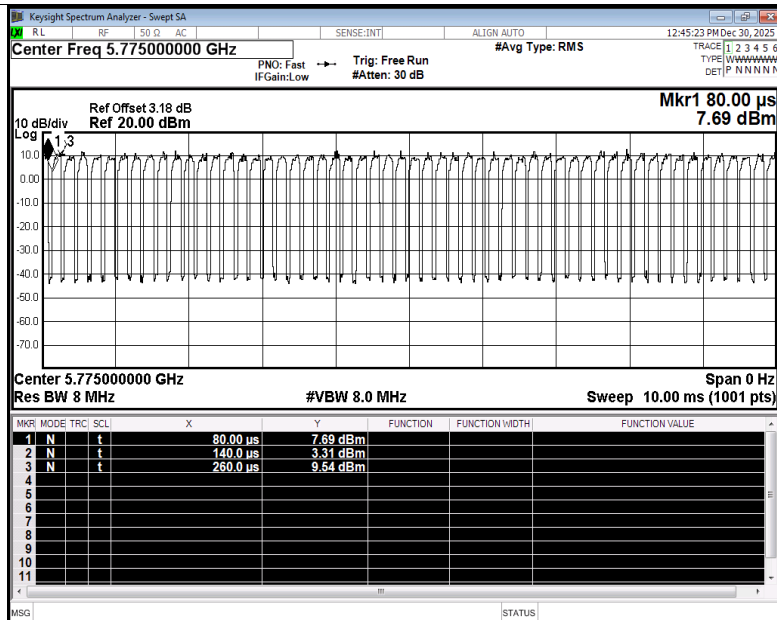
Duty Cycle NVNT ac80 5775MHz Ant4
