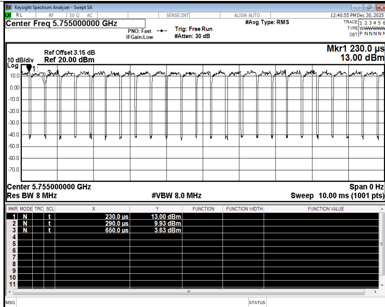
Duty Cycle NVNT be40 5755MHz Ant4
