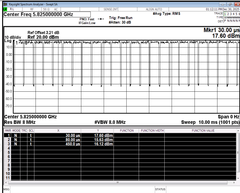
Duty Cycle NVNT ac20 5825MHz Ant5
