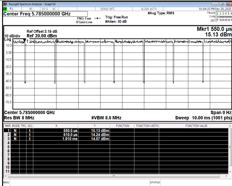
Duty Cycle NVNT n20 5785MHz Ant5
