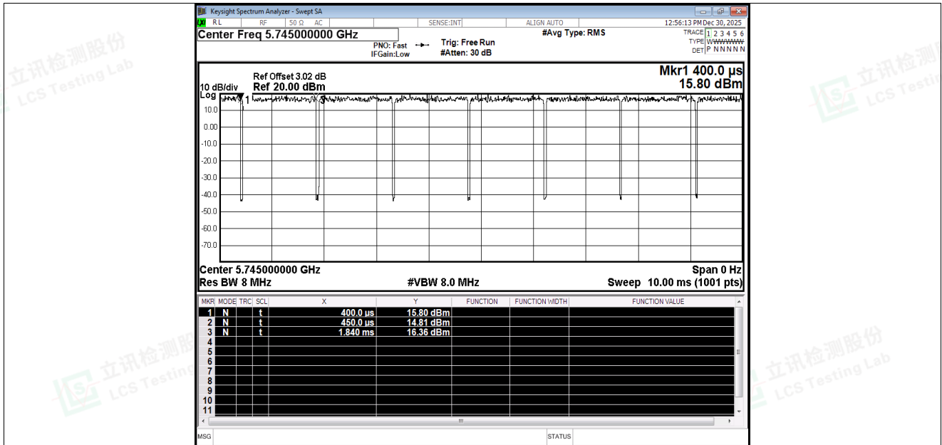
Duty Cycle NVNT a 5745MHz Ant5
