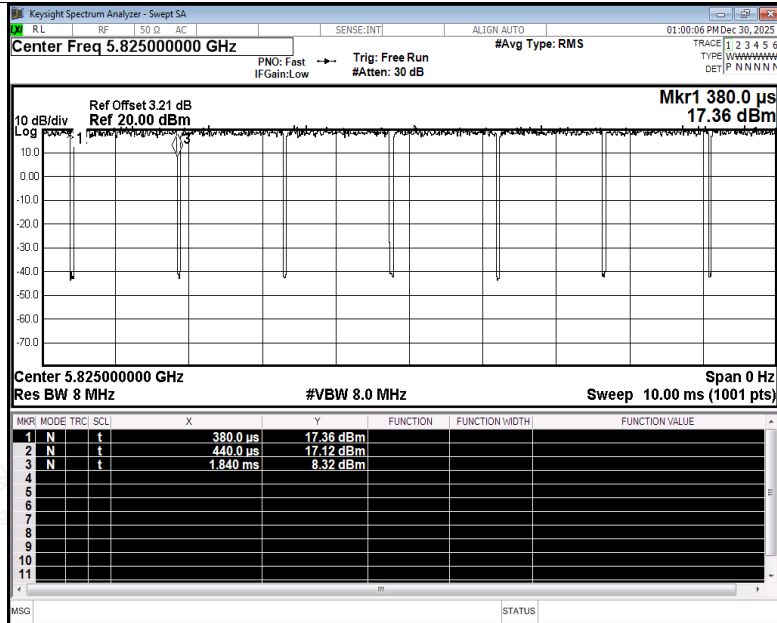
Duty Cycle NVNT a 5825MHz Ant5
