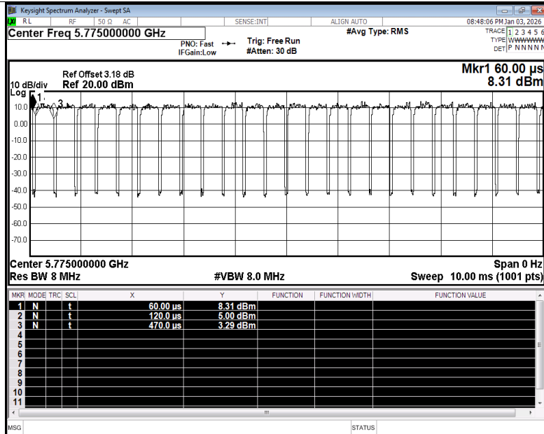
Duty Cycle NVNT be80 5775MHz Ant5
