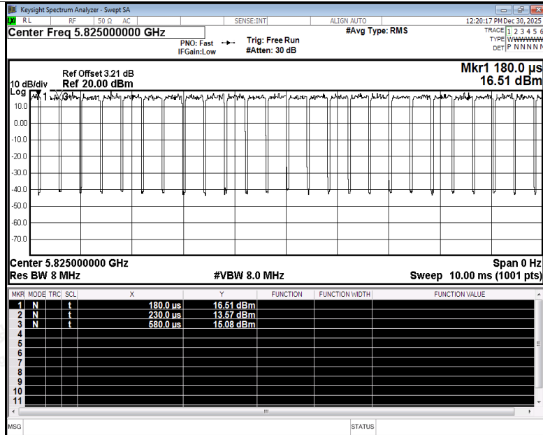
Duty Cycle NVNT ax20 5825MHz Ant4
