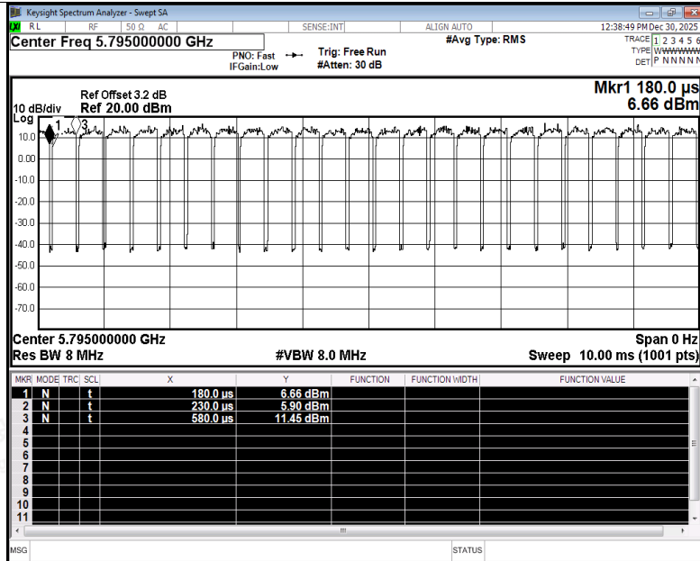
Duty Cycle NVNT ax40 5795MHz Ant4
