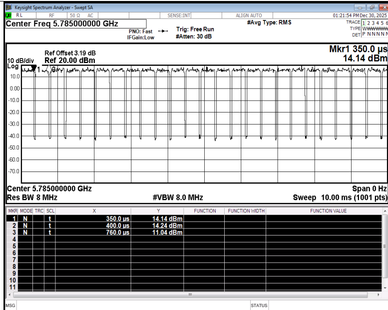
Duty Cycle NVNT be20 5785MHz Ant5
