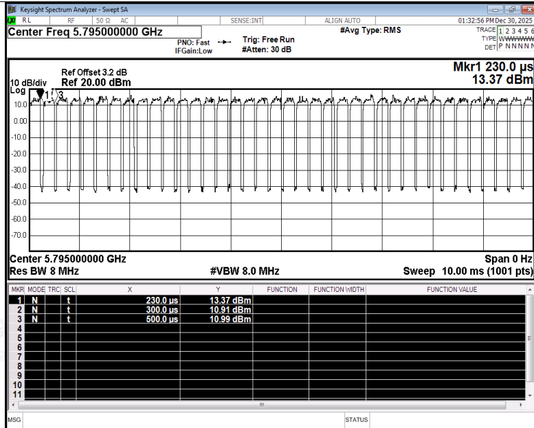
Duty Cycle NVNT ac40 5795MHz Ant5
