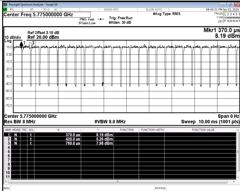
Duty Cycle NVNT ax80 5775MHz Ant5
