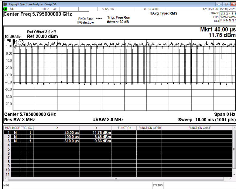
Duty Cycle NVNT ac40 5795MHz Ant4
