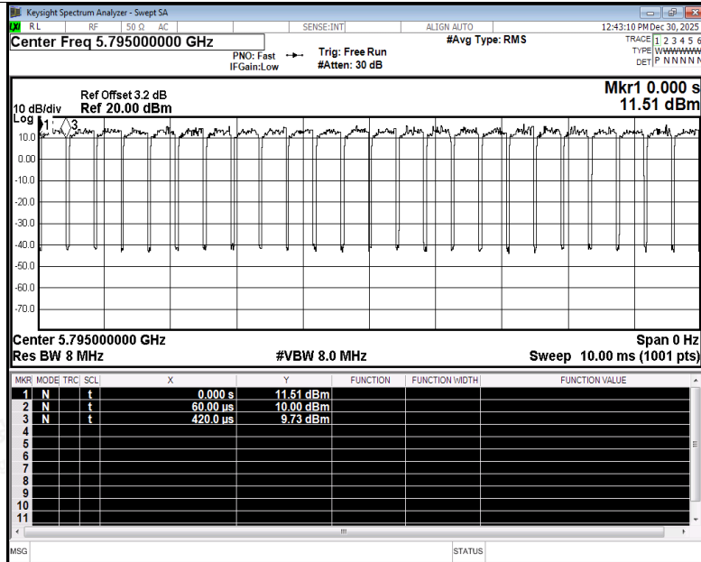
Duty Cycle NVNT be40 5795MHz Ant4
