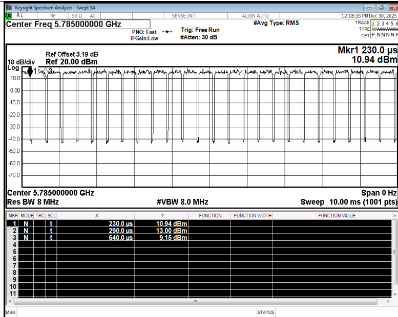
Duty Cycle NVNT ax20 5785MHz Ant4
