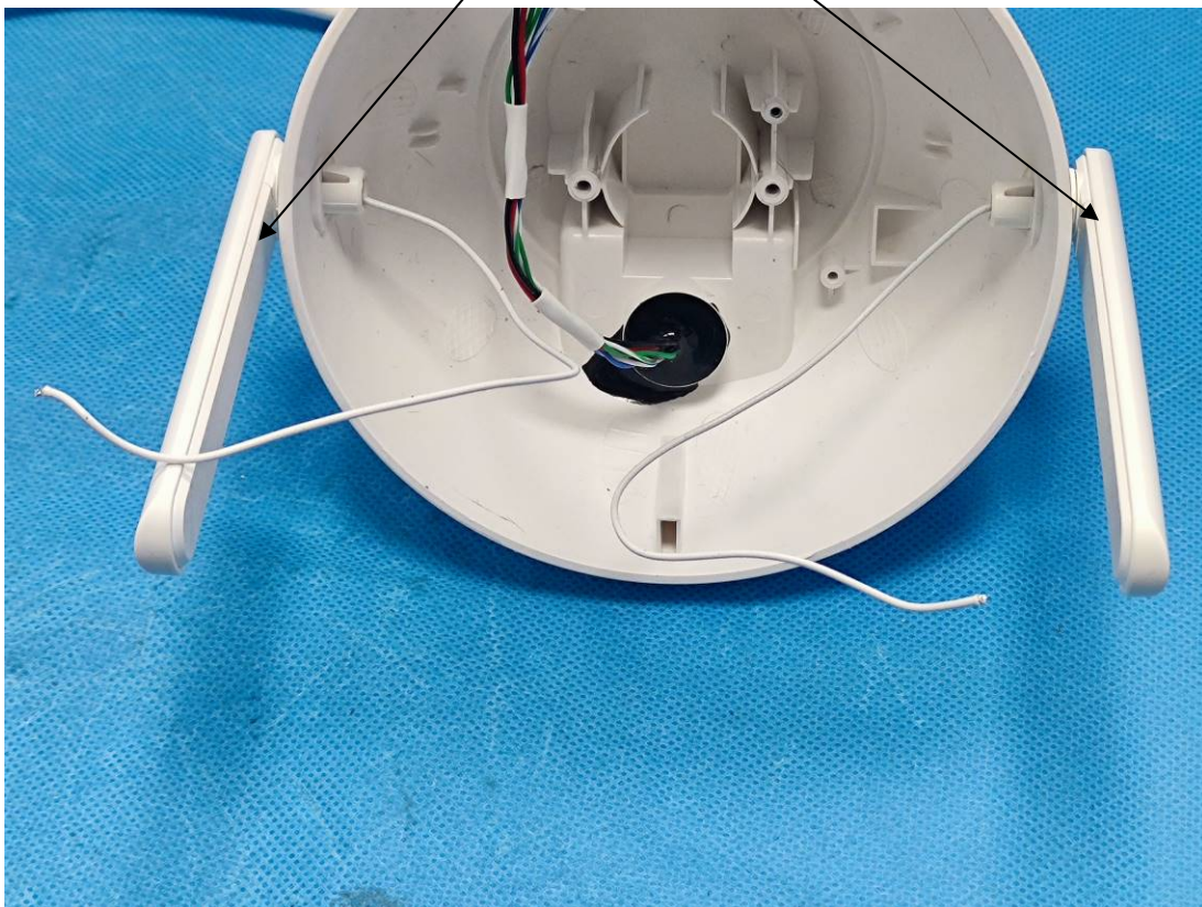
Antenna Chain 0 Antenna Chain 1
