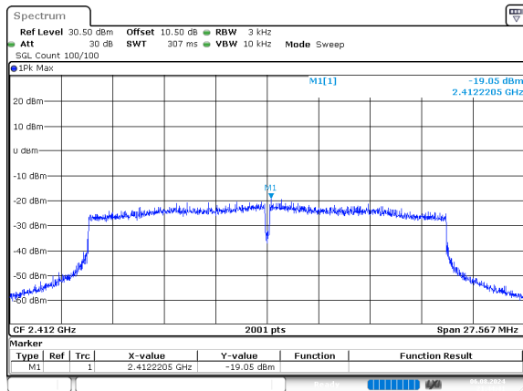
ax20_2412MHz_RU_Full
