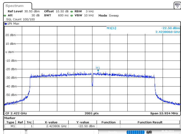
ax40_2422MHz_RU_Full
