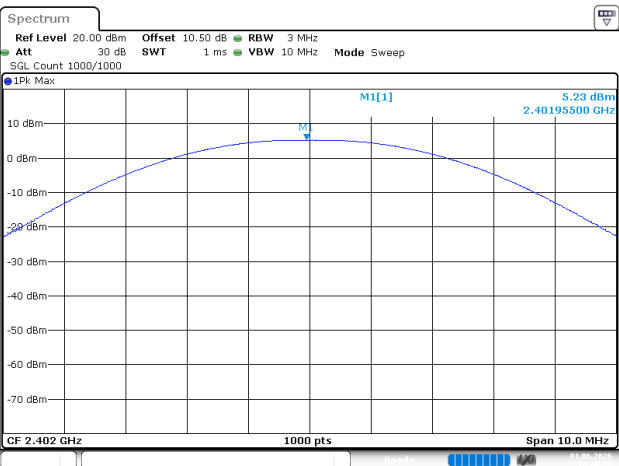
BLE_125kbps_Low Channel
