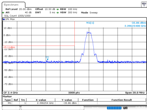
BLE_500kbps_Low Channel
