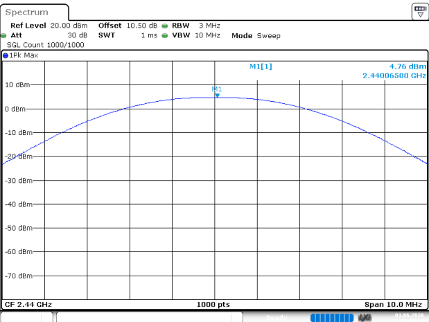
BLE_500kbps_Middle Channel
