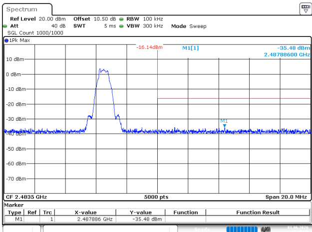
BLE_500kbps_High Channel
