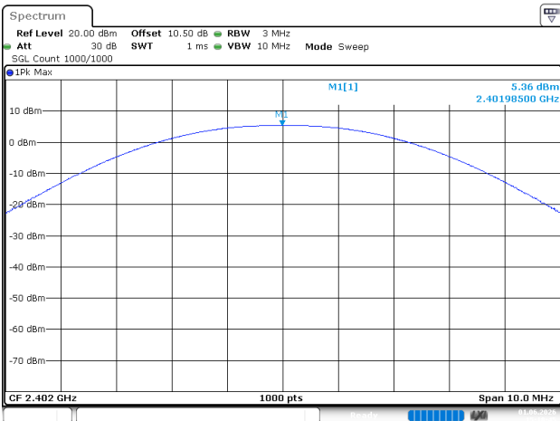
BLE_500kbps_Low Channel
