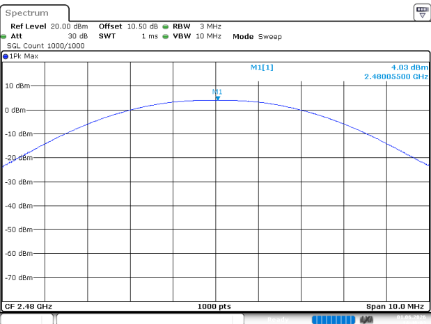
BLE_125kbps_High Channel
