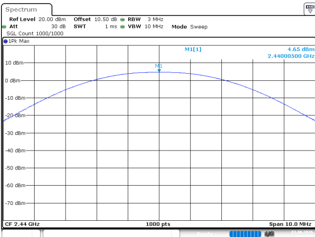
BLE_125kbps_Middle Channel
