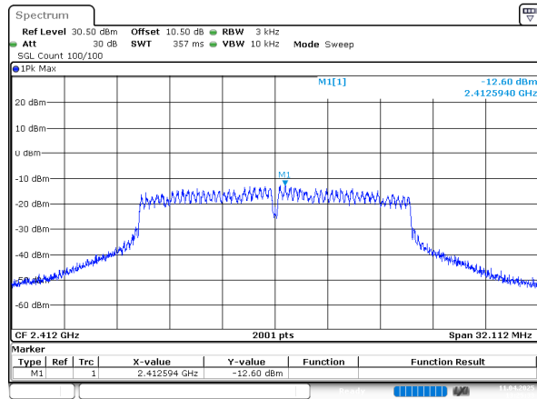
802.11g_2412MHz
