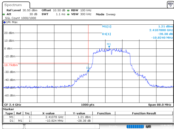
802.11ax20_2412MHz_RU_Full
