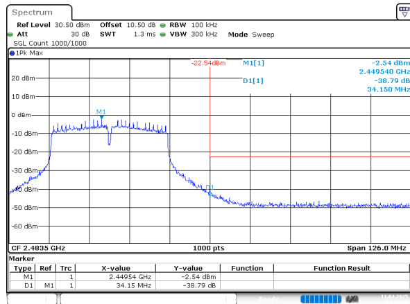
802.11n40_2452MHz
