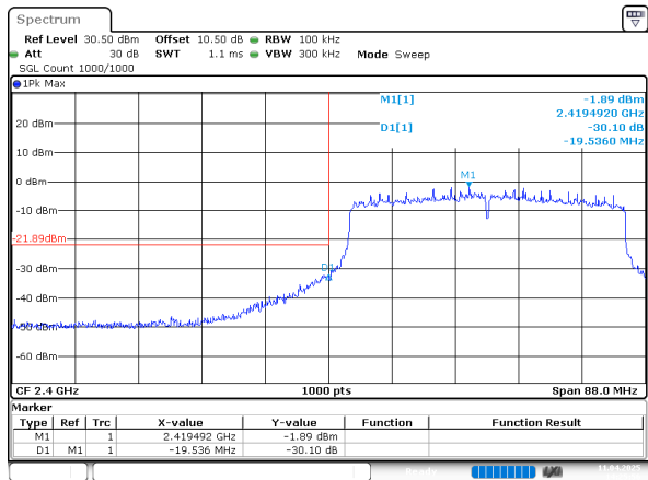
802.11ax40_2422MHz_RU_Full
