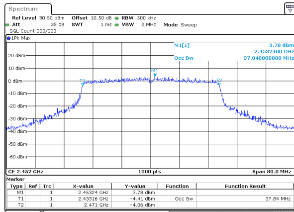
802.11ax40_2452MHz_RU_Full
