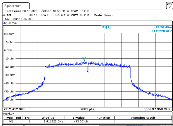
802.11ax20_2412MHz_RU_Full
