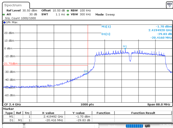
802.11n40_2422MHz
