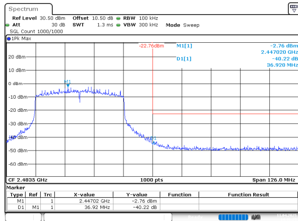
802.11ax40_2452MHz_RU_Full
