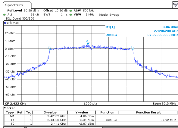
802.11ax40_2422MHz_RU_Full
