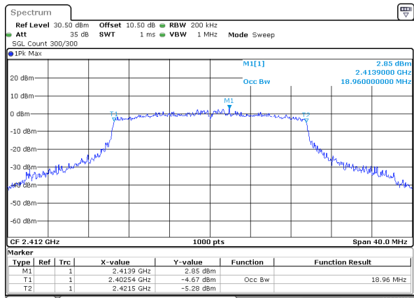
802.11ax20_2412MHz_RU_Full
