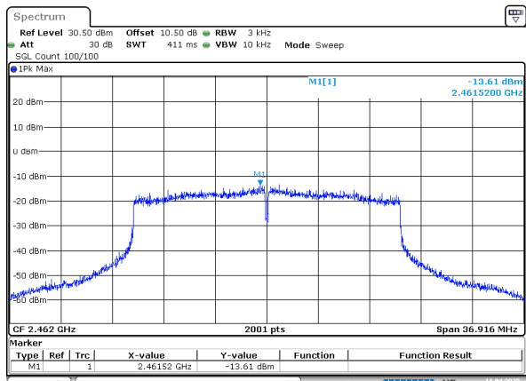
802.11ax20_2462MHz_RU_Full
