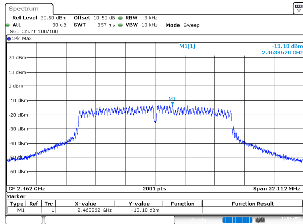
802.11g_2462MHz
