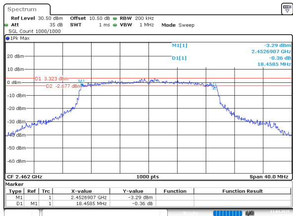
802.11ax20_2462MHz_RU_Full
