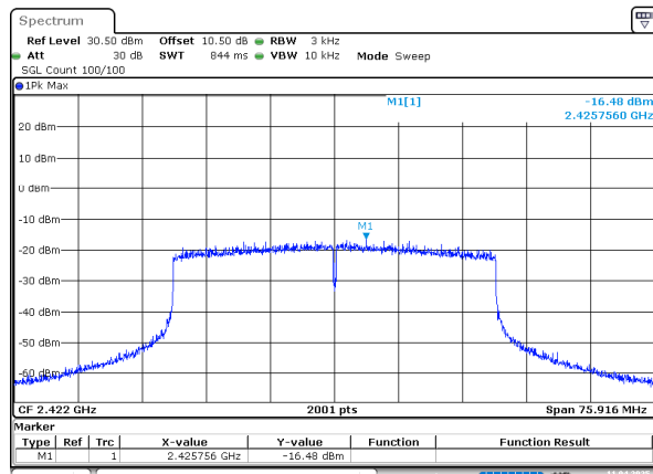
802.11ax40_2422MHz_RU_Full
