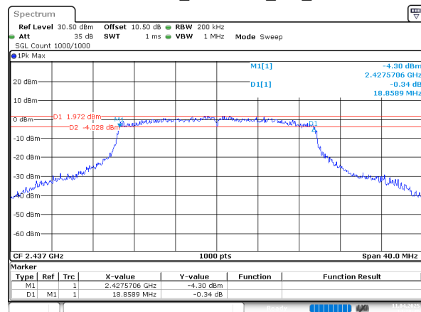
802.11ax20_2437MHz_RU_Full
