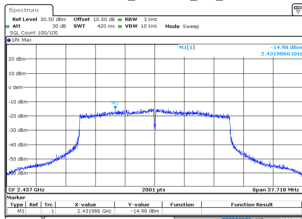
802.11ax20_2437MHz_RU_Full
