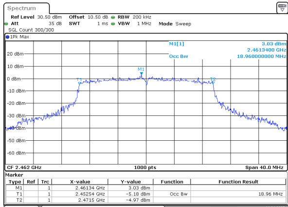
802.11ax20_2462MHz_RU_Full
