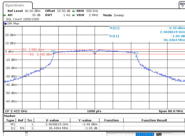
802.11n40_2422MHz
