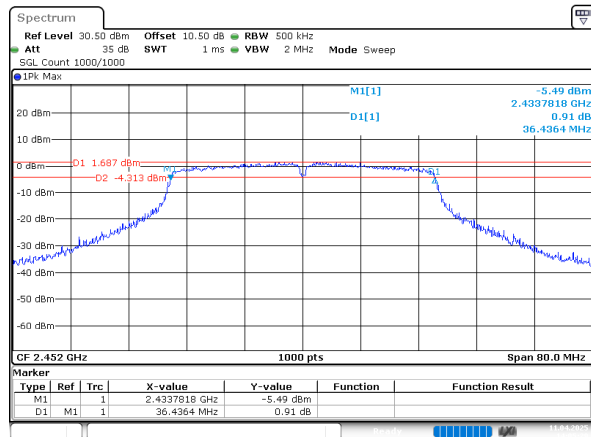
802.11n40_2452MHz
