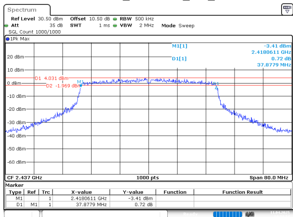
802.11ax40_2437MHz_RU_Full
