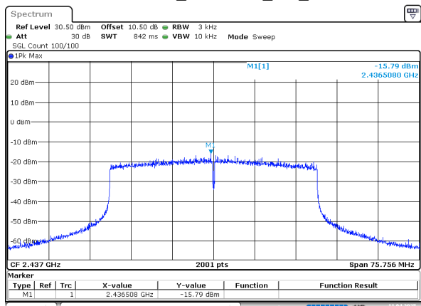
802.11ax40_2437MHz_RU_Full
