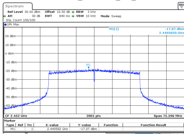
802.11ax40_2452MHz_RU_Full
