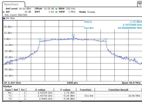
802.11ax20_2437MHz_RU_Full
