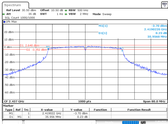
802.11n40_2437MHz
