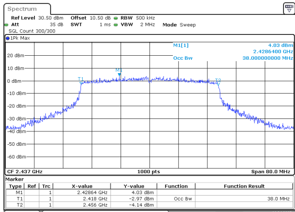
802.11ax40_2437MHz_RU_Full
