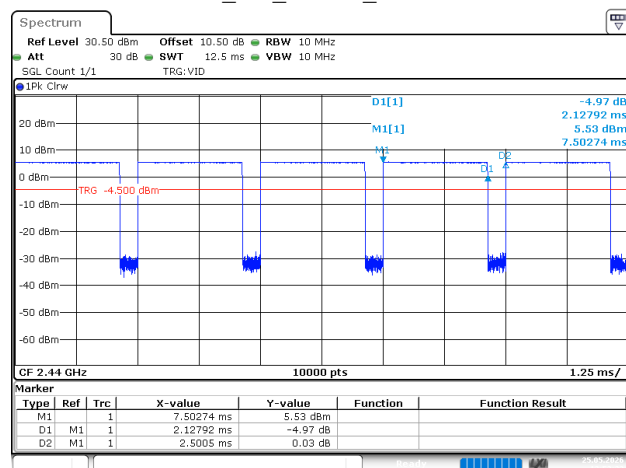
BLE_1M_Middle_Channel
