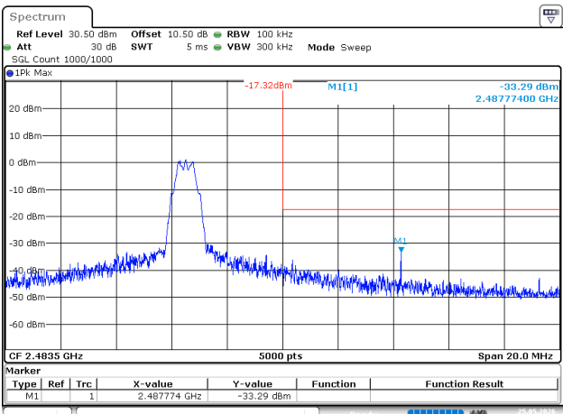
BLE_125kHz_High_Channel
