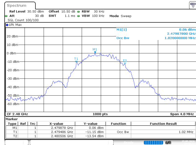
BLE_500kHz_High_Channel
