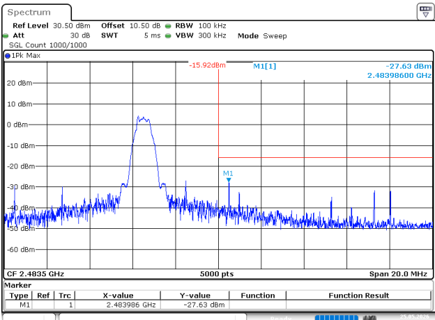
BLE_500kHz_High_Channel
