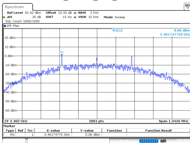
BLE_500kHz_Low_Channel
