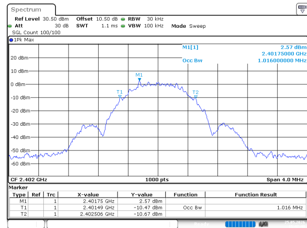
BLE_500kHz_Low_Channel
