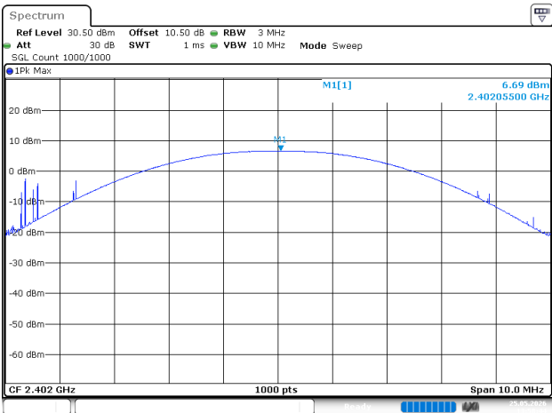
BLE_1M_Low_Channel
