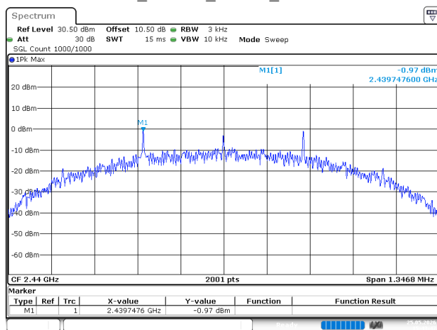
BLE_500kHz_Middle_Channel
