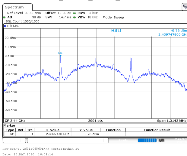
BLE_125kHz_Middle_Channel
