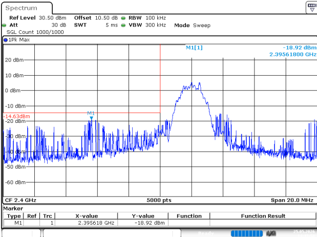
BLE_2M_Low_Channel
