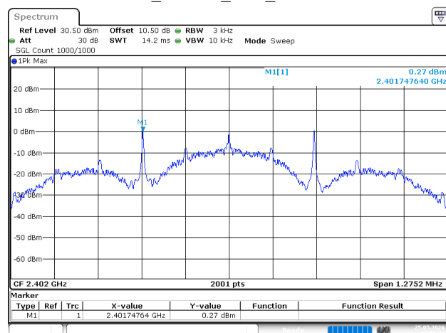
BLE_125kHz_Low_Channel
