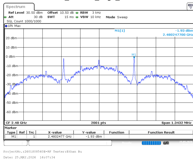
BLE_125kHz_High_Channel
