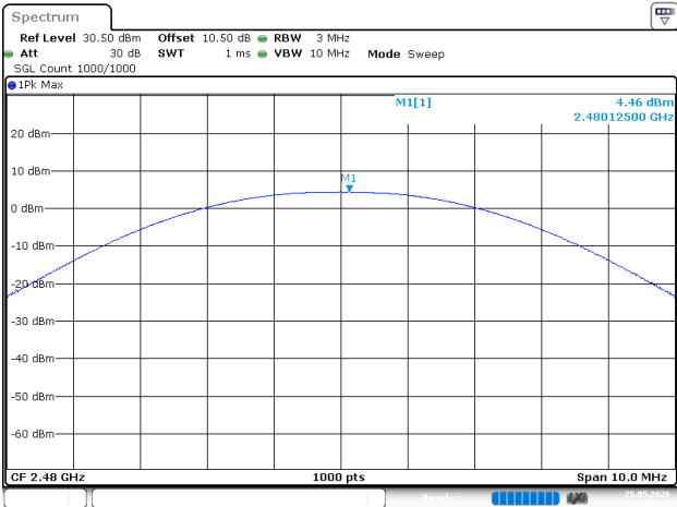
BLE_125kHz_High_Channel
