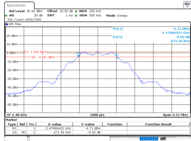
BLE_125kHz_High_Channel
