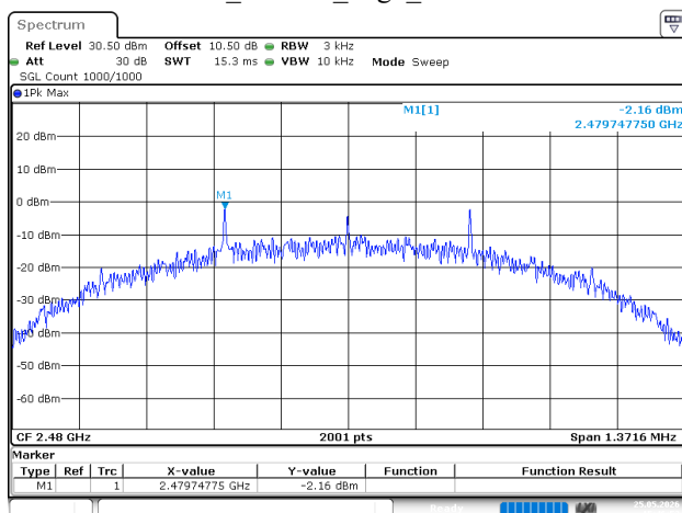
BLE_500kHz_High_Channel
