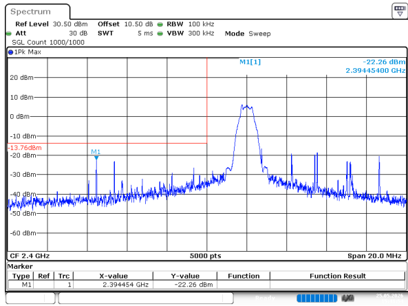
BLE_500kHz_Low_Channel
