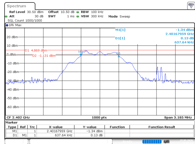
BLE_125kHz_Low_Channel
