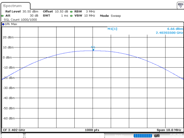
BLE_500kHz_Low_Channel
