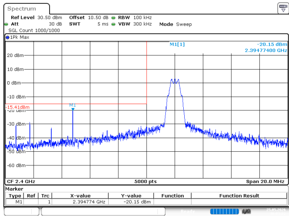
BLE_125kHz_Low_Channel
