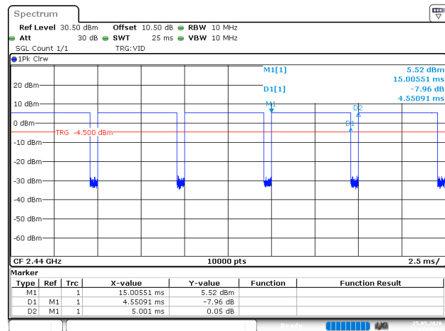
BLE_500kHz_Middle_Channel
