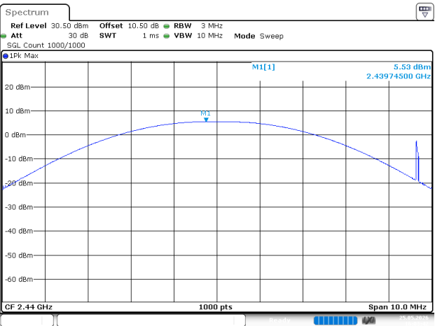
BLE_125kHz_Middle_Channel
