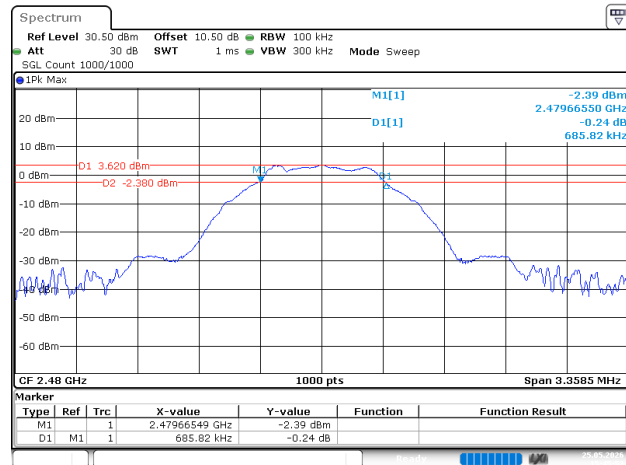
BLE_500kHz_High_Channel
