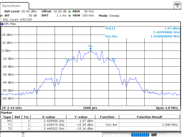
BLE_125kHz_Middle_Channel
