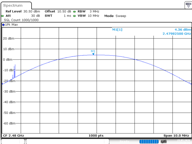
BLE_500kHz_High_Channel
