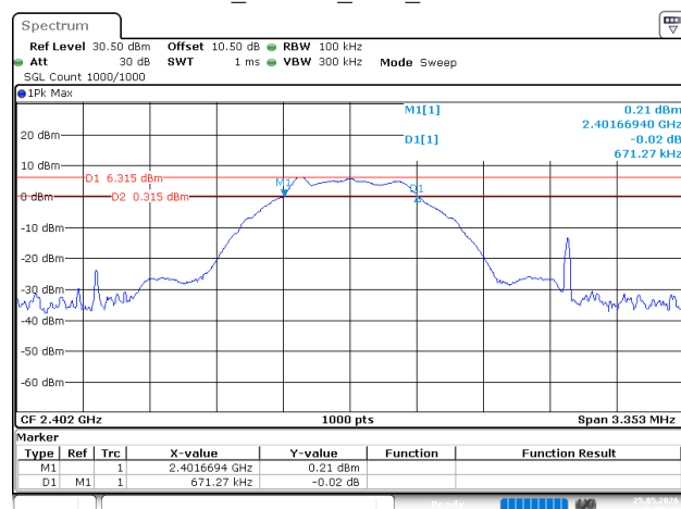
BLE_500kHz_Low_Channel
