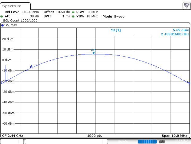
BLE_500kHz_Middle_Channel
