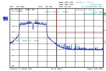
n40_2452MHz_Chain 0
