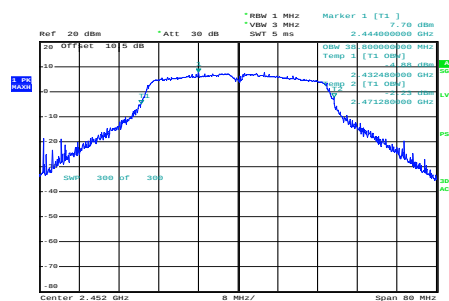
n40_2452MHz_Chain 0
