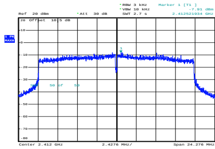
ax20_2412MHz_RU_Full_Chain 0
