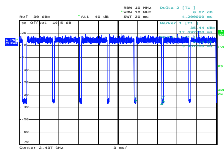
ax40_2437MHz_RU_Full_Chain 0
