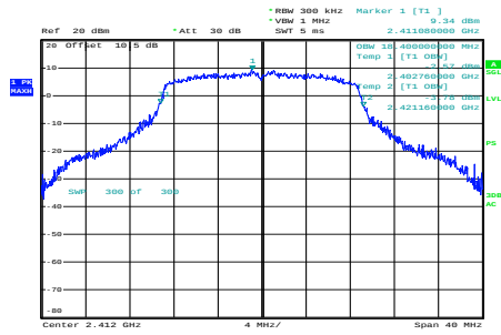
n20_2412MHz_Chain 0
