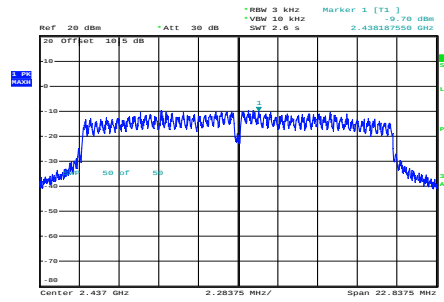
n20_2437MHz_Chain 0
