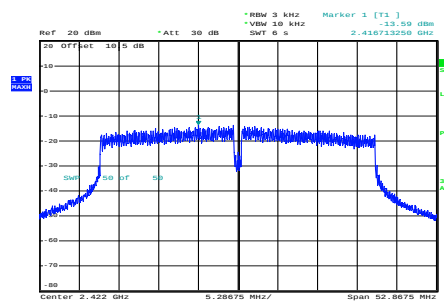
n40_2422MHz_Chain 0
