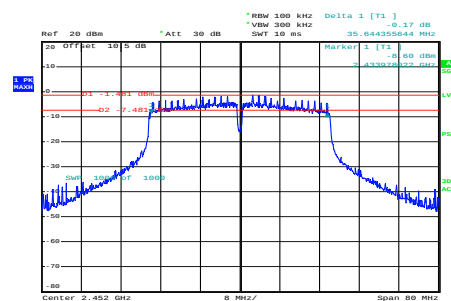
n40_2452MHz_Chain 0
