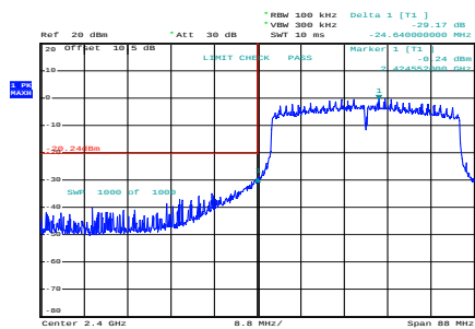
ax40_2422MHz_RU_Full_Chain 0
