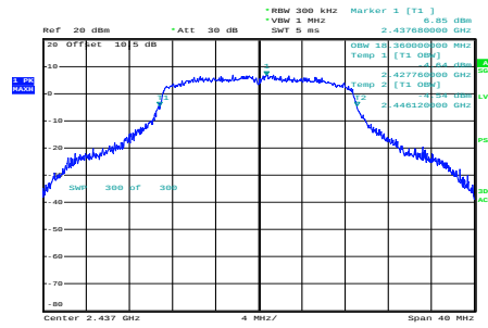
n20_2437MHz_Chain 0
