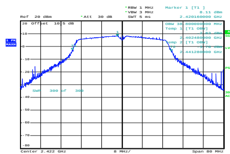
n40_2422MHz_Chain 0
