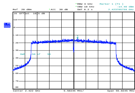
ax40_2422MHz_RU_Full_Chain 0
