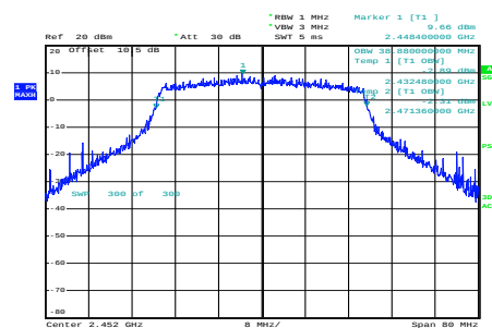
ax40_2452MHz_RU_Full_Chain 0
