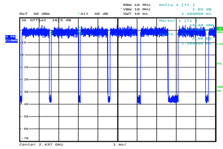
g_2437MHz_Chain 0
