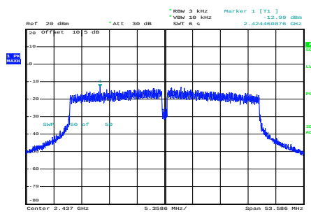
n40_2437MHz_Chain 0
