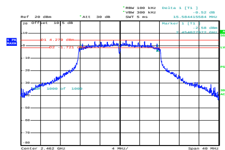
g_2462MHz_Chain 0
