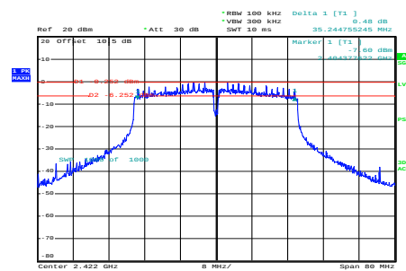
n40_2422MHz_Chain 0
