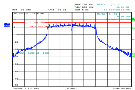
g_2412MHz_Chain 0
