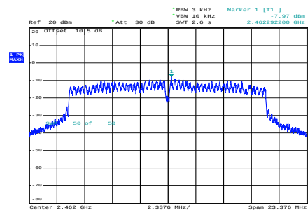
g_2462MHz_Chain 0
