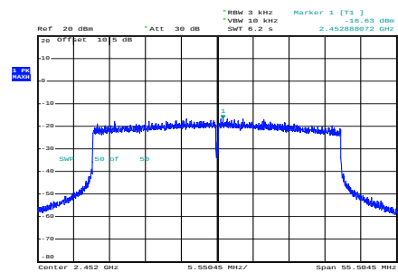
ax40_2452MHz_RU_Full_Chain 0
