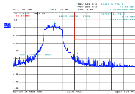
ax20_2462MHz_RU_Full_Chain 0
