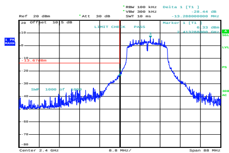
n20_2412MHz_Chain 0
