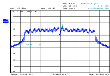
g_2412MHz_Chain 0
