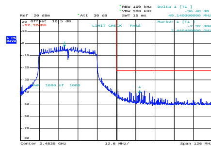
ax40_2452MHz_RU_Full_Chain 0
