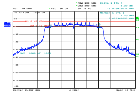
ax20_2437MHz_RU_Full_Chain 0
