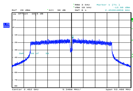
n40_2452MHz_Chain 0
