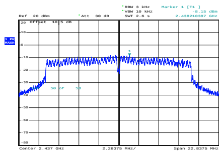
g_2437MHz_Chain 0
