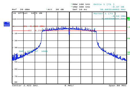
ax40_2422MHz_RU_Full_Chain 0
