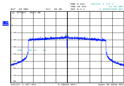
ax40_2437MHz_RU_Full_Chain 0
