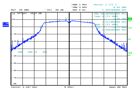
n40_2437MHz_Chain 0
