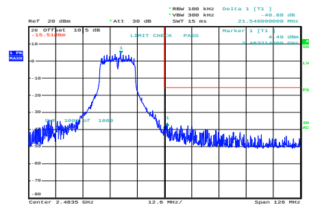
g_2462MHz_Chain 0
