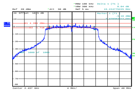
n20_2437MHz_Chain 0
