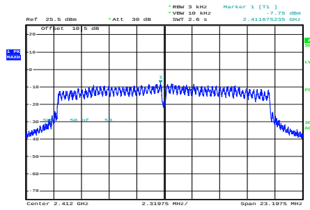
n20_2412MHz_Chain 0
