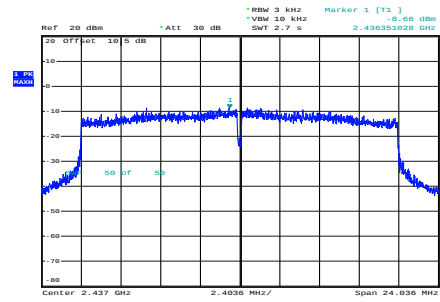
ax20_2437MHz_RU_Full_Chain 0
