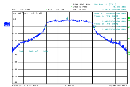
g_2412MHz_Chain 0
