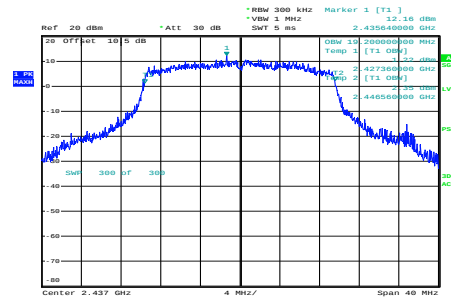
ax20_2437MHz_RU_Full_Chain 0
