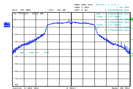
g_2462MHz_Chain 0
