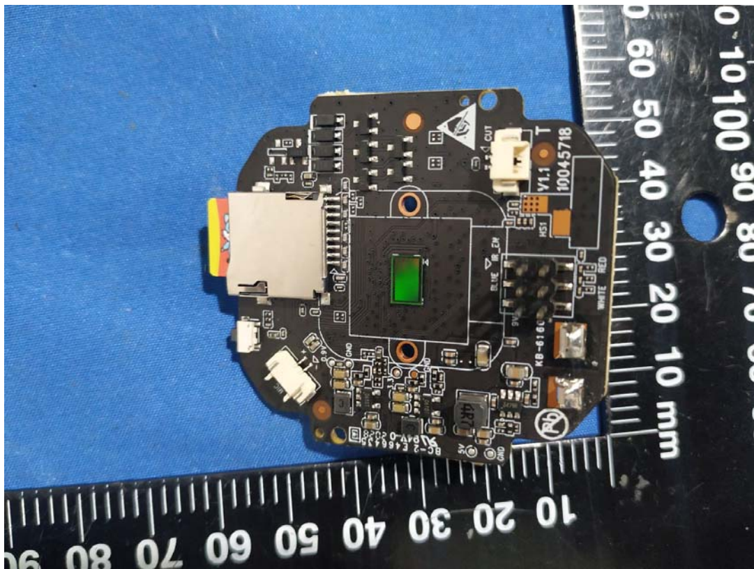
Antenna Board
