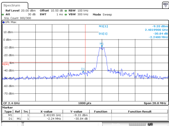
BLE_125K_Low_Channel
