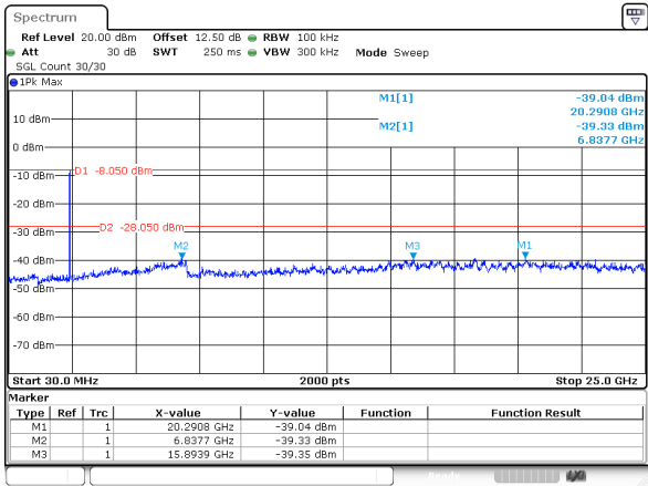
BLE_125K_Middle_Channel
