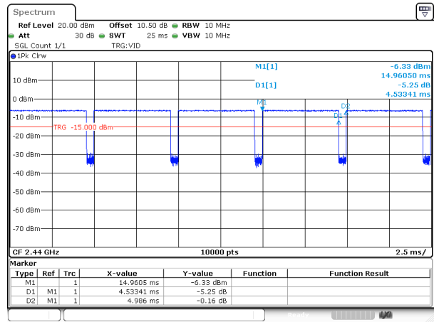
BLE_500K_Middle_Channel
