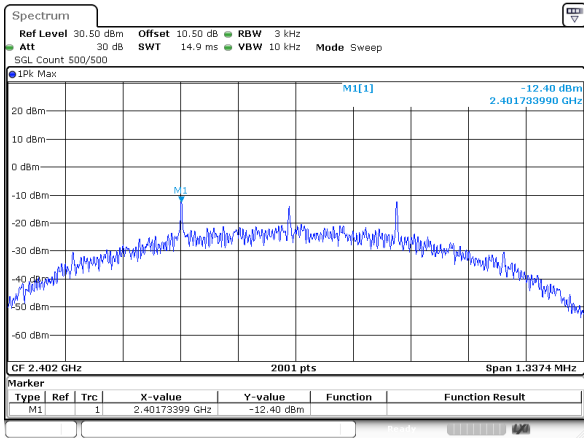
BLE_500K_Low_Channel
