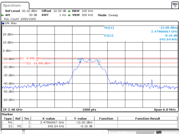
BLE_125K_High_Channel
