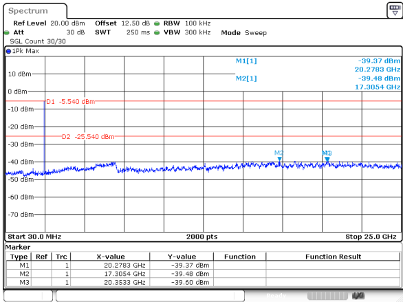
BLE_500K_High_Channel
