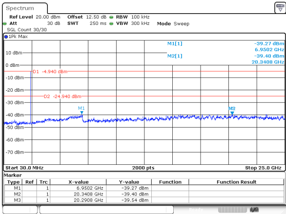
BLE_500K_Low_Channel
