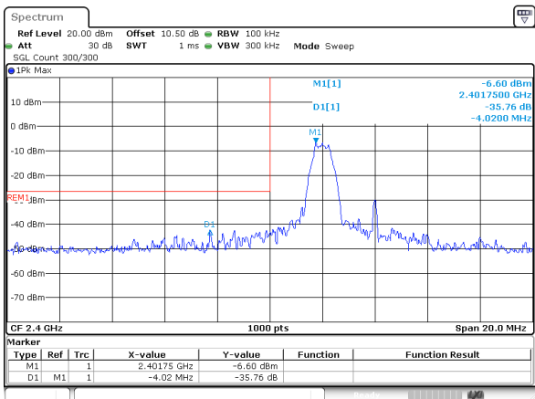
BLE_500K_Low_Channel
