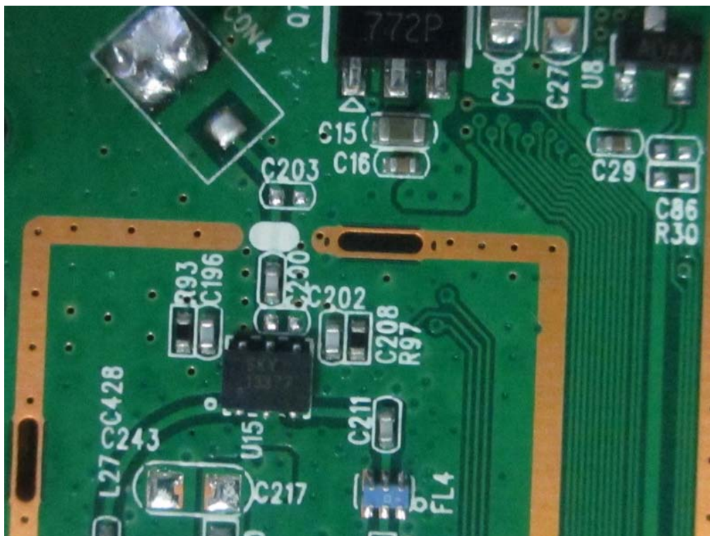
Antenna connector
