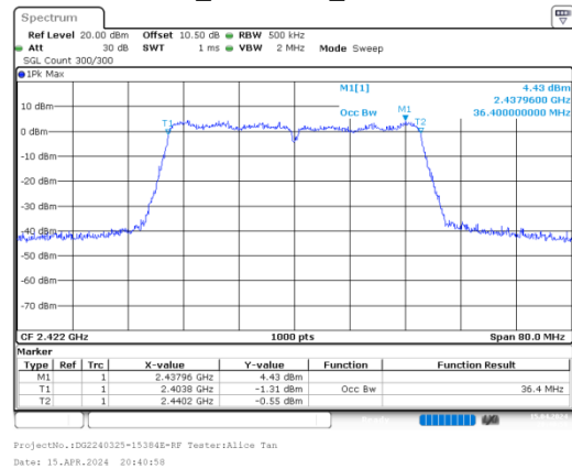
n40_2422MHz_Chain 0
