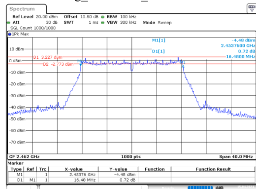
g_2462MHz_Chain 1
