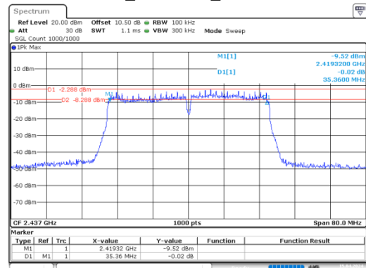
n40_2437MHz_Chain 1
