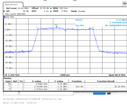
n40 2452MHz Chain 0
