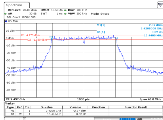
g_2437MHz_Chain 1
