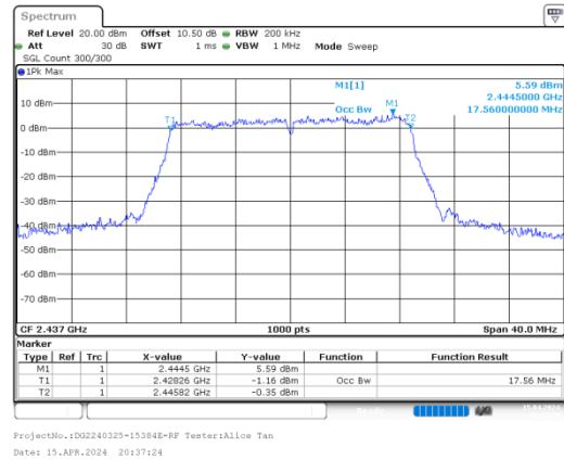
n20_2437MHz_Chain 0
