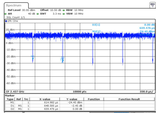
n40_2437MHz_Chain 0
