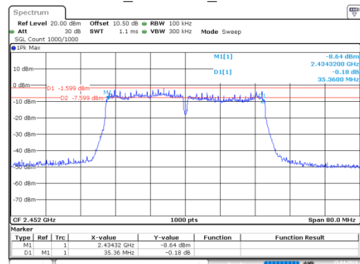
n40_2452MHz_Chain 1
