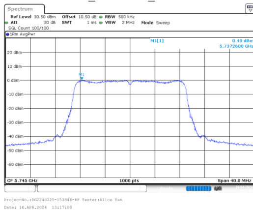
ac20_5745MHz_Chain 0
