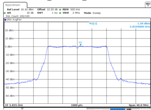
a_5825MHz_Chain 1
