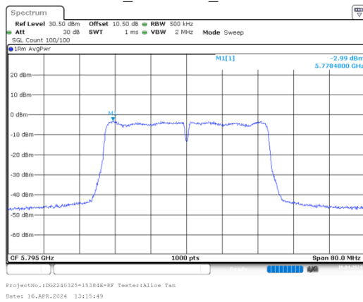
n40_5795MHz_Chain 0
