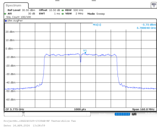
ac80_5775MHz_Chain 1
