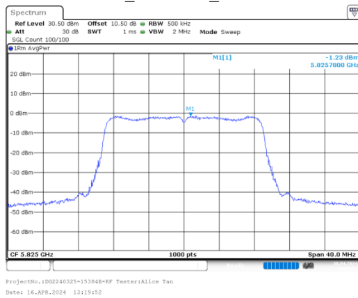
ac20_5825MHz_Chain 0
