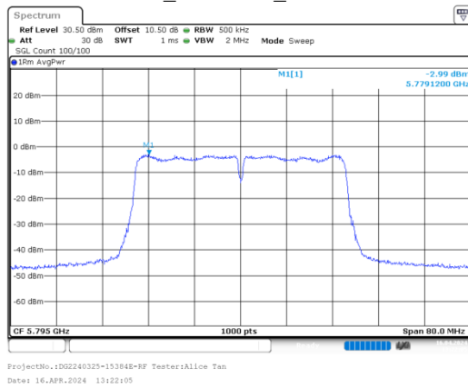
ac40_5795MHz_Chain 0
