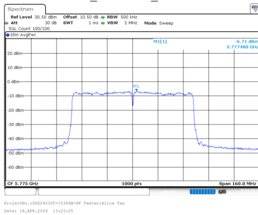
ac80_5775MHz_Chain 0
