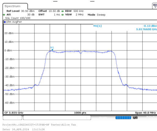
n20_5825MHz_Chain 0
