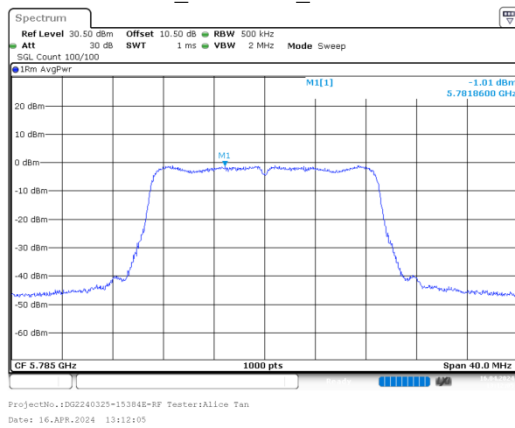
n20_5785MHz_Chain 0
