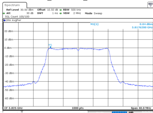
a_5825MHz_Chain 0
