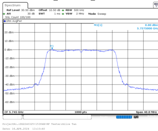
n20_5745MHz_Chain 0
