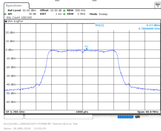
n20_5785MHz_Chain 1
