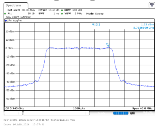
ac20_5745MHz_Chain 1
