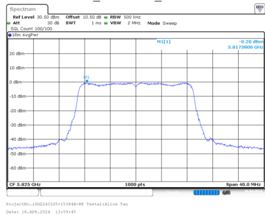
ac20_5825MHz_Chain 1
