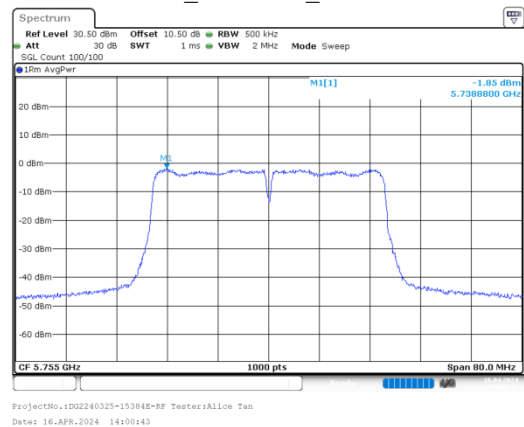
ac40_5755MHz_Chain 1
