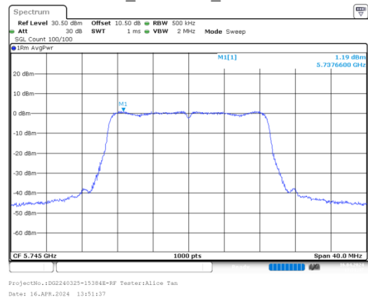
n20_5745MHz_Chain 1
