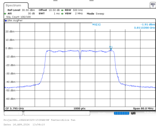
n40_5795MHz_Chain 1
