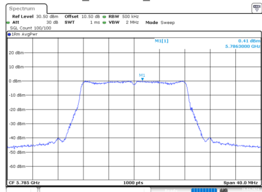
a_5785MHz_Chain 1
