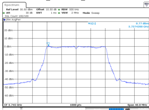
a_5745MHz_Chain 0
