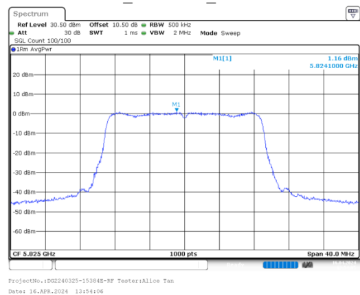
n20_5825MHz_Chain 1
