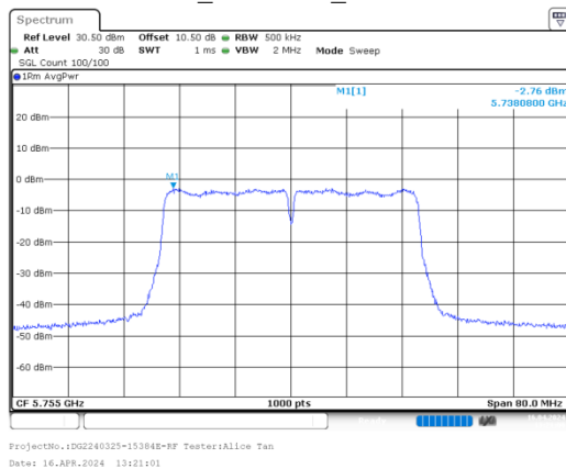
ac40_5755MHz_Chain 0
