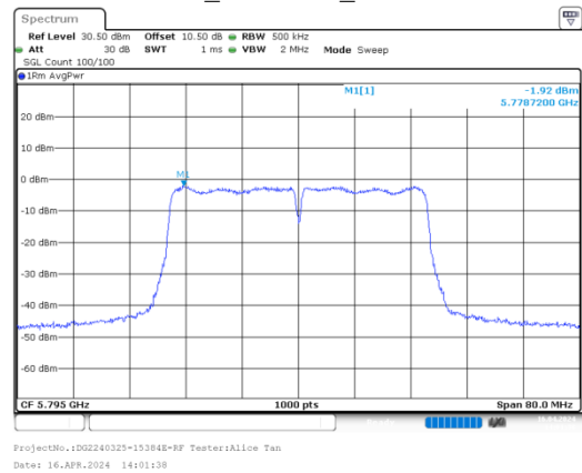
ac40_5795MHz_Chain 1
