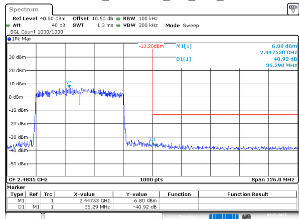
802.11ax40_2452MHz_RU_Full_Chain 0
