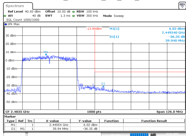
802.11ax40_2452MHz_RU_Full_Chain 1
