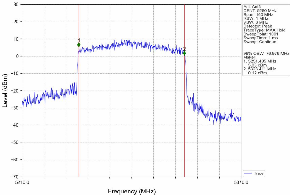
802.11ax(HEW80)_MCH_5290MHz_SU_ / _Ant3_NTNV
