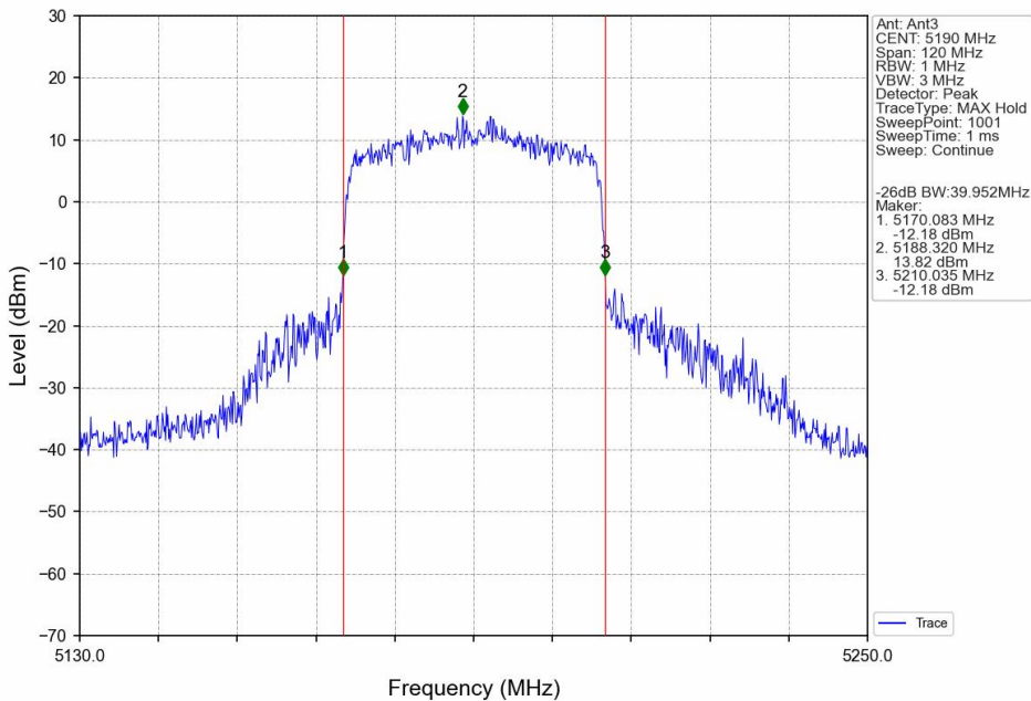
802.11ax(HEW40)_LCH_5190MHz_SU_/_Ant3_NTNV
