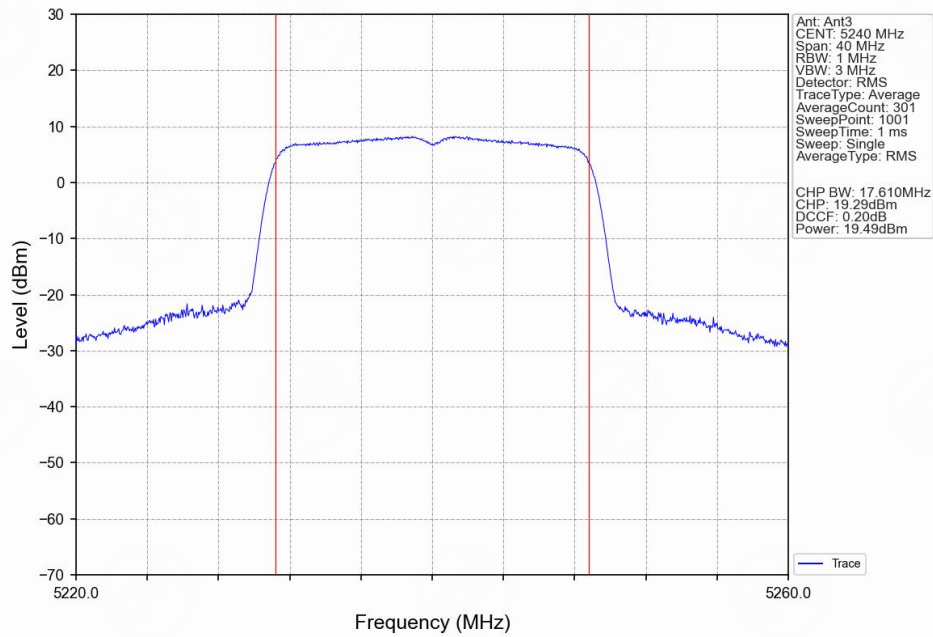
802.11n(HT20)_HCH_5240MHz_Ant3_NTNV
