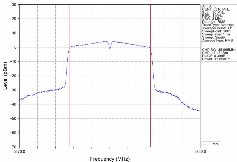
802.11n(HT40)_HCH_5310MHz_Ant3_NTNV
