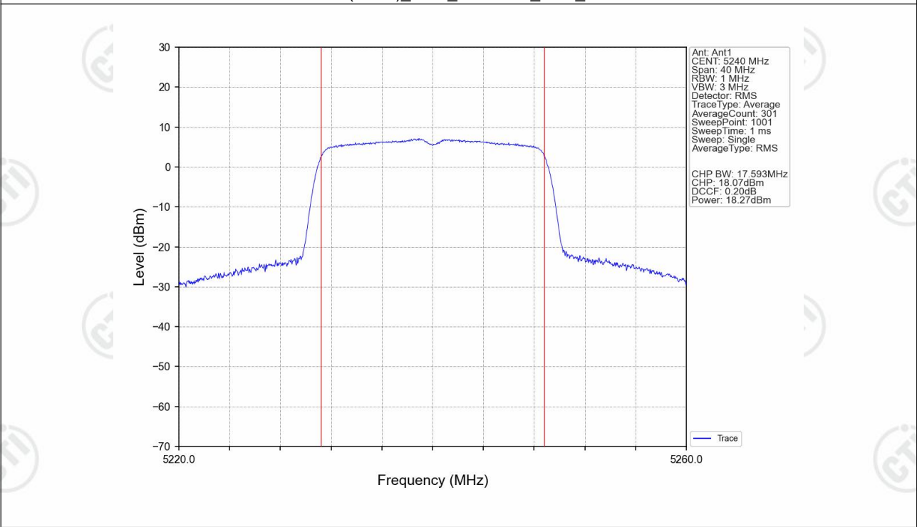
802.11n(HT20)_HCH_5240MHz_Ant1_NTNV
