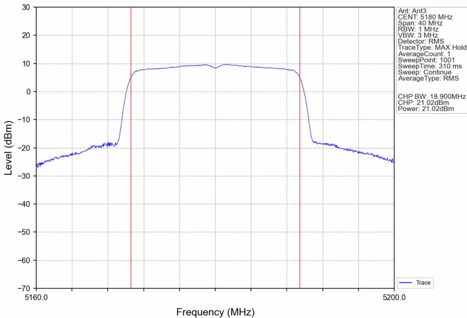
802.11ax(HEW20)_LCH_5180MHz_SU_ / _Ant3_NTNV
