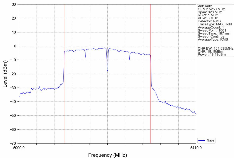
802.11ac(VHT160)_MCH_5250MHz_Ant2_NTNV
