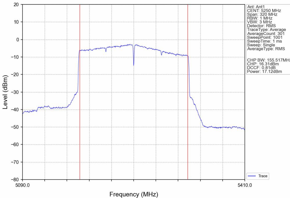
802.11ax(HEW160)_MCH_5250MHz_SU_ / _Ant1_NTNV
