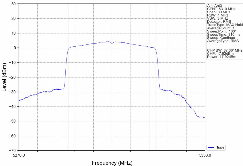
802.11ax(HEW40)_HCH_5310MHz_SU_/_Ant3_NTNV
