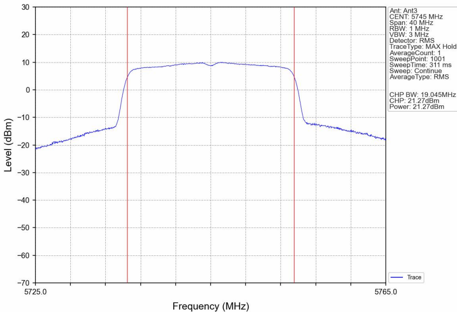
802.11ax(HEW20)_LCH_5745MHz_SU_ / _Ant3_NTNV
