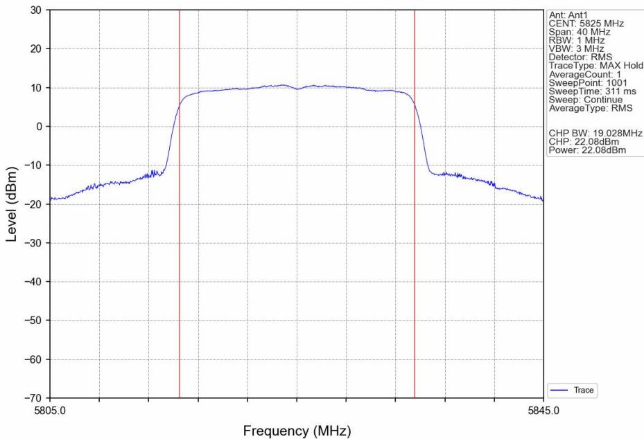
802.11ax(HEW20)_HCH_5825MHz_SU_/_Ant1_NTNV
