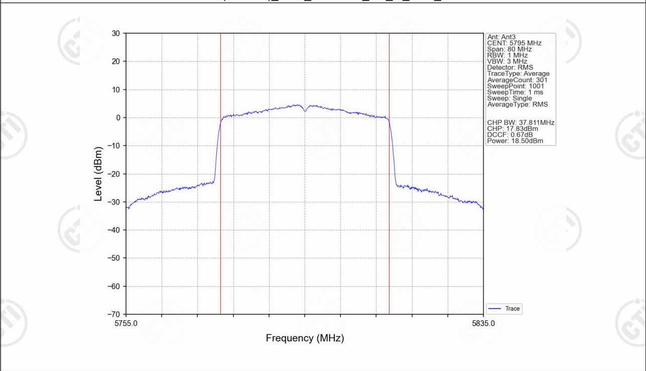
802.11ax(HEW40)_HCH_5795MHz_SU_/_Ant3_NTNV
