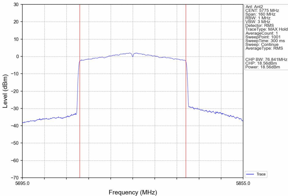
802.11ax(HEW80)_MCH_5775MHz_SU_ / _Ant2_NTNV
