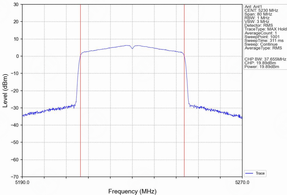
802.11ax(HEW40)_HCH_5230MHz_SU_/_Ant1_NTNV
