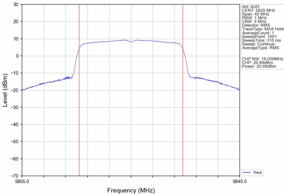
802.11ax(HEW20)_HCH_5825MHz_SU_/_Ant3_NTNV
