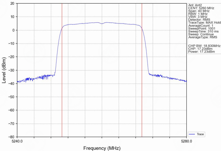
802.11ax(HEW20)_LCH_5260MHz_SU_ / _Ant2_NTNV
