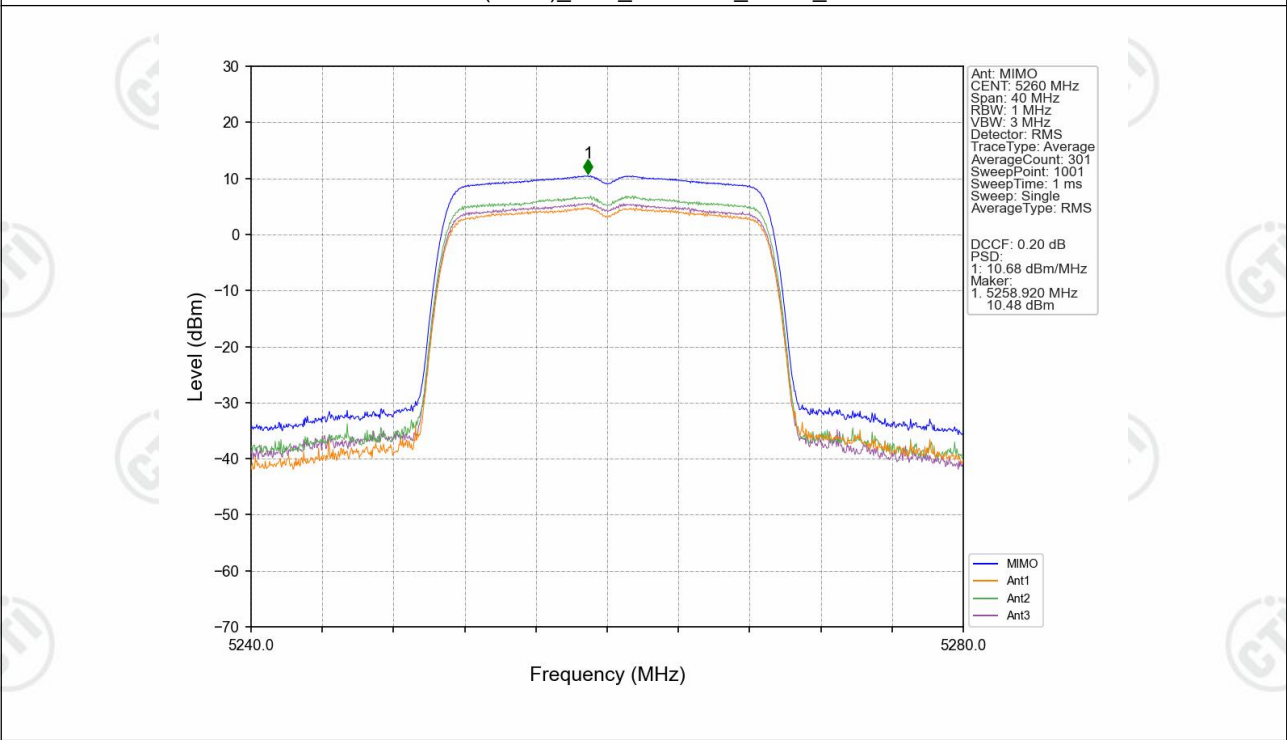
802.11n(HT20)_LCH_5260MHz_MIMO_NTNV
