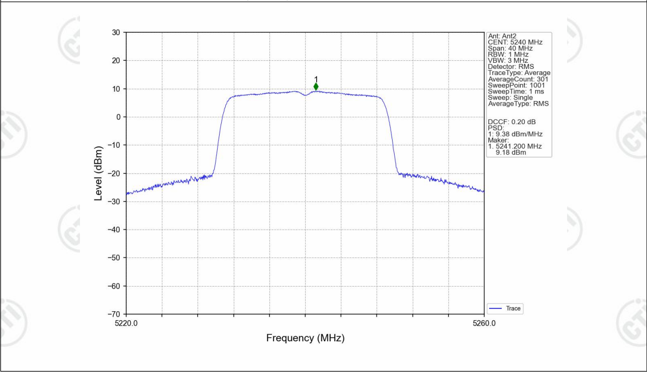
802.11ac(VHT20)_HCH_5240MHz_Ant2_NTNV
