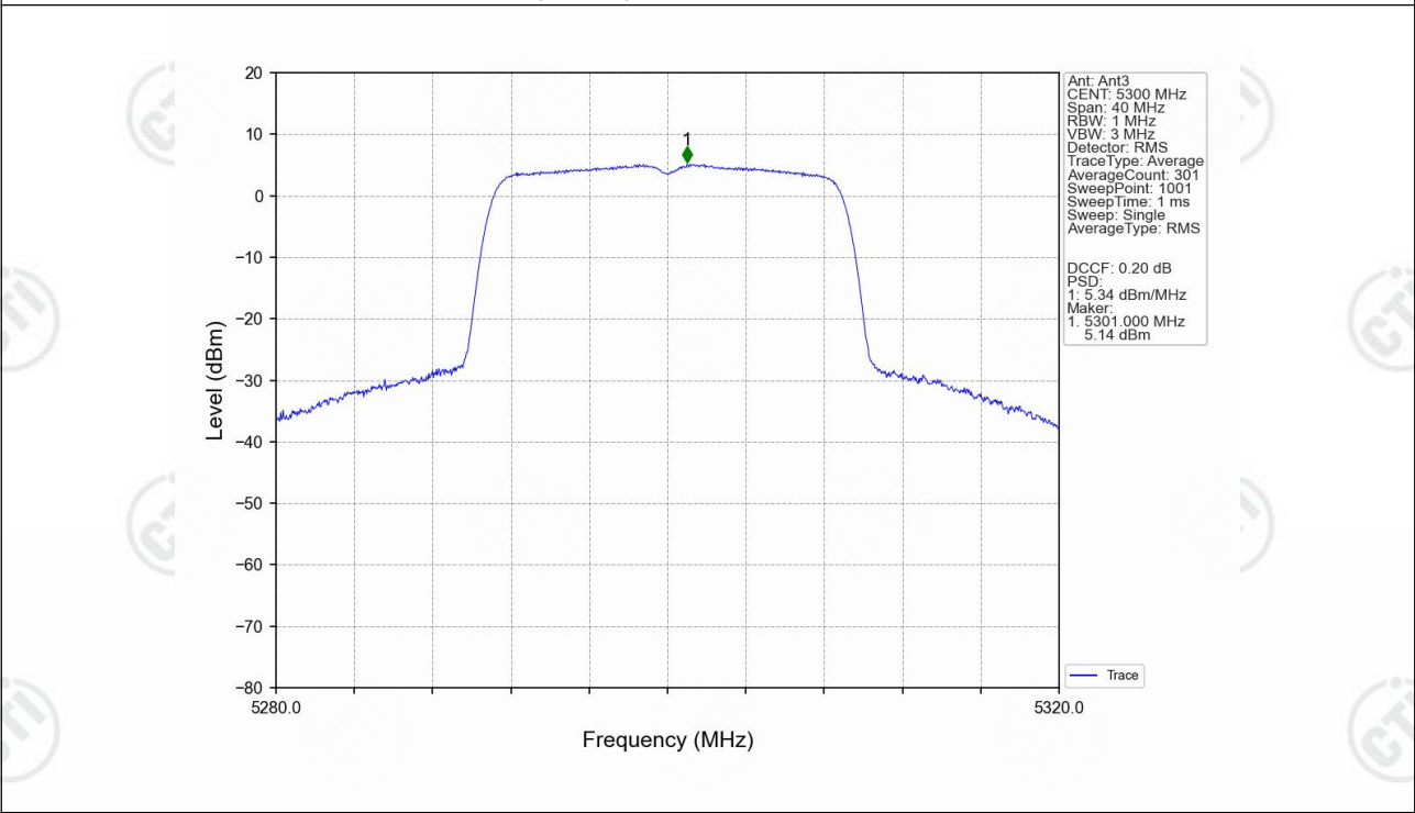
802.11ac(VHT20)_MCH_5300MHz_MIMO_NTNV
