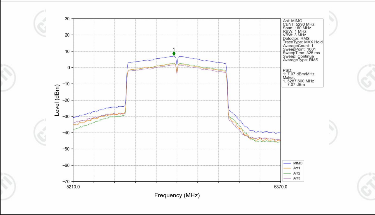
802.11ac(VHT80)_MCH_5290MHz_MIMO_NTNV
