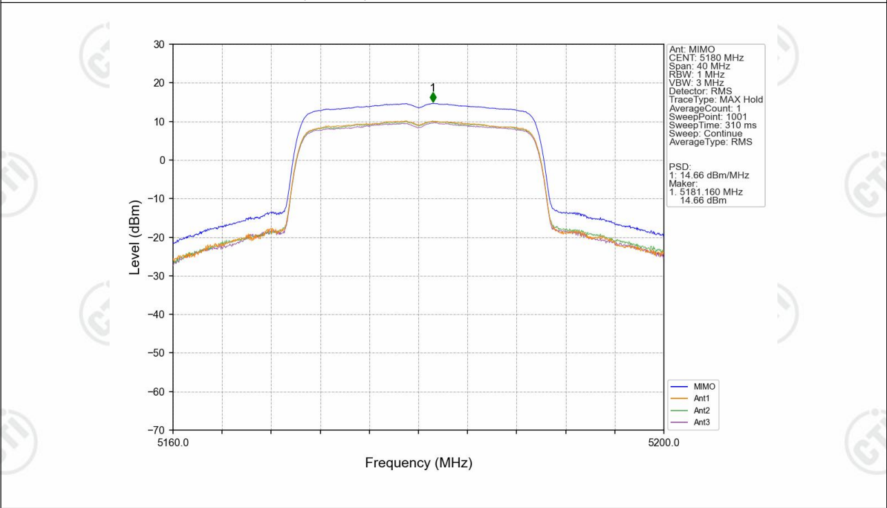
802.11ax(HEW20)_LCH_5180MHz_SU_/_MIMO_NTNV
