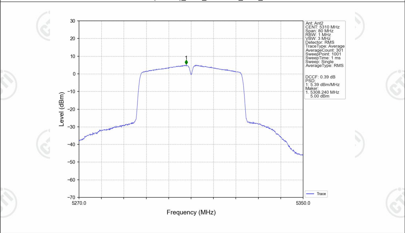
802.11ac(VHT40)_HCH_5310MHz_Ant2_NTNV
