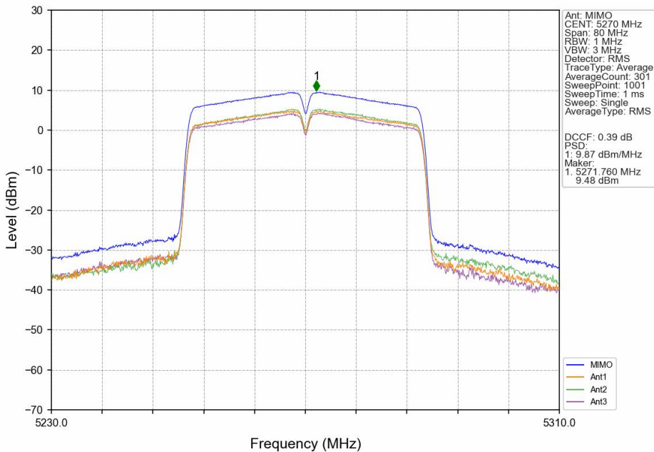
802.11ac(VHT40)_LCH_5270MHz_MIMO_NTNV
