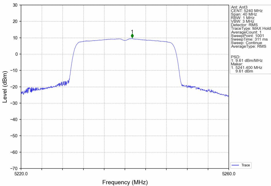
802.11ax(HEW20)_HCH_5240MHz_SU_/_MIMO_NTNV
