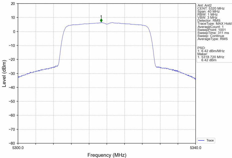
802.11ax(HEW20)_HCH_5320MHz_SU_/_Ant2_NTNV
