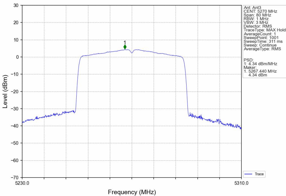
802.11ax(HEW40)_LCH_5270MHz_SU_/_MIMO_NTNV
