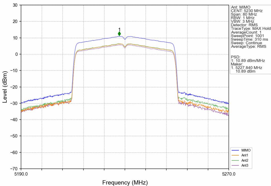
802.11ax(HEW40)_HCH_5230MHz_SU_/_MIMO_NTNV
