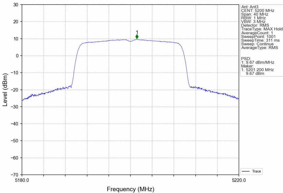
802.11ax(HEW20)_MCH_5200MHz_SU_/_MIMO_NTNV
