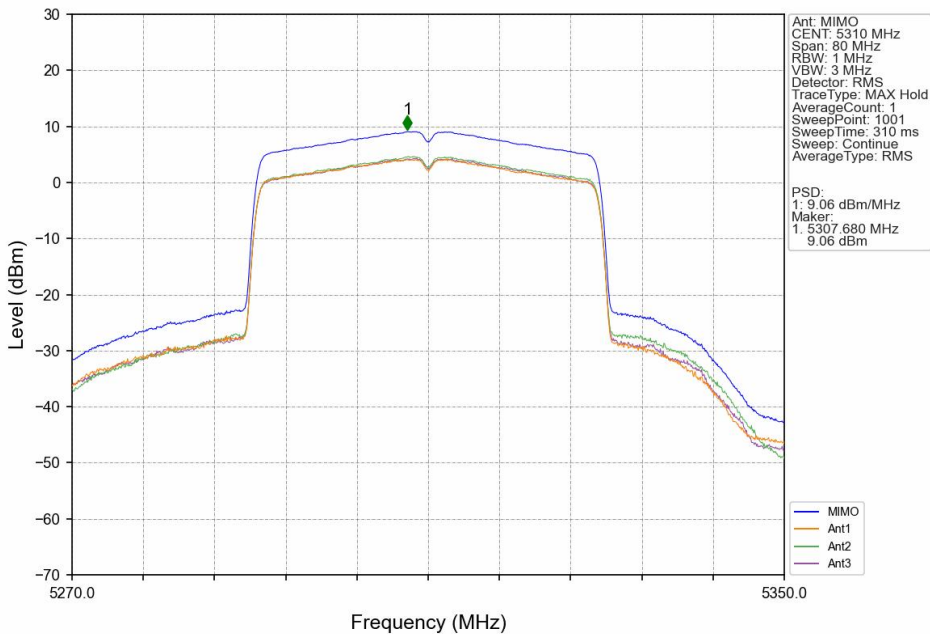
802.11ax(HEW40)_HCH_5310MHz_SU_/_MIMO_NTNV
