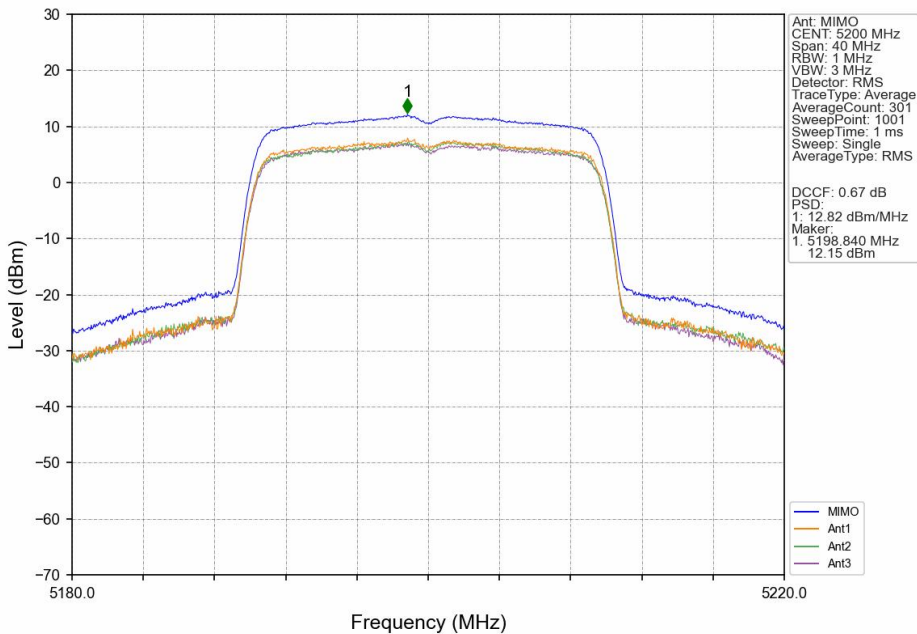
802.11be(EHT20)_MCH_5200MHz_SU_/_MIMO_NTNV
