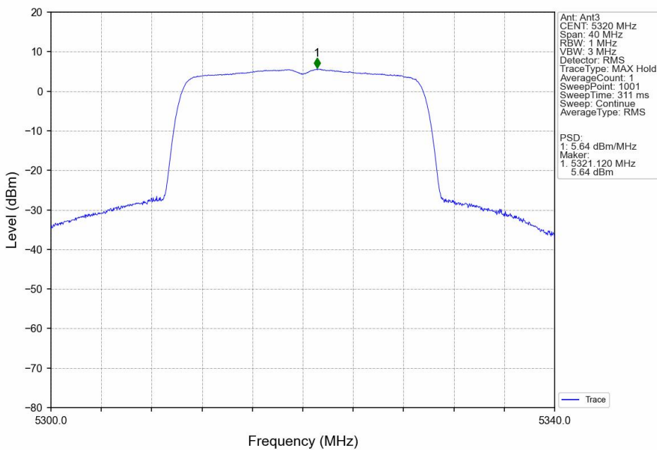
802.11ax(HEW20)_HCH_5320MHz_SU_/_MIMO_NTNV
