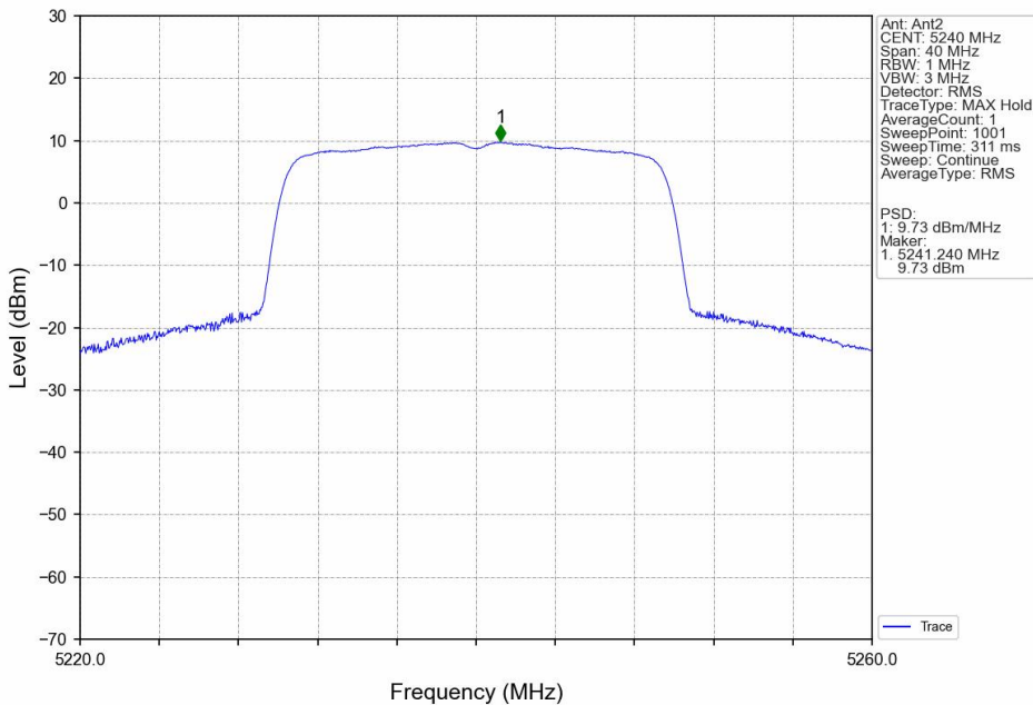
802.11ax(HEW20)_HCH_5240MHz_SU_/_Ant2_NTNV
