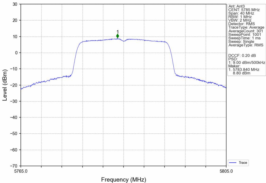
802.11ac(VHT20)_MCH_5785MHz_Ant3_NTNV
