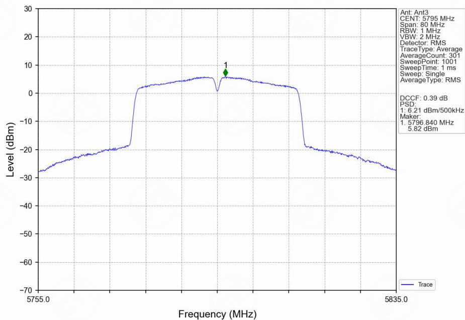
802.11n(HT40)_HCH_5795MHz_Ant3_NTNV
