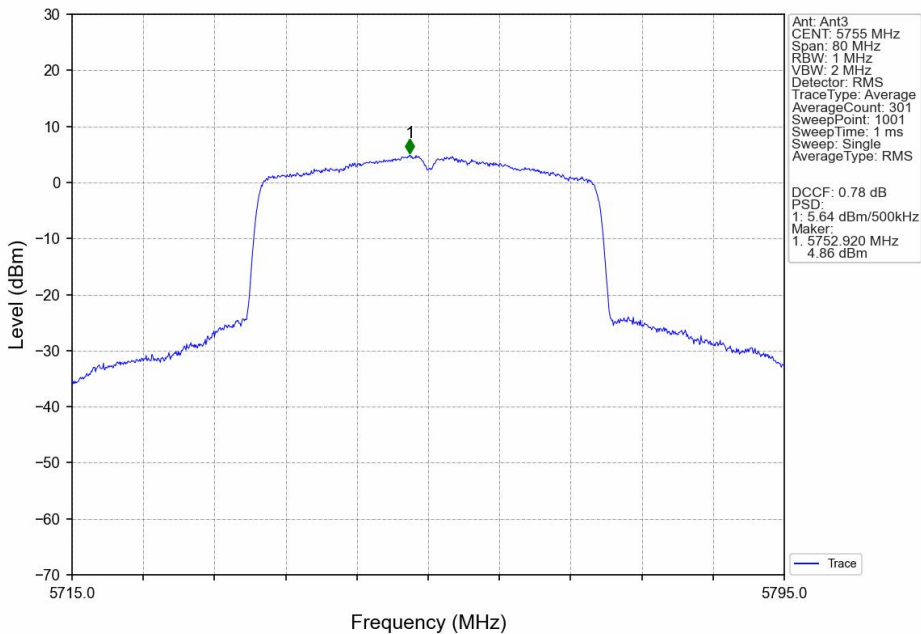
802.11ax(HEW40)_LCH_5755MHz_SU_/_Ant3_NTNV
