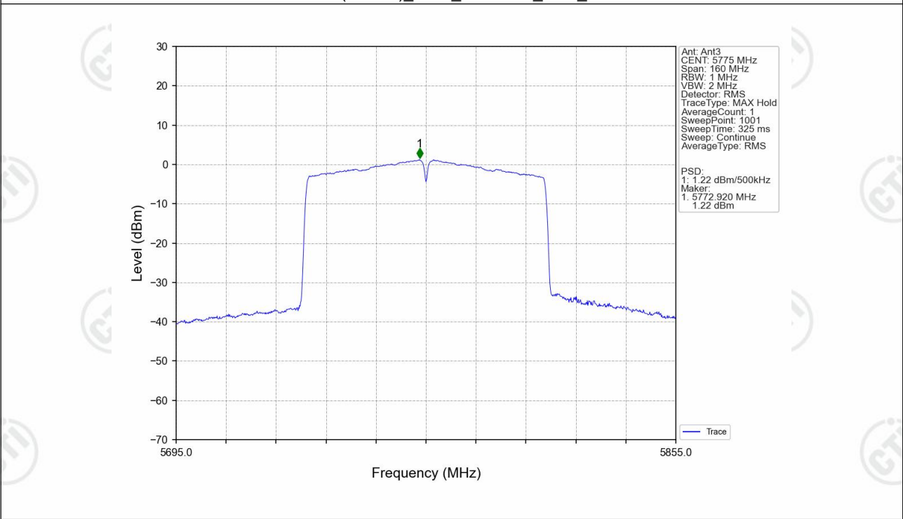
802.11ac(VHT80)_MCH_5775MHz_Ant3_NTNV
