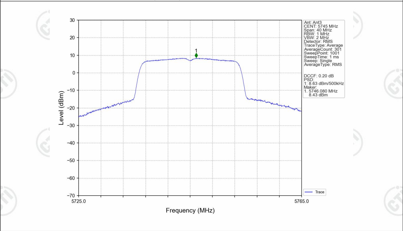
802.11ac(VHT20)_LCH_5745MHz_Ant3_NTNV
