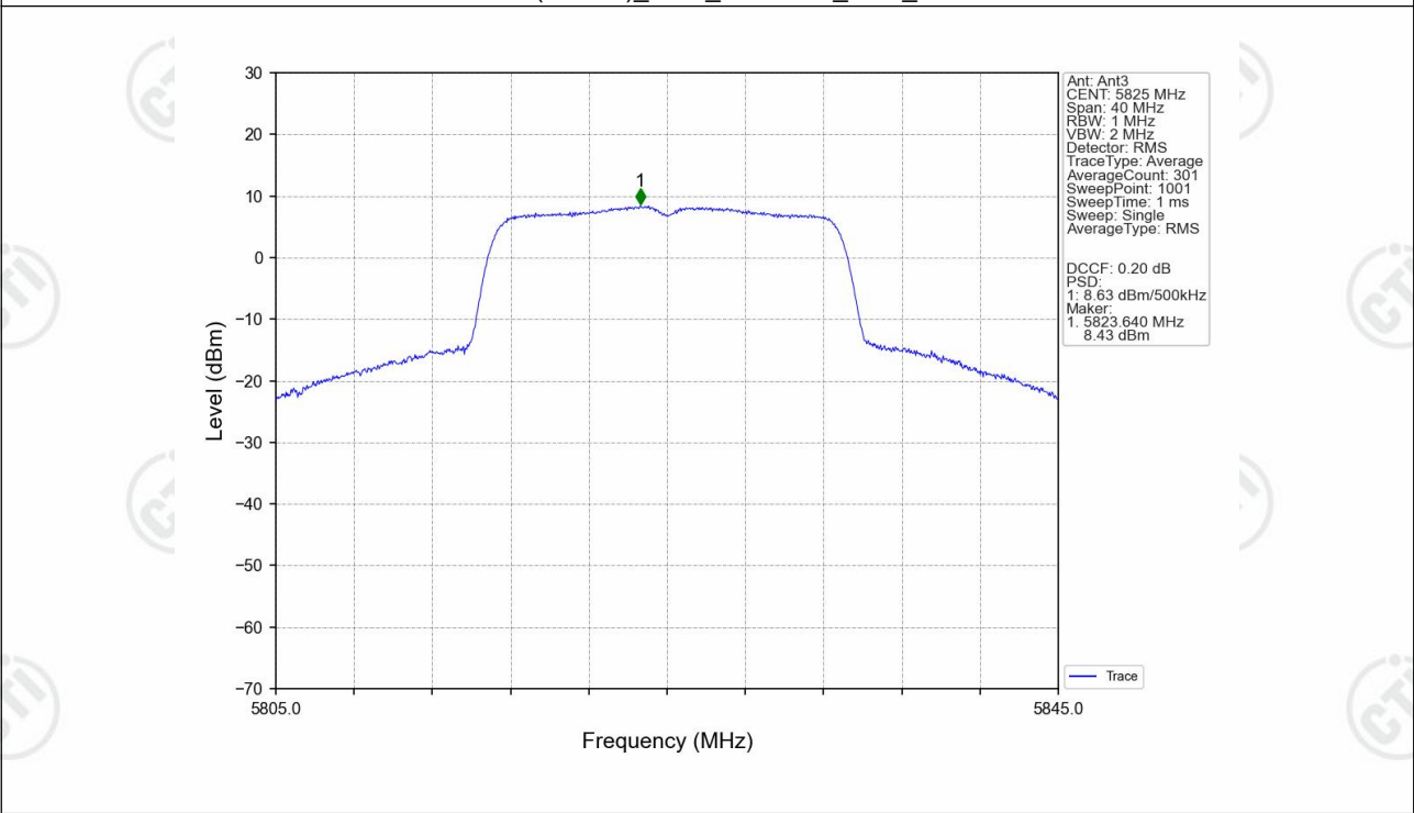
802.11ac(VHT20)_HCH_5825MHz_Ant3_NTNV
