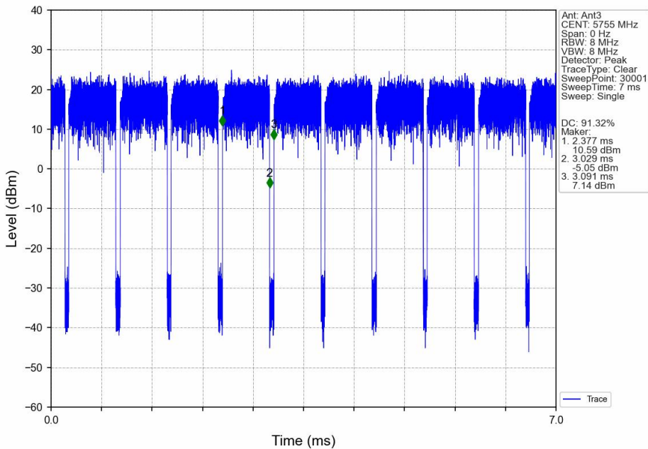
802.11ac(VHT40)_LCH_5755MHz_Ant3_NTNV
