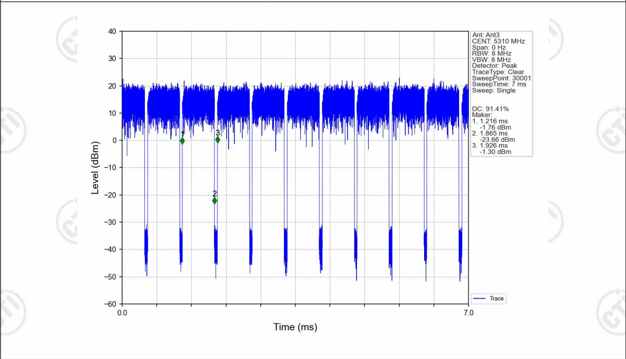
802.11n(HT40)_HCH_5310MHz_Ant3_NTNV
