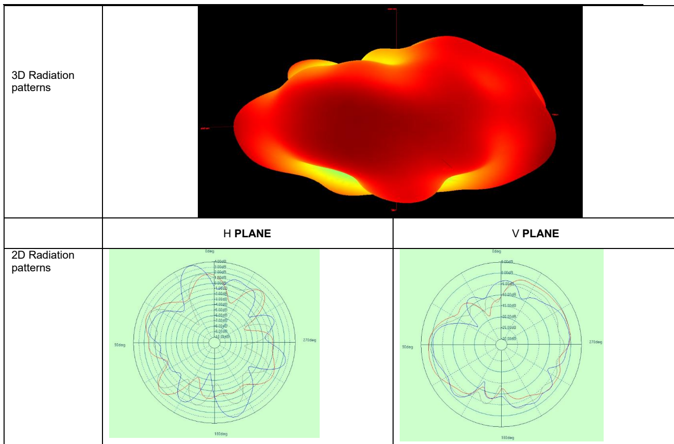
Directional diagram for 5GHz Antenna5
