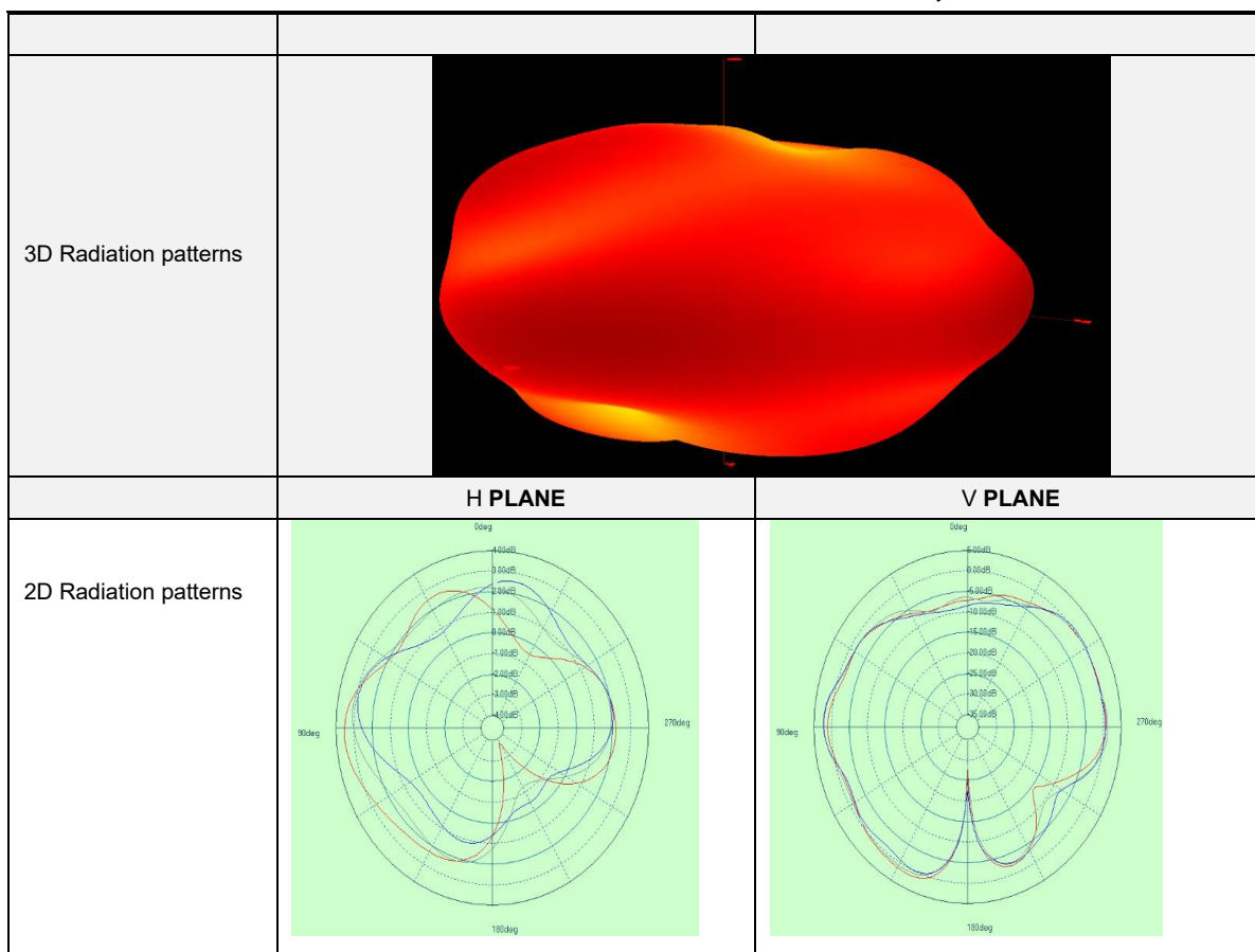
Directional diagram for 5GHz Antenna3
