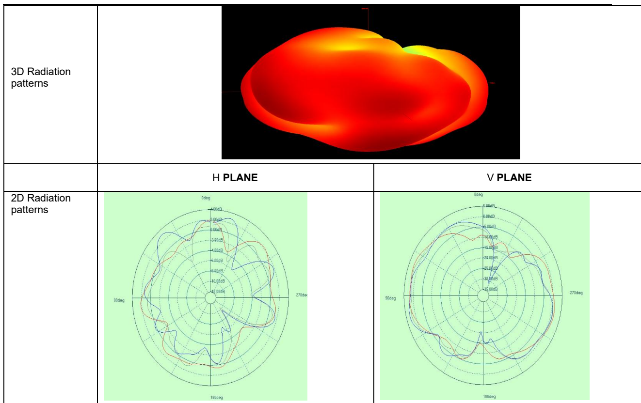
Directional diagram for 5GHz Antenna4
