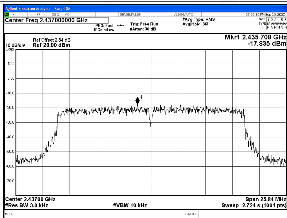
PSD NVNT be20 2437MHz Ant2
