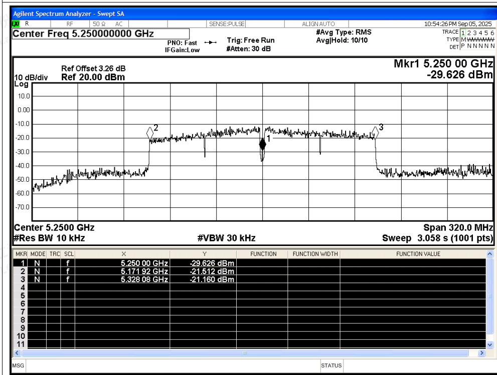
Freq. Stability NVNT ax160 5250MHz Ant5
