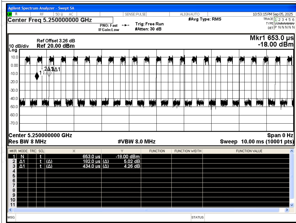
Duty Cycle NVNT ax160 5250MHz Ant5
