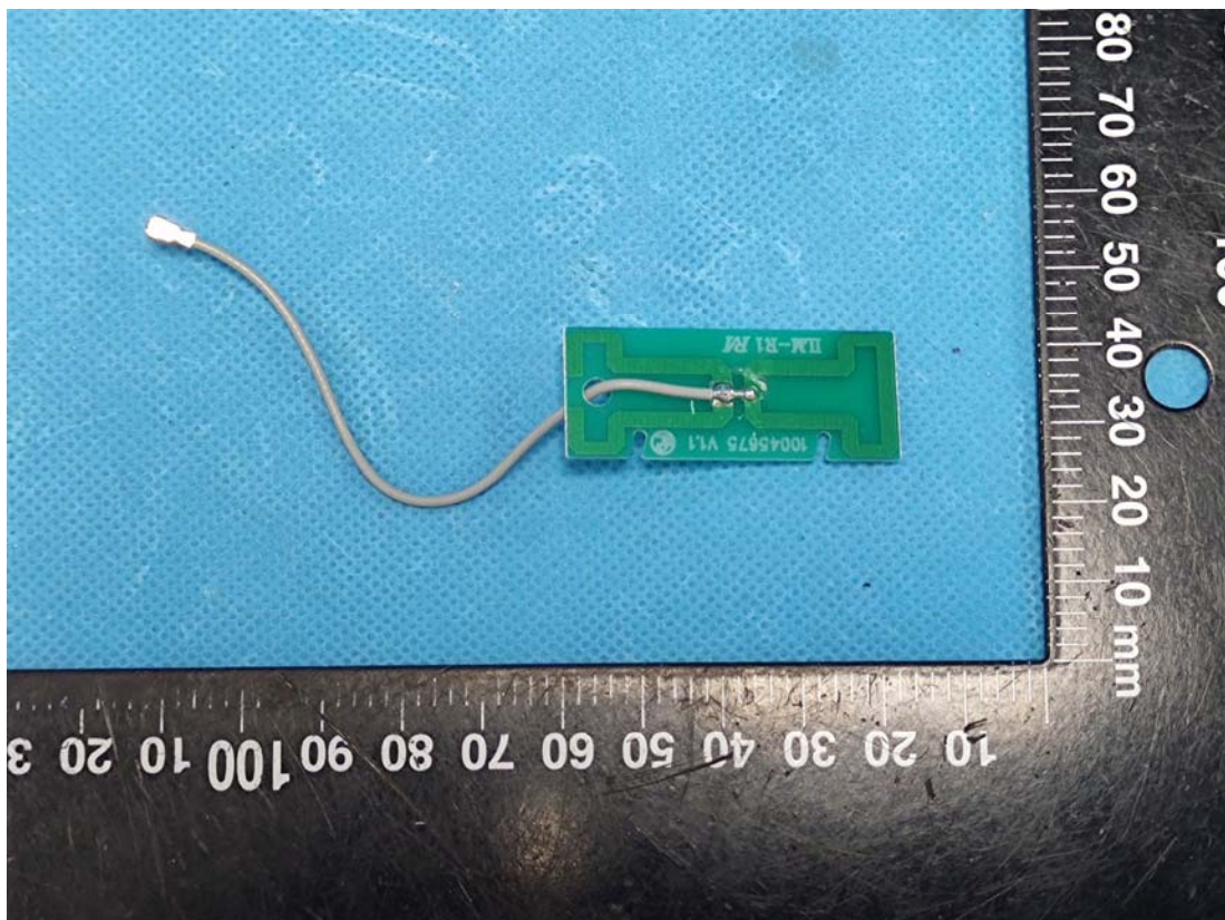
2.4GHz Antenna Chain 1
