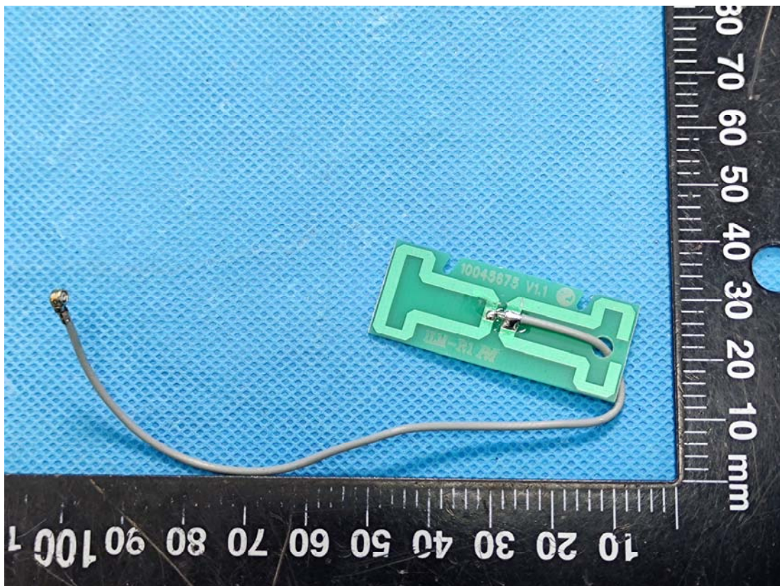
2.4G Antenna Chain 1
