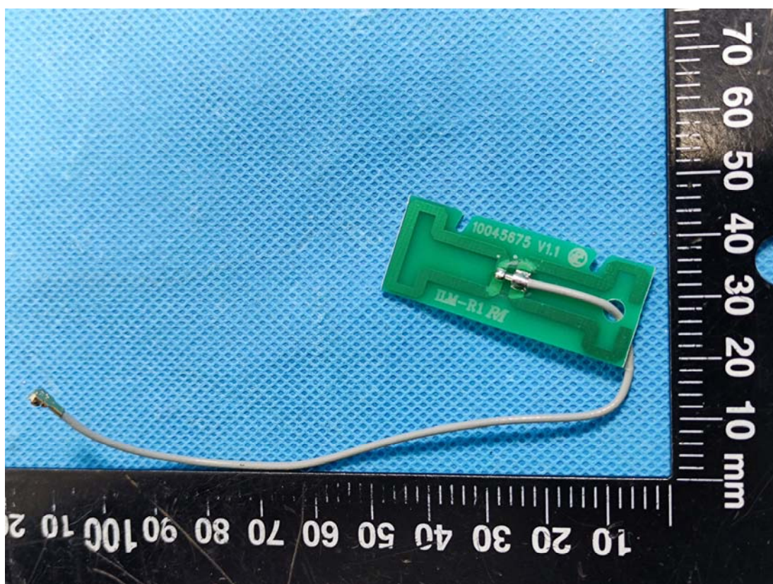
2.4G Antenna Chain 0
