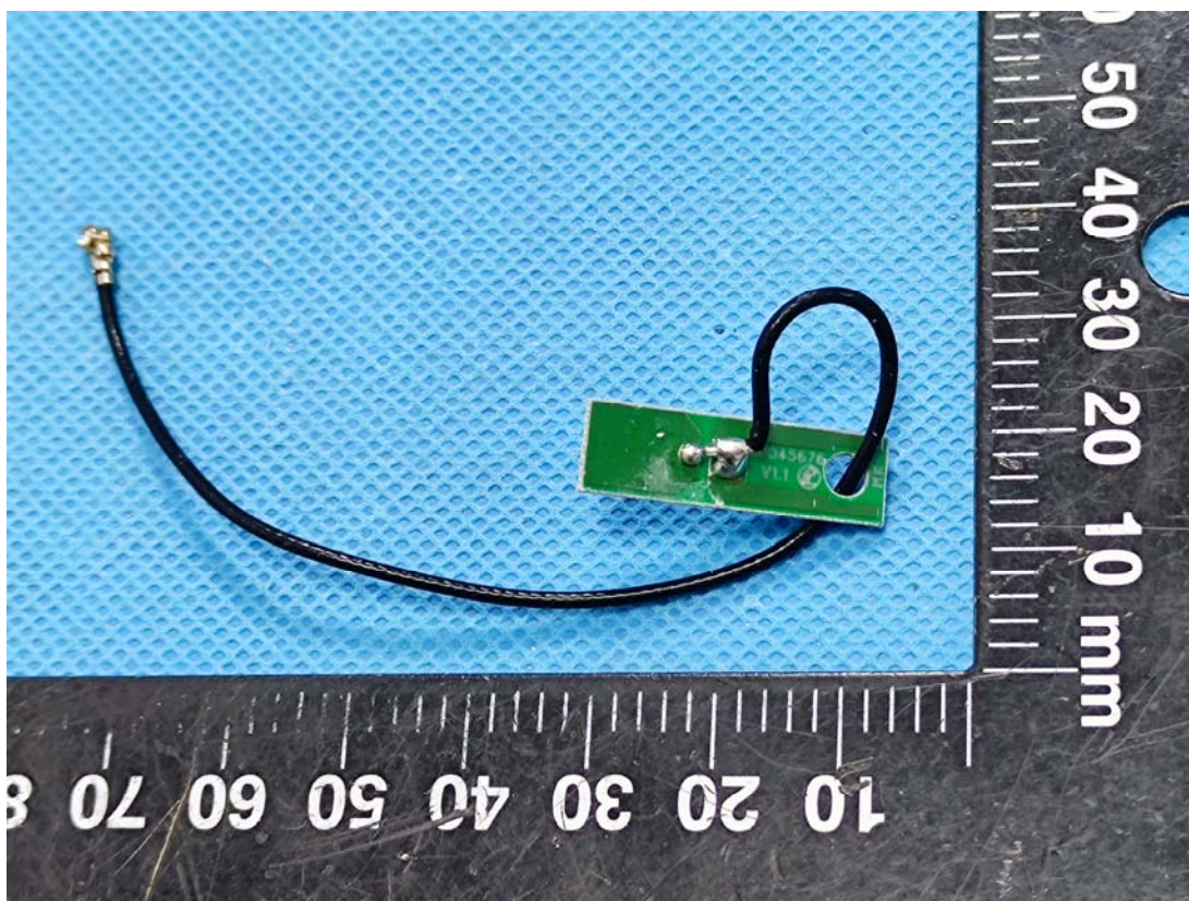
5G Antenna Chain 1
