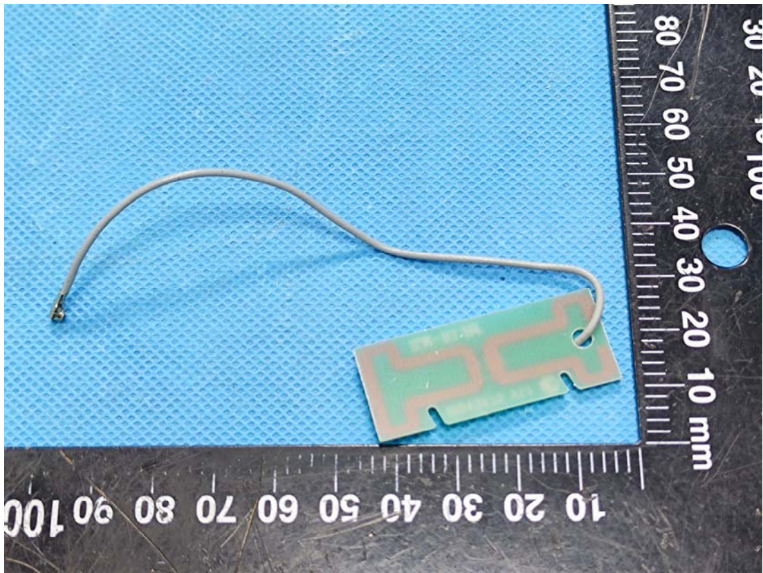
5G Antenna Chain 0
