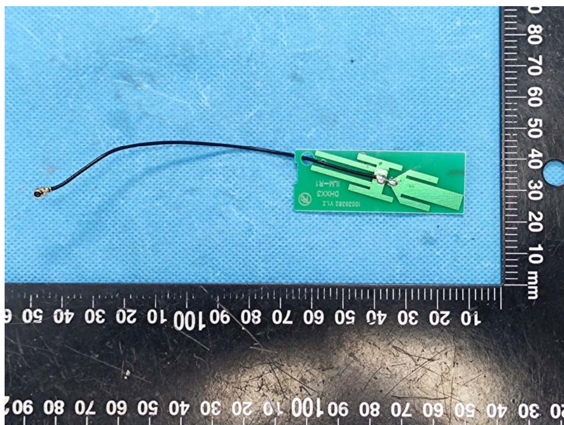
Antenna Chain 1
