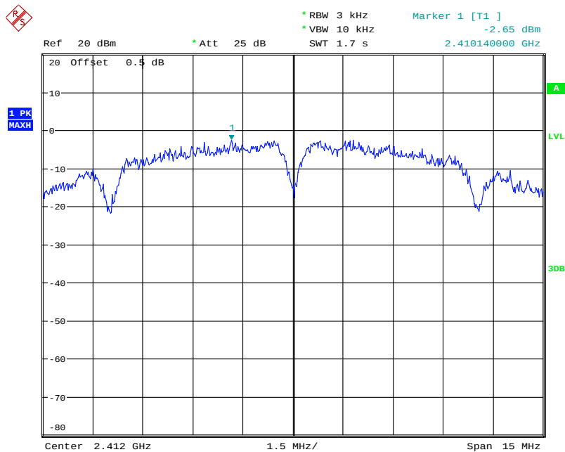
Chain 0, Power Spectral Density, 802.11b Low Channel
