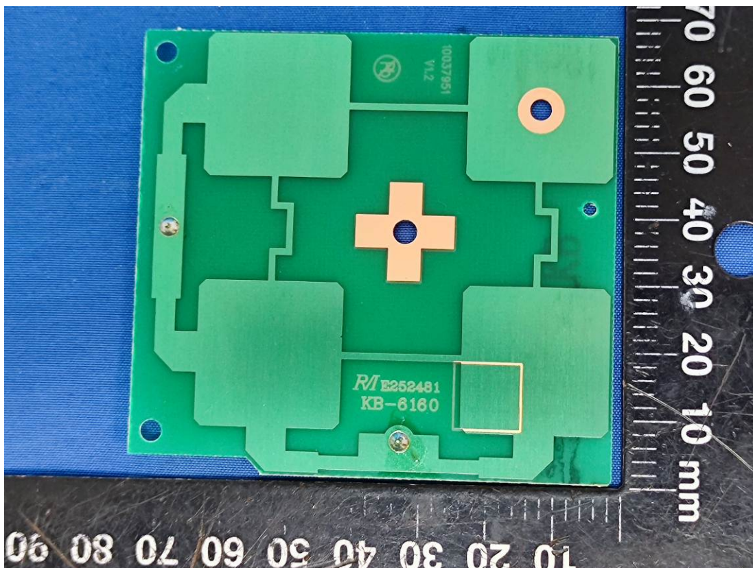
5G Antenna Board
