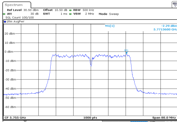
ac40_5755MHz_Chain 0
