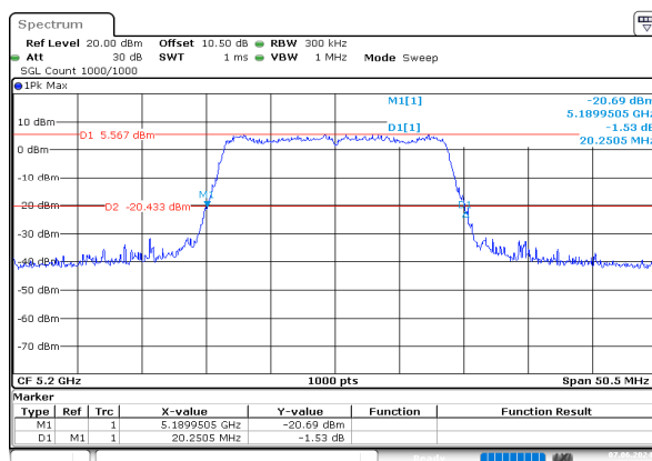
n20_5200MHz_Chain 0
