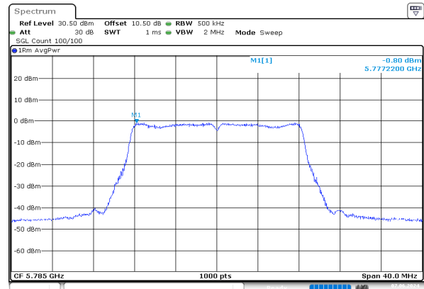
a_5785MHz_Chain 1
