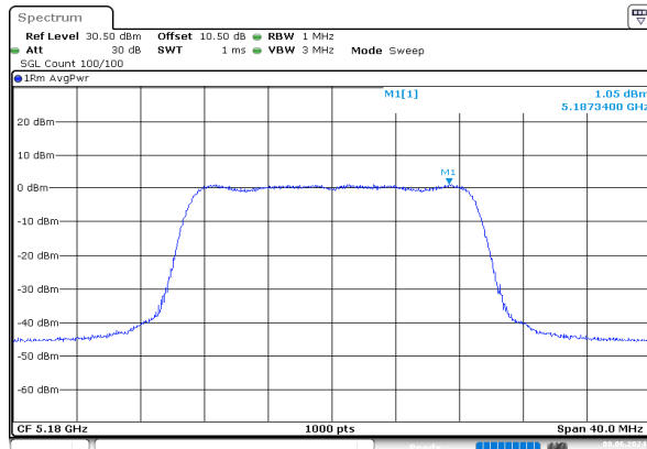
n20_5180MHz_Chain 0
