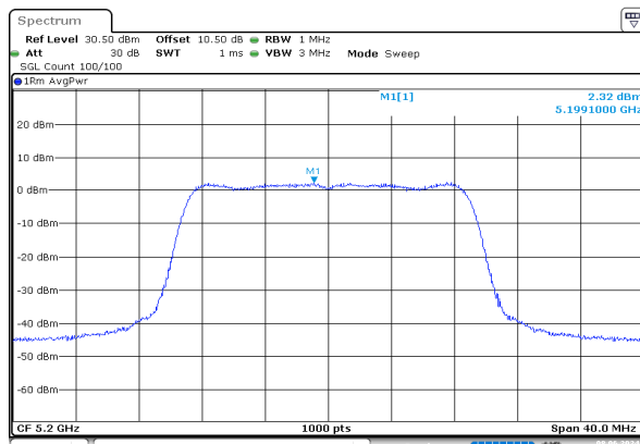
n20_5200MHz_Chain 0
