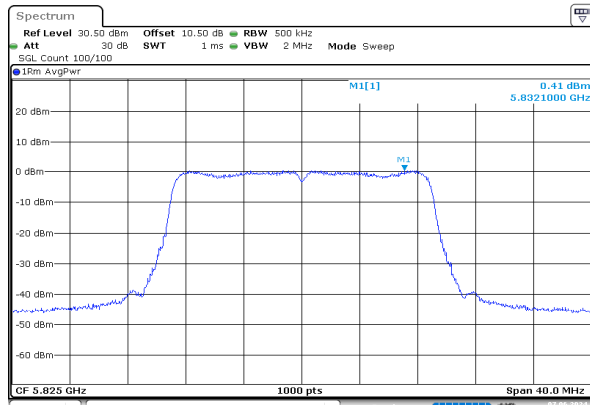
n20_5825MHz_Chain 0
