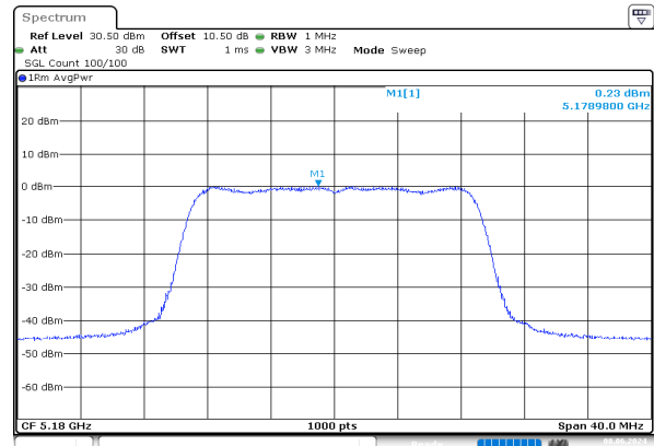
n20_5180MHz_Chain 1
