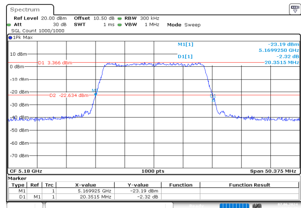
n20_5180MHz_Chain 0
