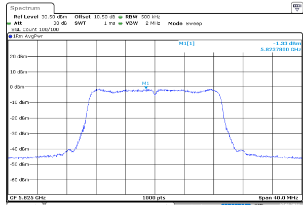
n20_5825MHz_Chain 1
