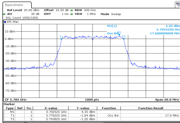
n20_5785MHz_Chain 0
