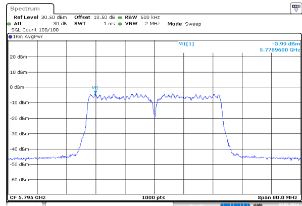
ac40_5795MHz_Chain 1
