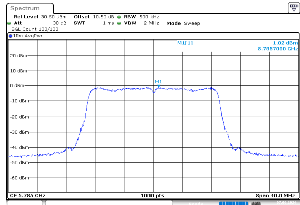
n20_5785MHz_Chain 1
