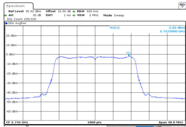
n20_5745MHz_Chain 1
