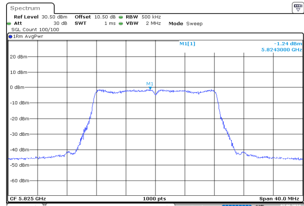
a_5825MHz_Chain 1
