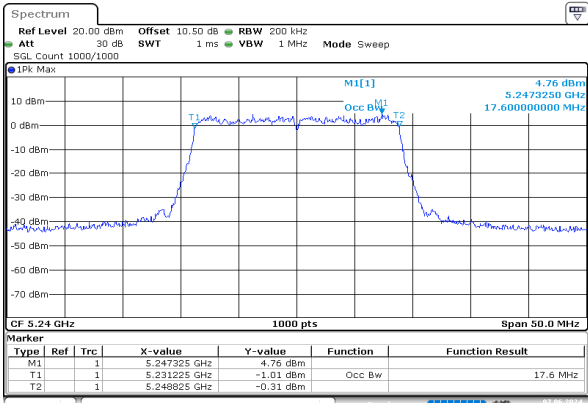
ac20_5240MHz_Chain 0
