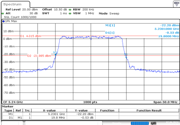
ac20_5240MHz_Chain 0
