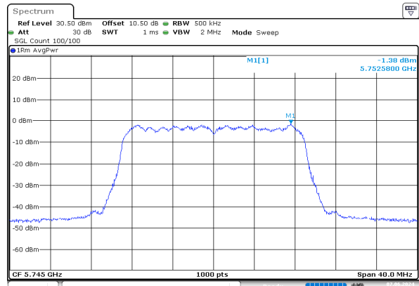
ac20_5745MHz_Chain 1
