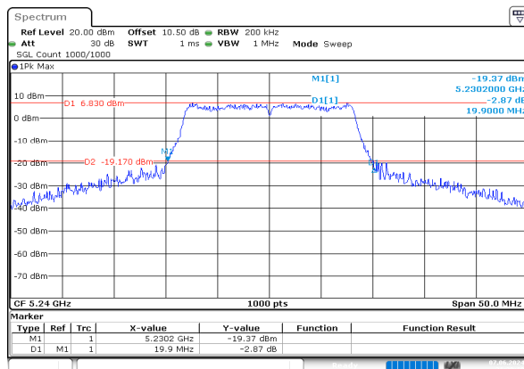
a_5240MHz_Chain 0
