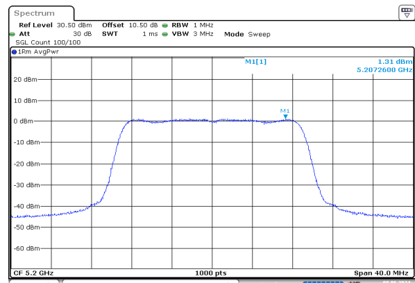
n20_5200MHz_Chain 1
