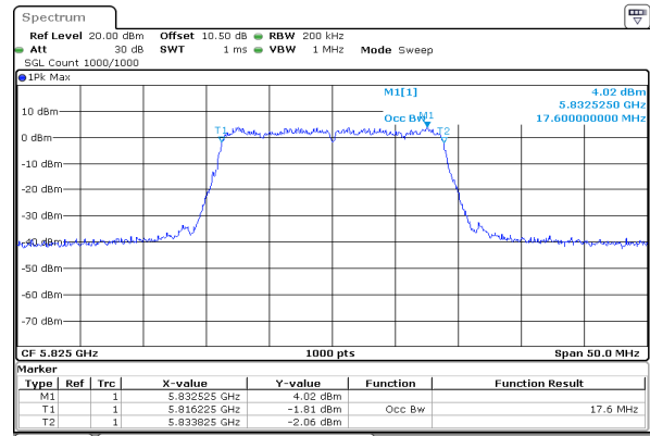
n20_5825MHz_Chain 0
