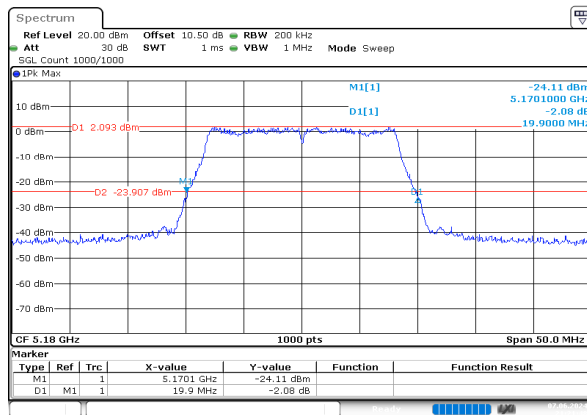
a_5180MHz_Chain 0
