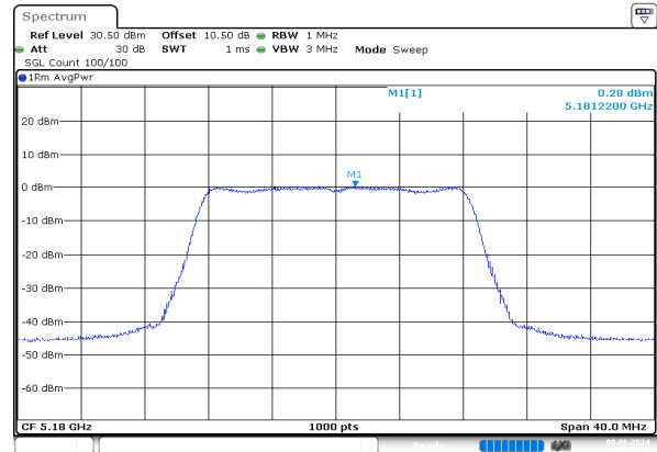
a_5180MHz_Chain 1
