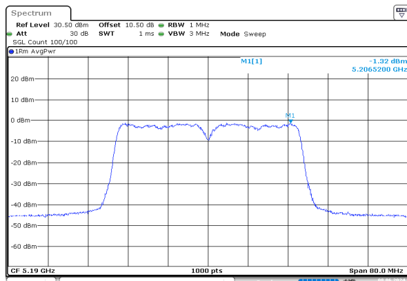
ac40_5190MHz_Chain 0
