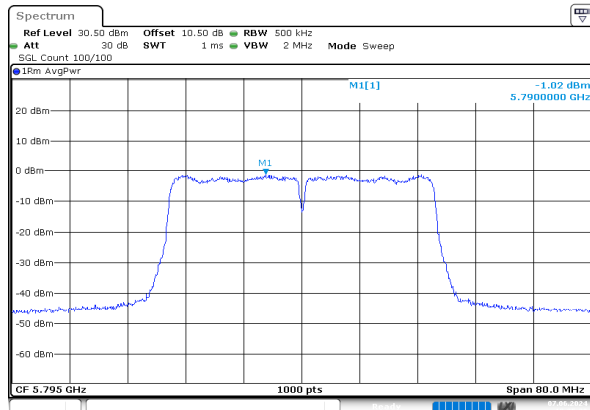
n40_5795MHz_Chain 0
