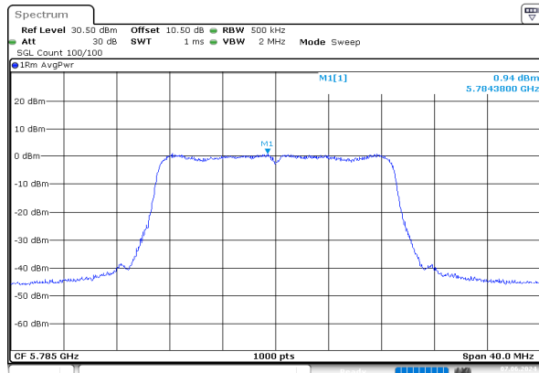
n20_5785MHz_Chain 0
