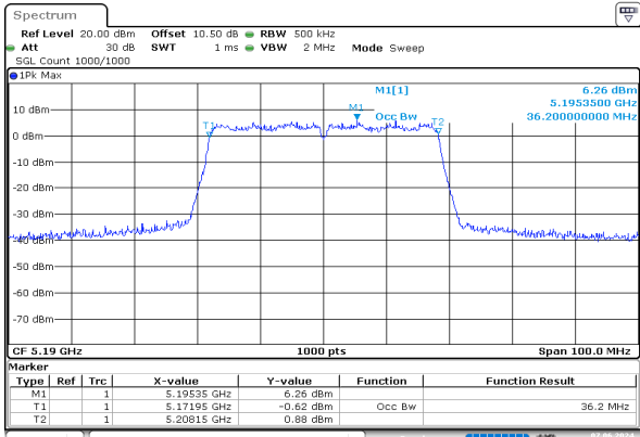
ac40_5190MHz_Chain 0
