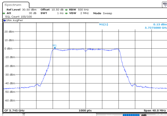
a_5745MHz_Chain 0
