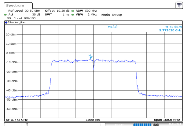
ac80_5775MHz_Chain 1
