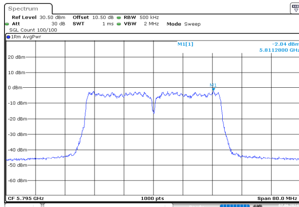
ac40_5795MHz_Chain 0
