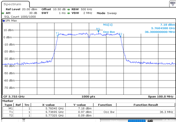
ac40_5755MHz_Chain 0
