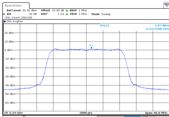
ac20_5240MHz_Chain 0
