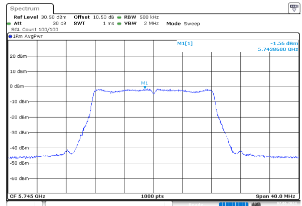
a_5745MHz_Chain 1
