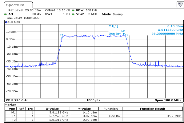
n40_5795MHz_Chain 0
