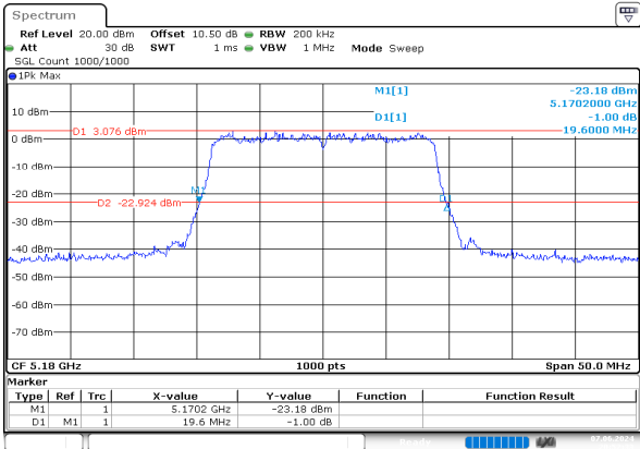
ac20_5180MHz_Chain 0
