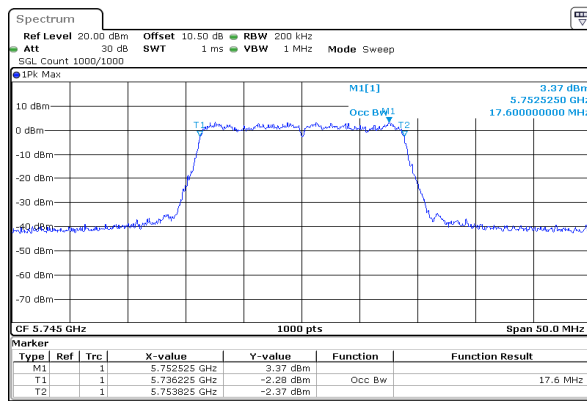
ac20_5745MHz_Chain 0
