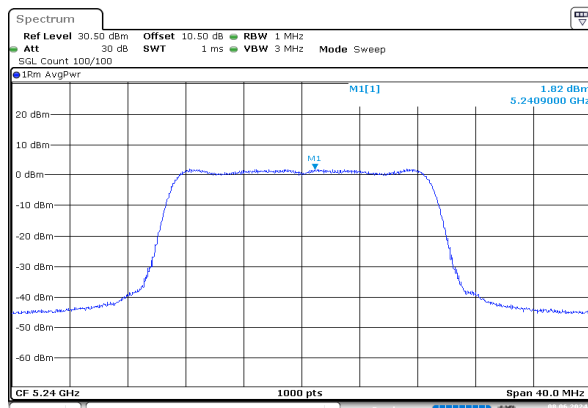
n20_5240MHz_Chain 0
