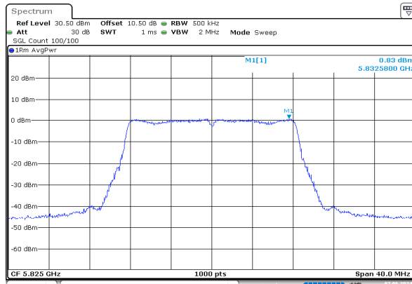
a_5825MHz_Chain 0
