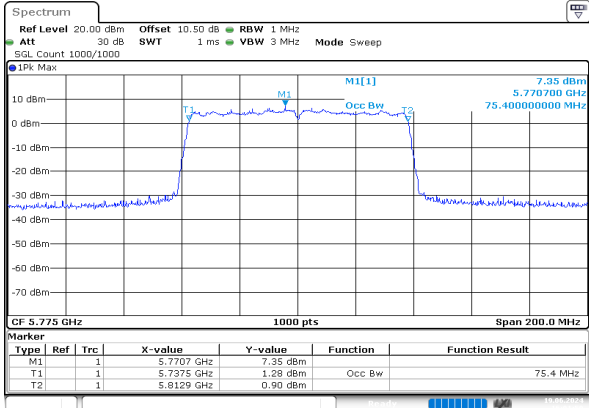
ac80_5775MHz_Chain 0
