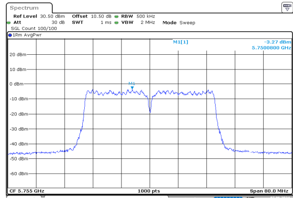
ac40_5755MHz_Chain 1
