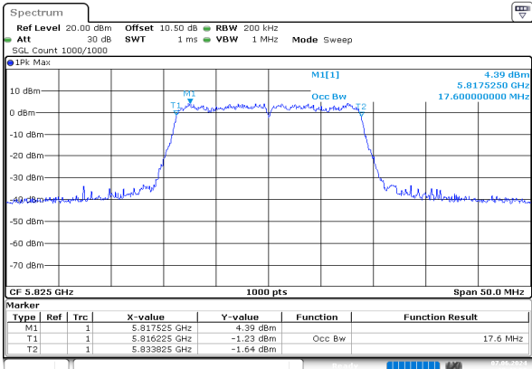
ac20_5825MHz_Chain 0
