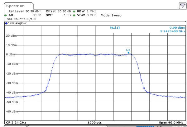
ac20_5240MHz_Chain 1
