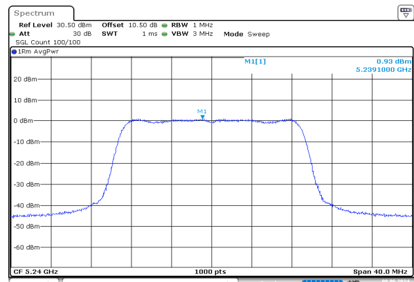
n20_5240MHz_Chain 1
