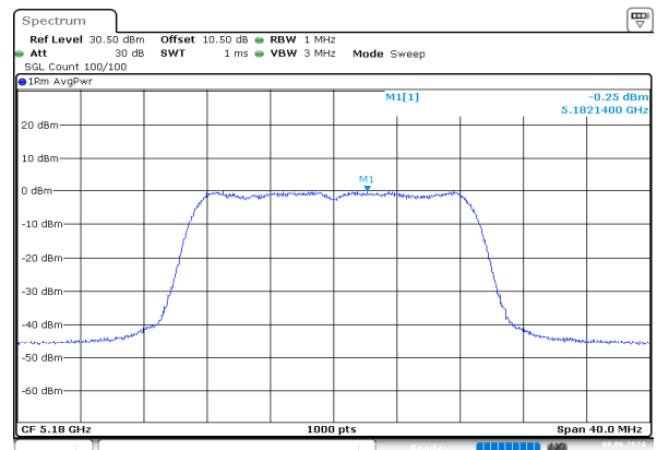
ac20_5180MHz_Chain 1
