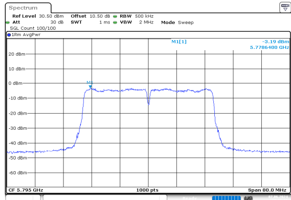
n40_5795MHz_Chain 1
