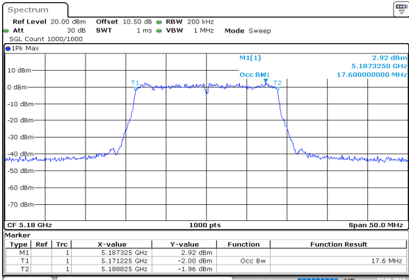
ac20_5180MHz_Chain 0
