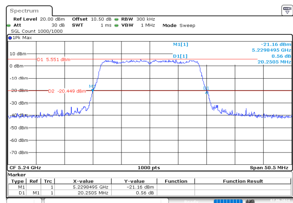
n20_5240MHz_Chain 0
