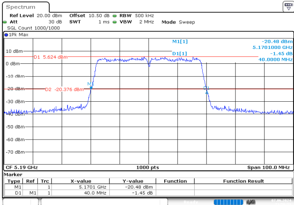
ac40_5190MHz_Chain 0
