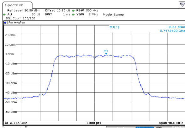
ac20_5745MHz_Chain 0
