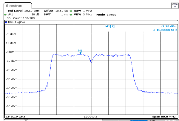
ac40_5190MHz_Chain 1
