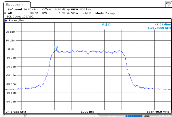
ac20_5825MHz_Chain 1
