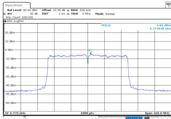
ac80_5775MHz_Chain 0
