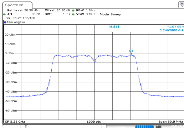
ac40_5230MHz_Chain 0
