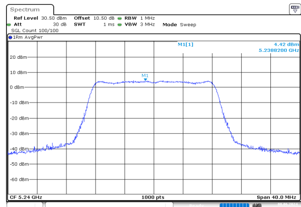
a_5240MHz_Chain 1
