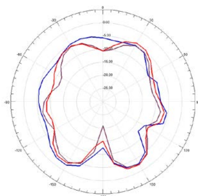
2D Radiation patterns
