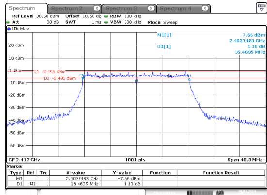
g_2412MHz_Chain 0
