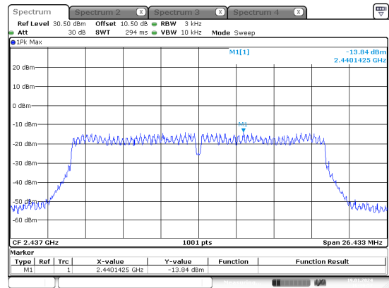
n20_2437MHz_Chain 0
