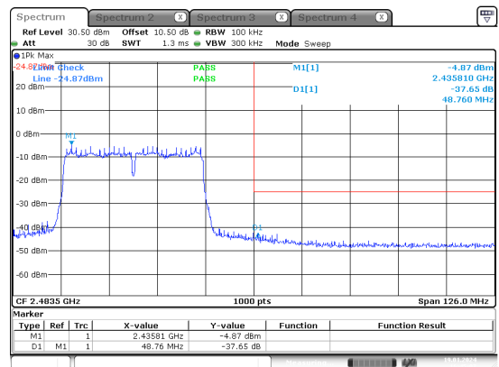
n40_2452MHz_Chain 0
