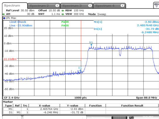
n40_2422MHz_Chain 0
