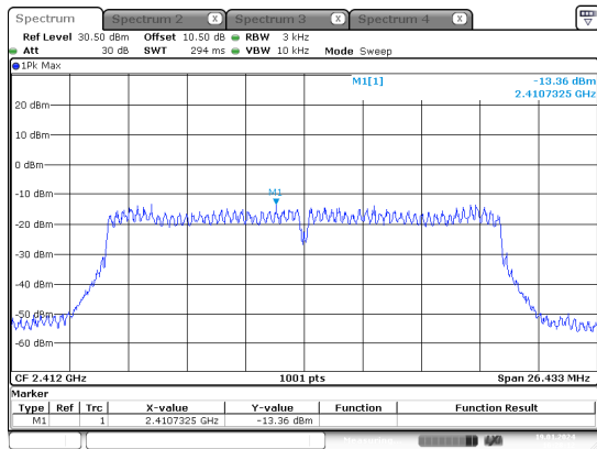
n20_2412MHz_Chain 0
