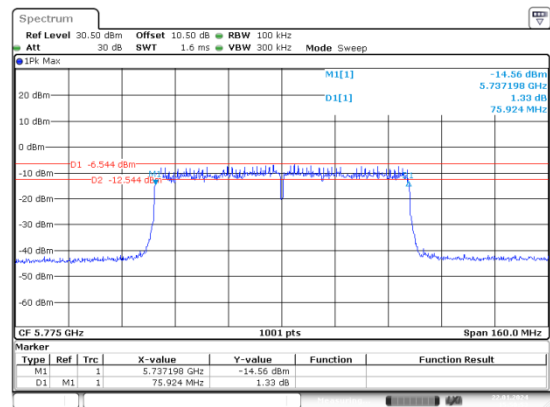
ac80_5775MHz_Chain 0
