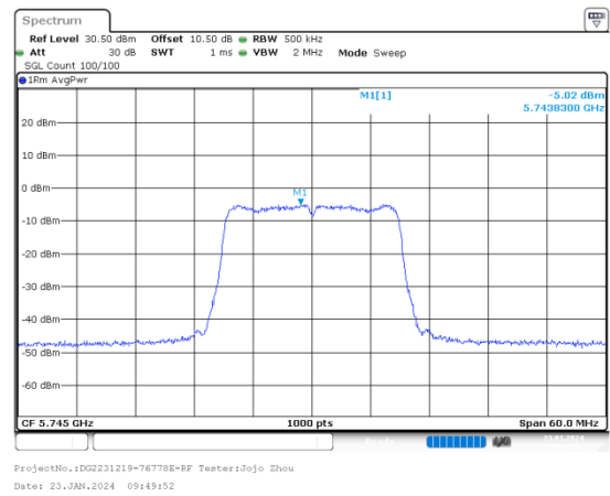
n20_5745MHz_Chain 1
