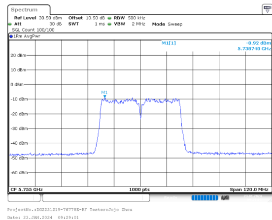
ac40_5755MHz_Chain 0
