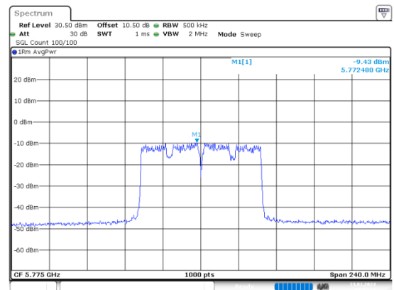
ac80_5775MHz_Chain 1
