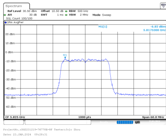
ac20_5825MHz_Chain 0
