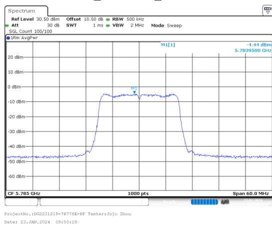
n20_5785MHz_Chain 1
