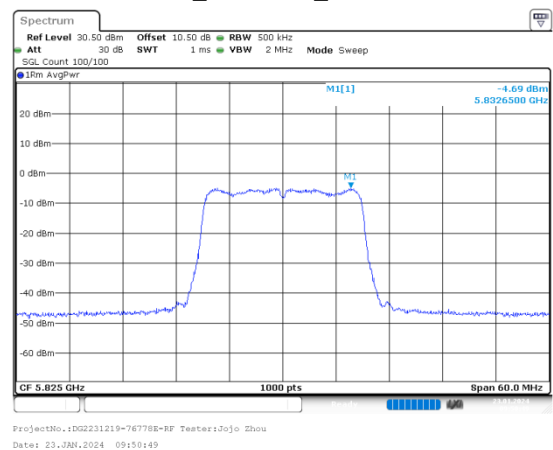
n20_5825MHz_Chain 1
