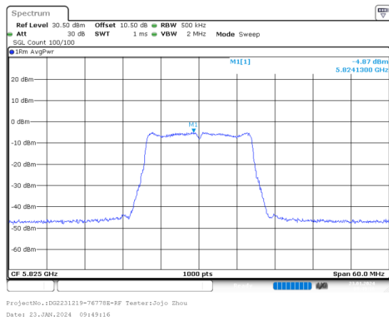
a_5825MHz_Chain 1
