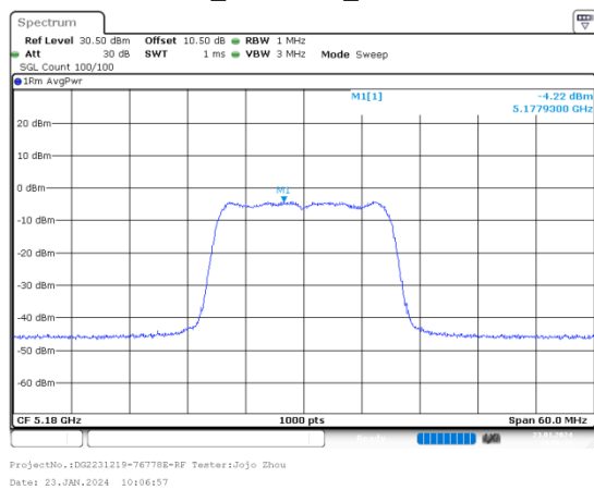
ac20_5180MHz_Chain 1
