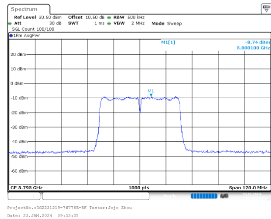
n40_5795MHz_Chain 0
