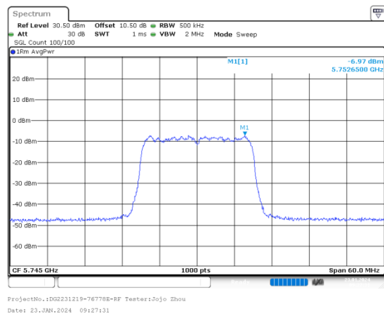
ac20_5745MHz_Chain 0
