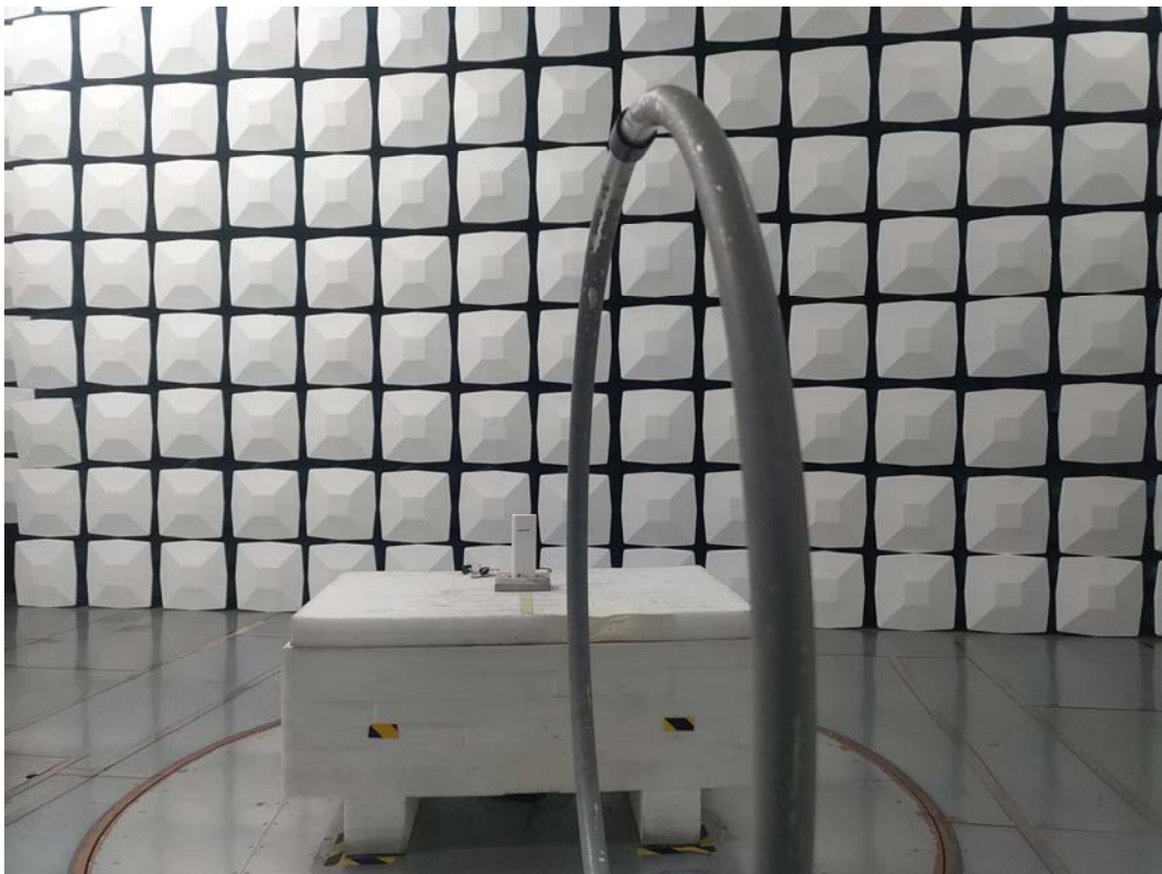
Radiated Emission 9k-30MHz Perpendicular front View –PoE Adapter
