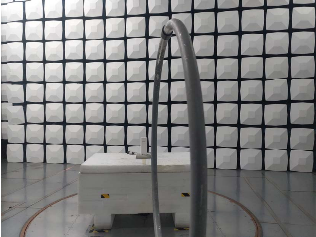
Radiated Emission 9k-30MHz Parallel front View-AC/DC Adapter
