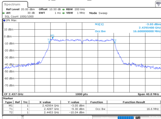
g_2437MHz_Chain 0
