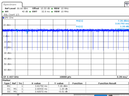
n20_2437MHz_Chain 0
