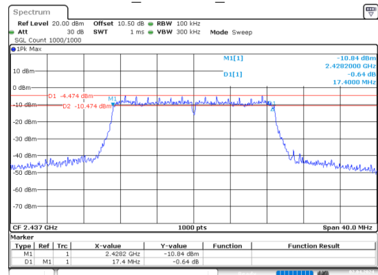
n20_2437MHz_Chain 0
