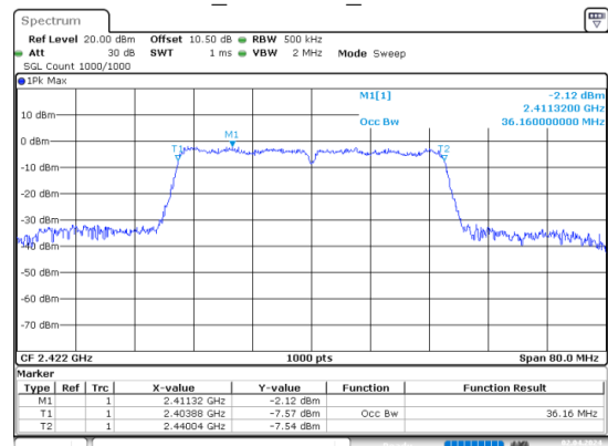
n40_2422MHz_Chain 0
