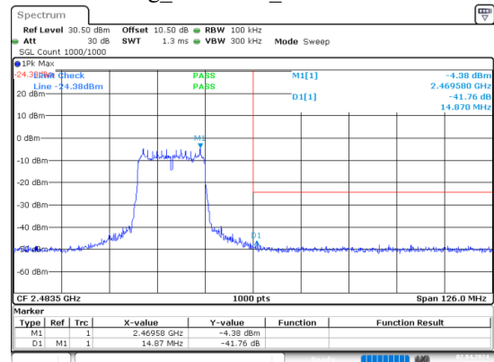
g_2462MHz_Chain 0
