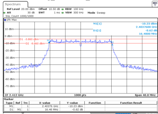
g_2412MHz_Chain 0
