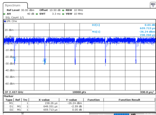
n40_2437MHz_Chain 0
