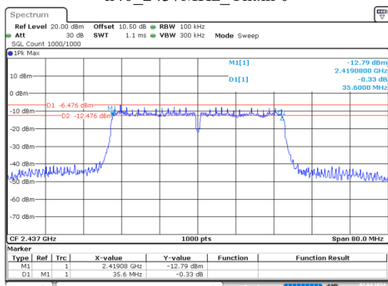
n40_2437MHz_Chain 0
