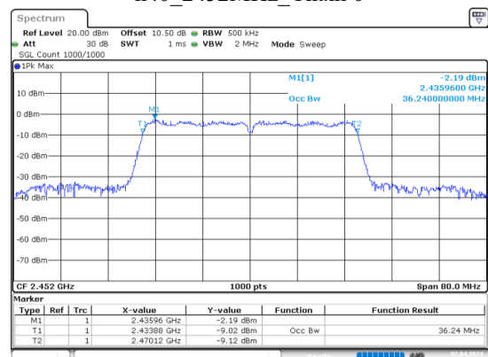
n40_2452MHz_Chain 0
