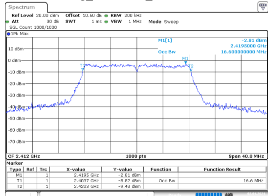
g_2412MHz_Chain 0
