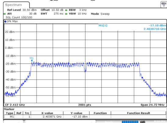
g_2412MHz_Chain 0
