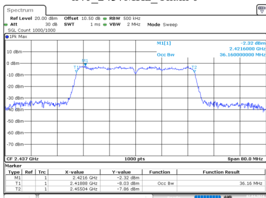
n40_2437MHz_Chain 0
