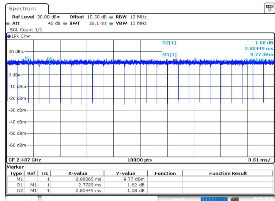
g_2437MHz_Chain 0
