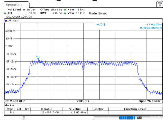
n20_2437MHz_Chain 0
