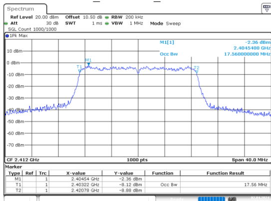
n20_2412MHz_Chain 0
