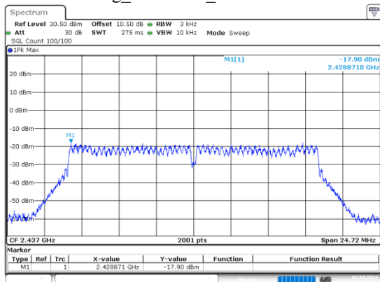
g_2437MHz_Chain 0
