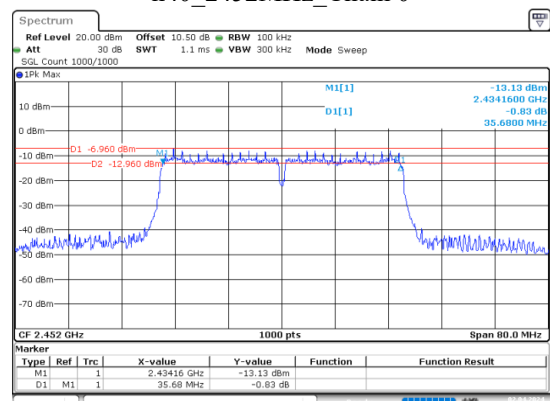
n40_2452MHz_Chain 0
