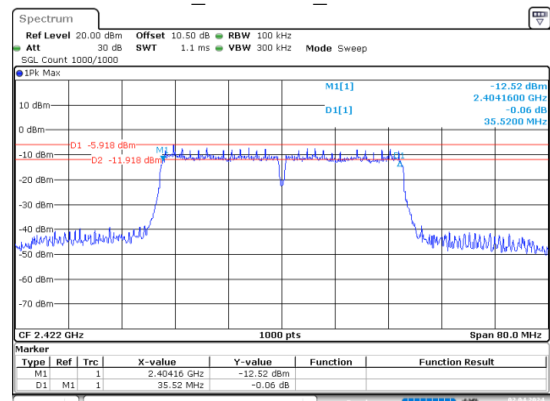
n40_2422MHz_Chain 0
