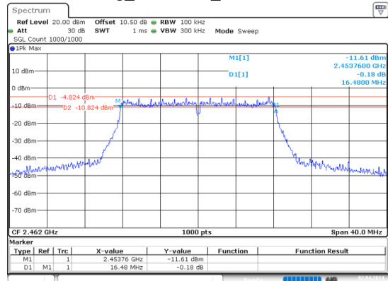
g_2462MHz_Chain 0
