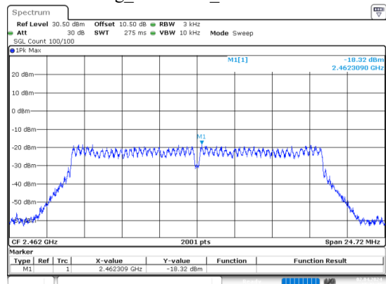
g_2462MHz_Chain 0
