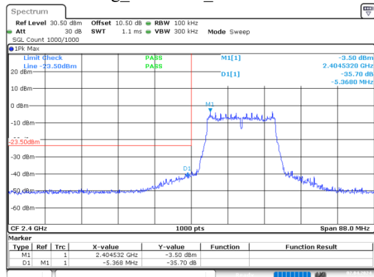
g_2412MHz_Chain 0
