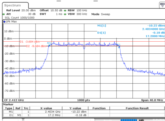
n20_2412MHz_Chain 0
